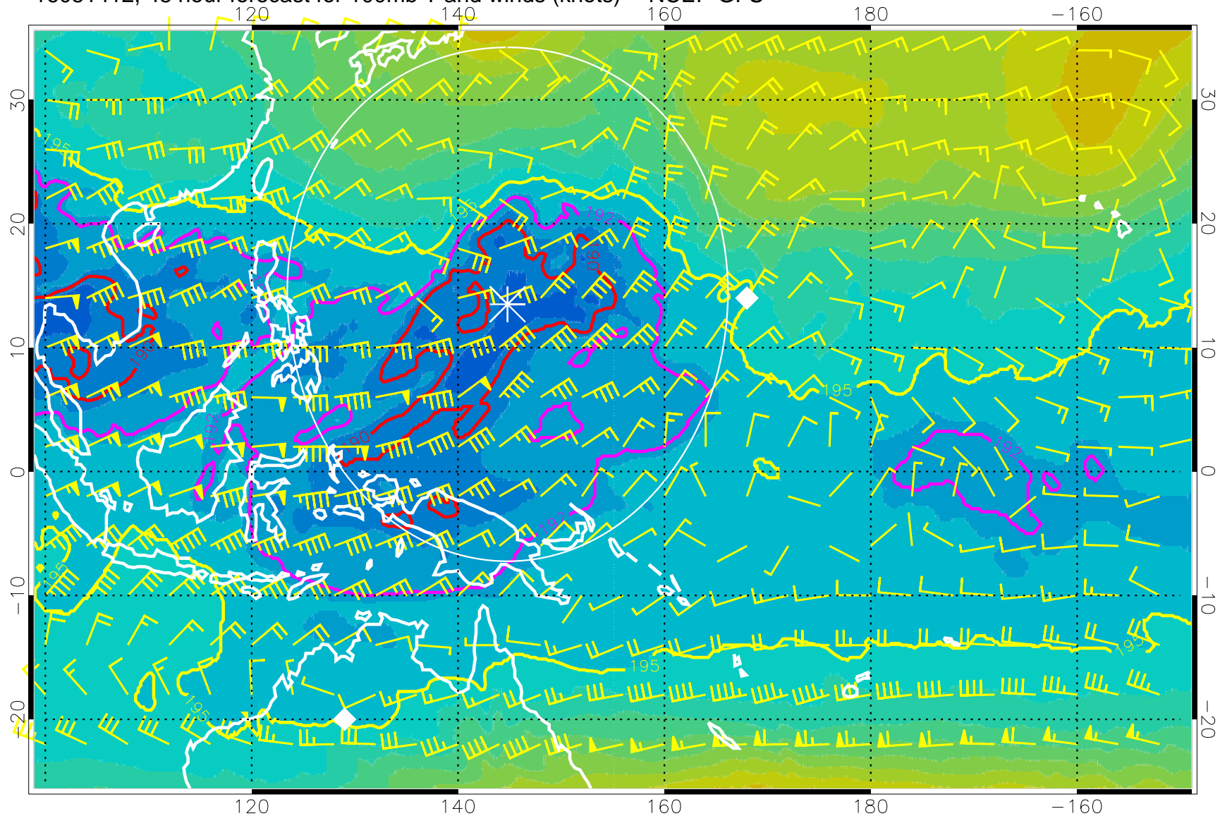
16081412, 48 hour forecast for 100mb T and winds (knots) -- NCEP GFS
