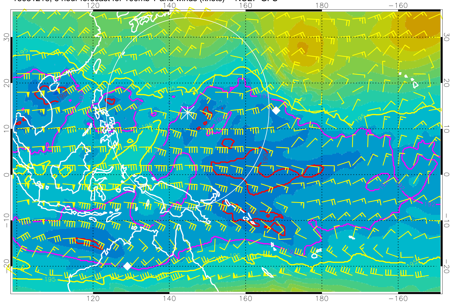
16081218, 6 hour forecast for 100mb T and winds (knots) -- NCEP GFS
