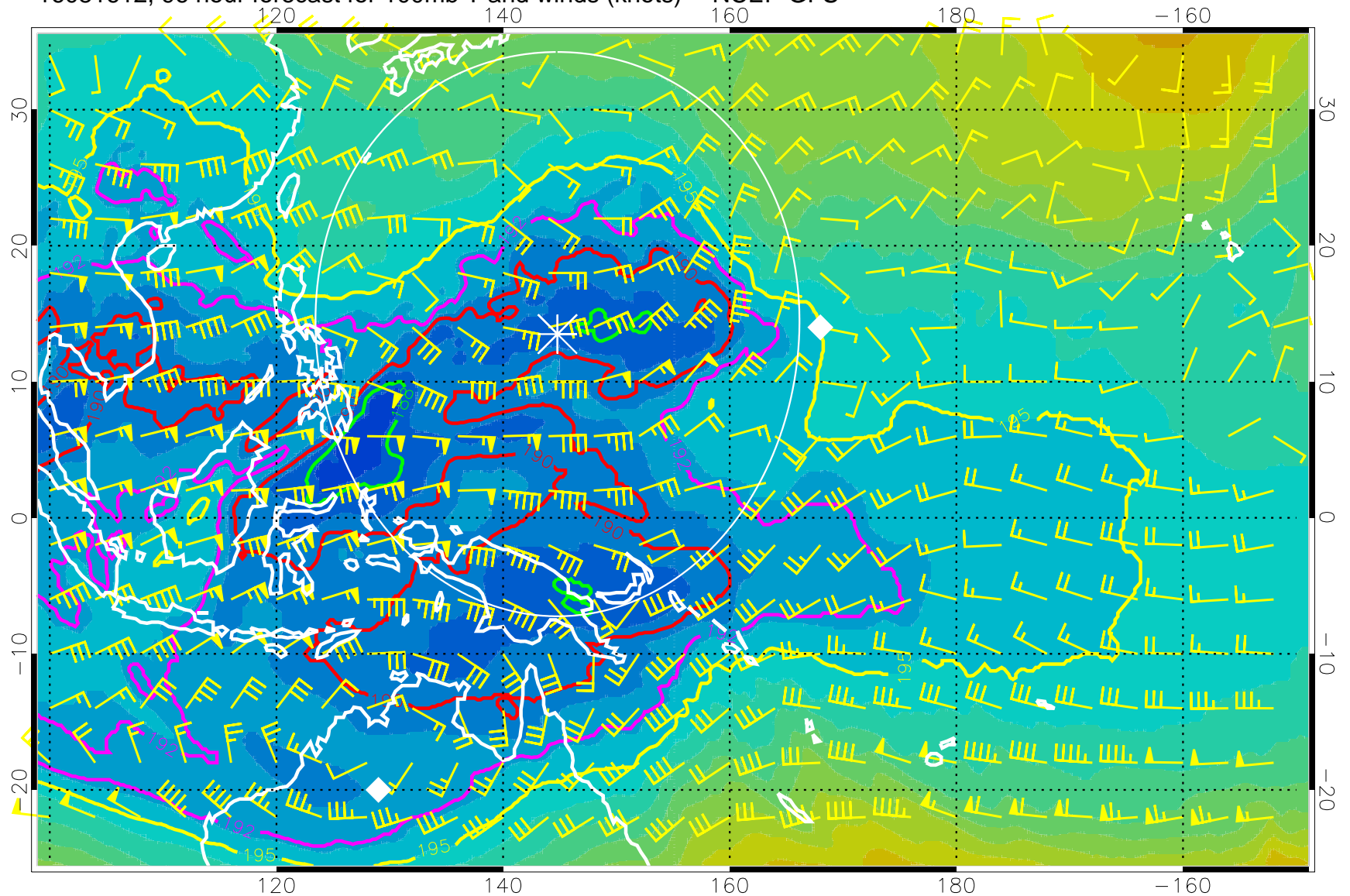
16081612, 96 hour forecast for 100mb T and winds (knots) -- NCEP GFS
