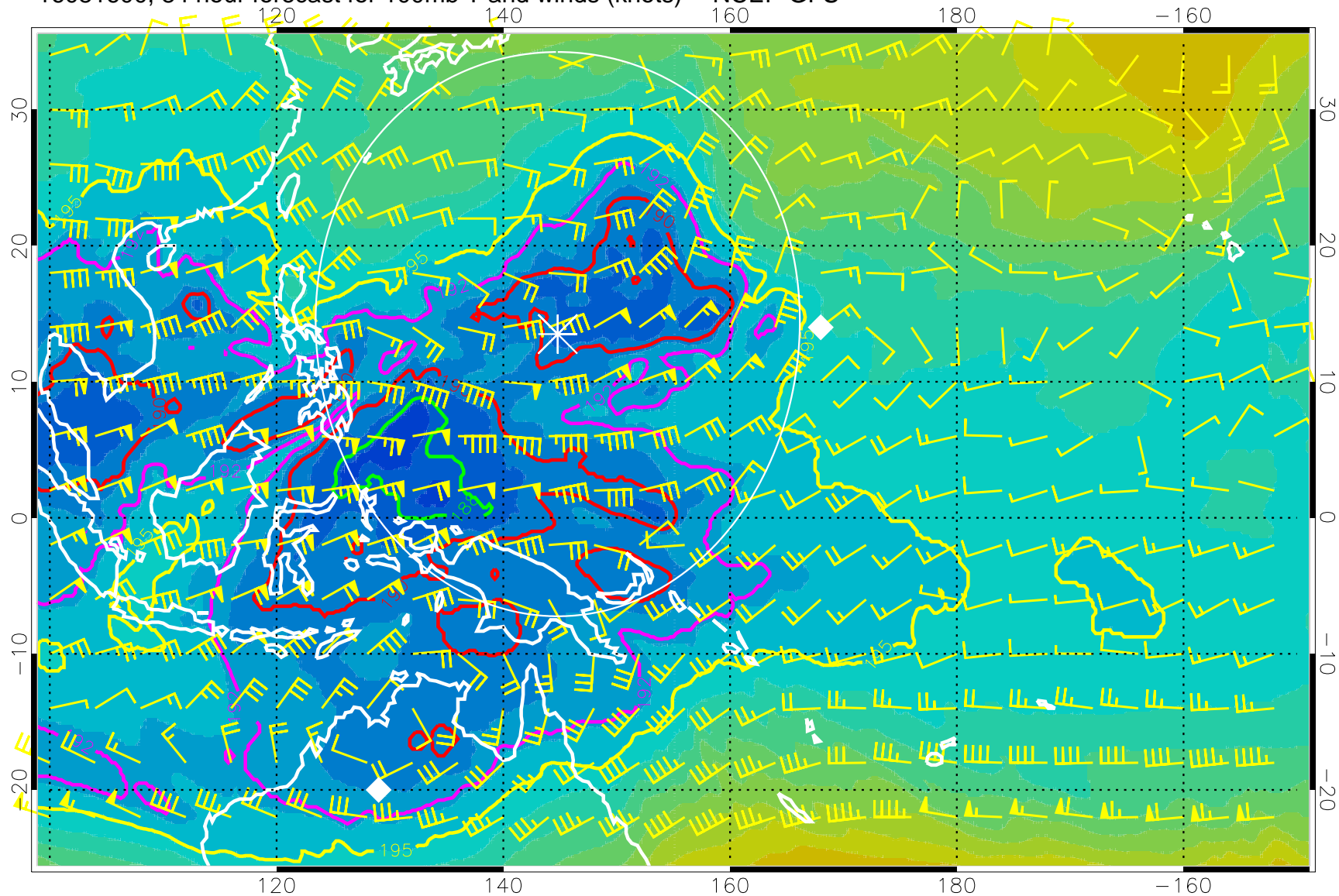
16081600, 84 hour forecast for 100mb T and winds (knots) -- NCEP GFS
