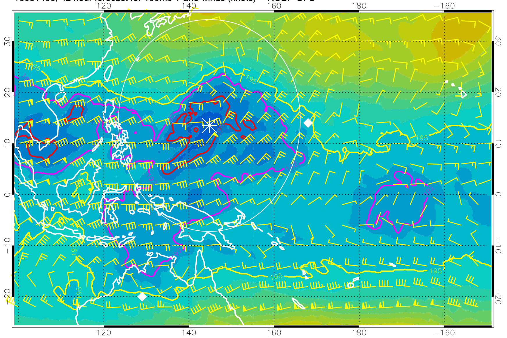
16081406, 42 hour forecast for 100mb T and winds (knots) -- NCEP GFS
