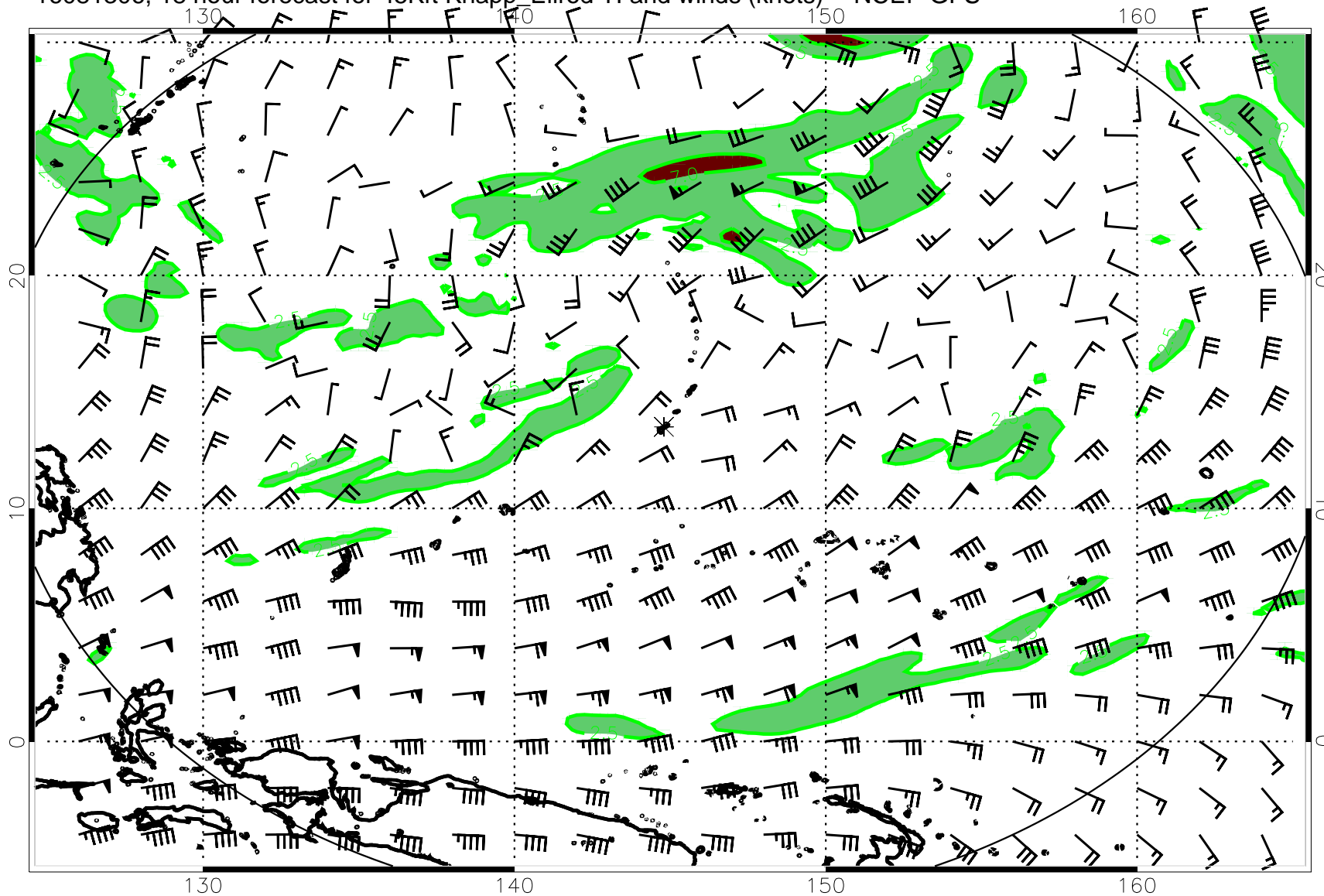
16081306, 18 hour forecast for 45Kft Knapp Ellrod TI and winds (knots) -- NCEP GFS
