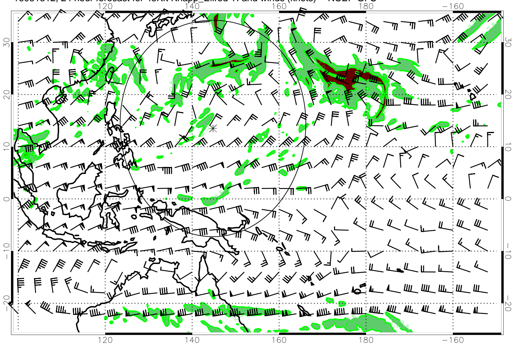
16081312, 24 hour forecast for 45Kft Knapp_Ellrod TI and winds (knots) -- NCEP GFS
