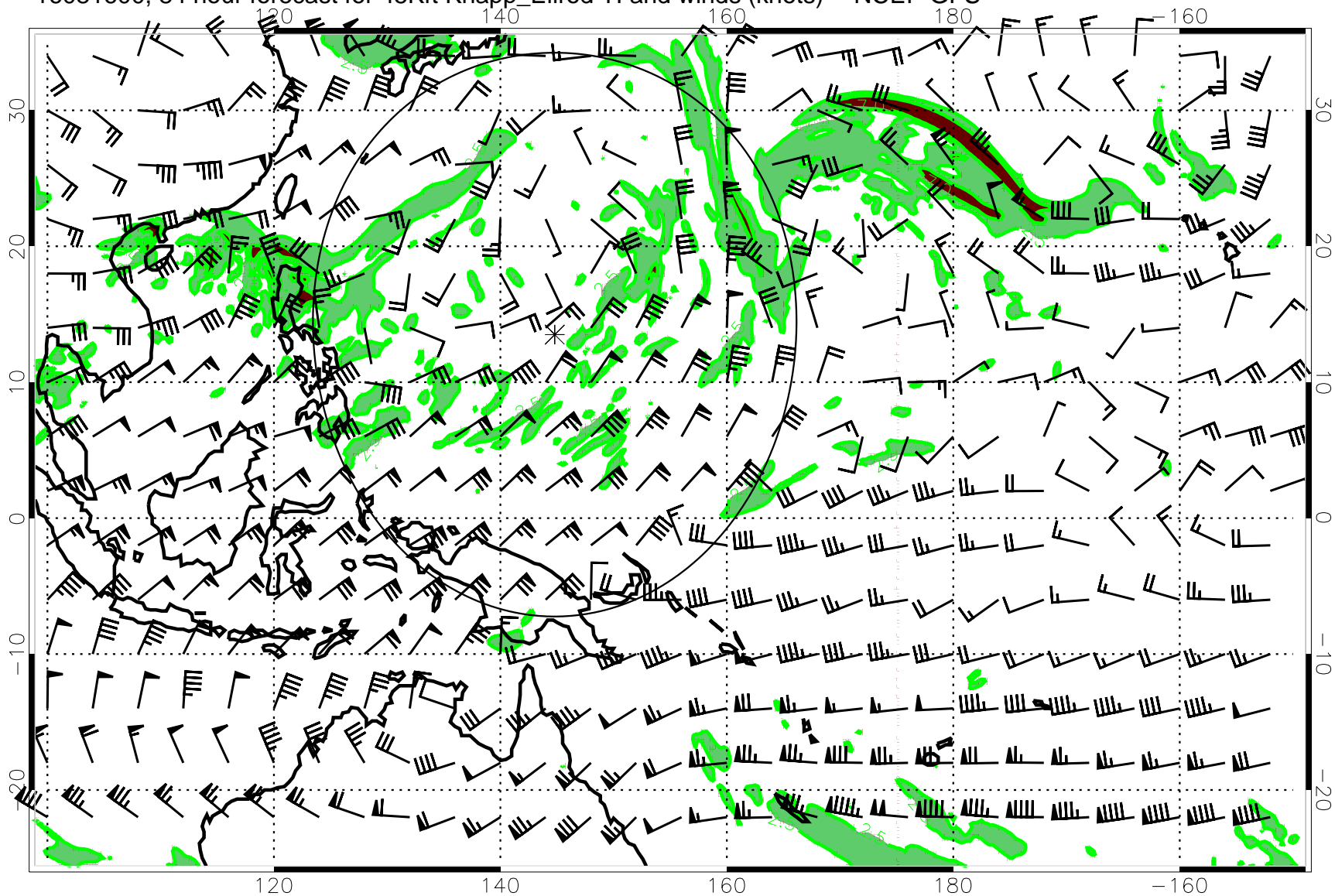
16081600, 84 hour forecast for 45Kft Knapp_Ellrod TI and winds (knots) -- NCEP GFS
