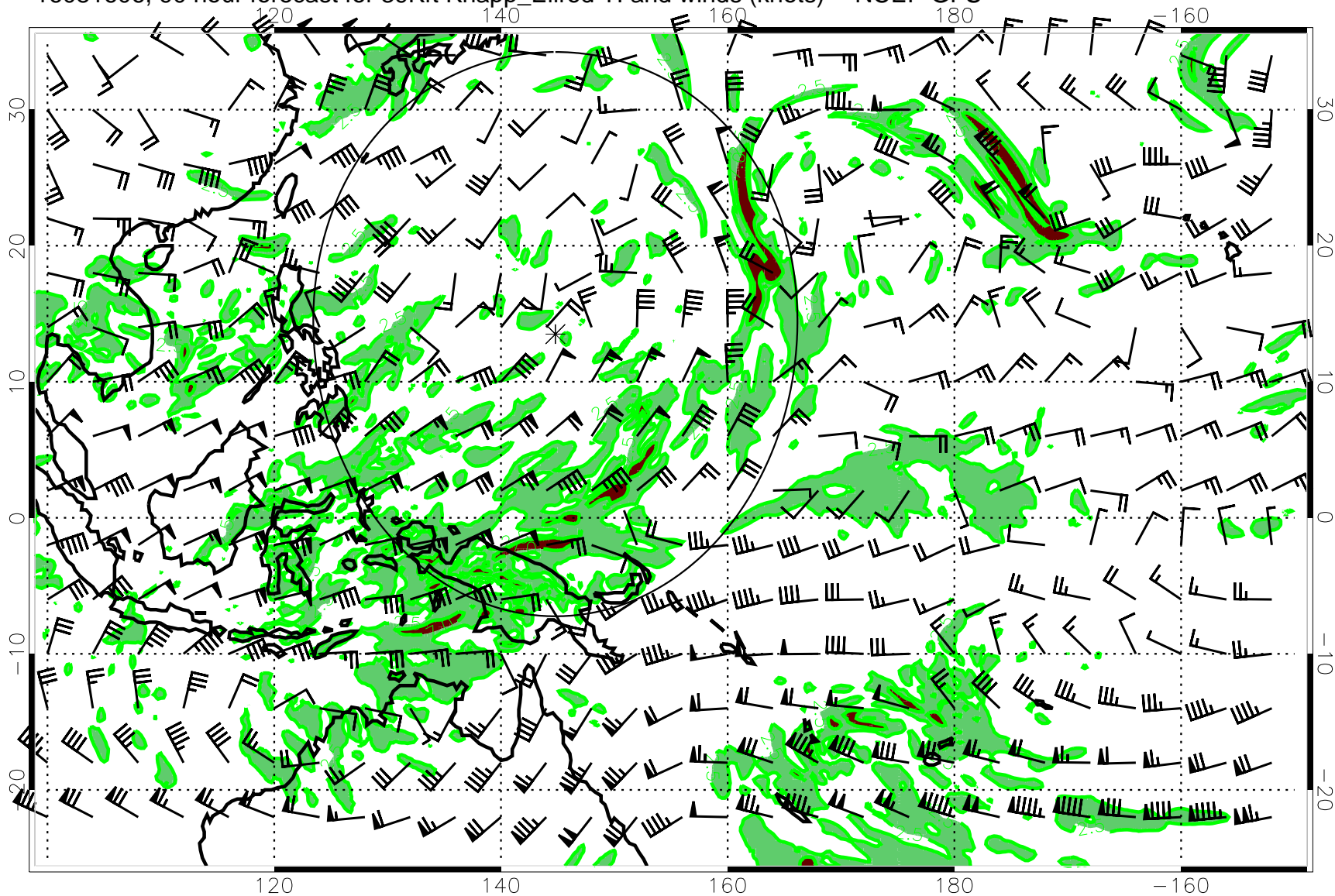
16081606, 90 hour forecast for 39Kft Knapp_Ellrod TI and winds (knots) -- NCEP GFS
