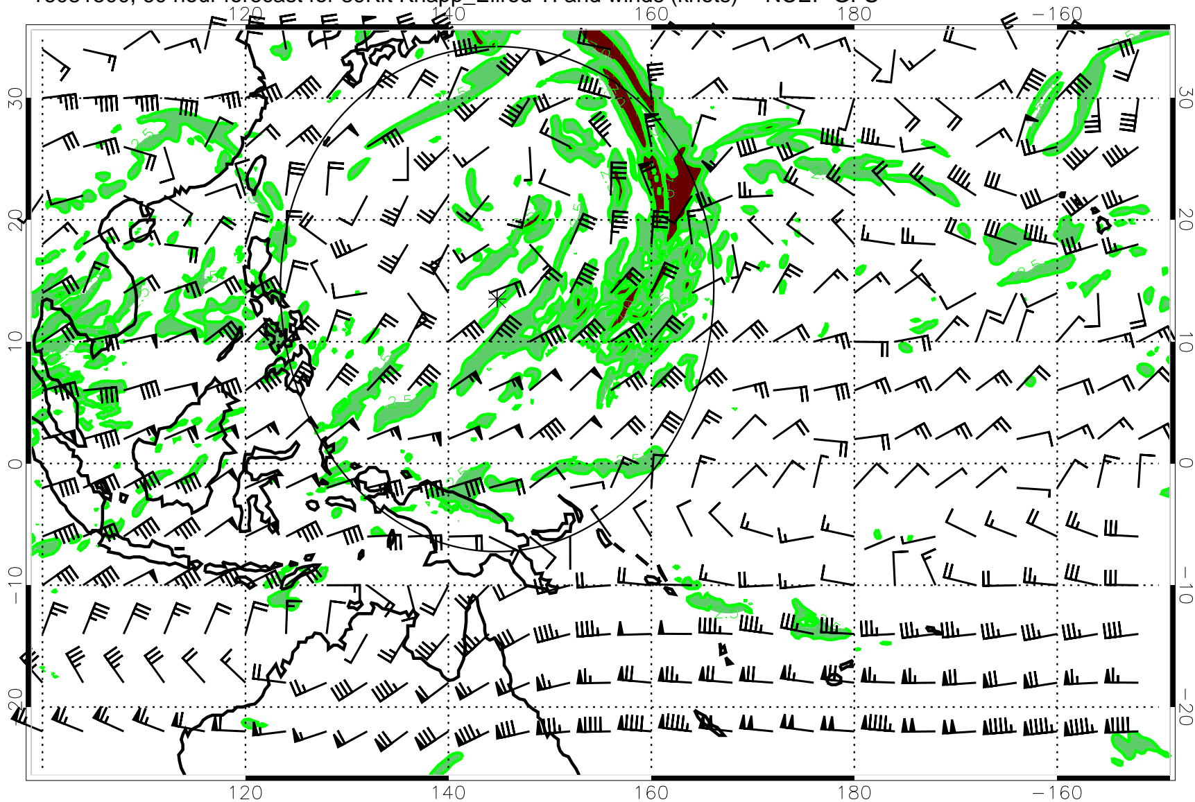
16081500, 60 hour forecast for 39Kft Knapp_Ellrod TI and winds (knots) -- NCEP GFS
