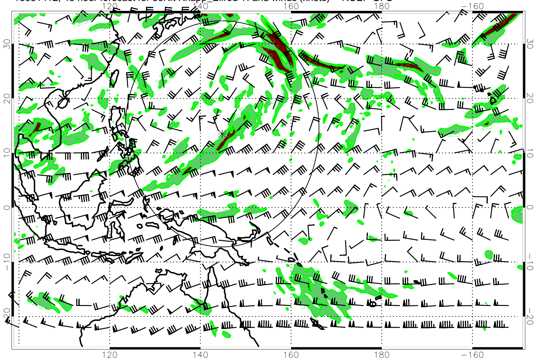
16081412, 48 hour forecast for 36Kft Knapp_Ellrod TI and winds (knots) -- NCEP GFS
