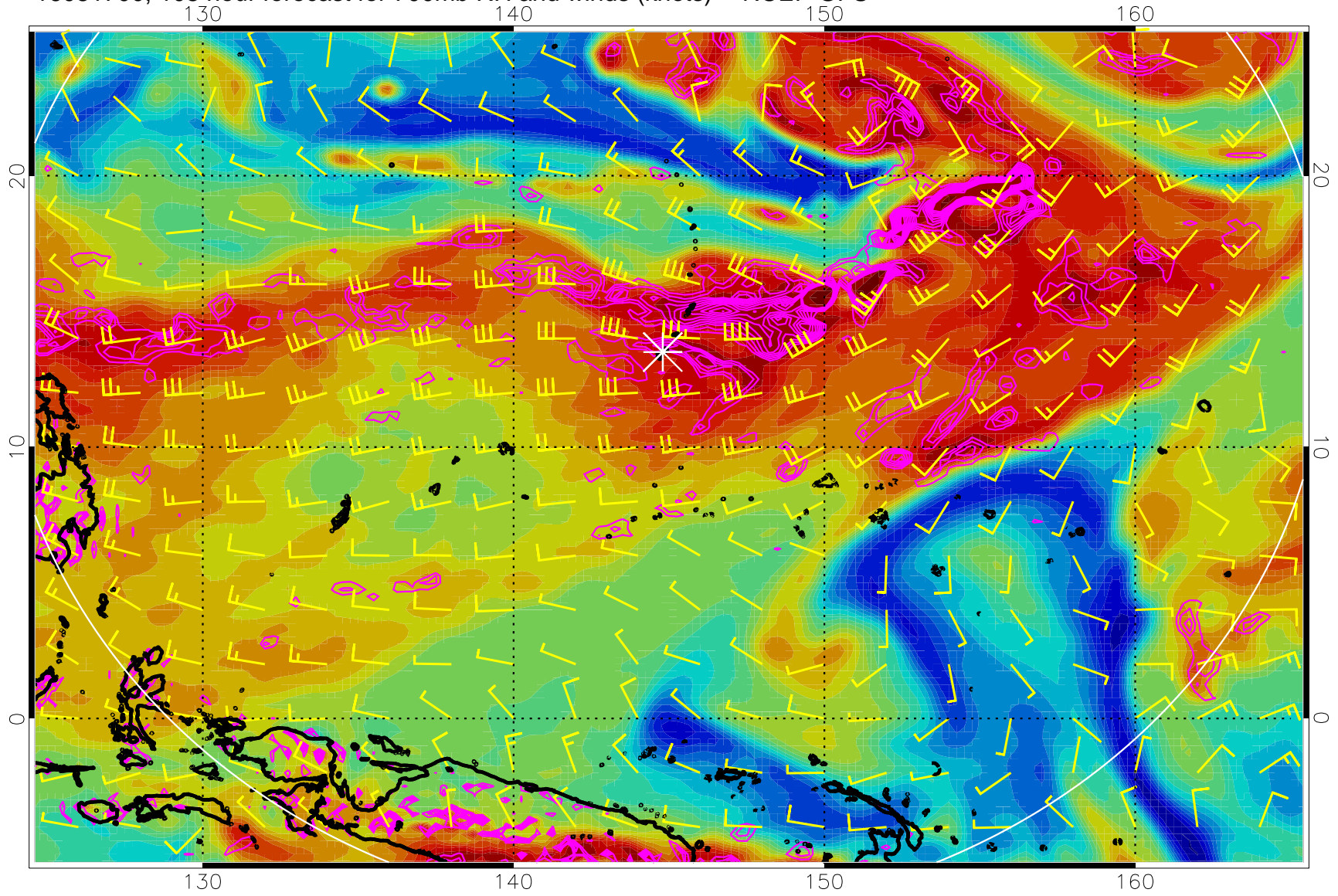
16081700, 108 hour forecast for 700mb RH and winds (knots) -- NCEP GFS
