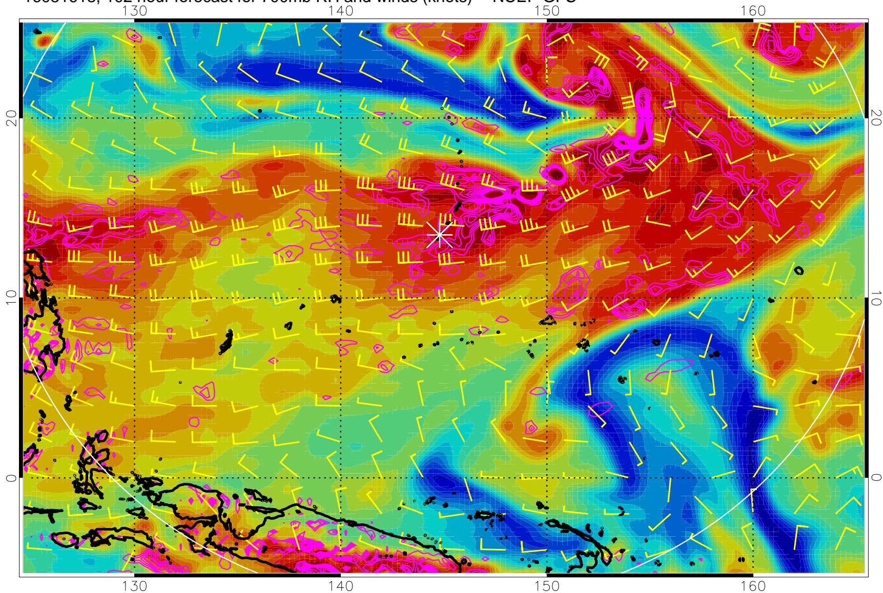
16081618, 102 hour forecast for 700mb RH and winds (knots) -- NCEP GFS
