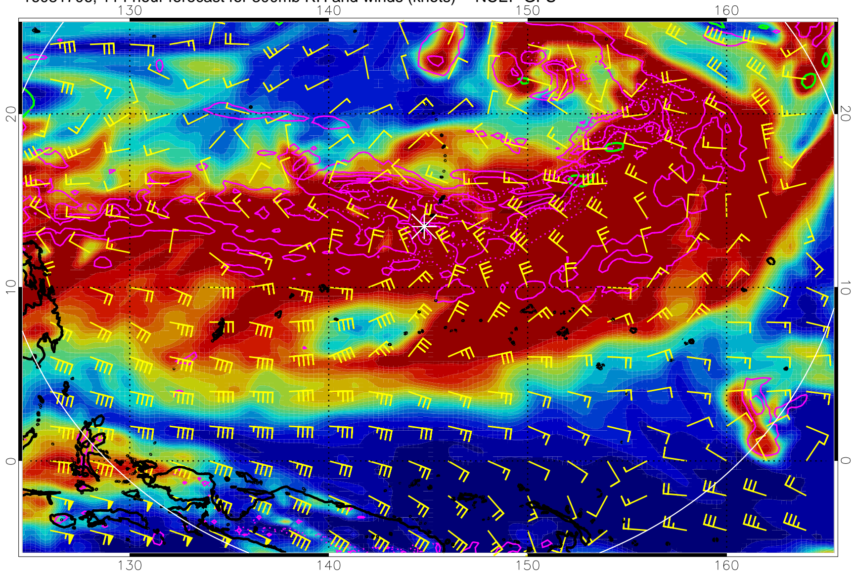
16081706, 114 hour forecast for 300mb RH and winds (knots) -- NCEP GFS
