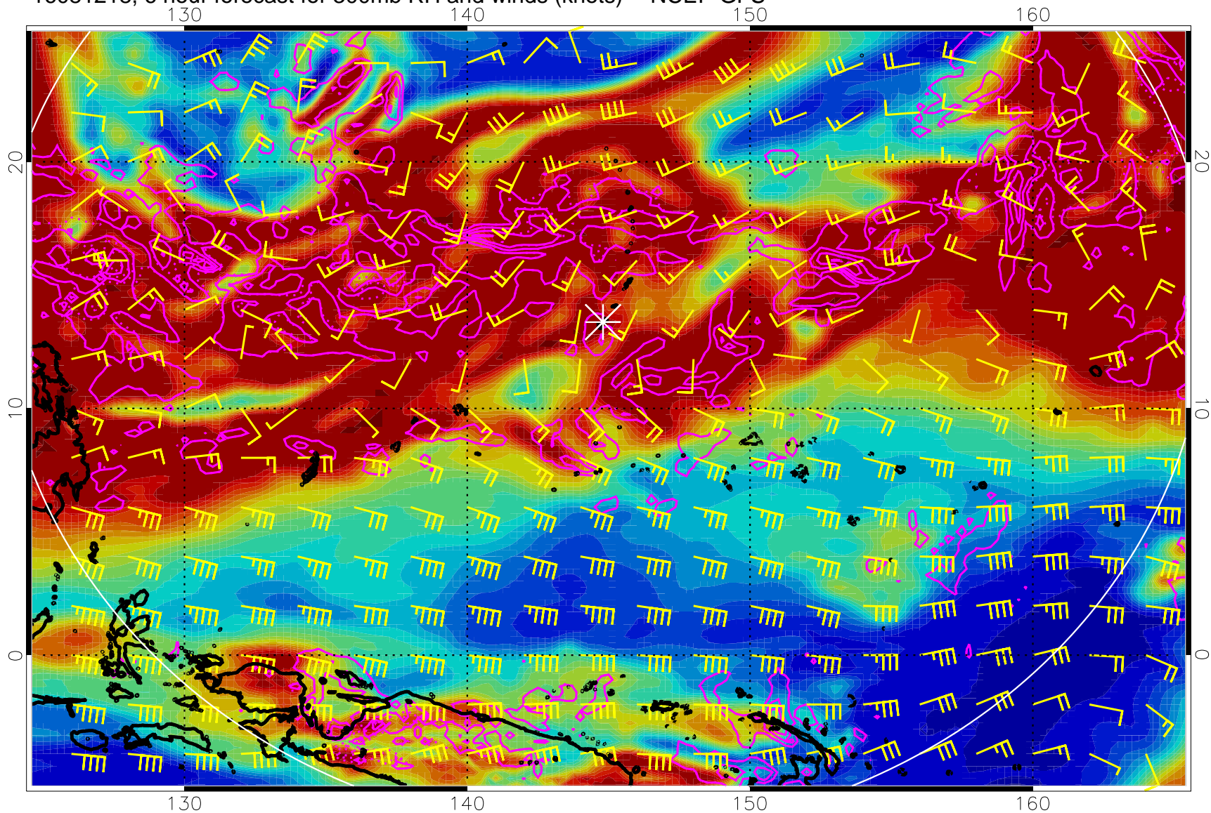
16081218, 6 hour forecast for 300mb RH and winds (knots) -- NCEP GFS
