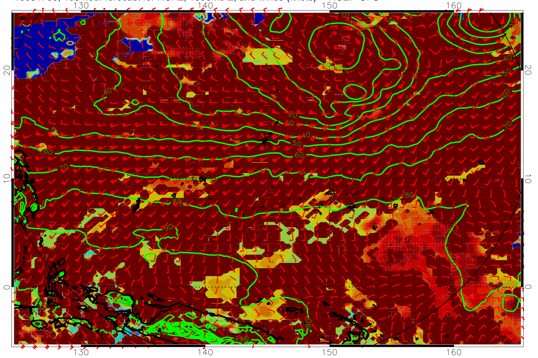
16081700, 108 hour forecast for HCAL, 1000mb Z, and winds (knots) -- NCEP GFS
