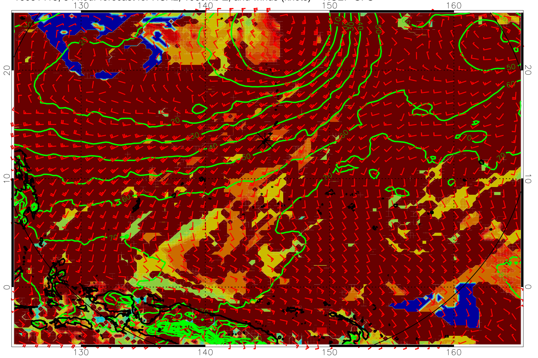
16081418, 54 hour forecast for HCAL, 1000mb Z, and winds (knots) -- NCEP GFS
