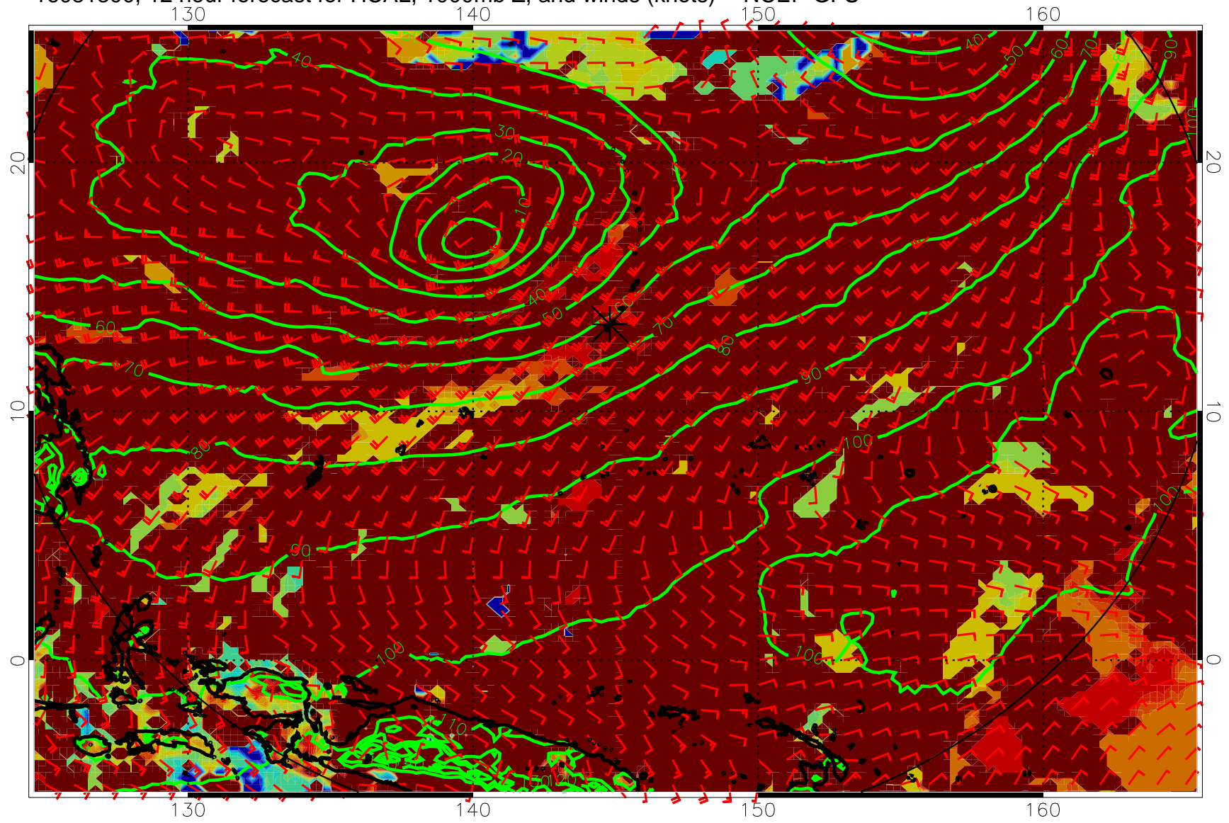
16081300, 12 hour forecast for HCAL, 1000mb Z, and winds (knots) -- NCEP GFS
