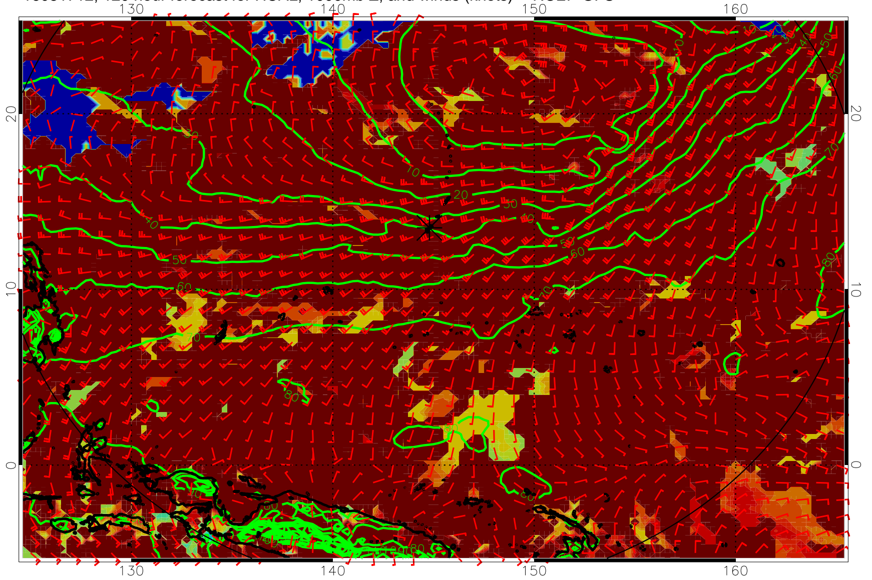
16081712, 120 hour forecast for HCAL, 1000mb Z, and winds (knots) -- NCEP GFS
