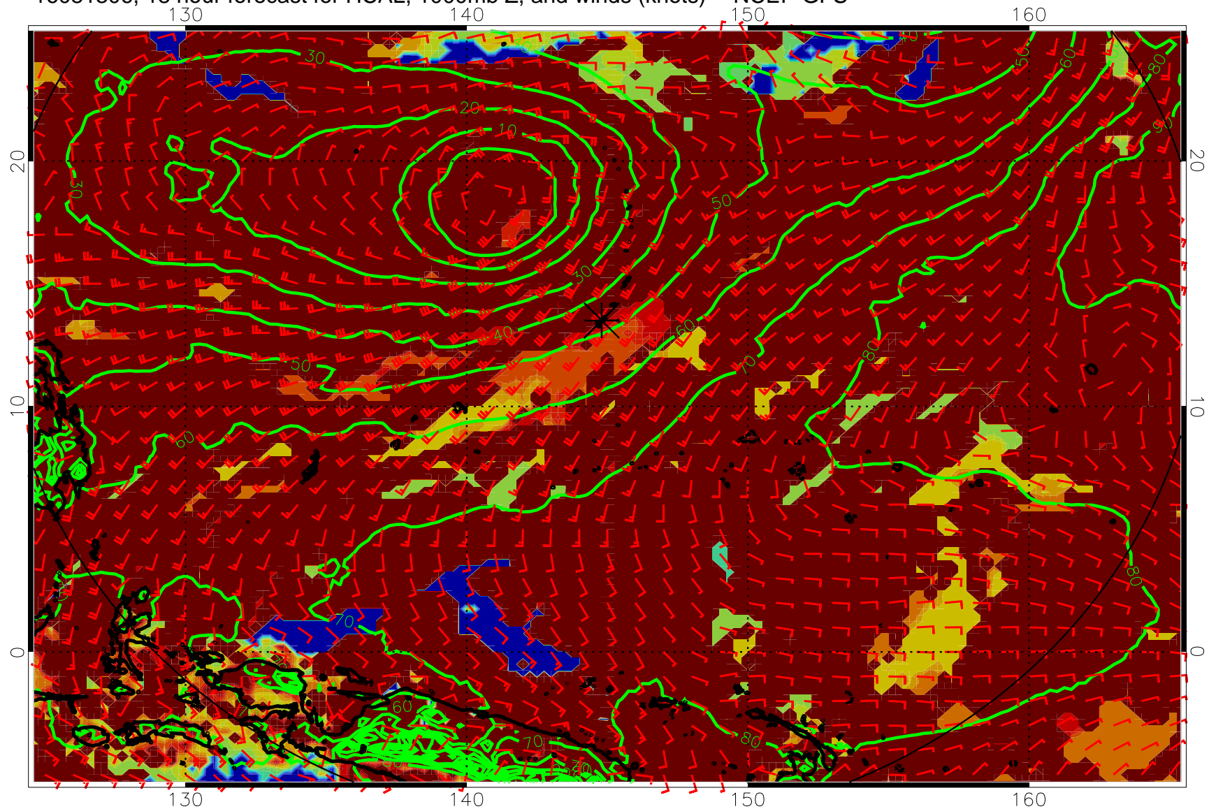
16081306, 18 hour forecast for HCAL, 1000mb Z, and winds (knots) -- NCEP GFS
