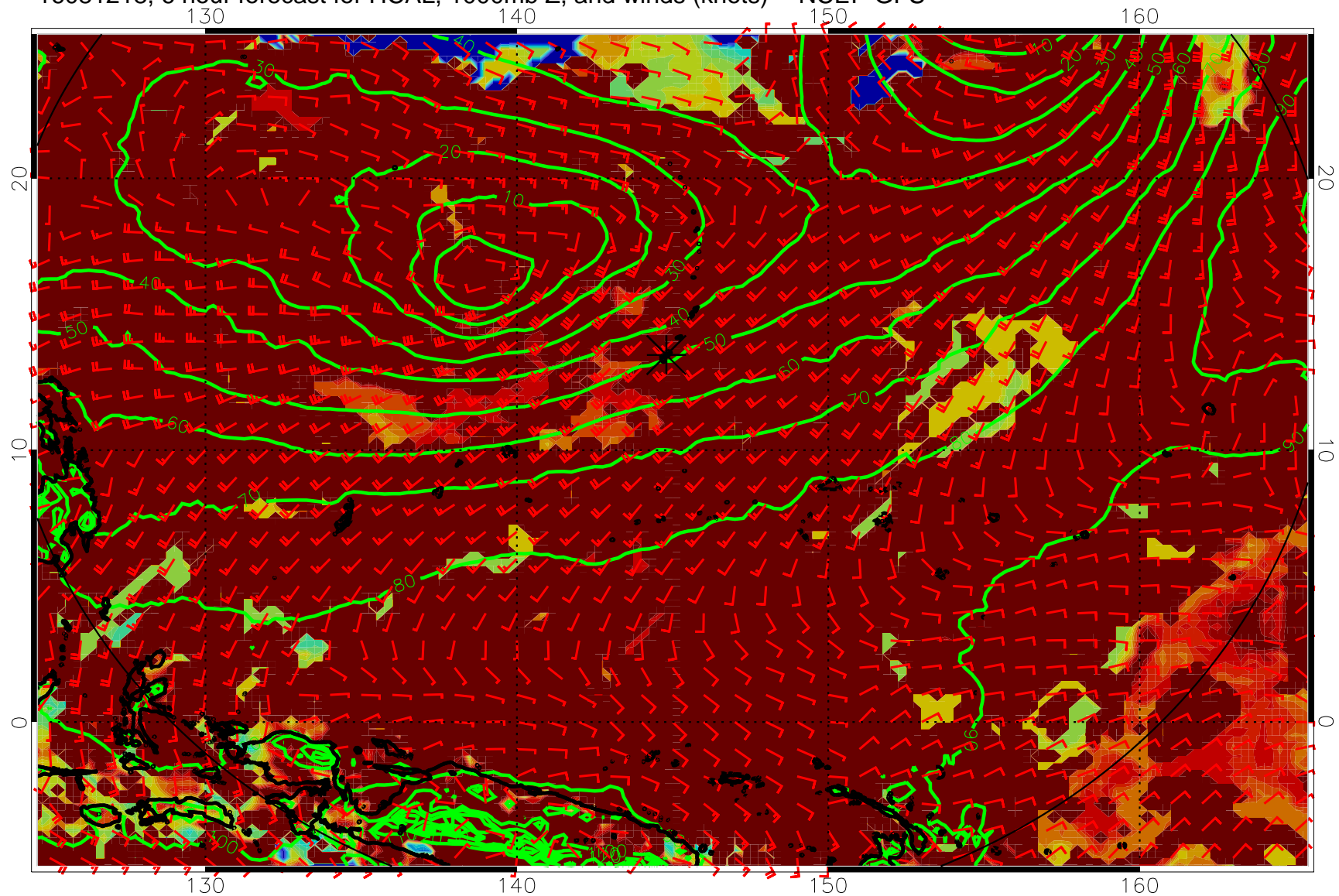
16081218, 6 hour forecast for HCAL, 1000mb Z, and winds (knots) -- NCEP GFS
