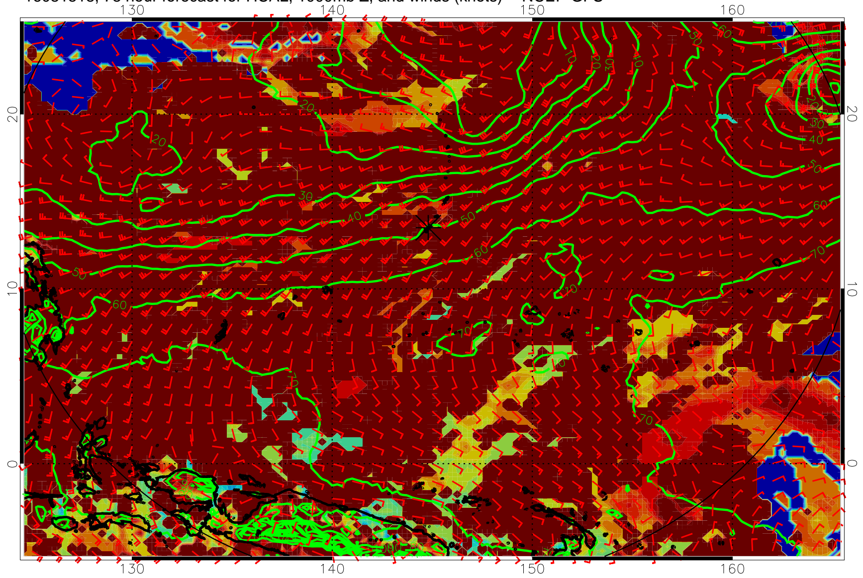
16081518, 78 hour forecast for HCAL, 1000mb Z, and winds (knots) -- NCEP GFS
