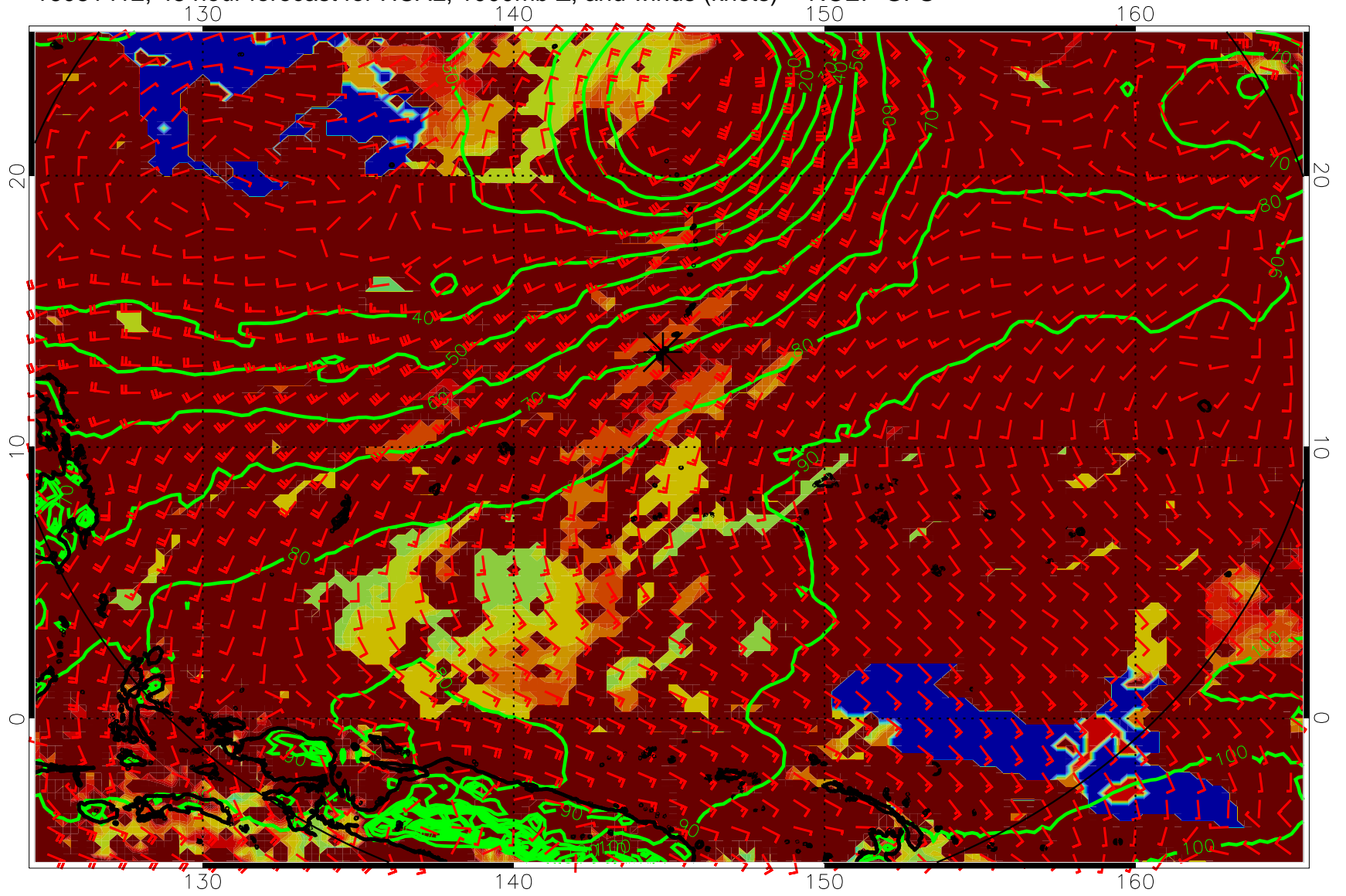
16081412, 48 hour forecast for HCAL, 1000mb Z, and winds (knots) -- NCEP GFS
