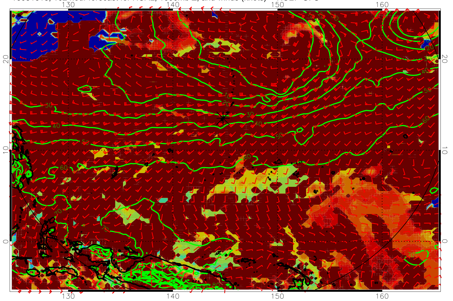
16081618, 102 hour forecast for HCAL, 1000mb Z, and winds (knots) -- NCEP GFS
