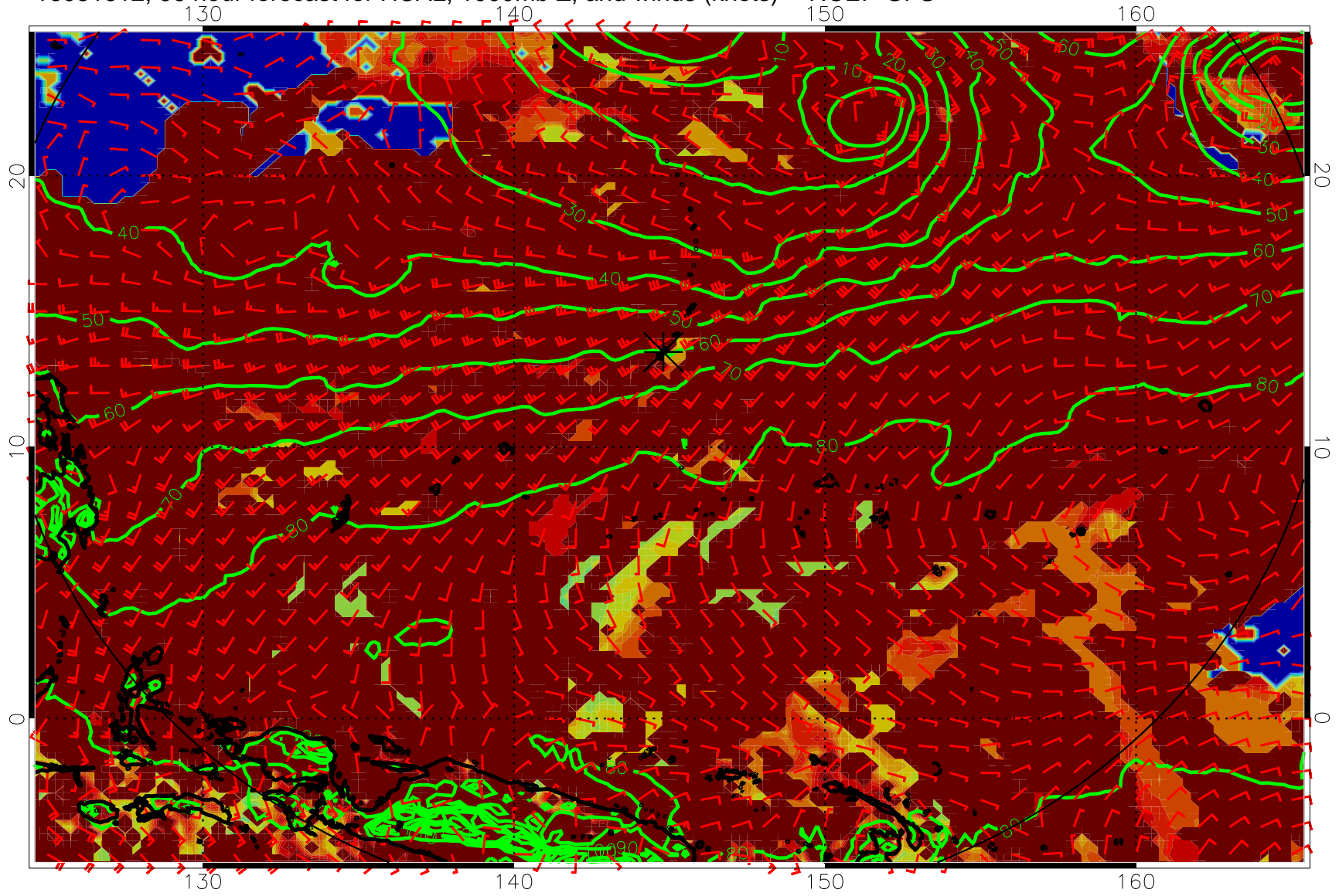
16081612, 96 hour forecast for HCAL, 1000mb Z, and winds (knots) -- NCEP GFS
