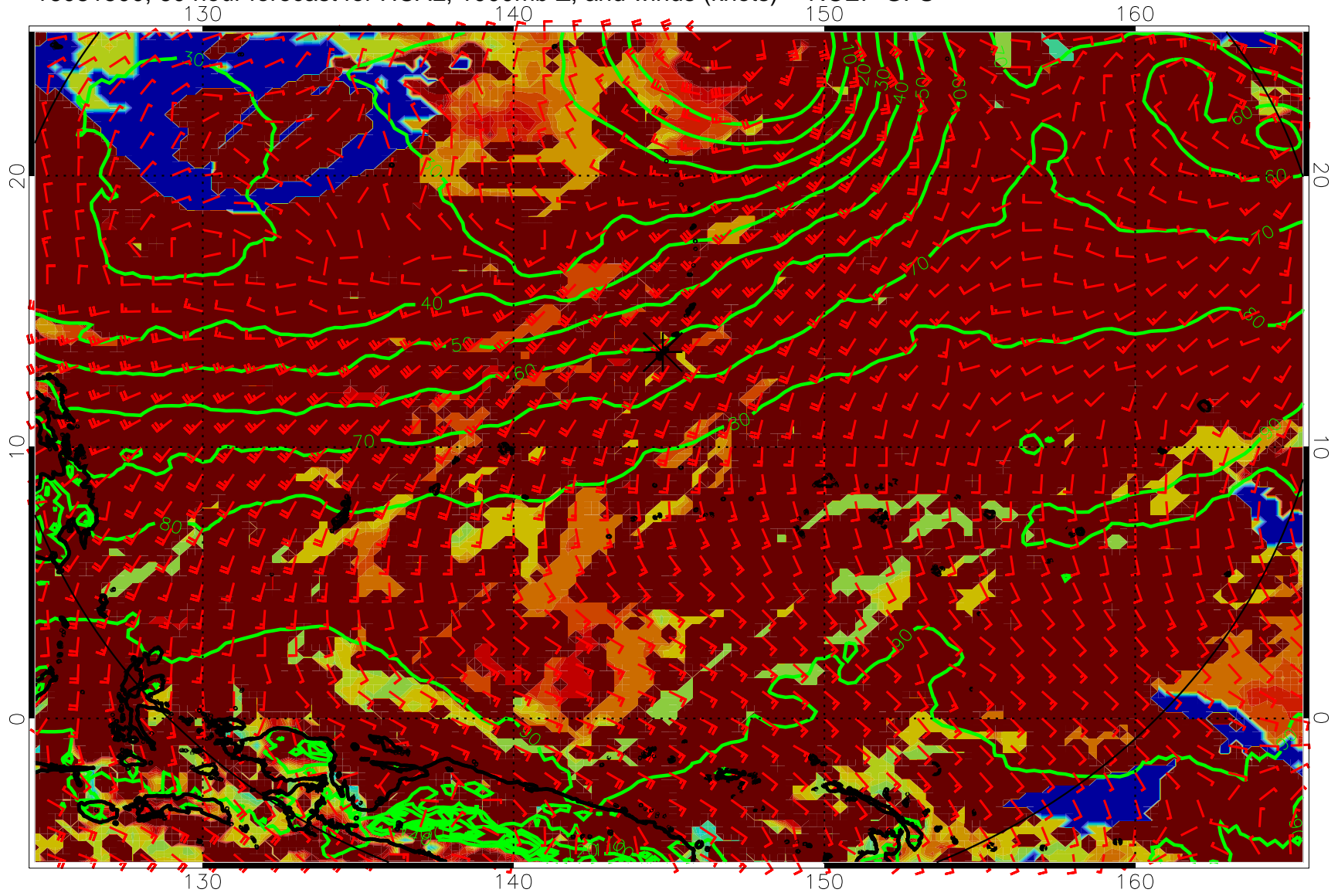
16081500, 60 hour forecast for HCAL, 1000mb Z, and winds (knots) -- NCEP GFS
