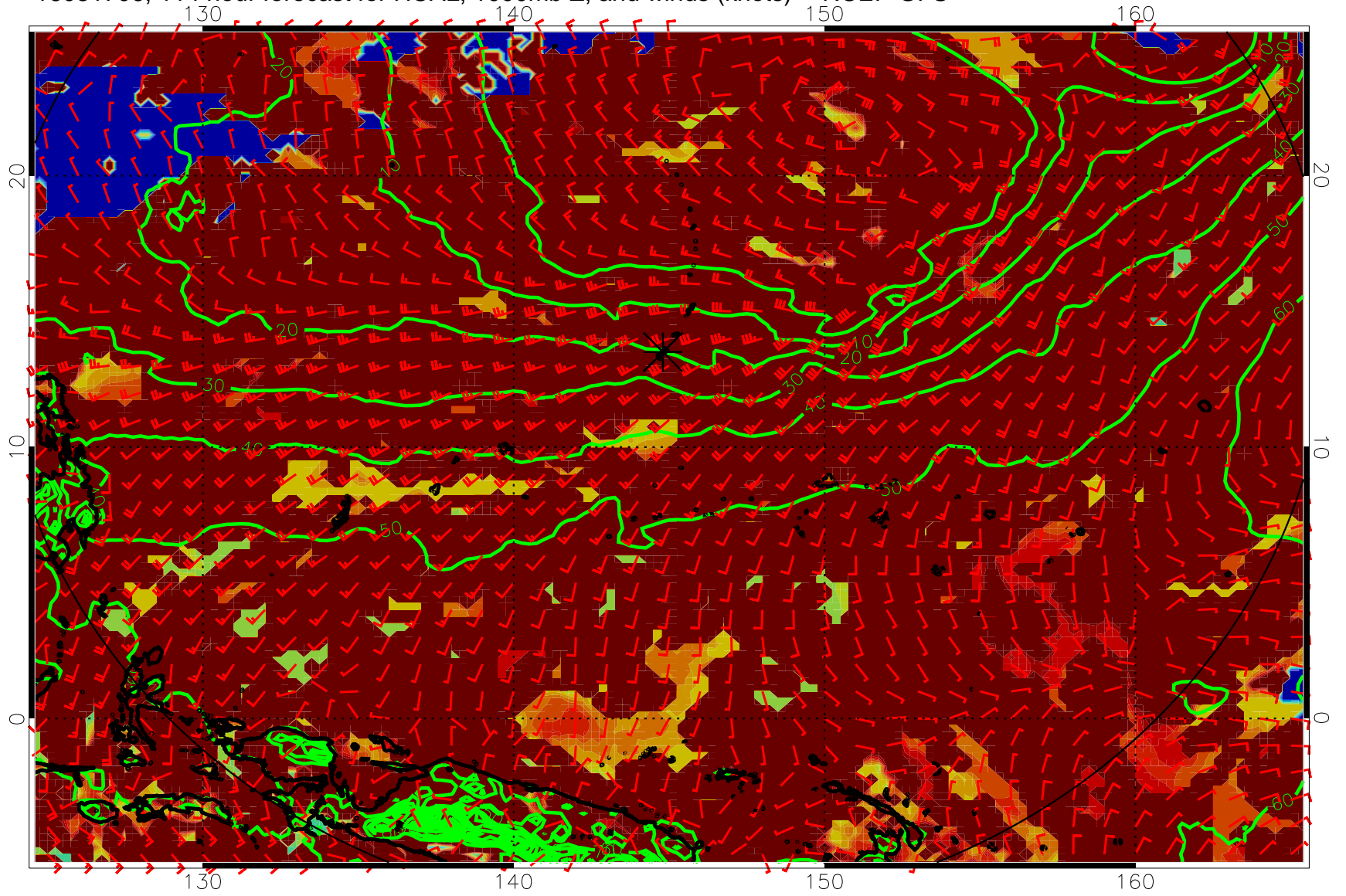
16081706, 114 hour forecast for HCAL, 1000mb Z, and winds (knots) -- NCEP GFS
