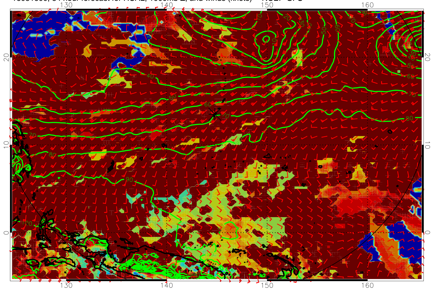
16081600, 84 hour forecast for HCAL, 1000mb Z, and winds (knots) -- NCEP GFS
