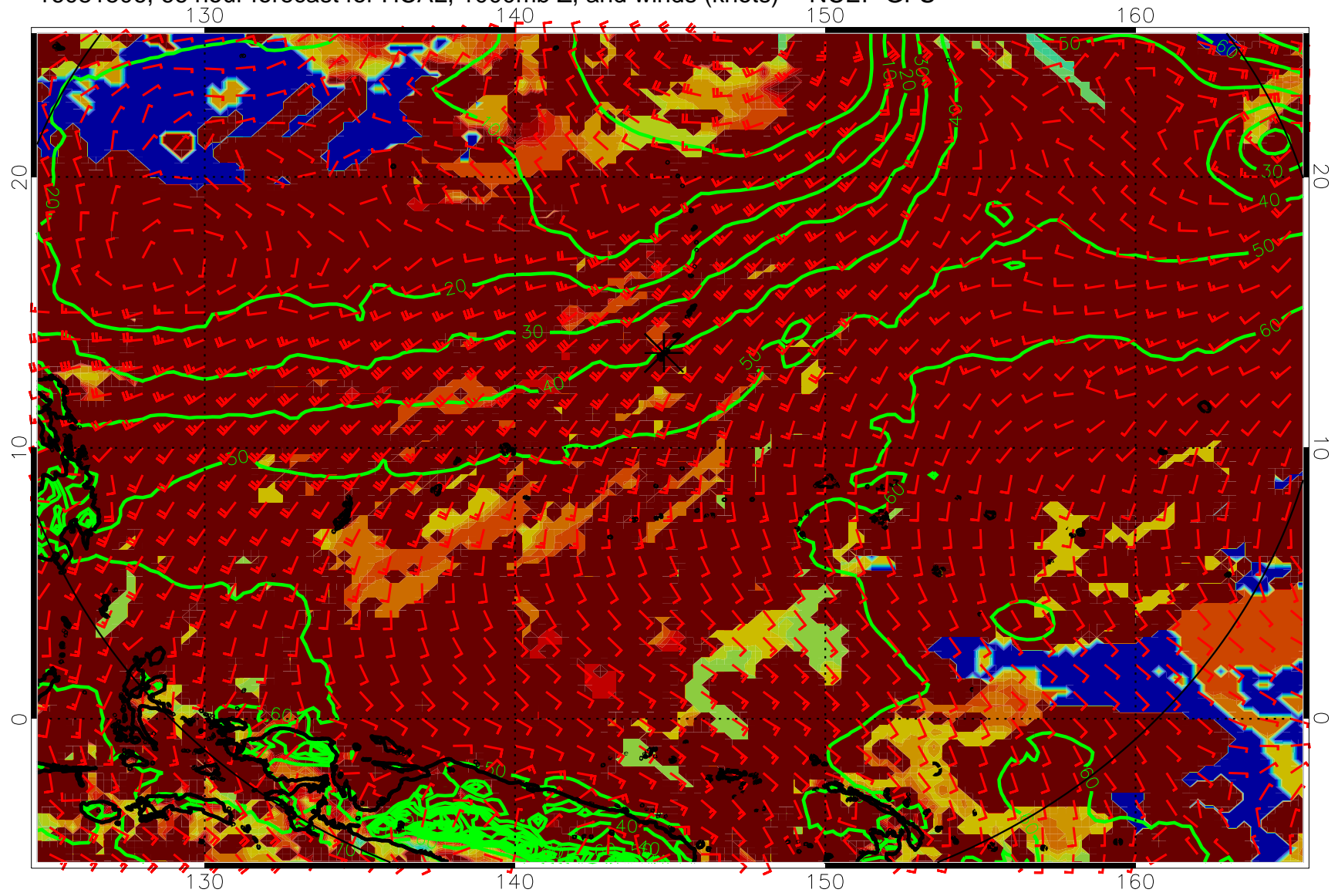
16081506, 66 hour forecast for HCAL, 1000mb Z, and winds (knots) -- NCEP GFS
