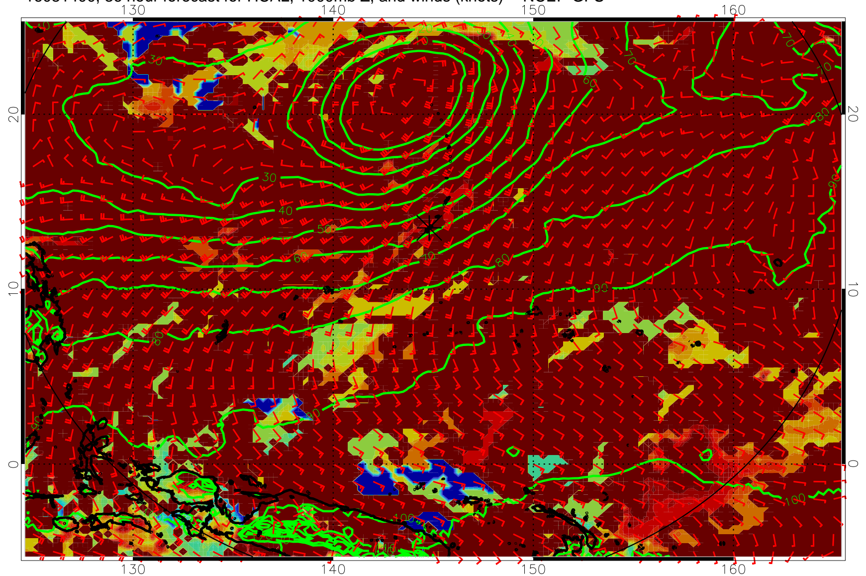
16081400, 36 hour forecast for HCAL, 1000mb Z, and winds (knots) -- NCEP GFS
