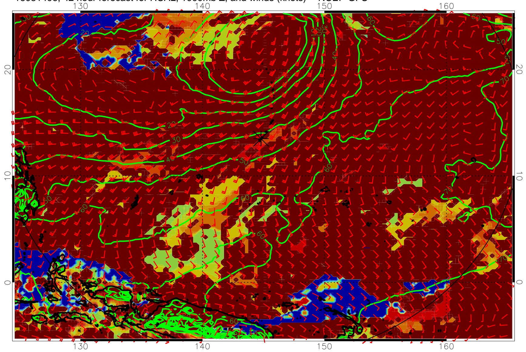
16081406, 42 hour forecast for HCAL, 1000mb Z, and winds (knots) -- NCEP GFS
