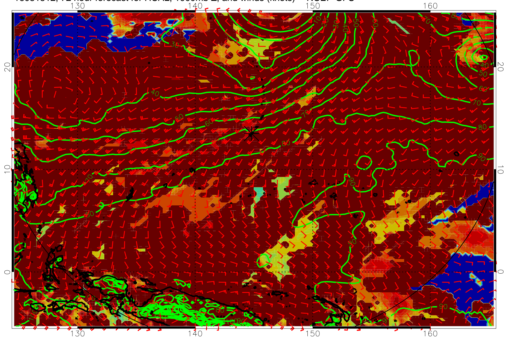
16081512, 72 hour forecast for HCAL, 1000mb Z, and winds (knots) -- NCEP GFS
