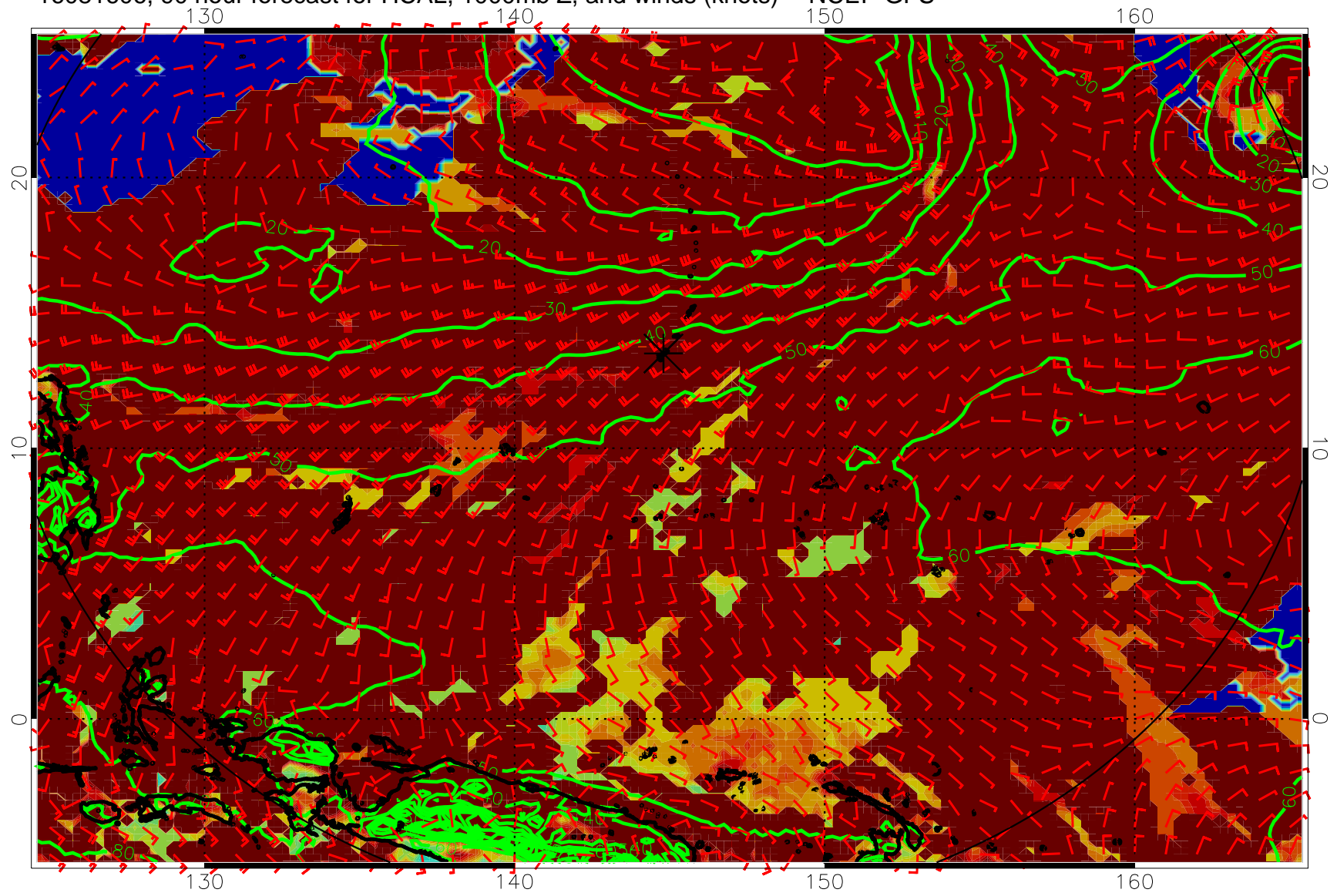
16081606, 90 hour forecast for HCAL, 1000mb Z, and winds (knots) -- NCEP GFS
