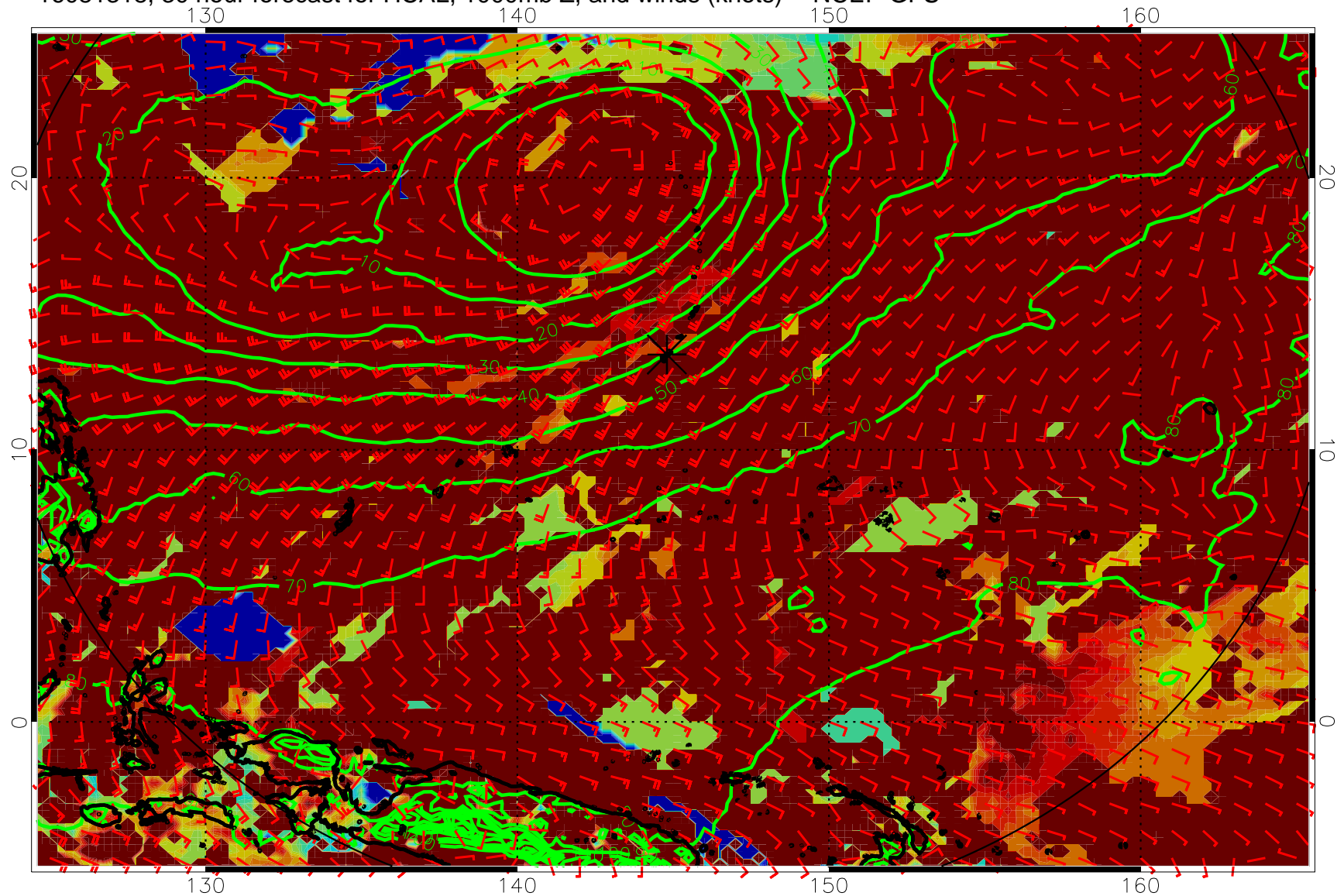
16081318, 30 hour forecast for HCAL, 1000mb Z, and winds (knots) -- NCEP GFS
