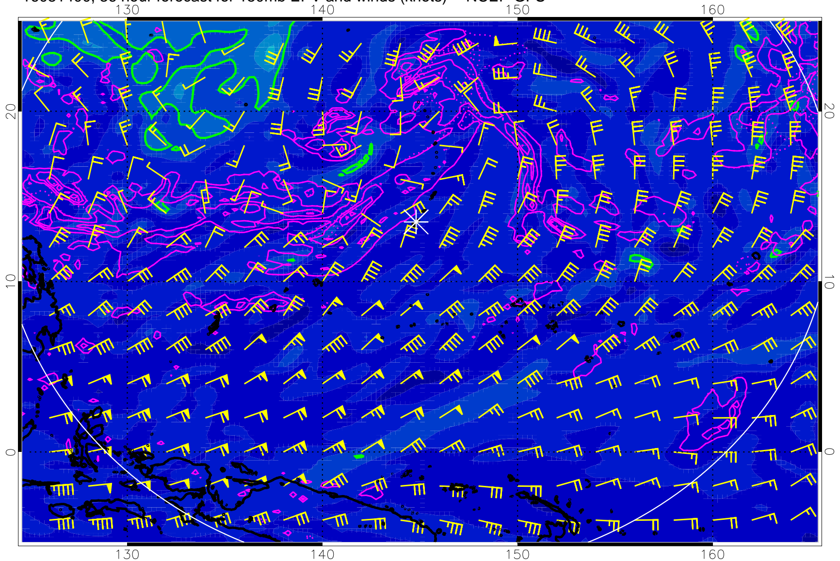
16081400, 36 hour forecast for 150mb EPV and winds (knots) -- NCEP GFS
