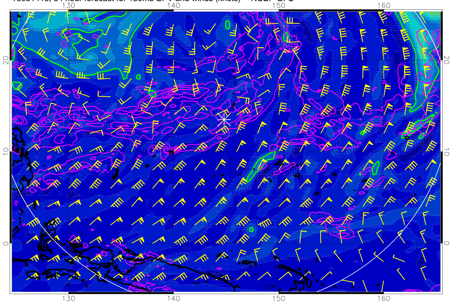
16081418, 54 hour forecast for 150mb EPV and winds (knots) -- NCEP GFS
