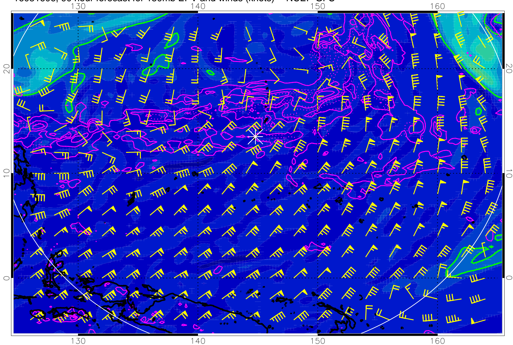
16081606, 90 hour forecast for 150mb EPV and winds (knots) -- NCEP GFS
