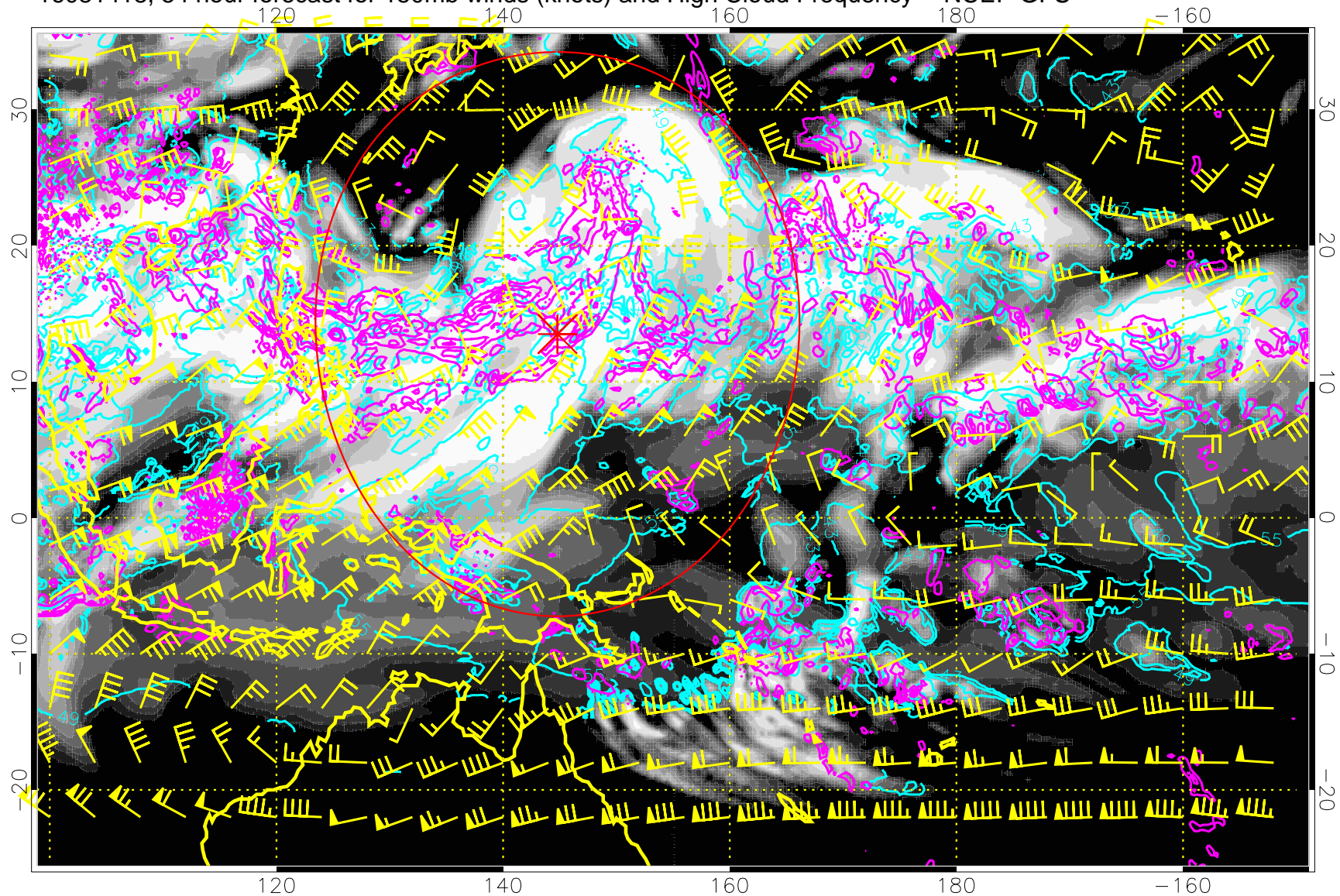
16081418, 54 hour forecast for 150mb winds (knots) and High Cloud Frequency -- NCEP GFS
