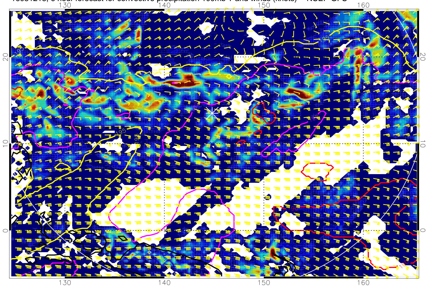
16081218, 6 hour forecast for convective precipitation 100mb T and winds (knots) -- NCEP GFS
