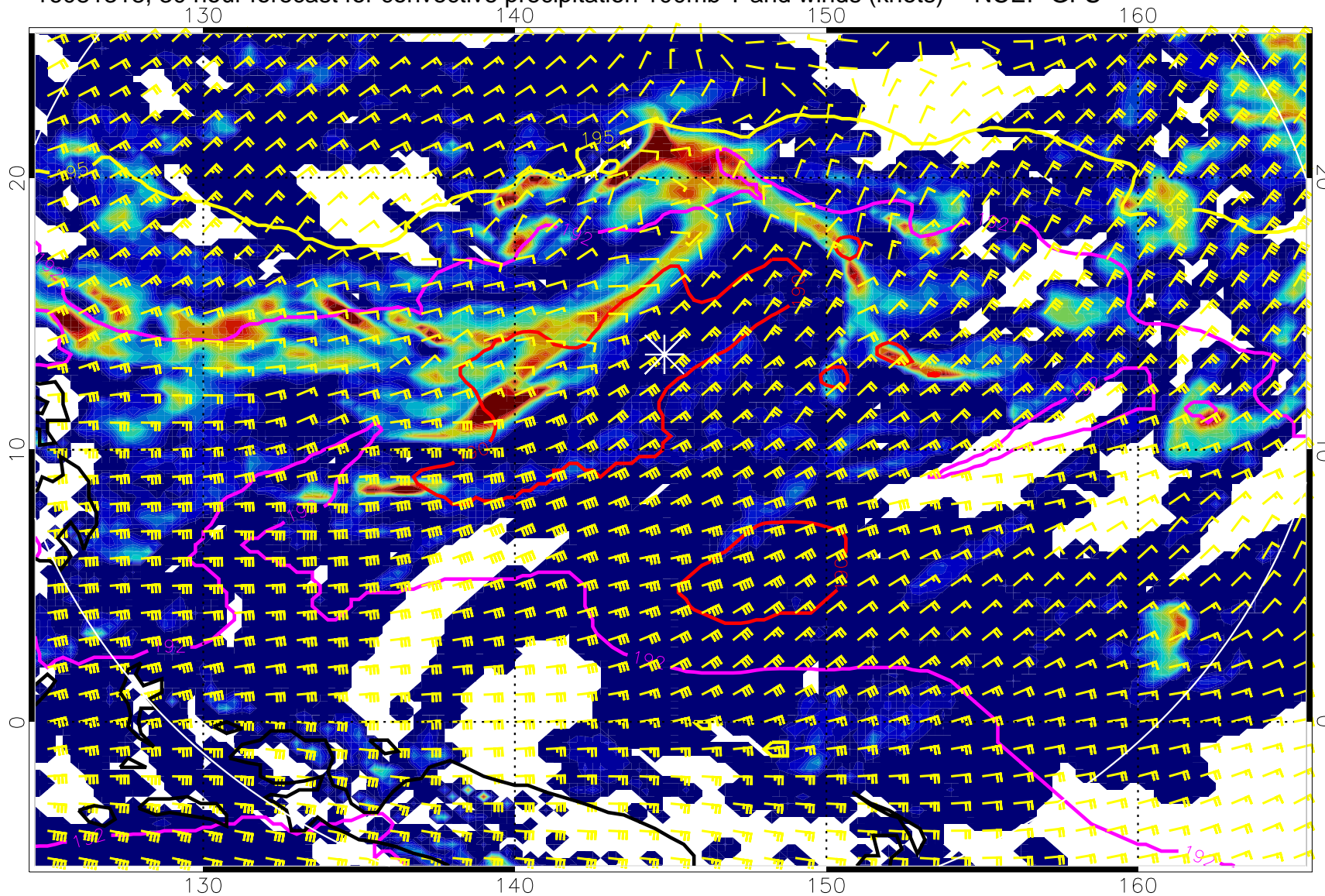
16081318, 30 hour forecast for convective precipitation 100mb T and winds (knots) -- NCEP GFS
