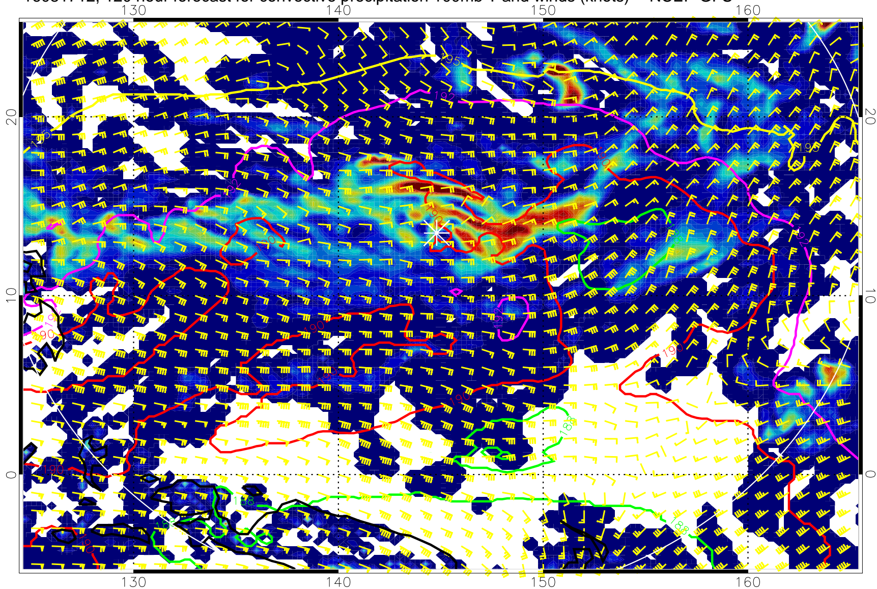
16081712, 120 hour forecast for convective precipitation 100mb T and winds (knots) -- NCEP GFS
