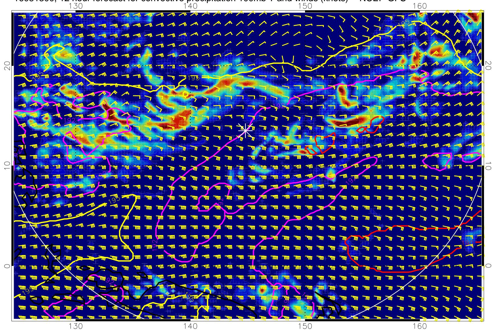
16081300, 12 hour forecast for convective precipitation 100mb T and winds (knots) -- NCEP GFS
