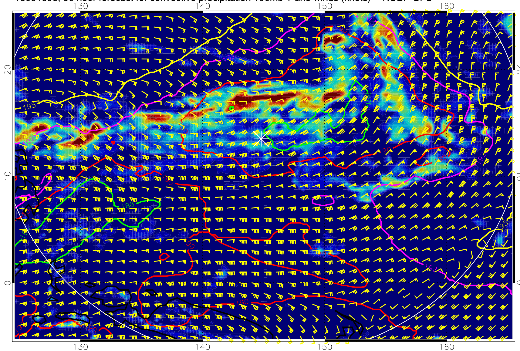
16081606, 90 hour forecast for convective precipitation 100mb T and winds (knots) -- NCEP GFS
