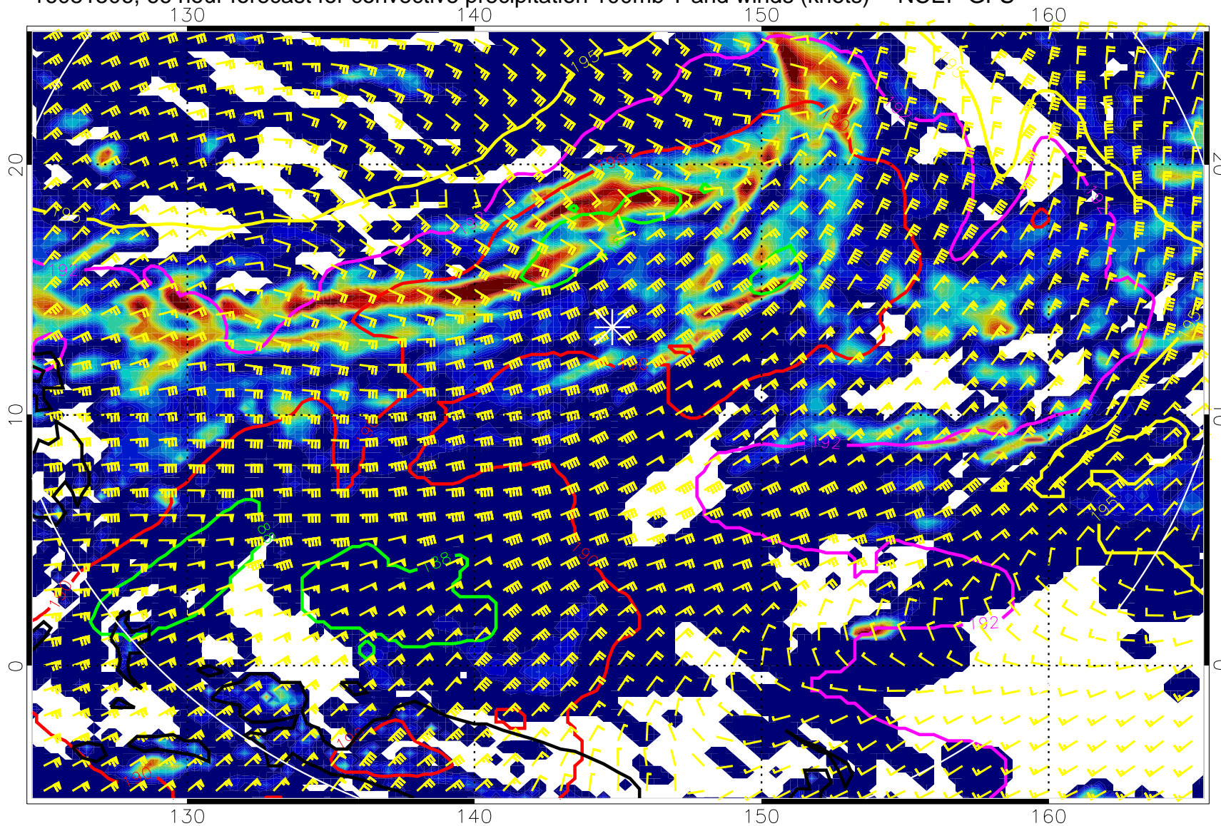
16081506, 66 hour forecast for convective precipitation 100mb T and winds (knots) -- NCEP GFS
