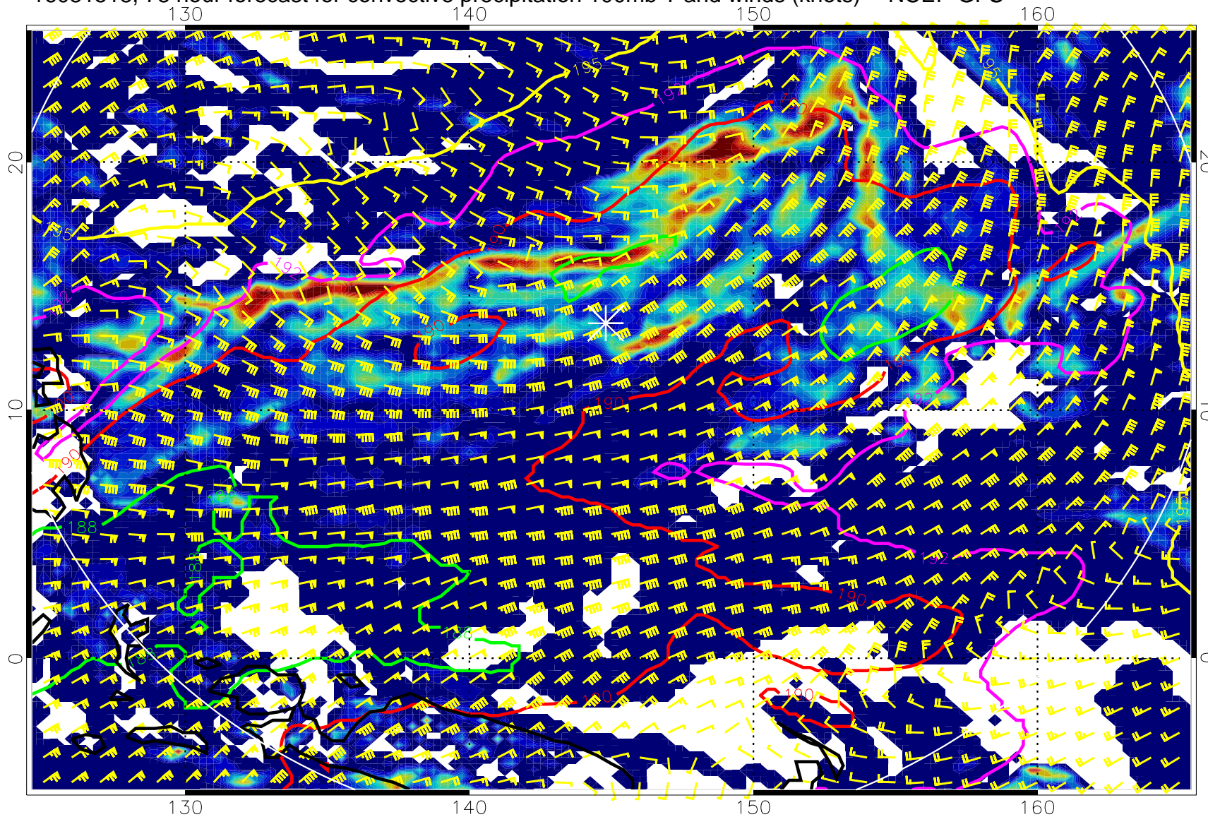
16081518, 78 hour forecast for convective precipitation 100mb T and winds (knots) -- NCEP GFS
