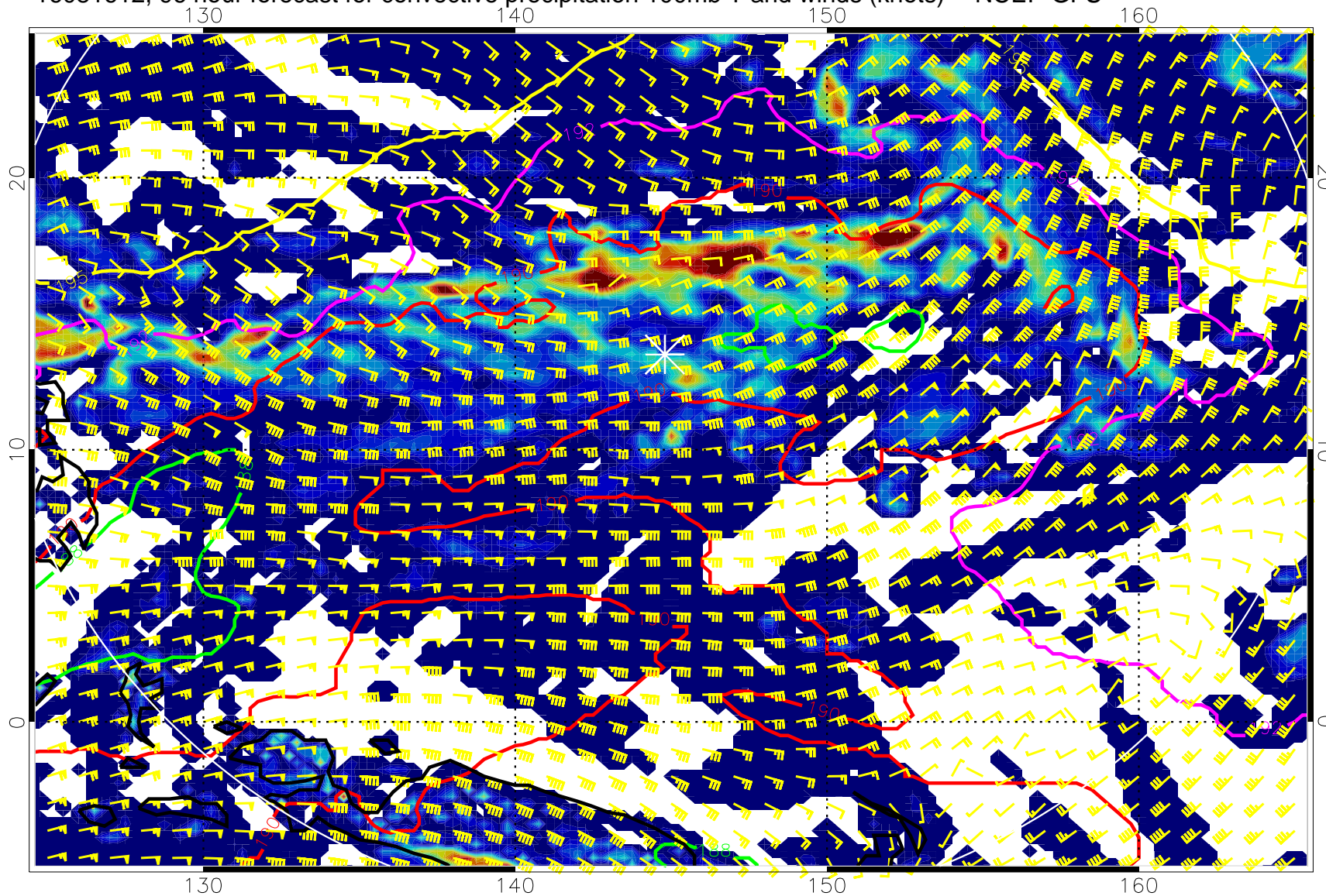
16081612, 96 hour forecast for convective precipitation 100mb T and winds (knots) -- NCEP GFS
