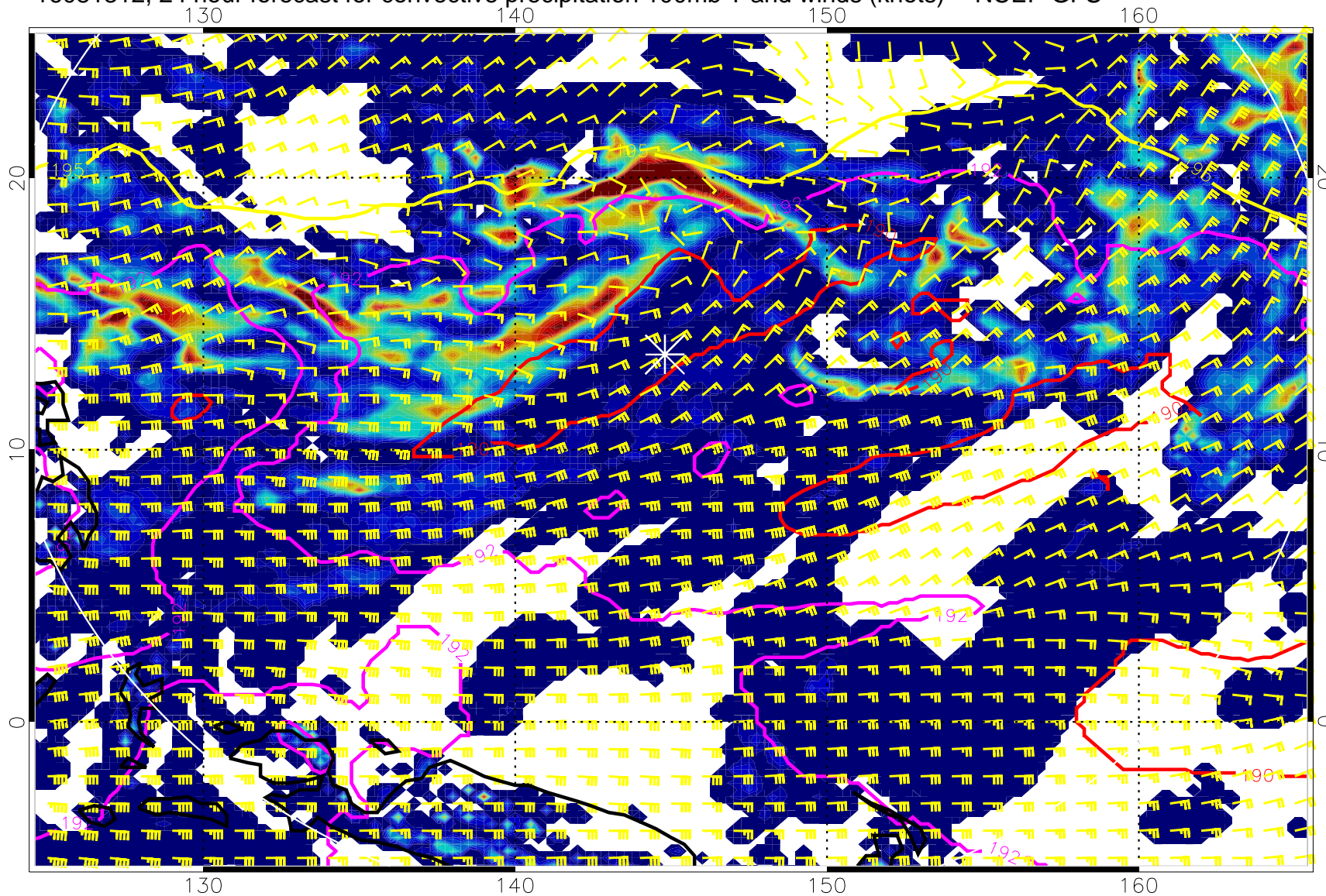
16081312, 24 hour forecast for convective precipitation 100mb T and winds (knots) -- NCEP GFS
