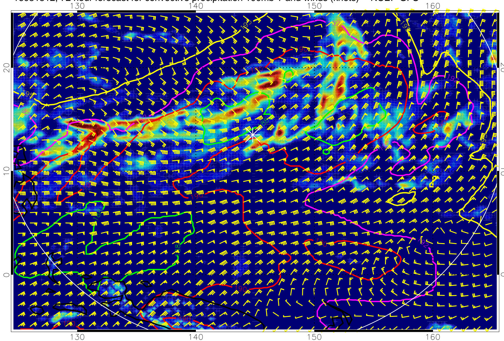
16081512, 72 hour forecast for convective precipitation 100mb T and winds (knots) -- NCEP GFS
