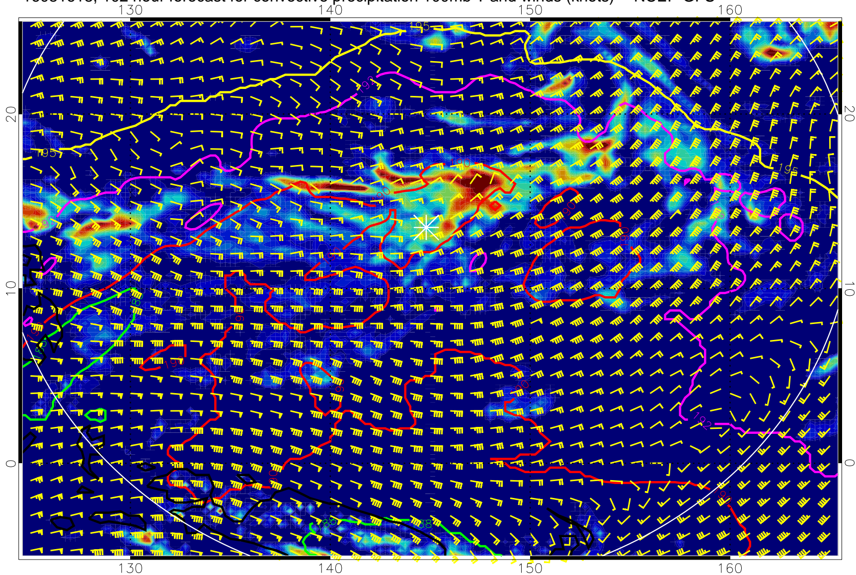
16081618, 102 hour forecast for convective precipitation 100mb T and winds (knots) -- NCEP GFS
