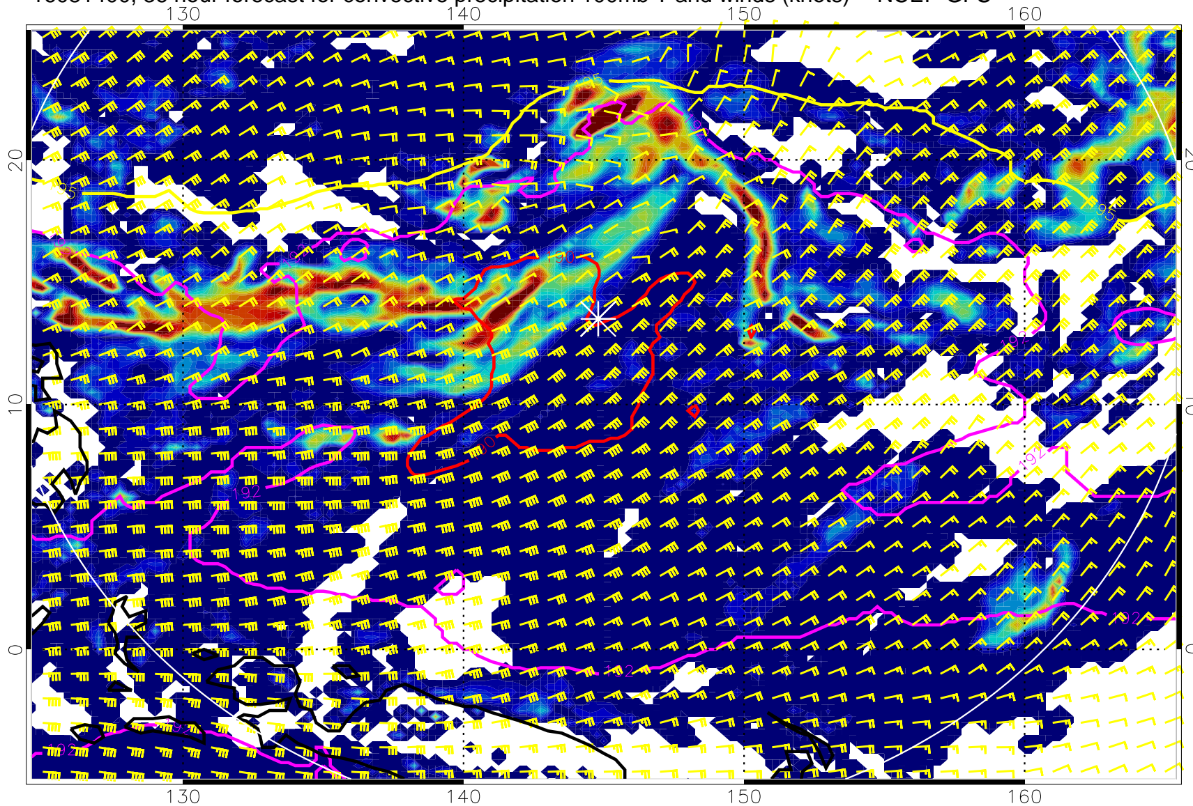
16081400, 36 hour forecast for convective precipitation 100mb T and winds (knots) -- NCEP GFS
