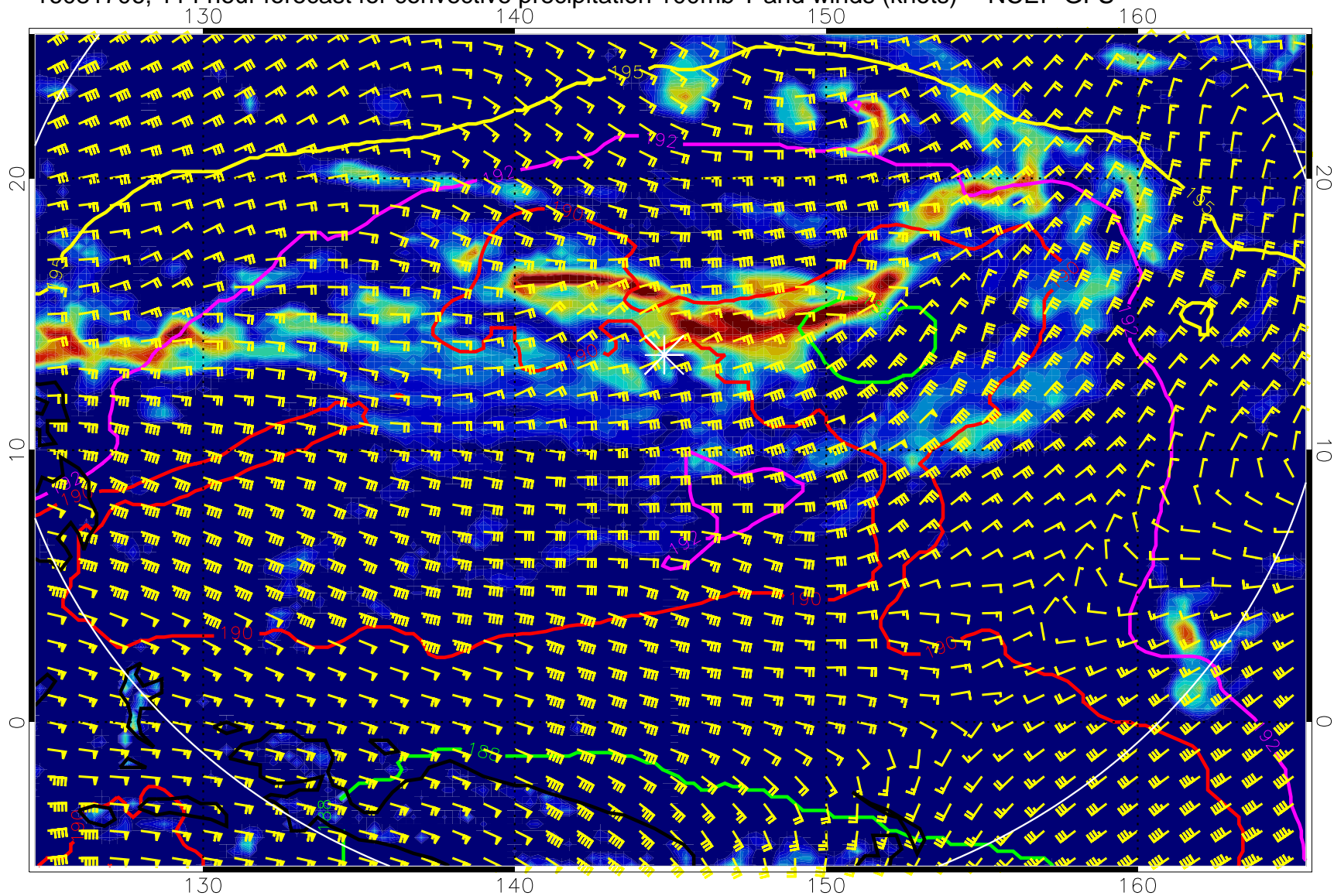
16081706, 114 hour forecast for convective precipitation 100mb T and winds (knots) -- NCEP GFS
