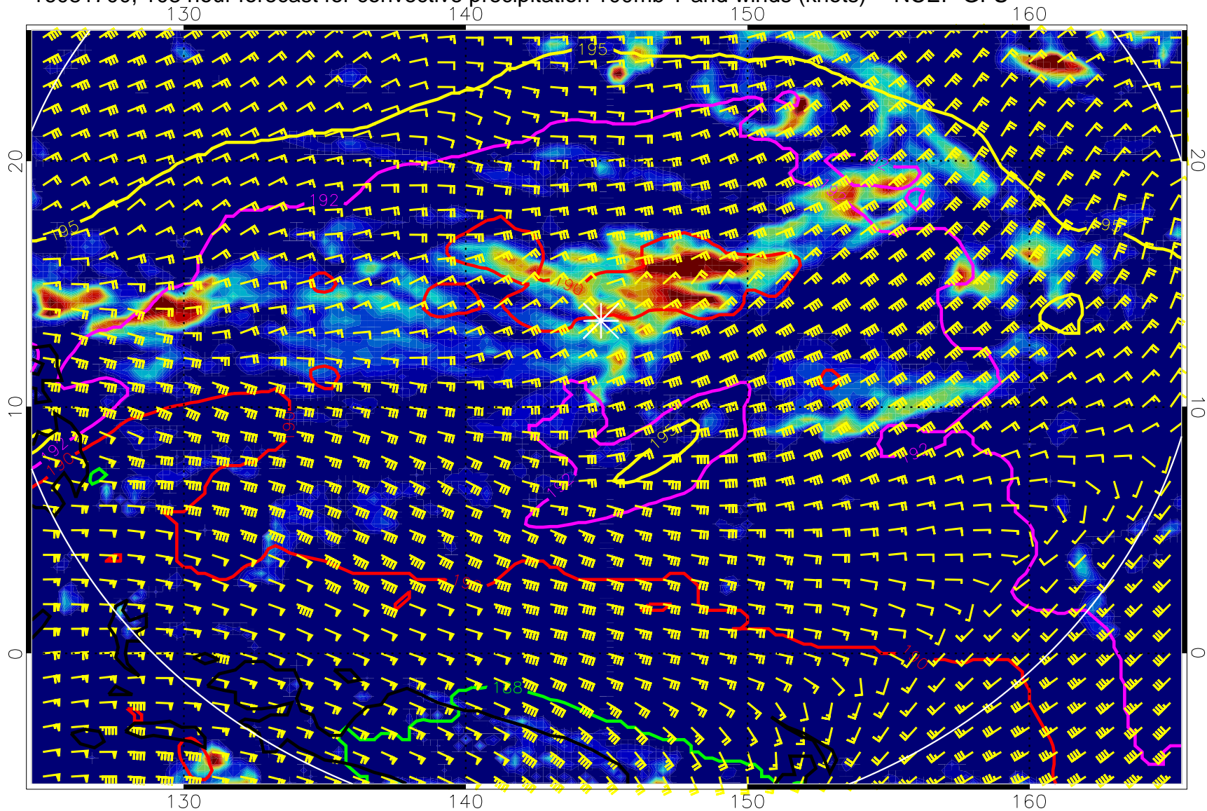
16081700, 108 hour forecast for convective precipitation 100mb T and winds (knots) -- NCEP GFS
