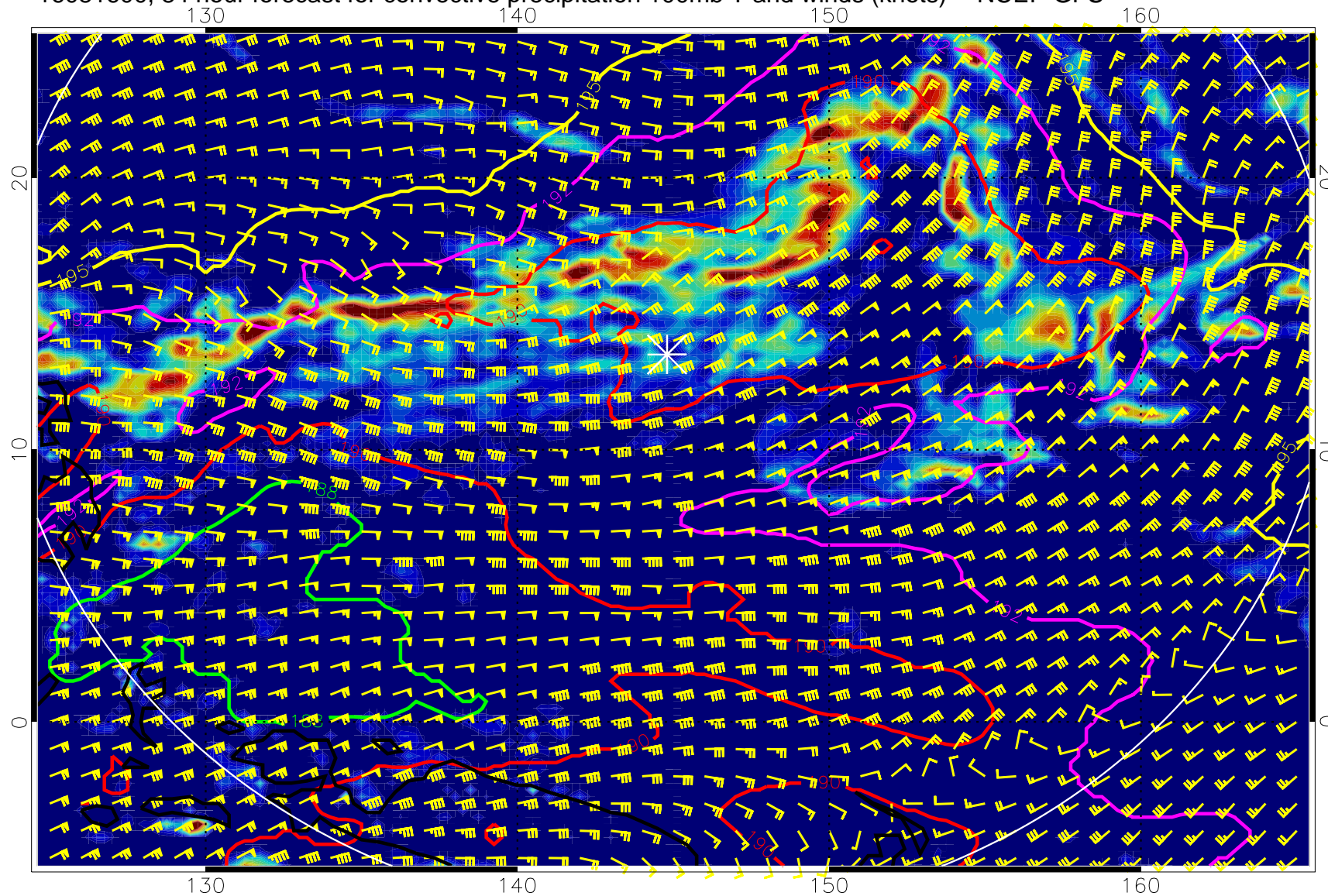
16081600, 84 hour forecast for convective precipitation 100mb T and winds (knots) -- NCEP GFS
