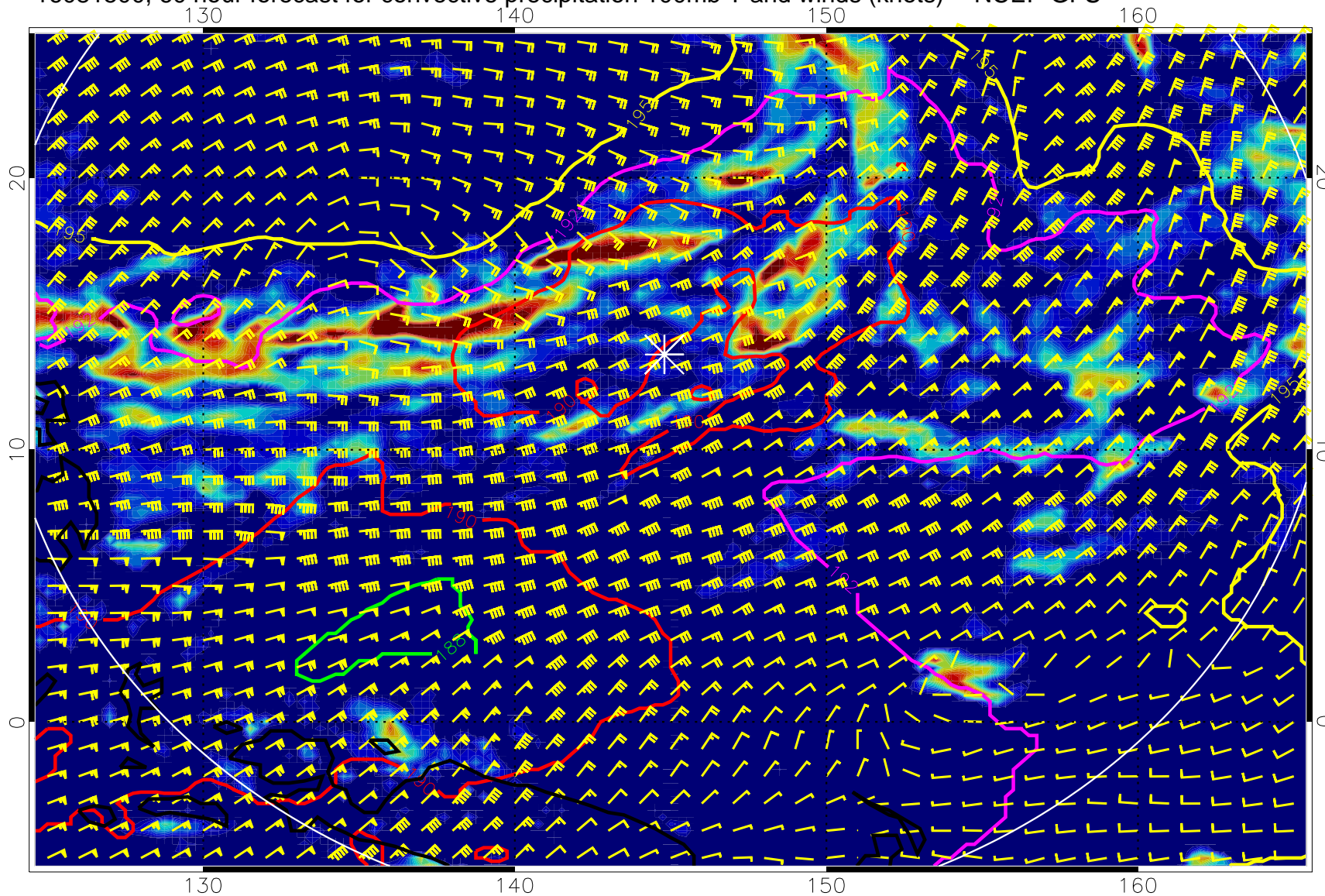
16081500, 60 hour forecast for convective precipitation 100mb T and winds (knots) -- NCEP GFS
