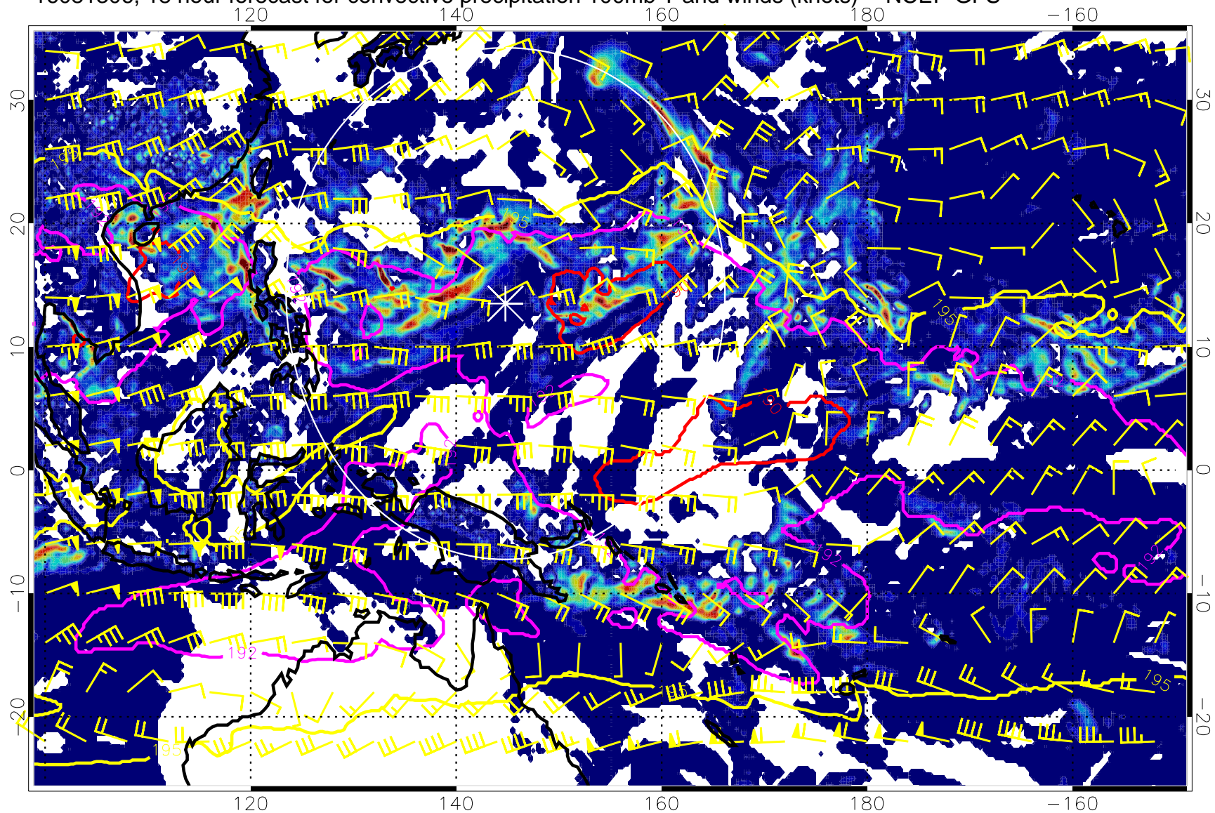
16081306, 18 hour forecast for convective precipitation 100mb T and winds (knots) -- NCEP GFS
