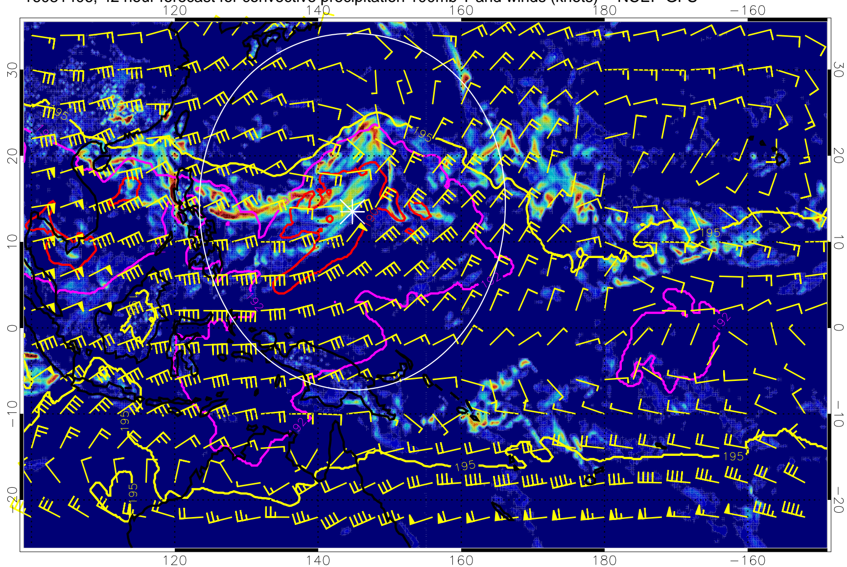
16081406, 42 hour forecast for convective precipitation 100mb T and winds (knots) -- NCEP GFS
