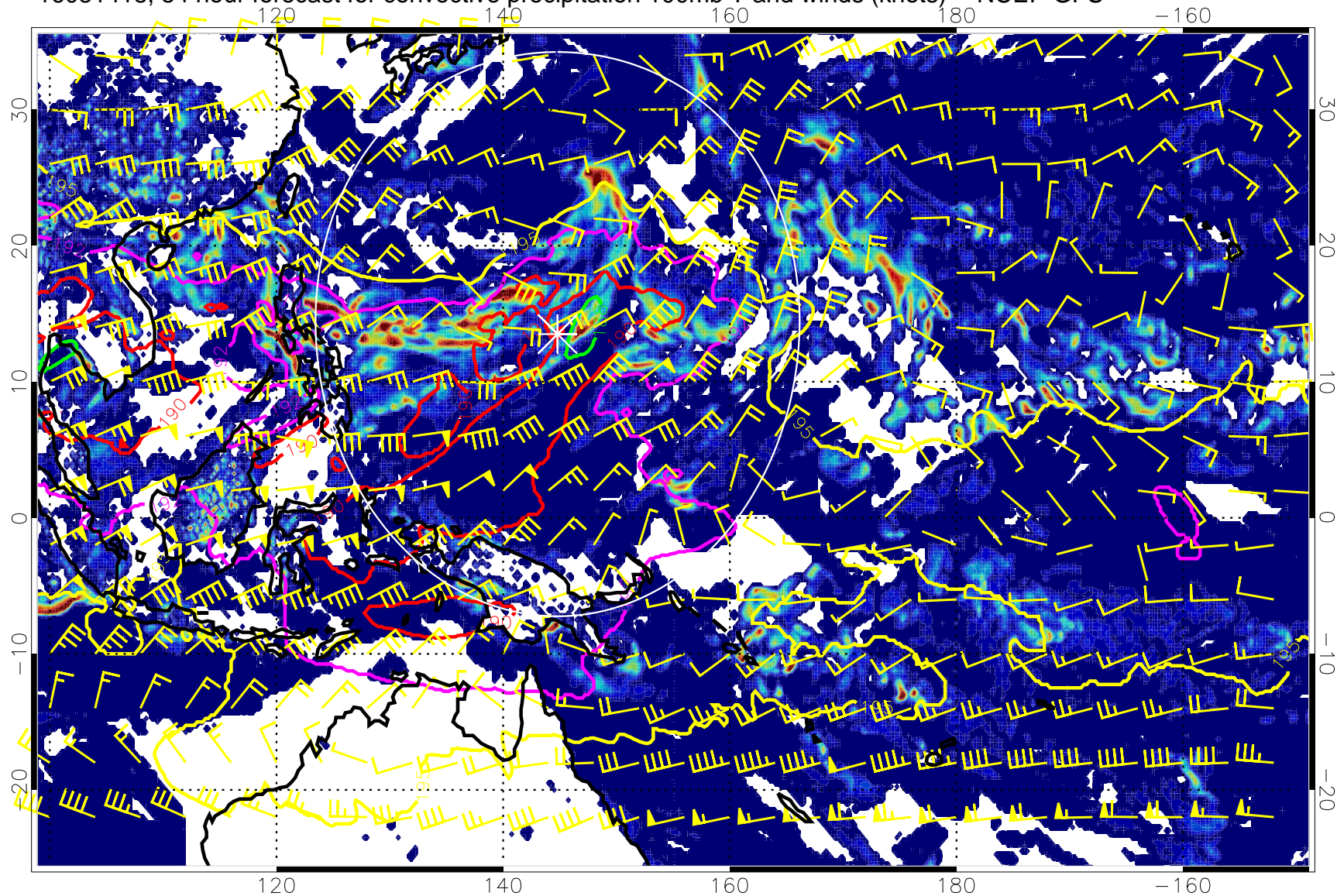
16081418, 54 hour forecast for convective precipitation 100mb T and winds (knots) -- NCEP GFS
