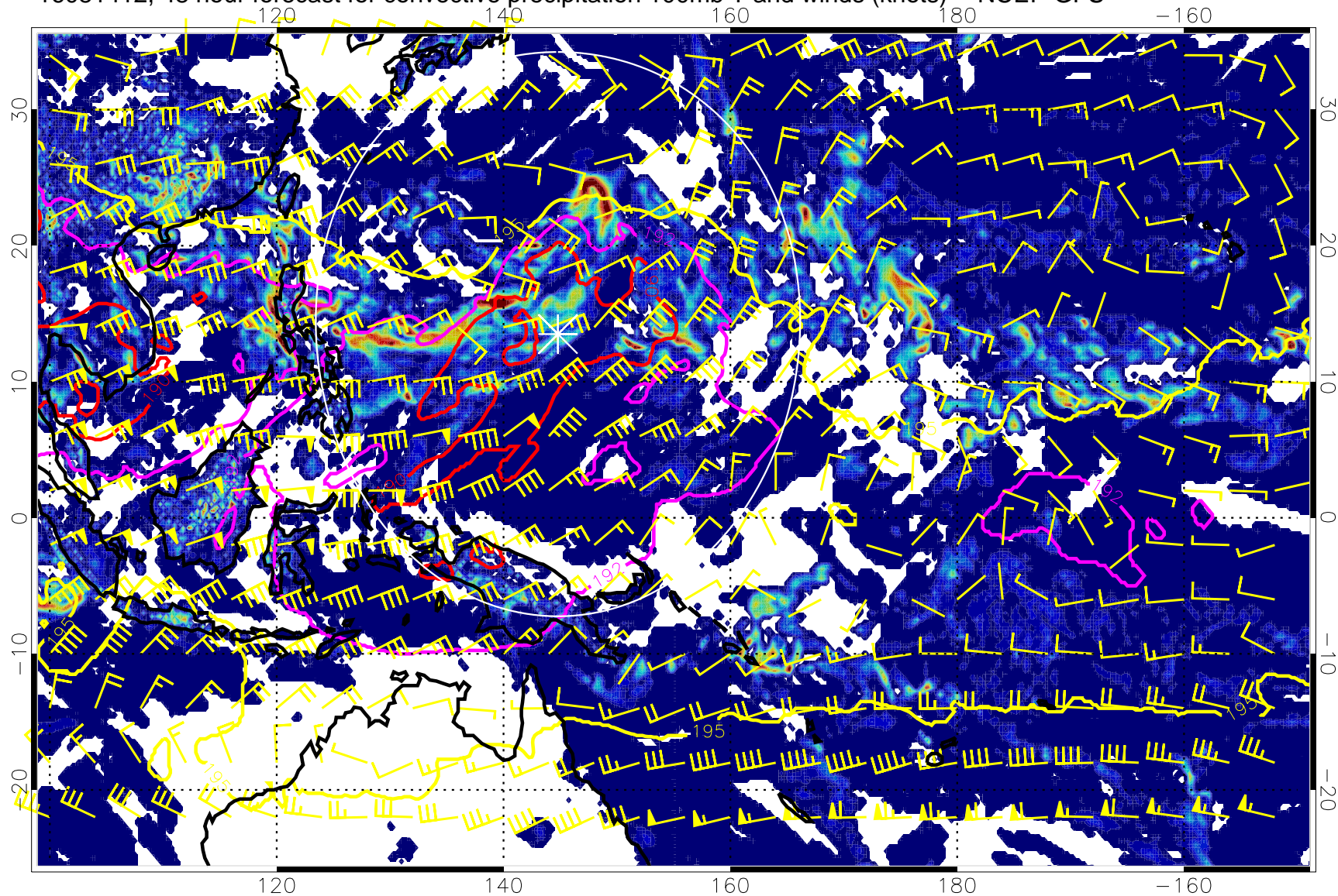
16081412, 48 hour forecast for convective precipitation 100mb T and winds (knots) -- NCEP GFS
