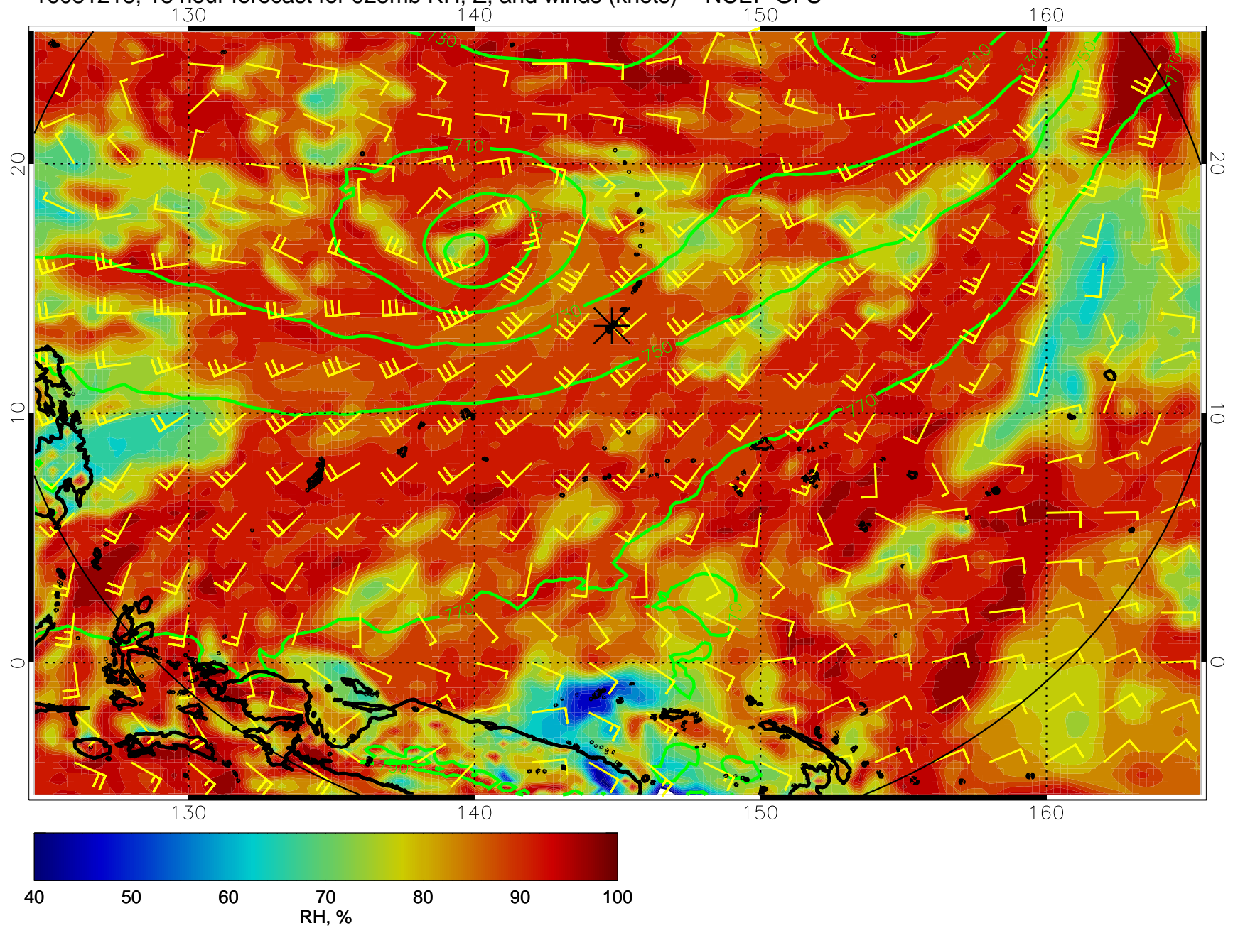
16081218, 18 hour forecast for 925mb RH, Z, and winds (knots) -- NCEP GFS
