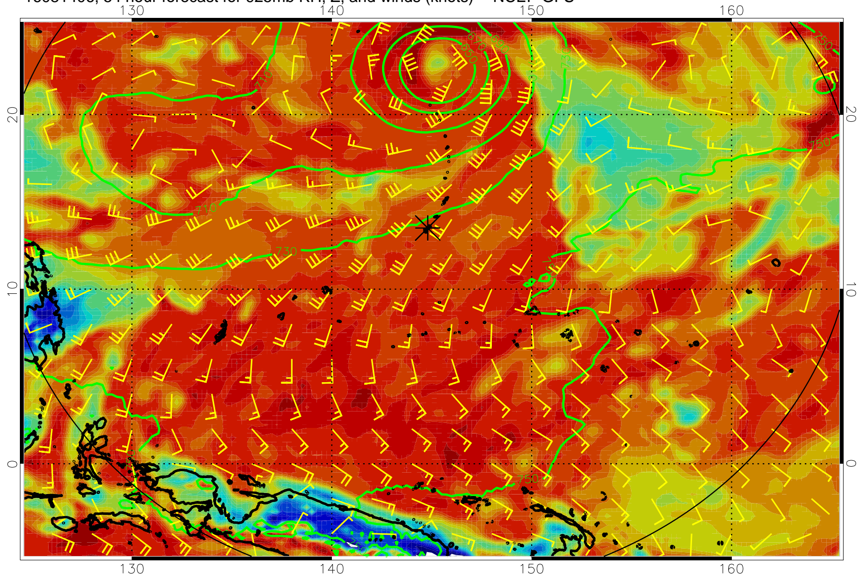
16081406, 54 hour forecast for 925mb RH, Z, and winds (knots) -- NCEP GFS
