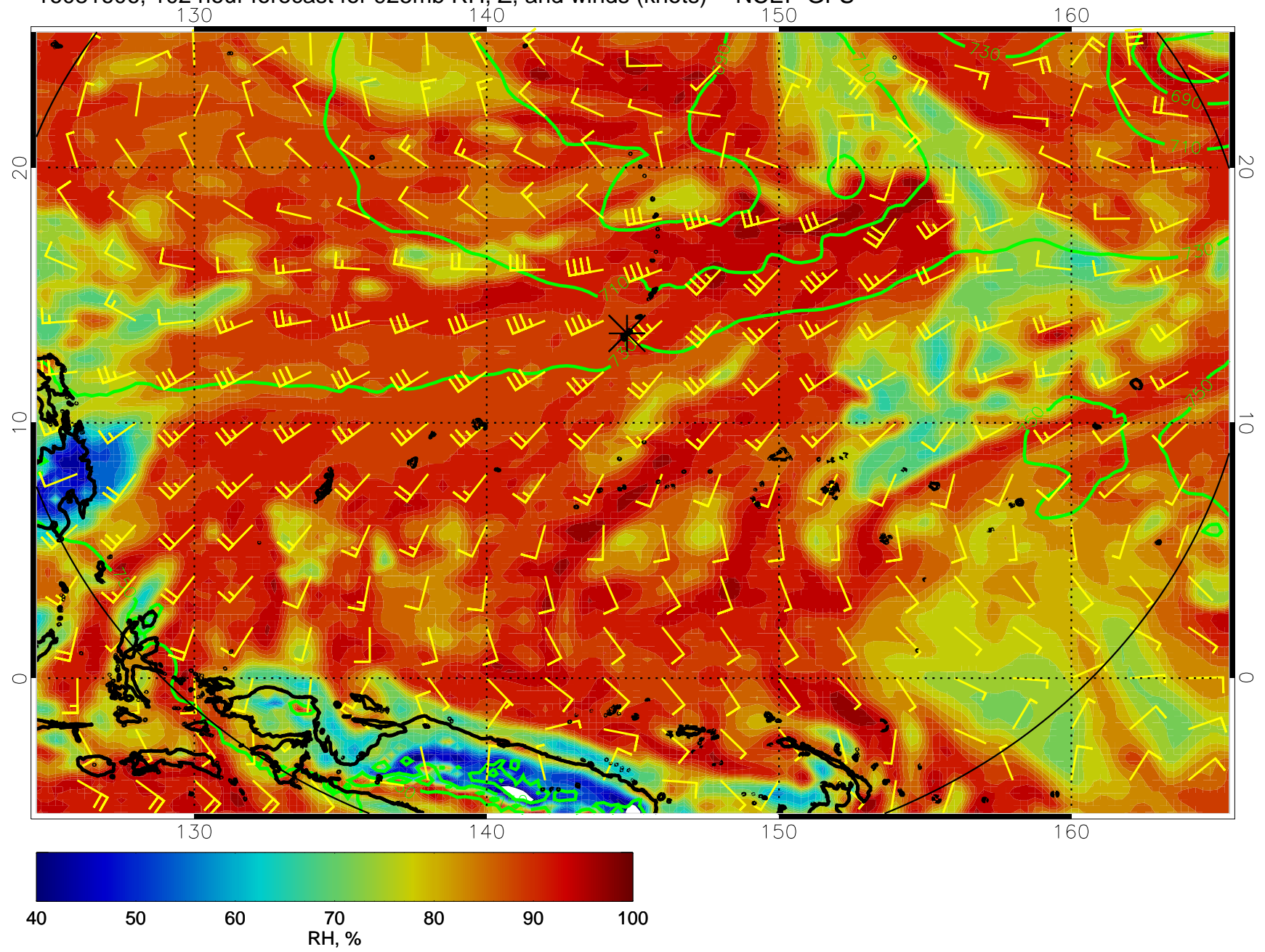
16081606, 102 hour forecast for 925mb RH, Z, and winds (knots) -- NCEP GFS
