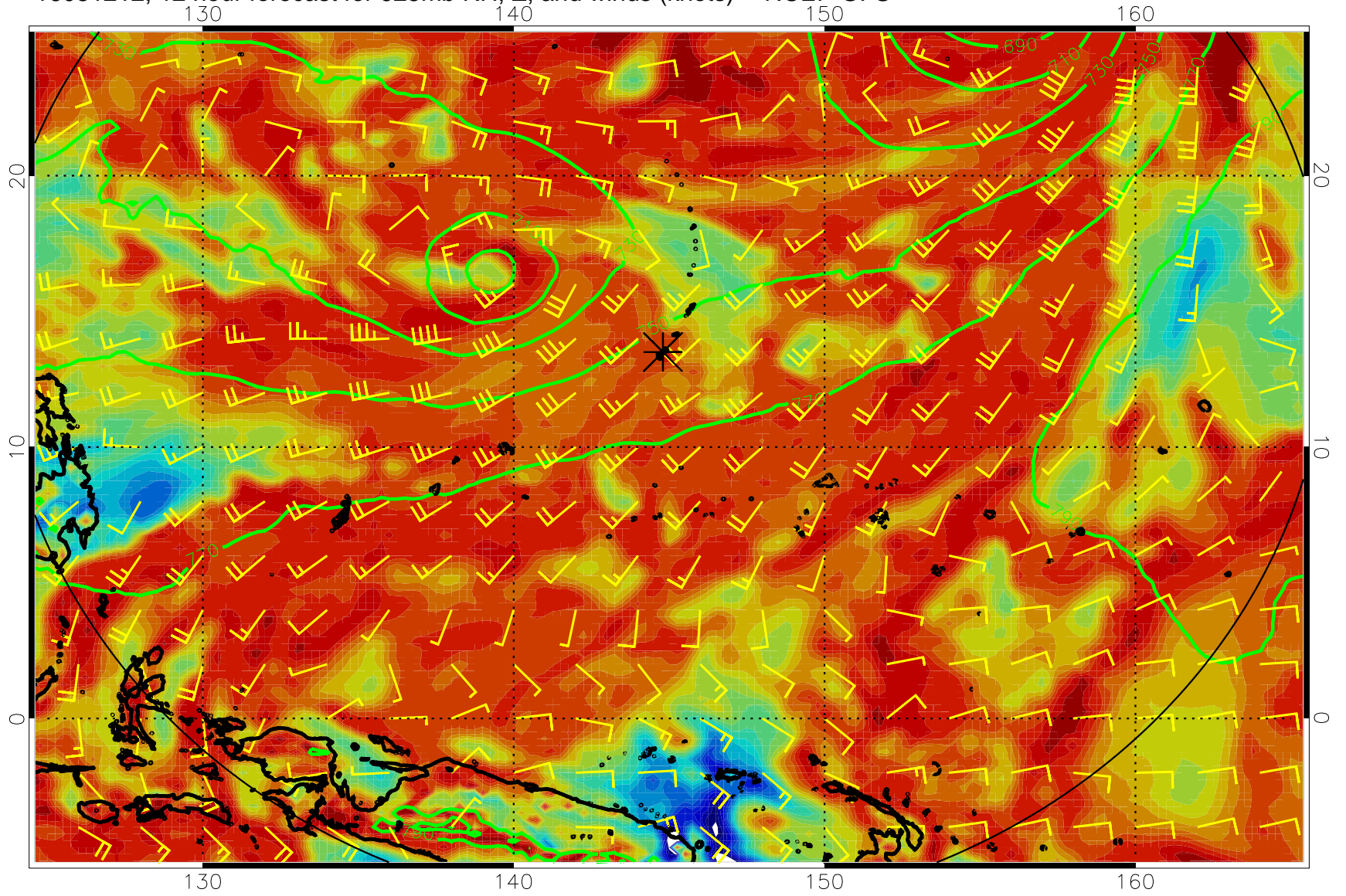
16081212, 12 hour forecast for 925mb RH, Z, and winds (knots) -- NCEP GFS
