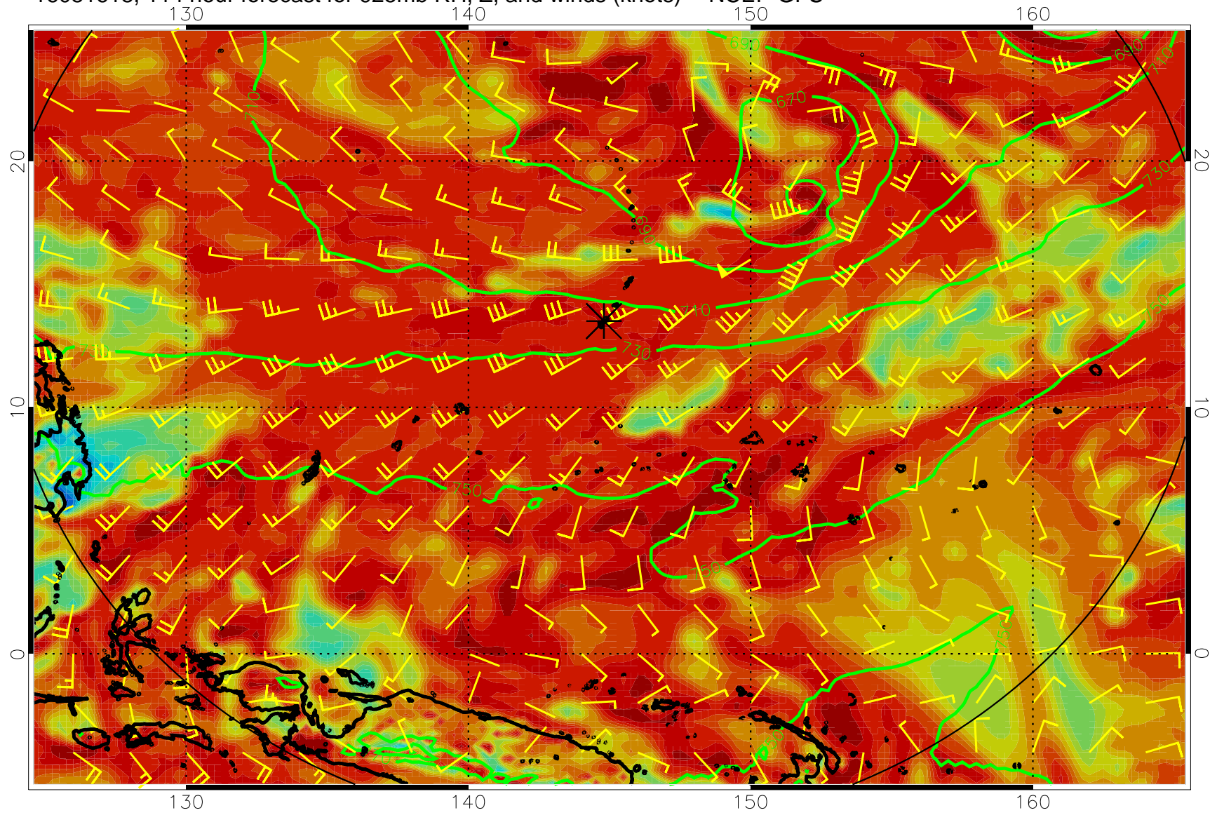
16081618, 114 hour forecast for 925mb RH, Z, and winds (knots) -- NCEP GFS
