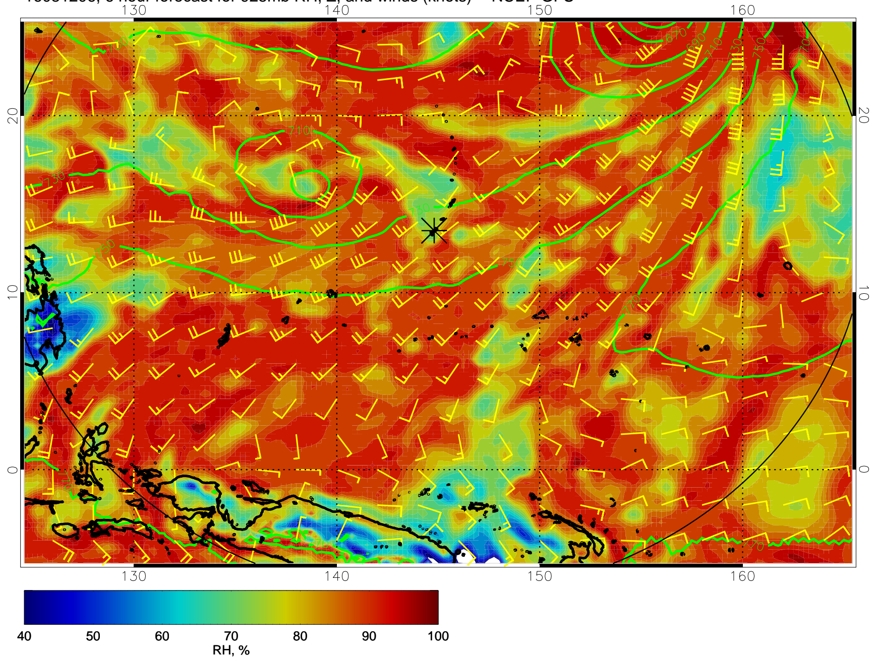
16081206, 6 hour forecast for 925mb RH, Z, and winds (knots) -- NCEP GFS
