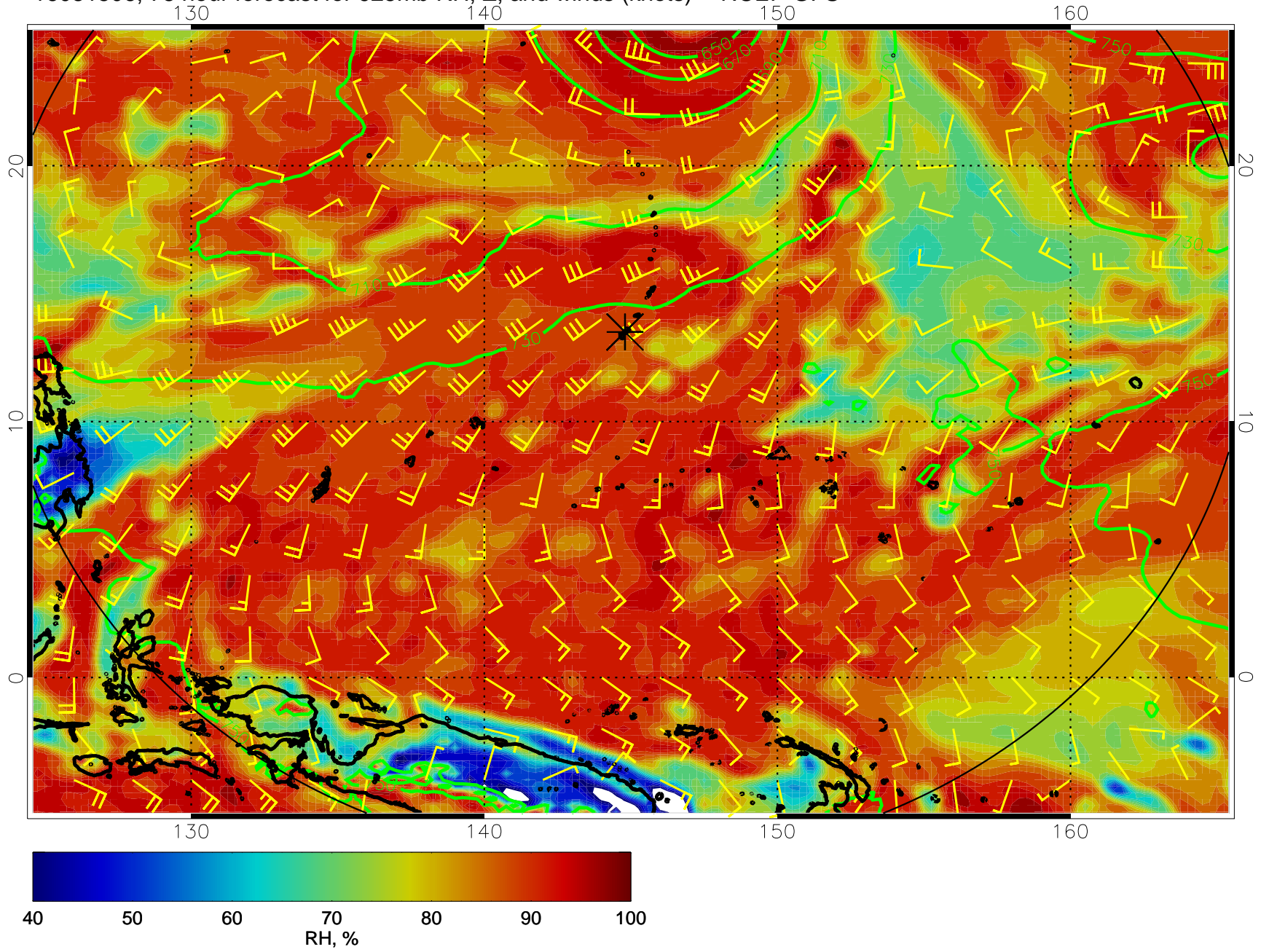
16081506, 78 hour forecast for 925mb RH, Z, and winds (knots) -- NCEP GFS
