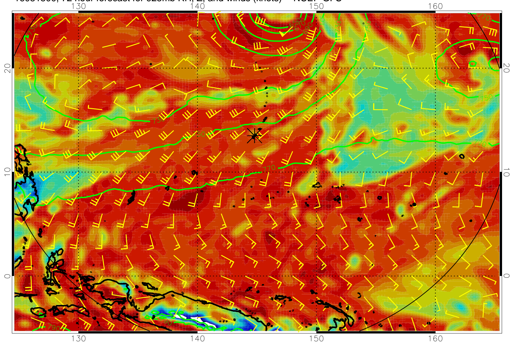
16081500, 72 hour forecast for 925mb RH, Z, and winds (knots) -- NCEP GFS
