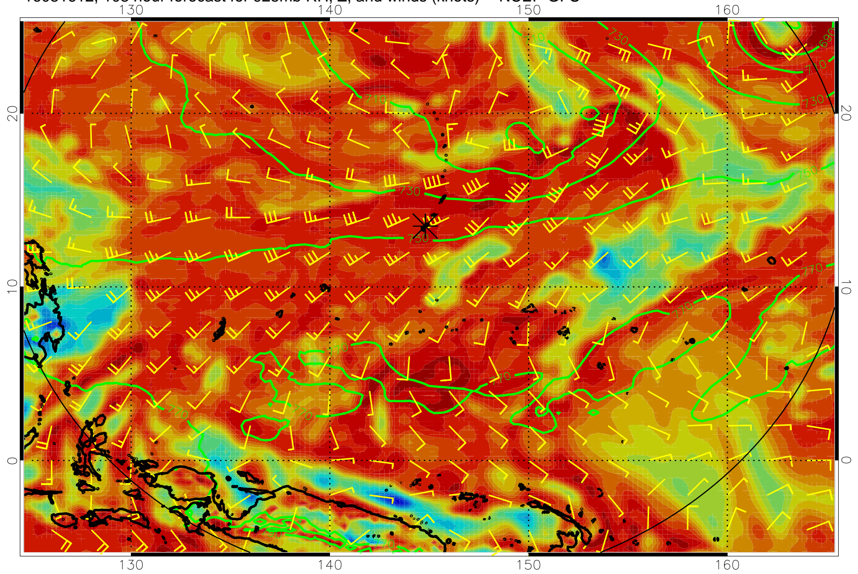
16081612, 108 hour forecast for 925mb RH, Z, and winds (knots) -- NCEP GFS
