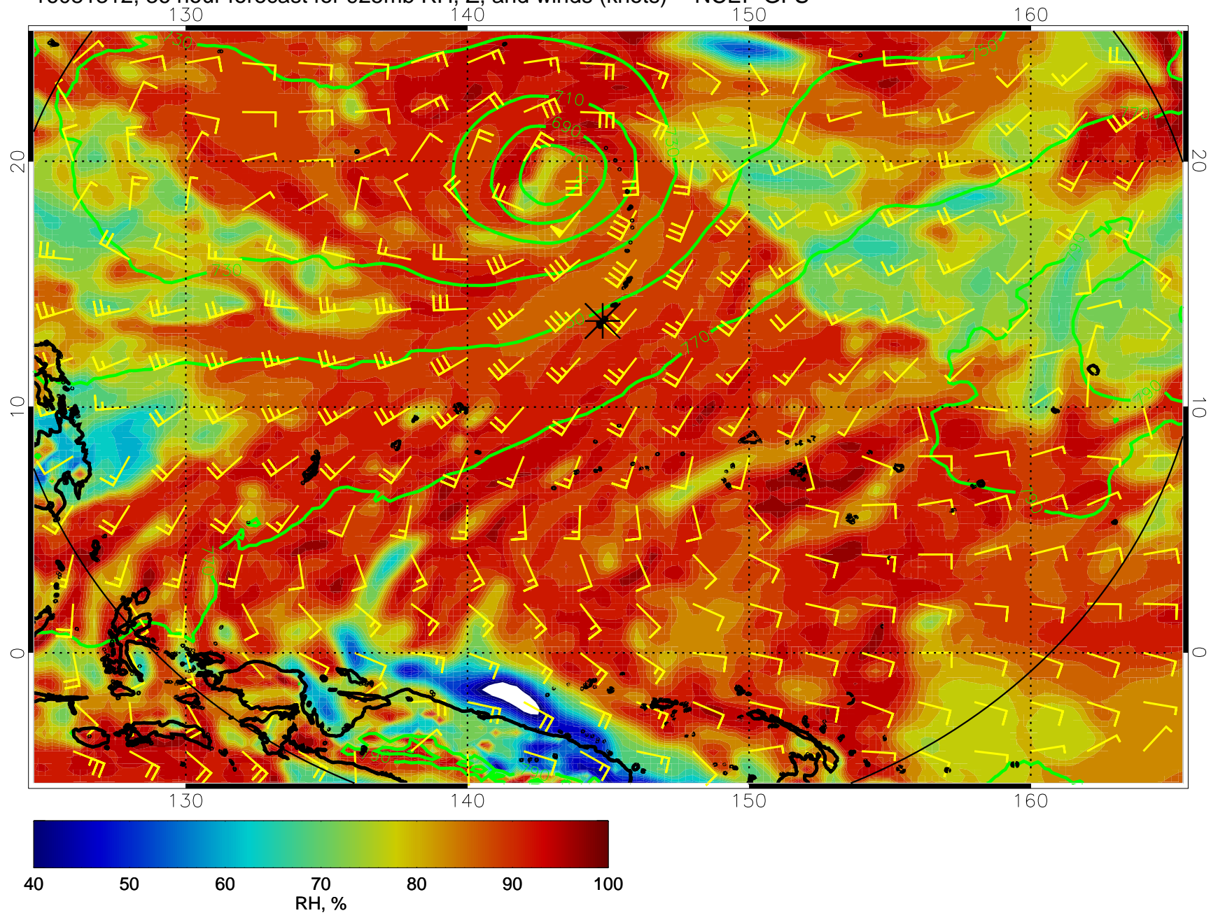
16081312, 36 hour forecast for 925mb RH, Z, and winds (knots) -- NCEP GFS
