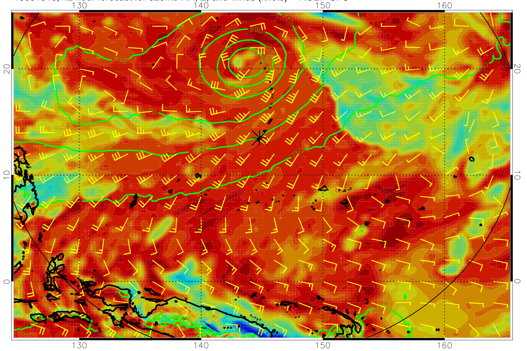
16081318, 42 hour forecast for 925mb RH, Z, and winds (knots) -- NCEP GFS
