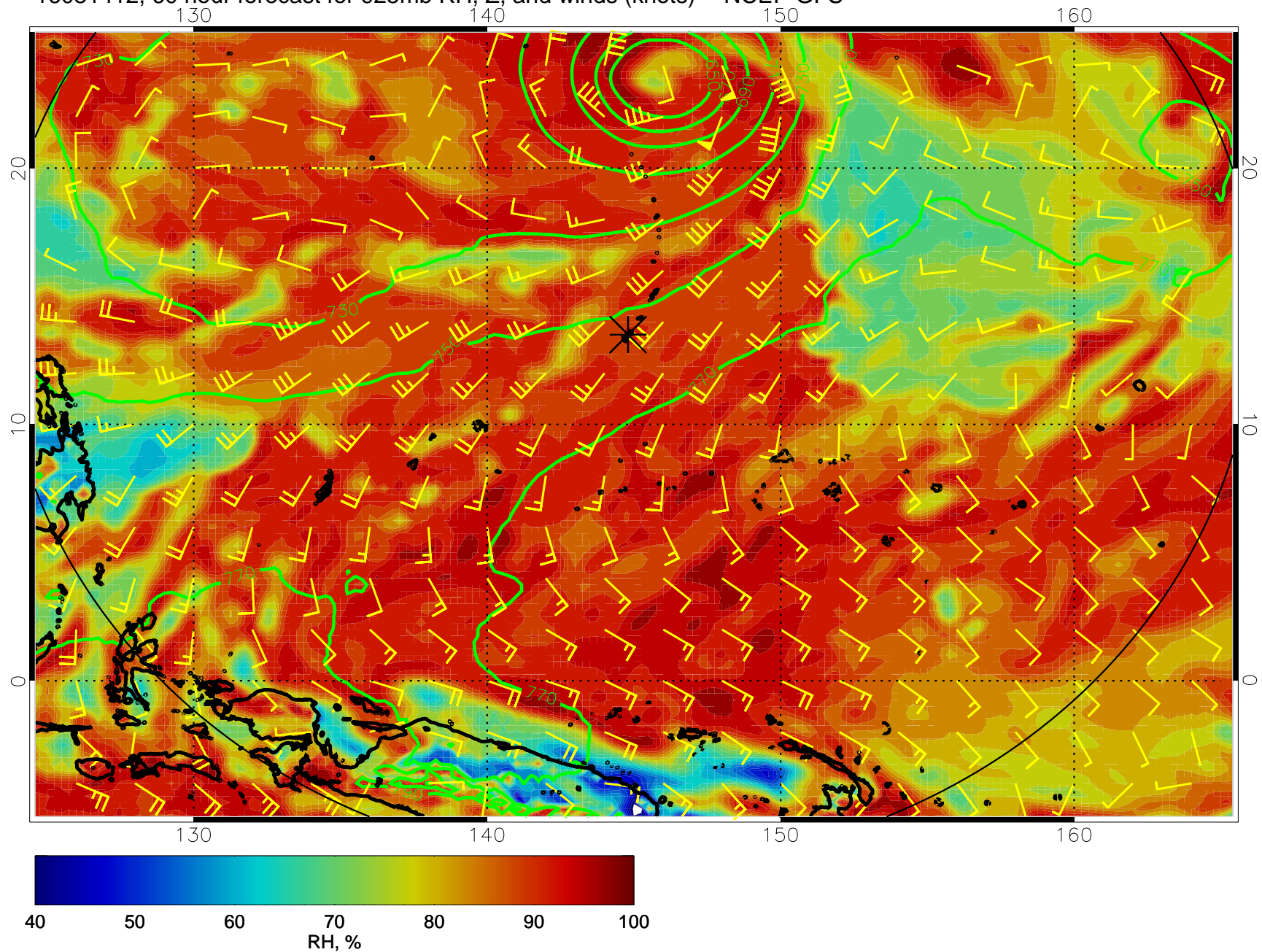
16081412, 60 hour forecast for 925mb RH, Z, and winds (knots) -- NCEP GFS
