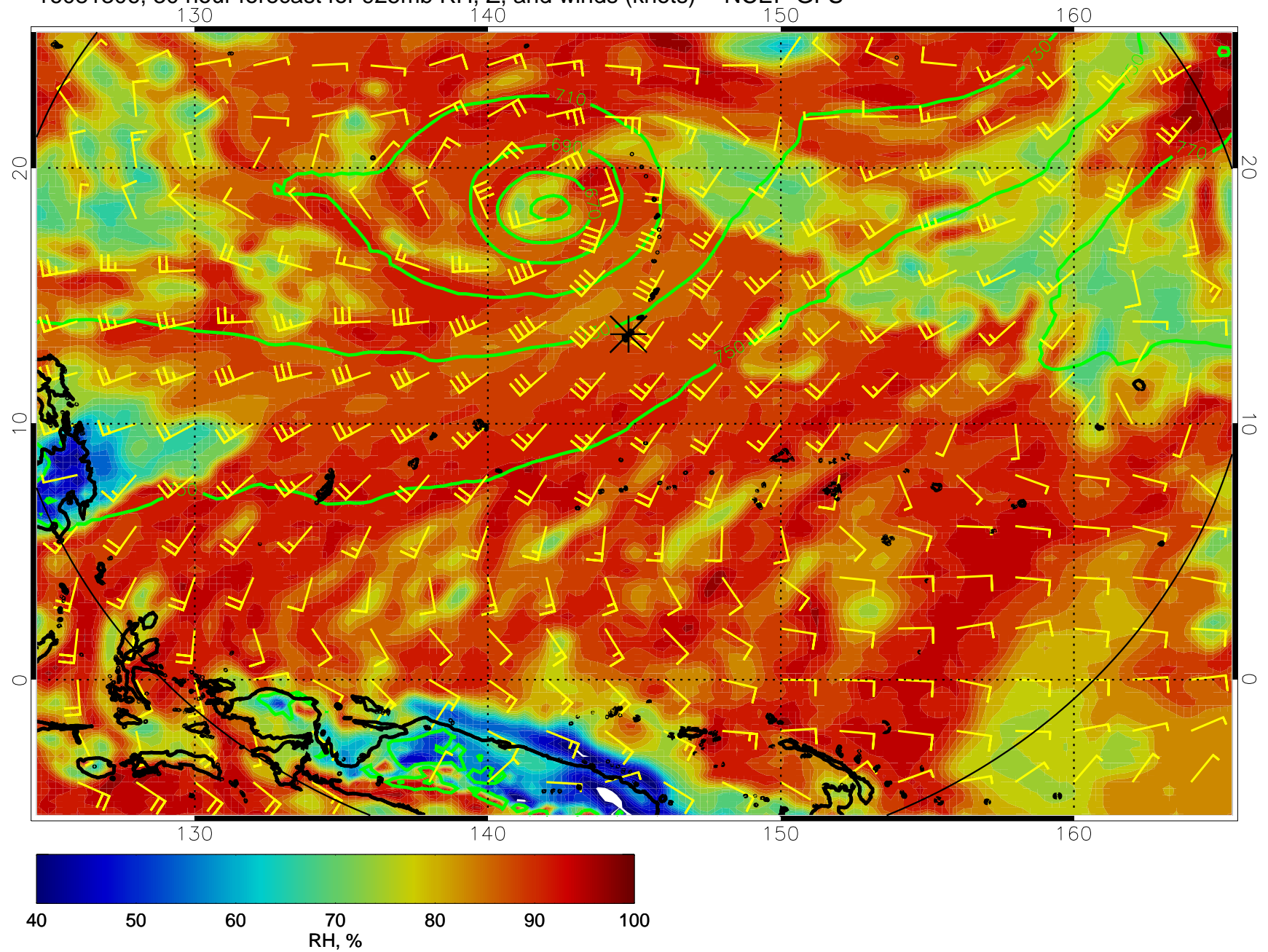
16081306, 30 hour forecast for 925mb RH, Z, and winds (knots) -- NCEP GFS
