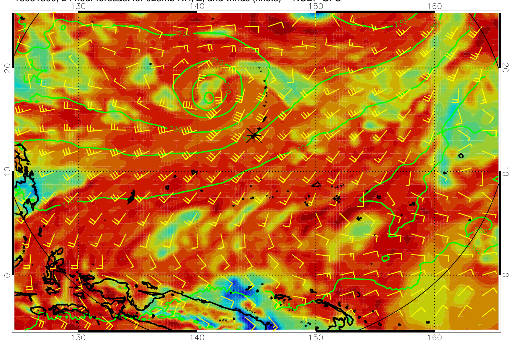
16081300, 24 hour forecast for 925mb RH, Z, and winds (knots) -- NCEP GFS
