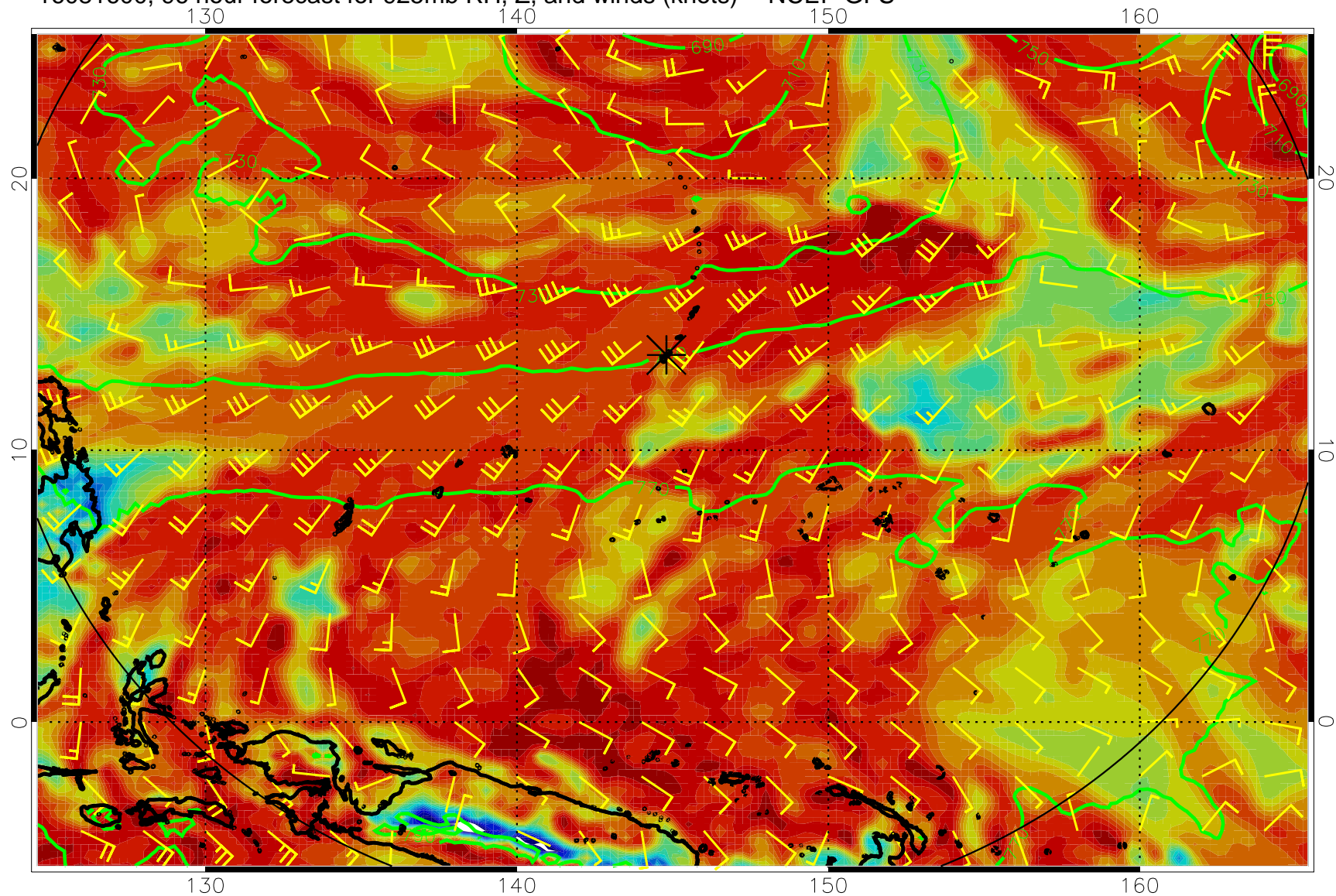
16081600, 96 hour forecast for 925mb RH, Z, and winds (knots) -- NCEP GFS
