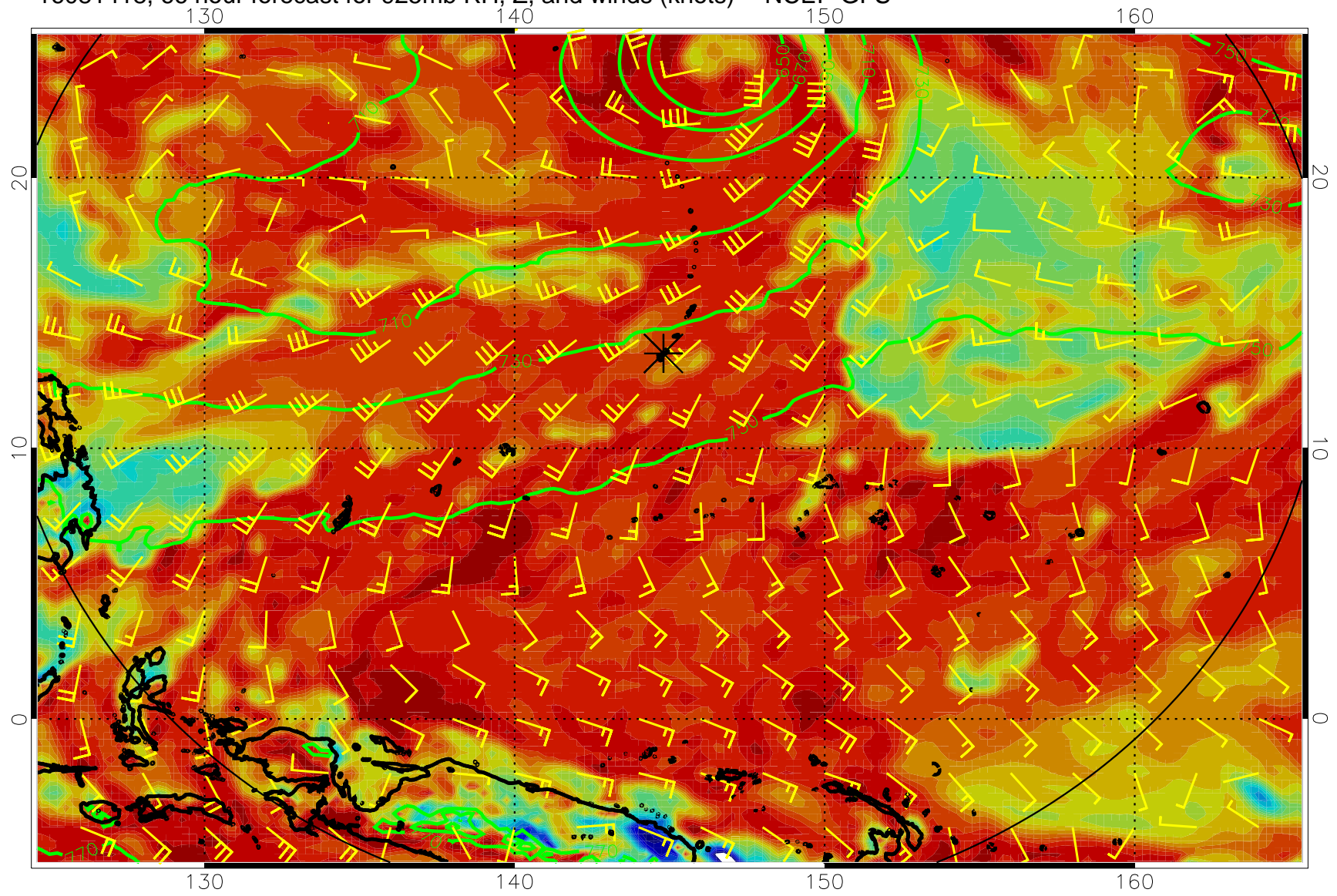
16081418, 66 hour forecast for 925mb RH, Z, and winds (knots) -- NCEP GFS
