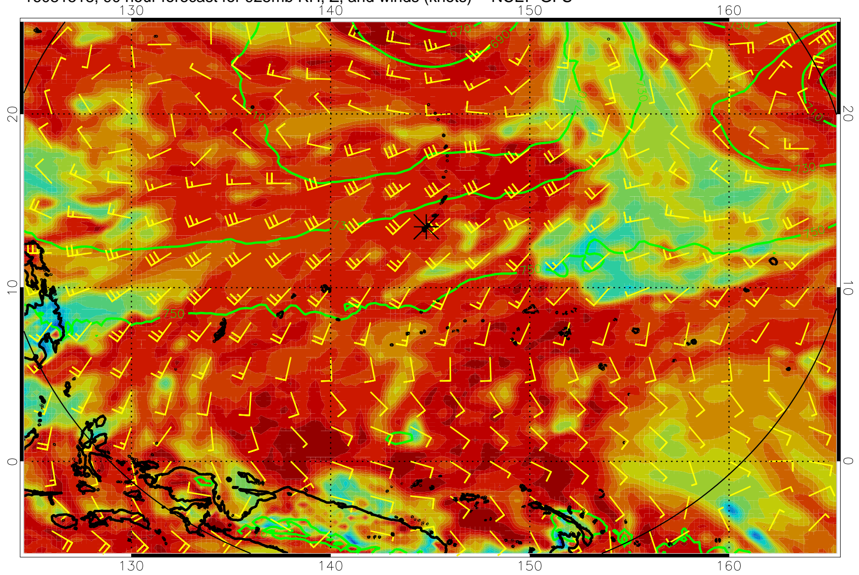
16081518, 90 hour forecast for 925mb RH, Z, and winds (knots) -- NCEP GFS
