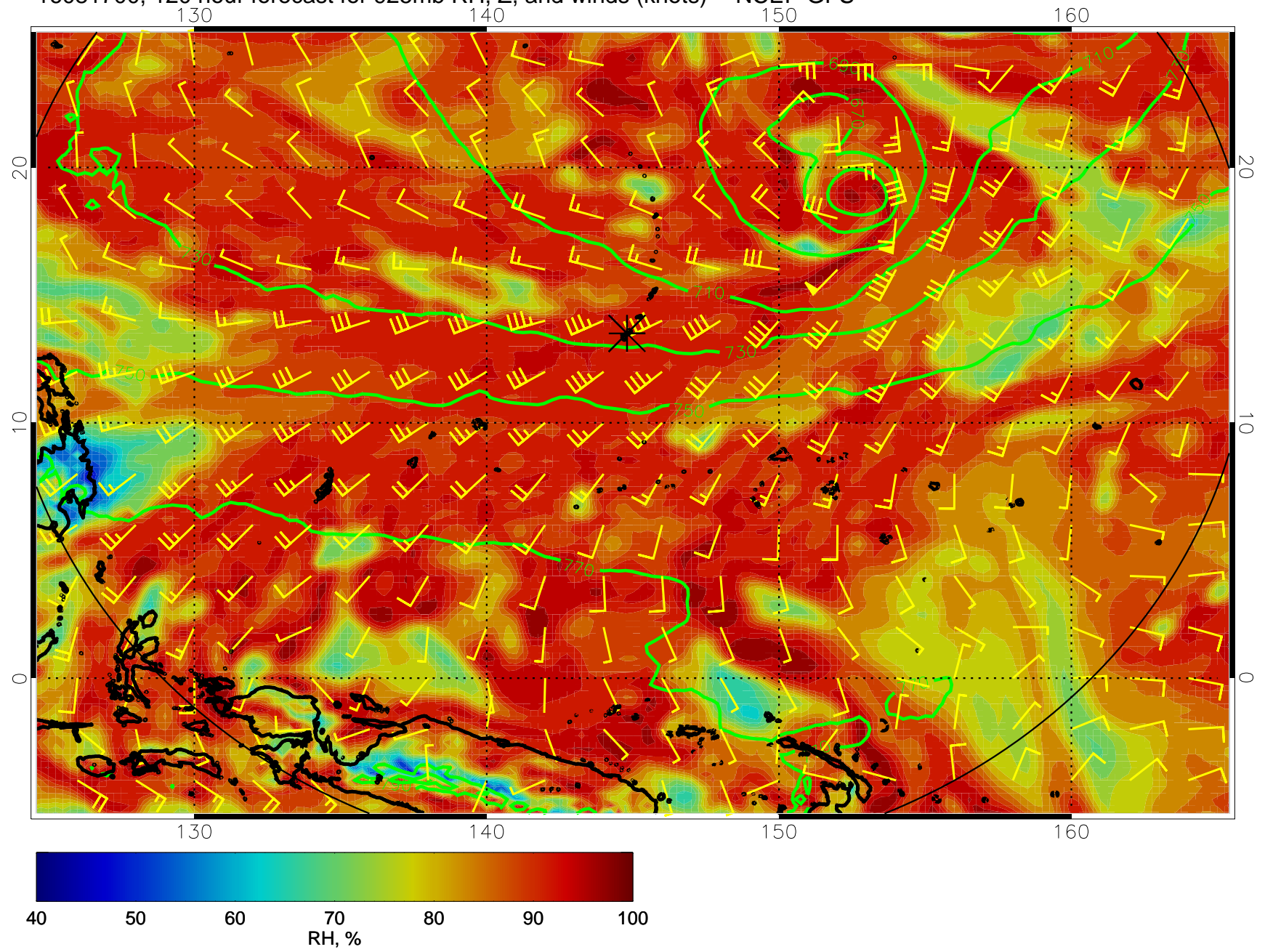
16081700, 120 hour forecast for 925mb RH, Z, and winds (knots) -- NCEP GFS
