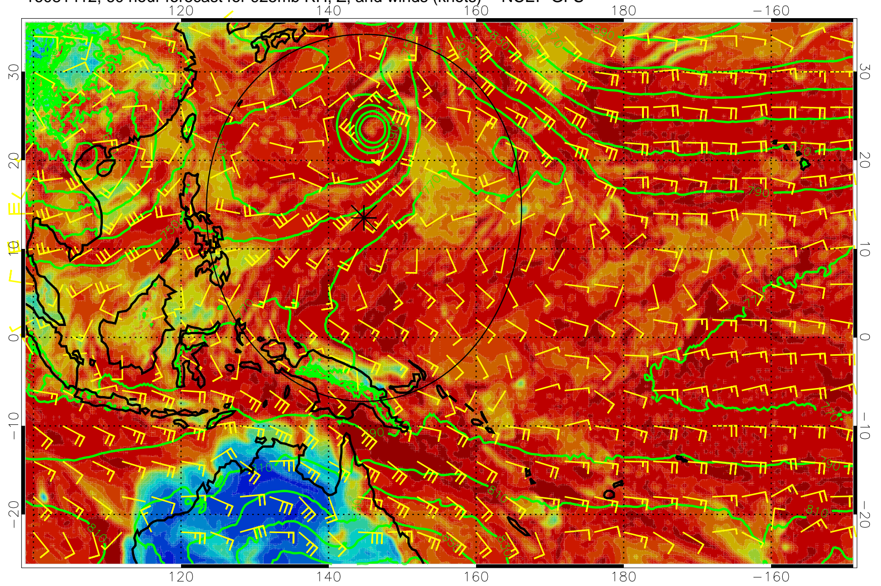
16081412, 60 hour forecast for 925mb RH, Z, and winds (knots) -- NCEP GFS
