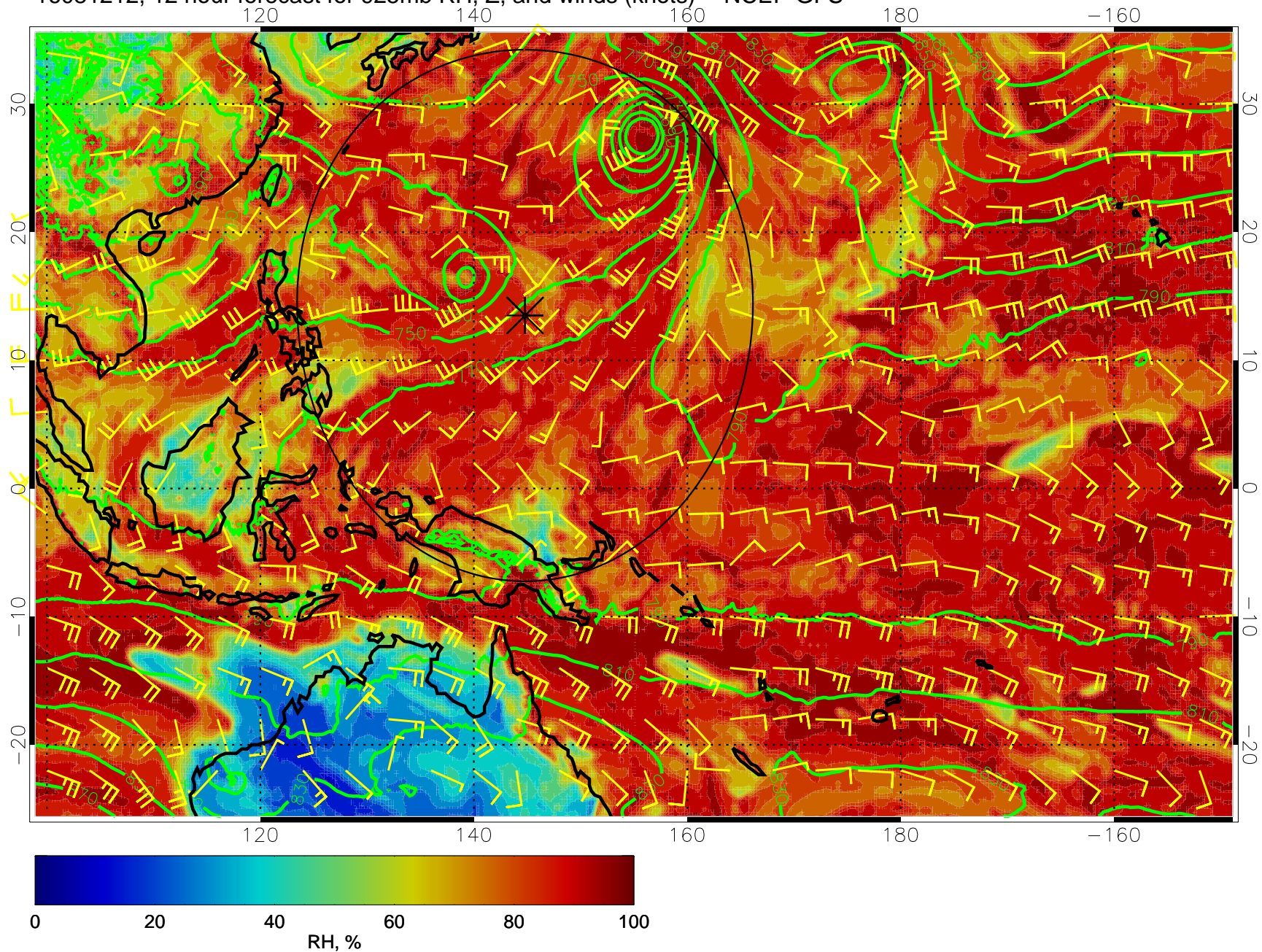
16081212, 12 hour forecast for 925mb RH, Z, and winds (knots) -- NCEP GFS
