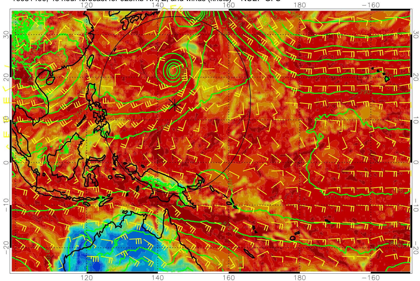
16081400, 48 hour forecast for 925mb RH, Z, and winds (knots) -- NCEP GFS
