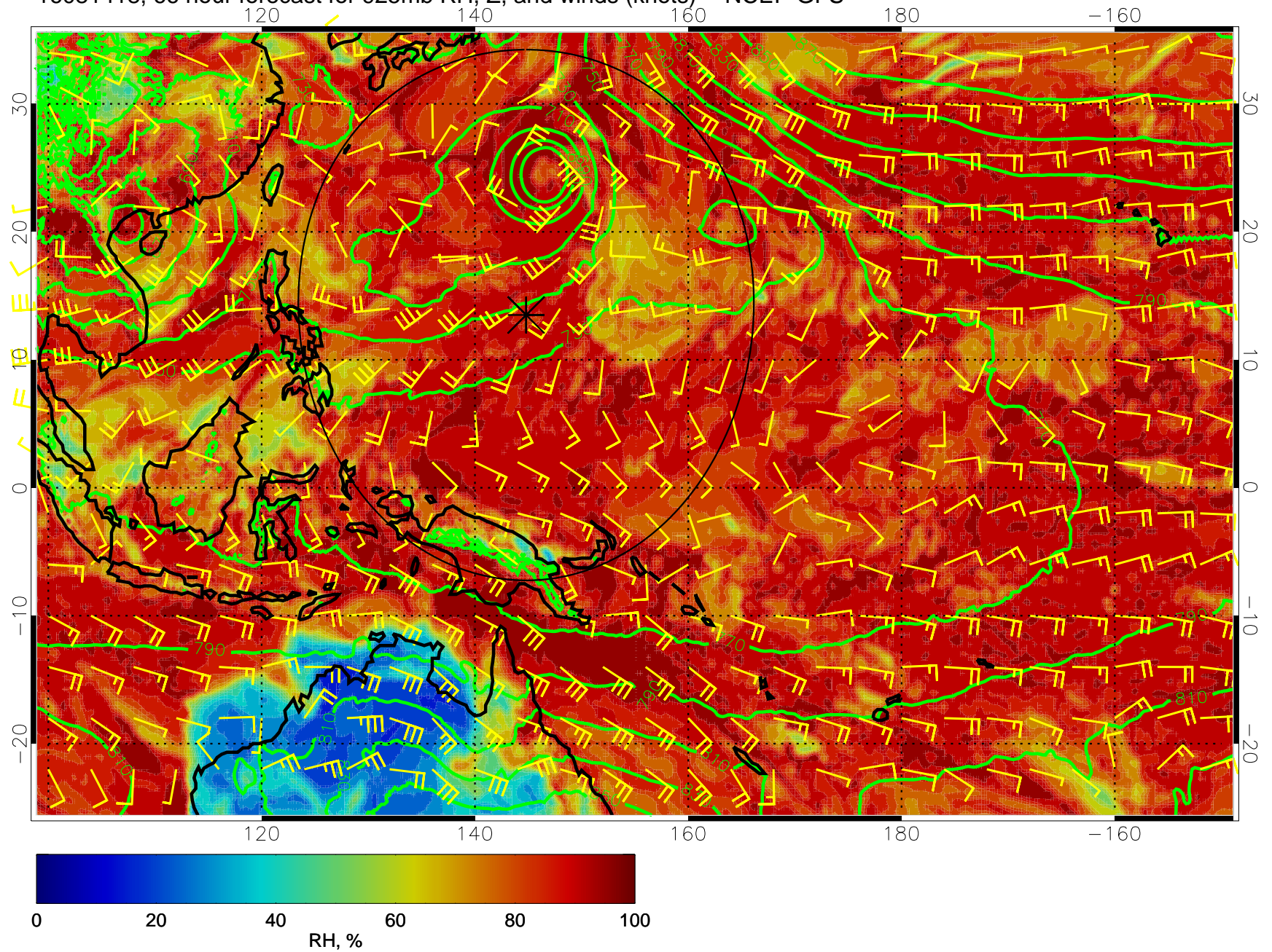
16081418, 66 hour forecast for 925mb RH, Z, and winds (knots) -- NCEP GFS
