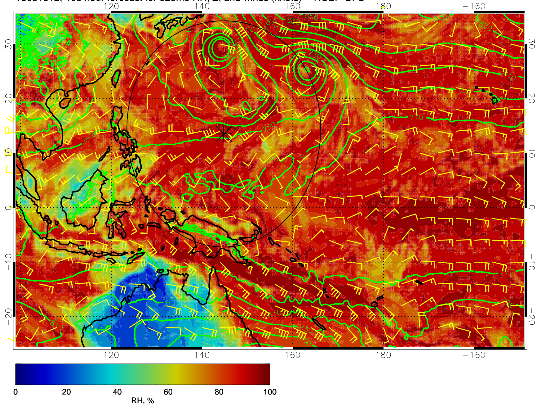
16081612, 108 hour forecast for 925mb RH, Z, and winds (knots) -- NCEP GFS
