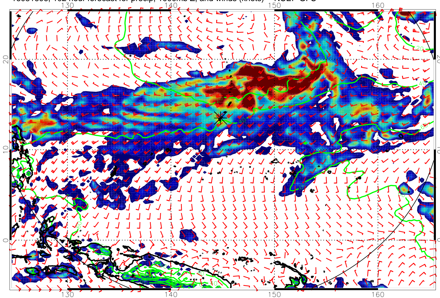
16081606, 102 hour forecast for precip, 1000mb Z, and winds (knots) -- NCEP GFS
