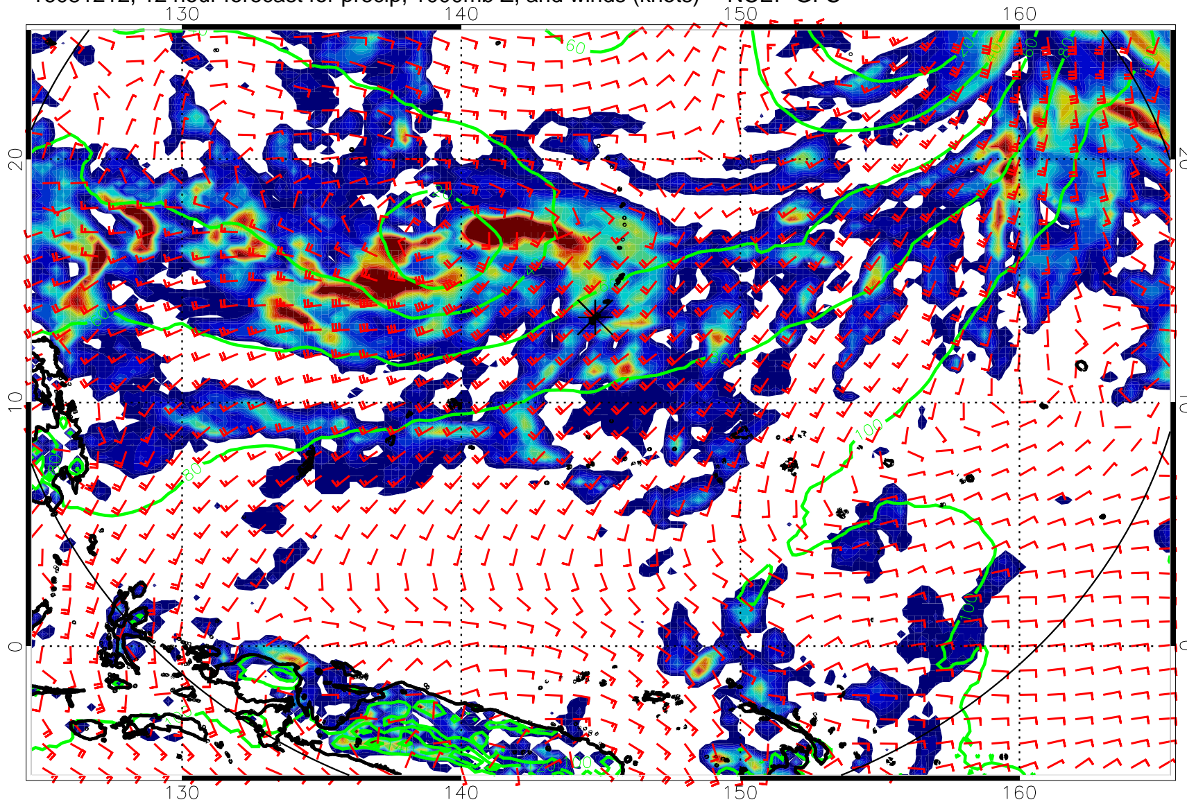
16081212, 12 hour forecast for precip, 1000mb Z, and winds (knots) -- NCEP GFS
