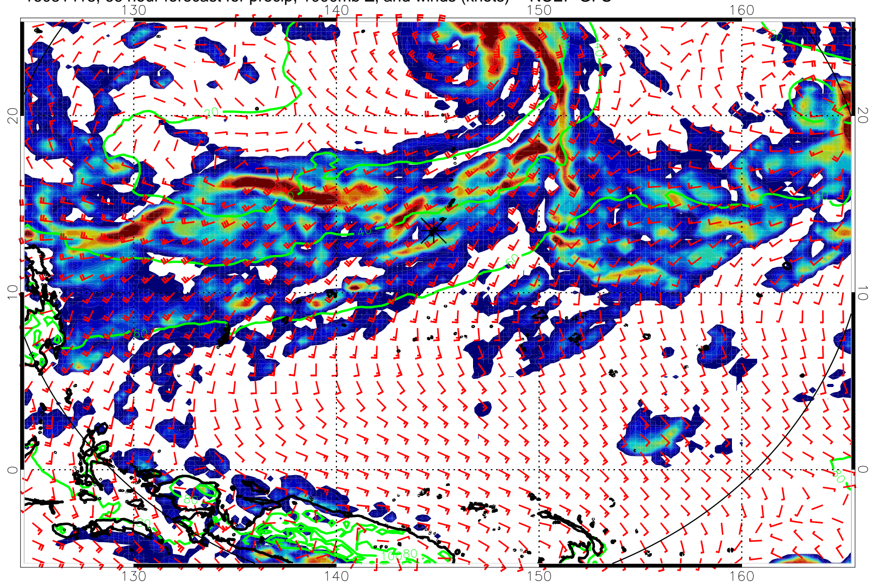
16081418, 66 hour forecast for precip, 1000mb Z, and winds (knots) -- NCEP GFS
