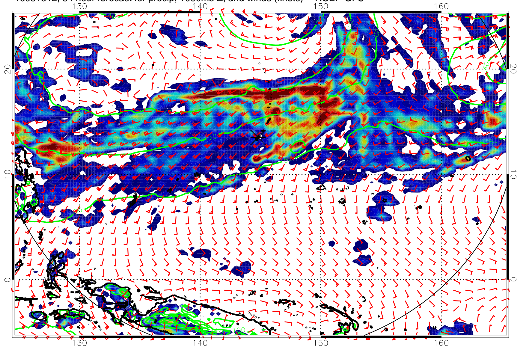
16081512, 84 hour forecast for precip, 1000mb Z, and winds (knots) -- NCEP GFS
