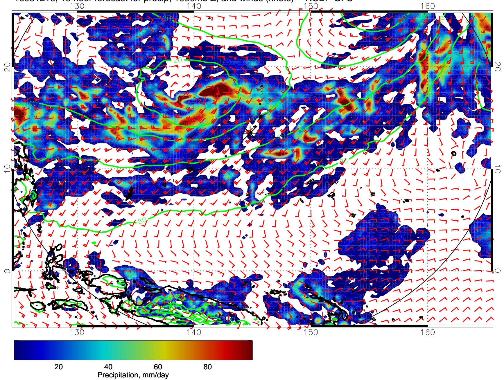
16081218, 18 hour forecast for precip, 1000mb Z, and winds (knots) -- NCEP GFS
