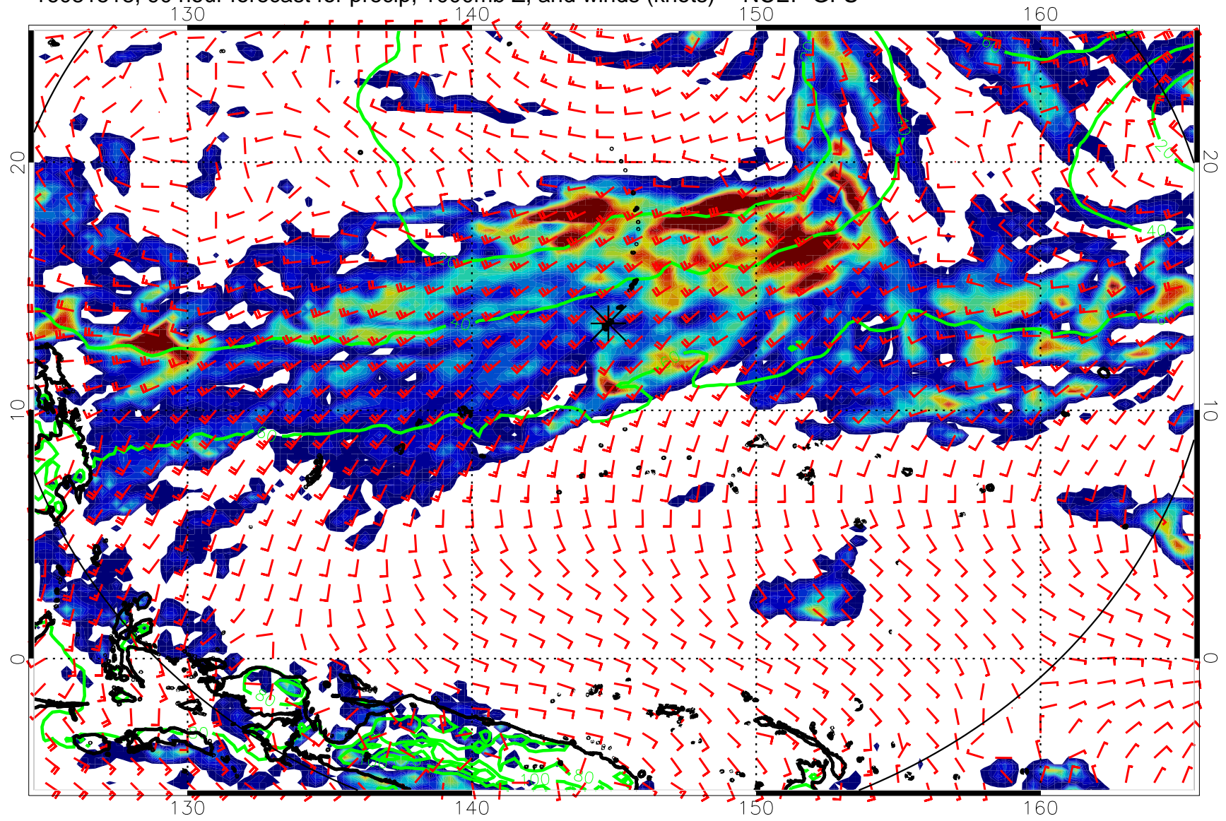
16081518, 90 hour forecast for precip, 1000mb Z, and winds (knots) -- NCEP GFS
