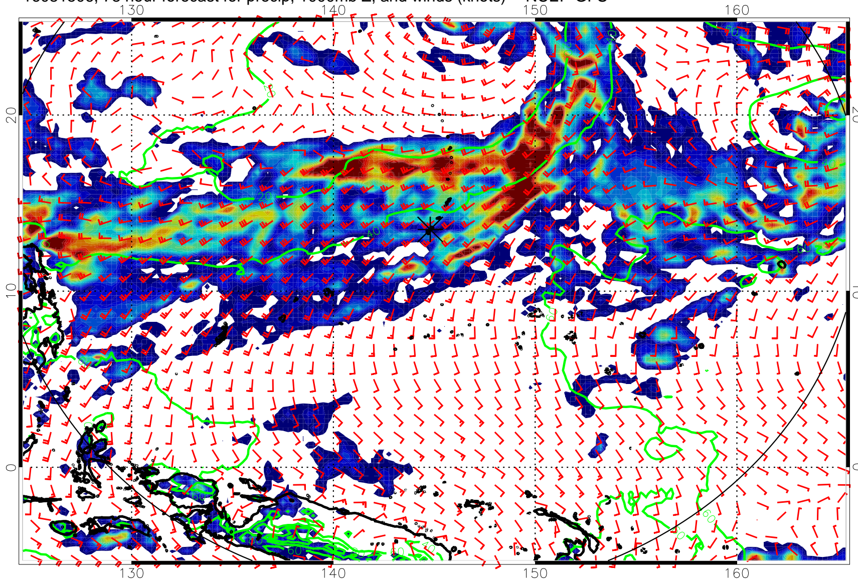
16081506, 78 hour forecast for precip, 1000mb Z, and winds (knots) -- NCEP GFS
