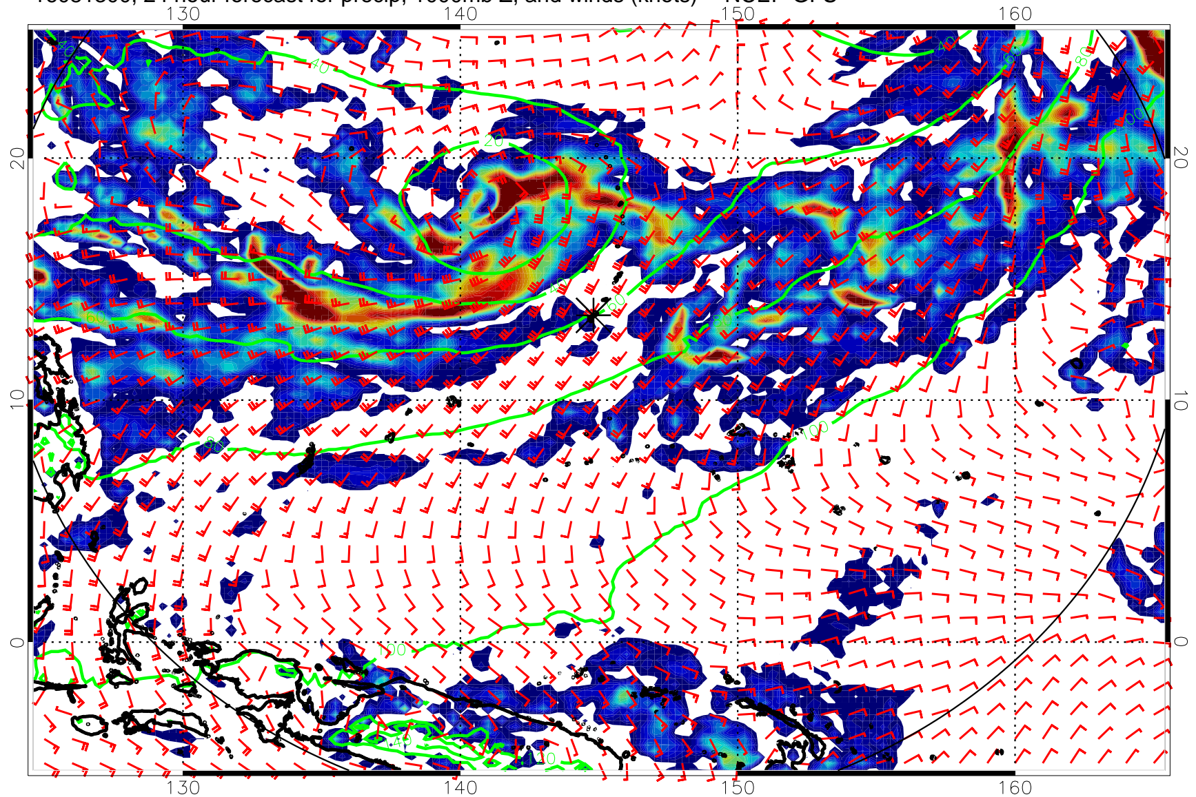
16081300, 24 hour forecast for precip, 1000mb Z, and winds (knots) -- NCEP GFS
