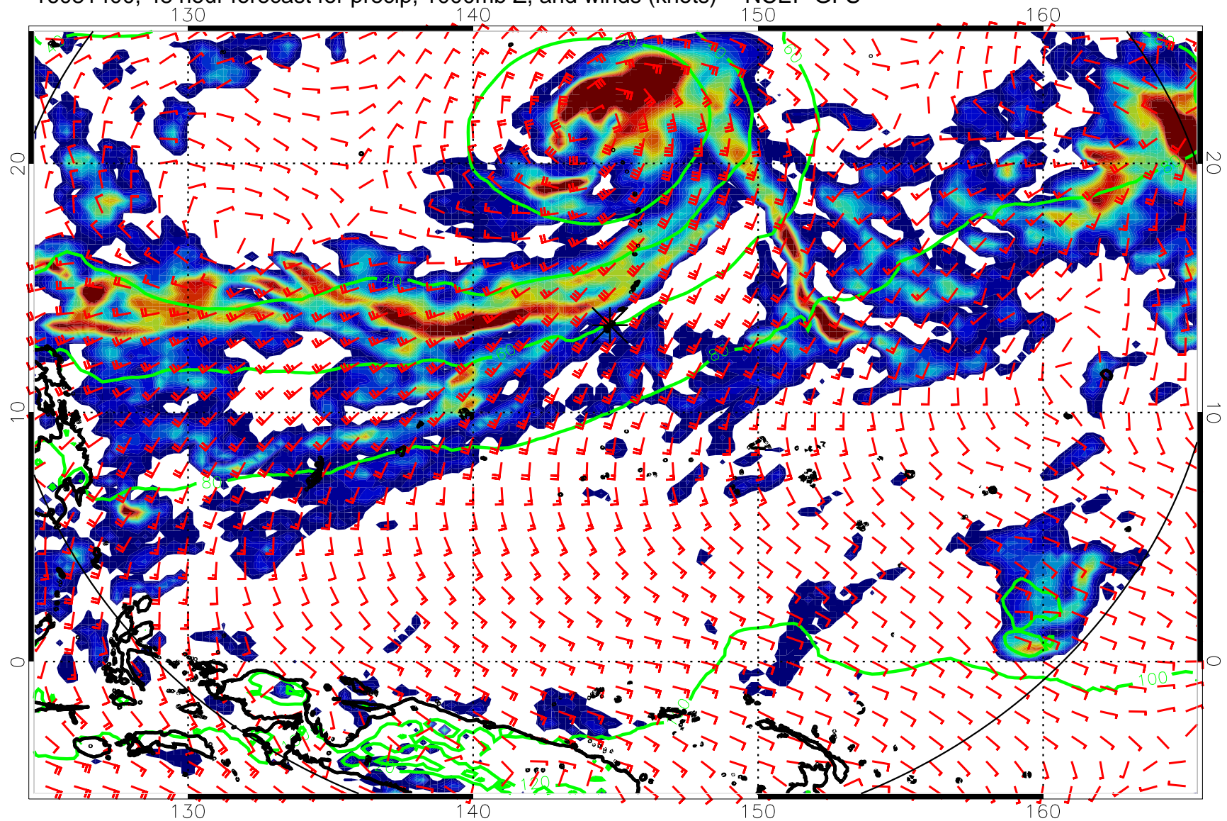
16081400, 48 hour forecast for precip, 1000mb Z, and winds (knots) -- NCEP GFS
