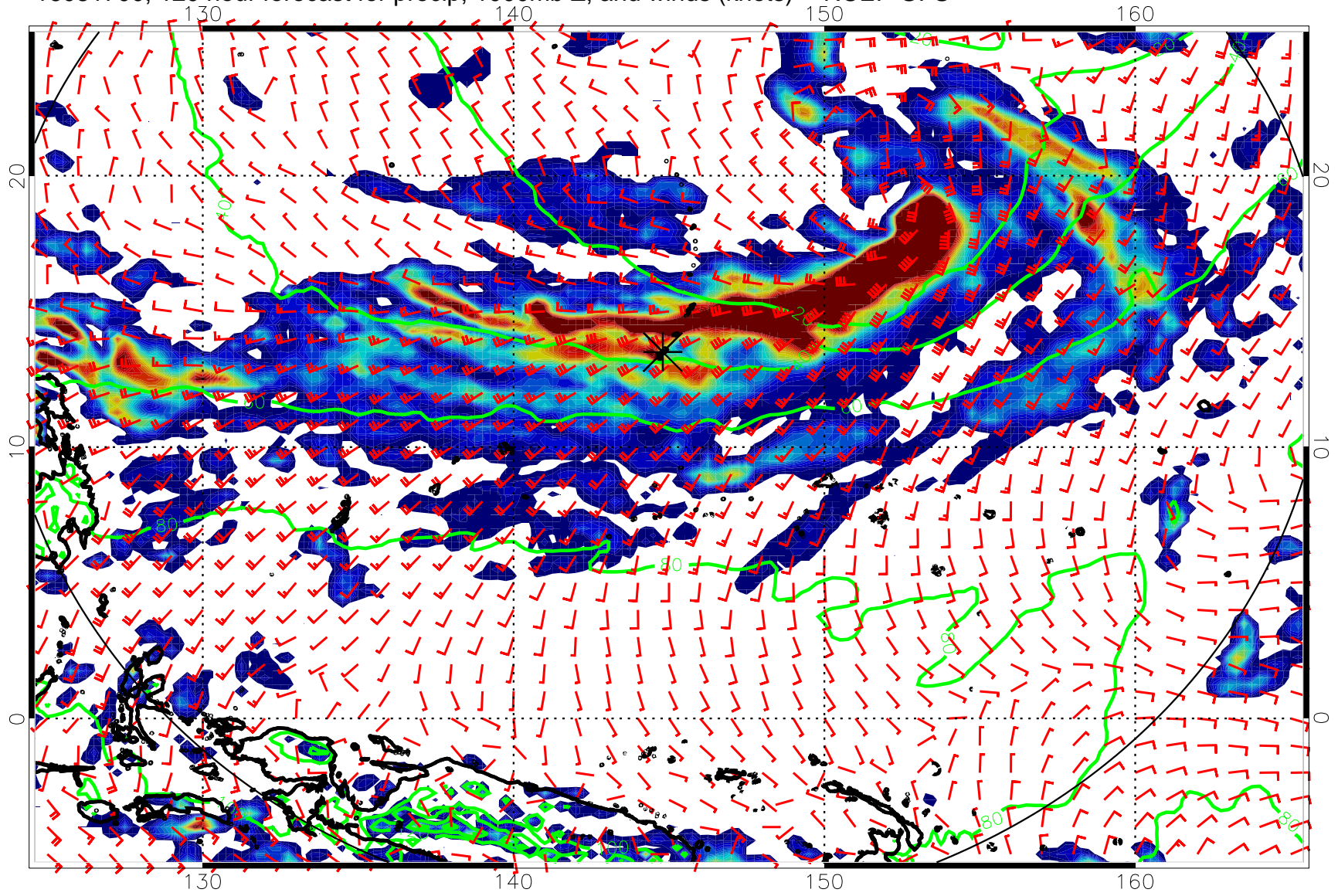
16081700, 120 hour forecast for precip, 1000mb Z, and winds (knots) -- NCEP GFS
