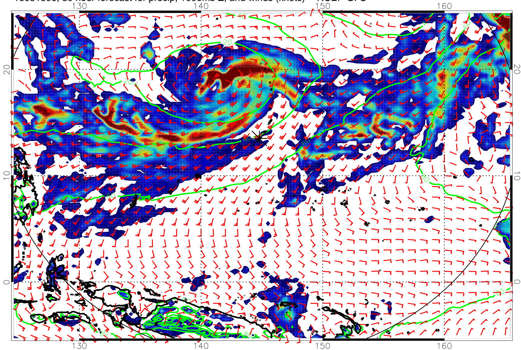
16081306, 30 hour forecast for precip, 1000mb Z, and winds (knots) -- NCEP GFS
