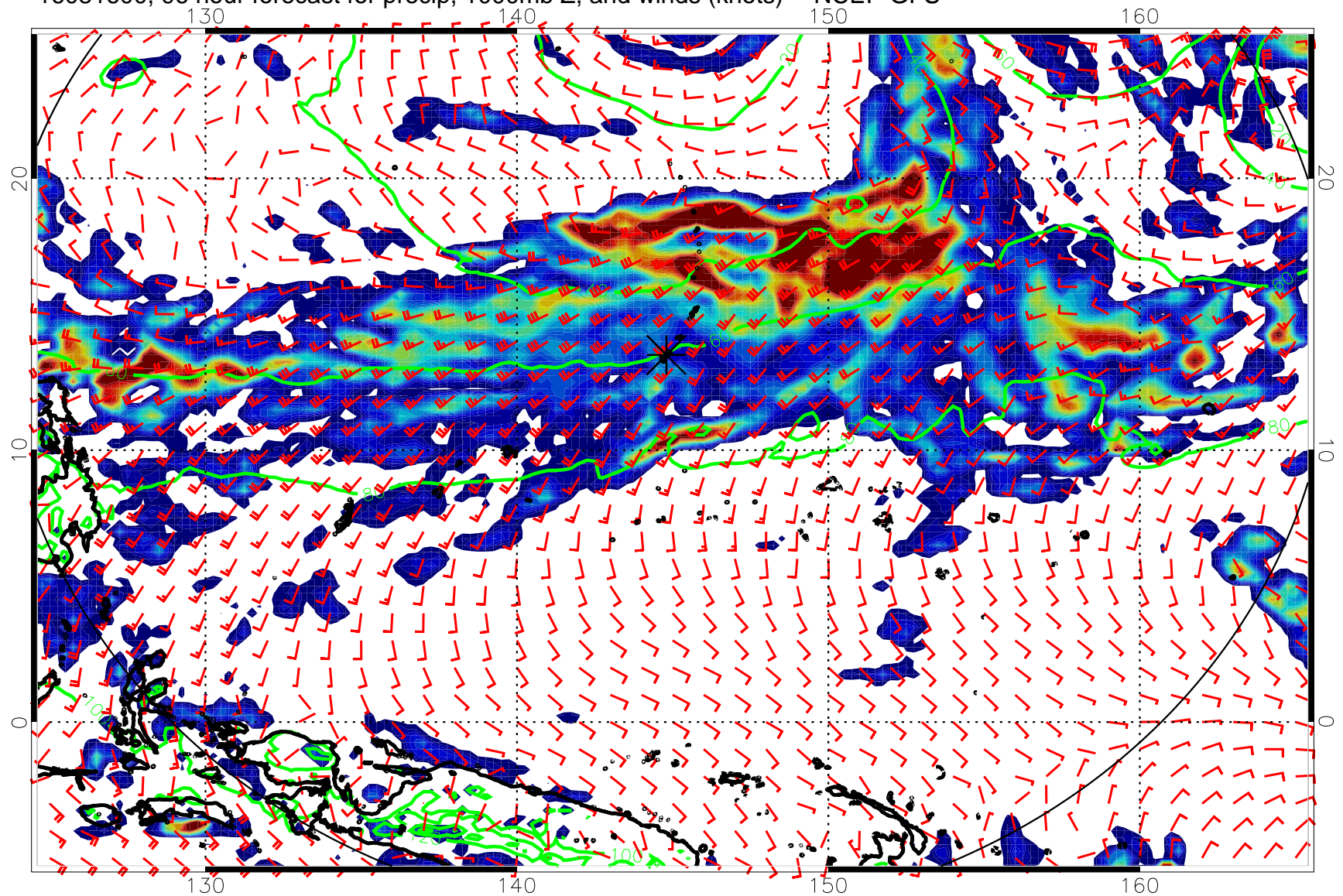
16081600, 96 hour forecast for precip, 1000mb Z, and winds (knots) -- NCEP GFS
