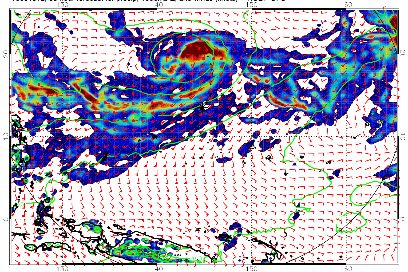
16081312, 36 hour forecast for precip, 1000mb Z, and winds (knots) -- NCEP GFS
