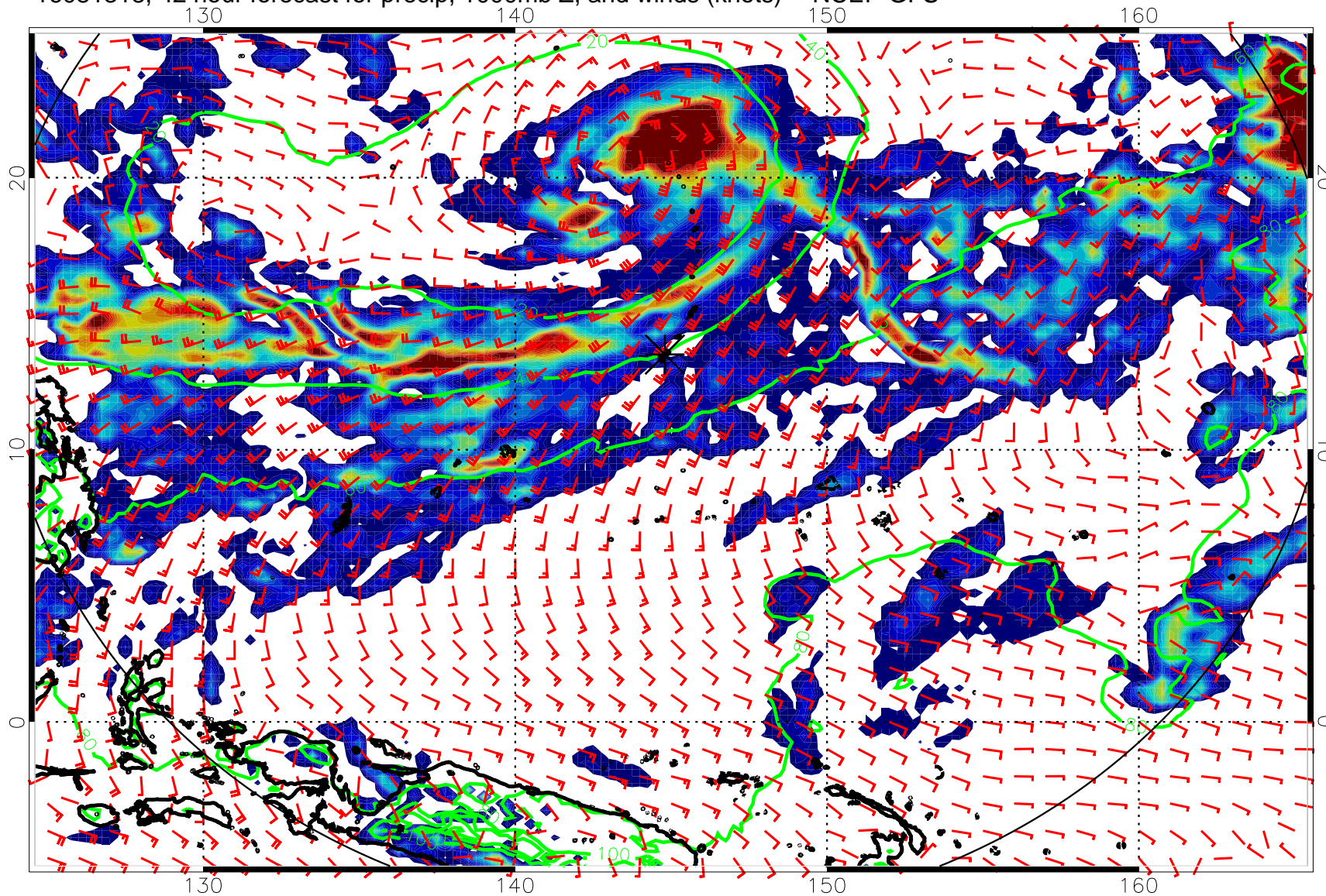
16081318, 42 hour forecast for precip, 1000mb Z, and winds (knots) -- NCEP GFS
