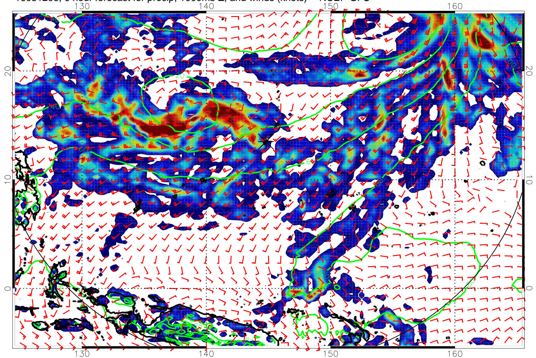
16081206, 6 hour forecast for precip, 1000mb Z, and winds (knots) -- NCEP GFS
