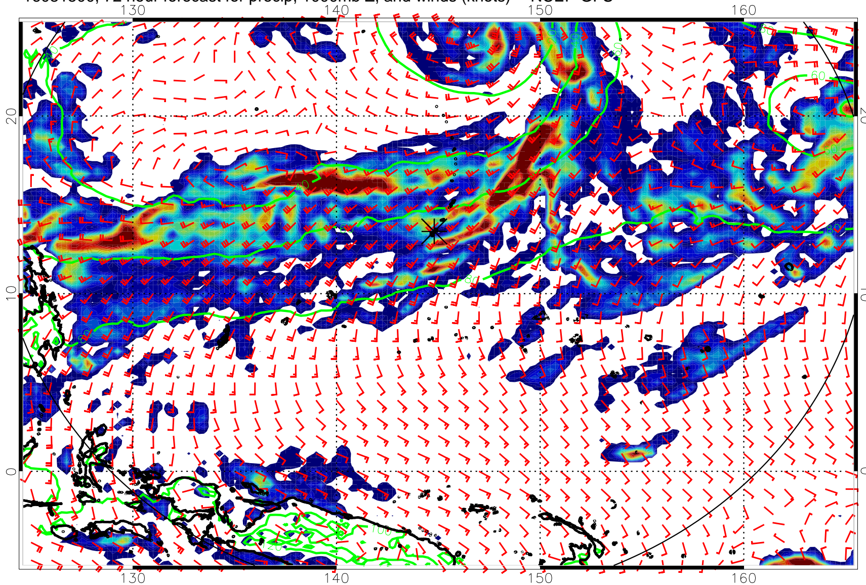
16081500, 72 hour forecast for precip, 1000mb Z, and winds (knots) -- NCEP GFS
