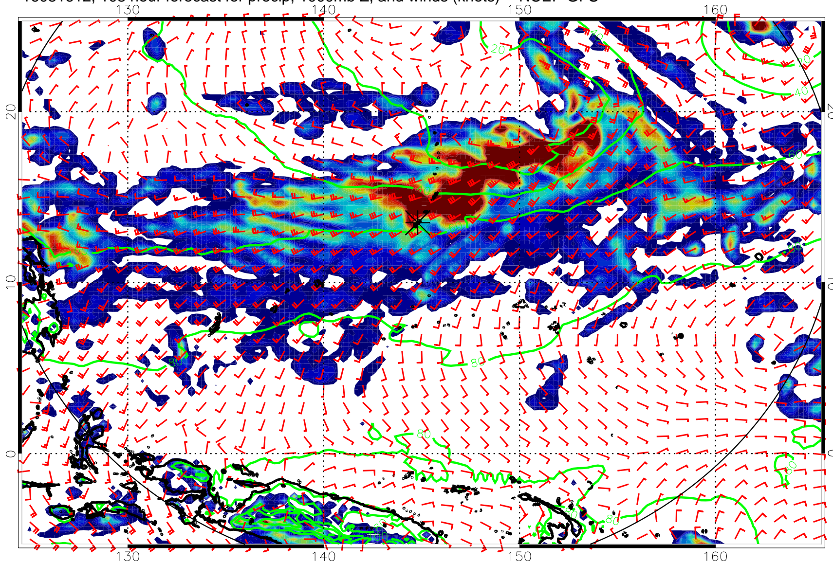
16081612, 108 hour forecast for precip, 1000mb Z, and winds (knots) -- NCEP GFS
