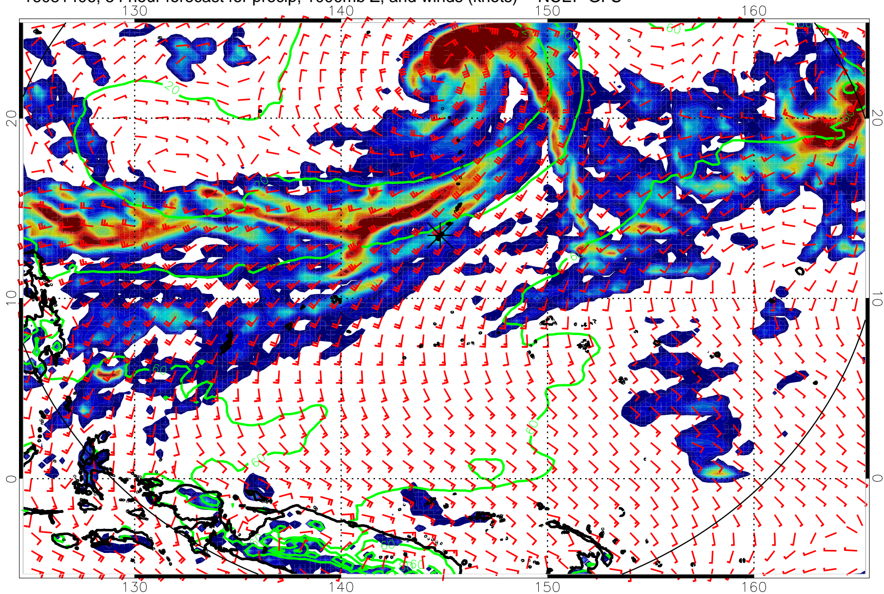
16081406, 54 hour forecast for precip, 1000mb Z, and winds (knots) -- NCEP GFS
