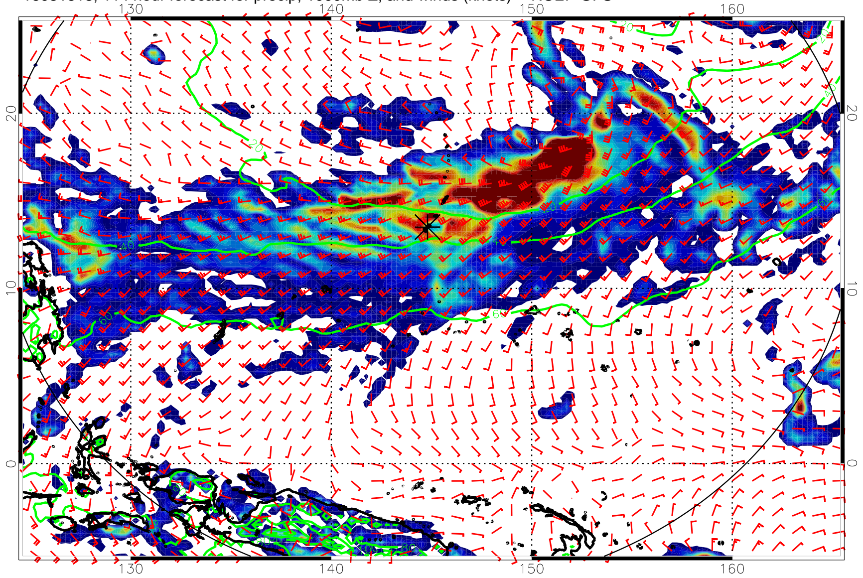
16081618, 114 hour forecast for precip, 1000mb Z, and winds (knots) -- NCEP GFS
