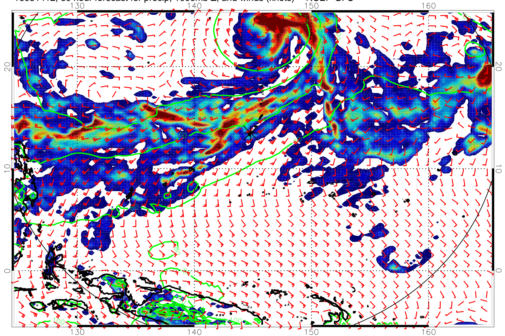
16081412, 60 hour forecast for precip, 1000mb Z, and winds (knots) -- NCEP GFS
