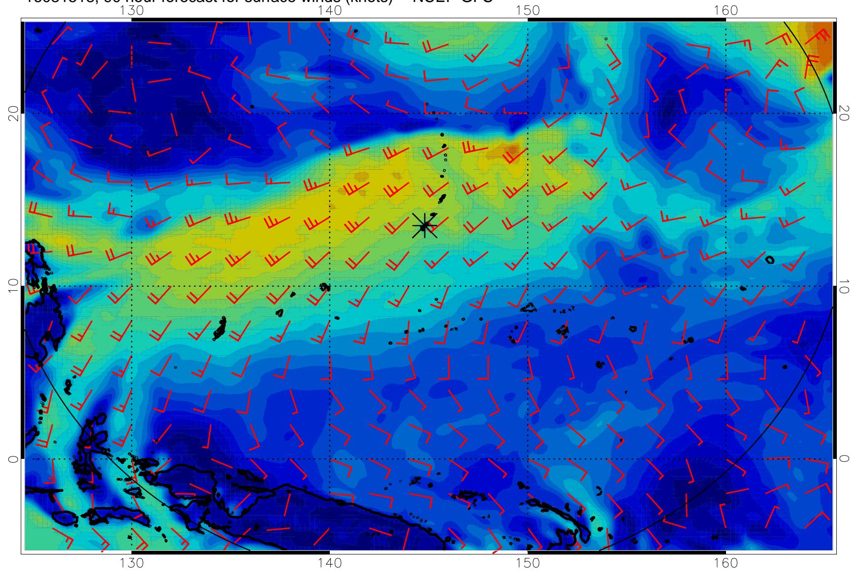
16081518, 90 hour forecast for surface winds (knots) -- NCEP GFS
