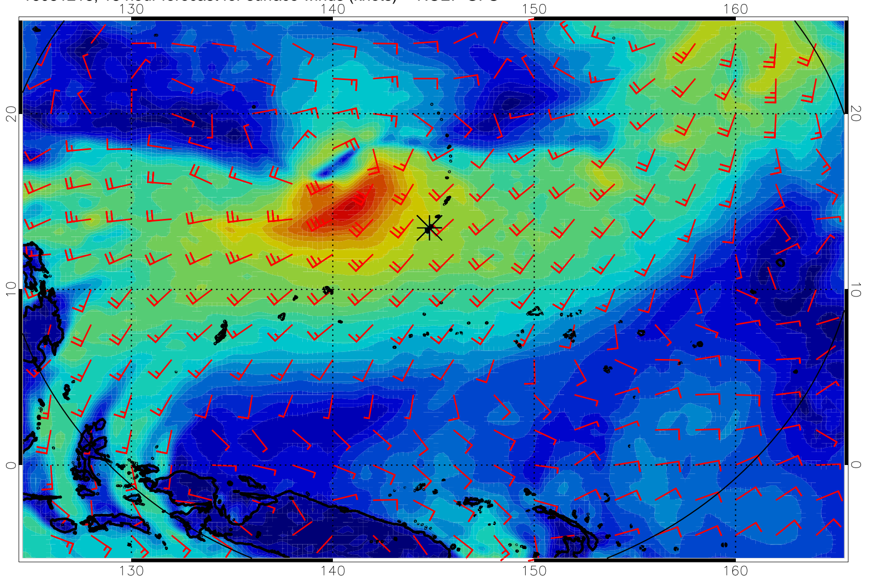
16081218, 18 hour forecast for surface winds (knots) -- NCEP GFS
