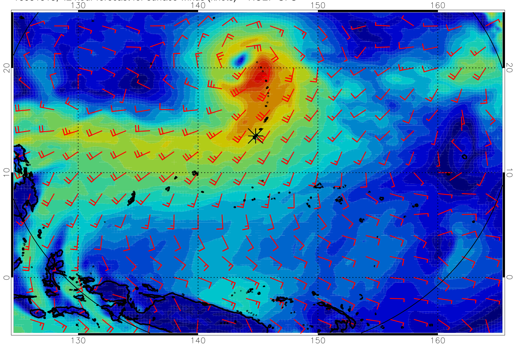
16081318, 42 hour forecast for surface winds (knots) -- NCEP GFS
