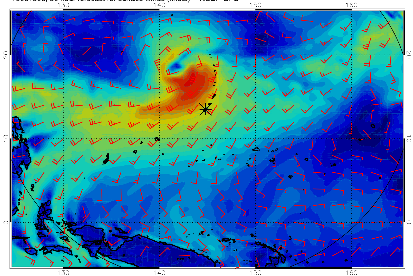
16081306, 30 hour forecast for surface winds (knots) -- NCEP GFS
