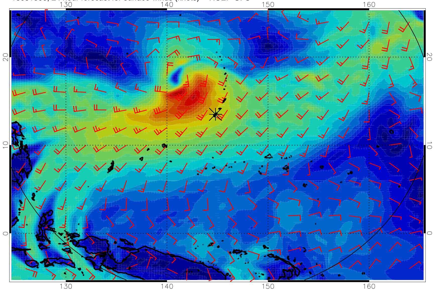
16081300, 24 hour forecast for surface winds (knots) -- NCEP GFS
