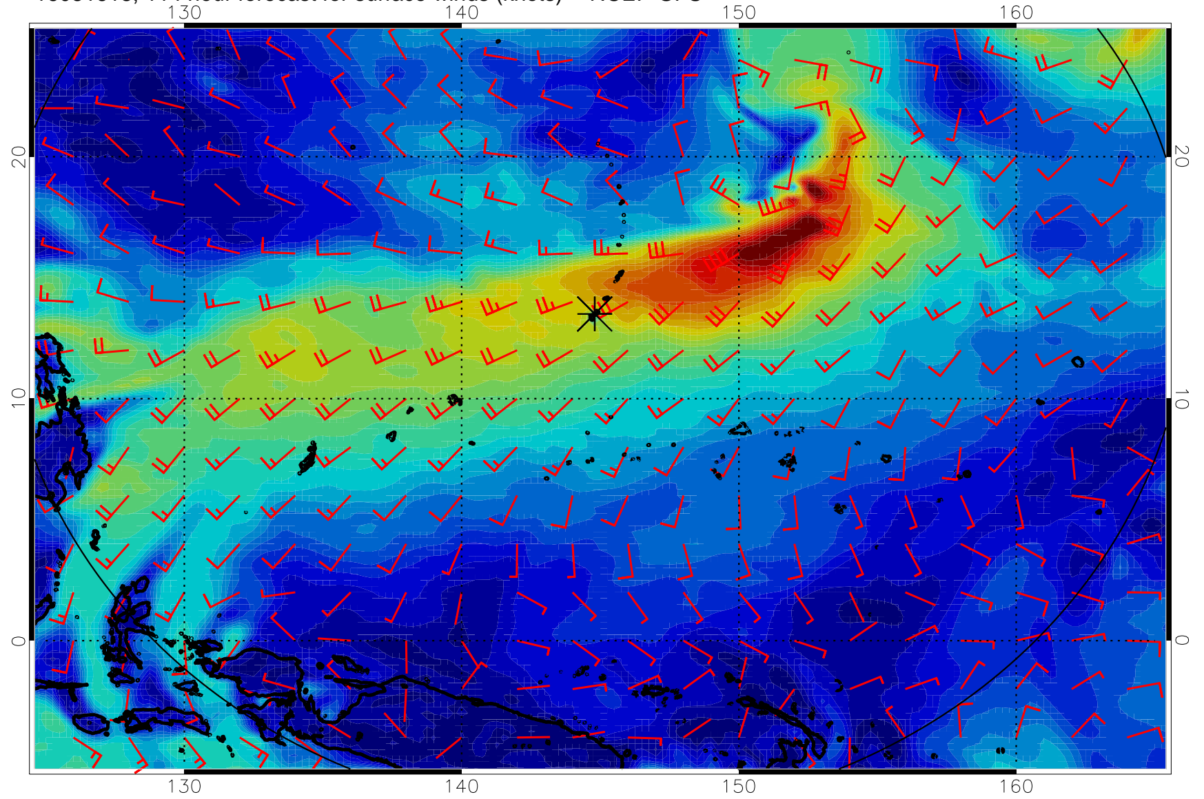
16081618, 114 hour forecast for surface winds (knots) -- NCEP GFS
