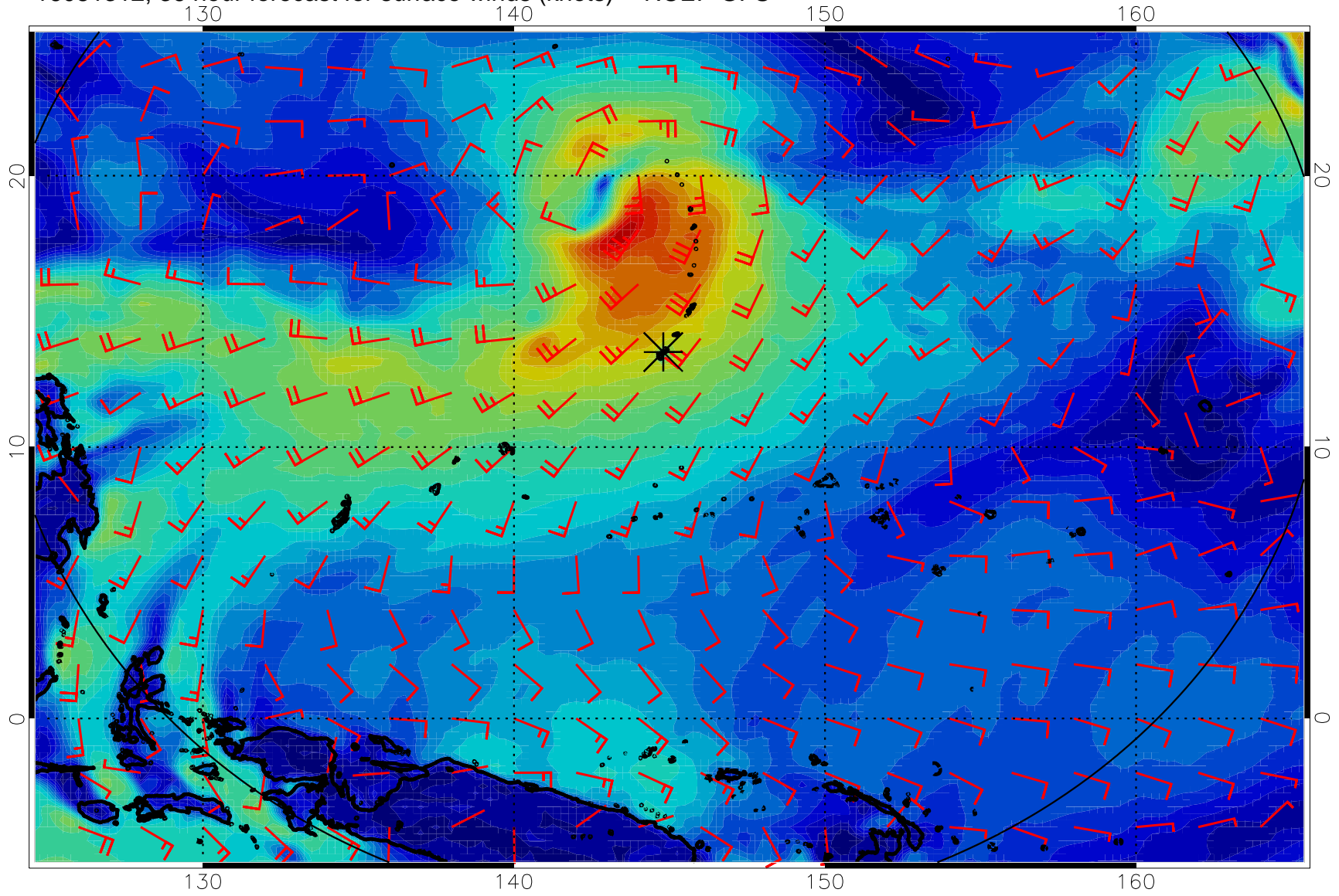
16081312, 36 hour forecast for surface winds (knots) -- NCEP GFS
