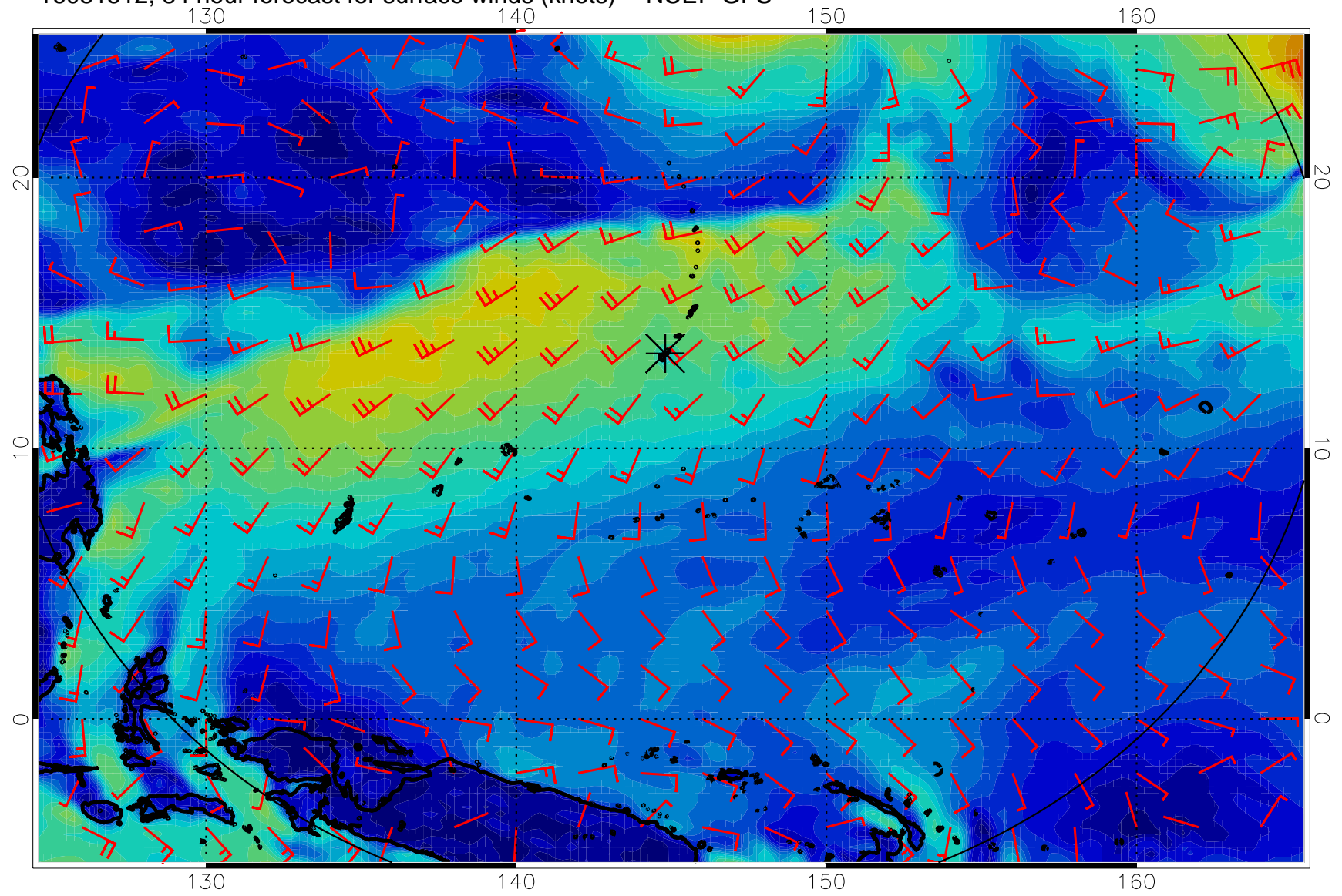
16081512, 84 hour forecast for surface winds (knots) -- NCEP GFS
