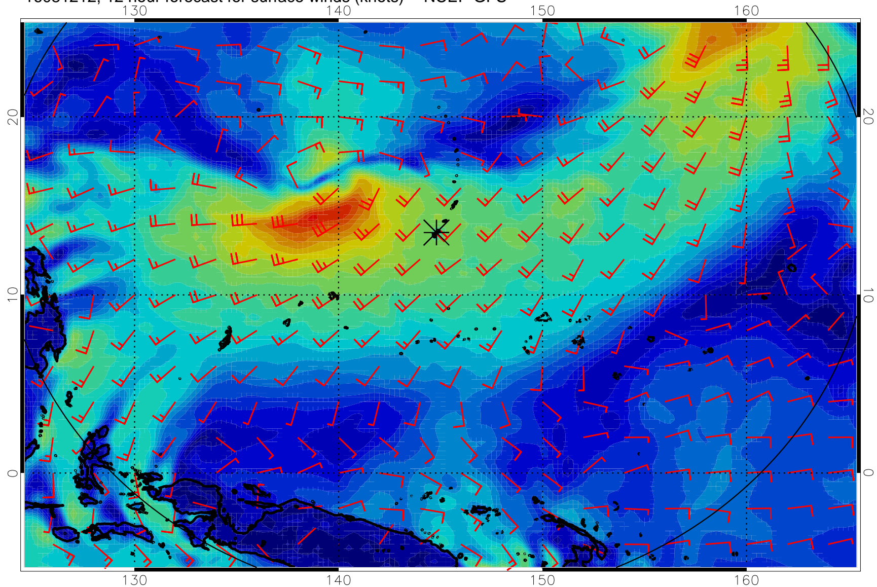
16081212, 12 hour forecast for surface winds (knots) -- NCEP GFS
