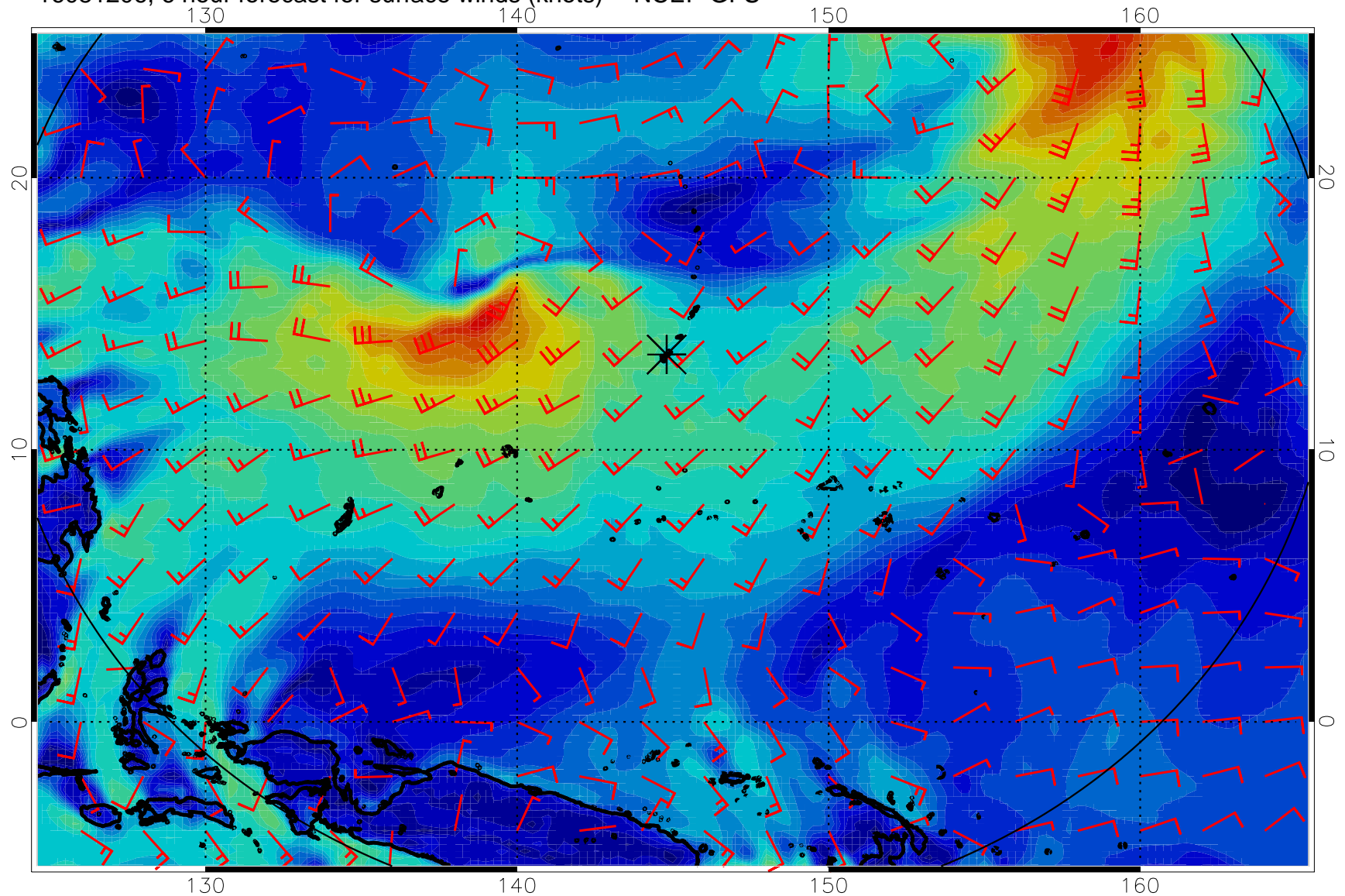
16081206, 6 hour forecast for surface winds (knots) -- NCEP GFS
