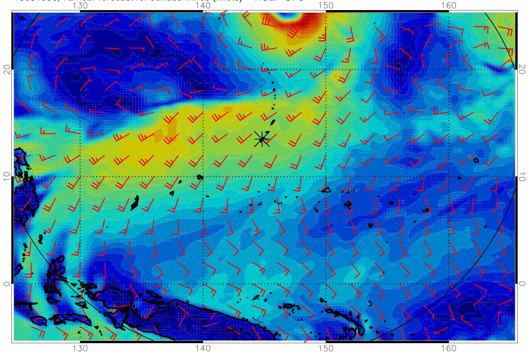
16081500, 72 hour forecast for surface winds (knots) -- NCEP GFS
