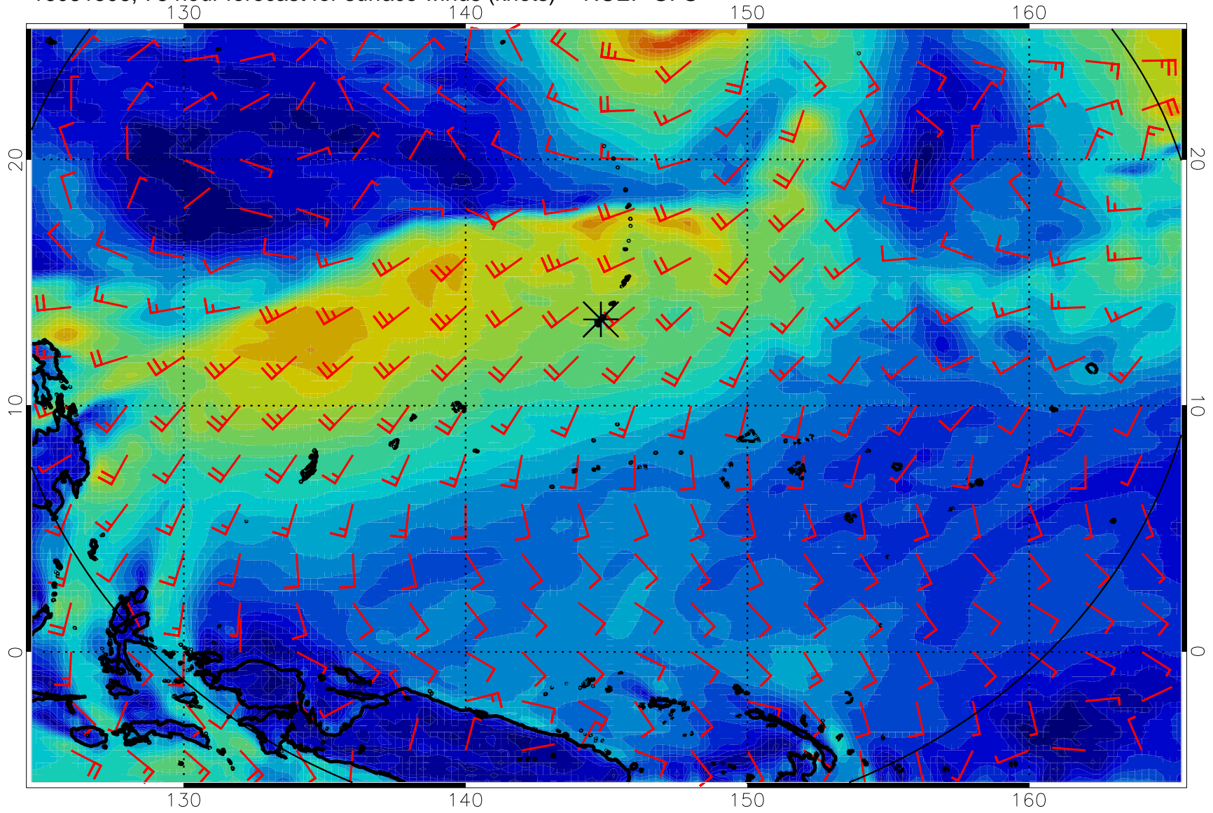
16081506, 78 hour forecast for surface winds (knots) -- NCEP GFS
