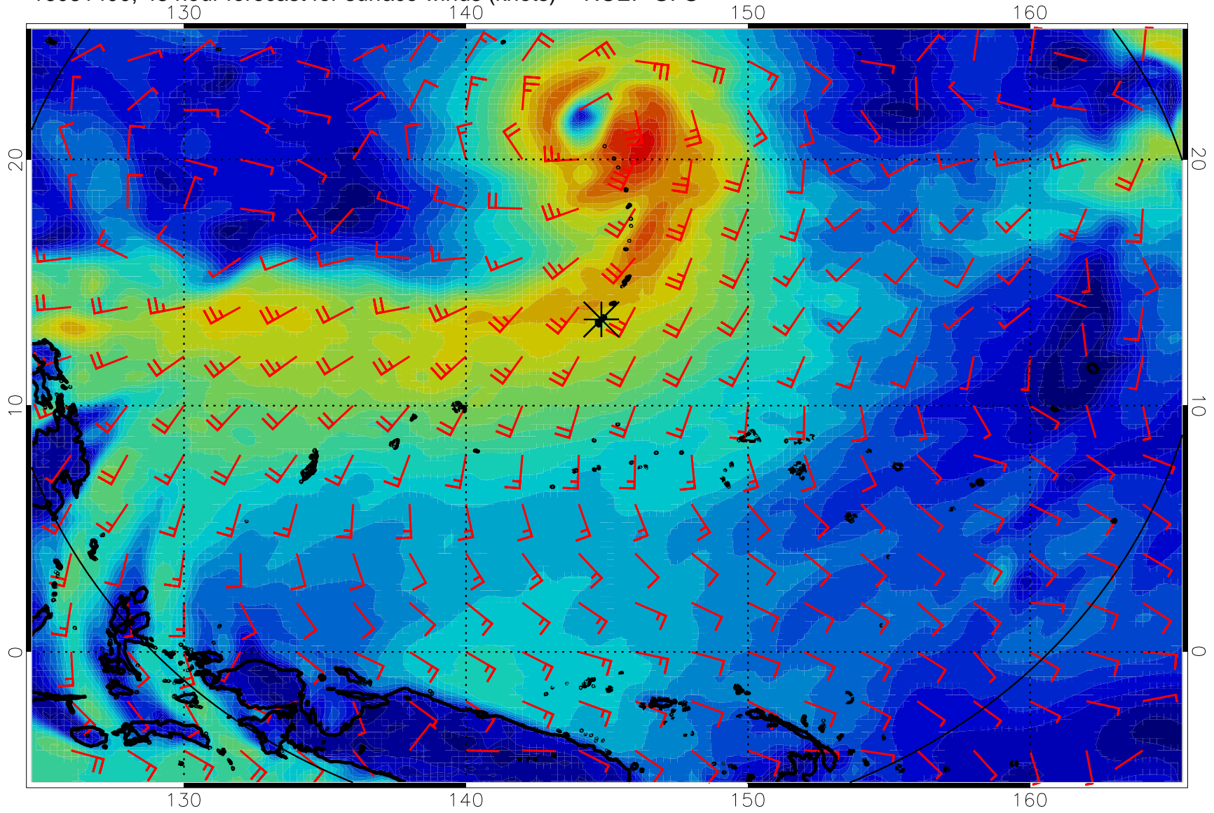
16081400, 48 hour forecast for surface winds (knots) -- NCEP GFS
