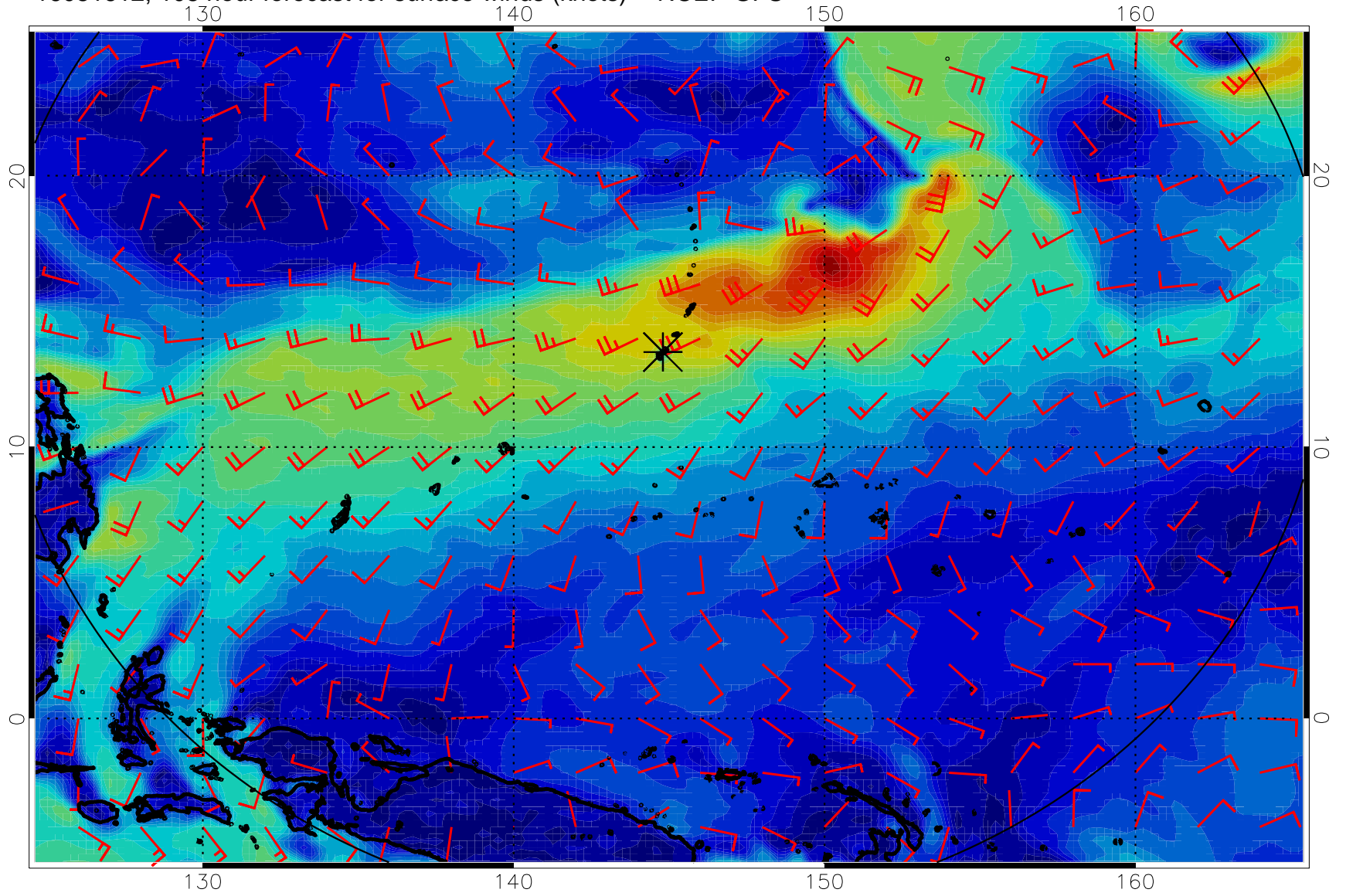
16081612, 108 hour forecast for surface winds (knots) -- NCEP GFS
