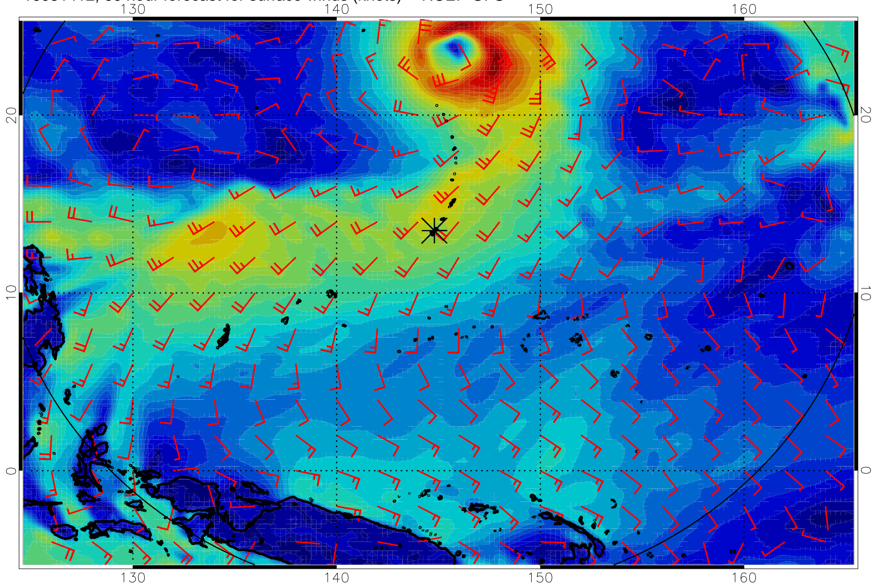
16081412, 60 hour forecast for surface winds (knots) -- NCEP GFS
