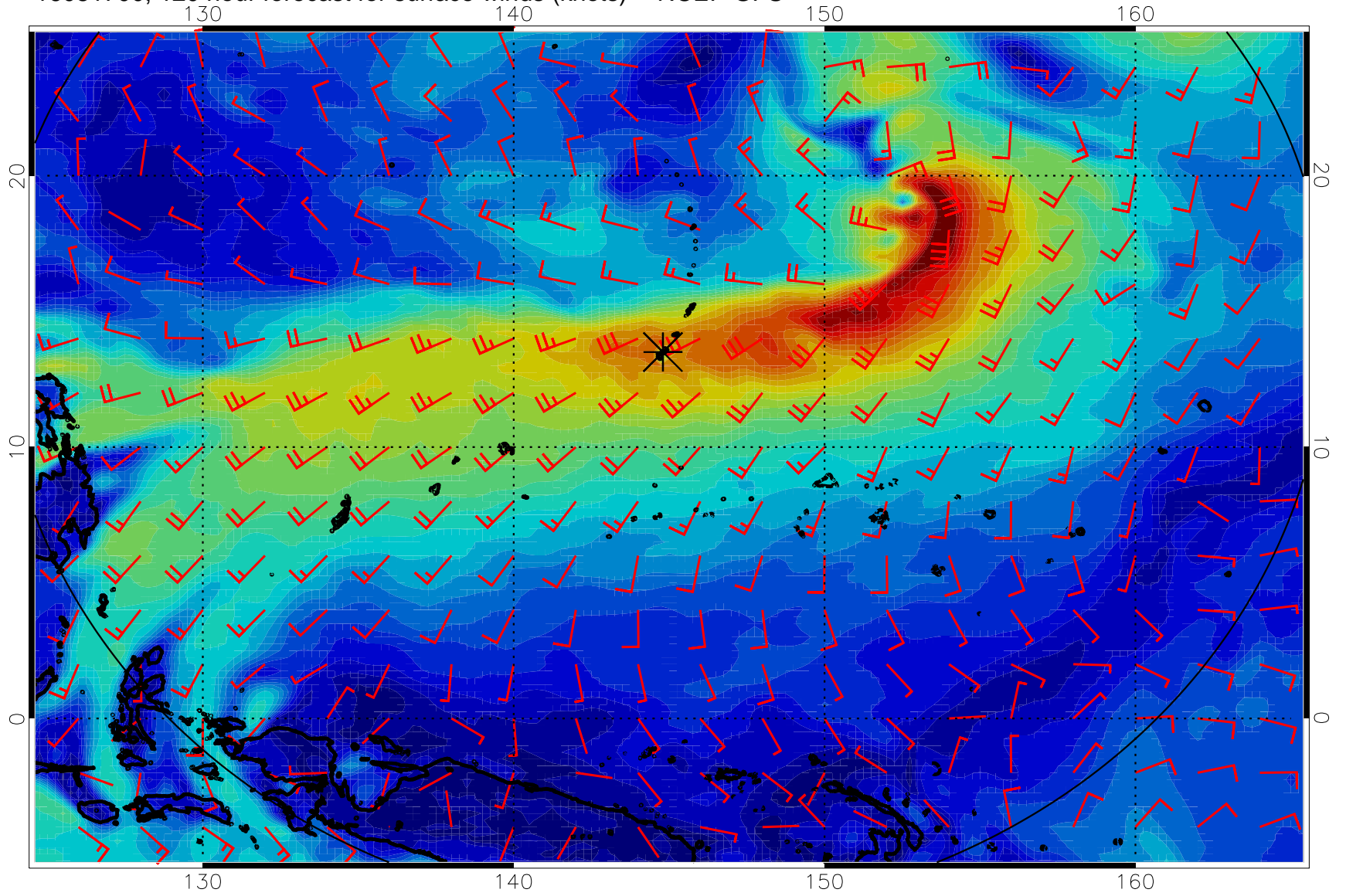
16081700, 120 hour forecast for surface winds (knots) -- NCEP GFS
