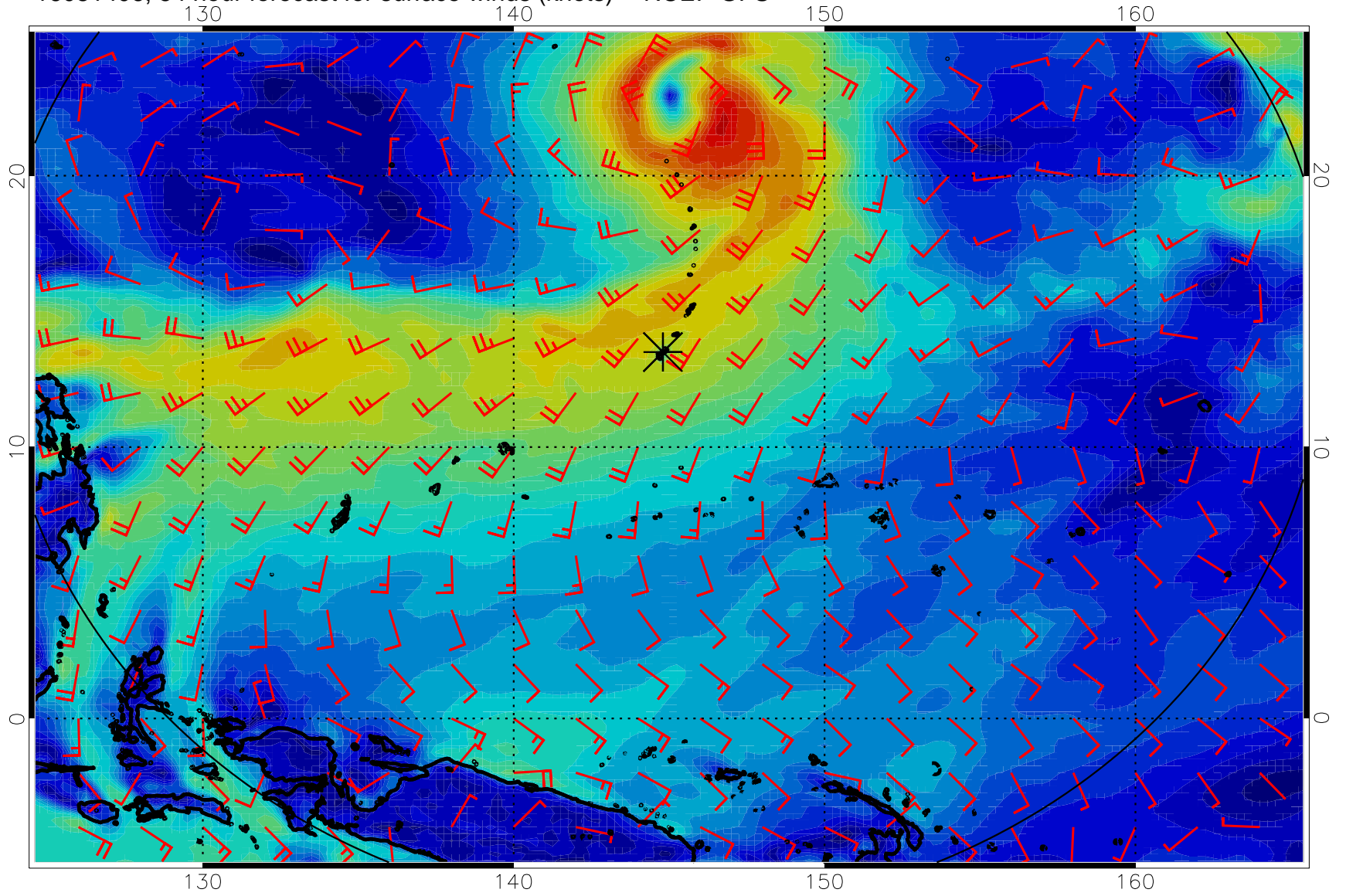
16081406, 54 hour forecast for surface winds (knots) -- NCEP GFS
