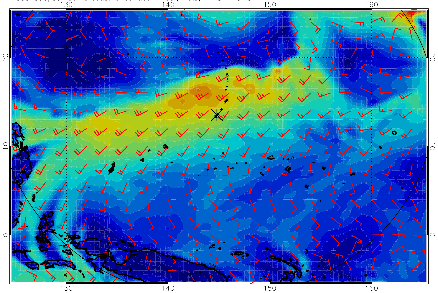
16081600, 96 hour forecast for surface winds (knots) -- NCEP GFS
