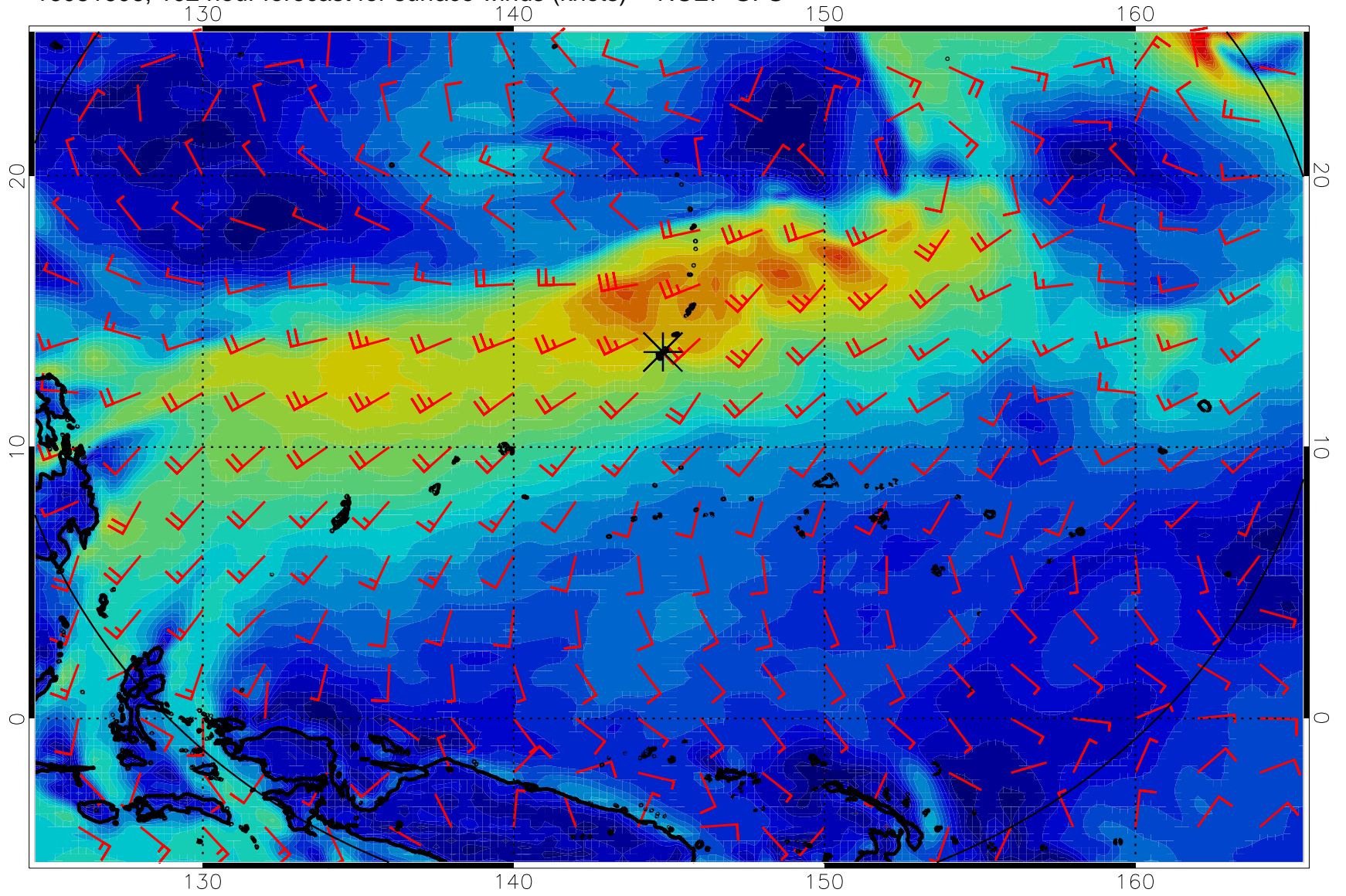
16081606, 102 hour forecast for surface winds (knots) -- NCEP GFS
