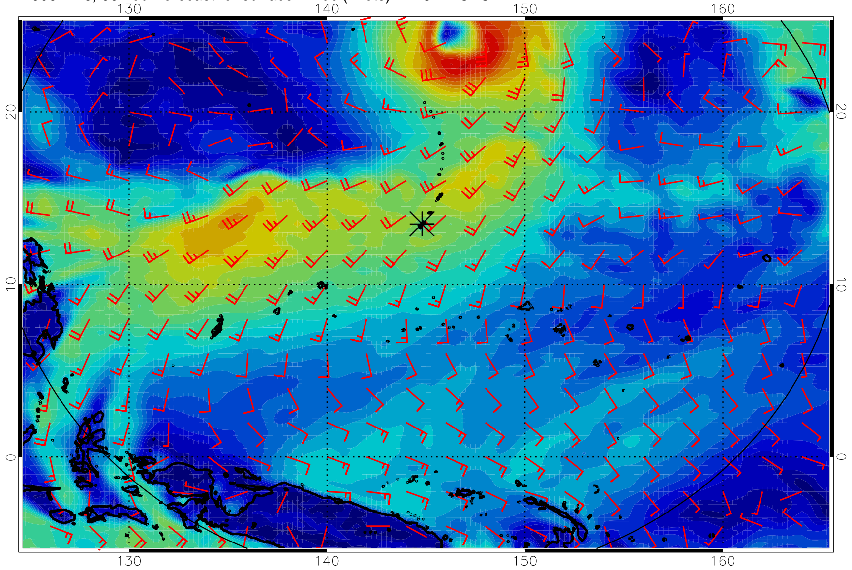
16081418, 66 hour forecast for surface winds (knots) -- NCEP GFS
