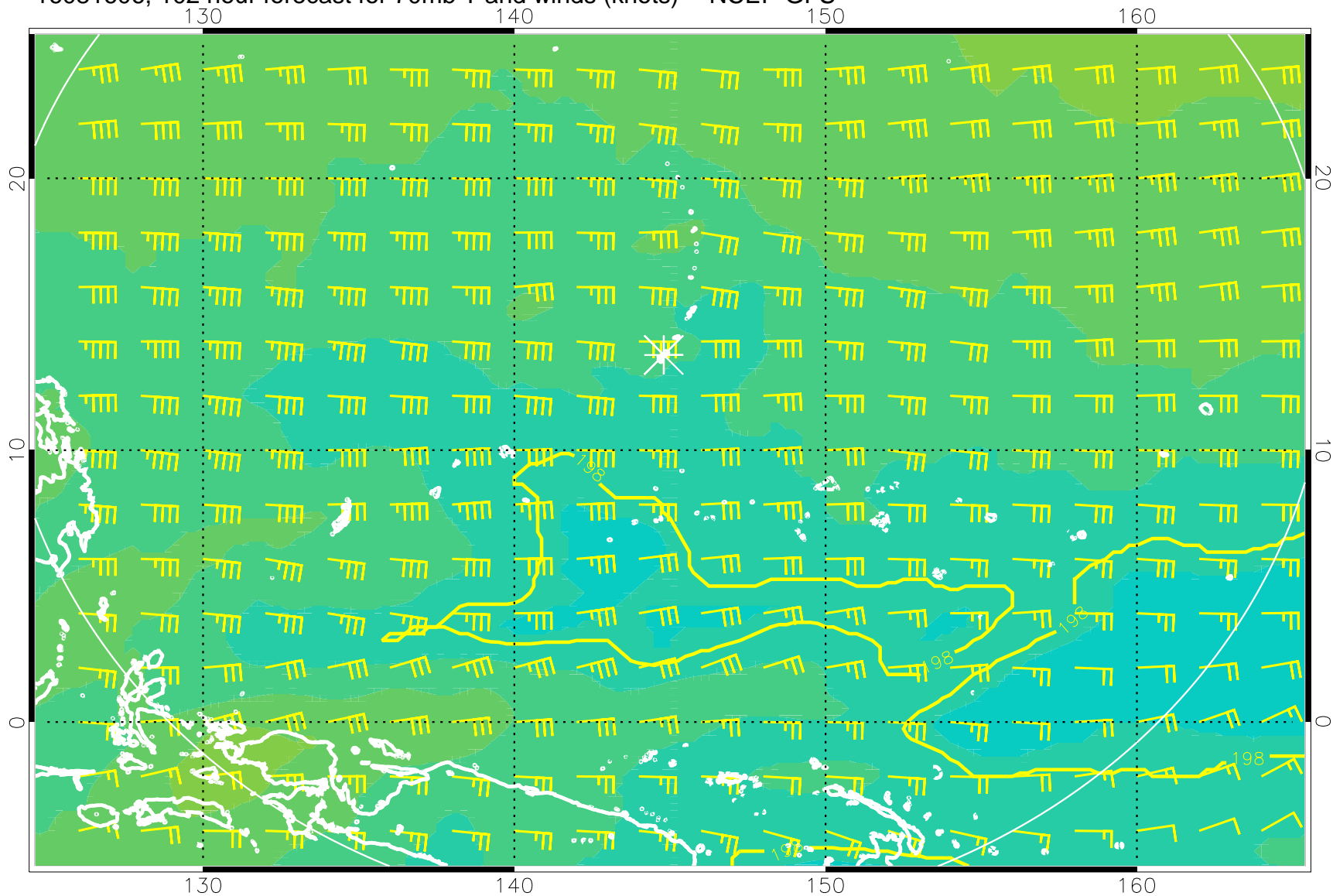
16081606, 102 hour forecast for 70mb T and winds (knots) -- NCEP GFS
