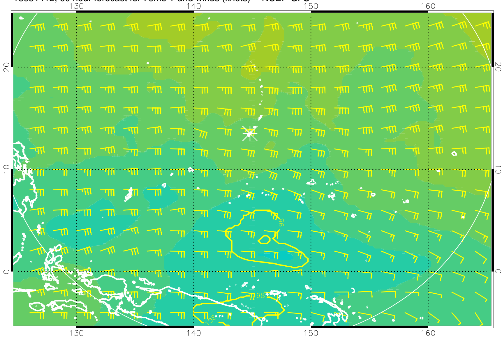
16081412, 60 hour forecast for 70mb T and winds (knots) -- NCEP GFS
