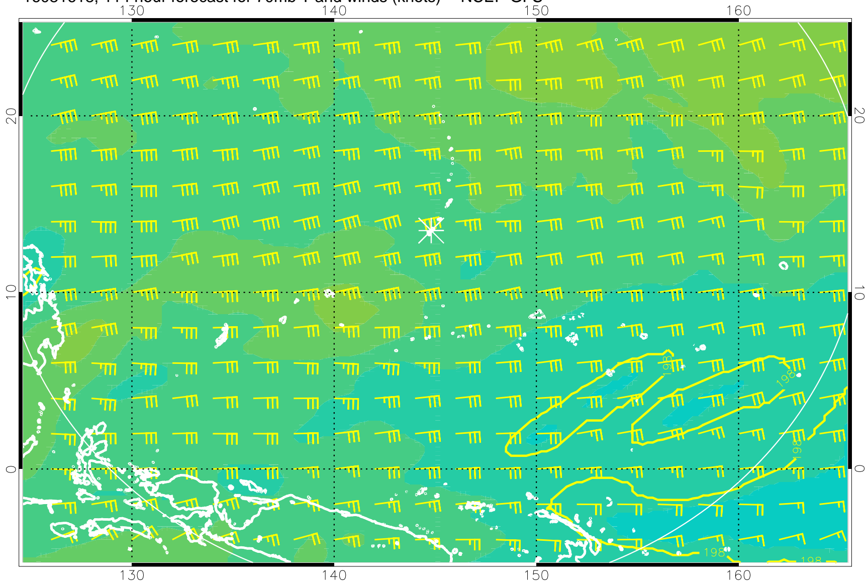
16081618, 114 hour forecast for 70mb T and winds (knots) -- NCEP GFS
