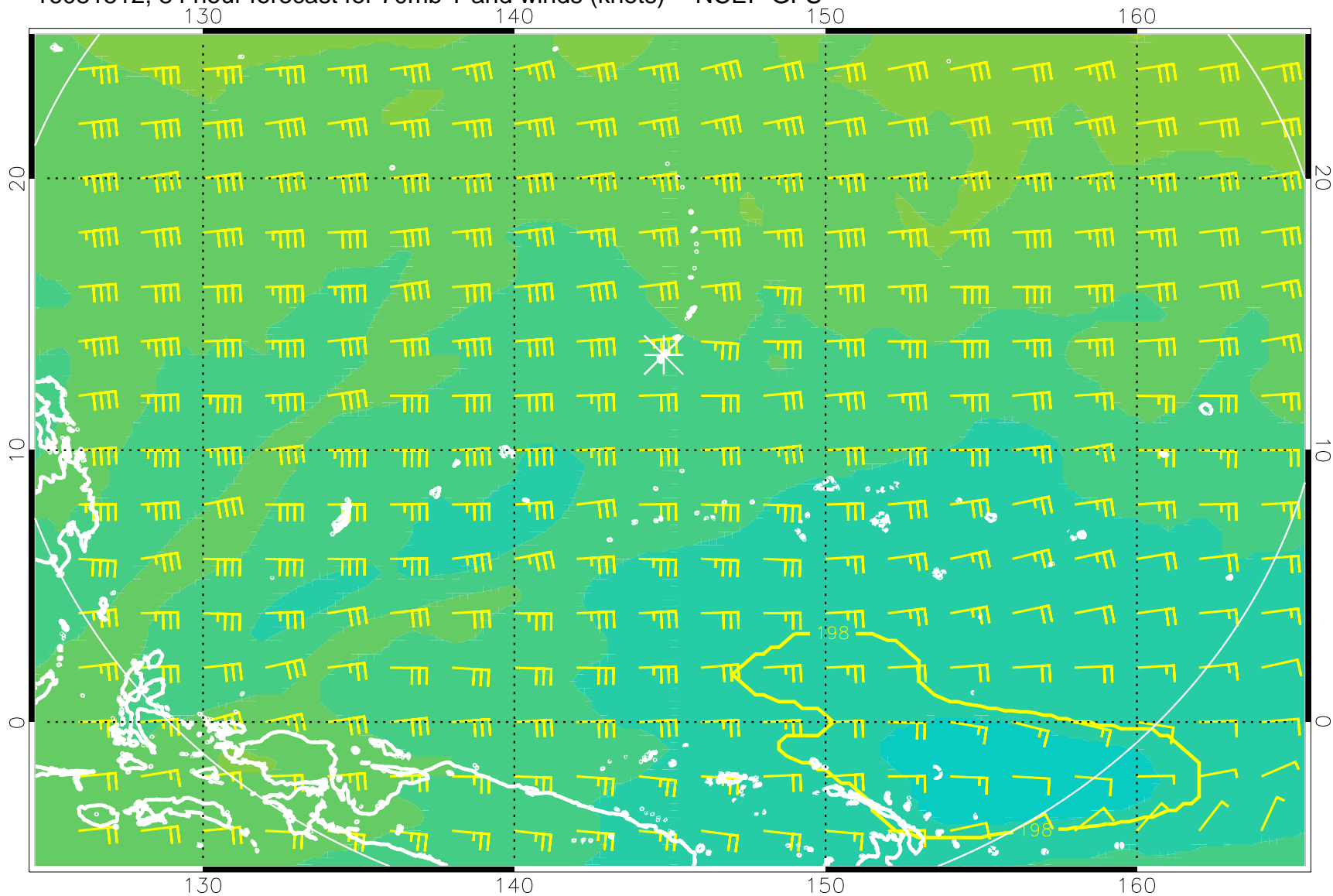
16081512, 84 hour forecast for 70mb T and winds (knots) -- NCEP GFS
