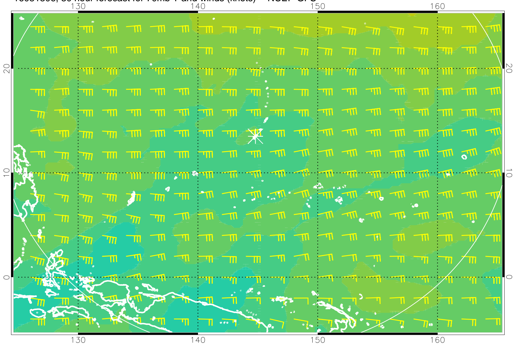
16081306, 30 hour forecast for 70mb T and winds (knots) -- NCEP GFS
