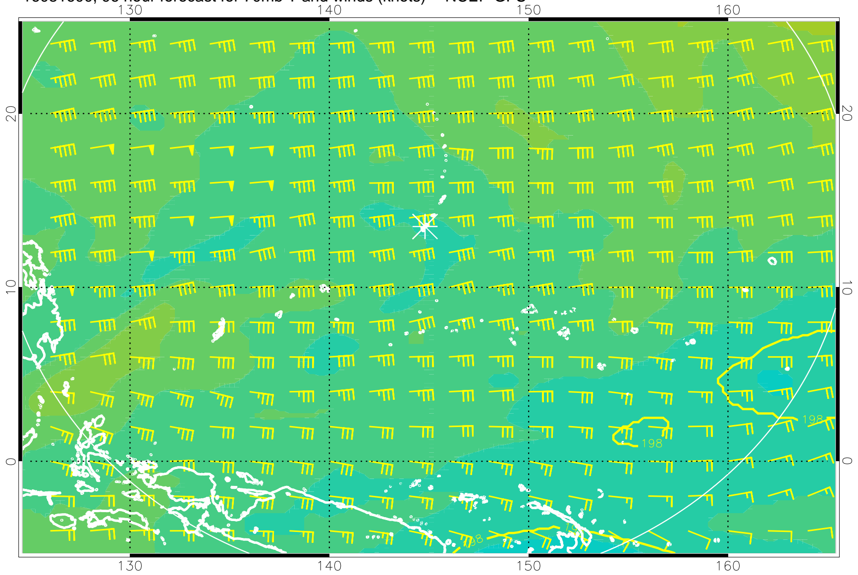
16081600, 96 hour forecast for 70mb T and winds (knots) -- NCEP GFS
