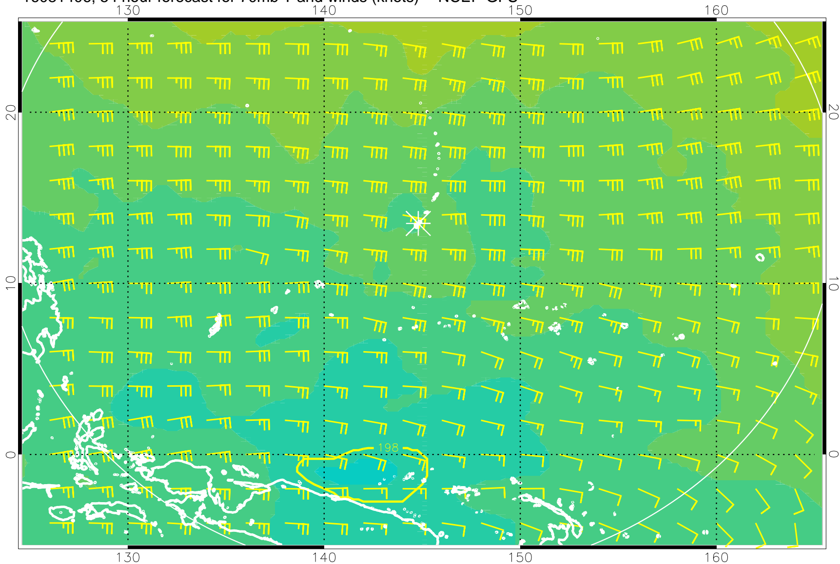
16081406, 54 hour forecast for 70mb T and winds (knots) -- NCEP GFS
