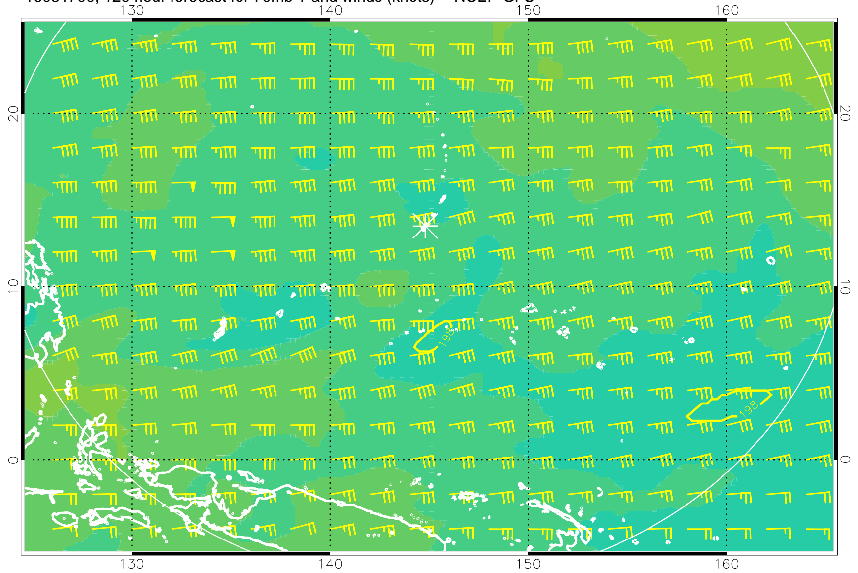
16081700, 120 hour forecast for 70mb T and winds (knots) -- NCEP GFS
