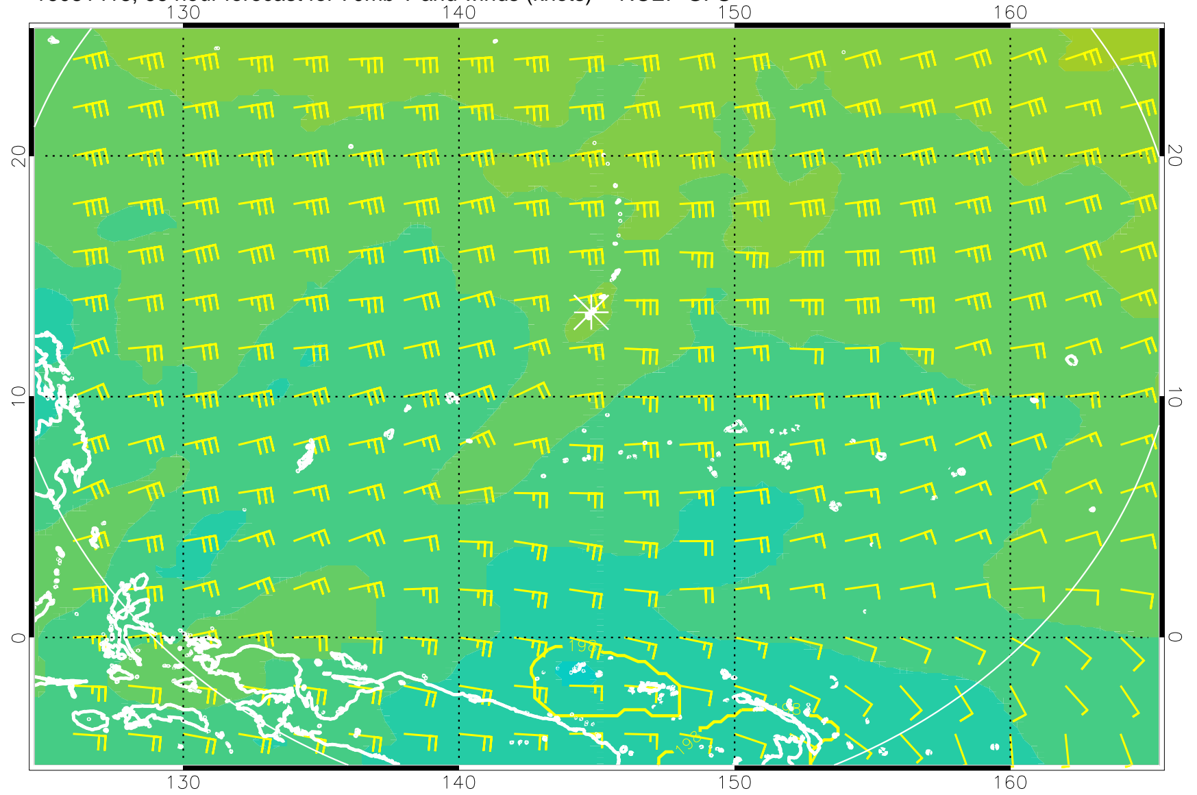
16081418, 66 hour forecast for 70mb T and winds (knots) -- NCEP GFS
