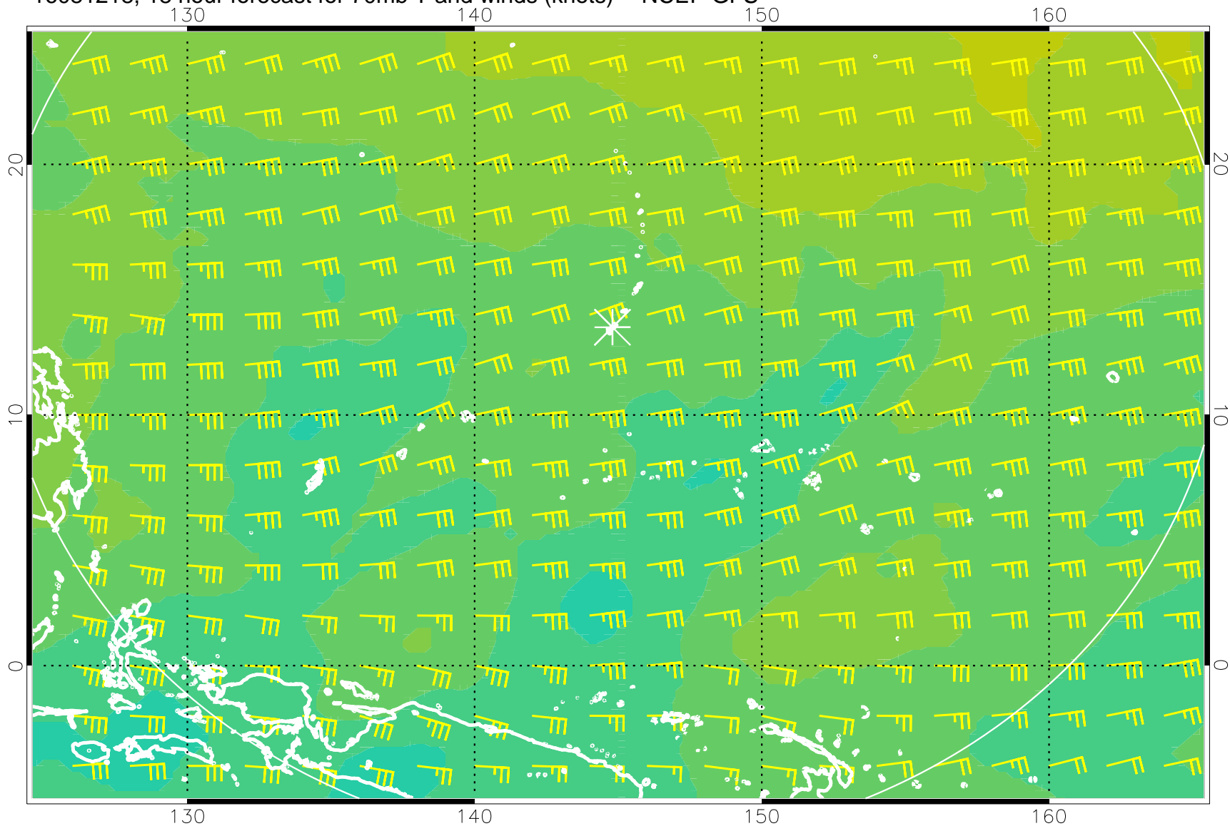
16081218, 18 hour forecast for 70mb T and winds (knots) -- NCEP GFS
