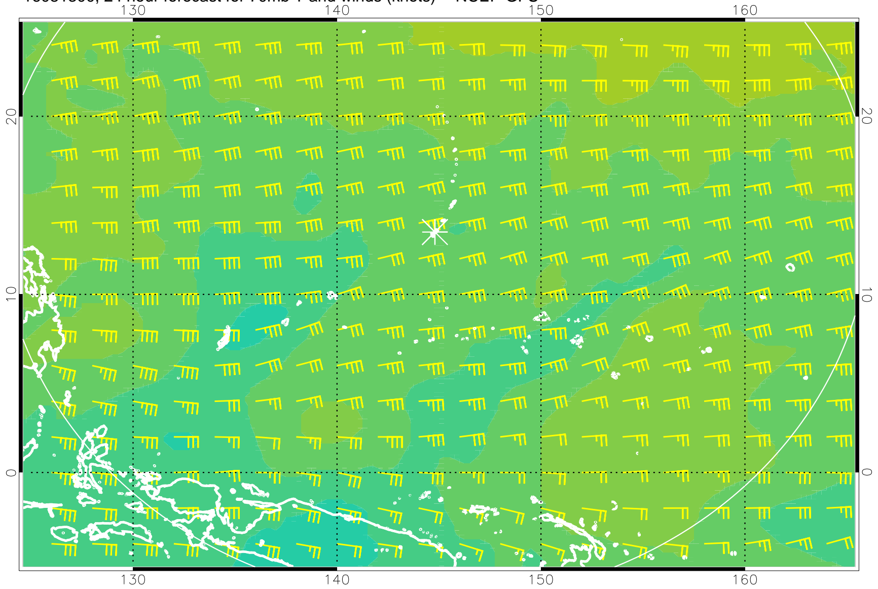
16081300, 24 hour forecast for 70mb T and winds (knots) -- NCEP GFS
