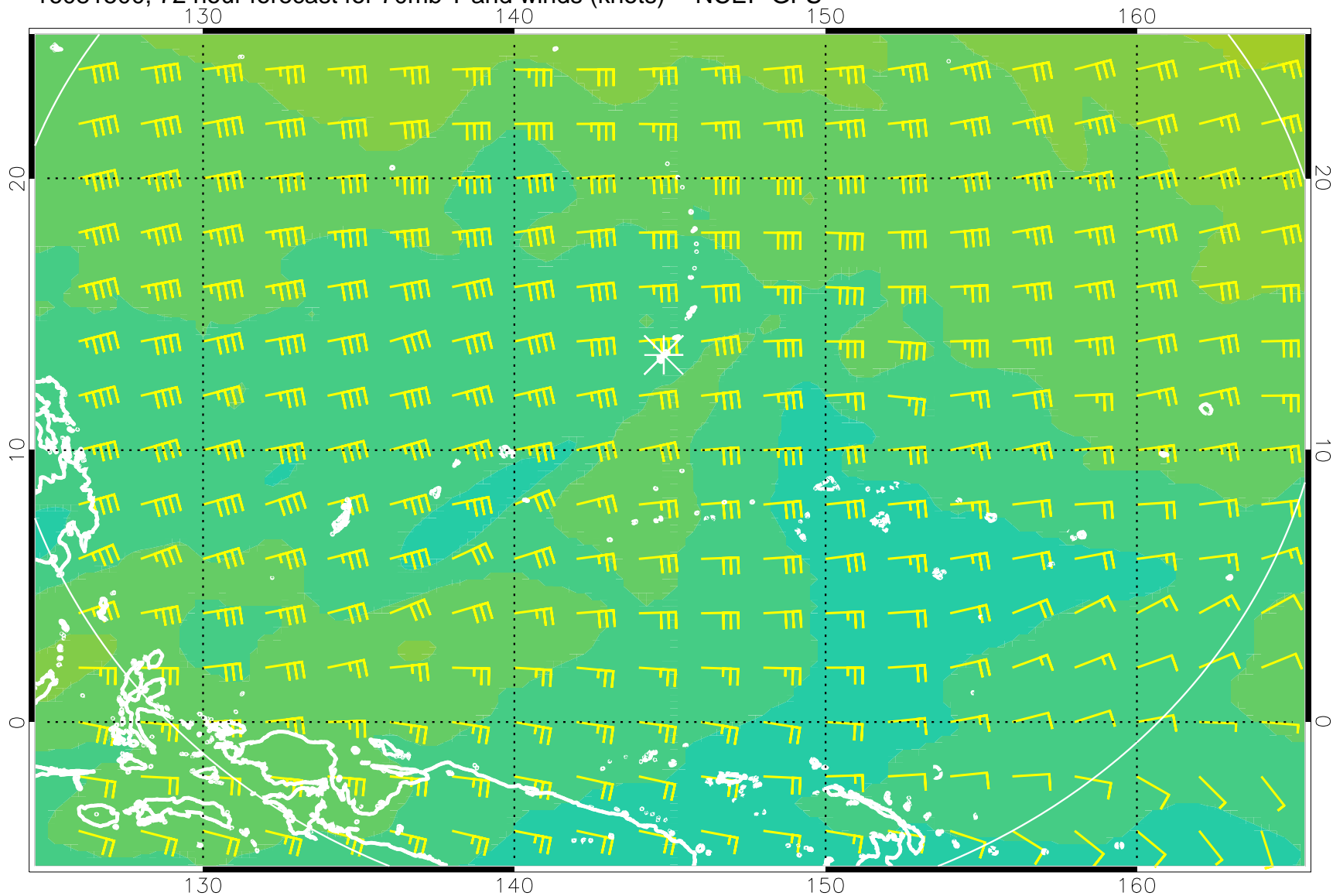
16081500, 72 hour forecast for 70mb T and winds (knots) -- NCEP GFS
