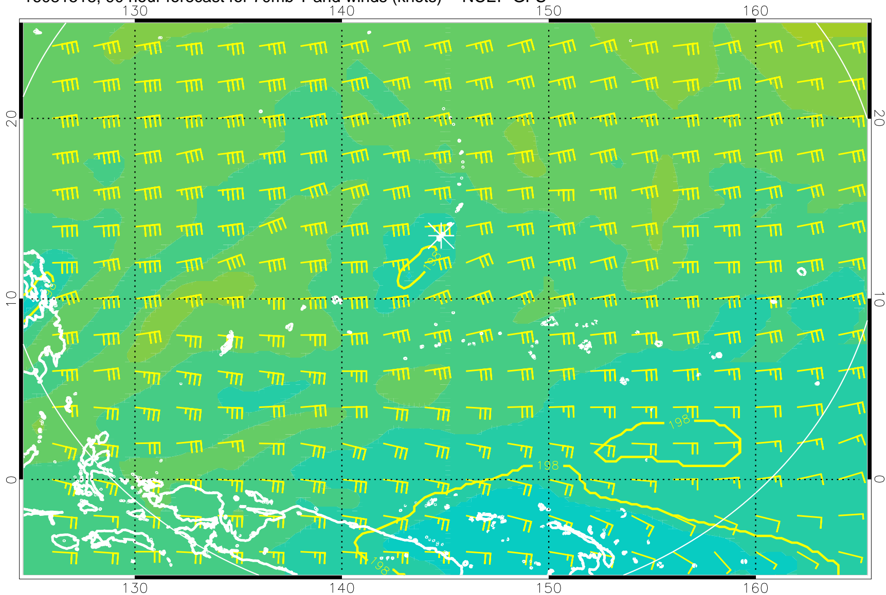
16081518, 90 hour forecast for 70mb T and winds (knots) -- NCEP GFS
