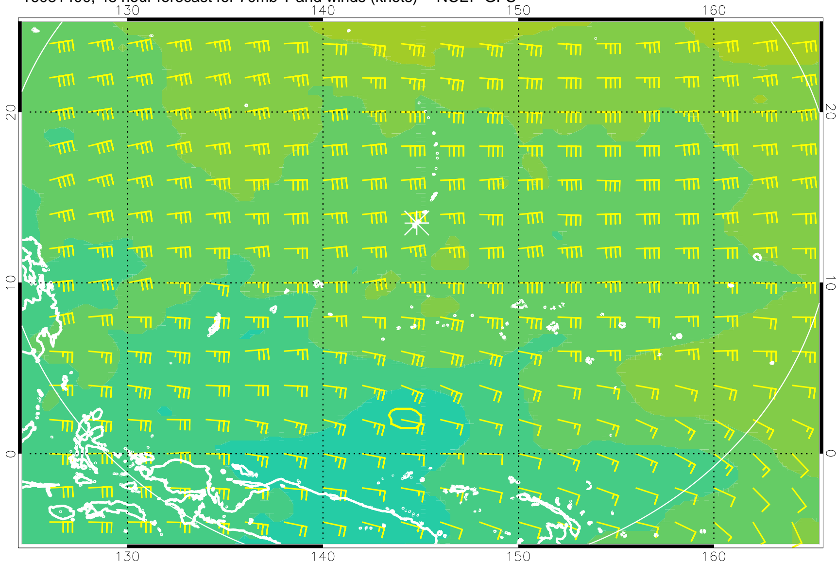
16081400, 48 hour forecast for 70mb T and winds (knots) -- NCEP GFS
