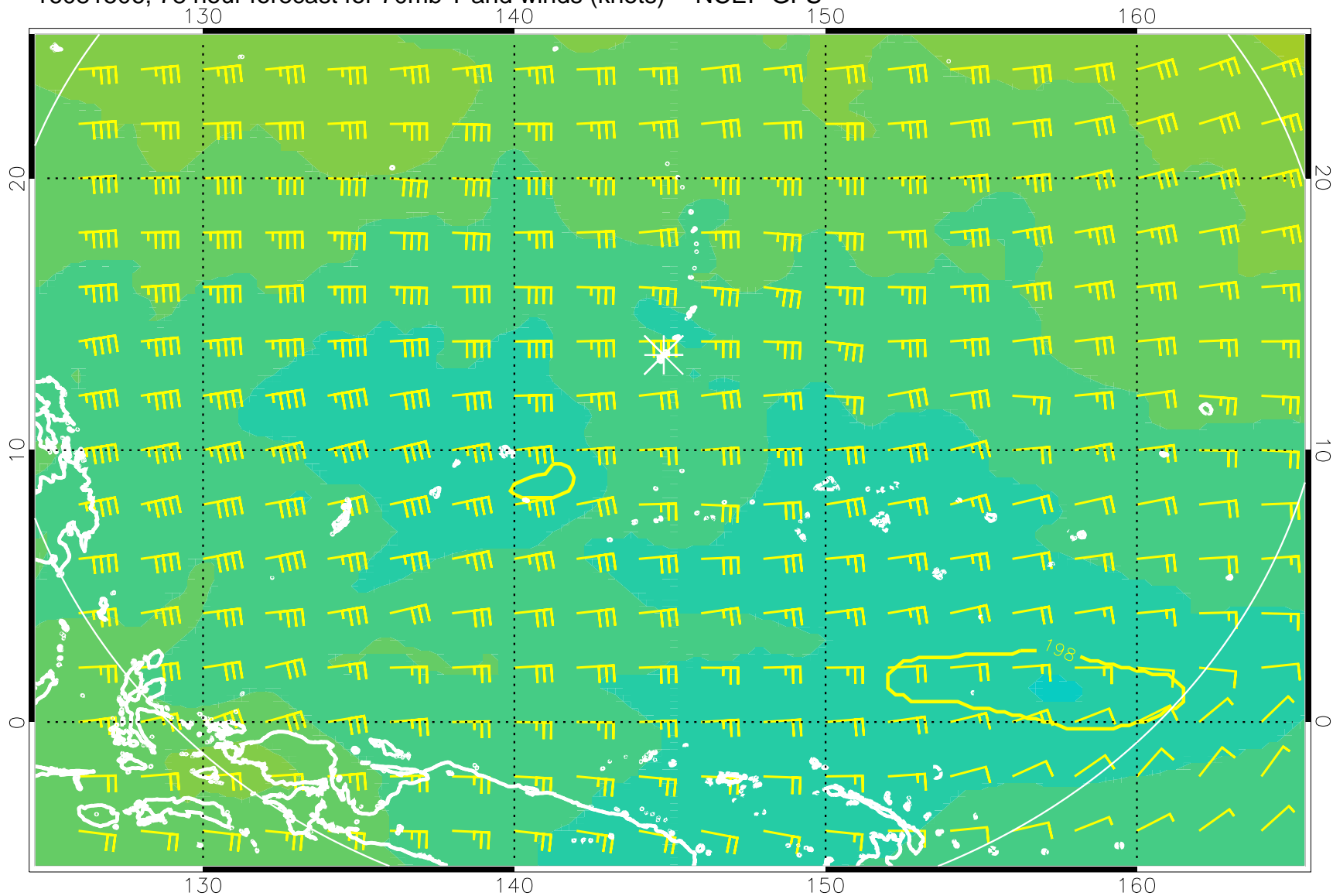
16081506, 78 hour forecast for 70mb T and winds (knots) -- NCEP GFS
