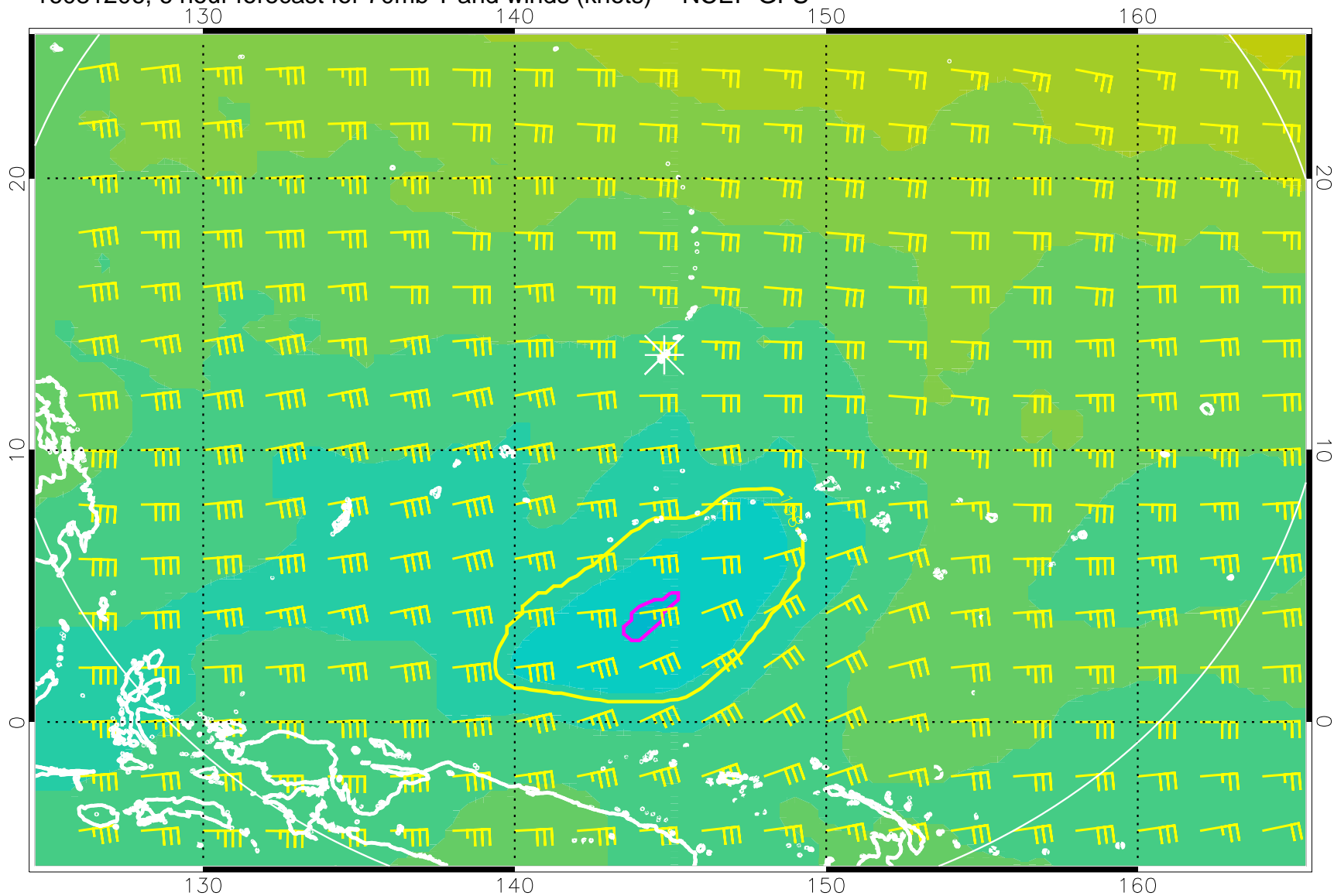
16081206, 6 hour forecast for 70mb T and winds (knots) -- NCEP GFS
