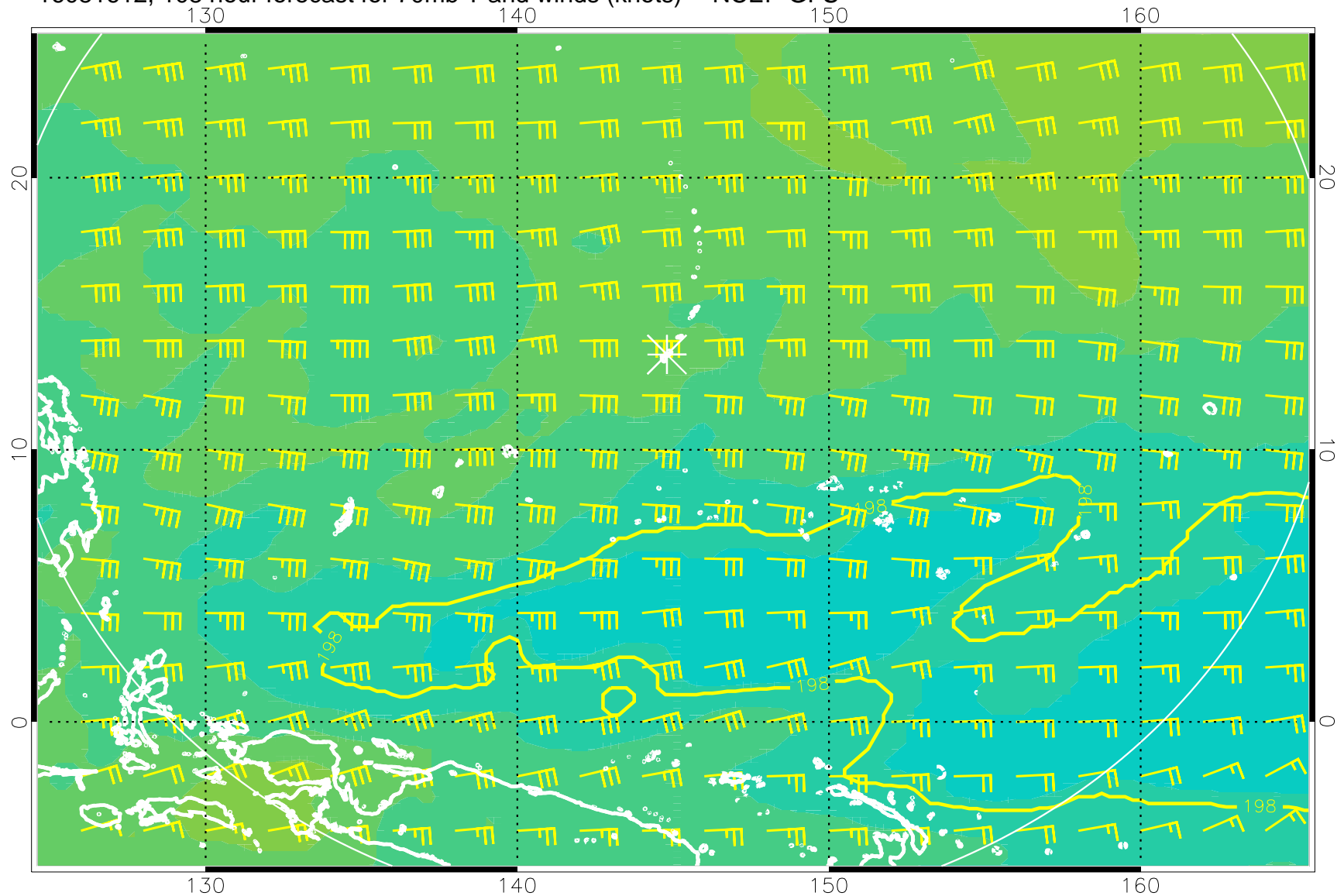
16081612, 108 hour forecast for 70mb T and winds (knots) -- NCEP GFS
