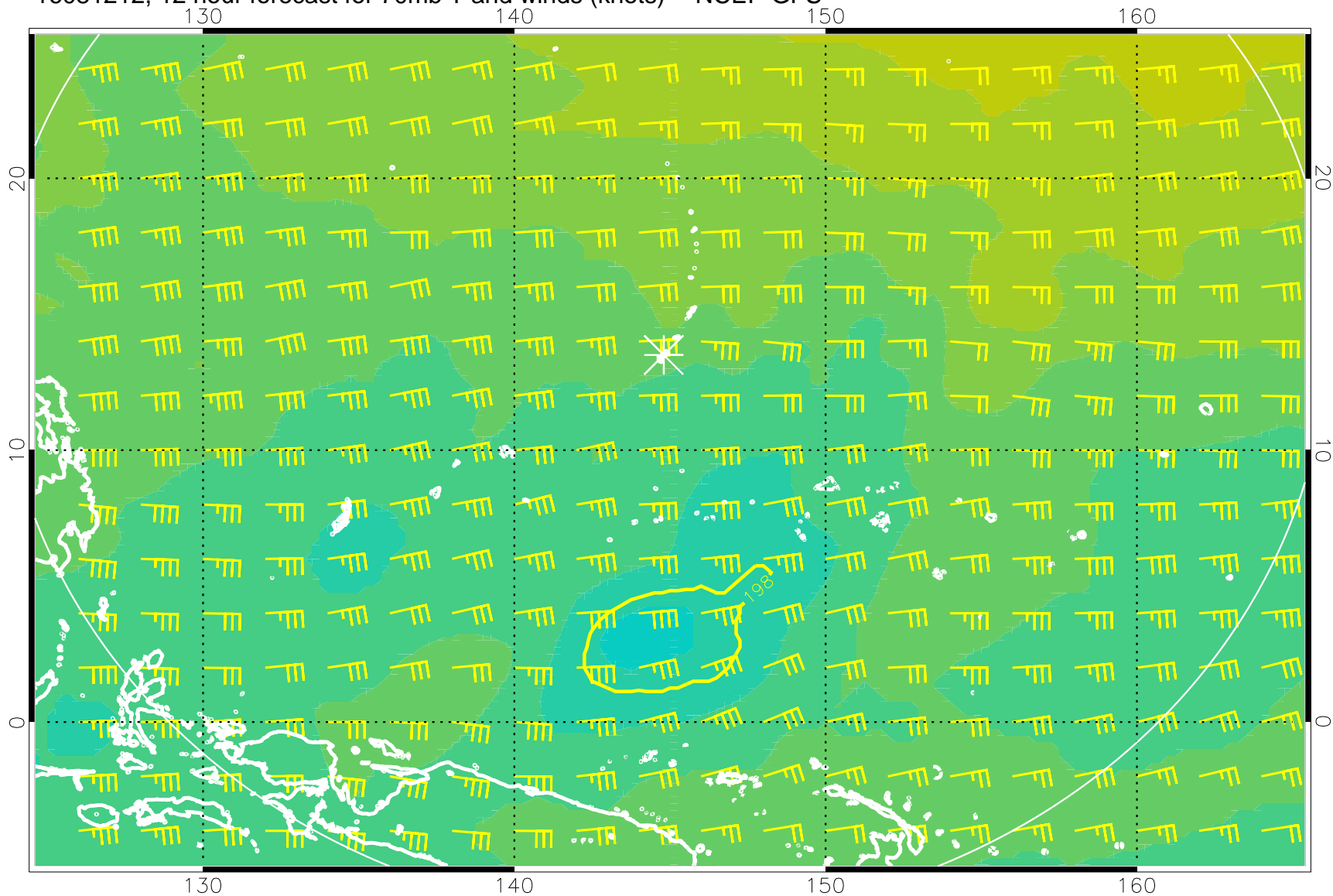
16081212, 12 hour forecast for 70mb T and winds (knots) -- NCEP GFS
