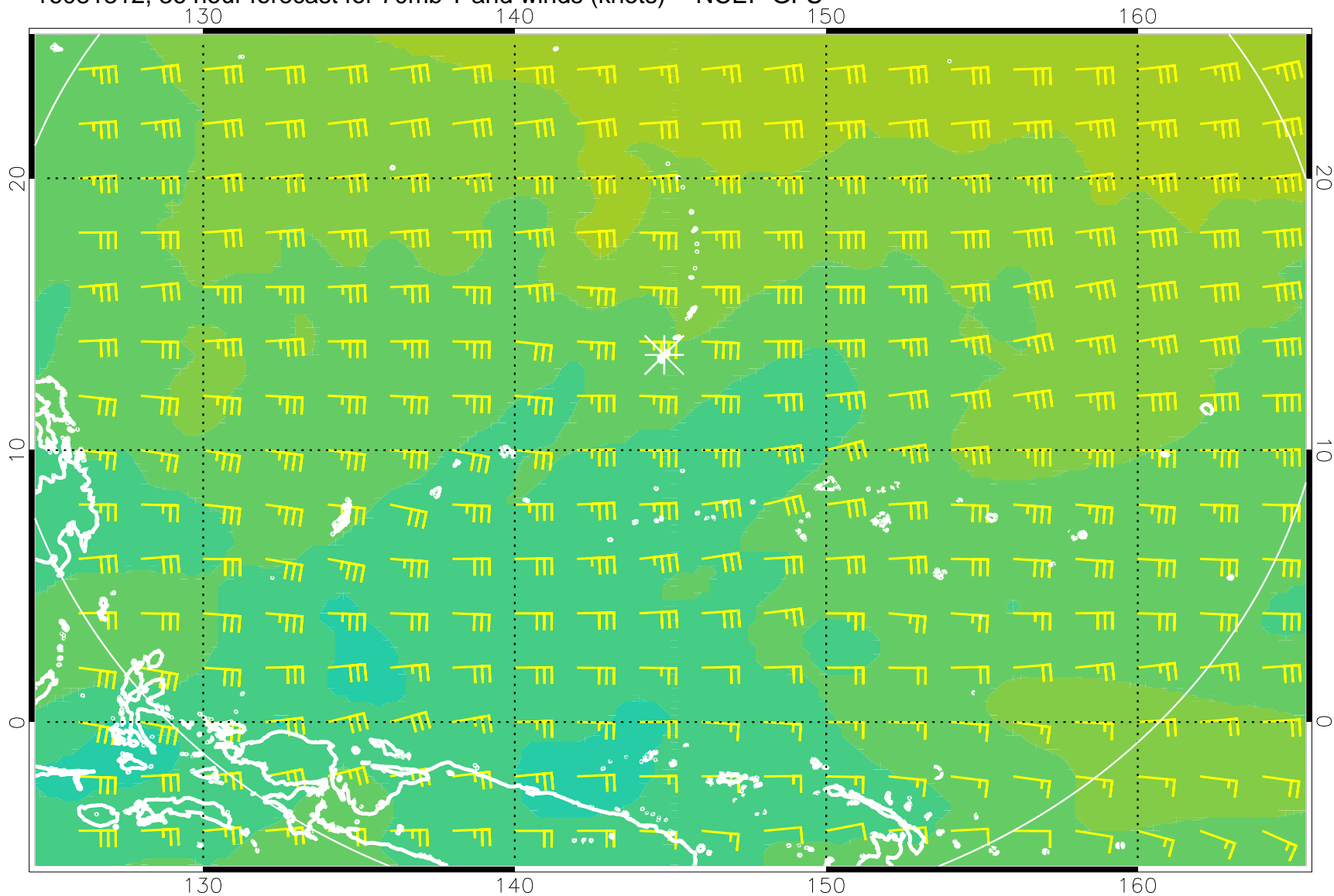
16081312, 36 hour forecast for 70mb T and winds (knots) -- NCEP GFS
