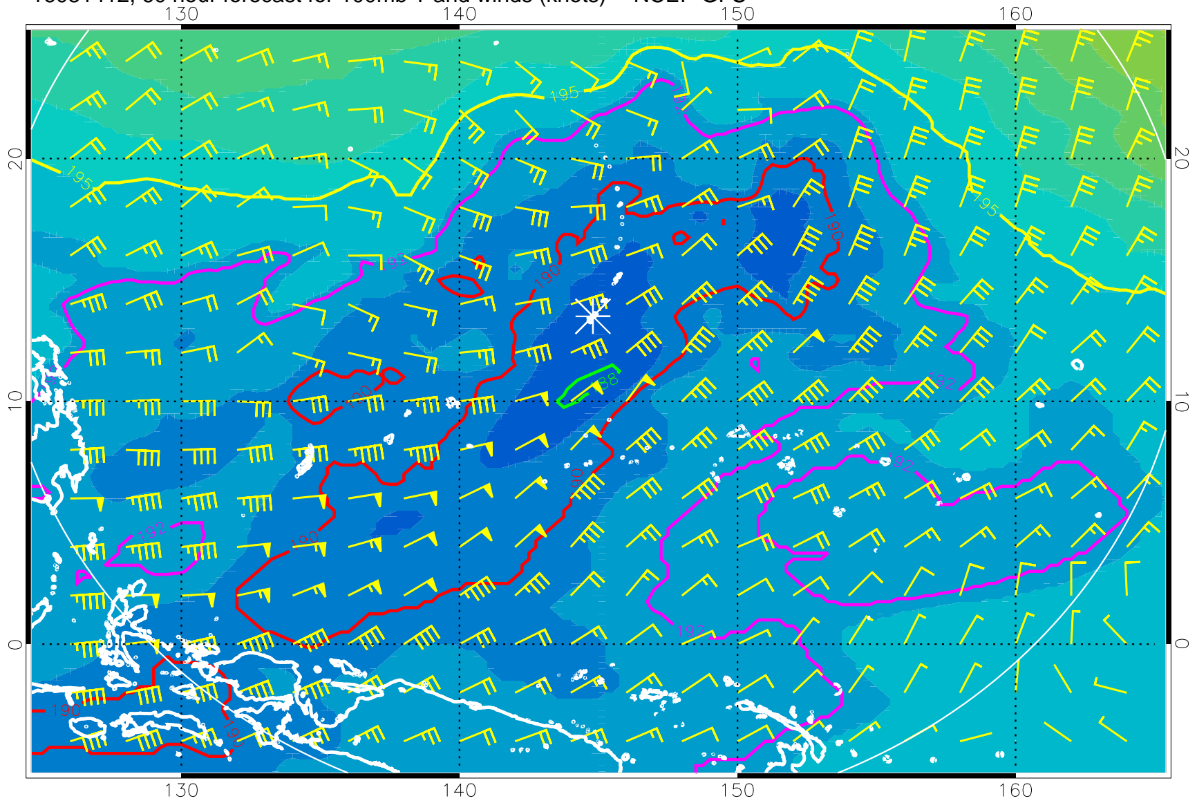
16081412, 60 hour forecast for 100mb T and winds (knots) -- NCEP GFS
