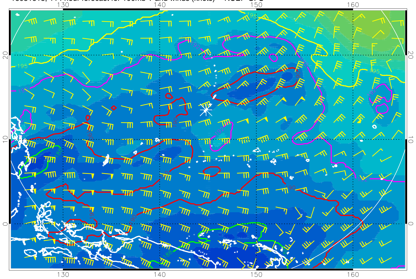
16081618, 114 hour forecast for 100mb T and winds (knots) -- NCEP GFS
