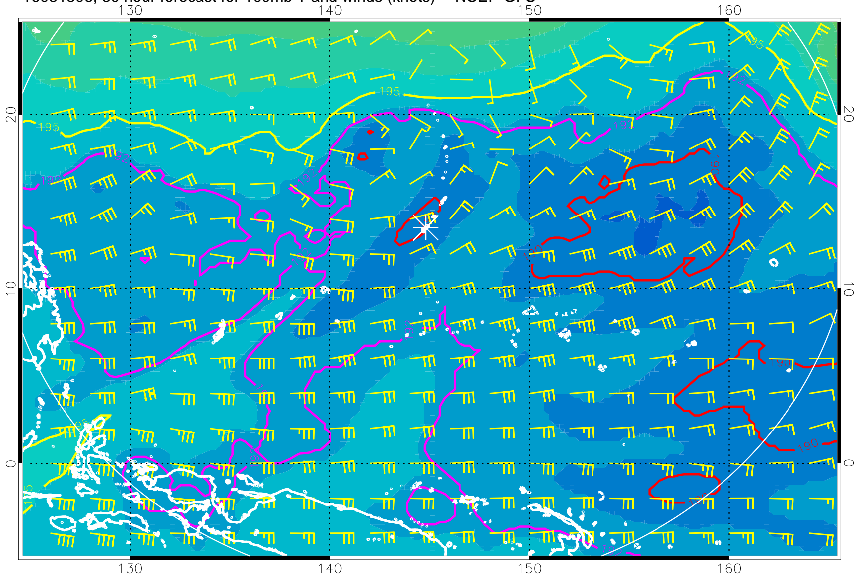
16081306, 30 hour forecast for 100mb T and winds (knots) -- NCEP GFS
