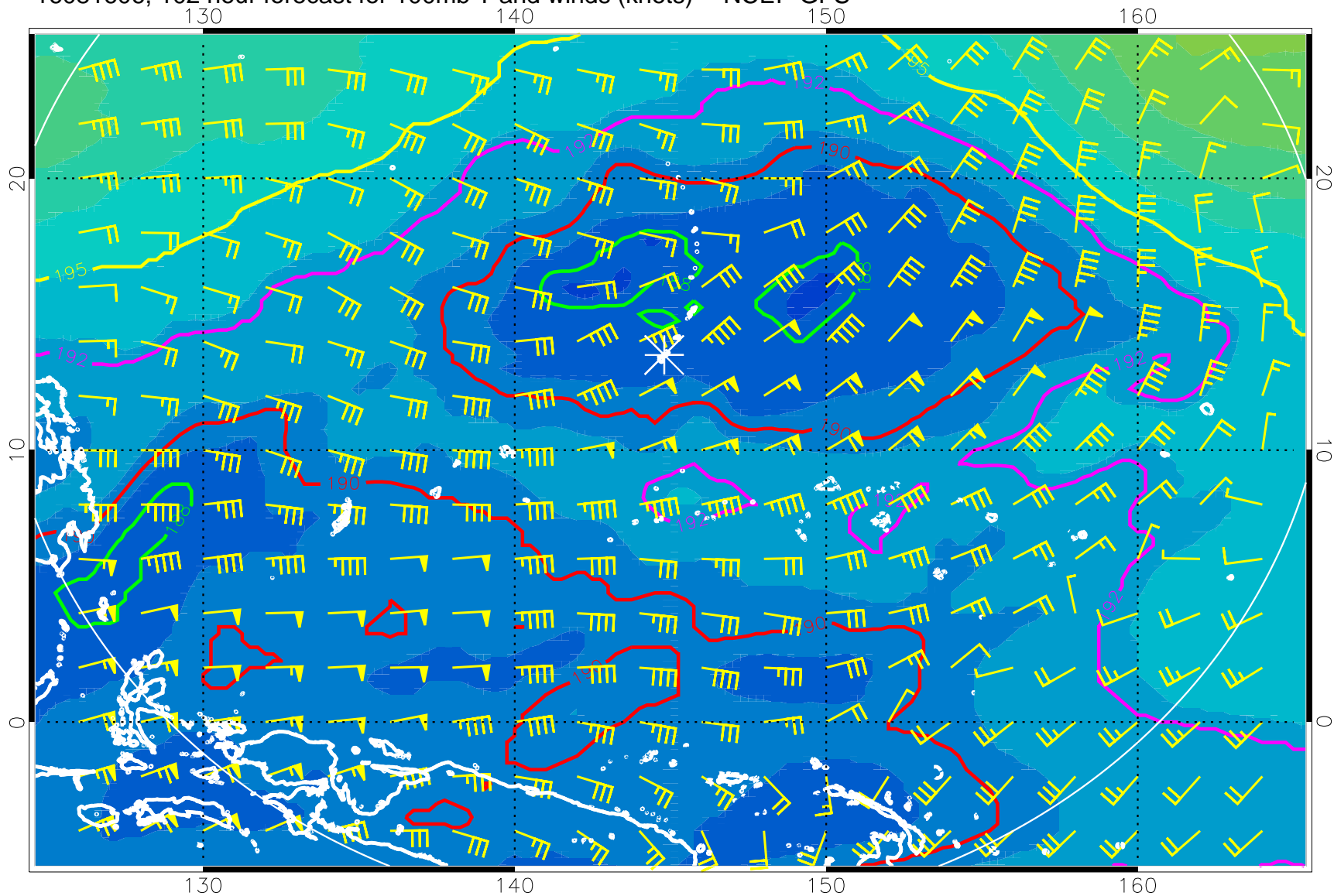
16081606, 102 hour forecast for 100mb T and winds (knots) -- NCEP GFS
