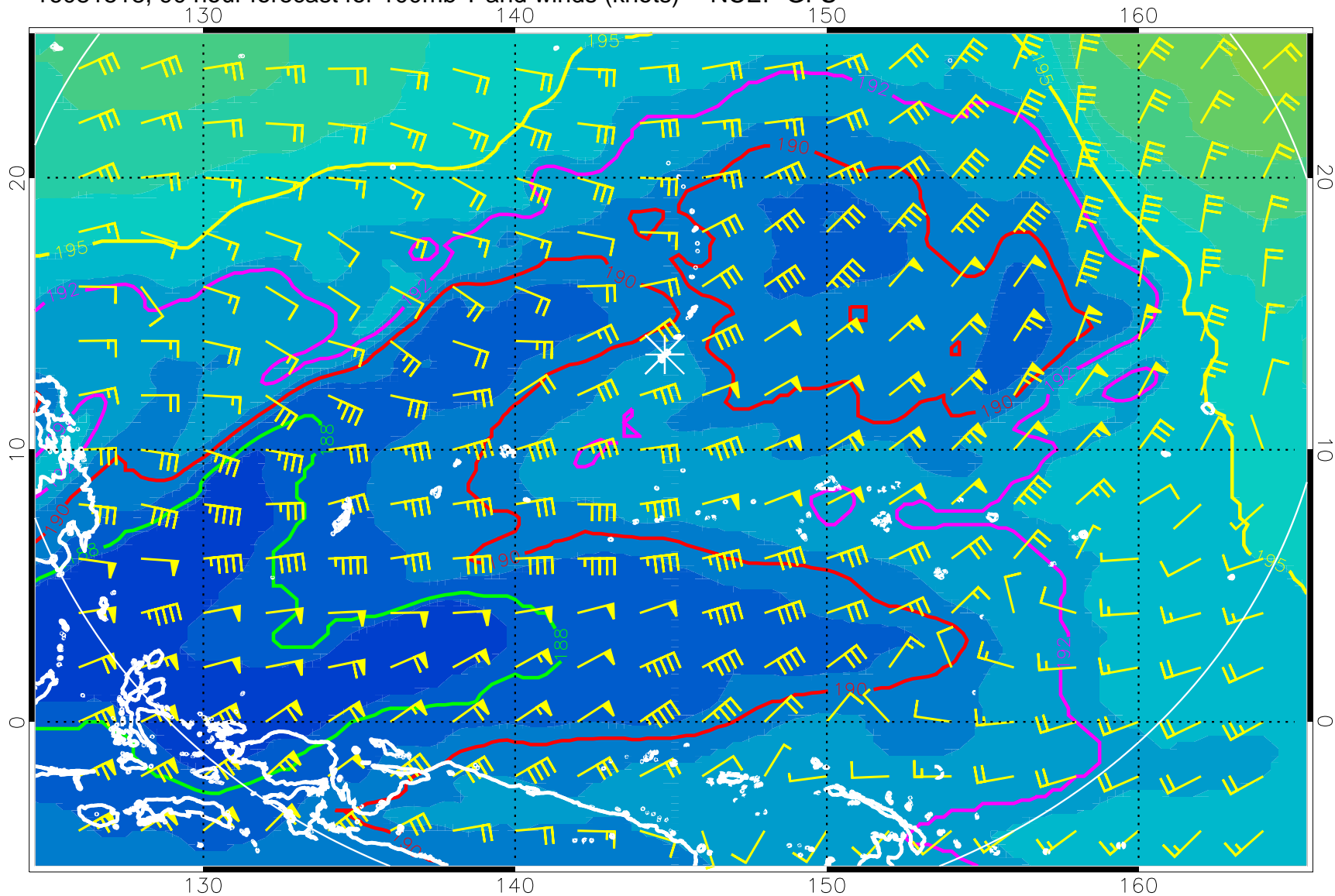
16081518, 90 hour forecast for 100mb T and winds (knots) -- NCEP GFS
