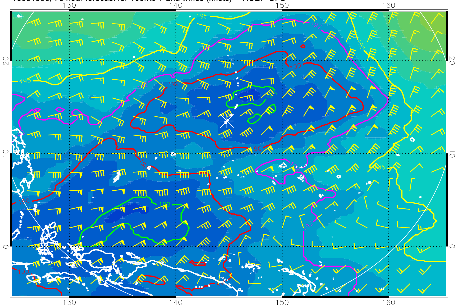
16081506, 78 hour forecast for 100mb T and winds (knots) -- NCEP GFS
