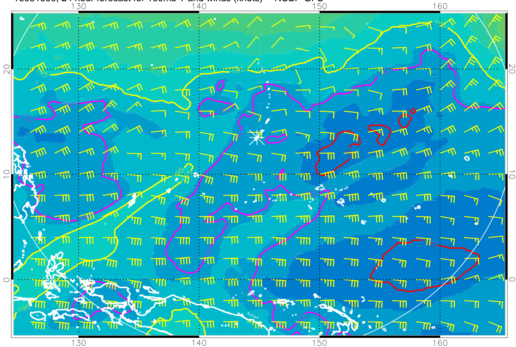
16081300, 24 hour forecast for 100mb T and winds (knots) -- NCEP GFS
