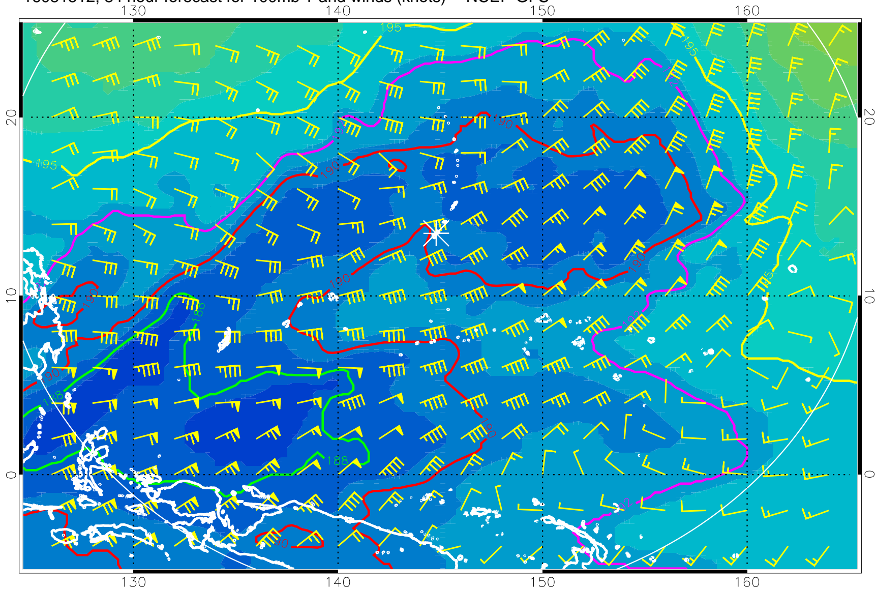
16081512, 84 hour forecast for 100mb T and winds (knots) -- NCEP GFS
