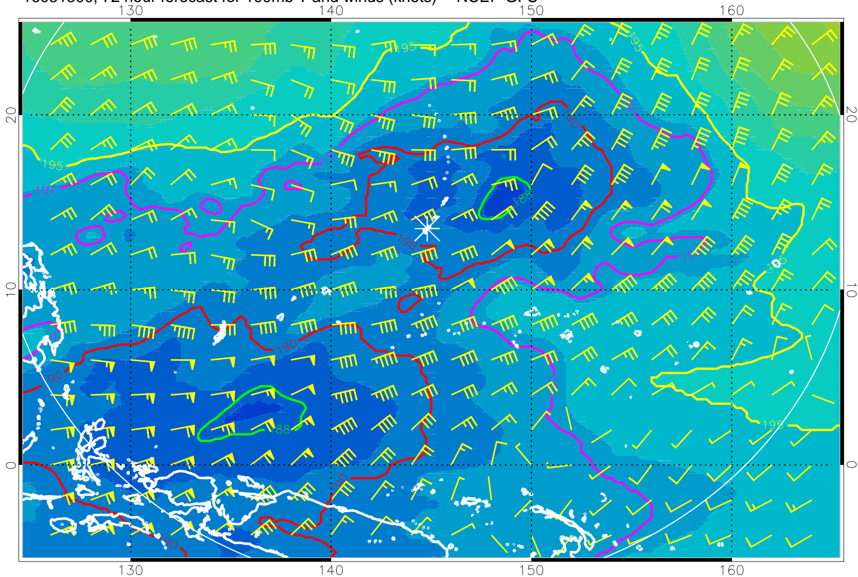
16081500, 72 hour forecast for 100mb T and winds (knots) -- NCEP GFS
