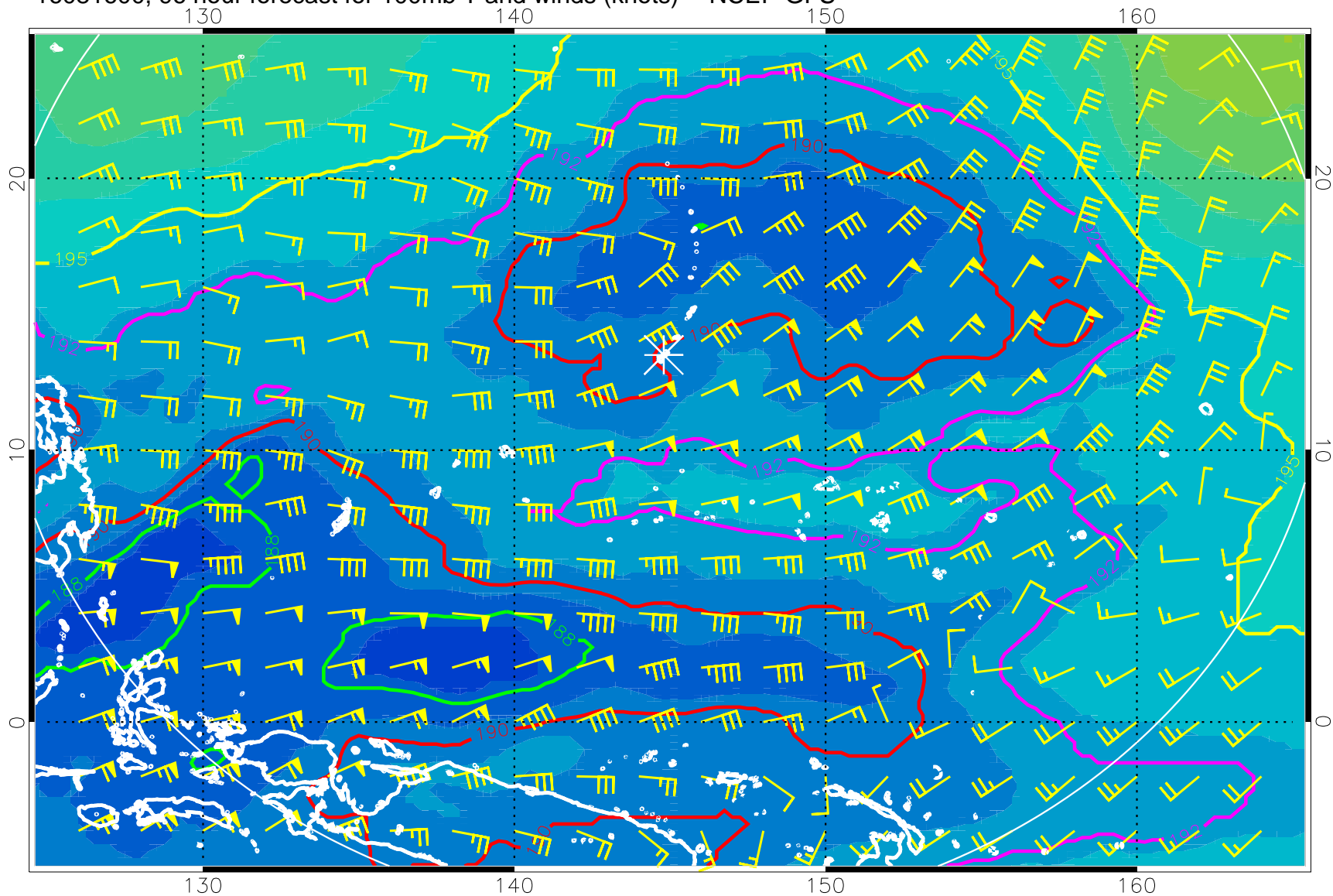
16081600, 96 hour forecast for 100mb T and winds (knots) -- NCEP GFS
