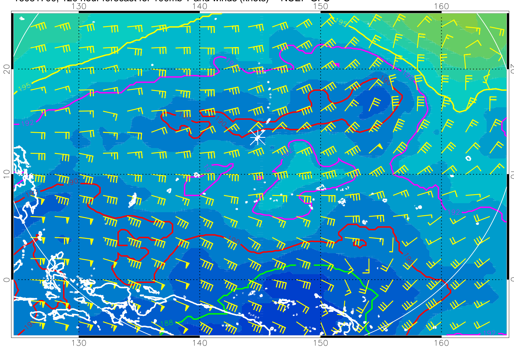
16081700, 120 hour forecast for 100mb T and winds (knots) -- NCEP GFS
