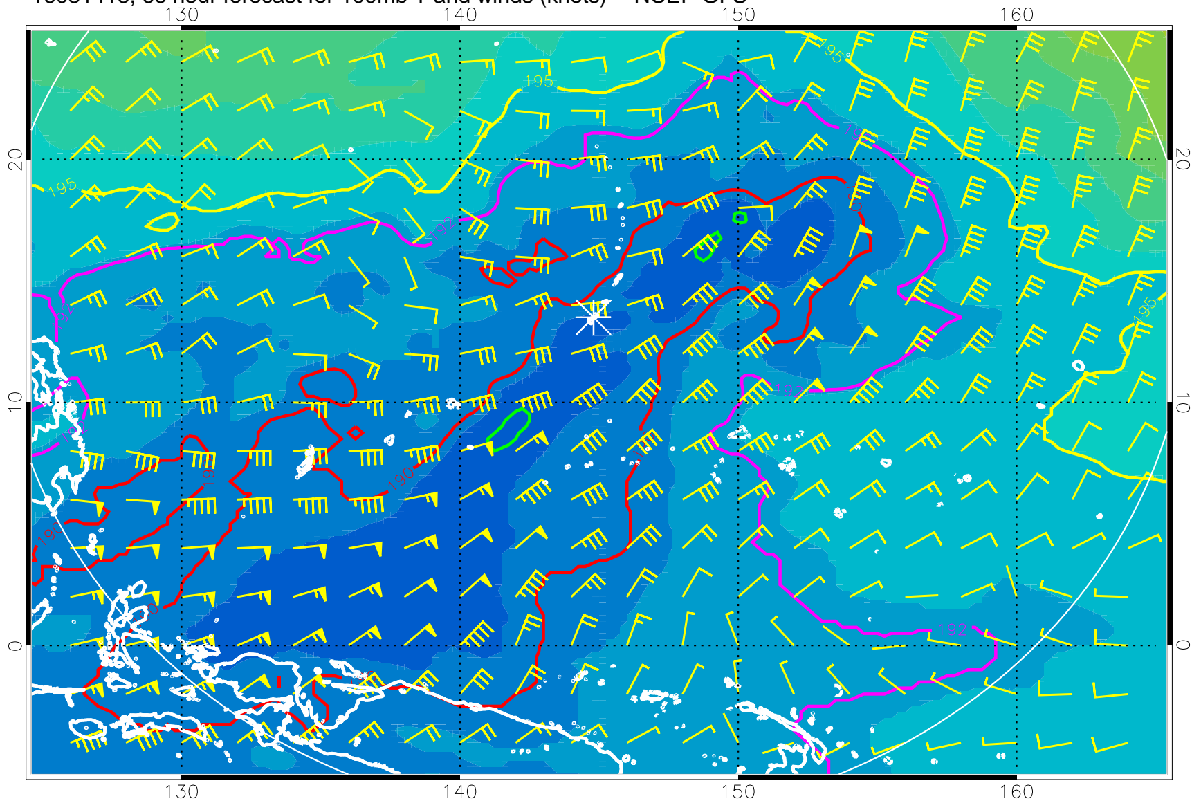
16081418, 66 hour forecast for 100mb T and winds (knots) -- NCEP GFS
