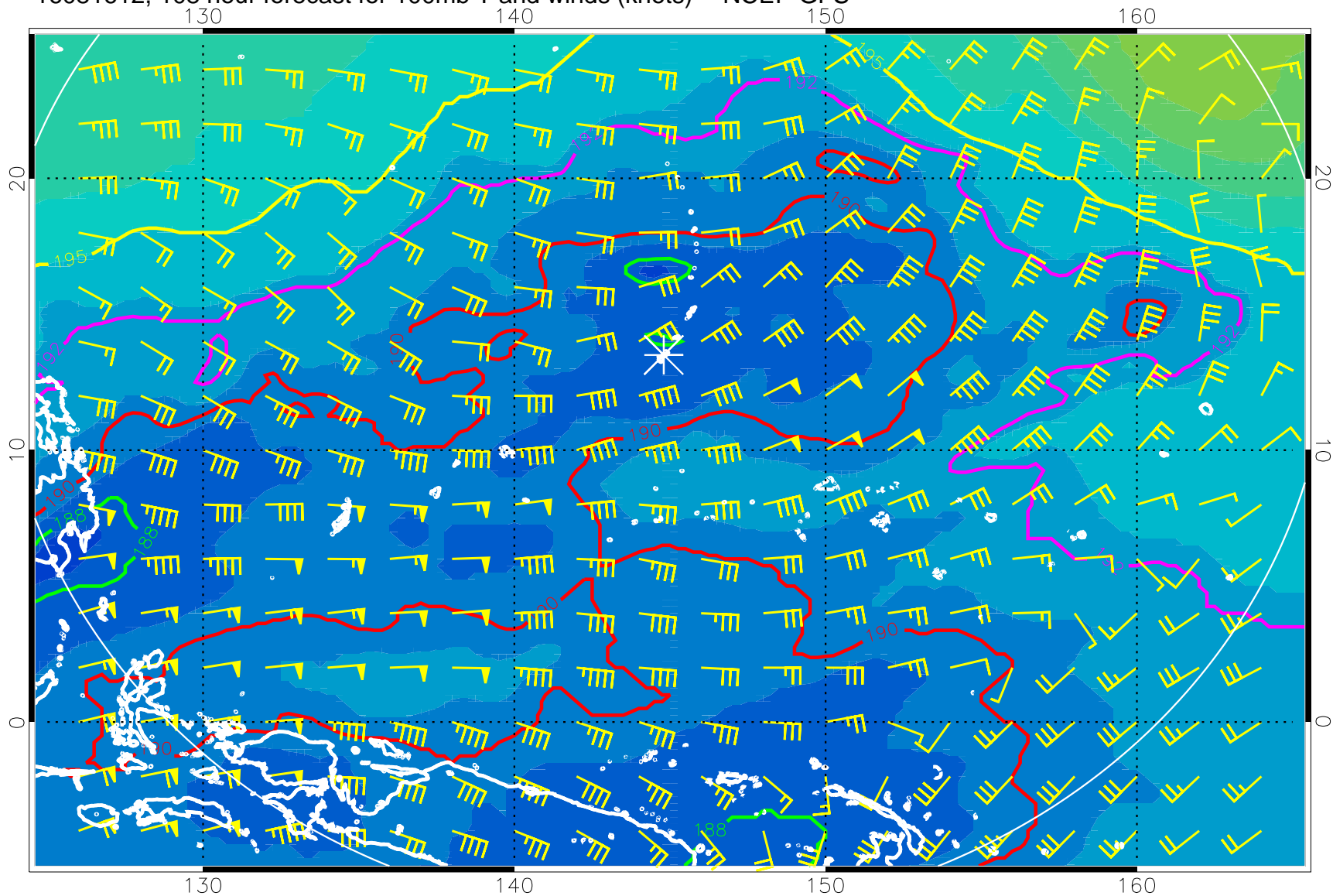
16081612, 108 hour forecast for 100mb T and winds (knots) -- NCEP GFS
