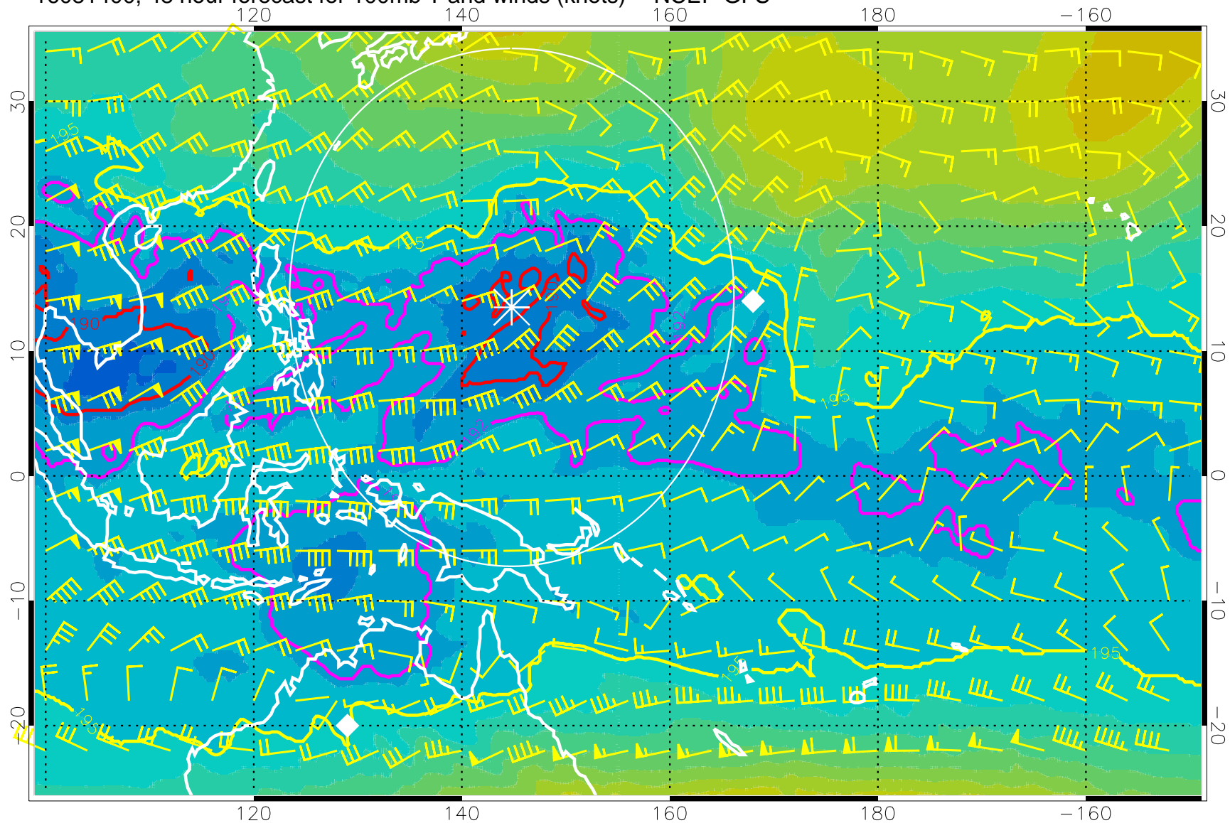
16081400, 48 hour forecast for 100mb T and winds (knots) -- NCEP GFS
