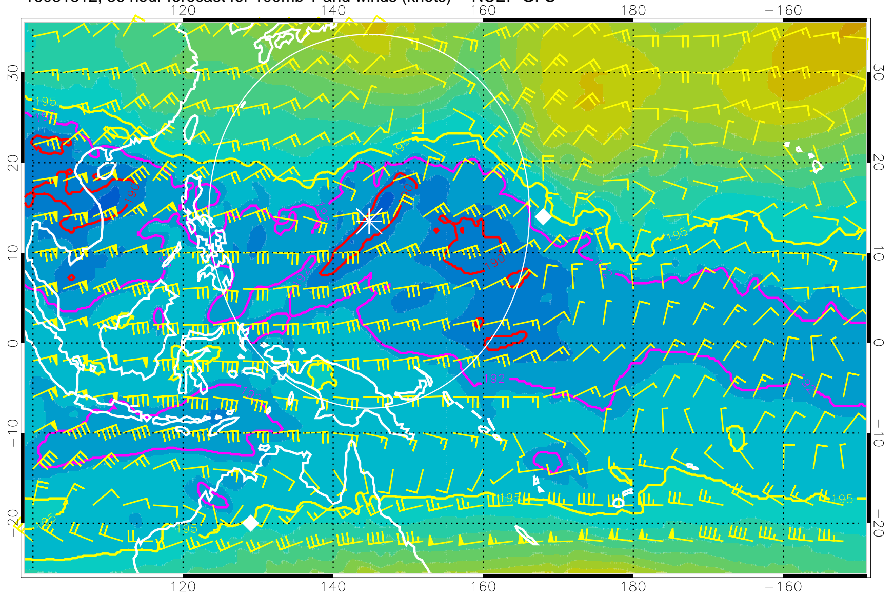
16081312, 36 hour forecast for 100mb T and winds (knots) -- NCEP GFS
