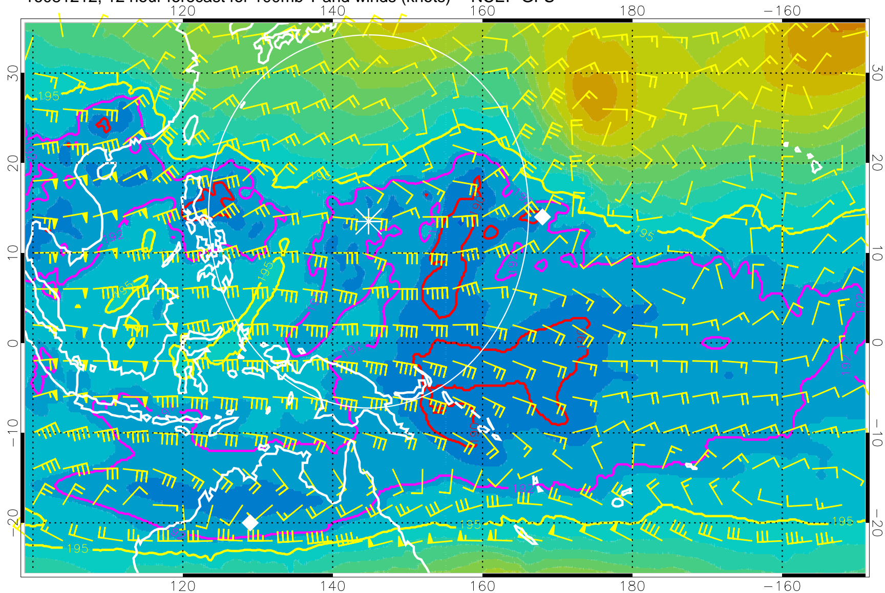
16081212, 12 hour forecast for 100mb T and winds (knots) -- NCEP GFS
