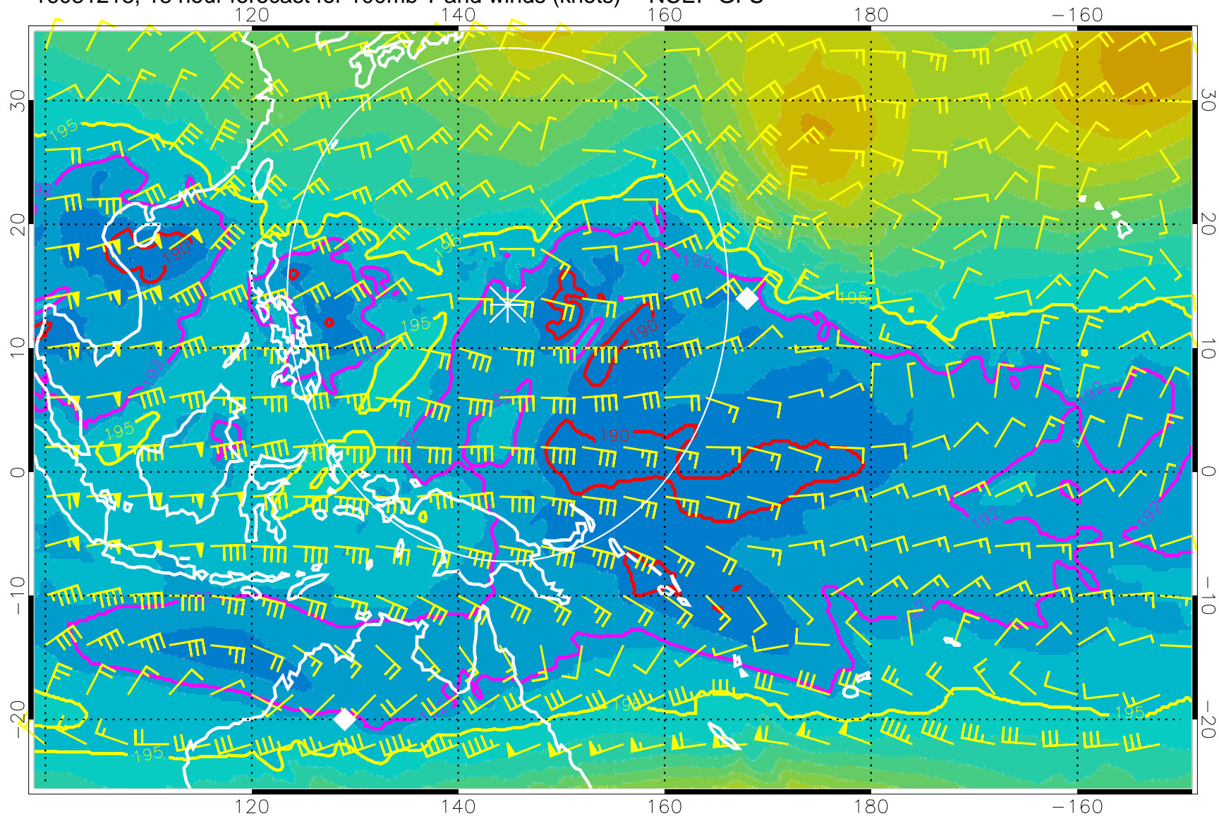
16081218, 18 hour forecast for 100mb T and winds (knots) -- NCEP GFS
