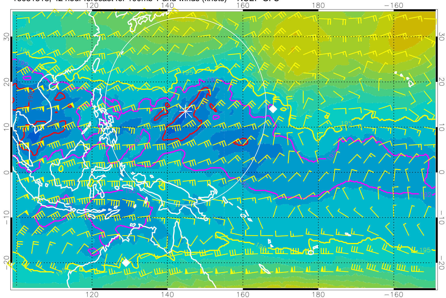
16081318, 42 hour forecast for 100mb T and winds (knots) -- NCEP GFS
