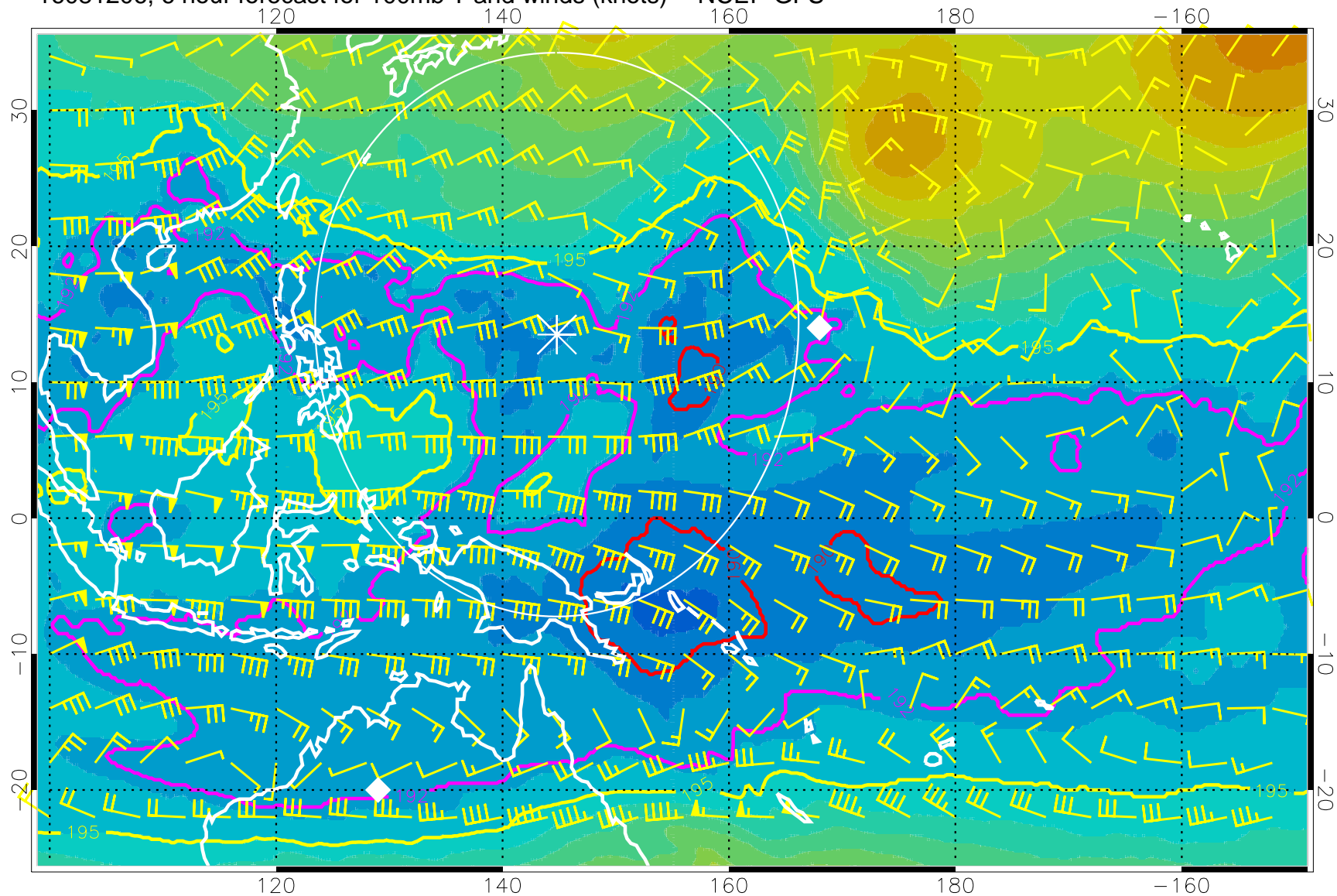
16081206, 6 hour forecast for 100mb T and winds (knots) -- NCEP GFS
