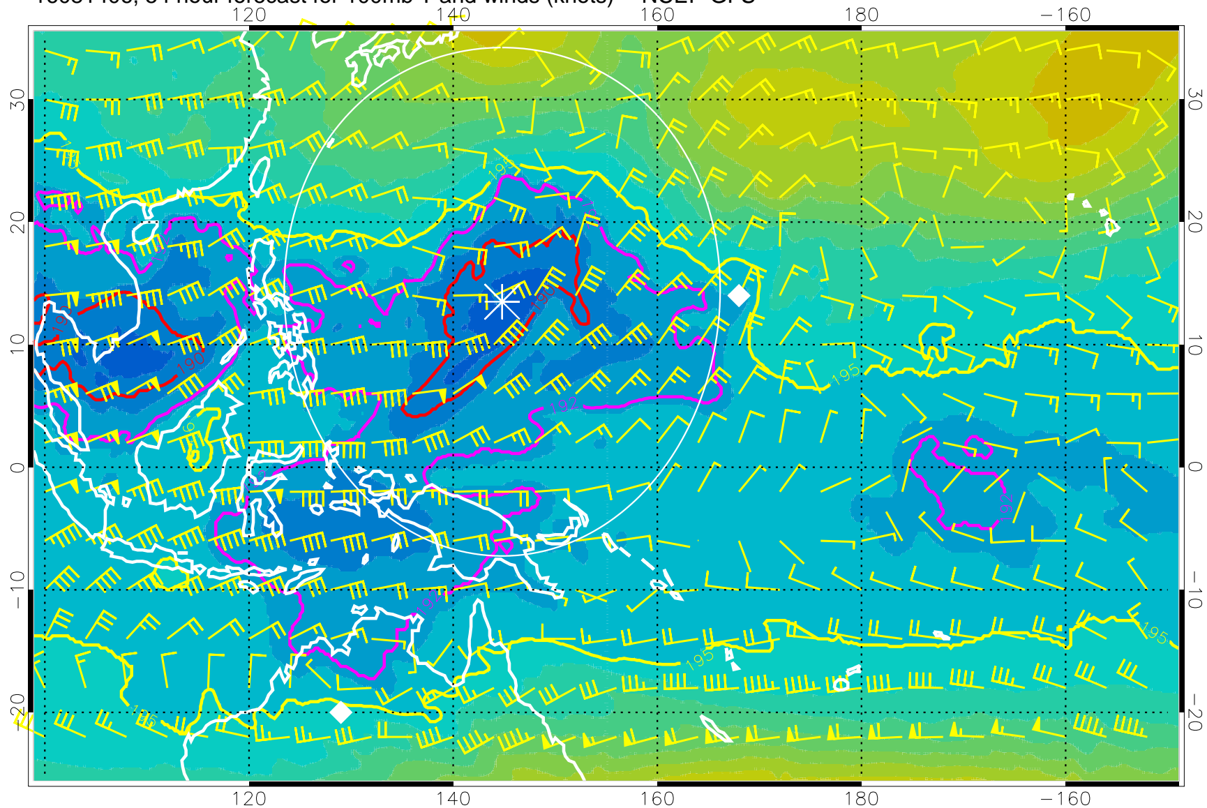
16081406, 54 hour forecast for 100mb T and winds (knots) -- NCEP GFS
