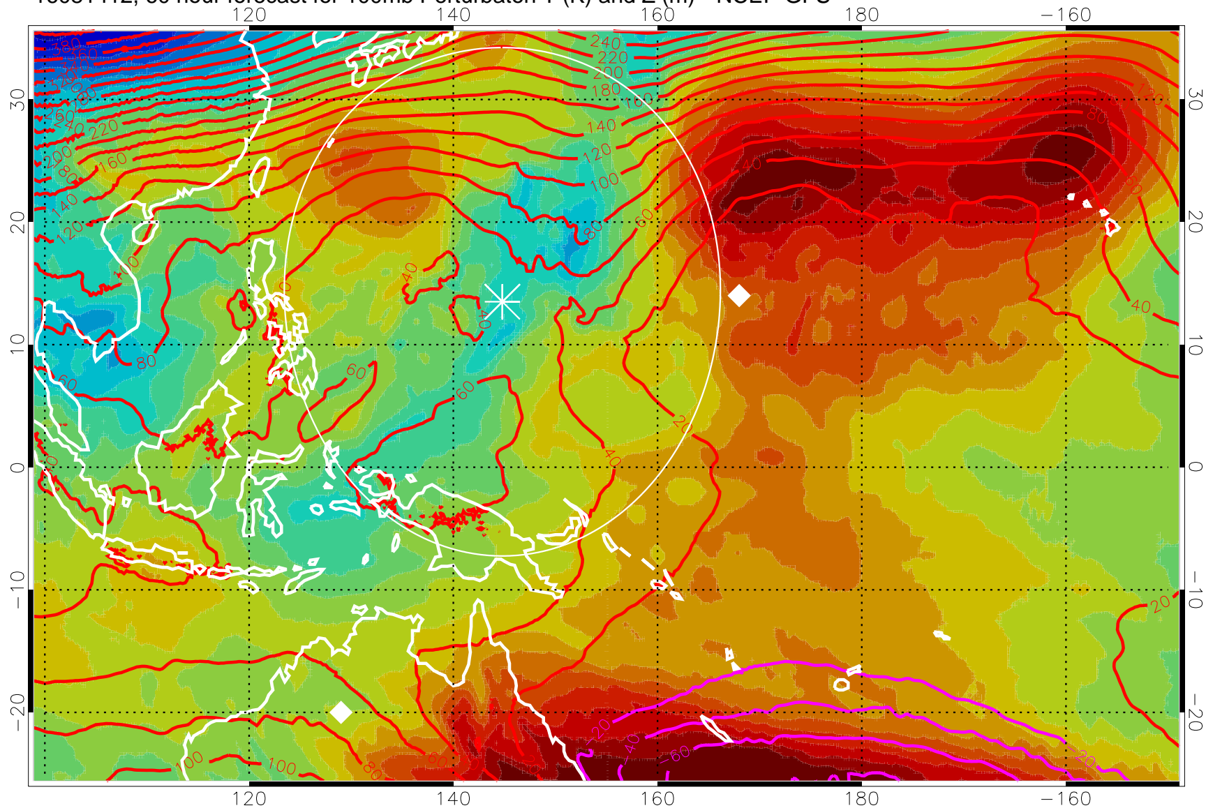
16081412, 60 hour forecast for 100mb Perturbation T (K) and Z (m)-- NCEP GFS
