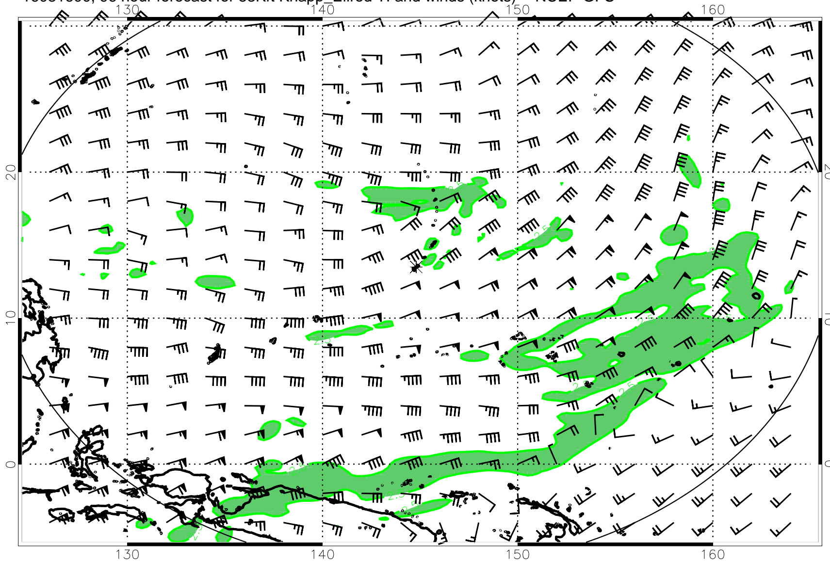
16081600, 96 hour forecast for 53Kft Knapp_Ellrod TI and winds (knots) -- NCEP GFS
