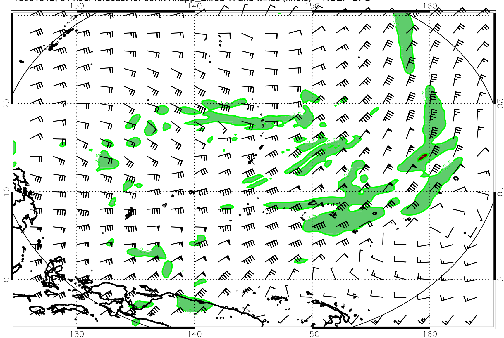
16081512, 84 hour forecast for 53Kft Knapp_Ellrod TI and winds (knots) -- NCEP GFS
