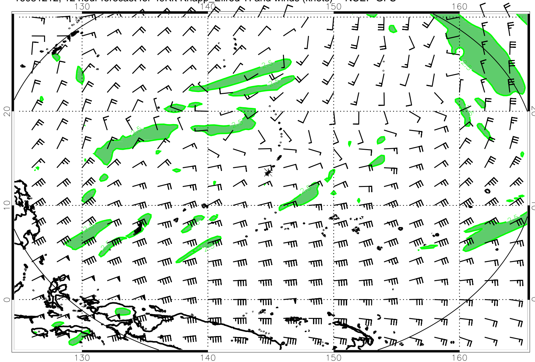
16081212, 12 hour forecast for 49Kft Knapp_Ellrod TI and winds (knots) -- NCEP GFS
