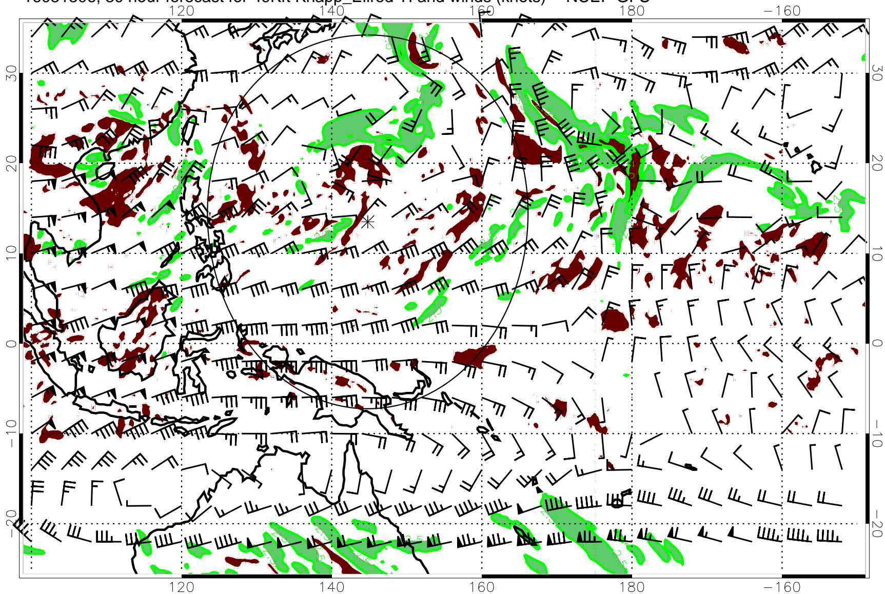
16081306, 30 hour forecast for 49Kft Knapp_Ellrod TI and winds (knots) -- NCEP GFS
