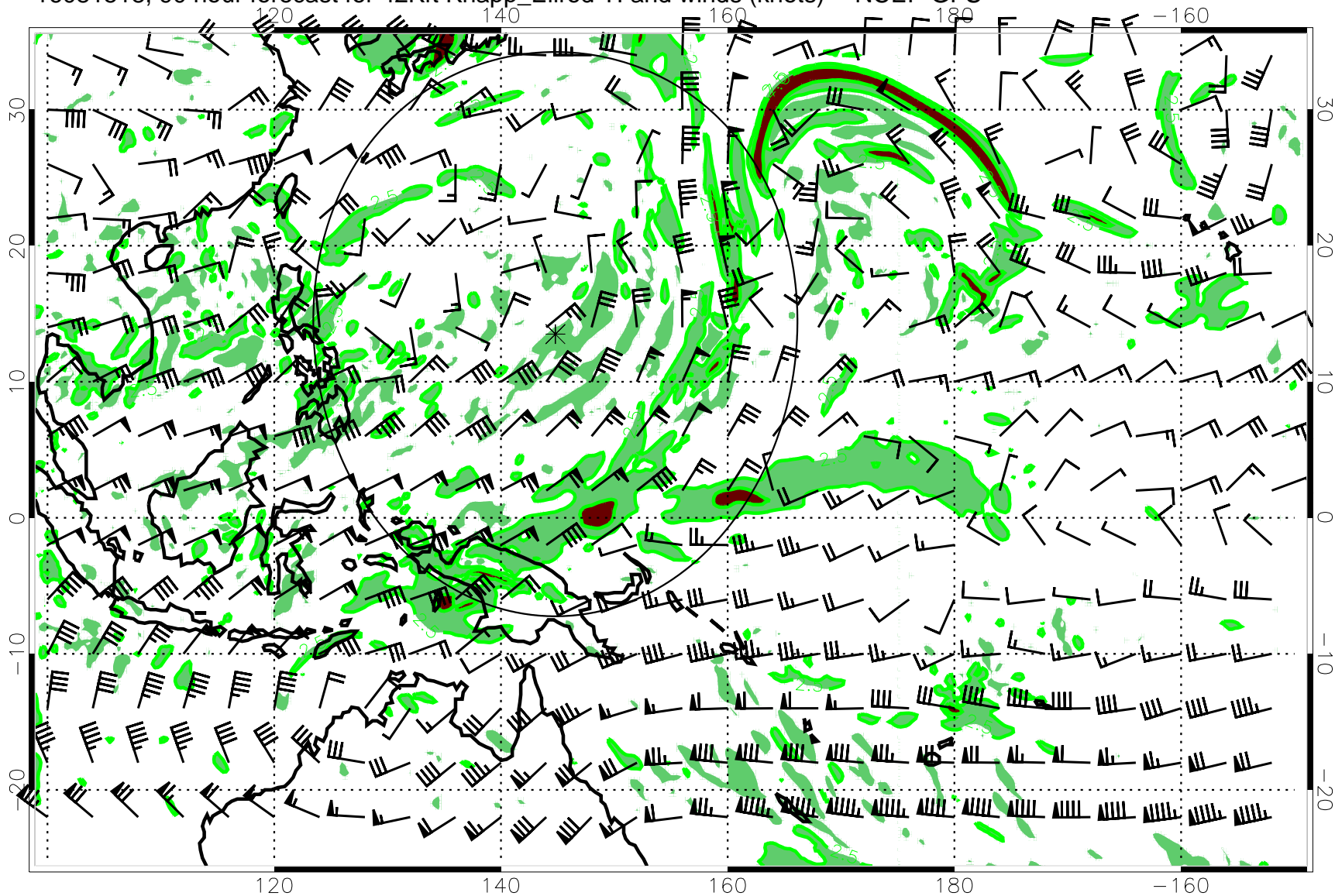
16081518, 90 hour forecast for 42Kft Knapp_Ellrod TI and winds (knots) -- NCEP GFS
