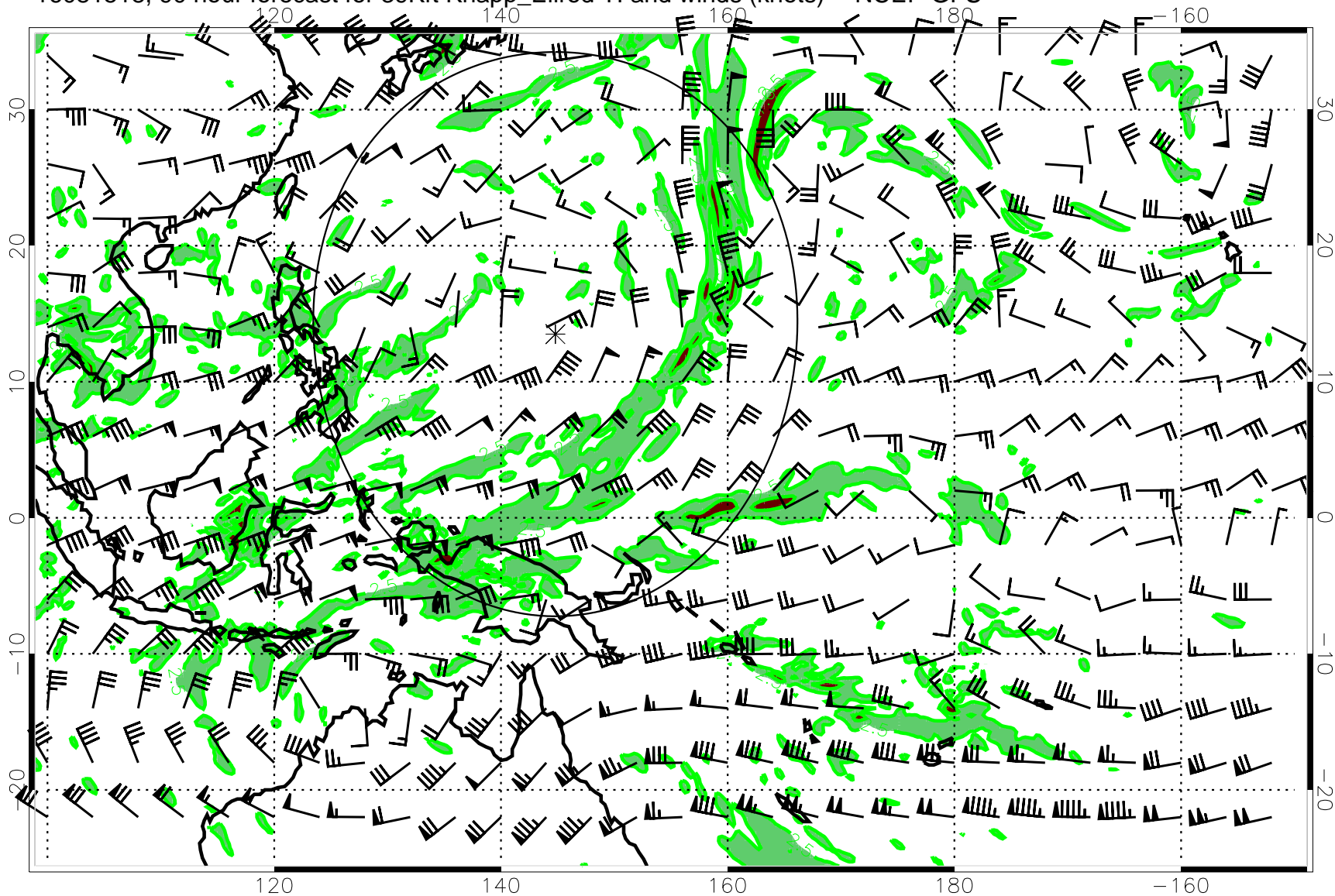
16081518, 90 hour forecast for 39Kft Knapp_Ellrod TI and winds (knots) -- NCEP GFS
