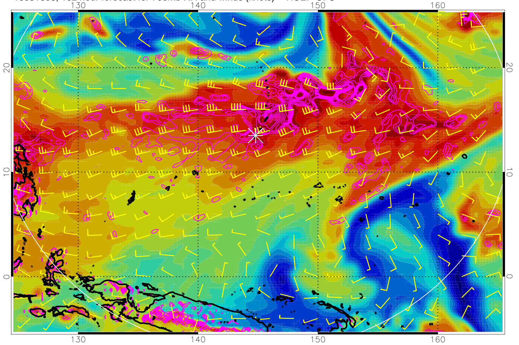
16081606, 102 hour forecast for 700mb RH and winds (knots) -- NCEP GFS
