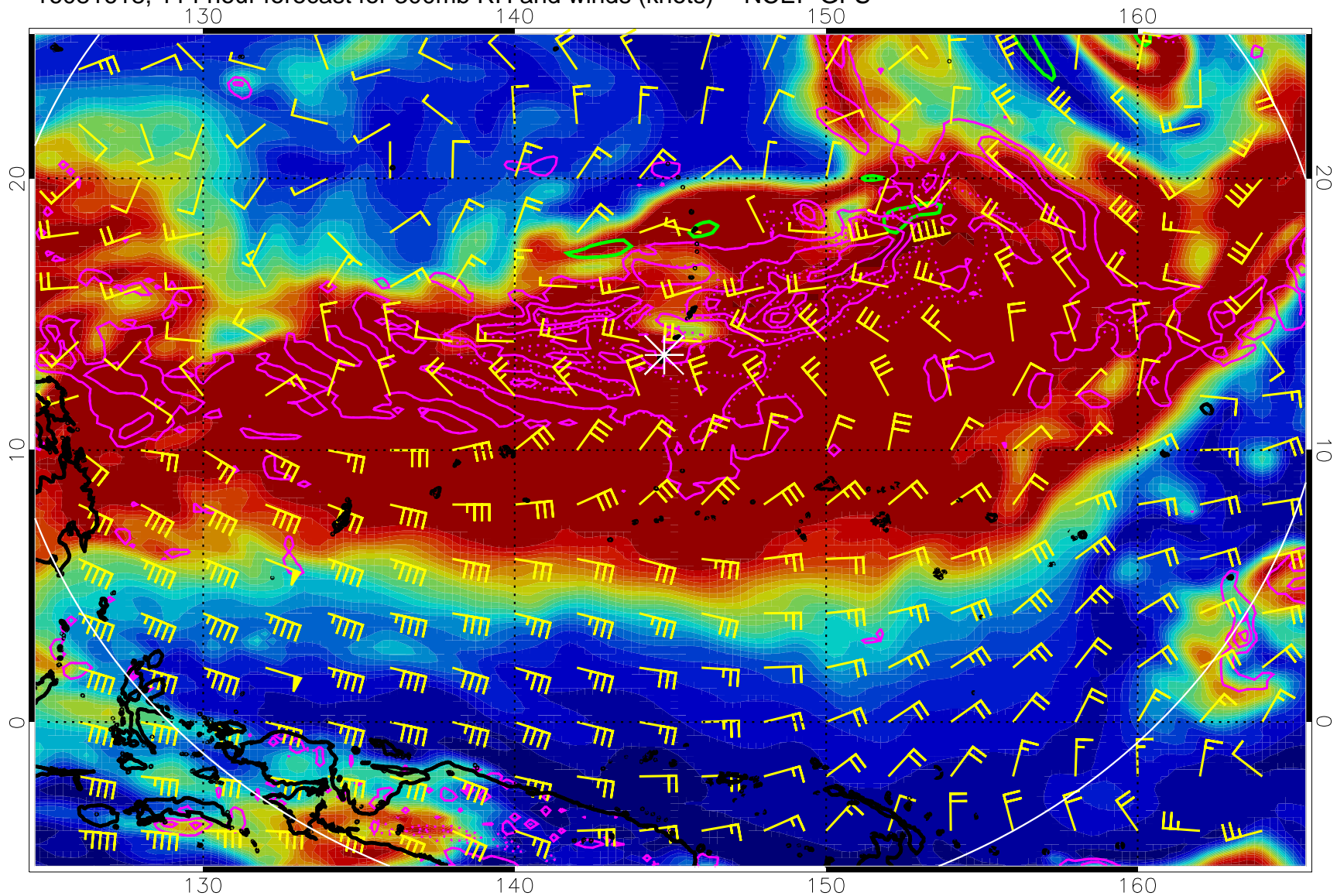
16081618, 114 hour forecast for 300mb RH and winds (knots) -- NCEP GFS
