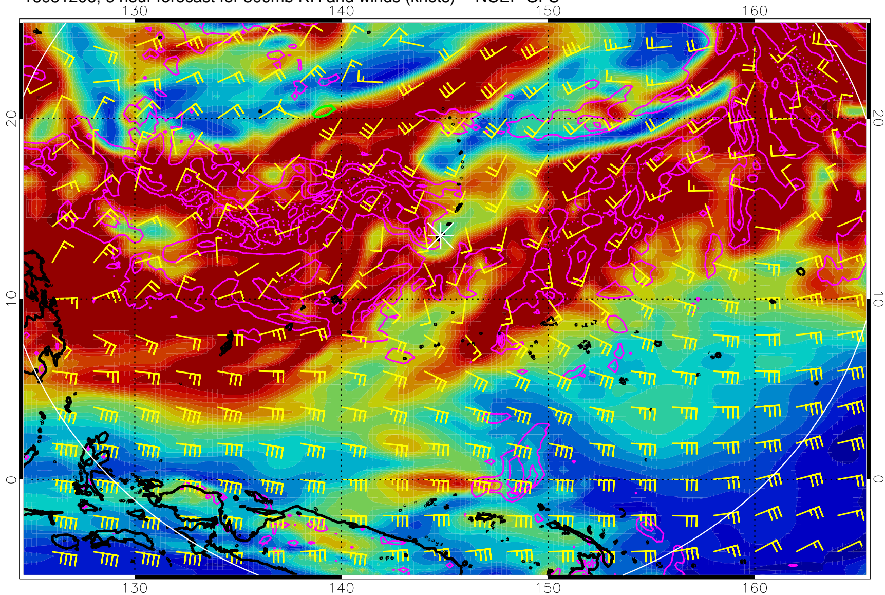
16081206, 6 hour forecast for 300mb RH and winds (knots) -- NCEP GFS
