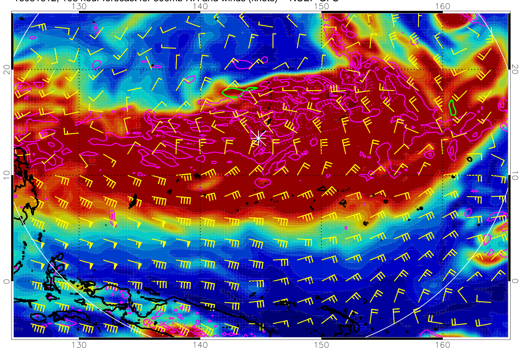
16081612, 108 hour forecast for 300mb RH and winds (knots) -- NCEP GFS
