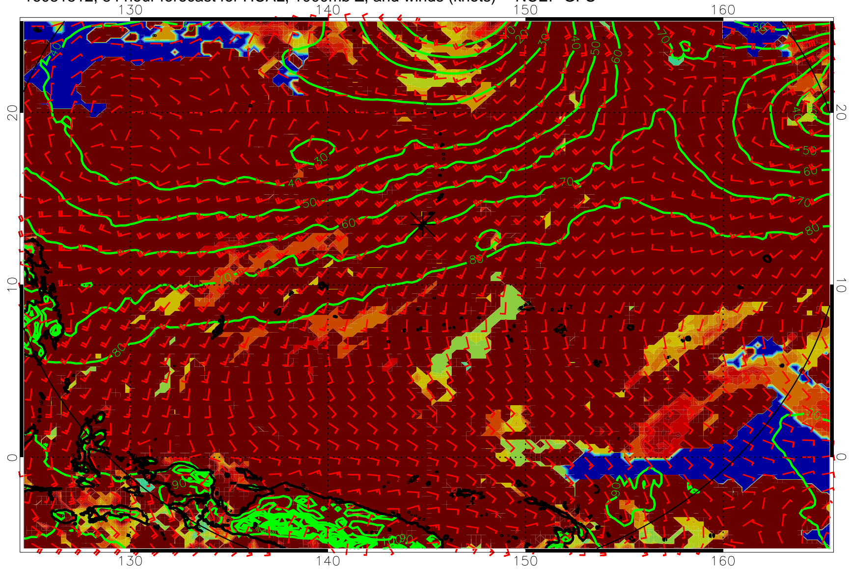
16081512, 84 hour forecast for HCAL, 1000mb Z, and winds (knots) -- NCEP GFS
