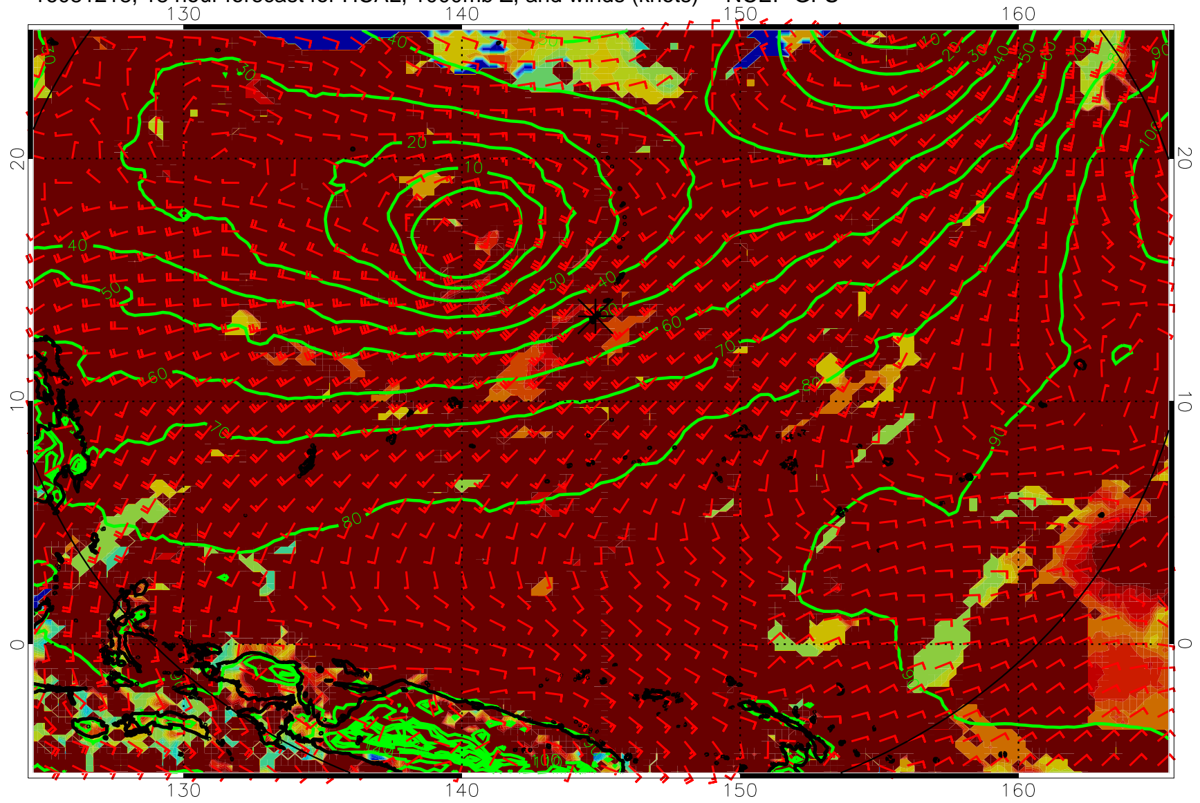
16081218, 18 hour forecast for HCAL, 1000mb Z, and winds (knots) -- NCEP GFS
