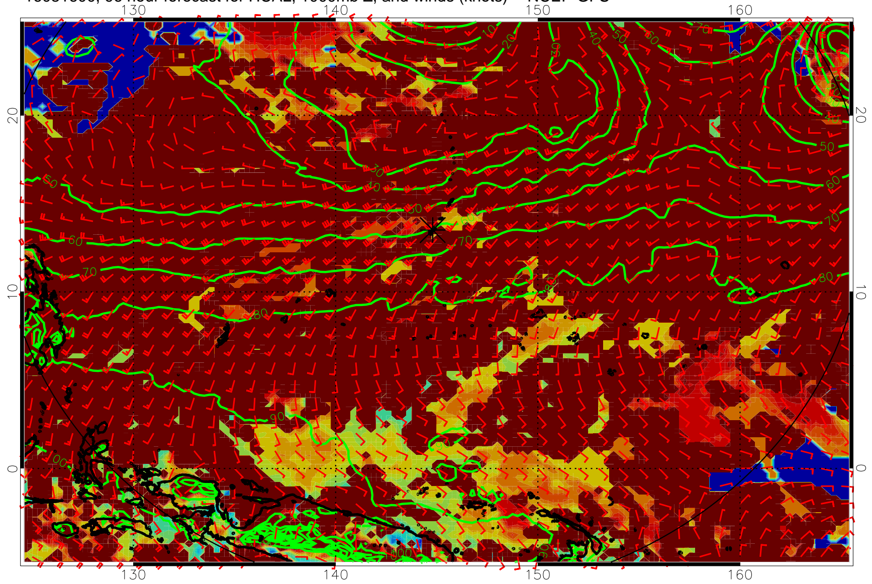
16081600, 96 hour forecast for HCAL, 1000mb Z, and winds (knots) -- NCEP GFS
