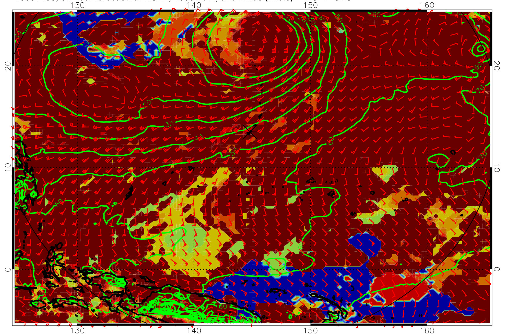
16081406, 54 hour forecast for HCAL, 1000mb Z, and winds (knots) -- NCEP GFS
