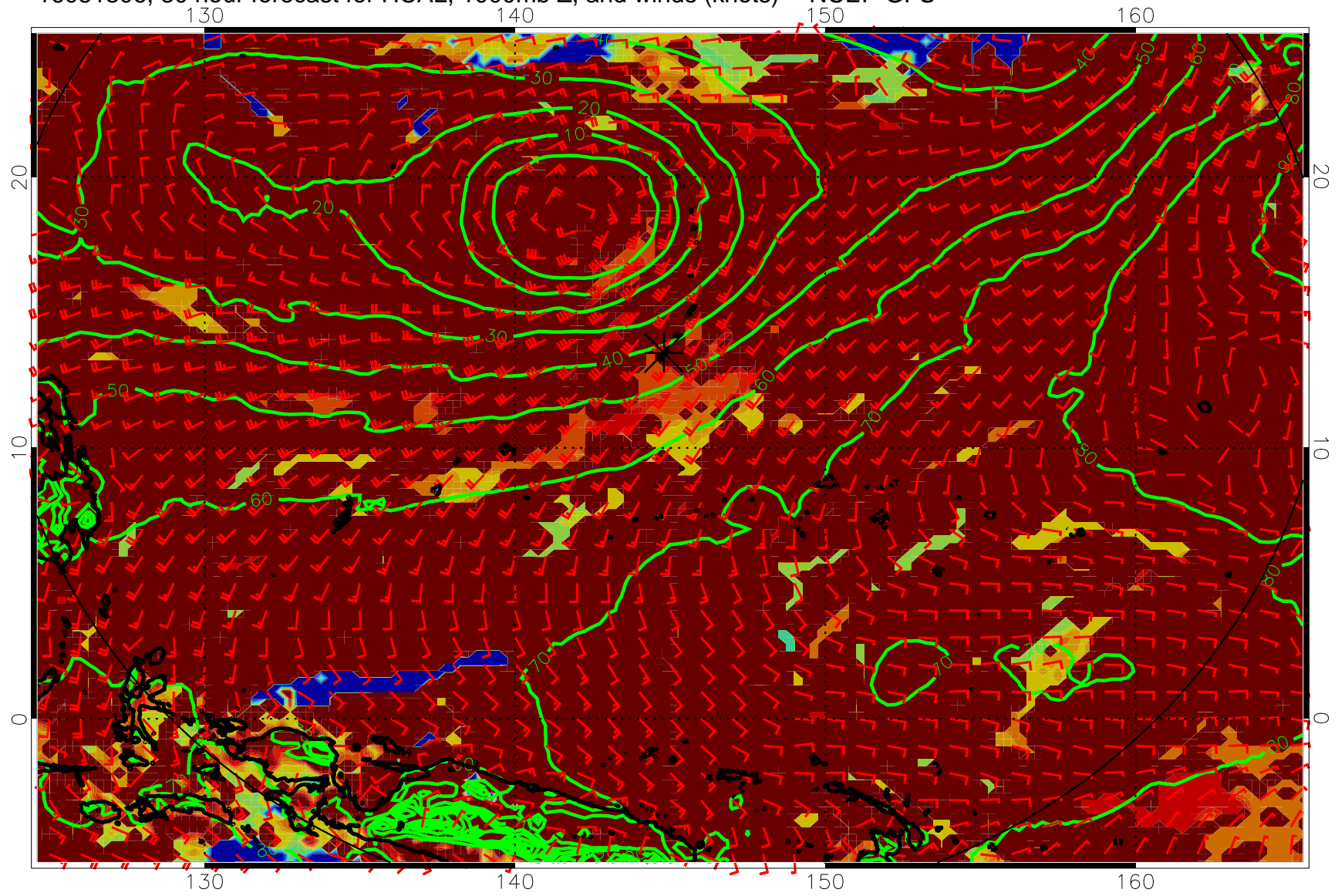
16081306, 30 hour forecast for HCAL, 1000mb Z, and winds (knots) -- NCEP GFS
