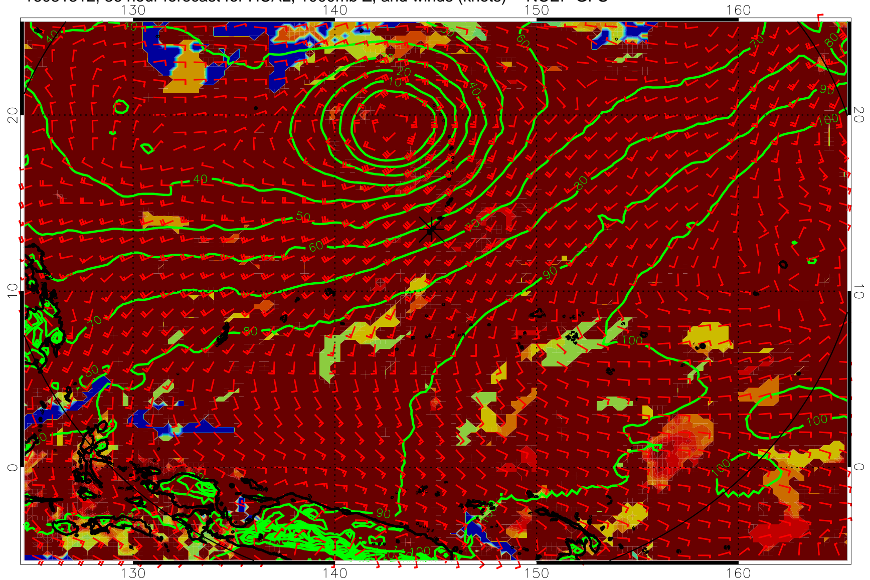
16081312, 36 hour forecast for HCAL, 1000mb Z, and winds (knots) -- NCEP GFS
