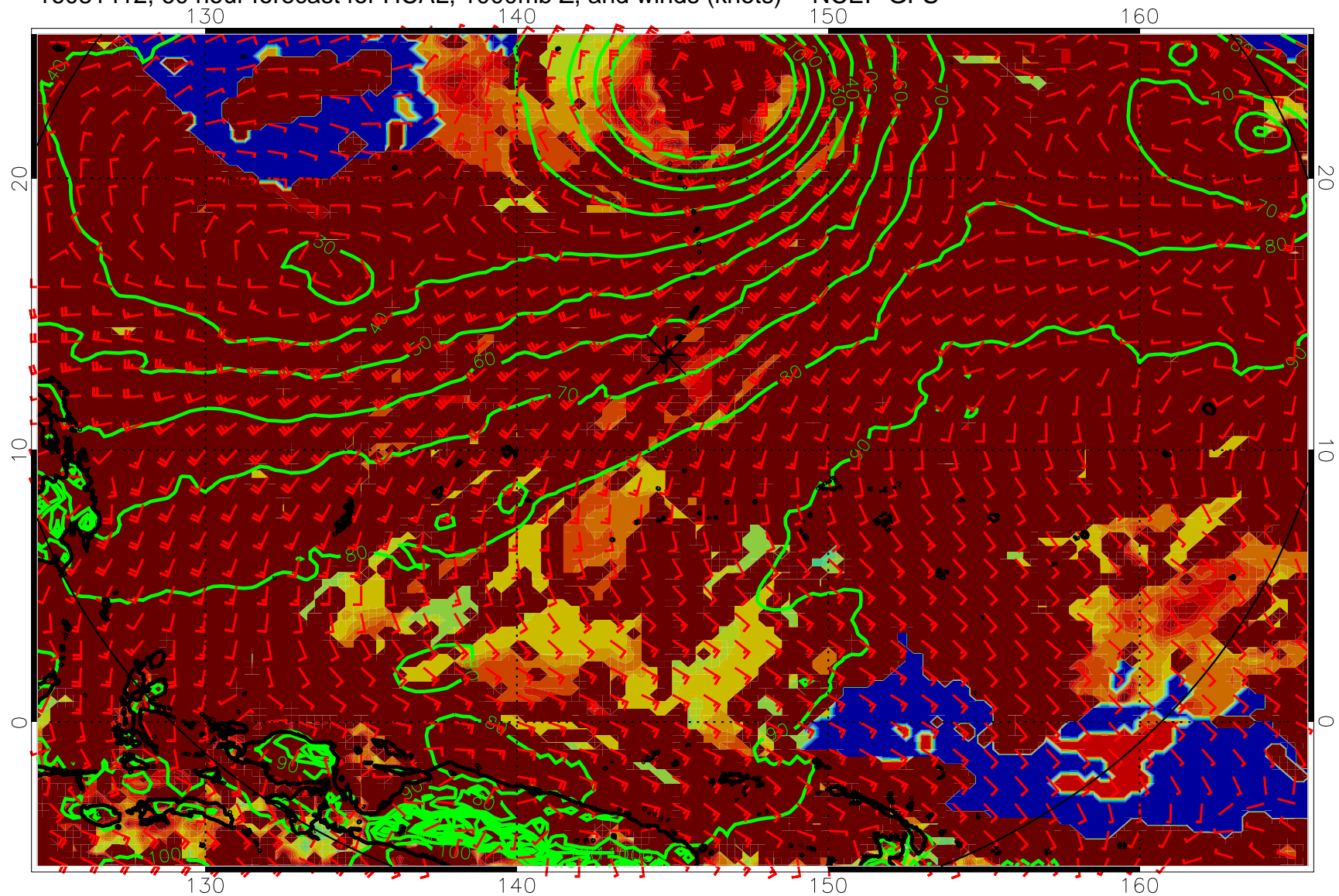
16081412, 60 hour forecast for HCAL, 1000mb Z, and winds (knots) -- NCEP GFS
