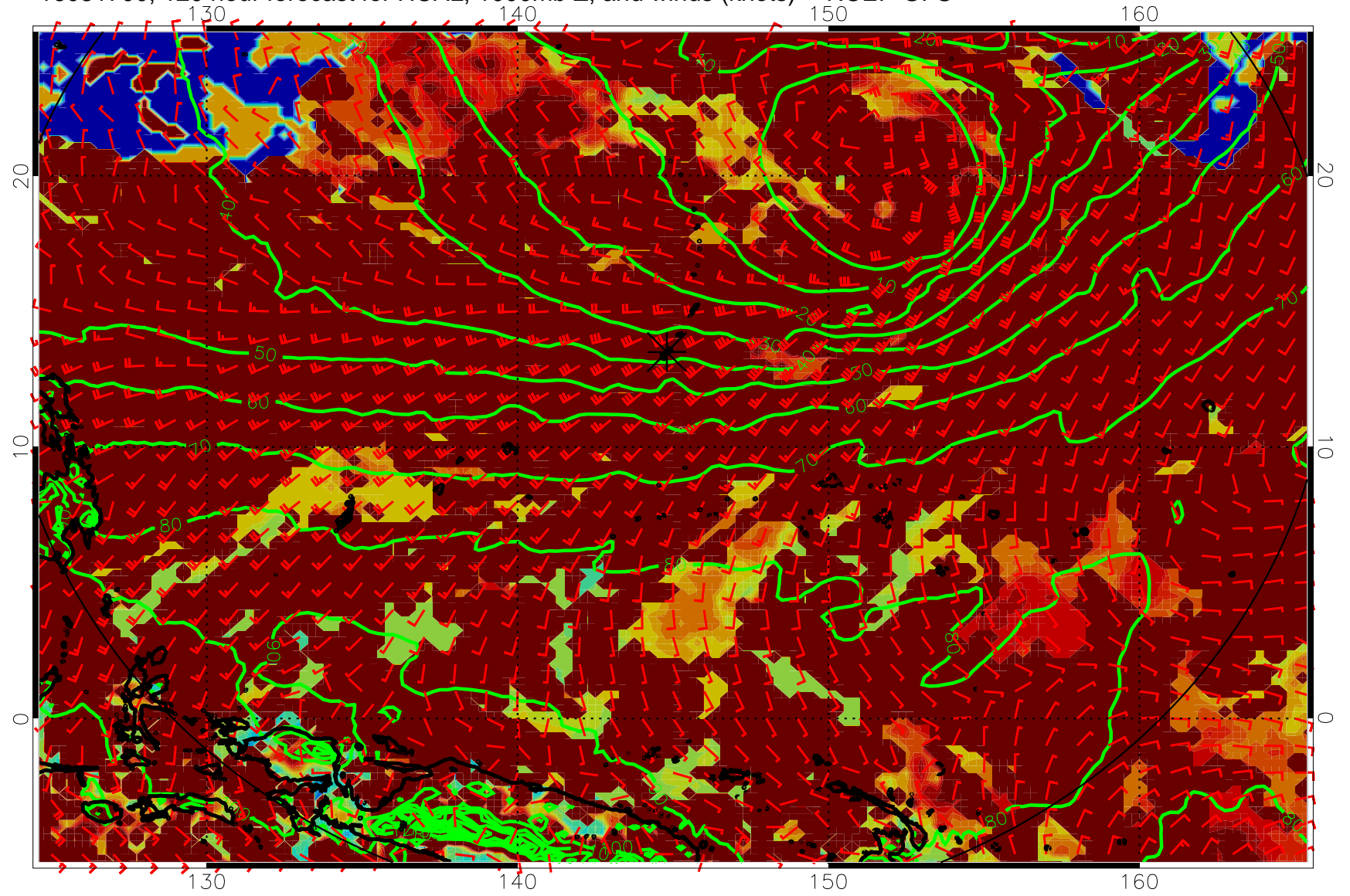
16081700, 120 hour forecast for HCAL, 1000mb Z, and winds (knots) -- NCEP GFS
