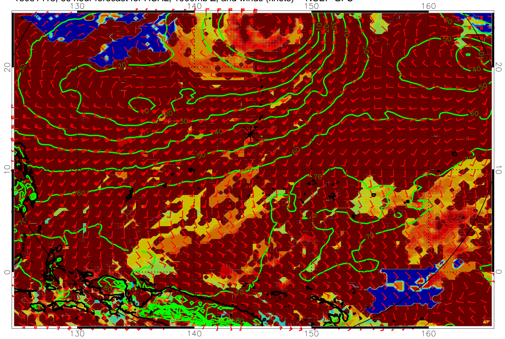
16081418, 66 hour forecast for HCAL, 1000mb Z, and winds (knots) -- NCEP GFS
