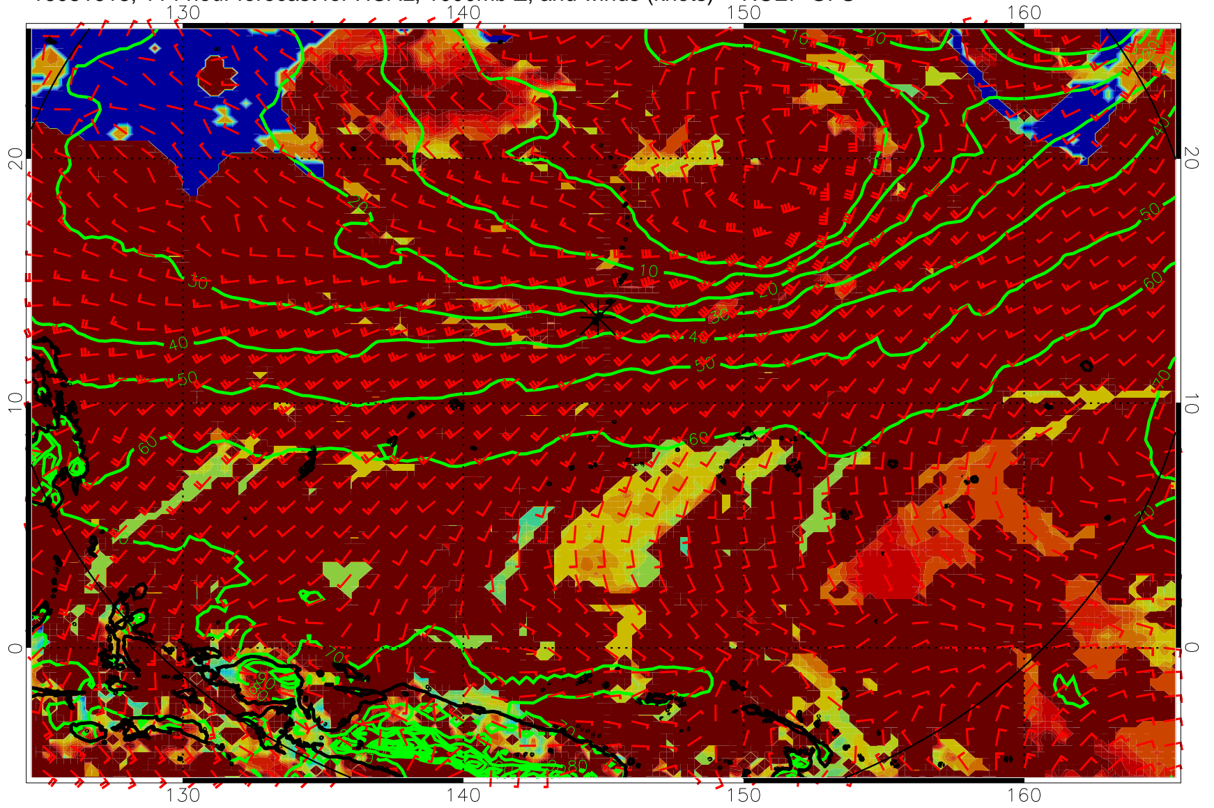
16081618, 114 hour forecast for HCAL, 1000mb Z, and winds (knots) -- NCEP GFS
