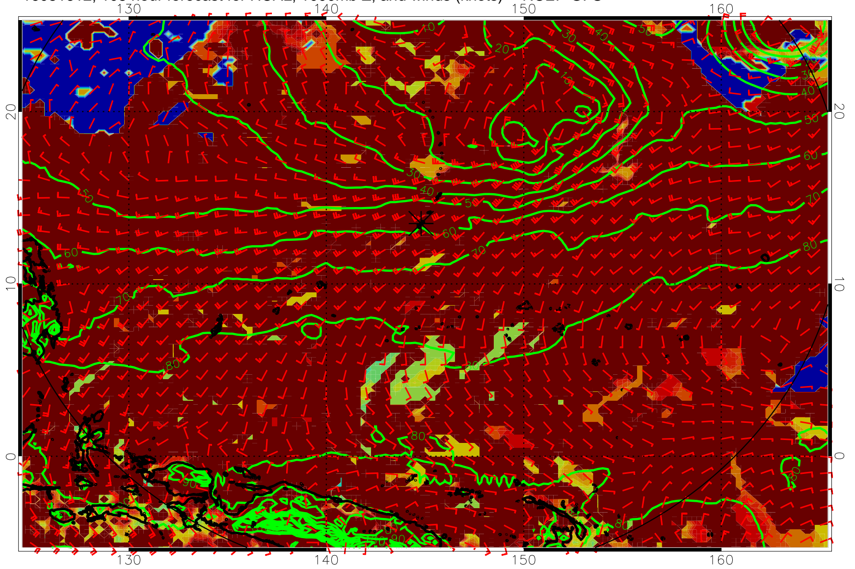
16081612, 108 hour forecast for HCAL, 1000mb Z, and winds (knots) -- NCEP GFS
