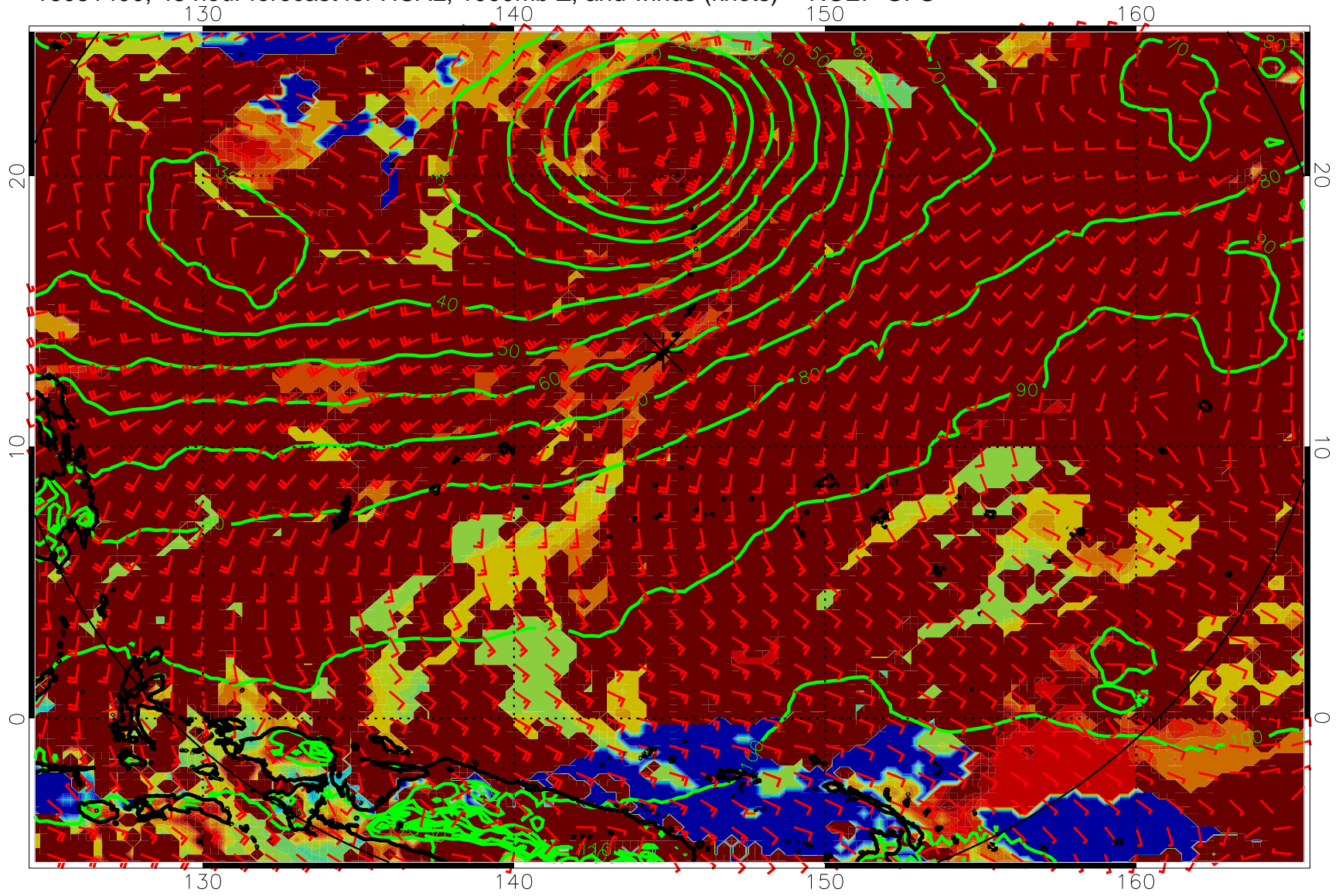
16081400, 48 hour forecast for HCAL, 1000mb Z, and winds (knots) -- NCEP GFS
