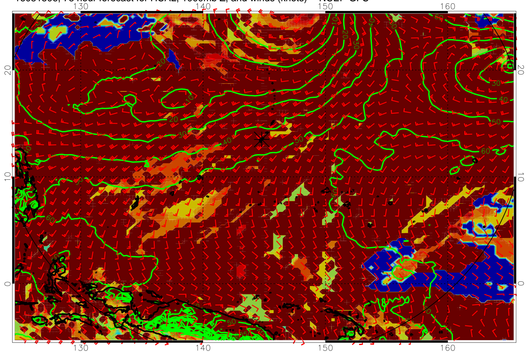
16081506, 78 hour forecast for HCAL, 1000mb Z, and winds (knots) -- NCEP GFS
