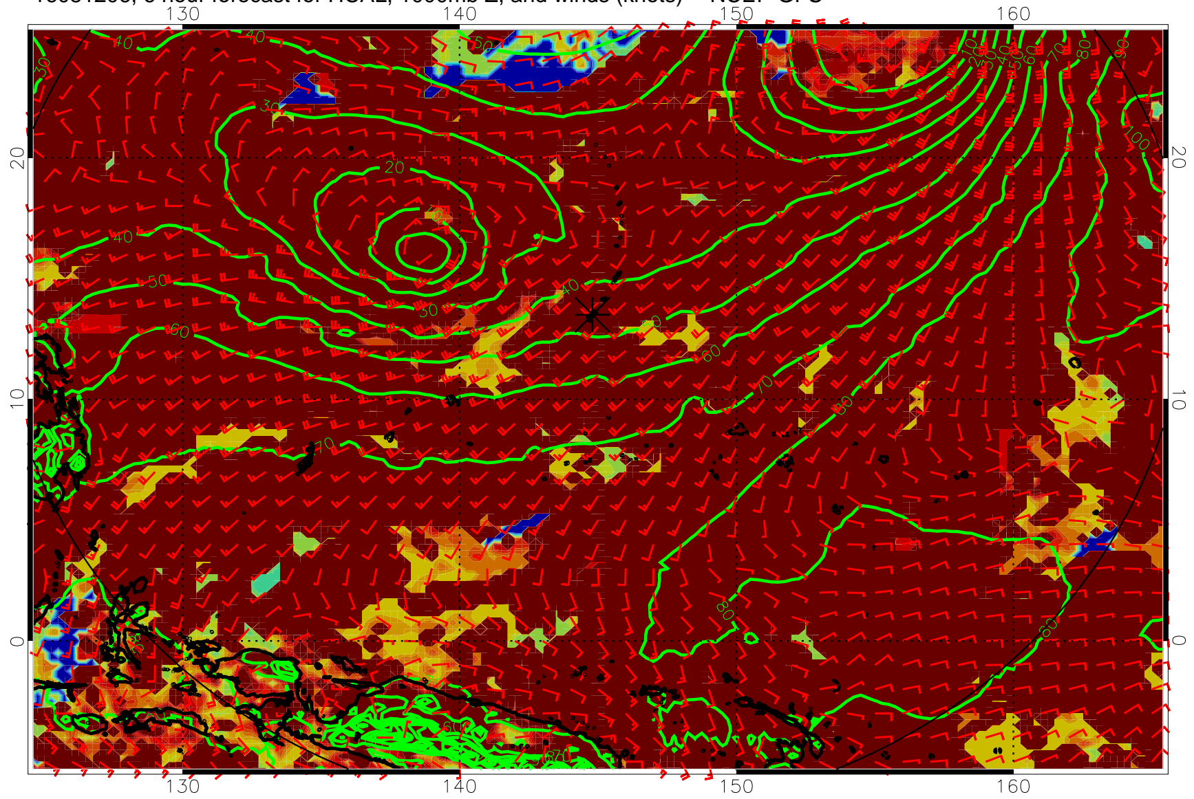
16081206, 6 hour forecast for HCAL, 1000mb Z, and winds (knots) -- NCEP GFS
