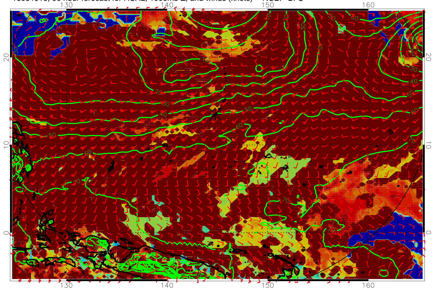
16081518, 90 hour forecast for HCAL, 1000mb Z, and winds (knots) -- NCEP GFS
