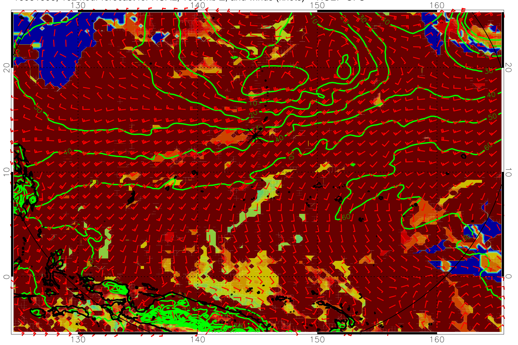
16081606, 102 hour forecast for HCAL, 1000mb Z, and winds (knots) -- NCEP GFS
