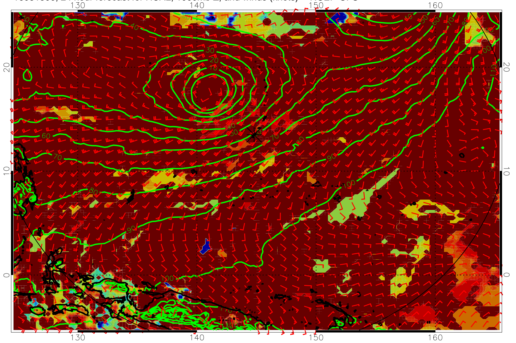
16081300, 24 hour forecast for HCAL, 1000mb Z, and winds (knots) -- NCEP GFS
