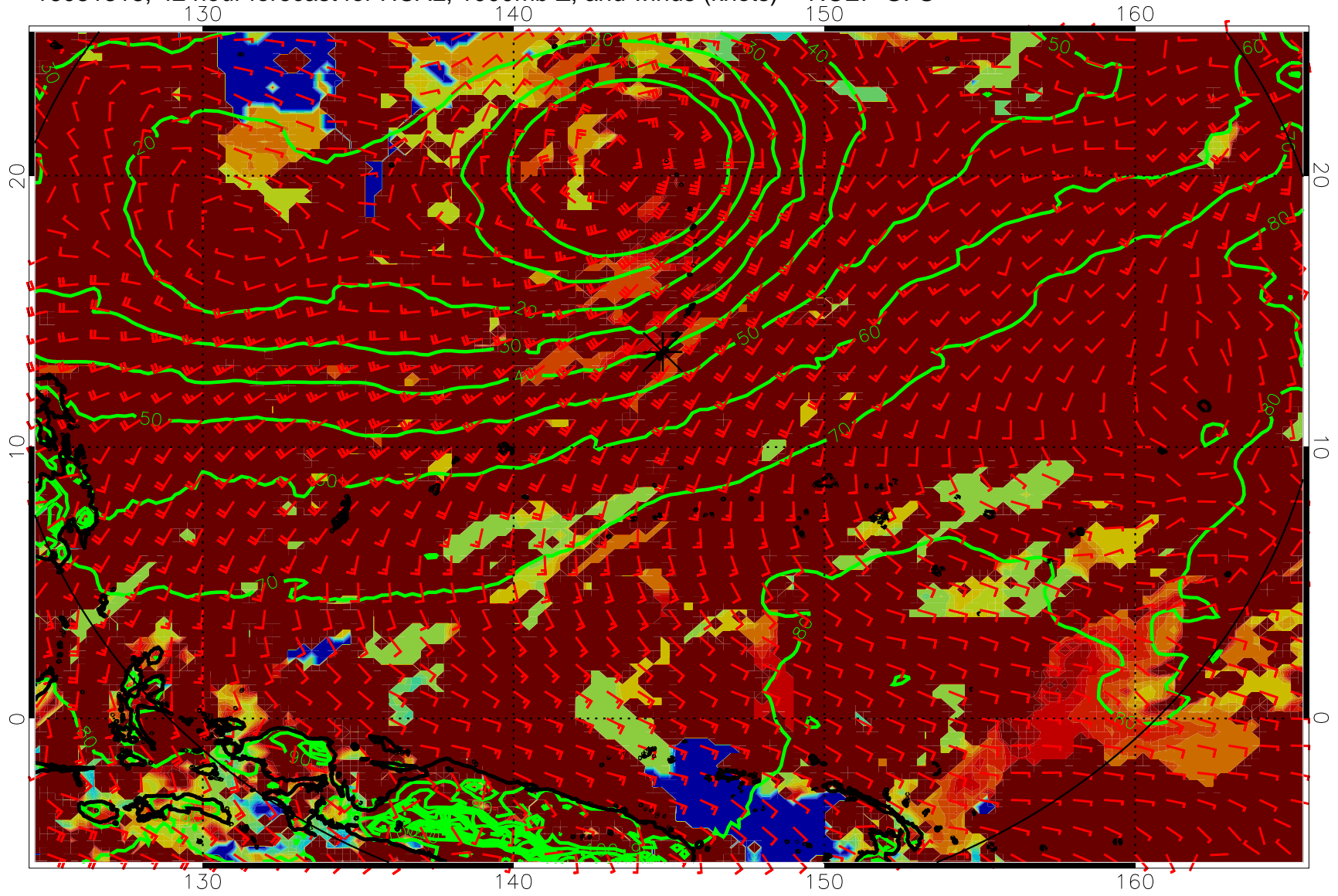
16081318, 42 hour forecast for HCAL, 1000mb Z, and winds (knots) -- NCEP GFS
