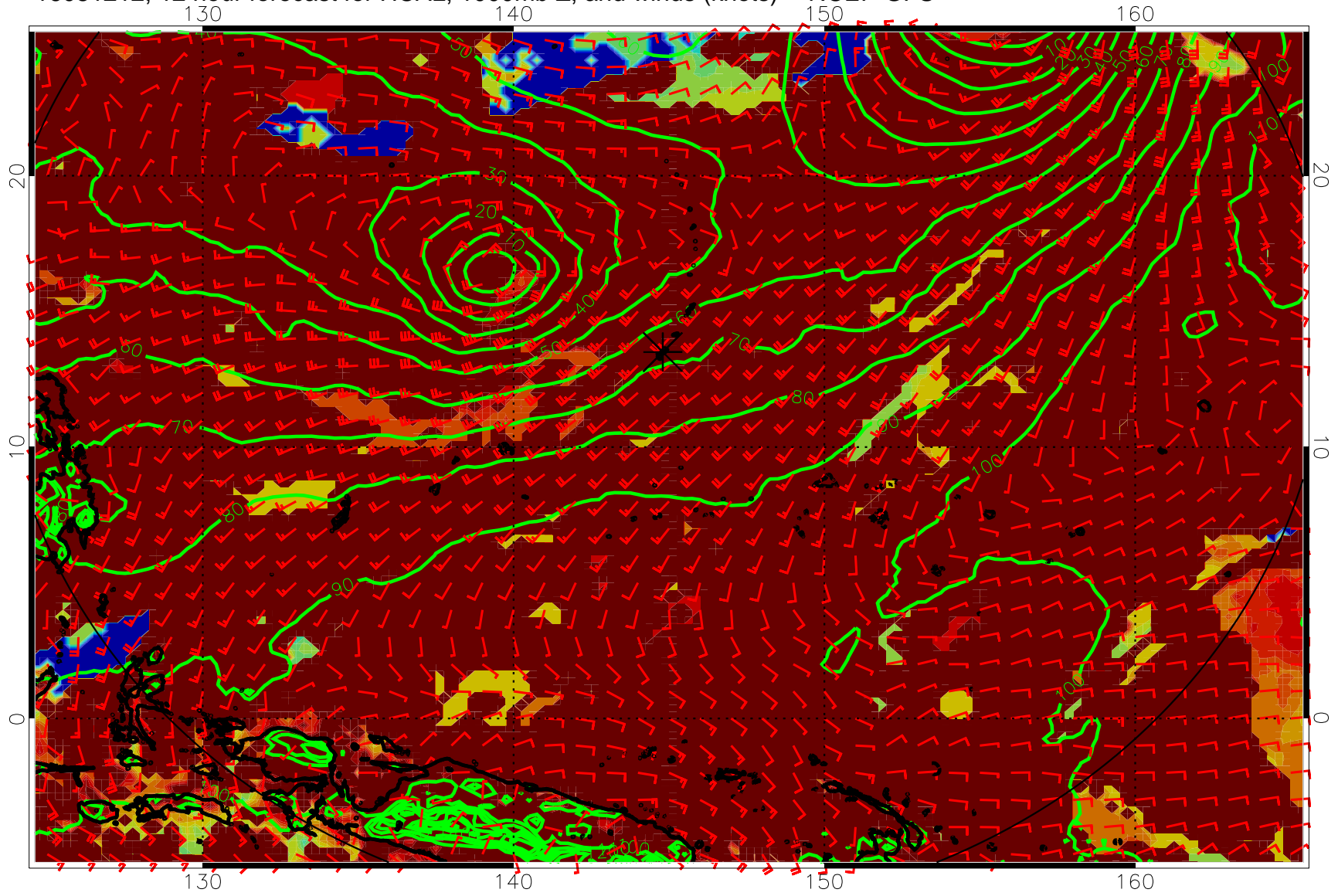
16081212, 12 hour forecast for HCAL, 1000mb Z, and winds (knots) -- NCEP GFS
