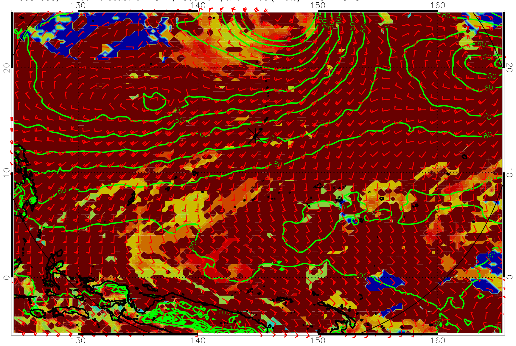
16081500, 72 hour forecast for HCAL, 1000mb Z, and winds (knots) -- NCEP GFS
