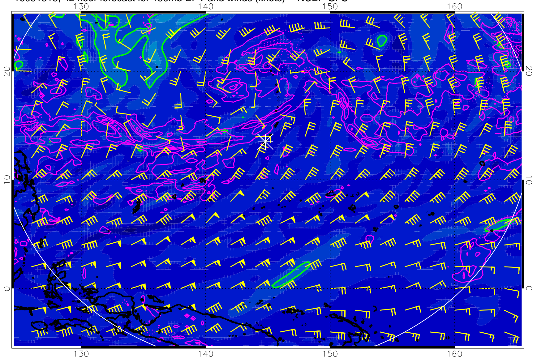
16081318, 42 hour forecast for 150mb EPV and winds (knots) -- NCEP GFS
