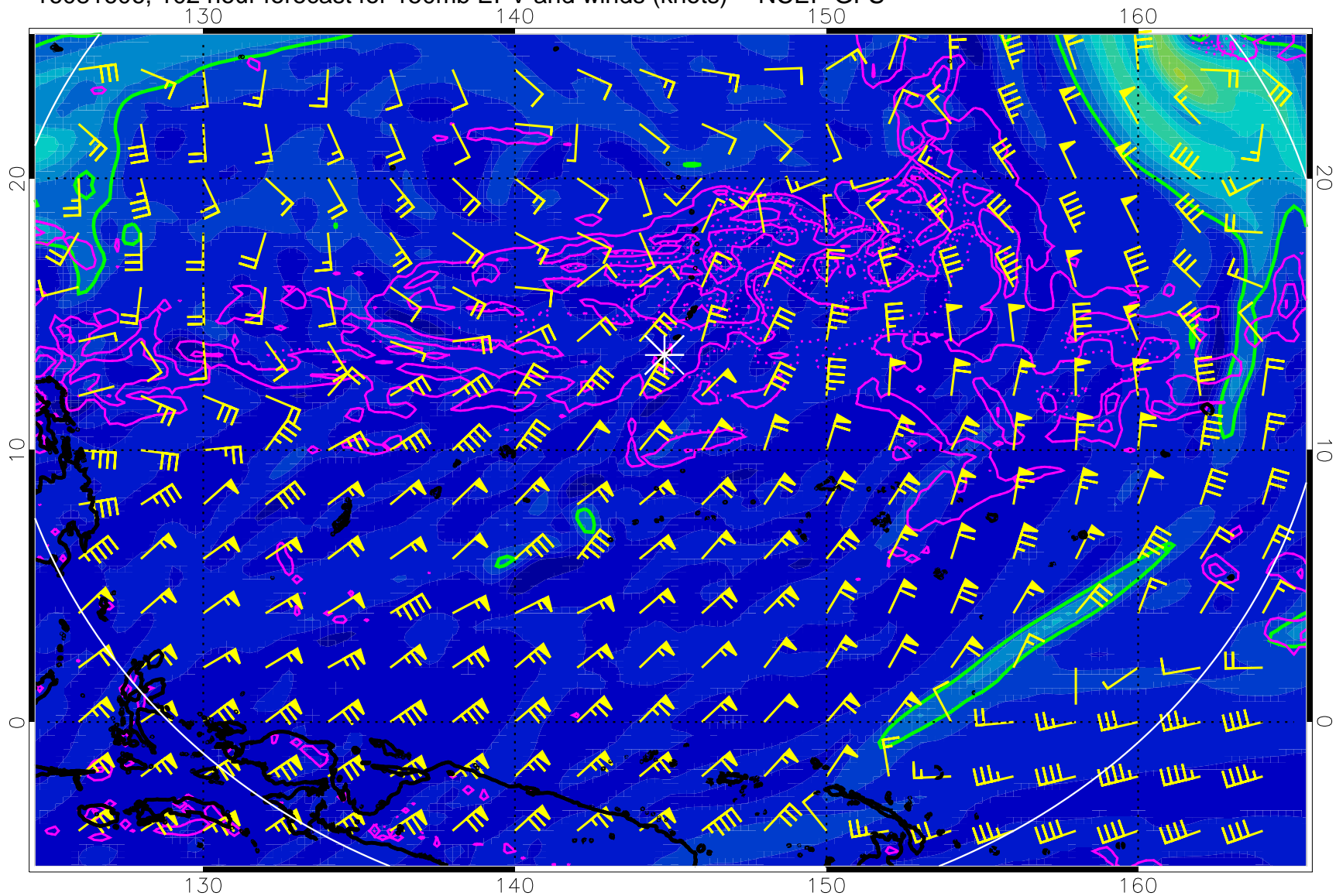
16081606, 102 hour forecast for 150mb EPV and winds (knots) -- NCEP GFS
