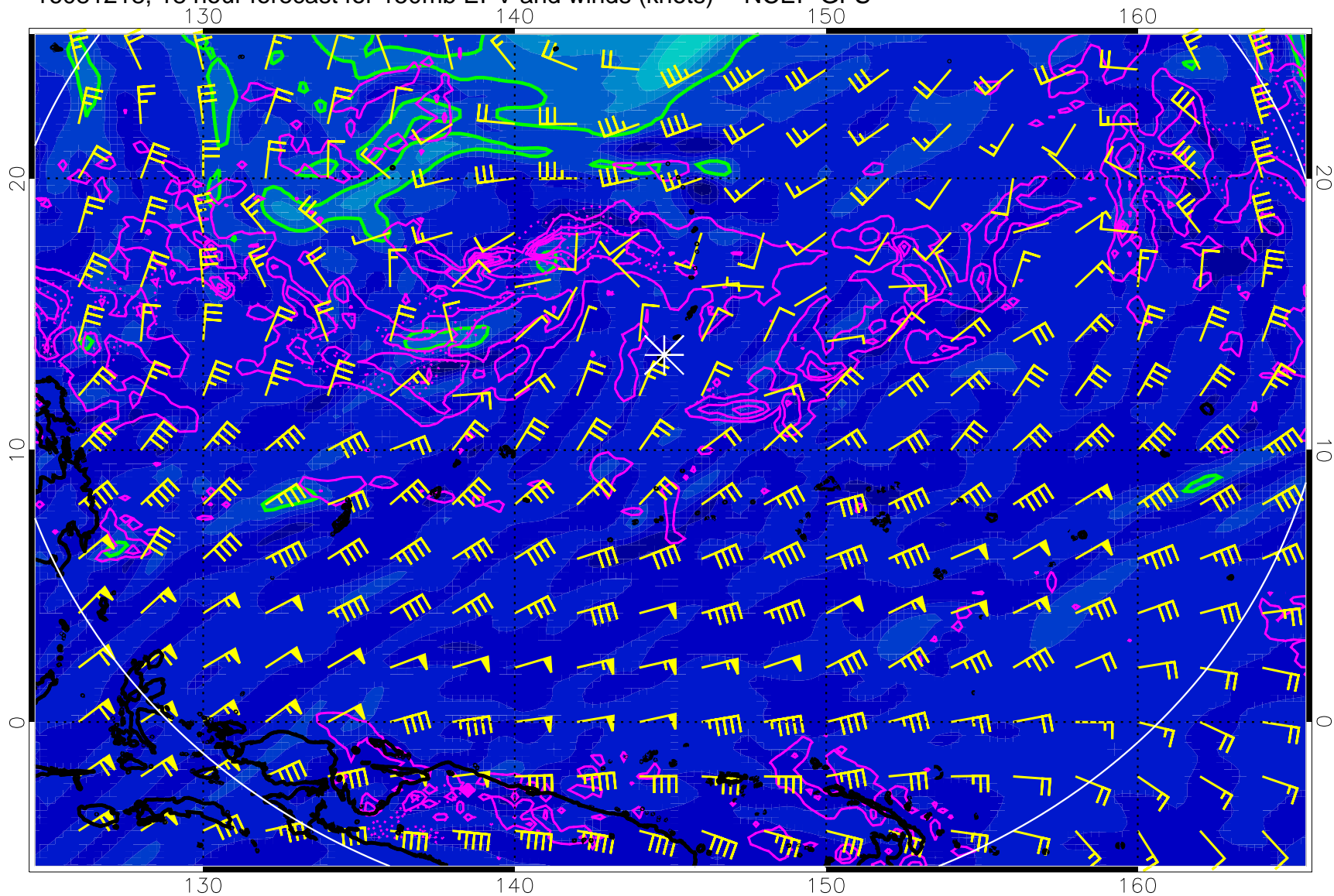
16081218, 18 hour forecast for 150mb EPV and winds (knots) -- NCEP GFS
