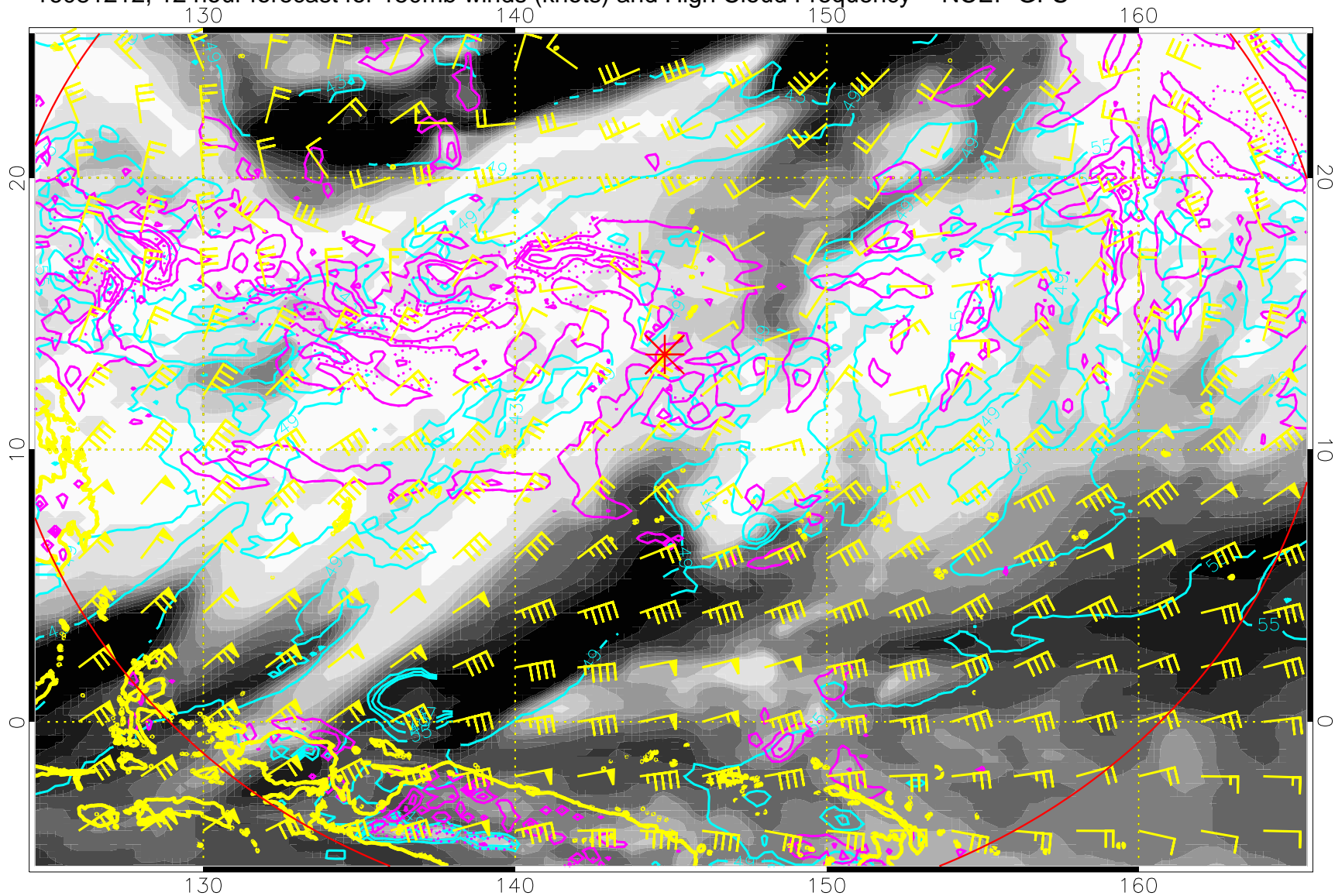
16081212, 12 hour forecast for 150mb winds (knots) and High Cloud Frequency -- NCEP GFS
