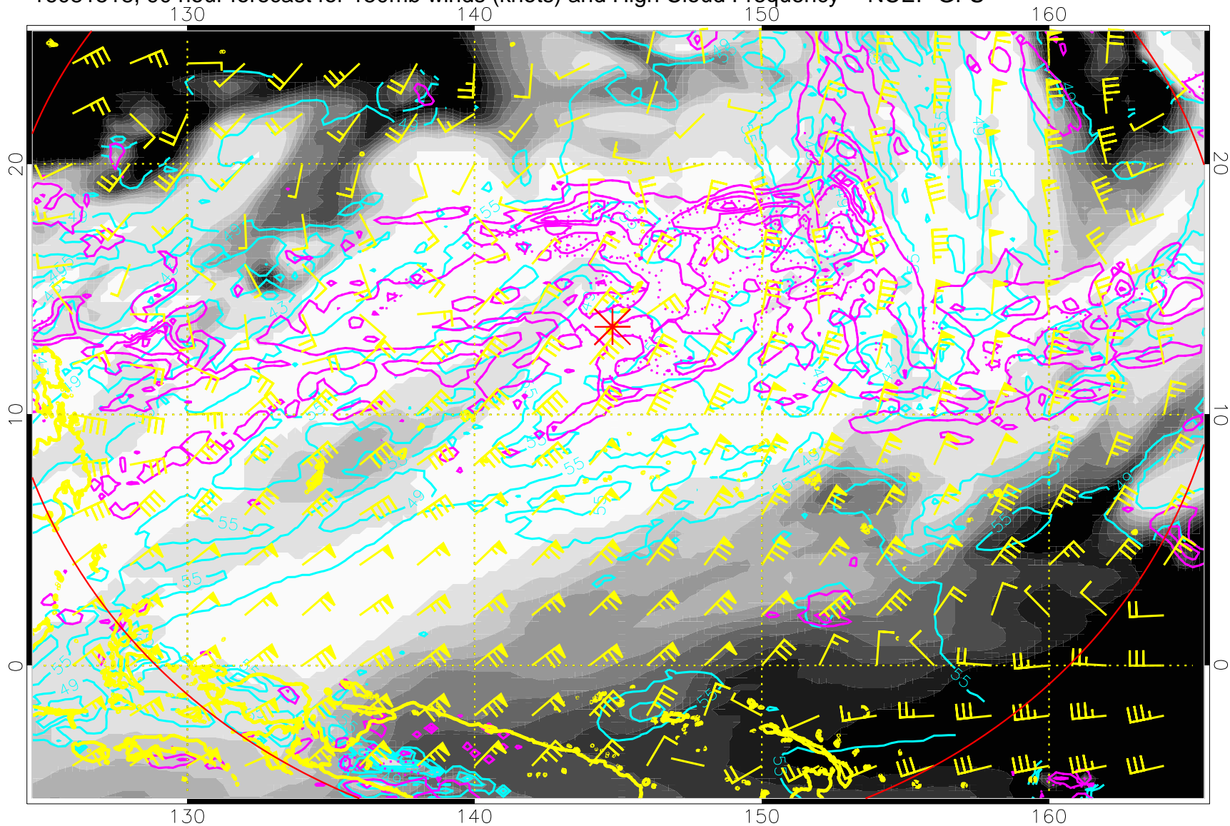
16081518, 90 hour forecast for 150mb winds (knots) and High Cloud Frequency -- NCEP GFS
