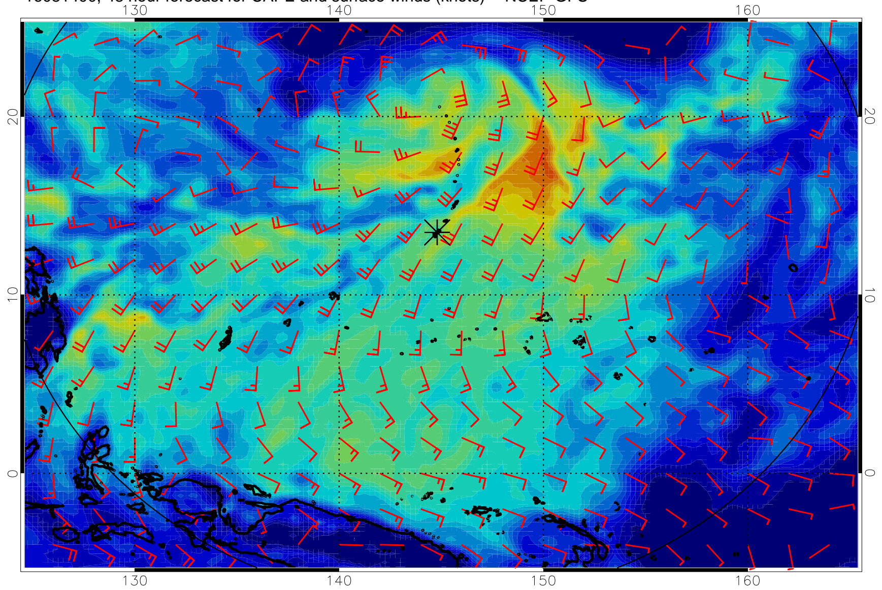
16081400, 48 hour forecast for CAPE and surface winds (knots) -- NCEP GFS
