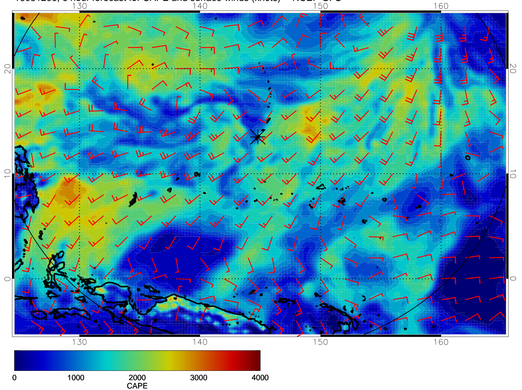
16081206, 6 hour forecast for CAPE and surface winds (knots) -- NCEP GFS
