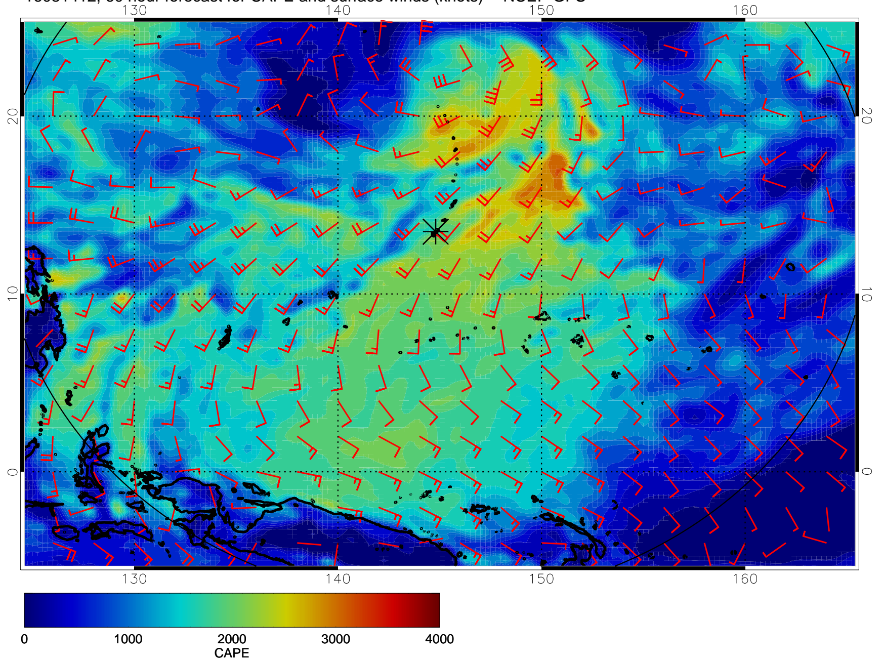
16081412, 60 hour forecast for CAPE and surface winds (knots) -- NCEP GFS
