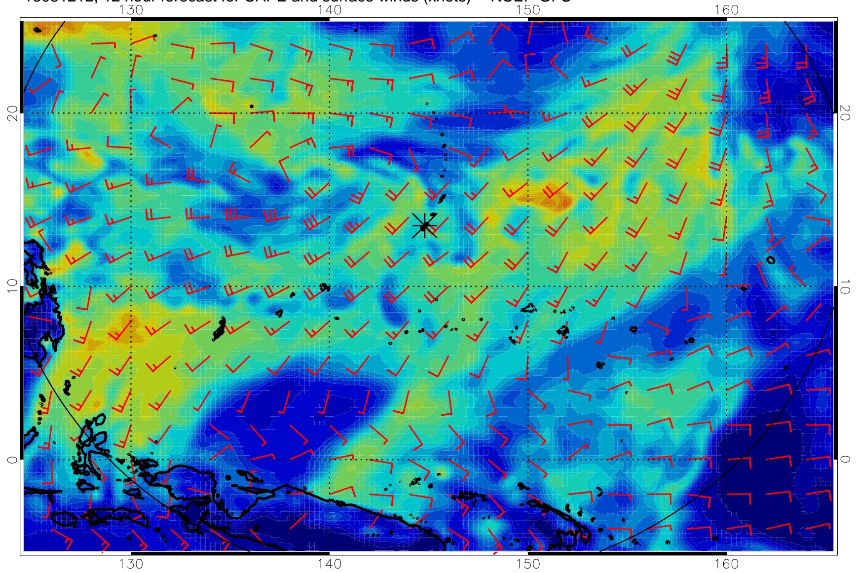
16081212, 12 hour forecast for CAPE and surface winds (knots) -- NCEP GFS
