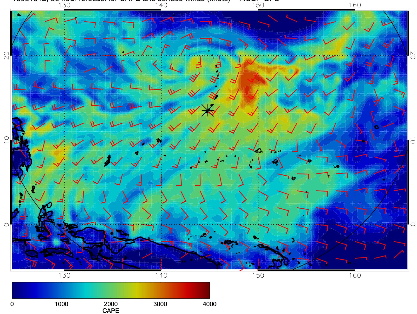
16081312, 36 hour forecast for CAPE and surface winds (knots) -- NCEP GFS
