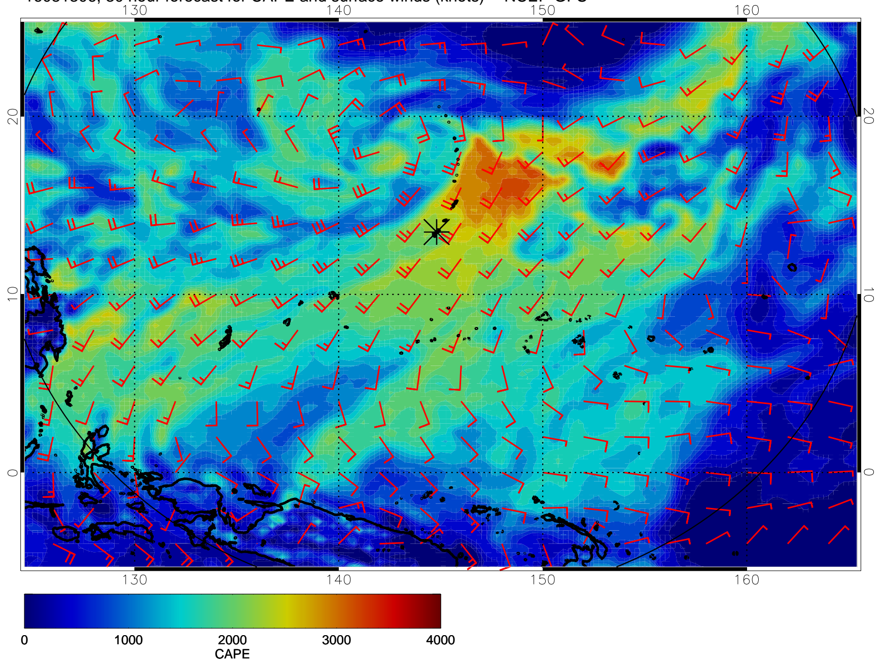
16081306, 30 hour forecast for CAPE and surface winds (knots) -- NCEP GFS
