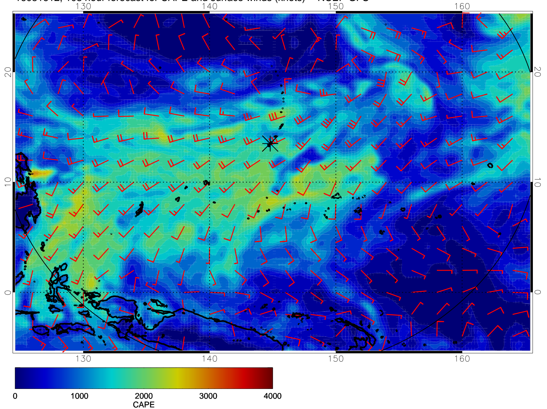
16081612, 108 hour forecast for CAPE and surface winds (knots) -- NCEP GFS
