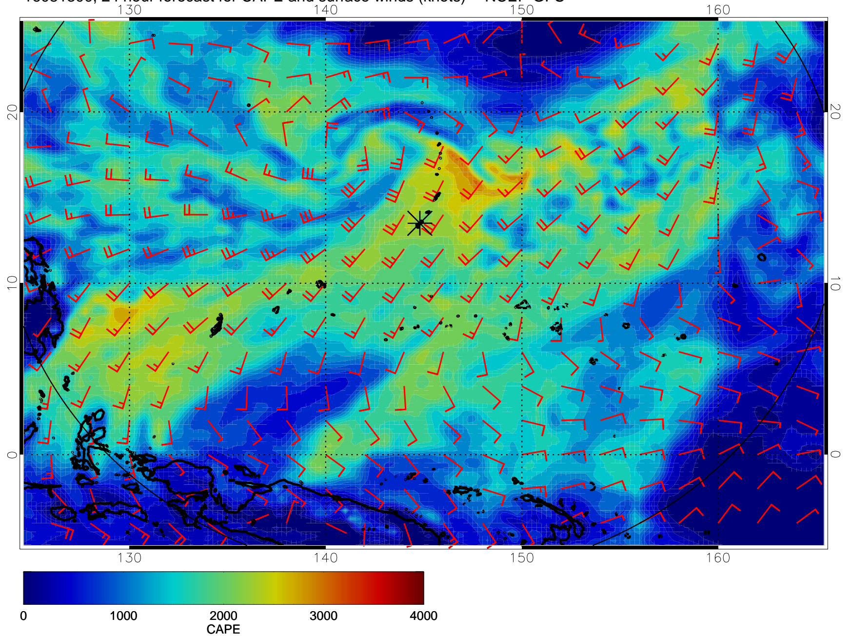
16081300, 24 hour forecast for CAPE and surface winds (knots) -- NCEP GFS
