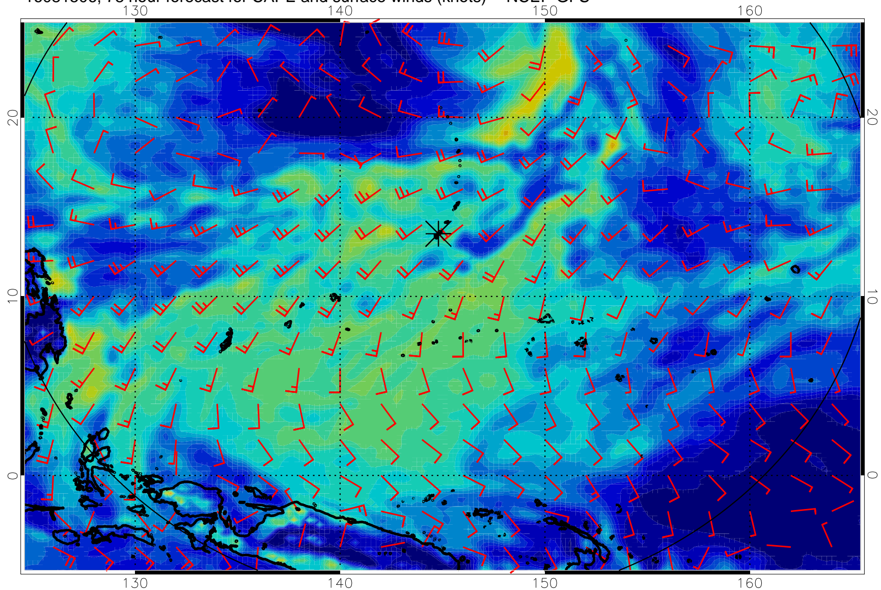
16081506, 78 hour forecast for CAPE and surface winds (knots) -- NCEP GFS
