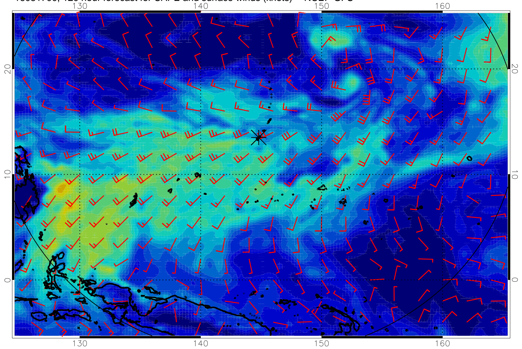
16081700, 120 hour forecast for CAPE and surface winds (knots) -- NCEP GFS
