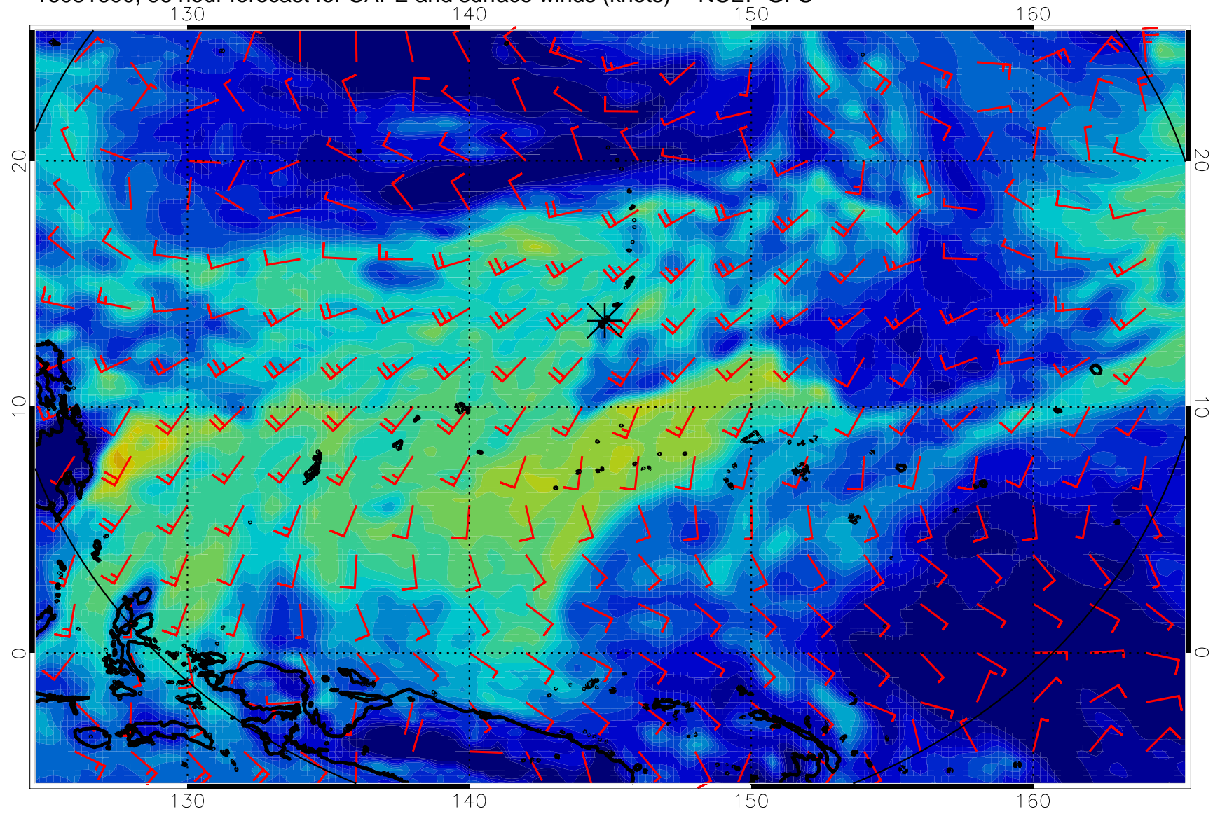
16081600, 96 hour forecast for CAPE and surface winds (knots) -- NCEP GFS
