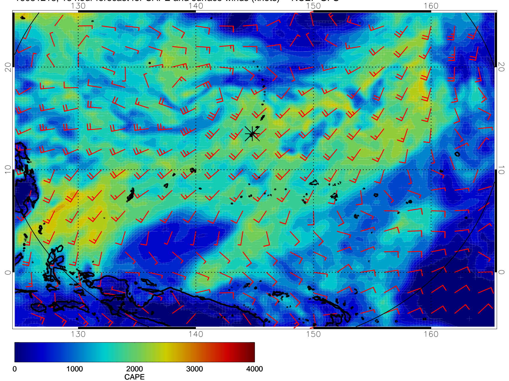
16081218, 18 hour forecast for CAPE and surface winds (knots) -- NCEP GFS
