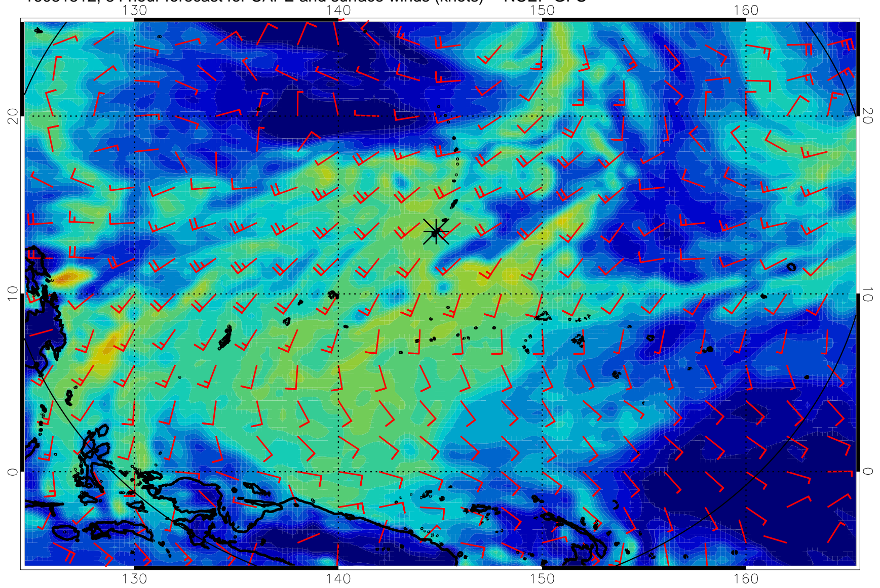
16081512, 84 hour forecast for CAPE and surface winds (knots) -- NCEP GFS
