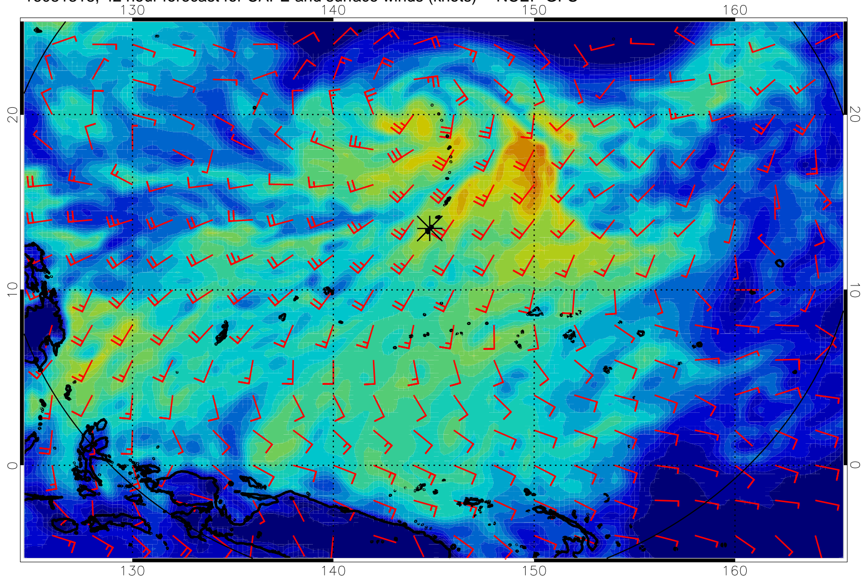
16081318, 42 hour forecast for CAPE and surface winds (knots) -- NCEP GFS
