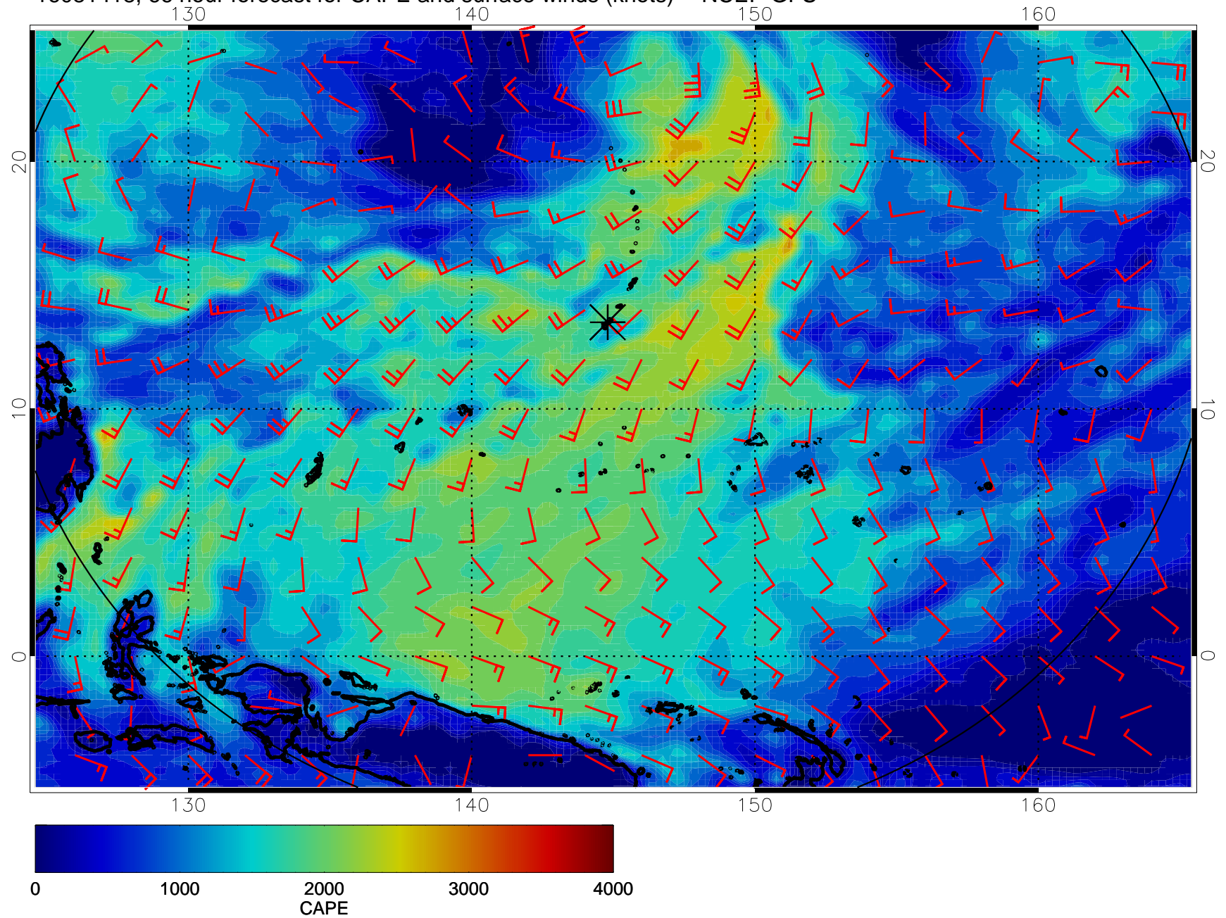
16081418, 66 hour forecast for CAPE and surface winds (knots) -- NCEP GFS
