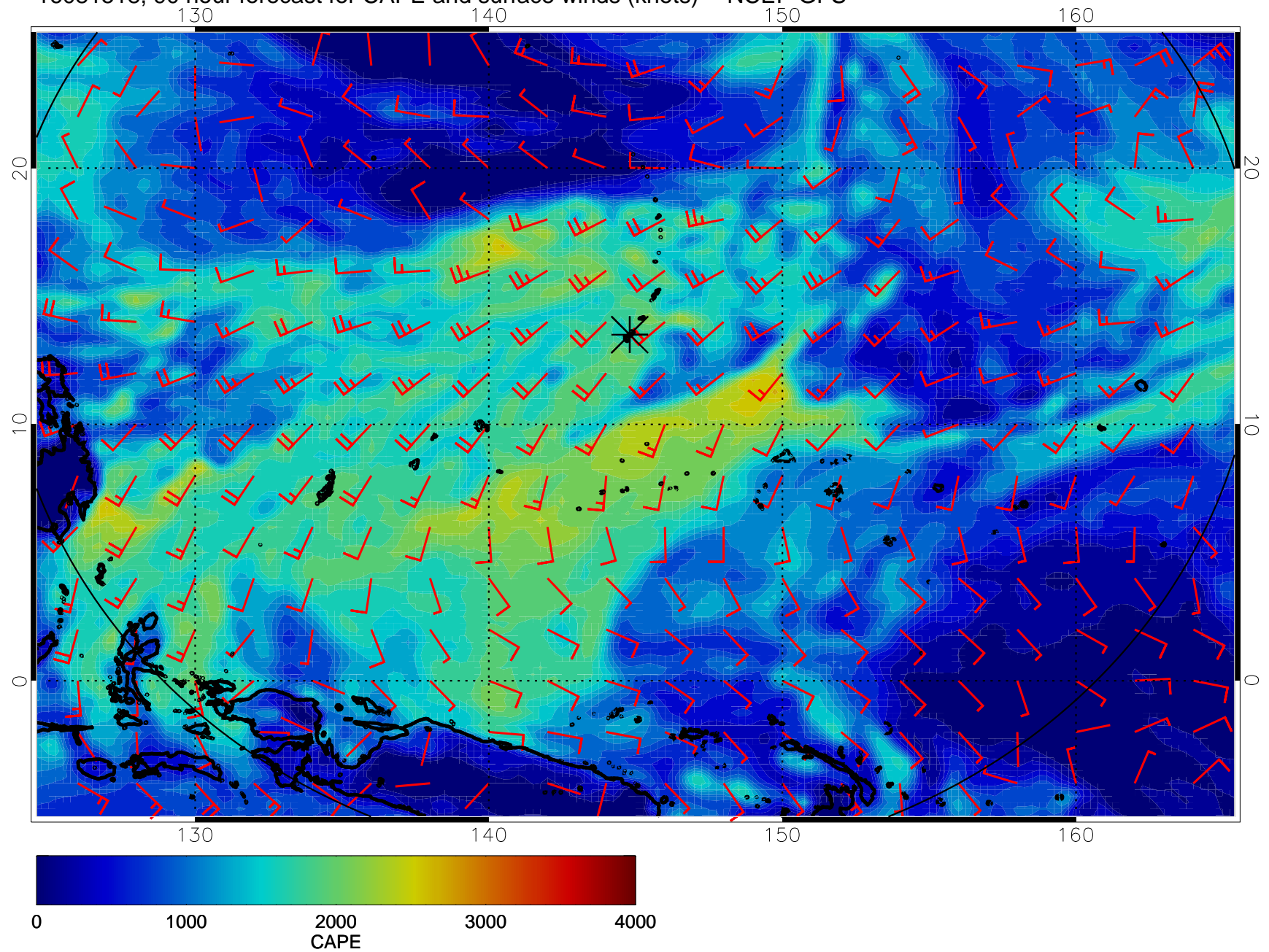
16081518, 90 hour forecast for CAPE and surface winds (knots) -- NCEP GFS
