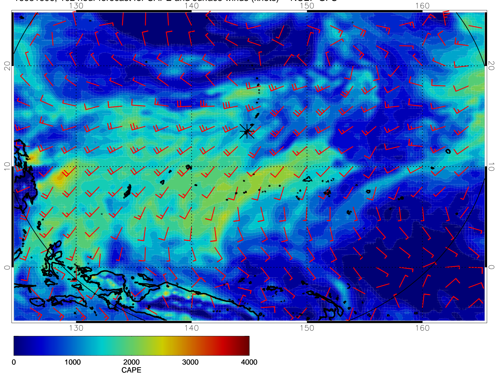
16081606, 102 hour forecast for CAPE and surface winds (knots) -- NCEP GFS
