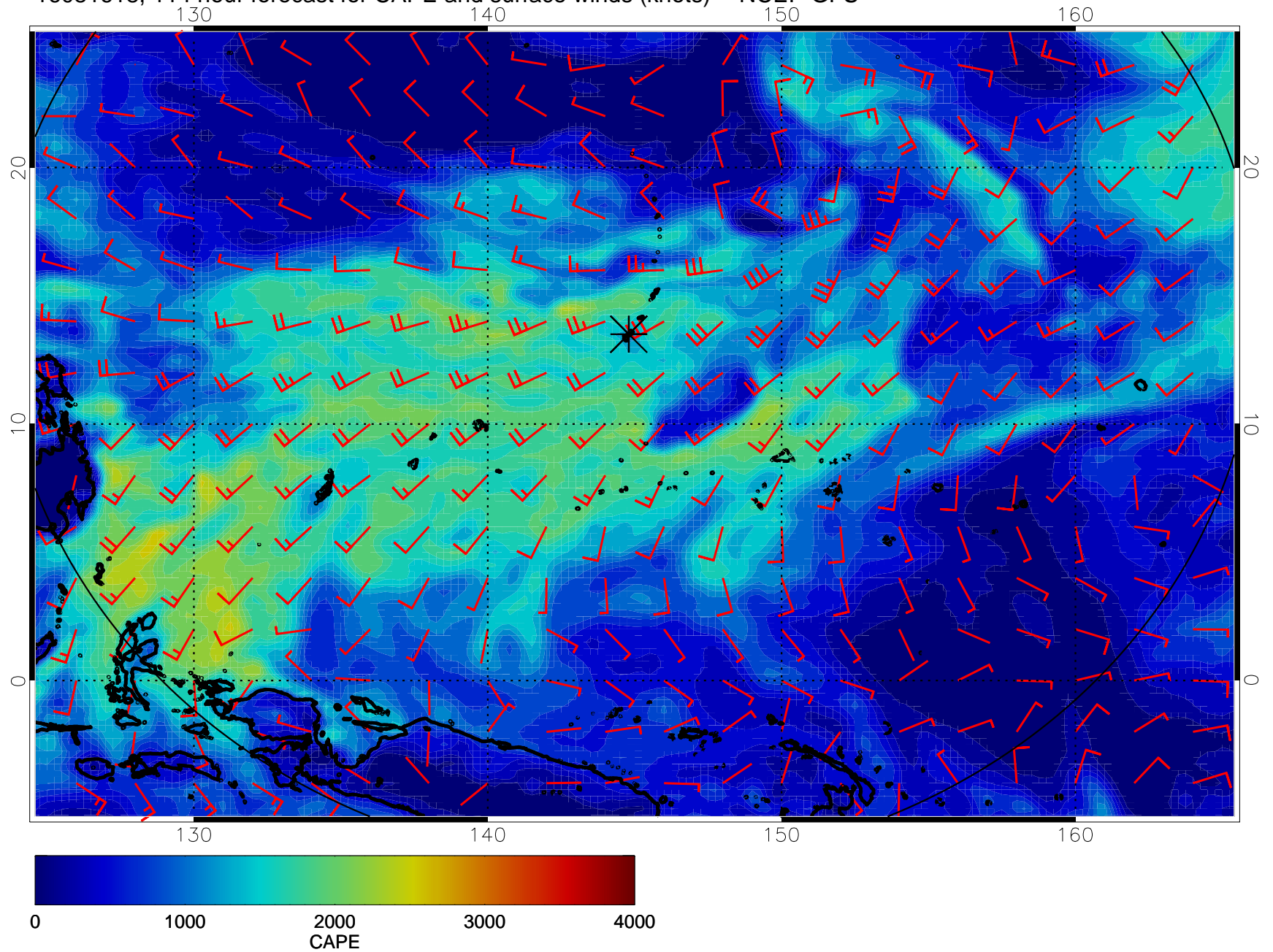
16081618, 114 hour forecast for CAPE and surface winds (knots) -- NCEP GFS
