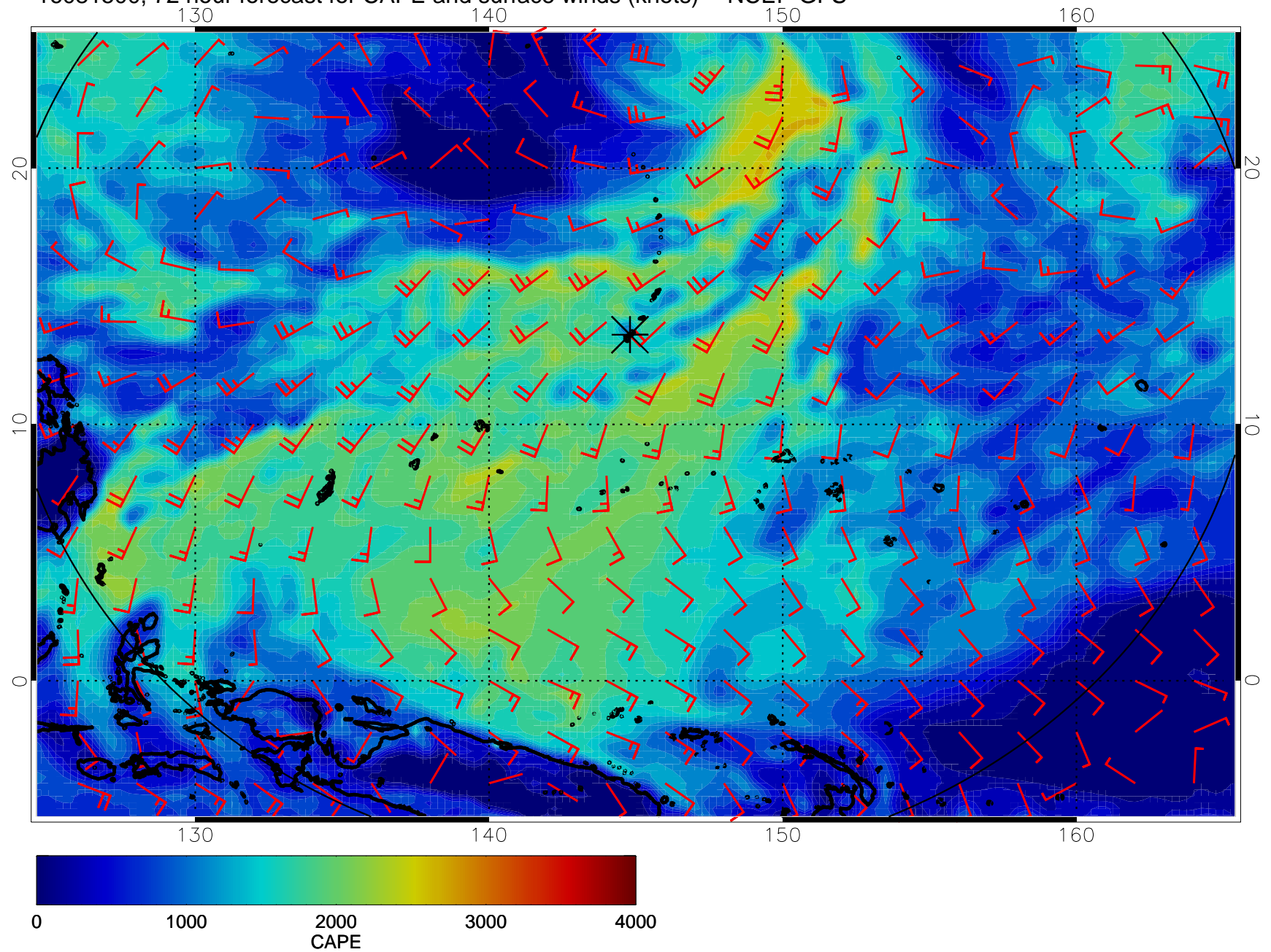
16081500, 72 hour forecast for CAPE and surface winds (knots) -- NCEP GFS
