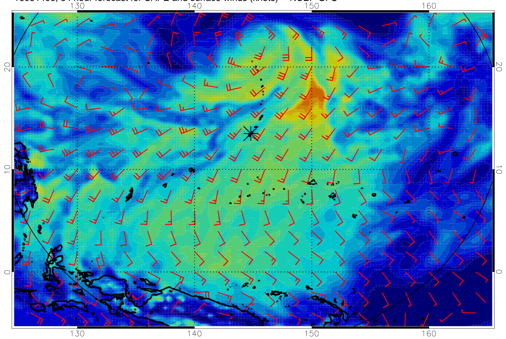
16081406, 54 hour forecast for CAPE and surface winds (knots) -- NCEP GFS
