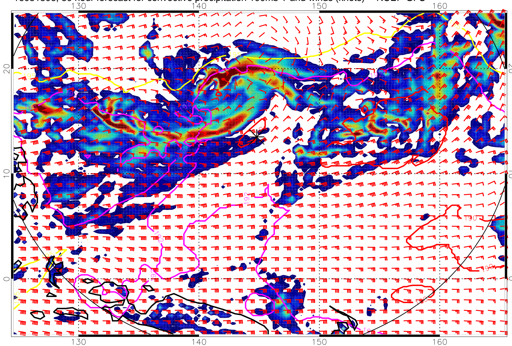
16081306, 30 hour forecast for convective precipitation 100mb T and winds (knots) -- NCEP GFS
