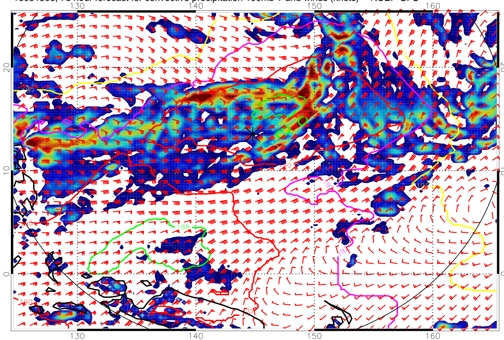
16081506, 78 hour forecast for convective precipitation 100mb T and winds (knots) -- NCEP GFS
