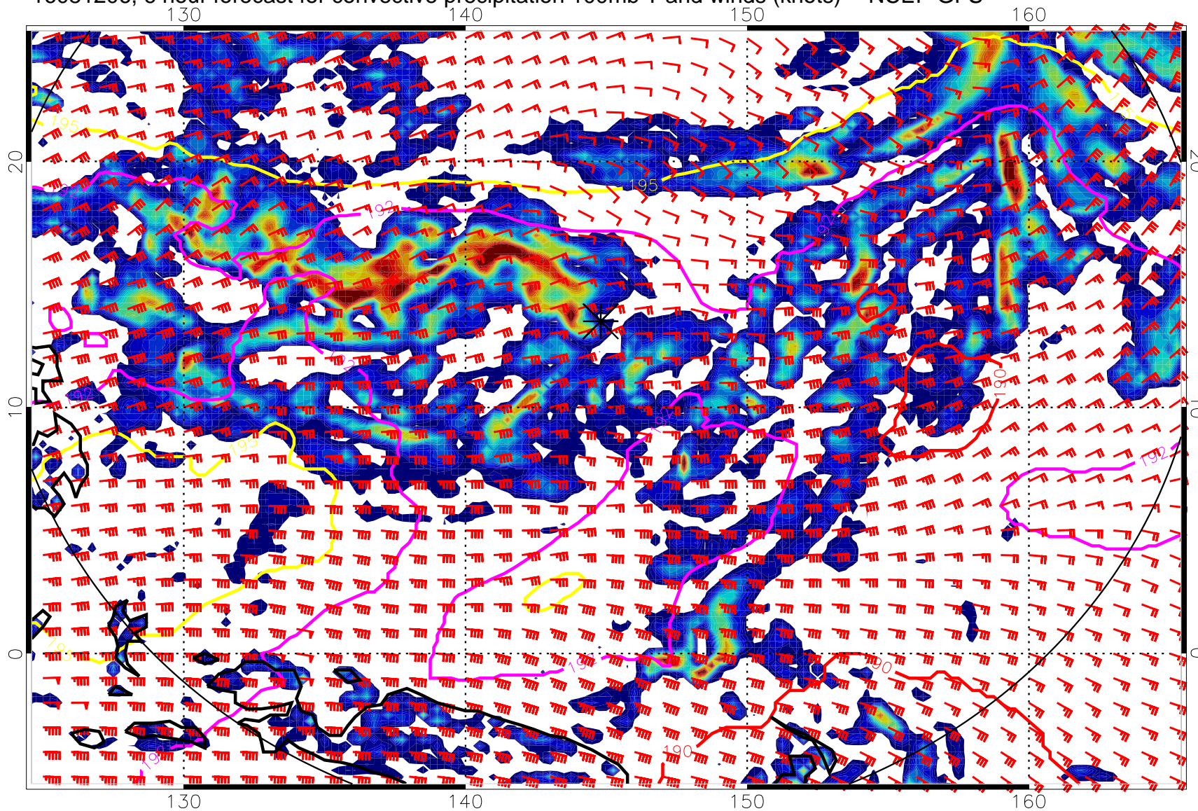
16081206, 6 hour forecast for convective precipitation 100mb T and winds (knots) -- NCEP GFS
