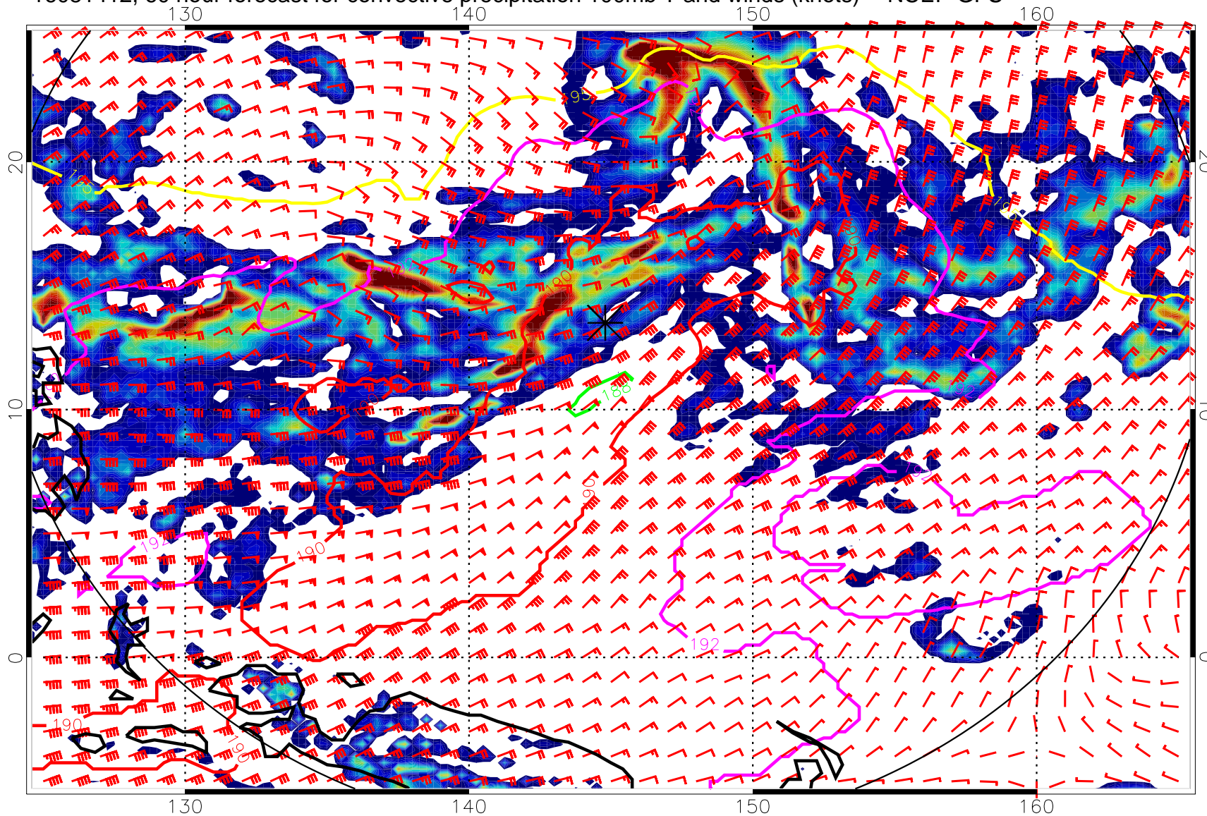
16081412, 60 hour forecast for convective precipitation 100mb T and winds (knots) -- NCEP GFS
