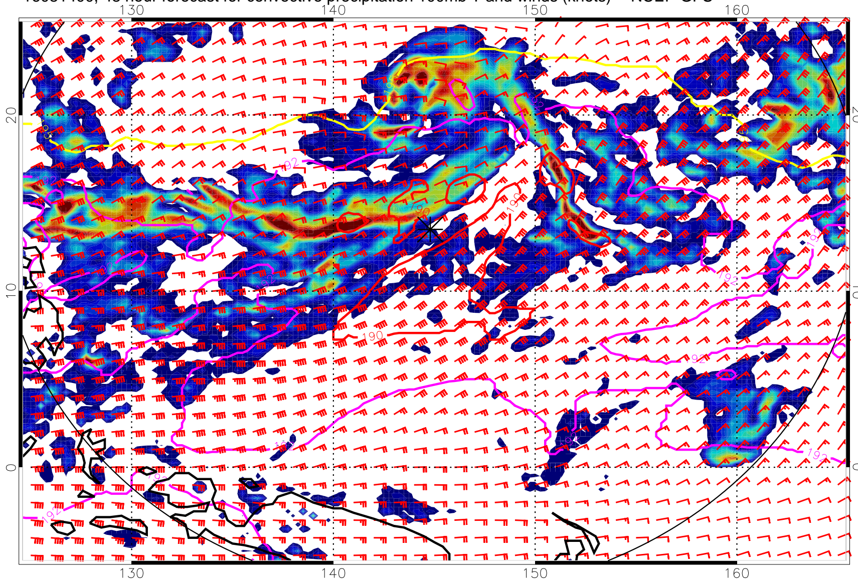
16081400, 48 hour forecast for convective precipitation 100mb T and winds (knots) -- NCEP GFS
