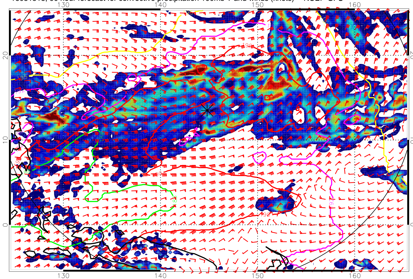
16081518, 90 hour forecast for convective precipitation 100mb T and winds (knots) -- NCEP GFS
