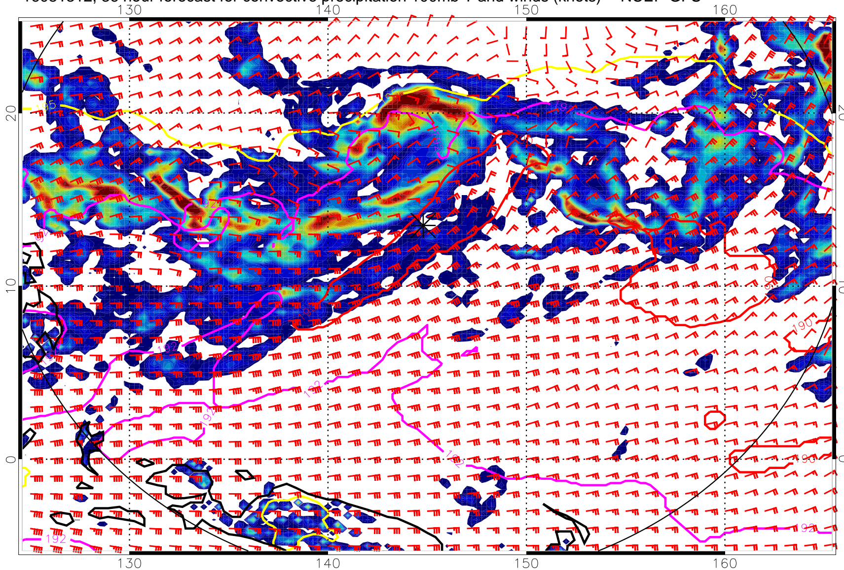
16081312, 36 hour forecast for convective precipitation 100mb T and winds (knots) -- NCEP GFS
