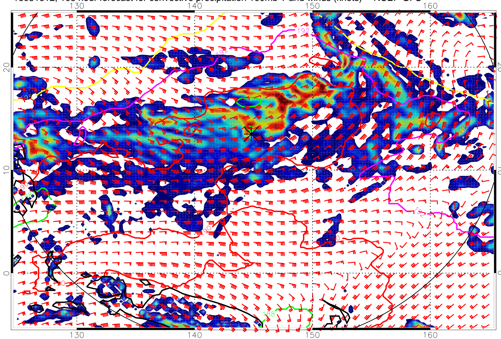
16081612, 108 hour forecast for convective precipitation 100mb T and winds (knots) -- NCEP GFS
