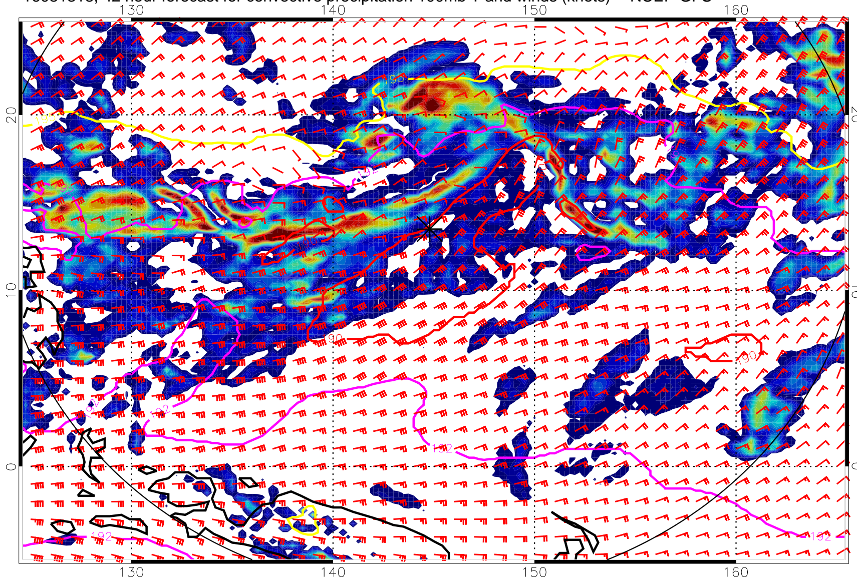
16081318, 42 hour forecast for convective precipitation 100mb T and winds (knots) -- NCEP GFS
