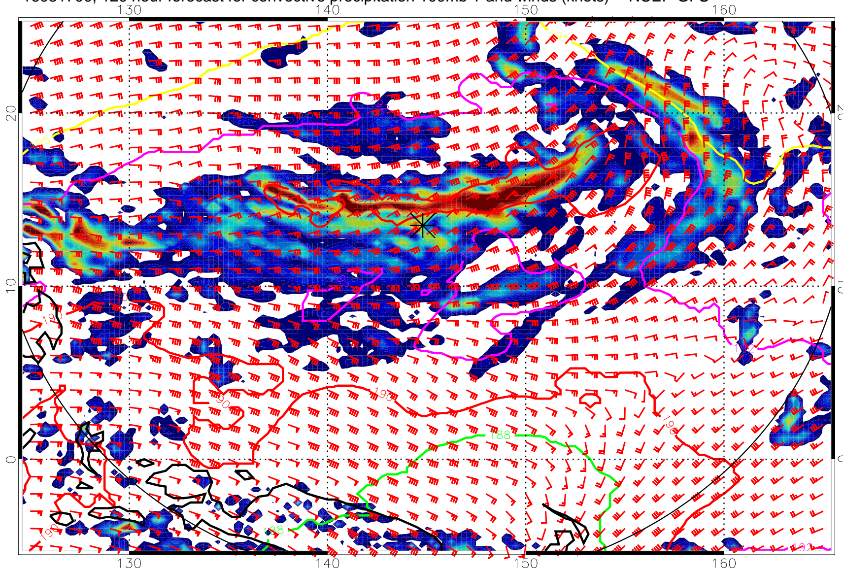
16081700, 120 hour forecast for convective precipitation 100mb T and winds (knots) -- NCEP GFS
