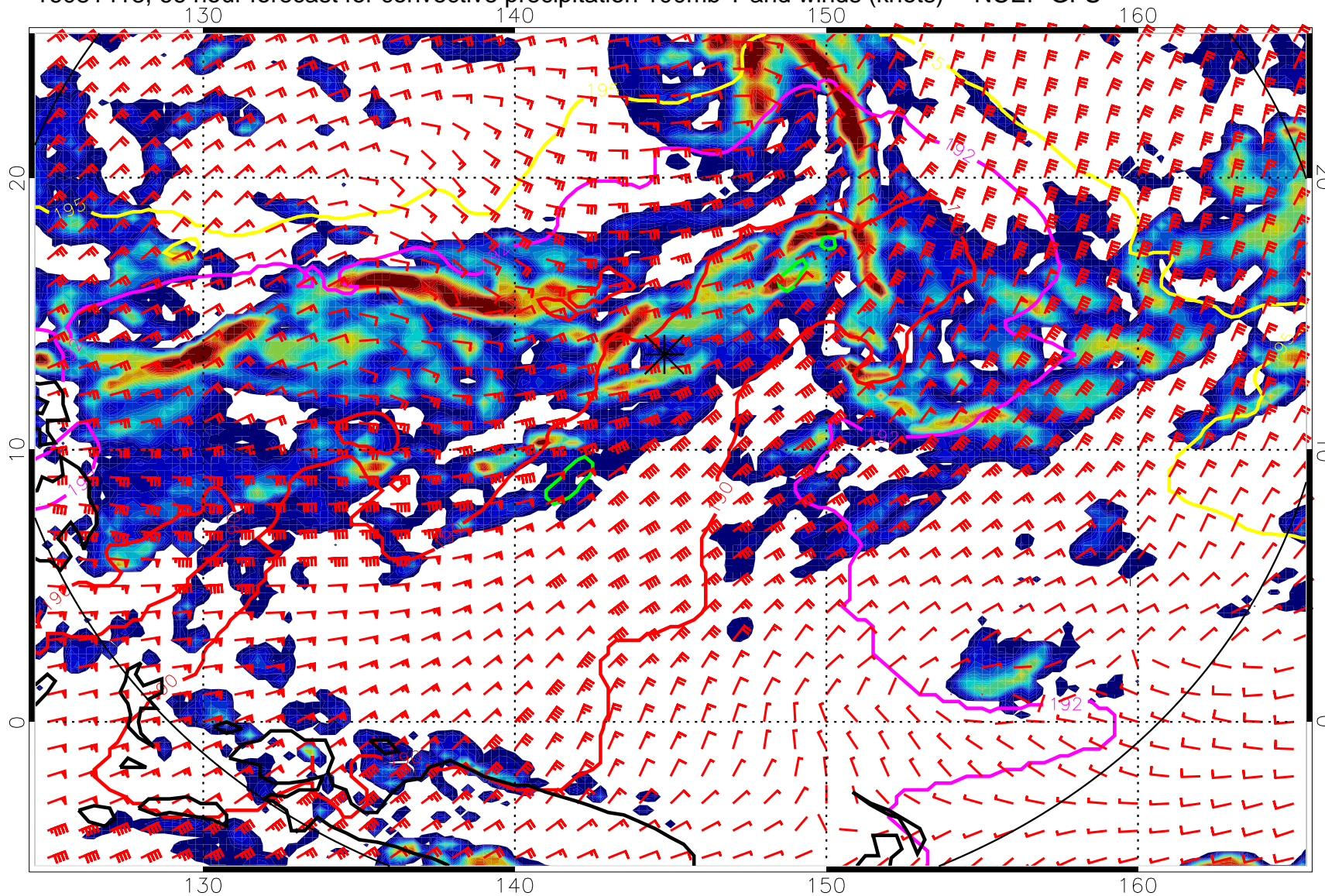
16081418, 66 hour forecast for convective precipitation 100mb T and winds (knots) -- NCEP GFS
