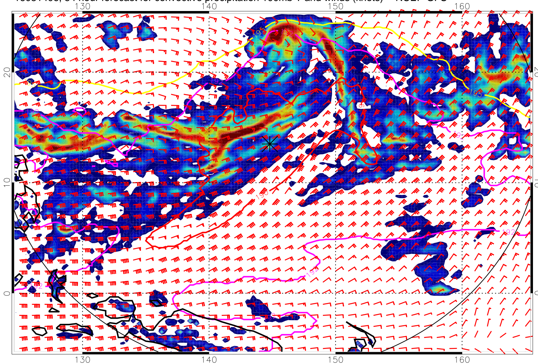
16081406, 54 hour forecast for convective precipitation 100mb T and winds (knots) -- NCEP GFS
