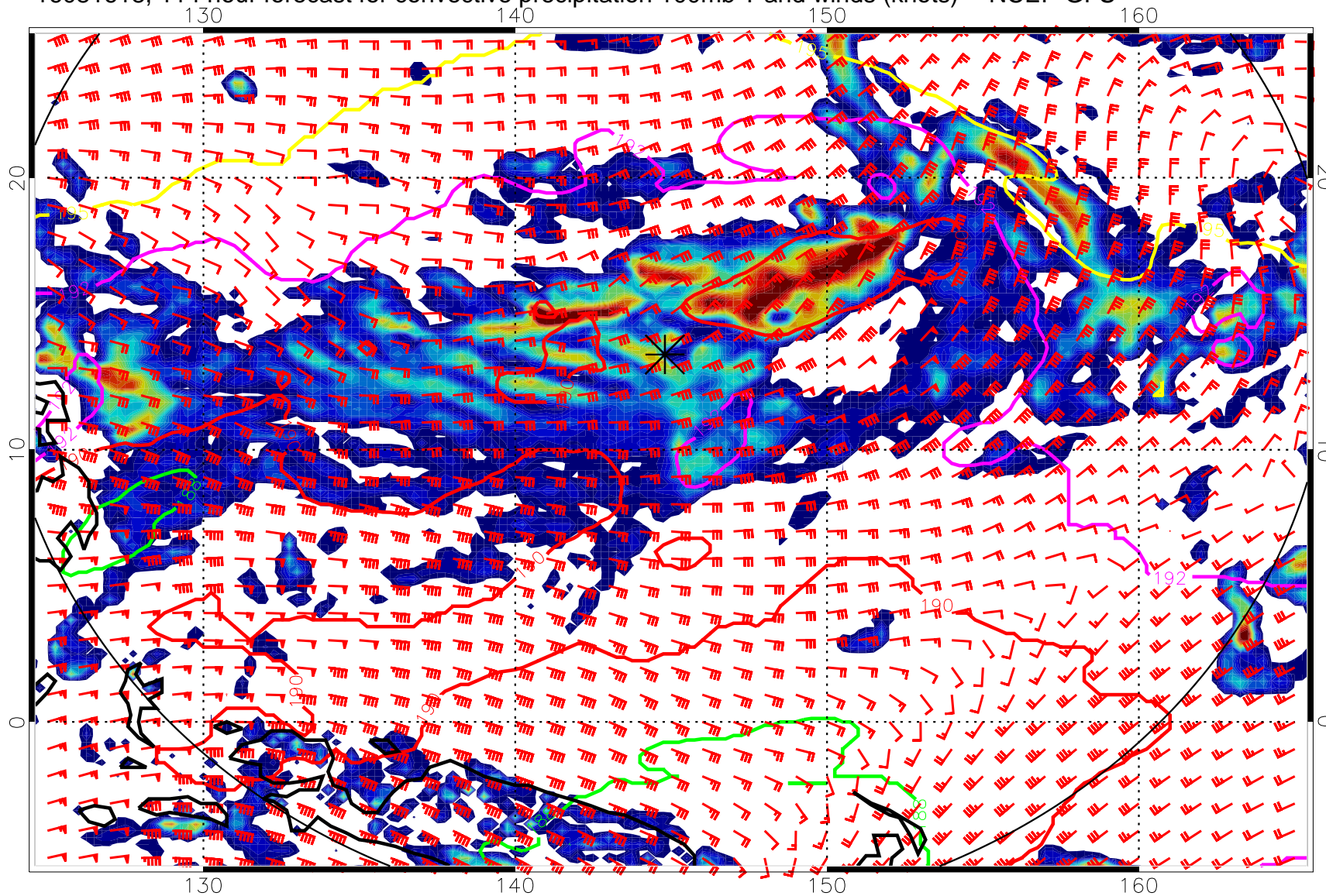
16081618, 114 hour forecast for convective precipitation 100mb T and winds (knots) -- NCEP GFS
