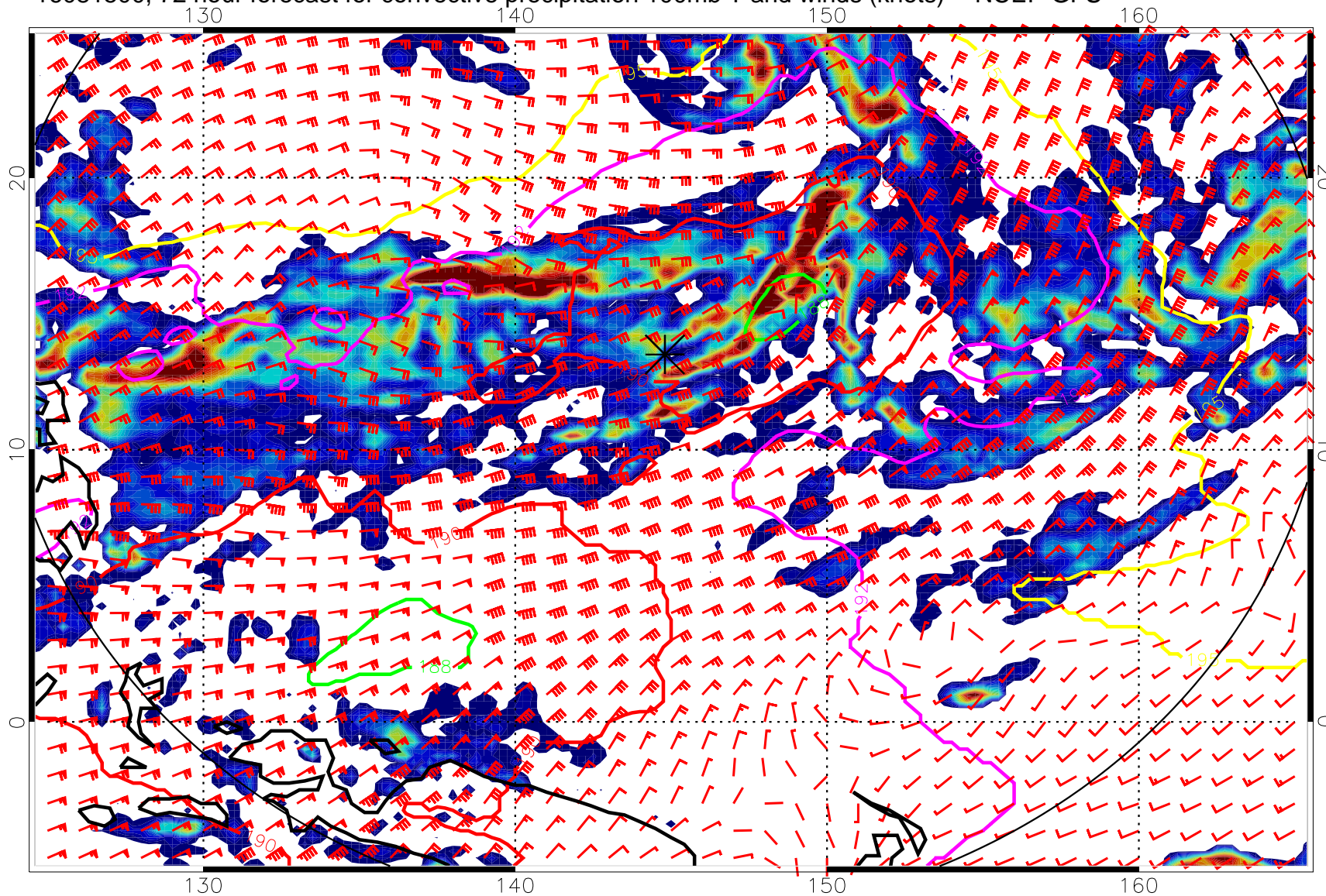
16081500, 72 hour forecast for convective precipitation 100mb T and winds (knots) -- NCEP GFS
