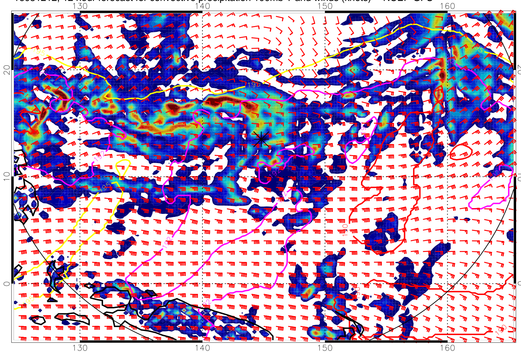
16081212, 12 hour forecast for convective precipitation 100mb T and winds (knots) -- NCEP GFS
