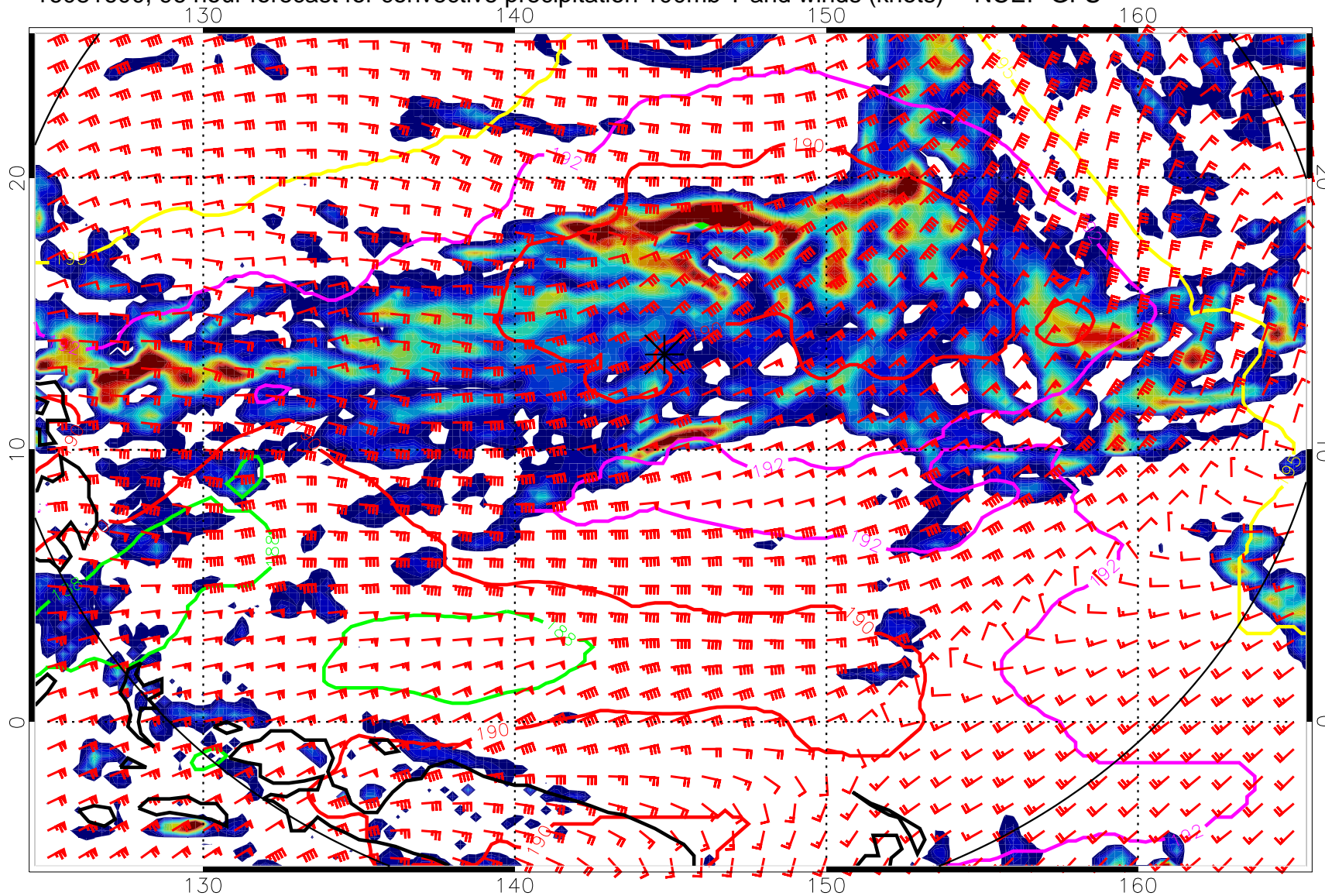
16081600, 96 hour forecast for convective precipitation 100mb T and winds (knots) -- NCEP GFS
