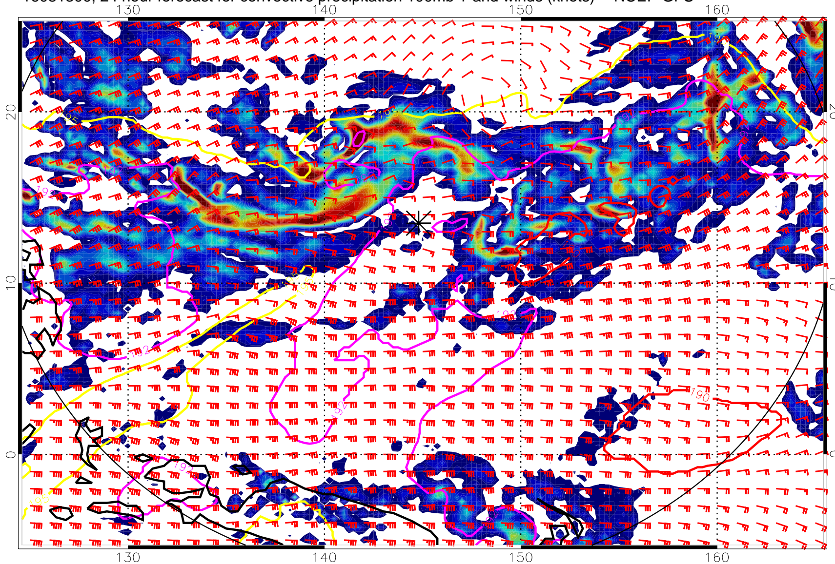
16081300, 24 hour forecast for convective precipitation 100mb T and winds (knots) -- NCEP GFS
