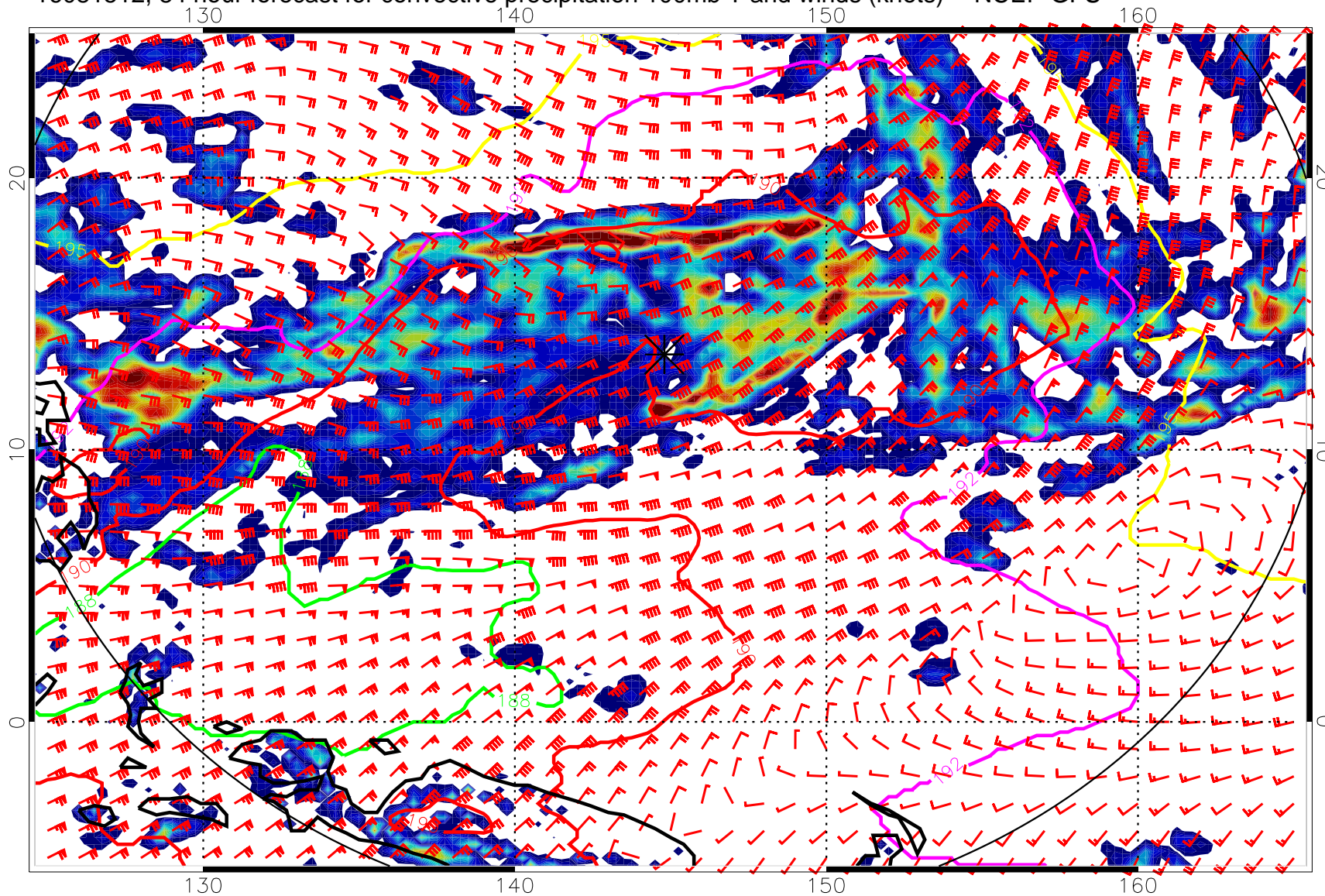
16081512, 84 hour forecast for convective precipitation 100mb T and winds (knots) -- NCEP GFS
