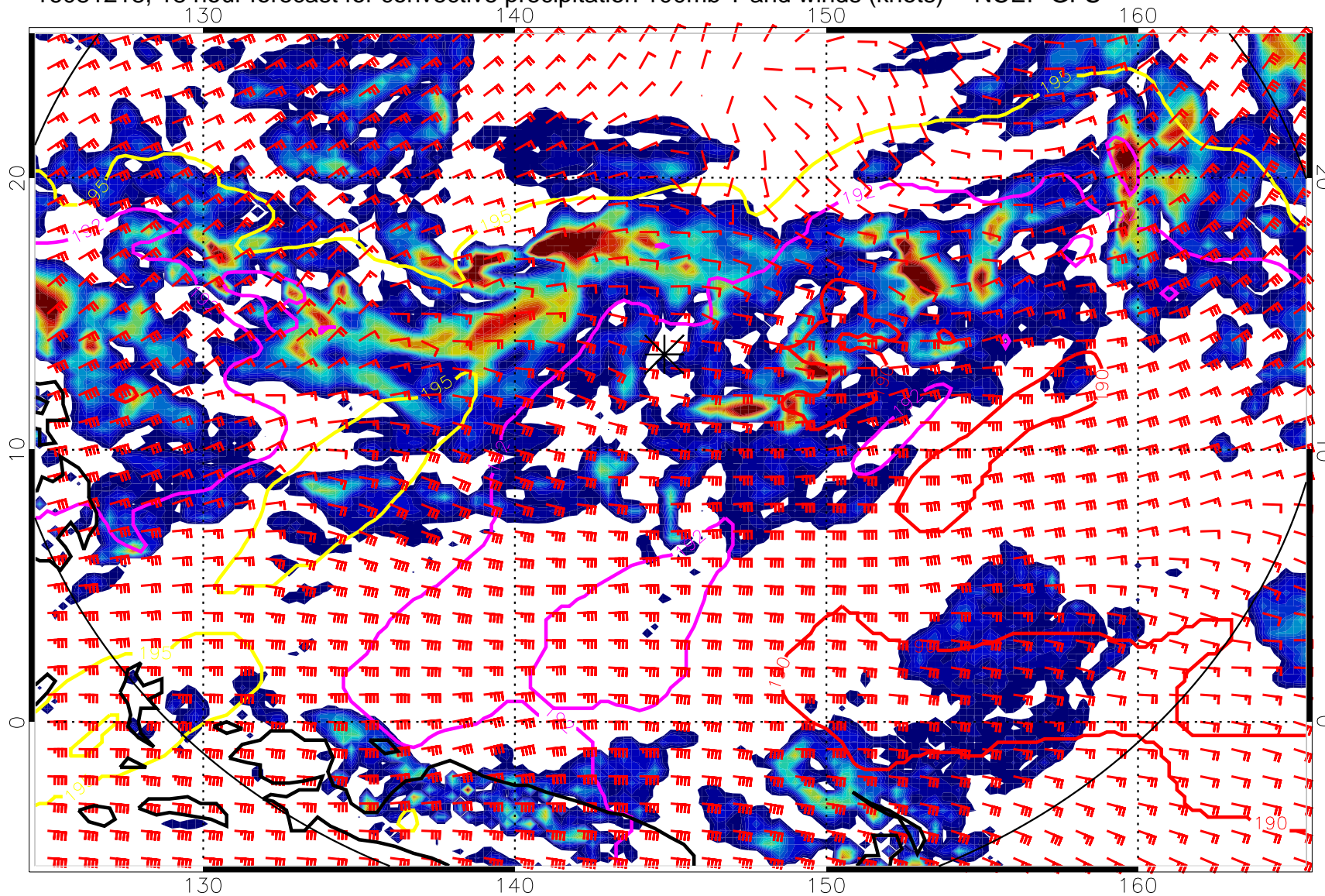
16081218, 18 hour forecast for convective precipitation 100mb T and winds (knots) -- NCEP GFS
