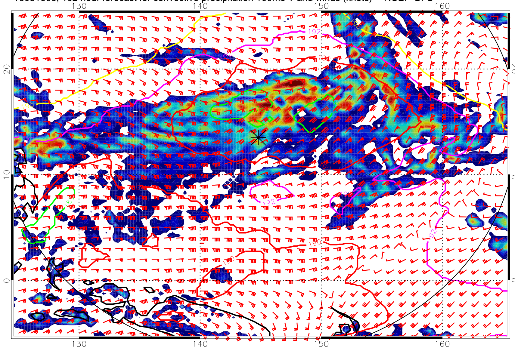
16081606, 102 hour forecast for convective precipitation 100mb T and winds (knots) -- NCEP GFS
