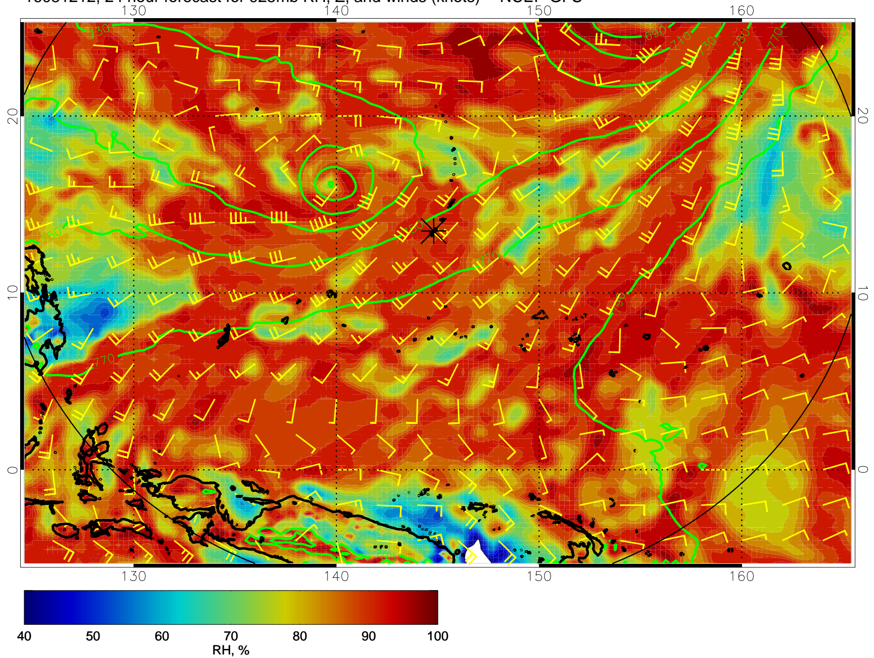
16081212, 24 hour forecast for 925mb RH, Z, and winds (knots) -- NCEP GFS
