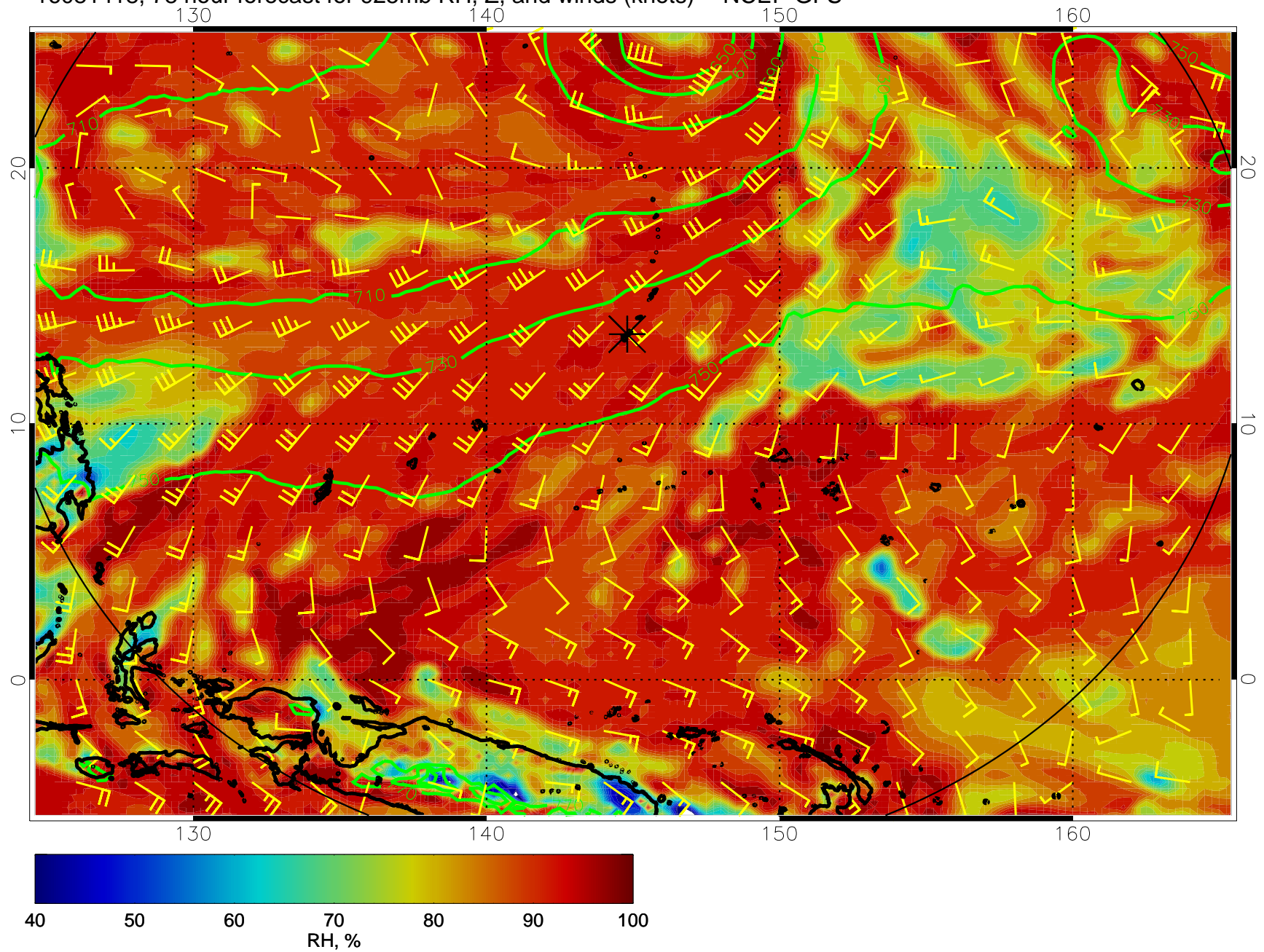
16081418, 78 hour forecast for 925mb RH, Z, and winds (knots) -- NCEP GFS
