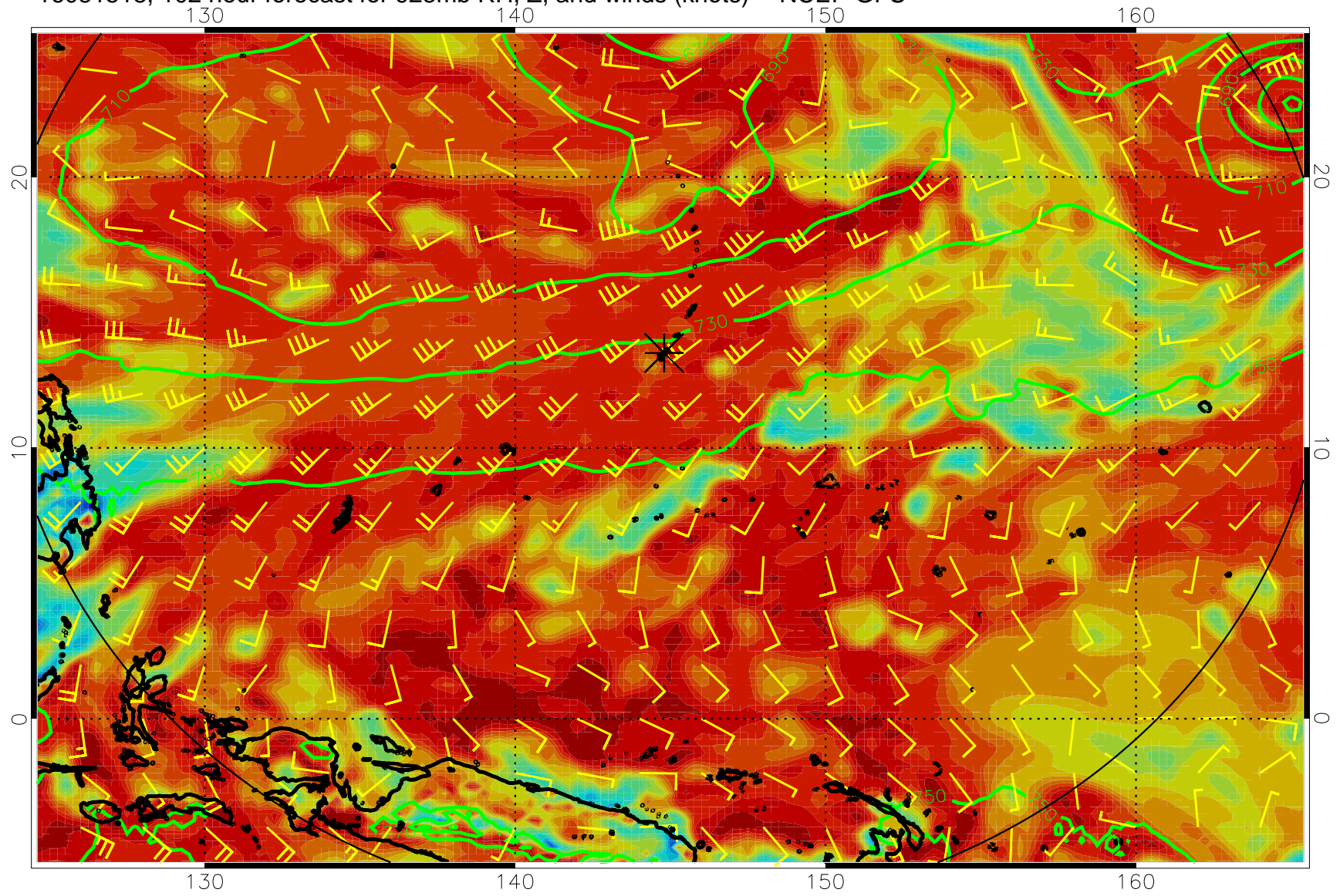
16081518, 102 hour forecast for 925mb RH, Z, and winds (knots) -- NCEP GFS
