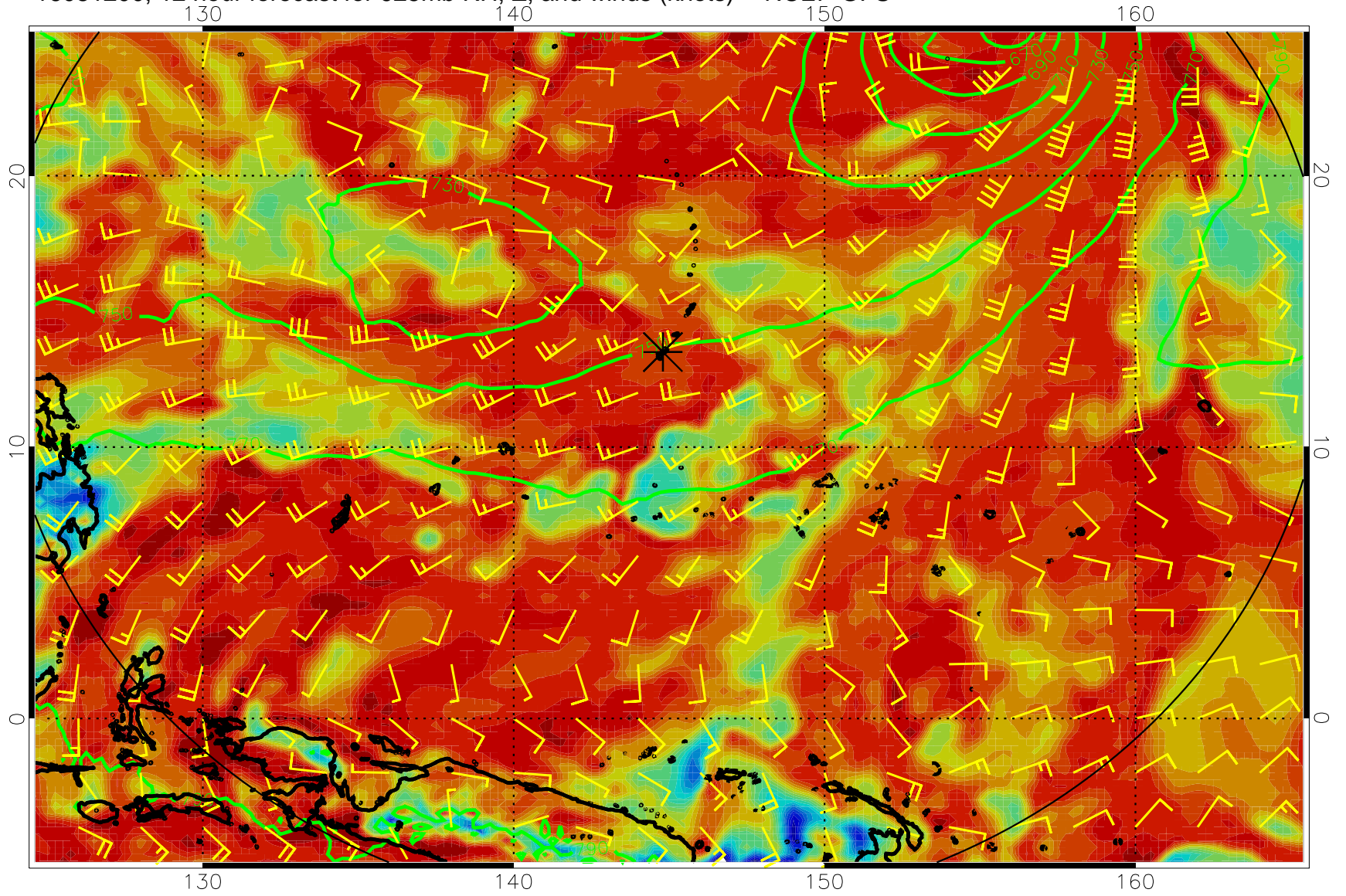
16081200, 12 hour forecast for 925mb RH, Z, and winds (knots) -- NCEP GFS
