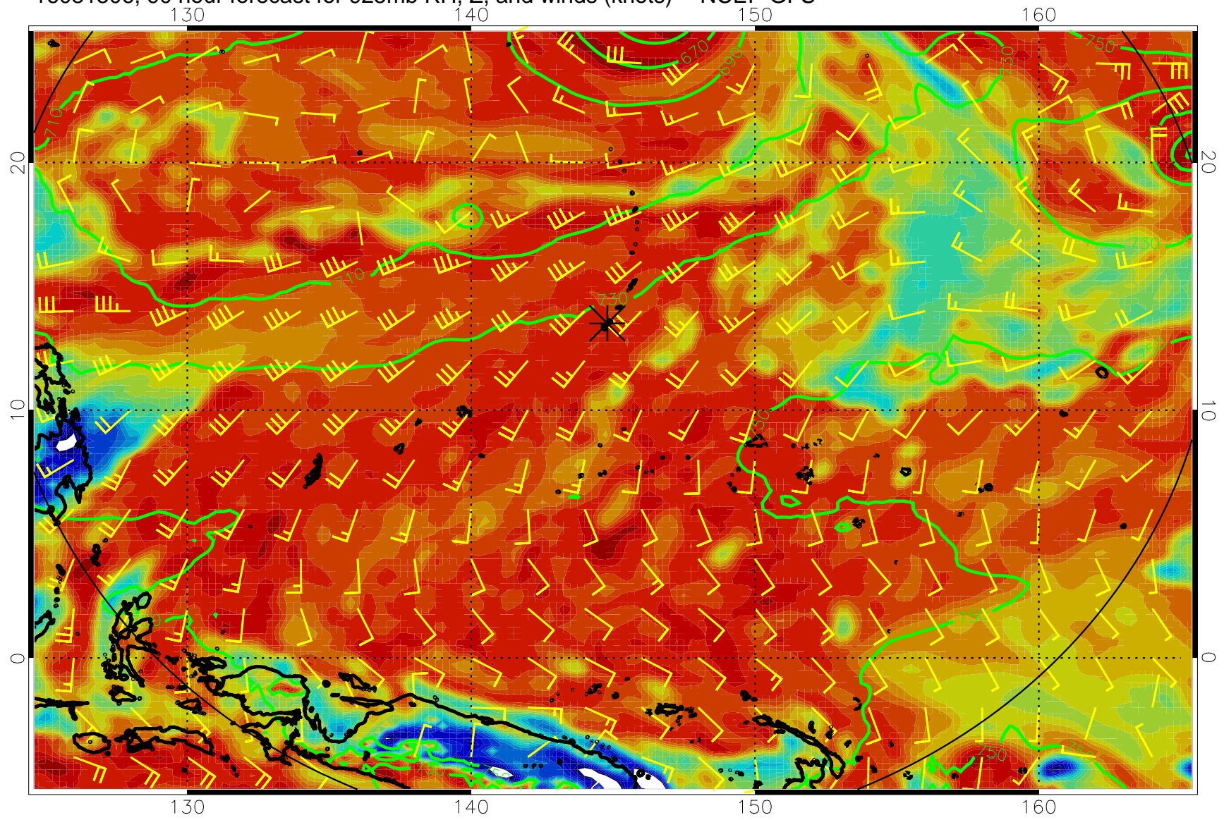
16081506, 90 hour forecast for 925mb RH, Z, and winds (knots) -- NCEP GFS
