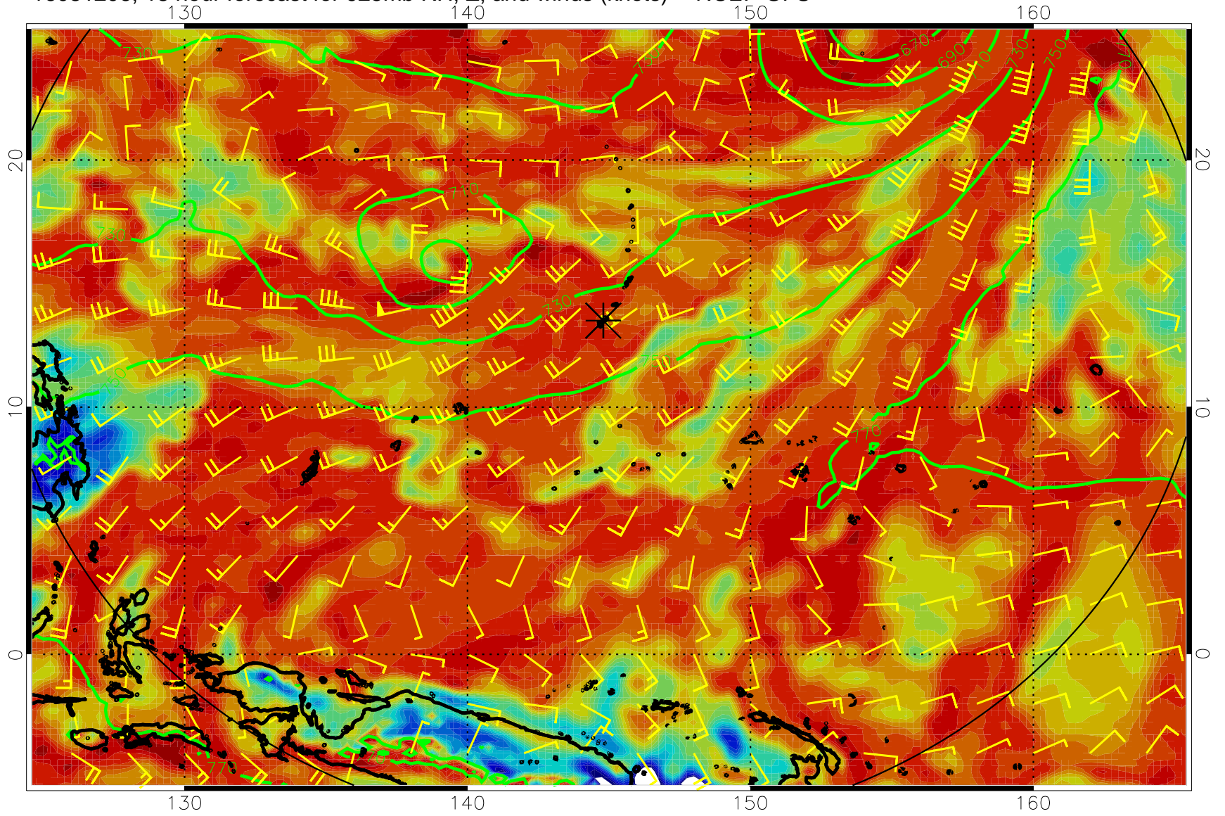
16081206, 18 hour forecast for 925mb RH, Z, and winds (knots) -- NCEP GFS
