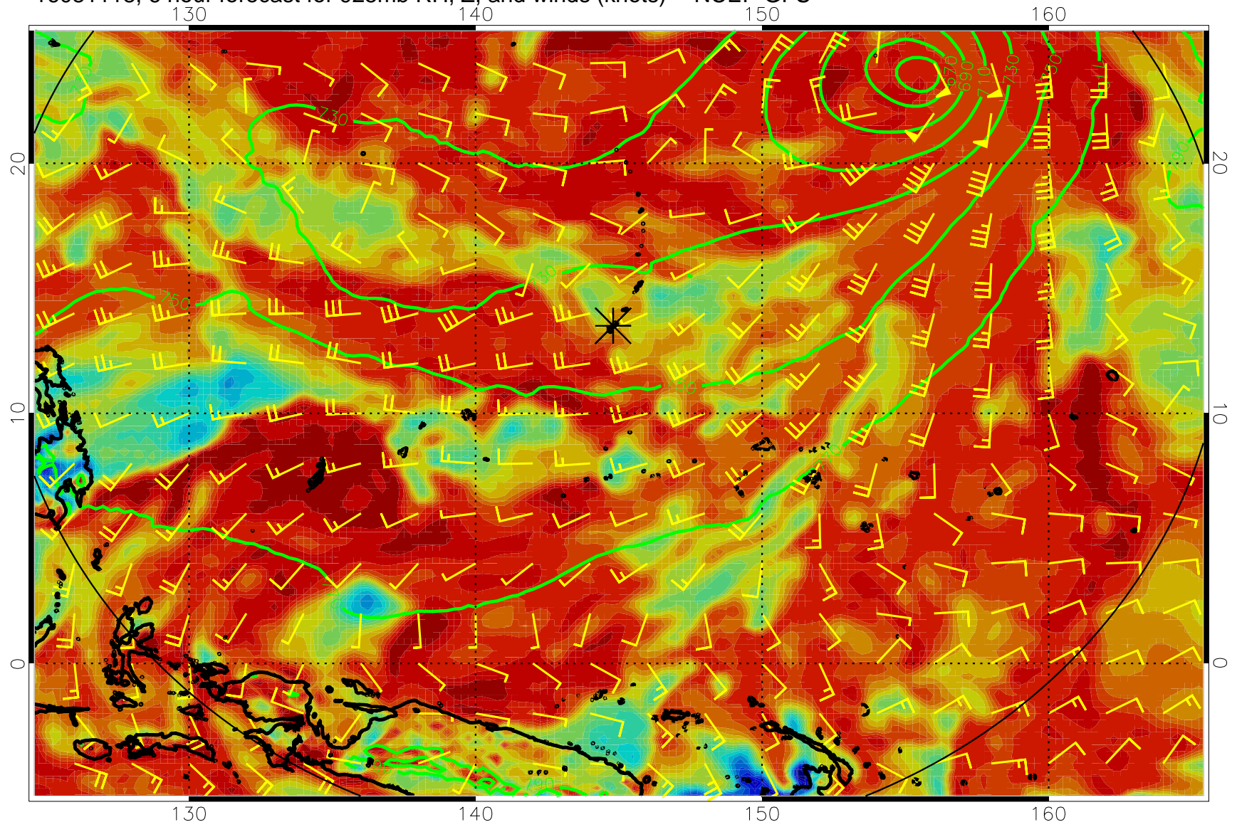
16081118, 6 hour forecast for 925mb RH, Z, and winds (knots) -- NCEP GFS
