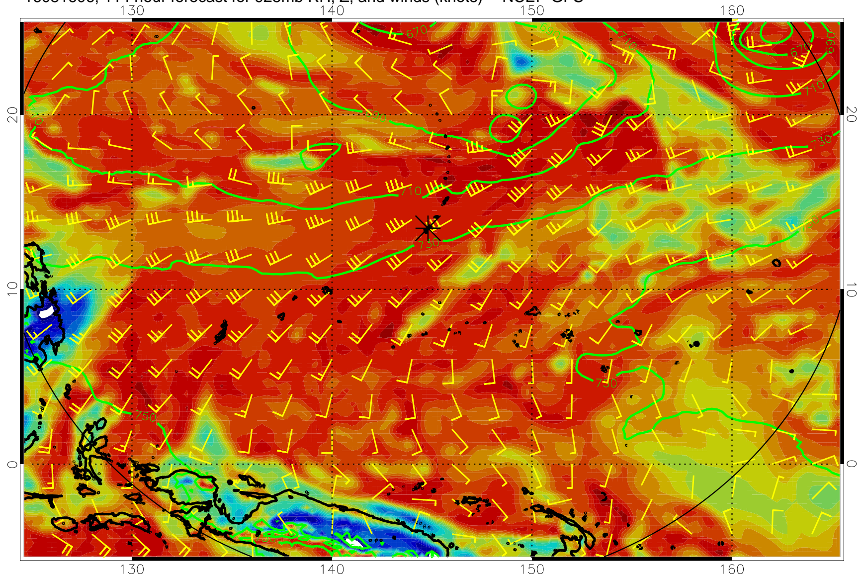
16081606, 114 hour forecast for 925mb RH, Z, and winds (knots) -- NCEP GFS
