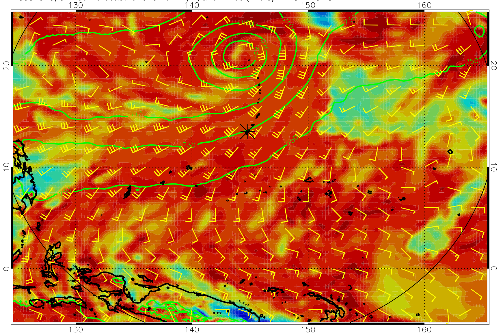
16081318, 54 hour forecast for 925mb RH, Z, and winds (knots) -- NCEP GFS
