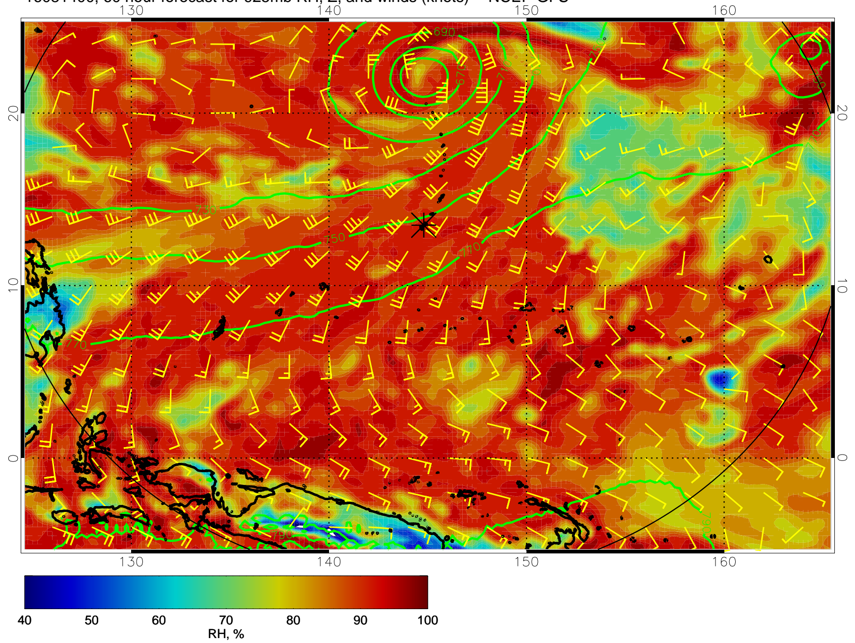
16081400, 60 hour forecast for 925mb RH, Z, and winds (knots) -- NCEP GFS
