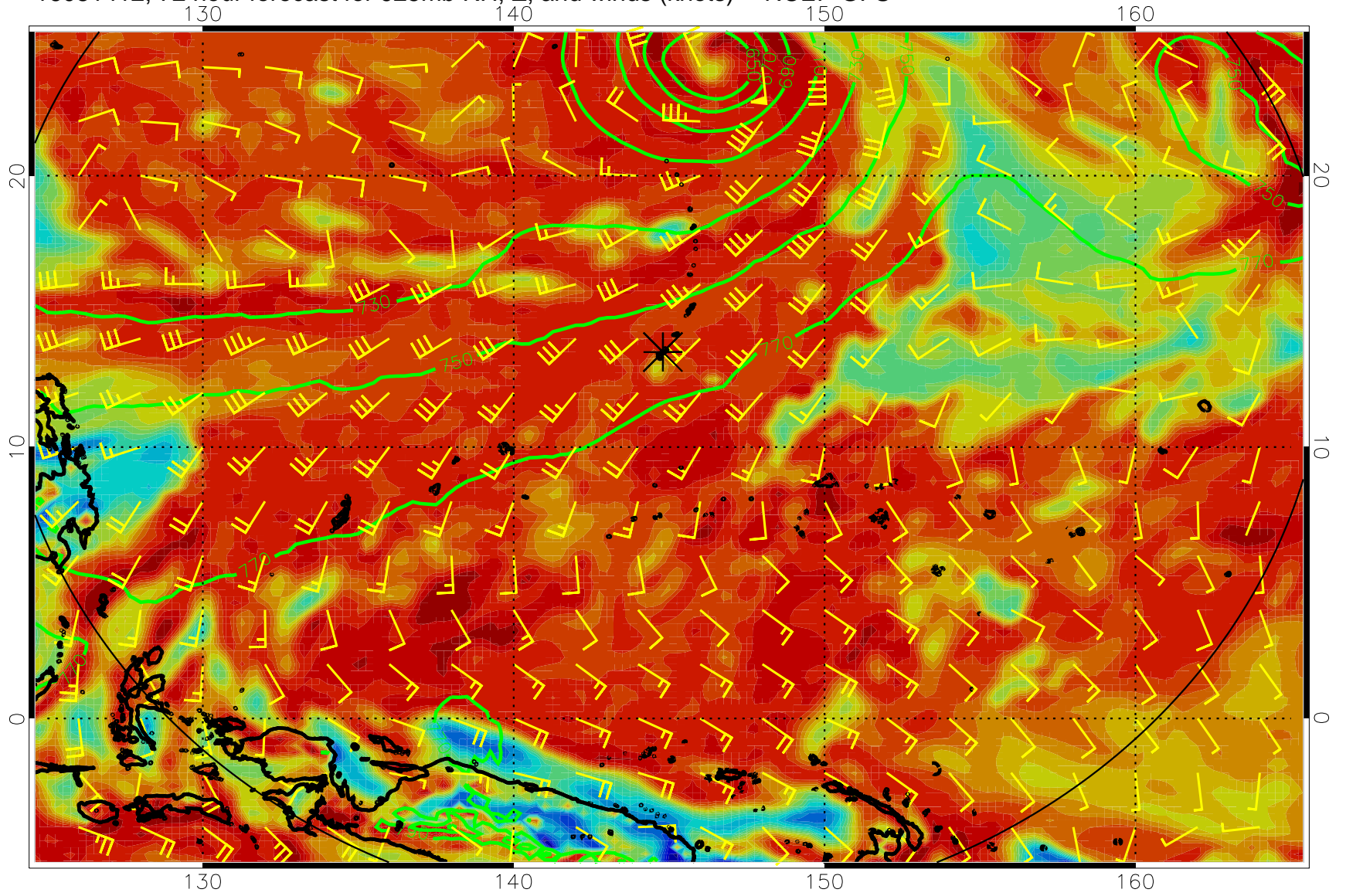
16081412, 72 hour forecast for 925mb RH, Z, and winds (knots) -- NCEP GFS
