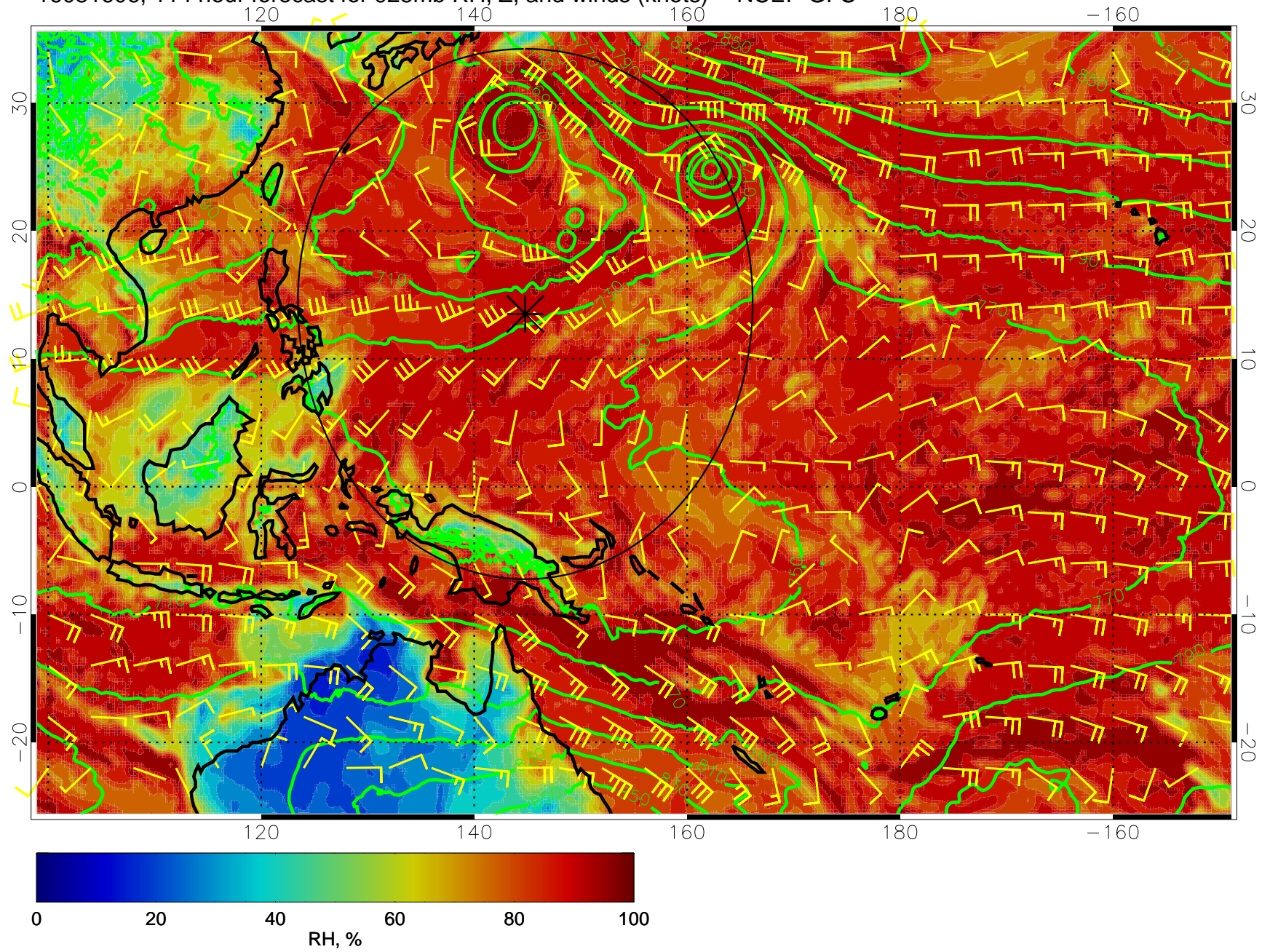
16081606, 114 hour forecast for 925mb RH, Z, and winds (knots) -- NCEP GFS
