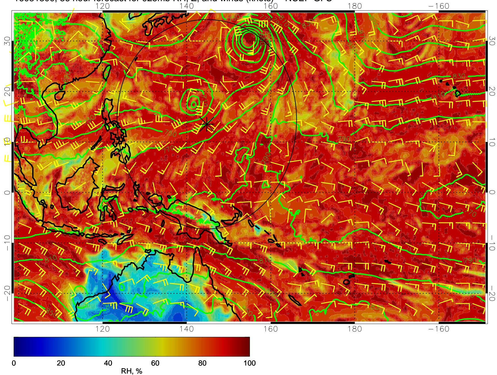
16081300, 36 hour forecast for 925mb RH, Z, and winds (knots) -- NCEP GFS
