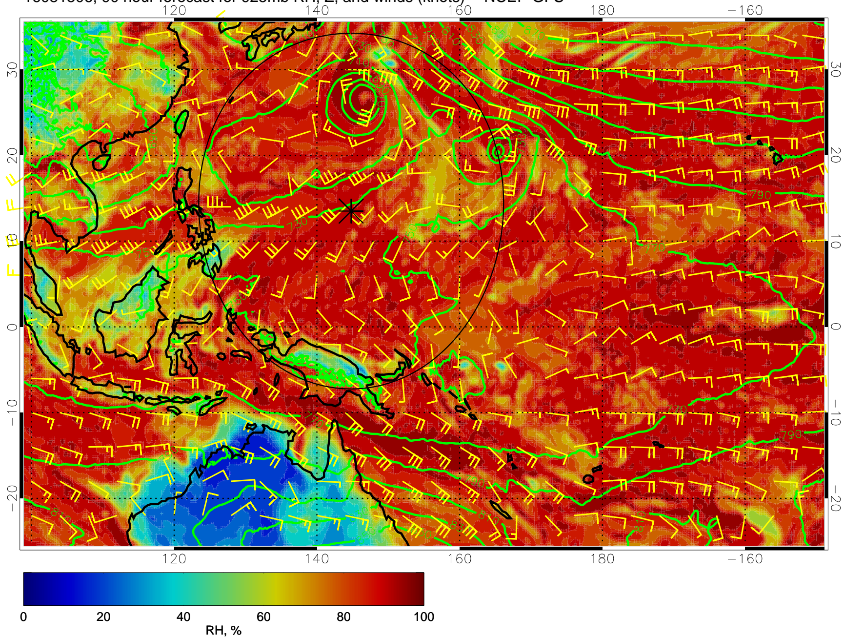
16081506, 90 hour forecast for 925mb RH, Z, and winds (knots) -- NCEP GFS
