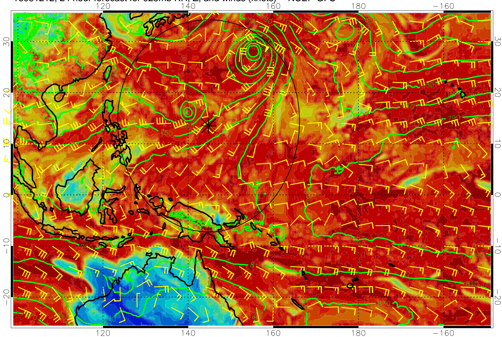
16081212, 24 hour forecast for 925mb RH, Z, and winds (knots) -- NCEP GFS
