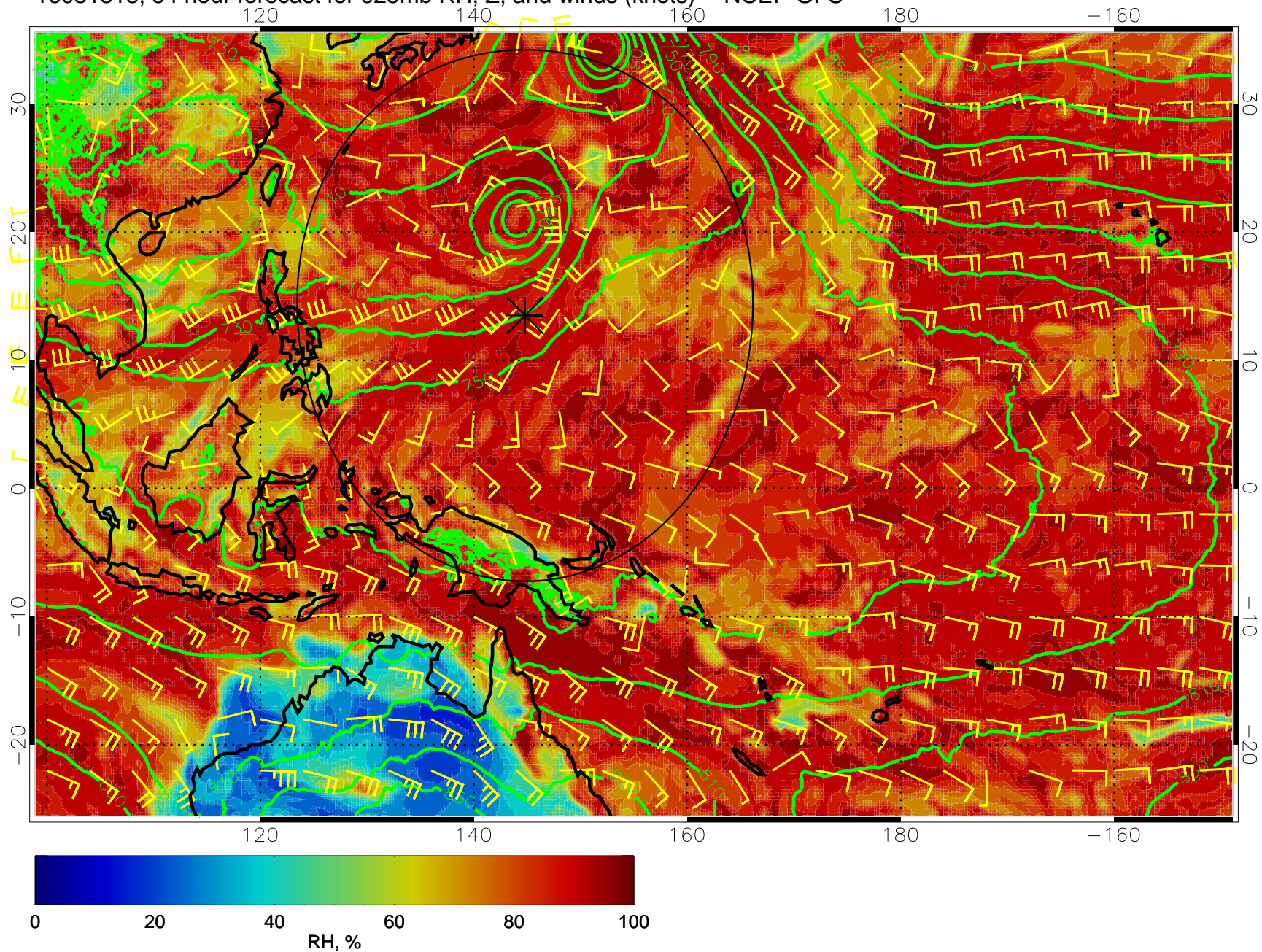
16081318, 54 hour forecast for 925mb RH, Z, and winds (knots) -- NCEP GFS
