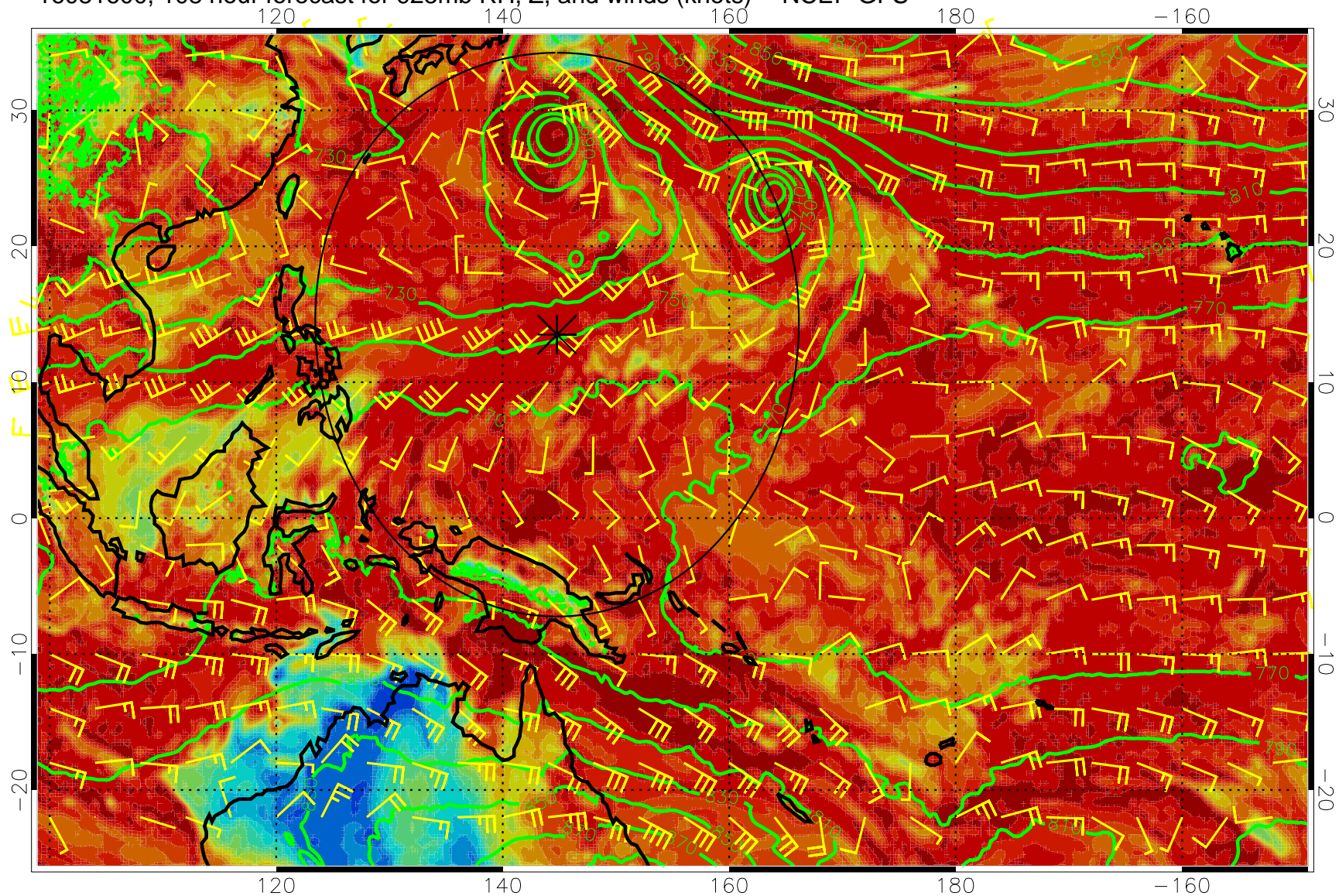
16081600, 108 hour forecast for 925mb RH, Z, and winds (knots) -- NCEP GFS
