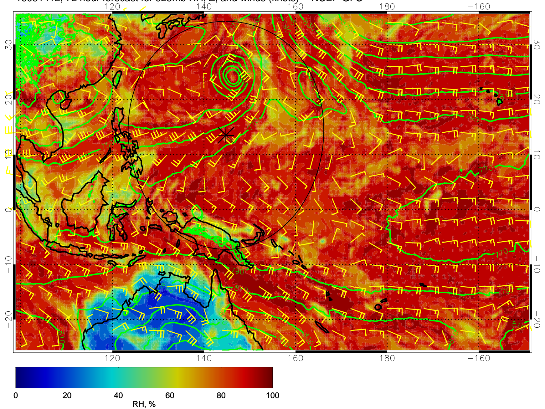
16081412, 72 hour forecast for 925mb RH, Z, and winds (knots) -- NCEP GFS
