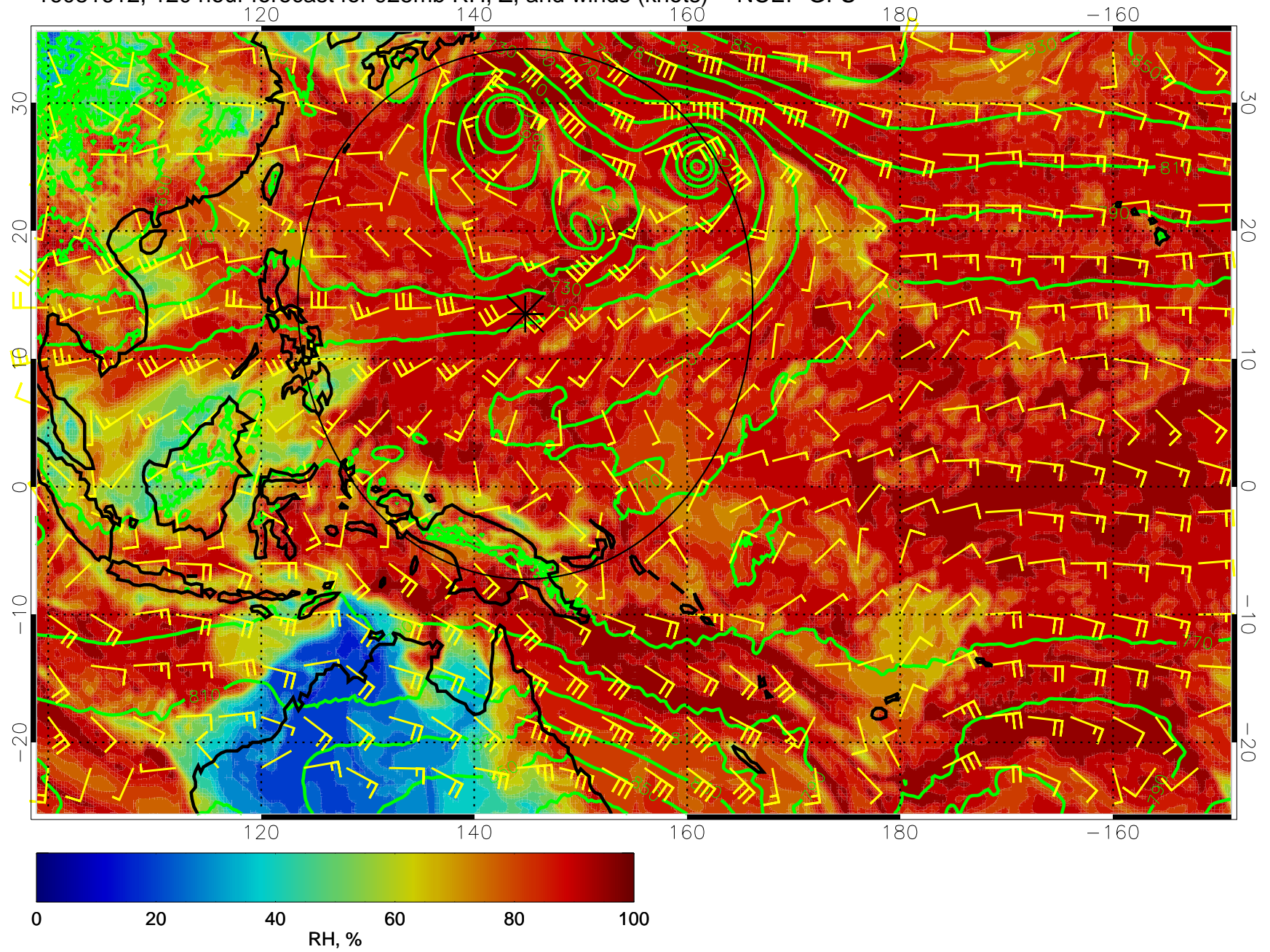
16081612, 120 hour forecast for 925mb RH, Z, and winds (knots) -- NCEP GFS
