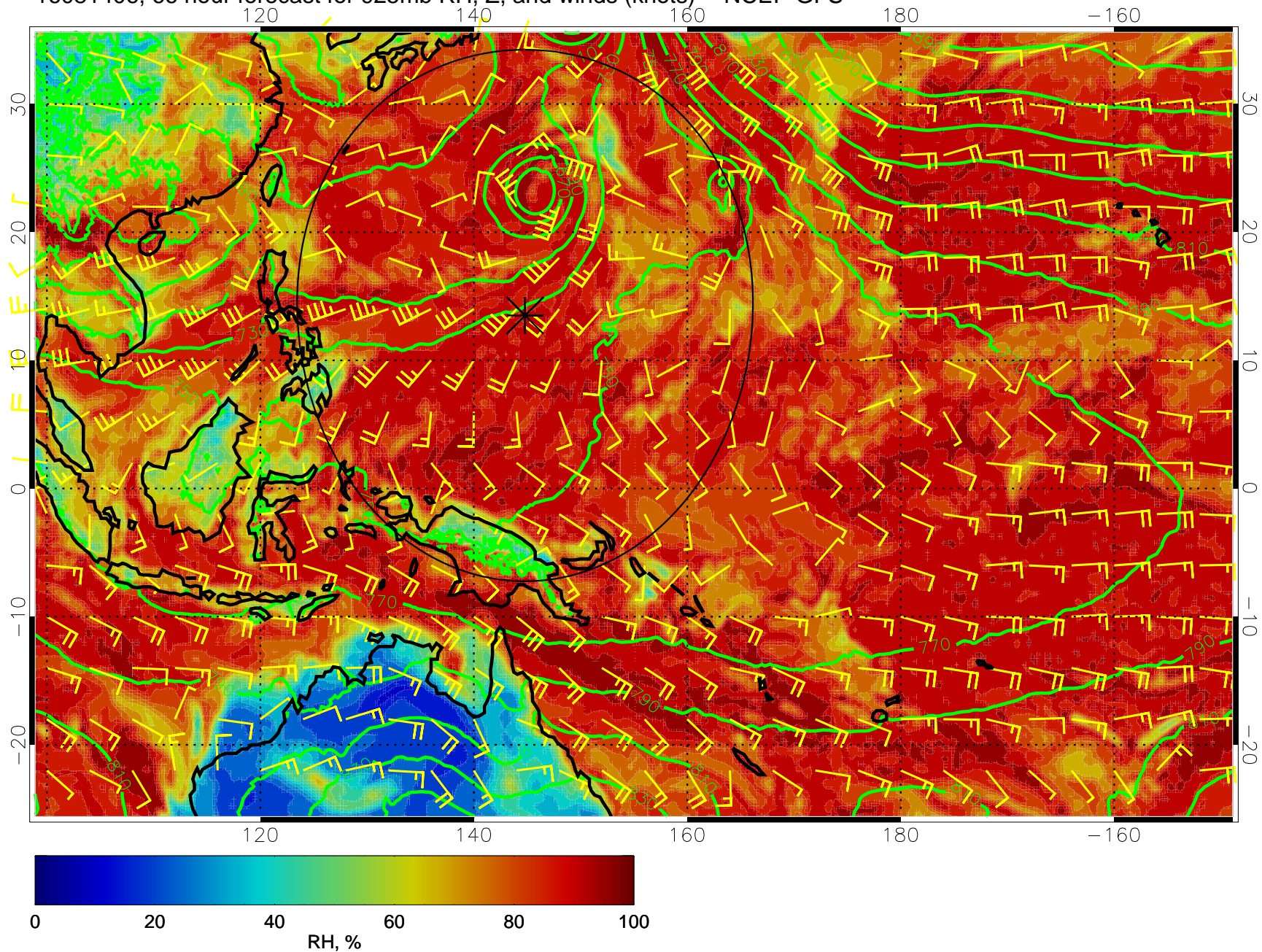
16081406, 66 hour forecast for 925mb RH, Z, and winds (knots) -- NCEP GFS
