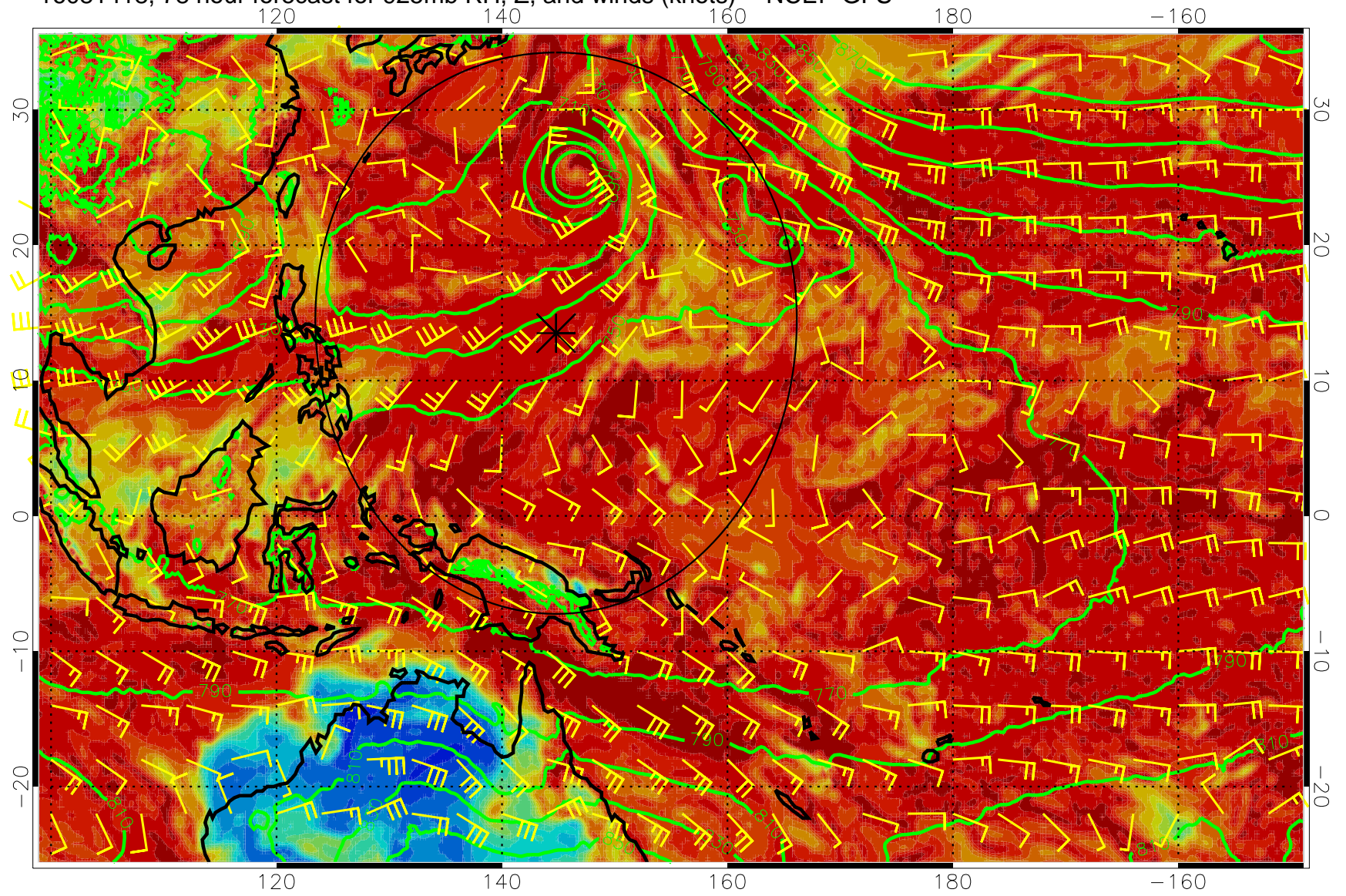
16081418, 78 hour forecast for 925mb RH, Z, and winds (knots) -- NCEP GFS
