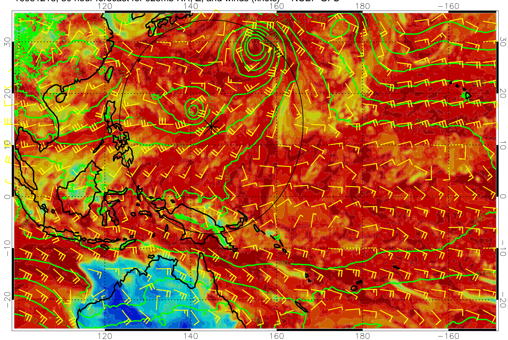
16081218, 30 hour forecast for 925mb RH, Z, and winds (knots) -- NCEP GFS
