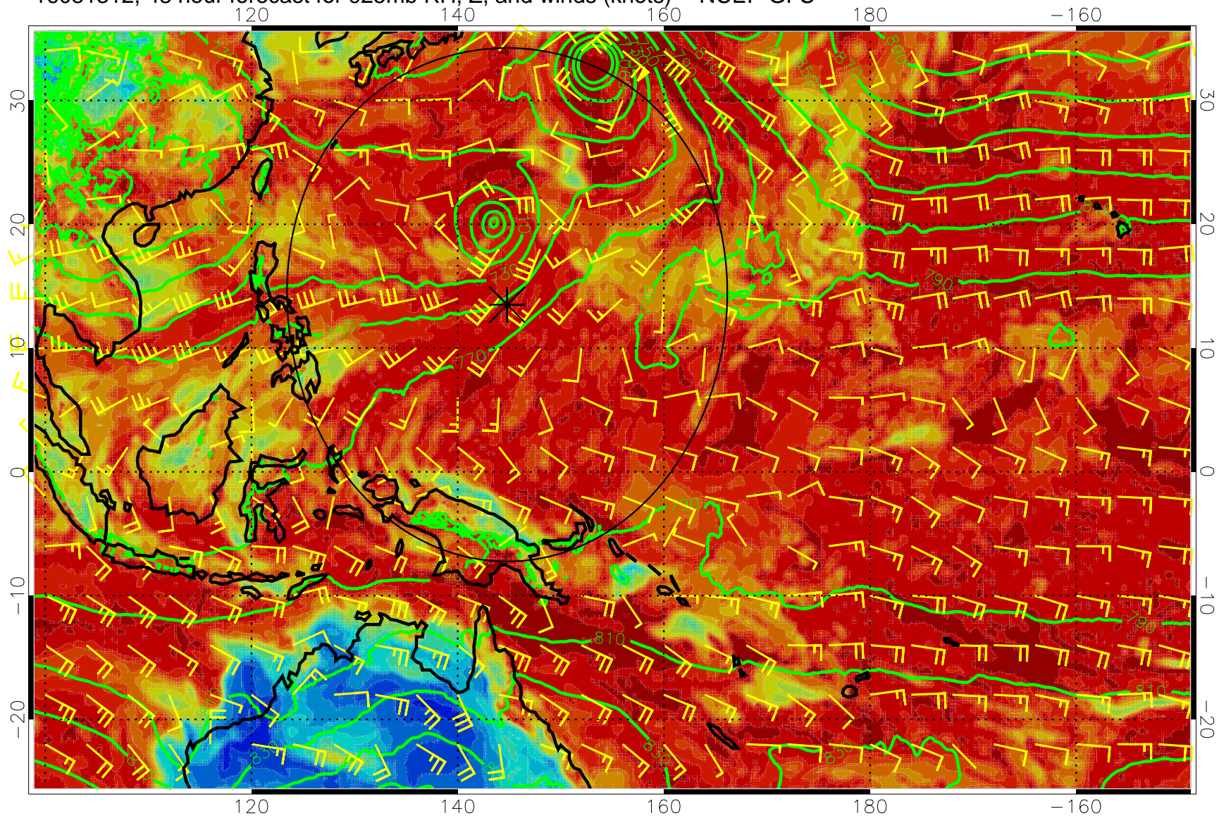
16081312, 48 hour forecast for 925mb RH, Z, and winds (knots) -- NCEP GFS
