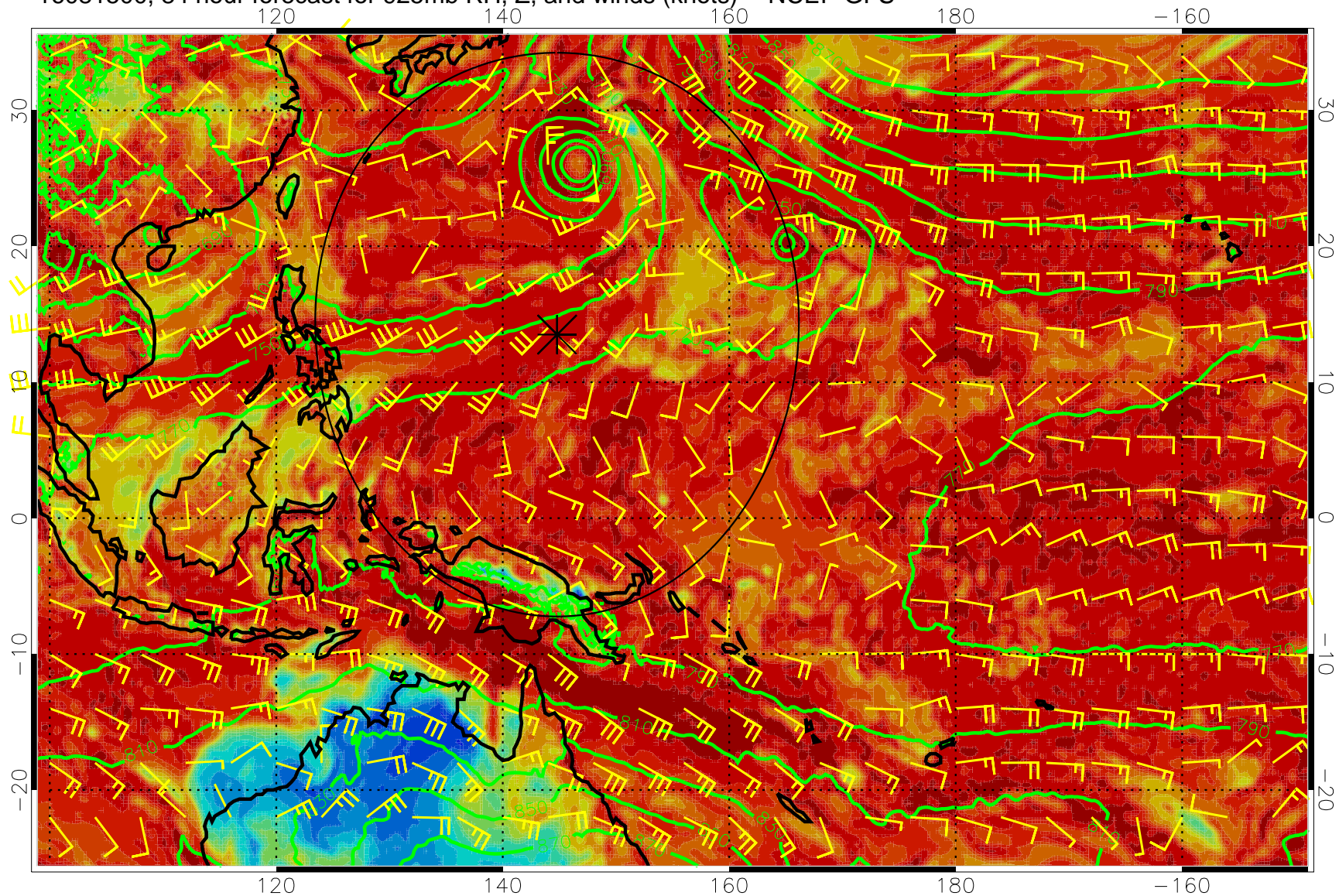
16081500, 84 hour forecast for 925mb RH, Z, and winds (knots) -- NCEP GFS
