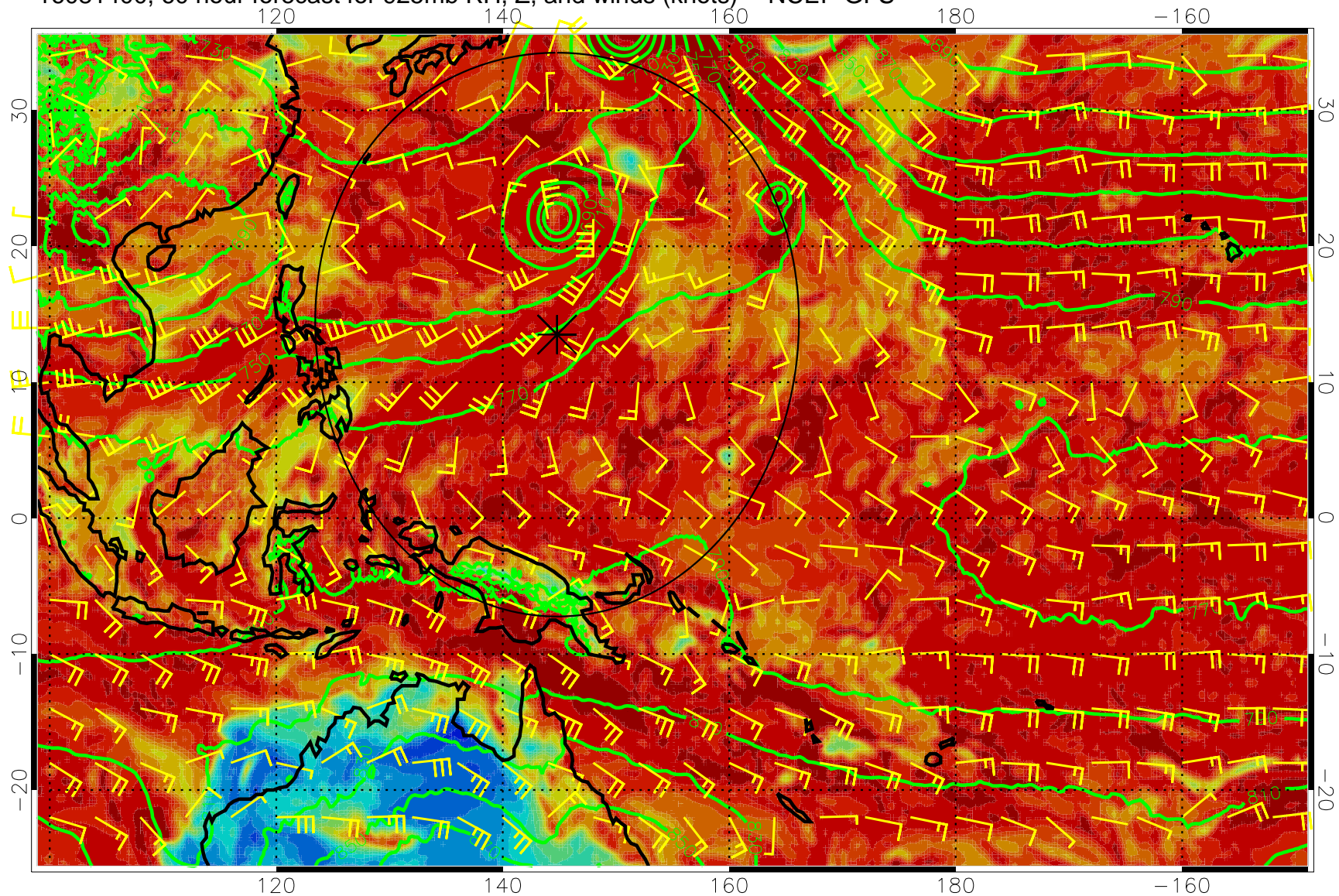
16081400, 60 hour forecast for 925mb RH, Z, and winds (knots) -- NCEP GFS
