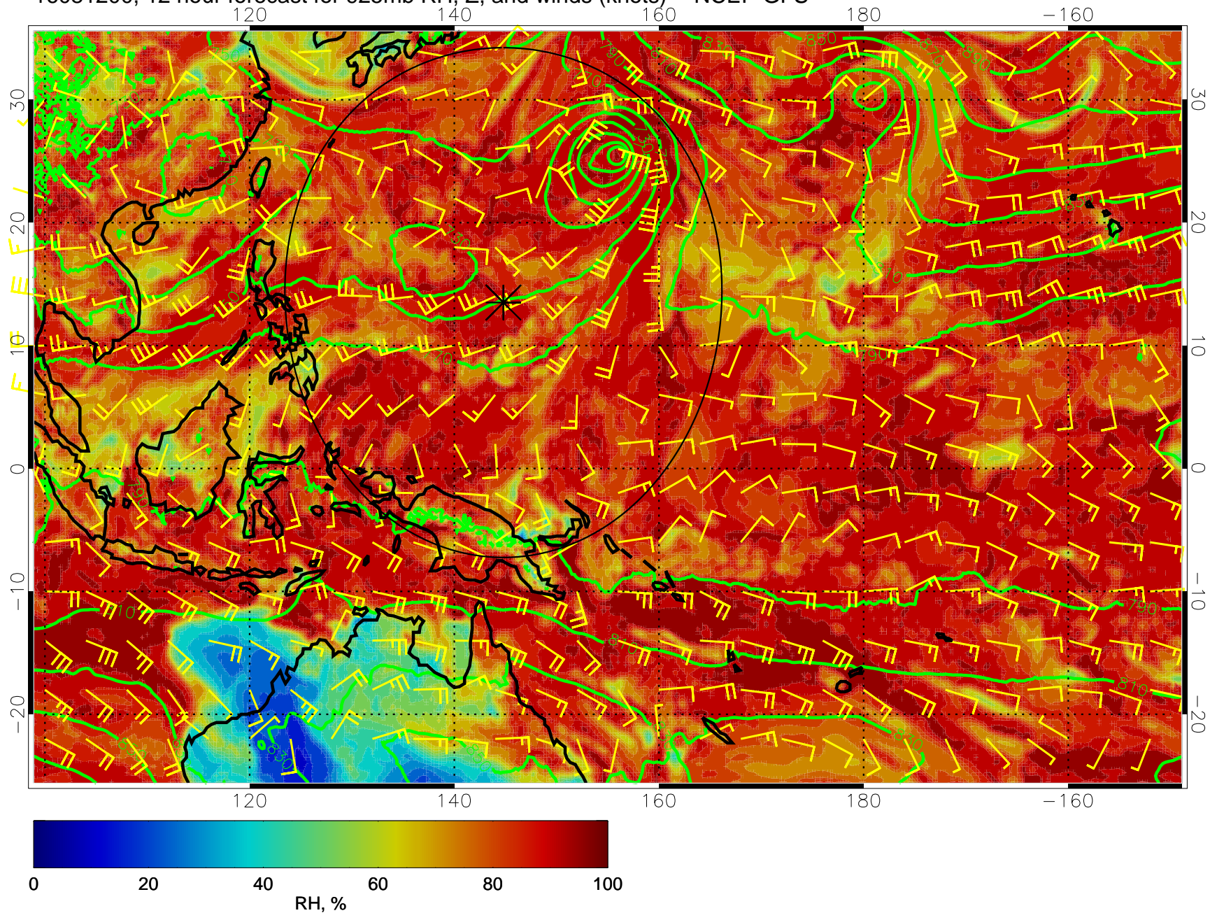
16081200, 12 hour forecast for 925mb RH, Z, and winds (knots) -- NCEP GFS
