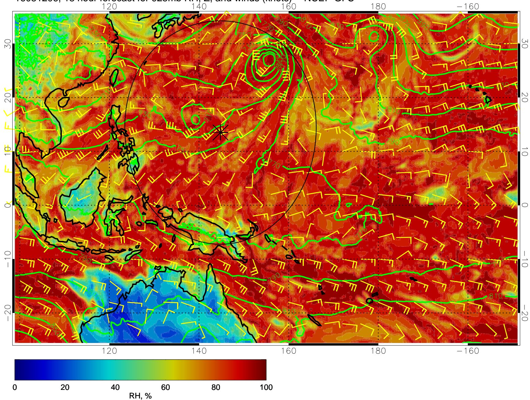
16081206, 18 hour forecast for 925mb RH, Z, and winds (knots) -- NCEP GFS
