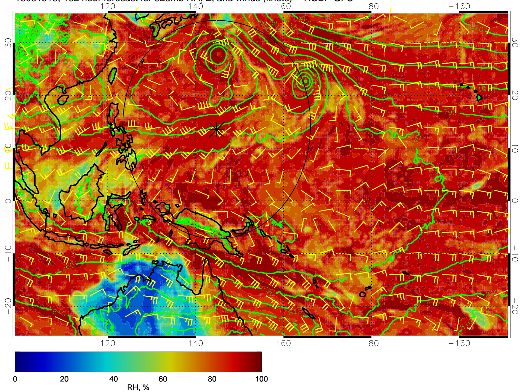
16081518, 102 hour forecast for 925mb RH, Z, and winds (knots) -- NCEP GFS
