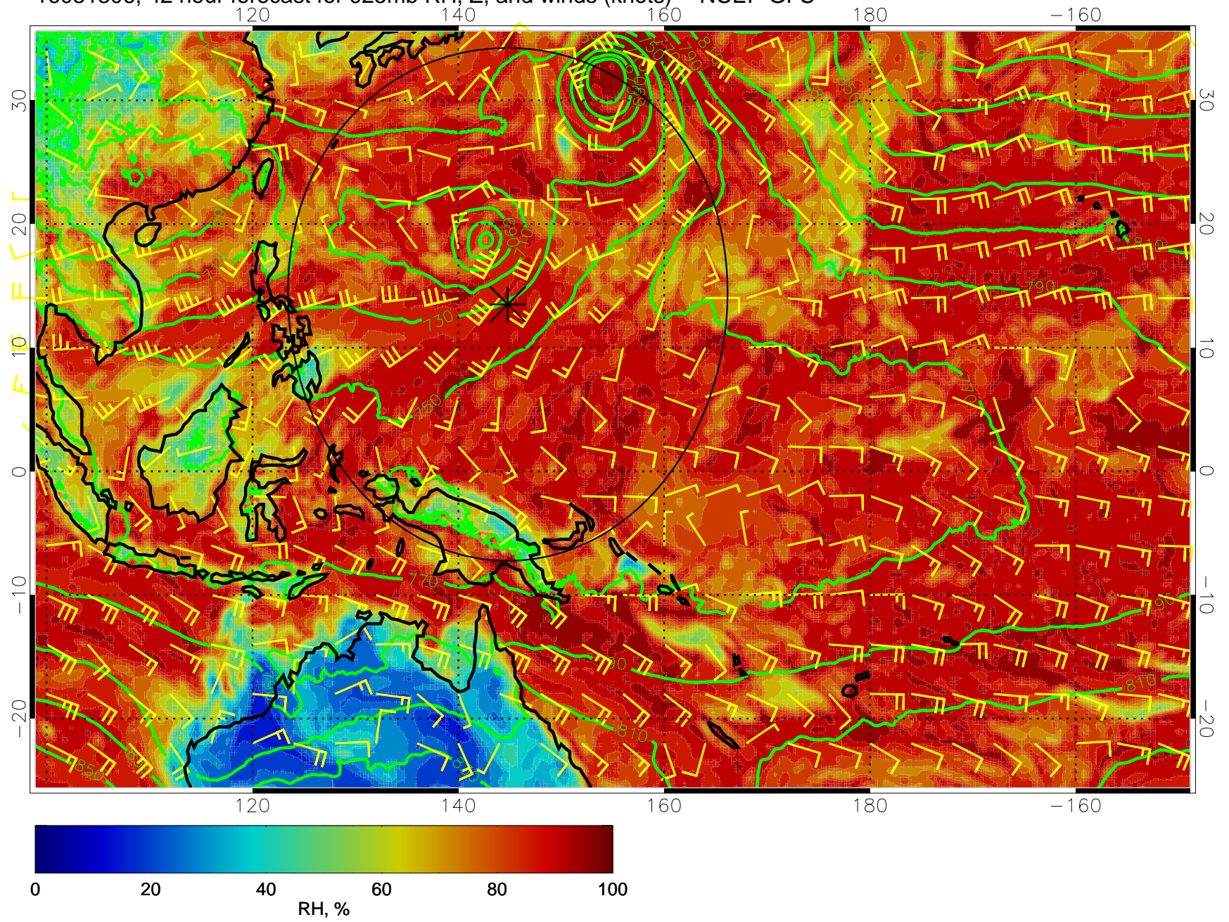
16081306, 42 hour forecast for 925mb RH, Z, and winds (knots) -- NCEP GFS
