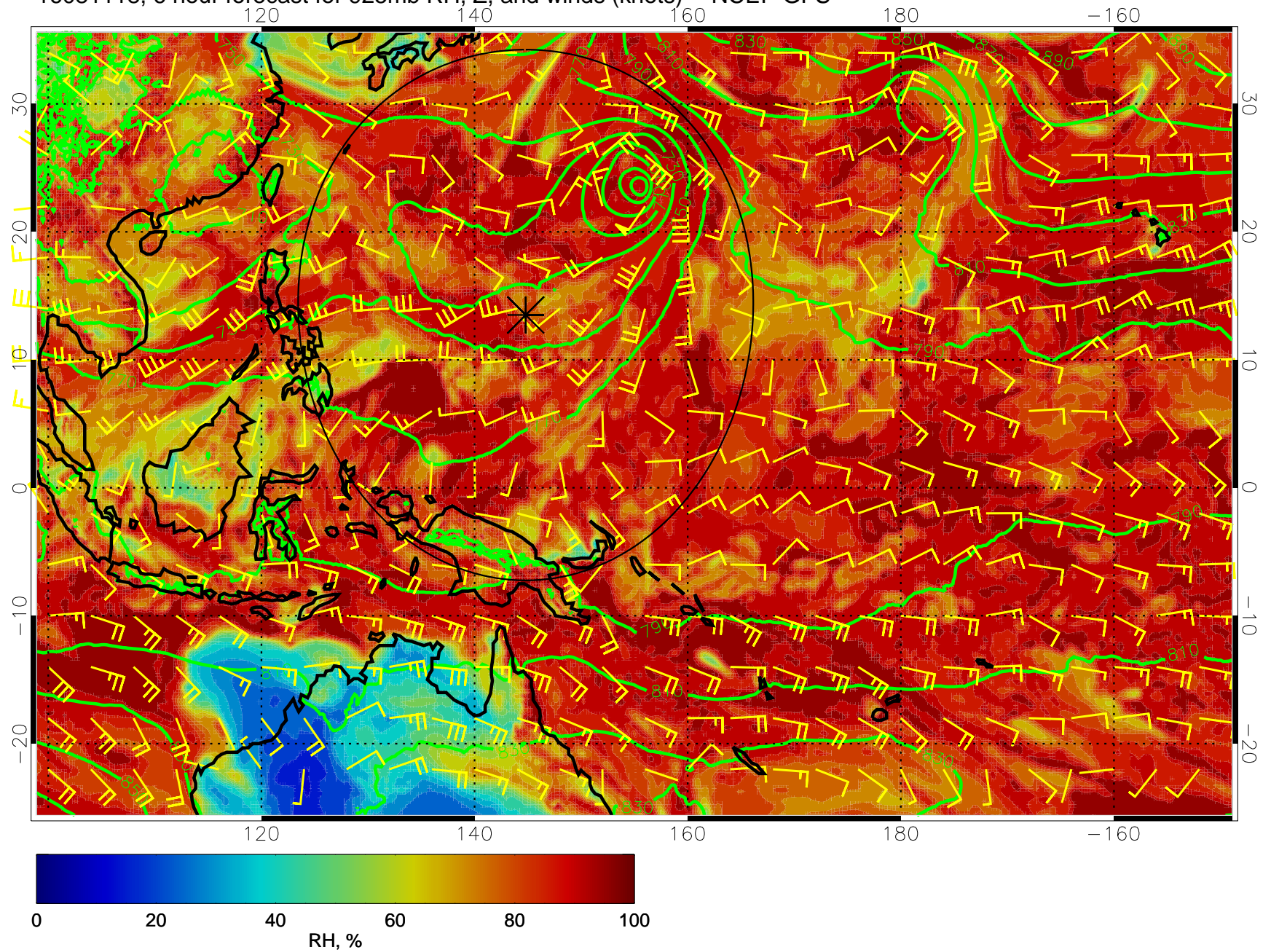
16081118, 6 hour forecast for 925mb RH, Z, and winds (knots) -- NCEP GFS
