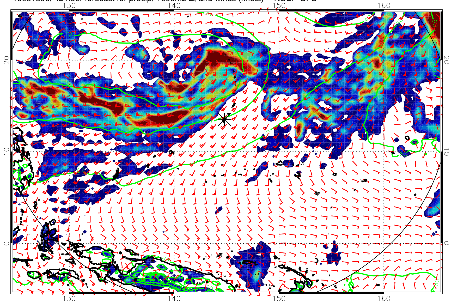
16081306, 42 hour forecast for precip, 1000mb Z, and winds (knots) -- NCEP GFS
