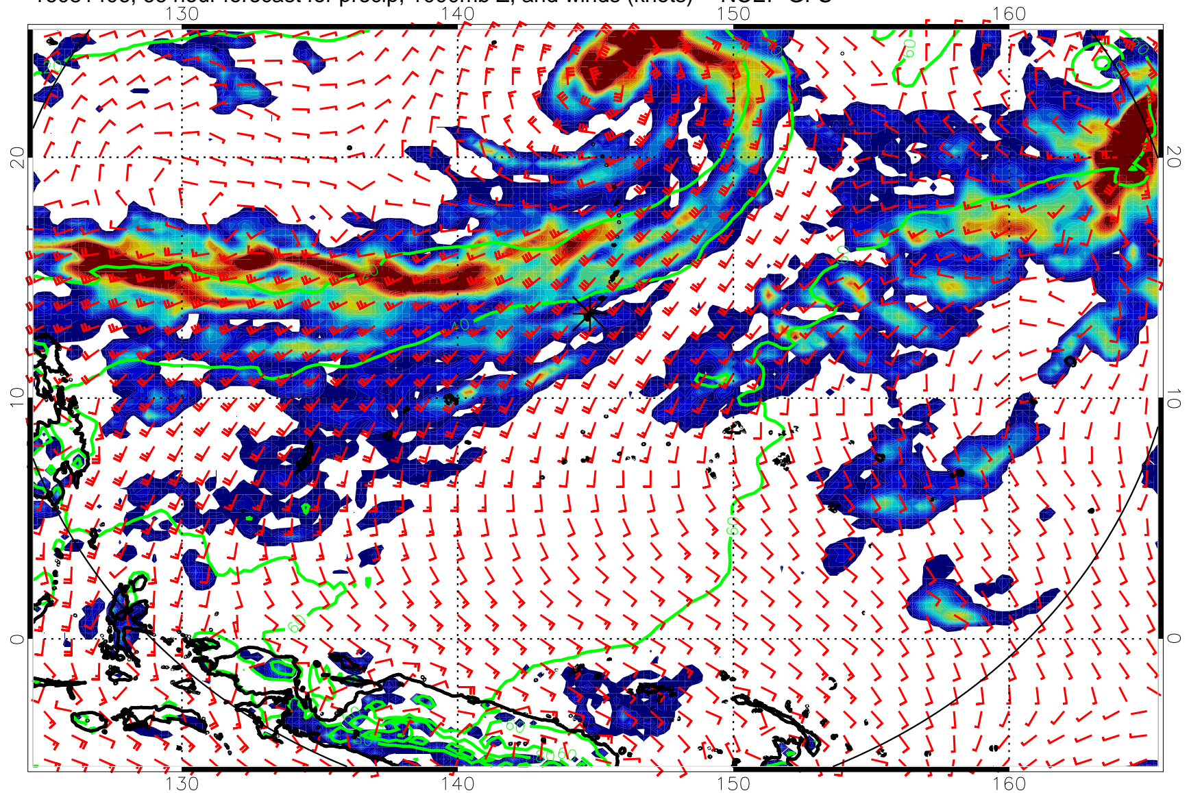
16081406, 66 hour forecast for precip, 1000mb Z, and winds (knots) -- NCEP GFS
