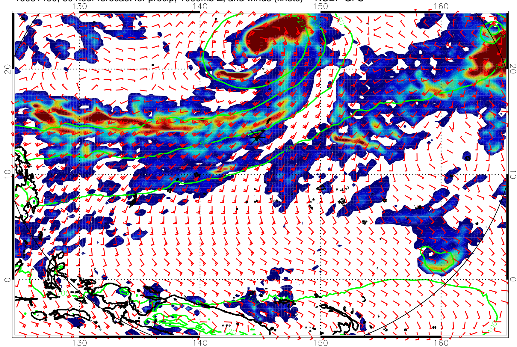
16081400, 60 hour forecast for precip, 1000mb Z, and winds (knots) -- NCEP GFS
