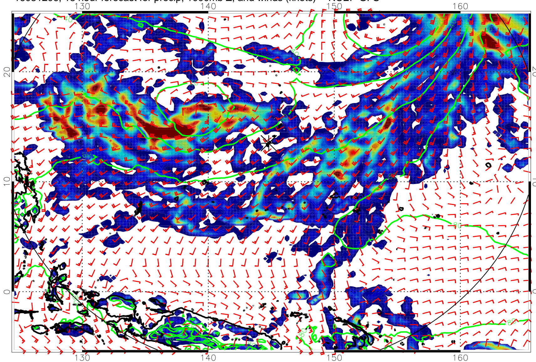
16081206, 18 hour forecast for precip, 1000mb Z, and winds (knots) -- NCEP GFS
