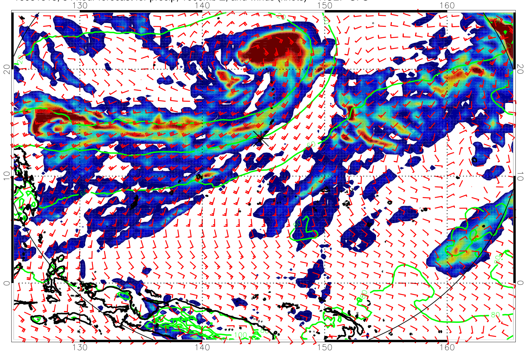
16081318, 54 hour forecast for precip, 1000mb Z, and winds (knots) -- NCEP GFS
