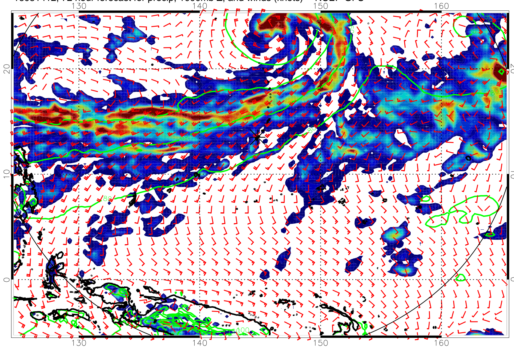
16081412, 72 hour forecast for precip, 1000mb Z, and winds (knots) -- NCEP GFS
