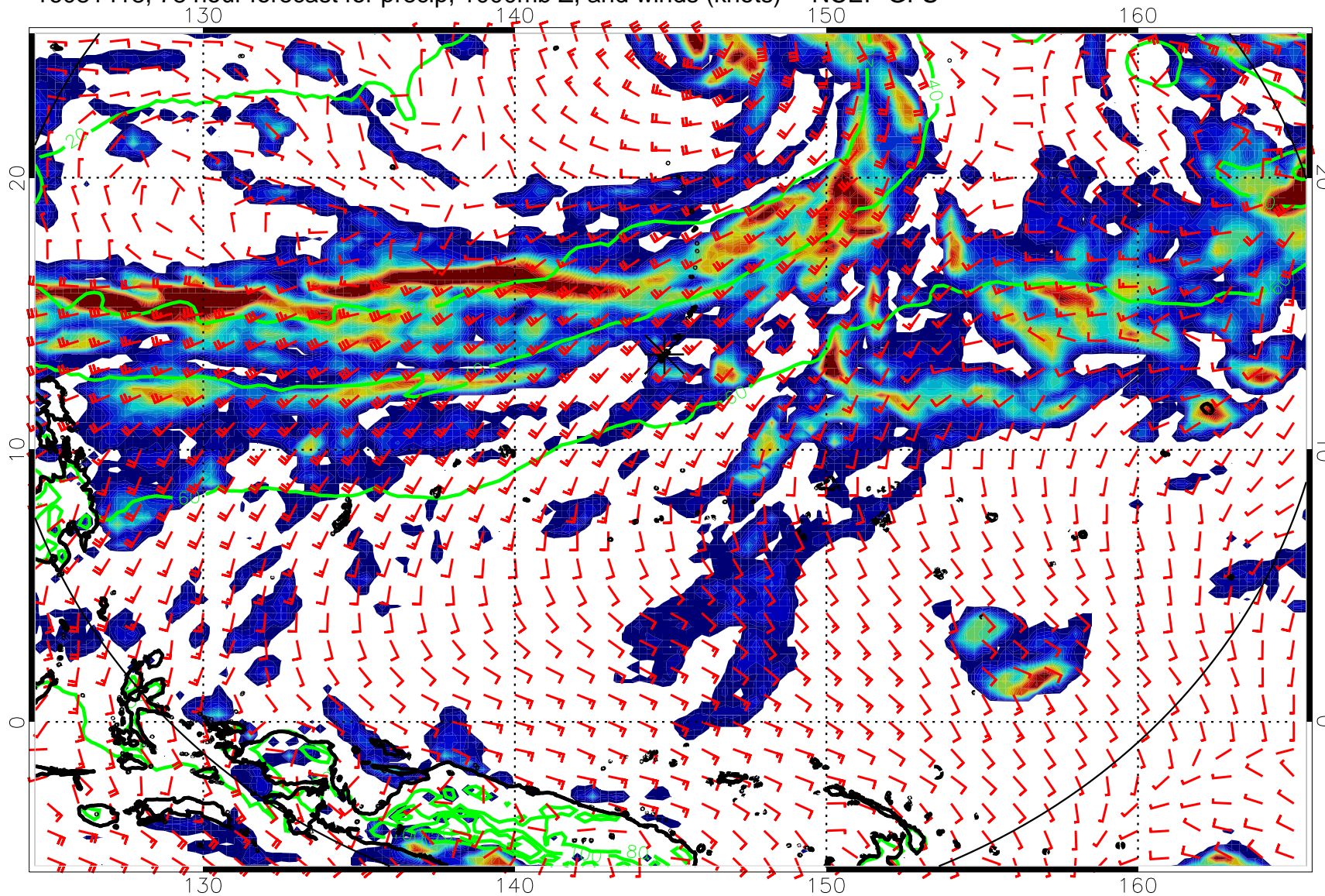
16081418, 78 hour forecast for precip, 1000mb Z, and winds (knots) -- NCEP GFS
