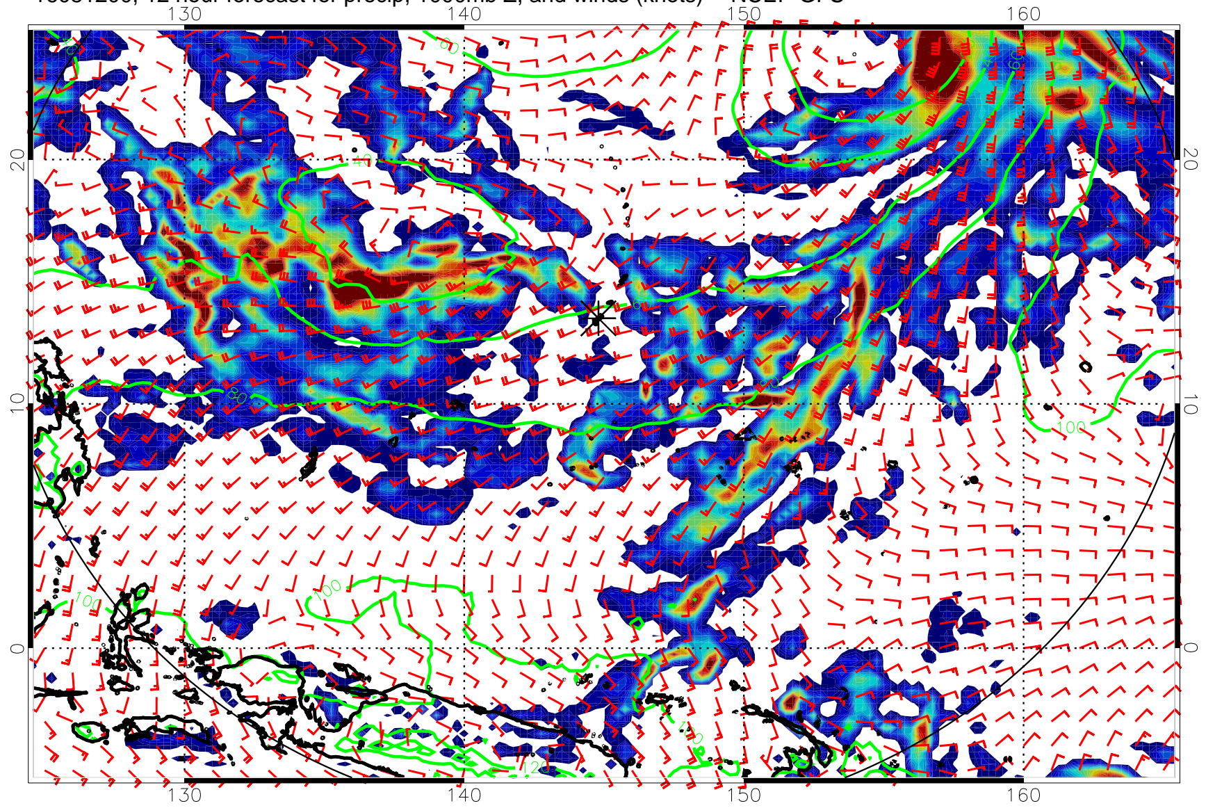
16081200, 12 hour forecast for precip, 1000mb Z, and winds (knots) -- NCEP GFS
