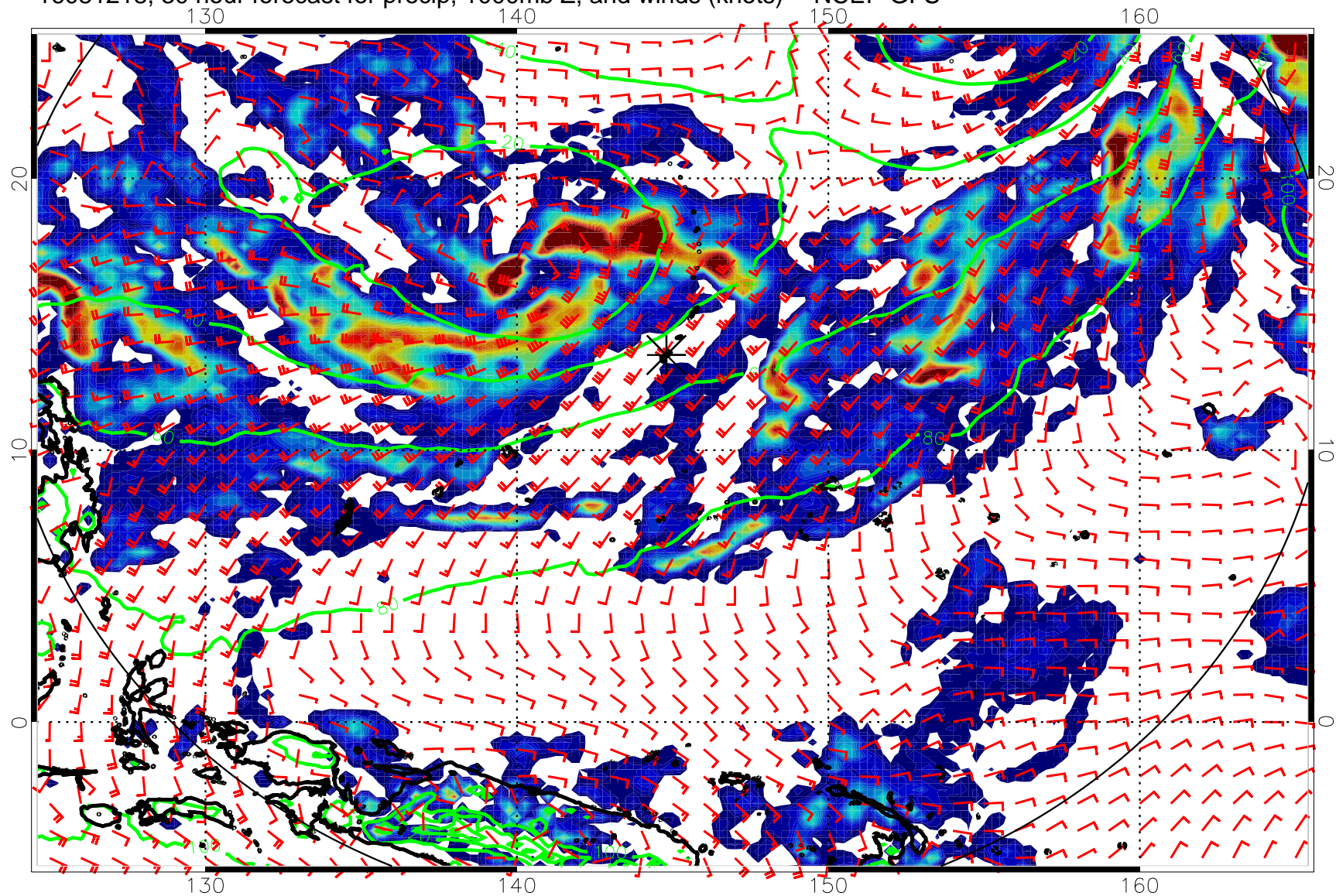
16081218, 30 hour forecast for precip, 1000mb Z, and winds (knots) -- NCEP GFS
