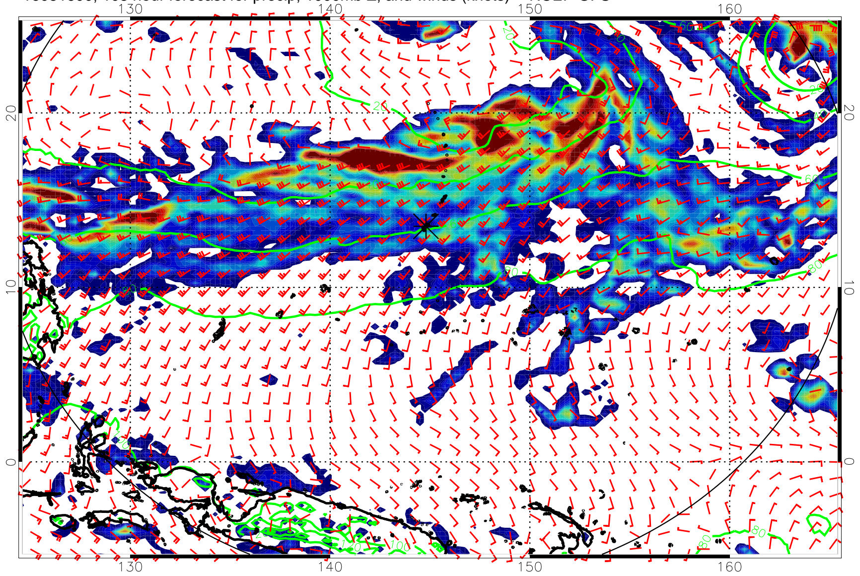
16081600, 108 hour forecast for precip, 1000mb Z, and winds (knots) -- NCEP GFS
