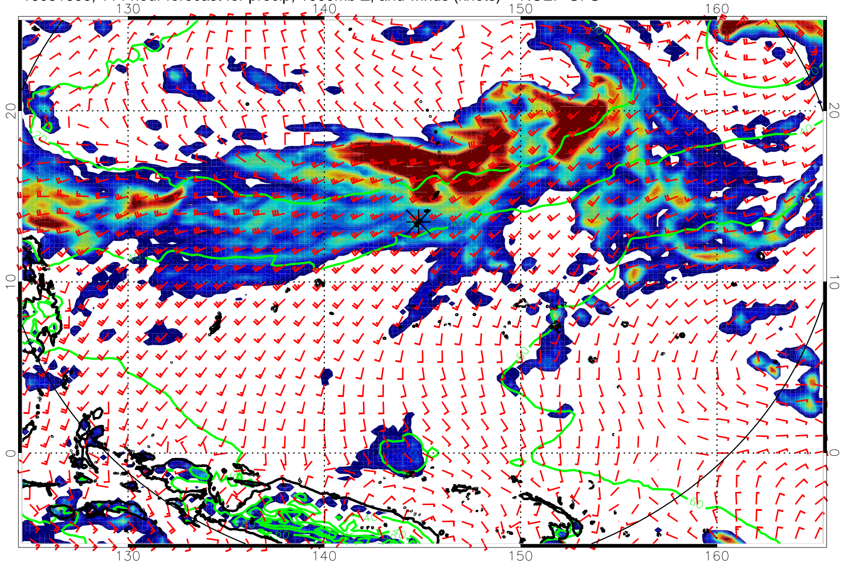
16081606, 114 hour forecast for precip, 1000mb Z, and winds (knots) -- NCEP GFS
