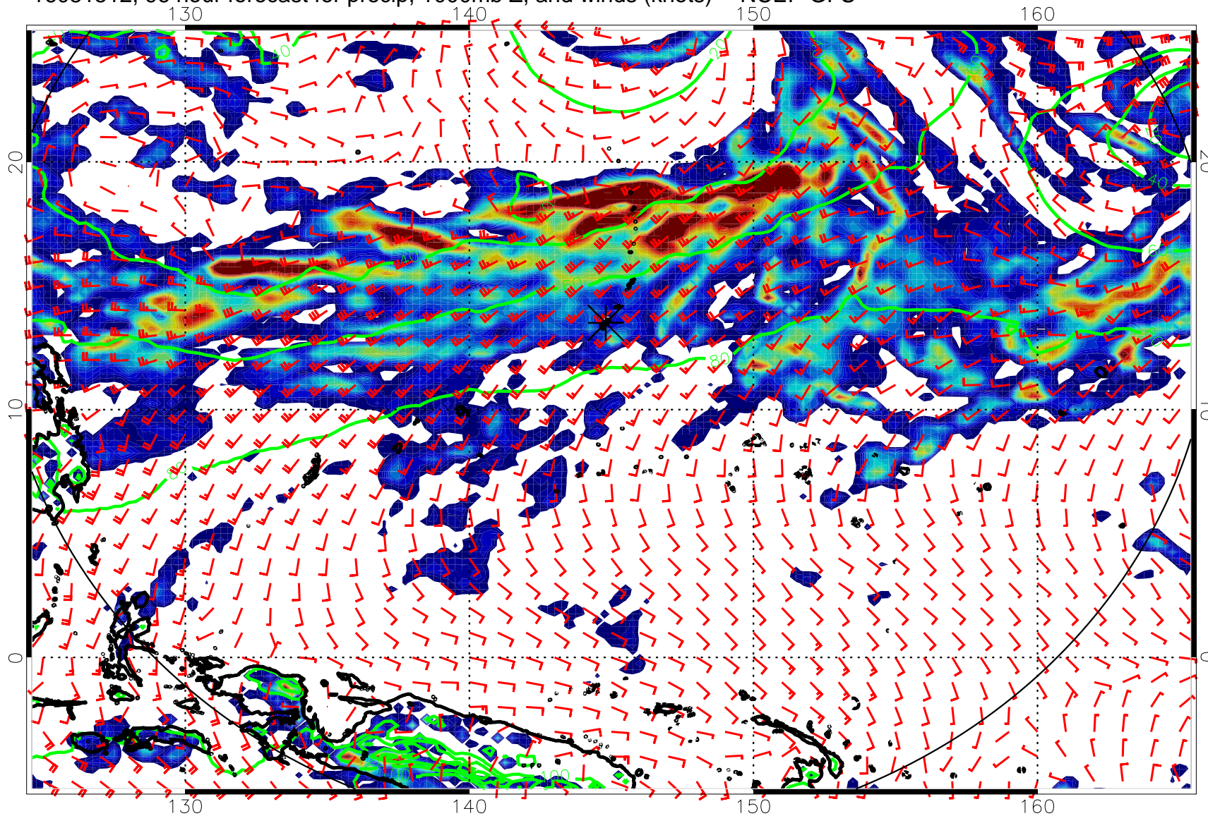
16081512, 96 hour forecast for precip, 1000mb Z, and winds (knots) -- NCEP GFS
