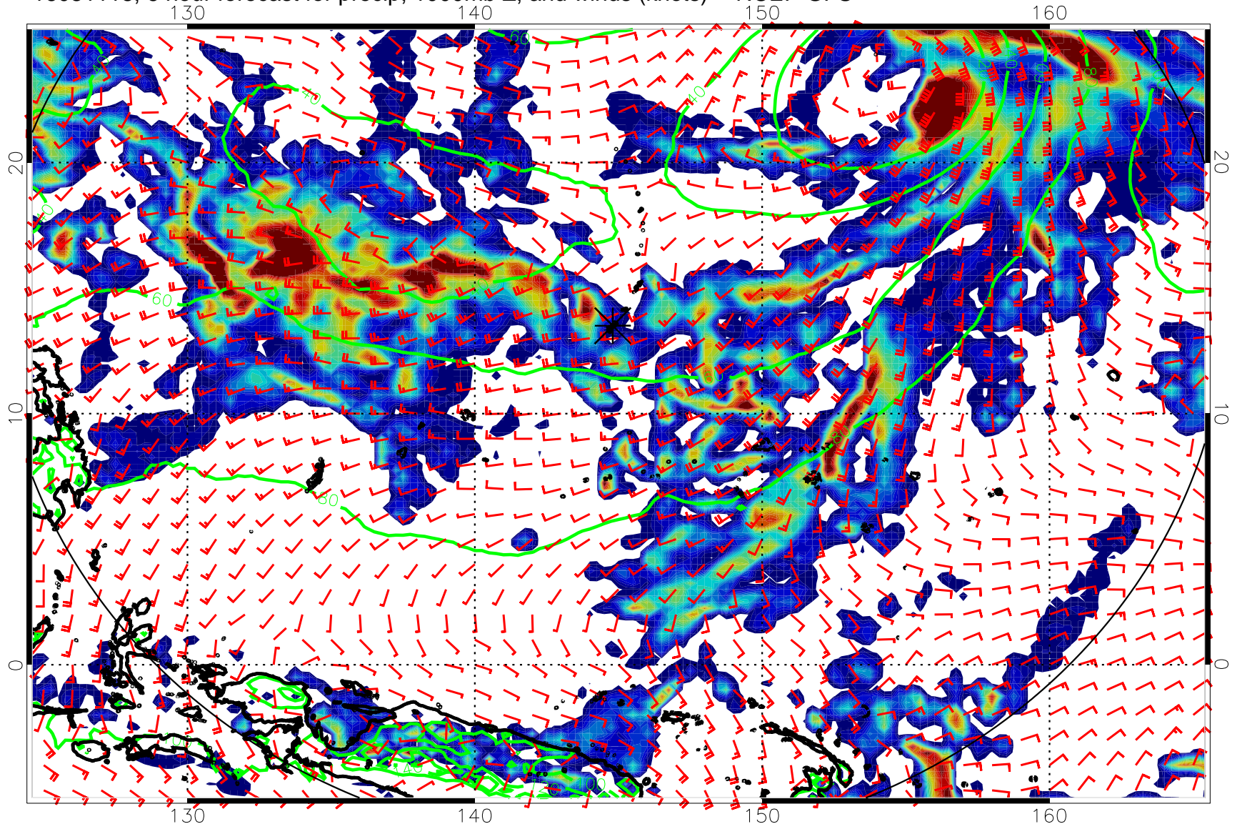
16081118, 6 hour forecast for precip, 1000mb Z, and winds (knots) -- NCEP GFS
