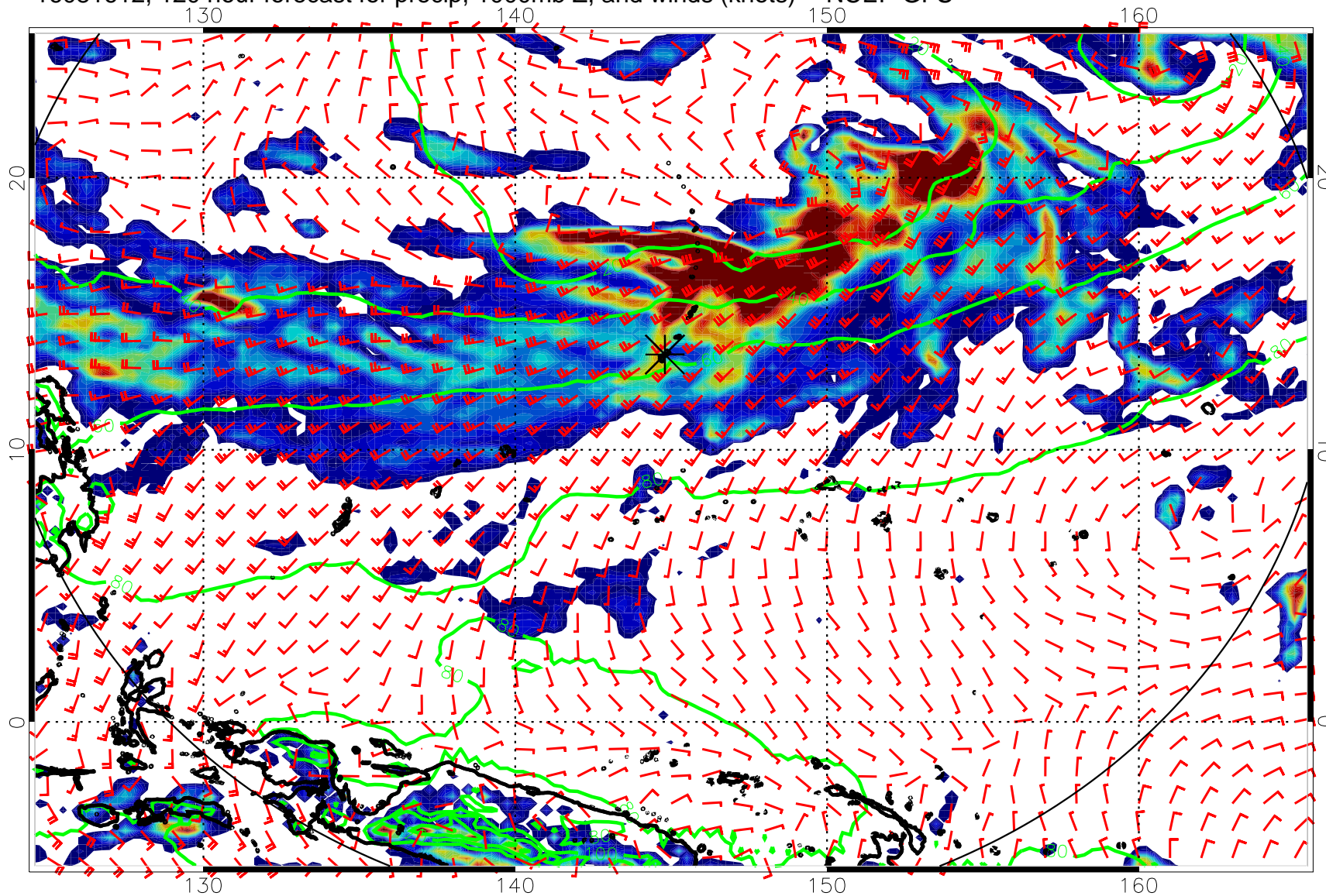
16081612, 120 hour forecast for precip, 1000mb Z, and winds (knots) -- NCEP GFS
