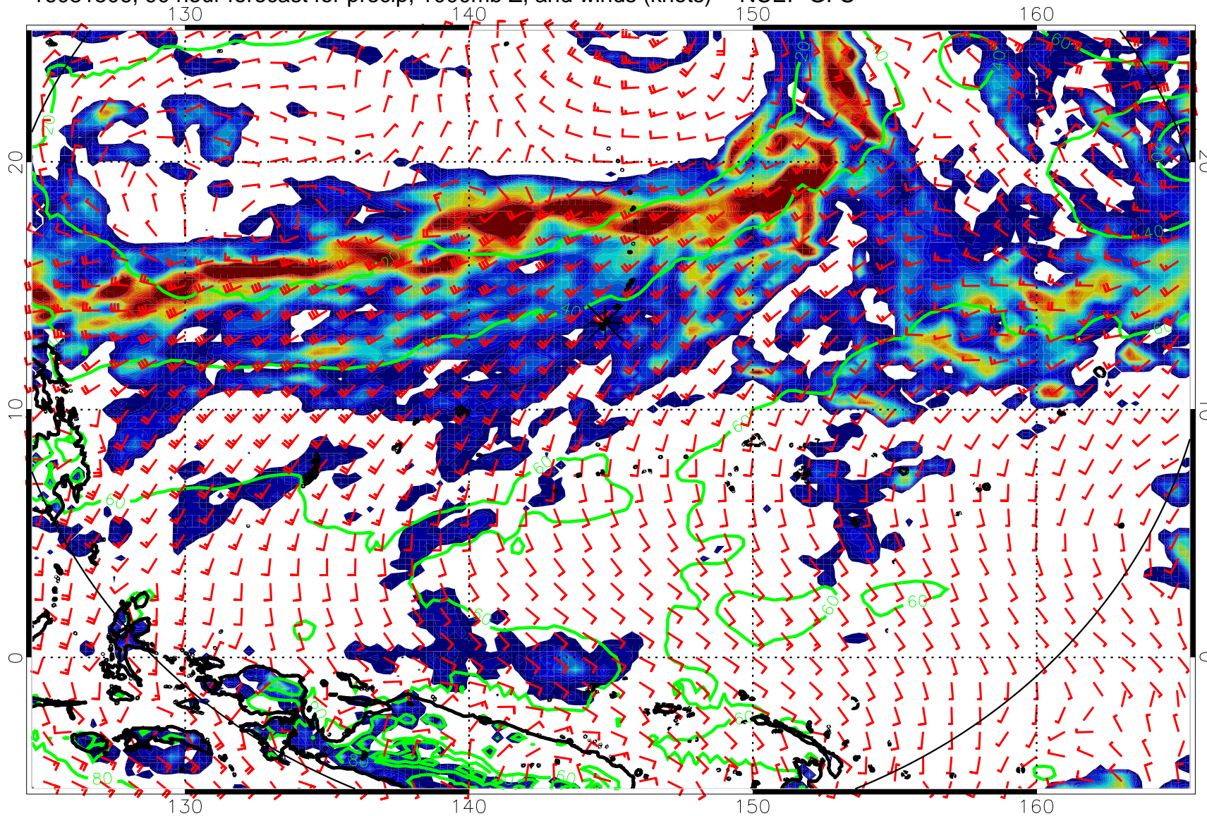
16081506, 90 hour forecast for precip, 1000mb Z, and winds (knots) -- NCEP GFS
