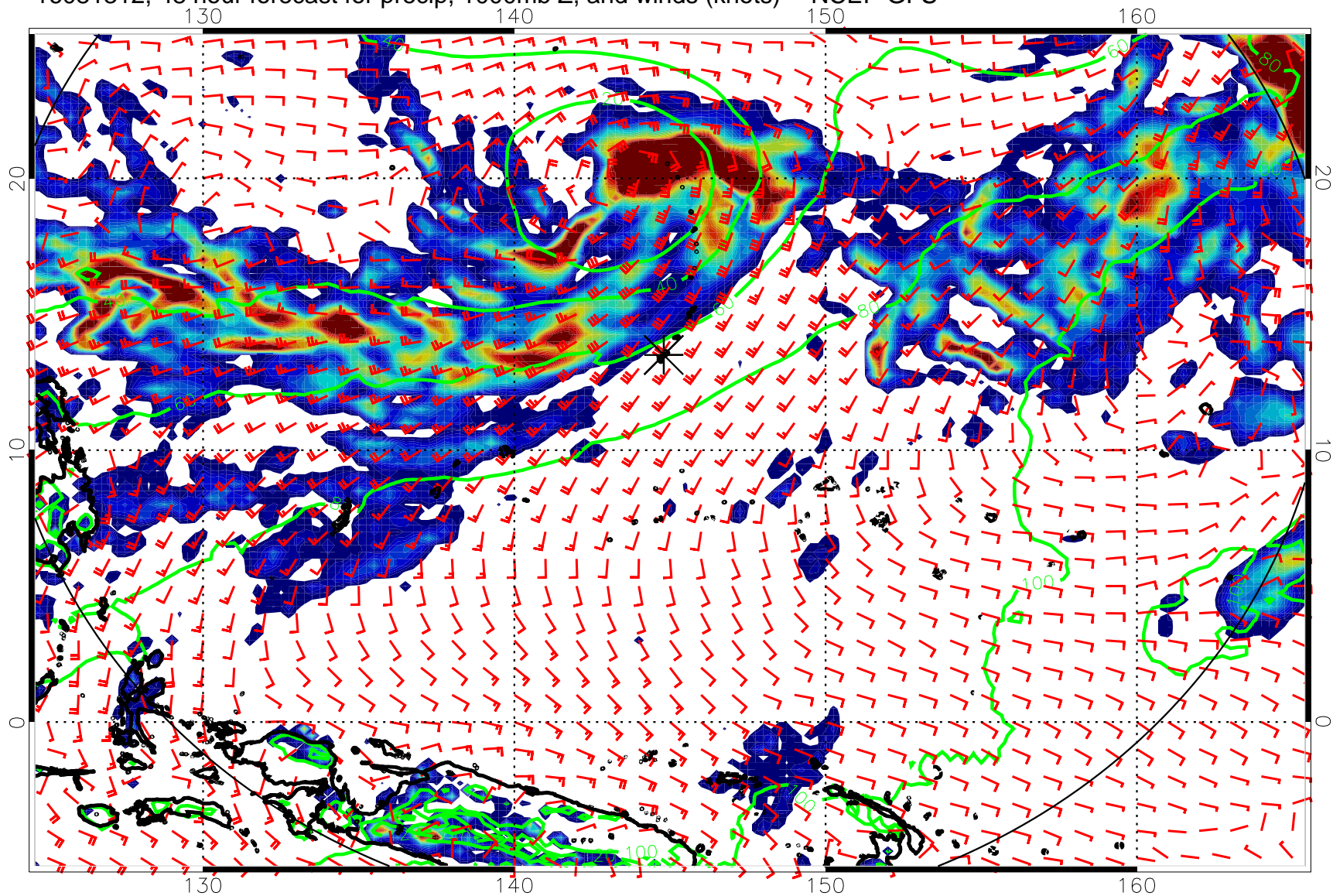
16081312, 48 hour forecast for precip, 1000mb Z, and winds (knots) -- NCEP GFS
