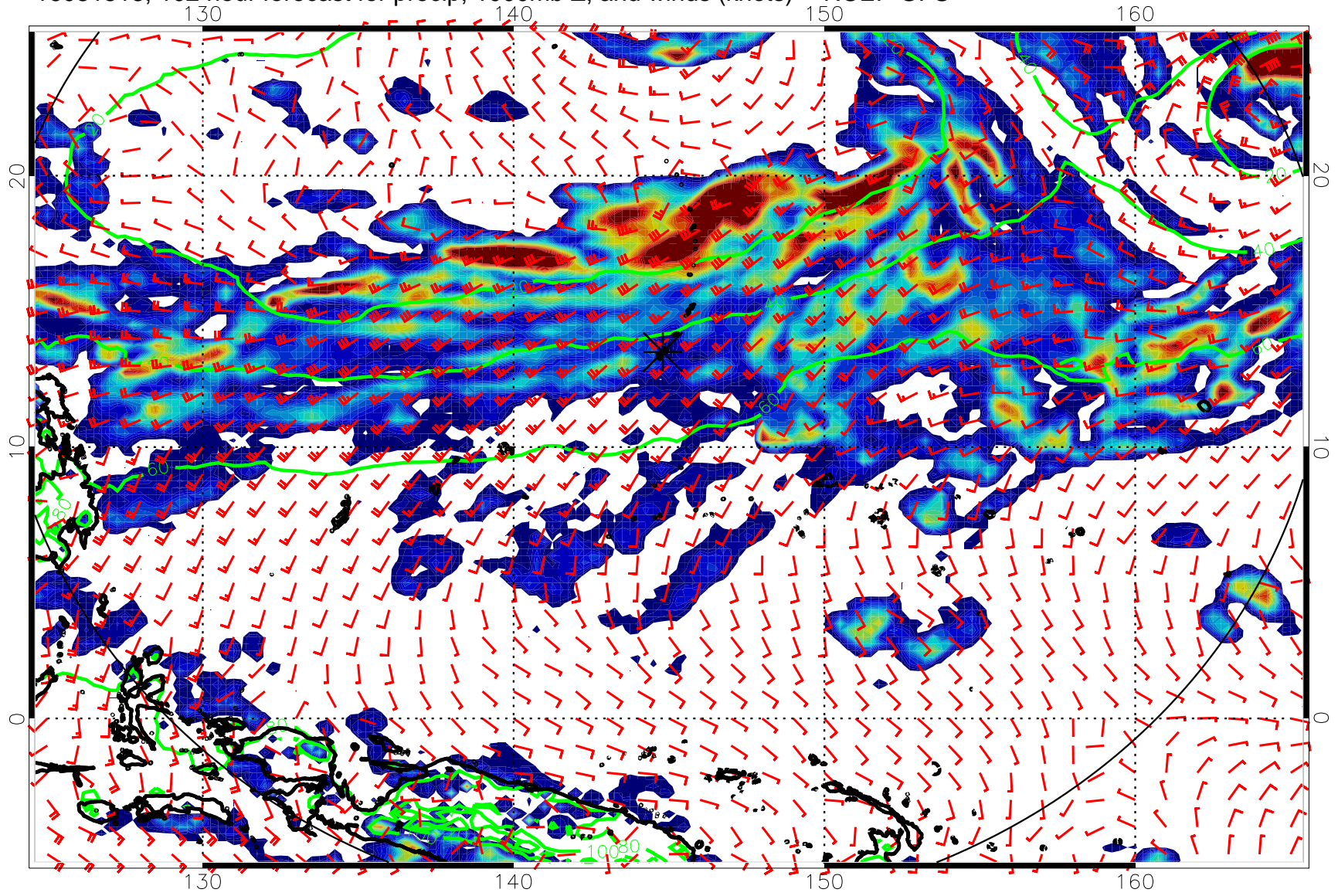
16081518, 102 hour forecast for precip, 1000mb Z, and winds (knots) -- NCEP GFS
