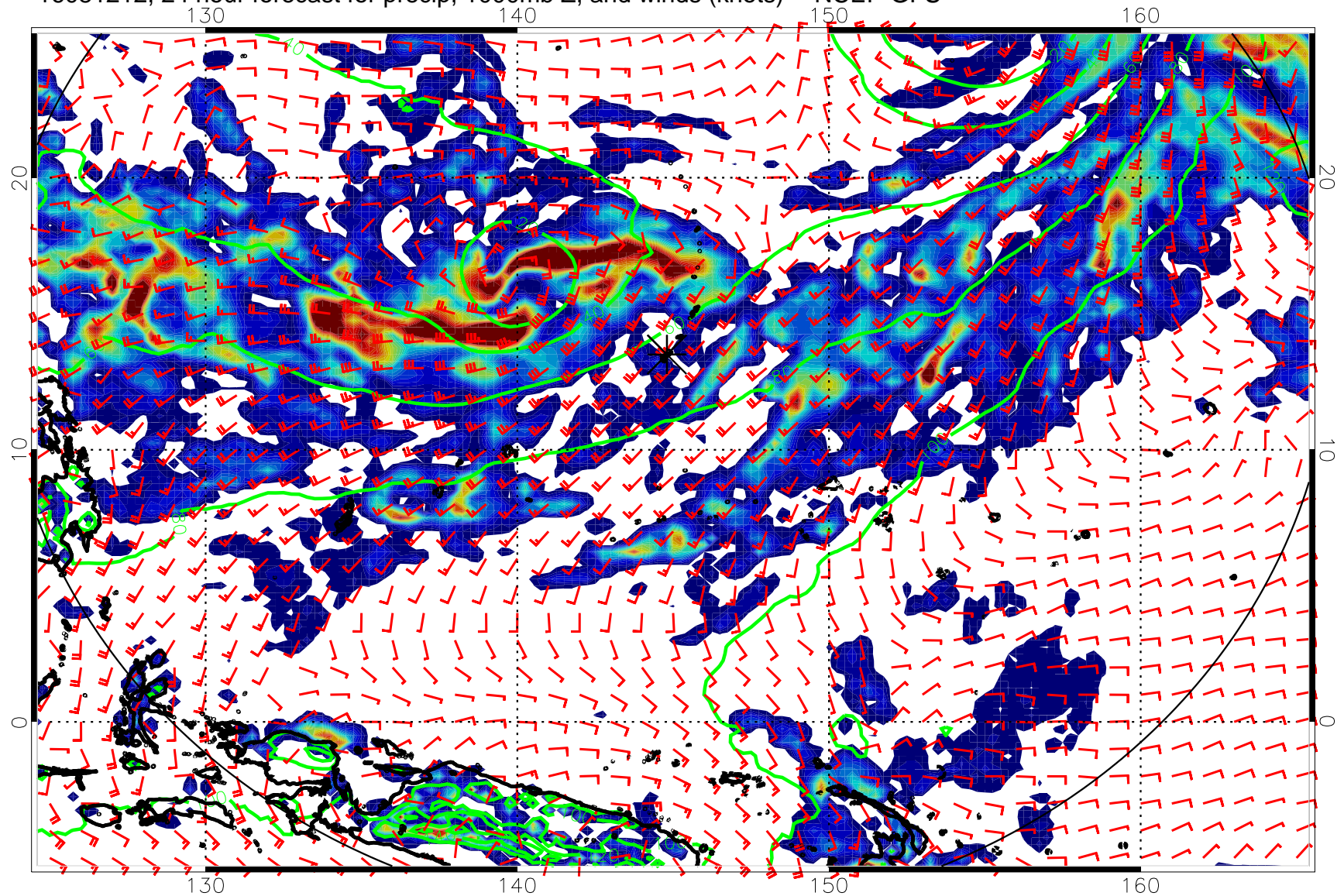
16081212, 24 hour forecast for precip, 1000mb Z, and winds (knots) -- NCEP GFS
