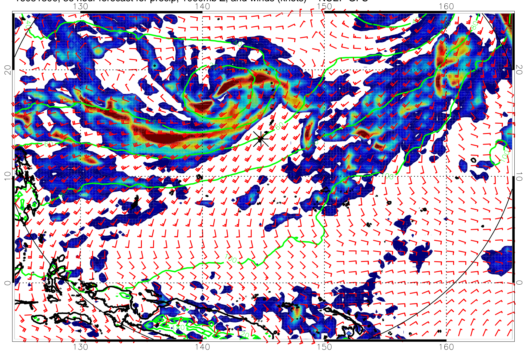
16081300, 36 hour forecast for precip, 1000mb Z, and winds (knots) -- NCEP GFS
