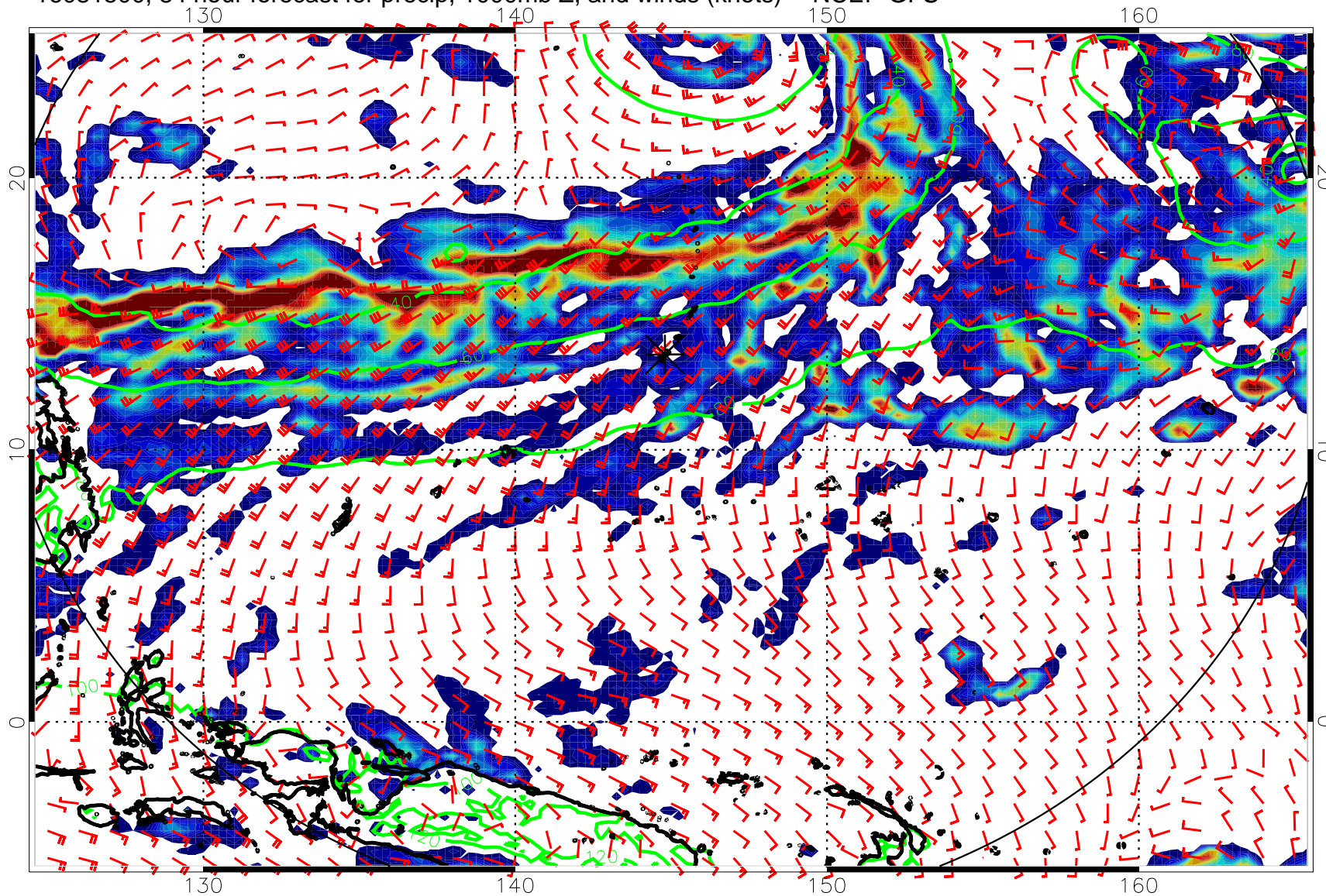
16081500, 84 hour forecast for precip, 1000mb Z, and winds (knots) -- NCEP GFS
