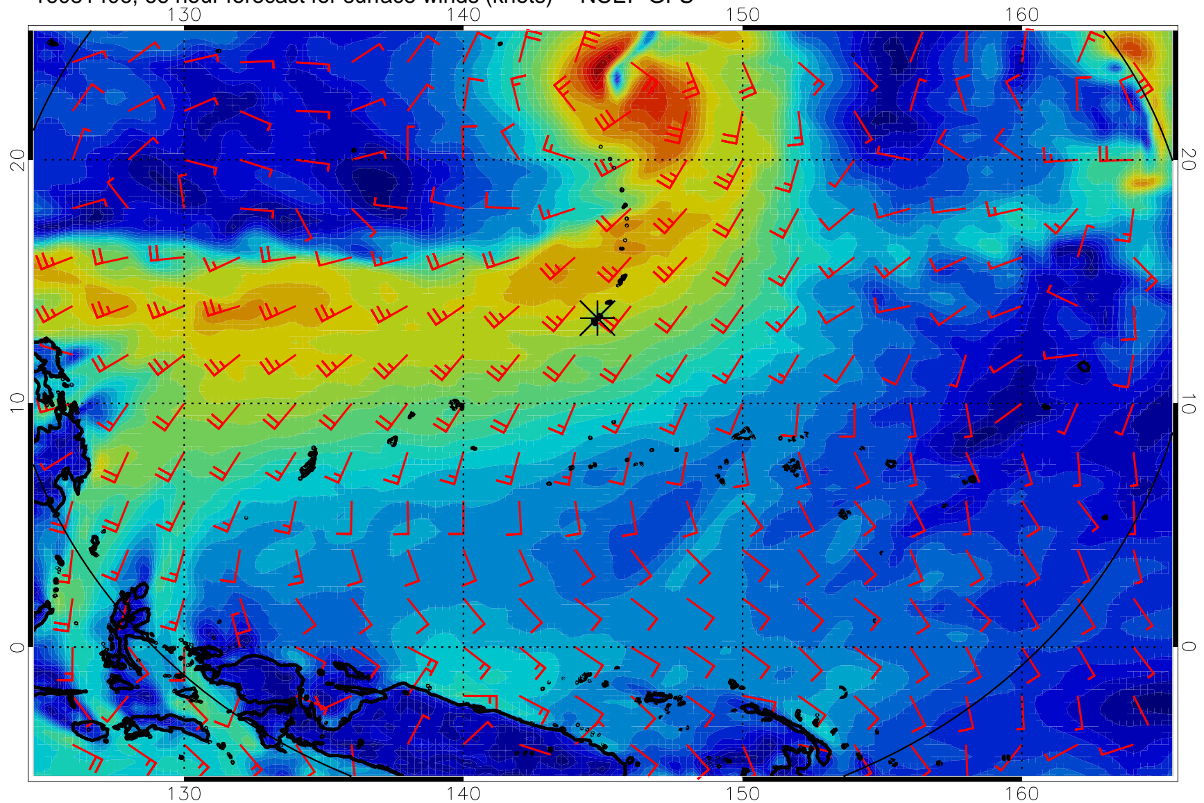
16081406, 66 hour forecast for surface winds (knots) -- NCEP GFS
