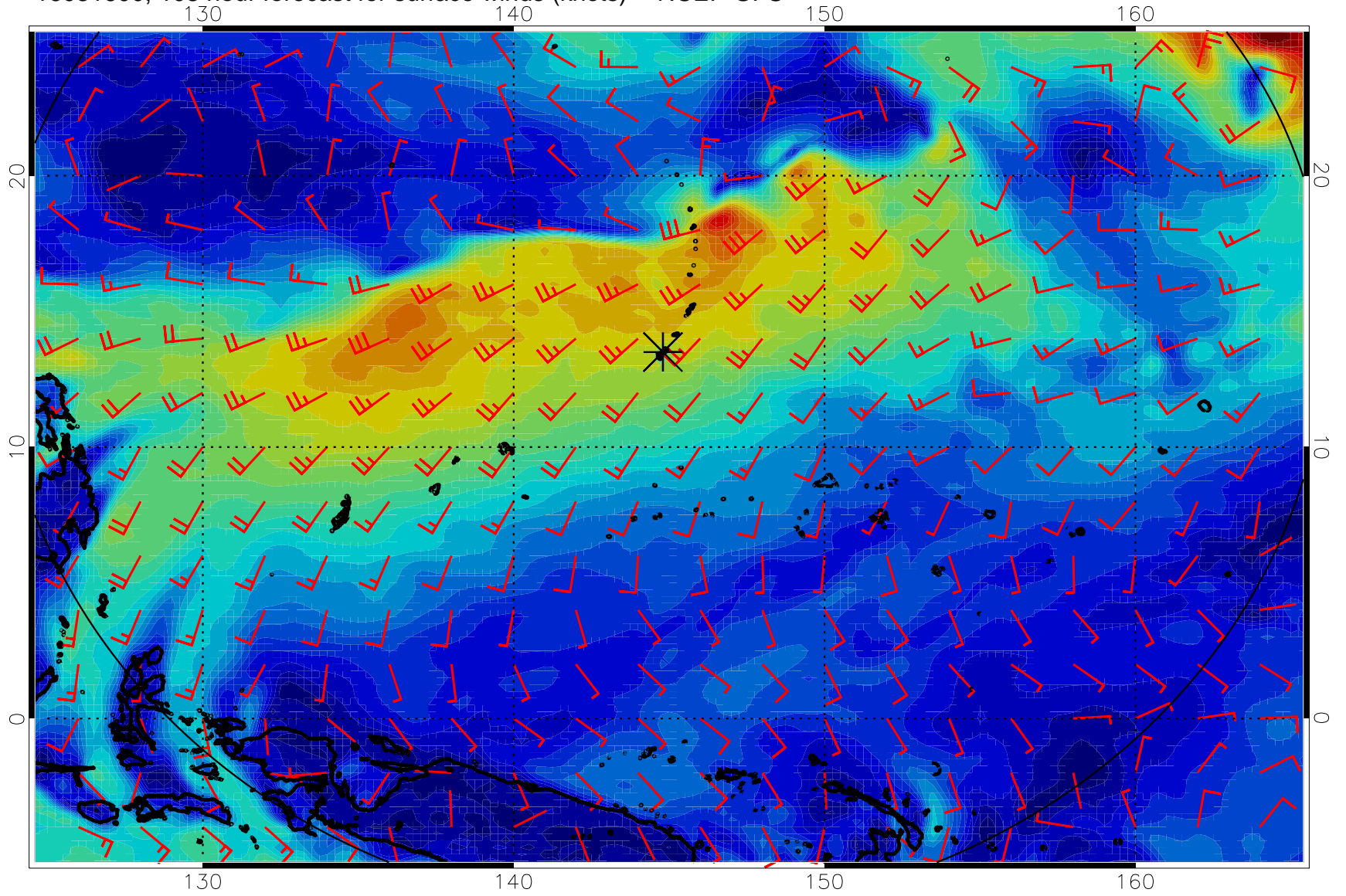
16081600, 108 hour forecast for surface winds (knots) -- NCEP GFS
