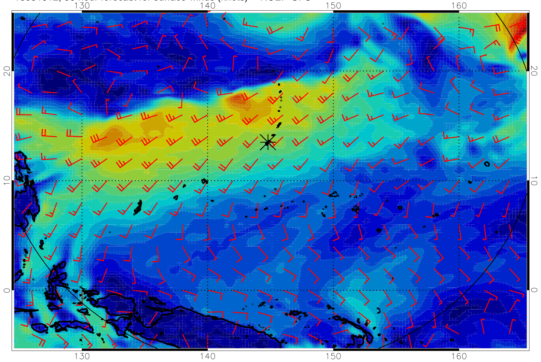
16081512, 96 hour forecast for surface winds (knots) -- NCEP GFS
