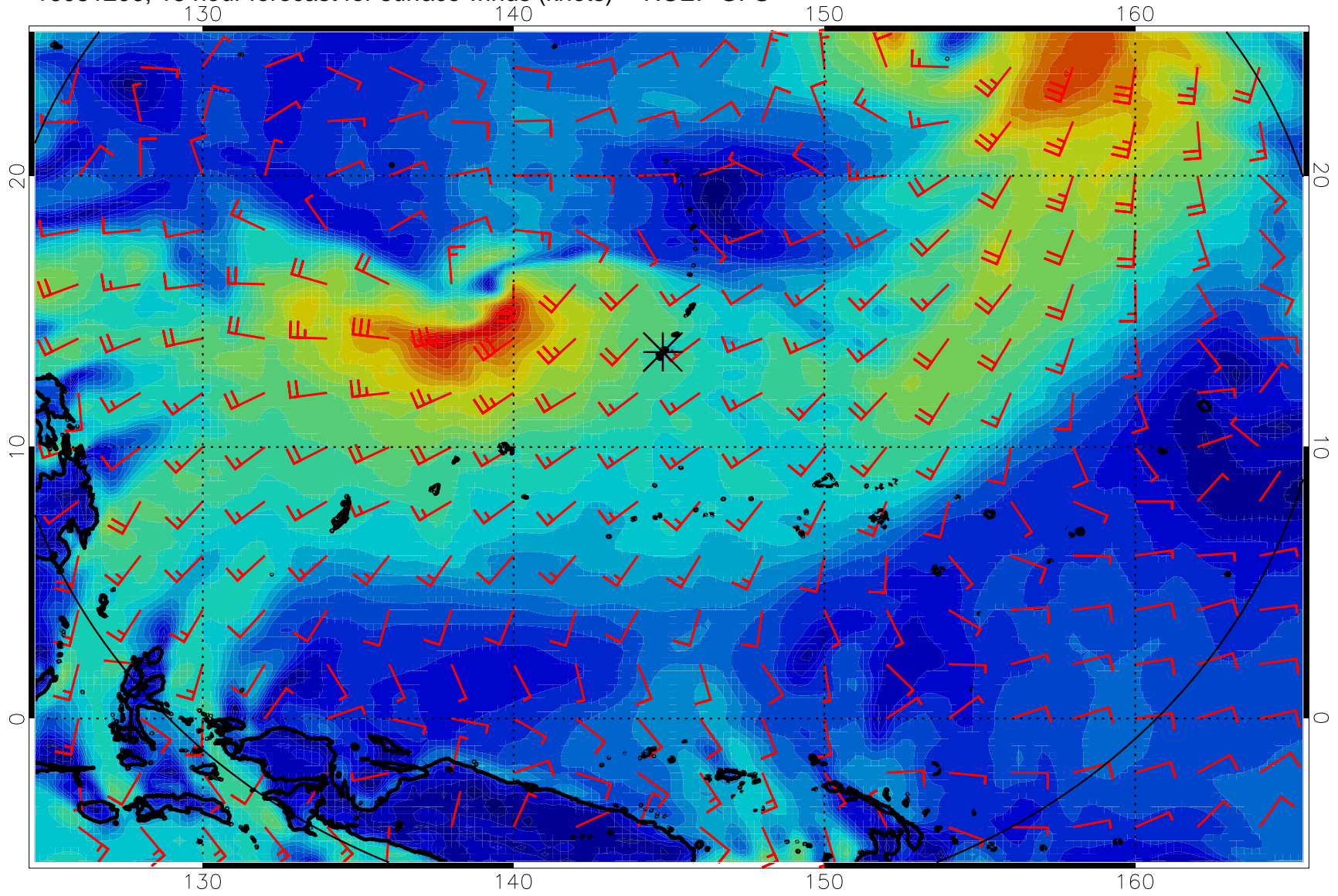
16081206, 18 hour forecast for surface winds (knots) -- NCEP GFS
