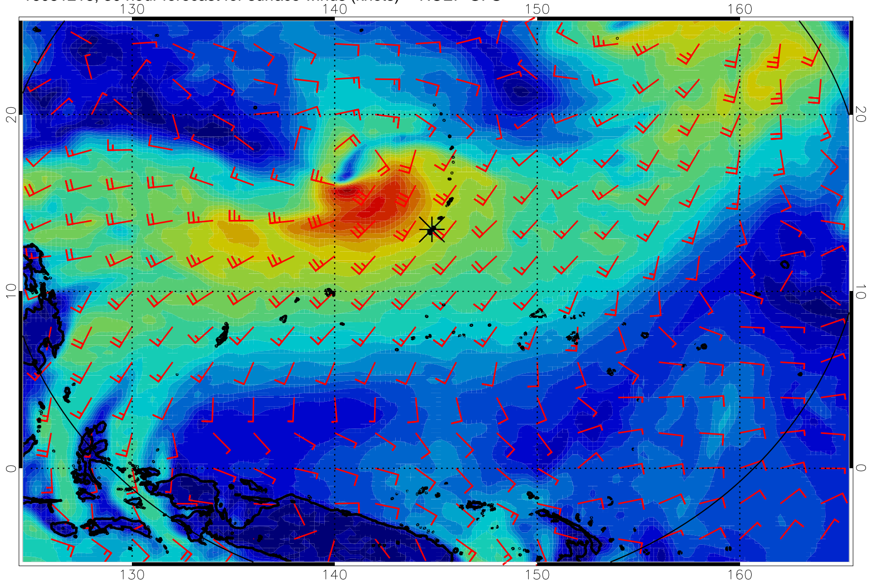
16081218, 30 hour forecast for surface winds (knots) -- NCEP GFS
