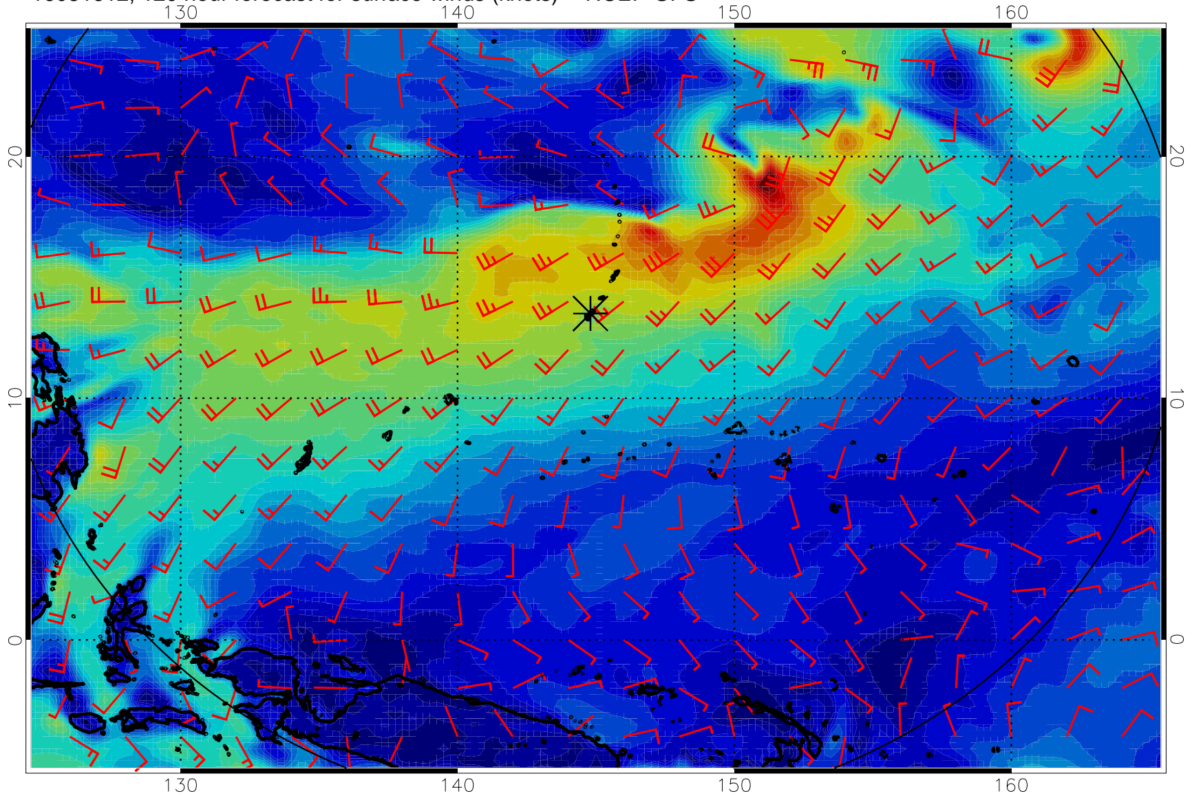
16081612, 120 hour forecast for surface winds (knots) -- NCEP GFS
