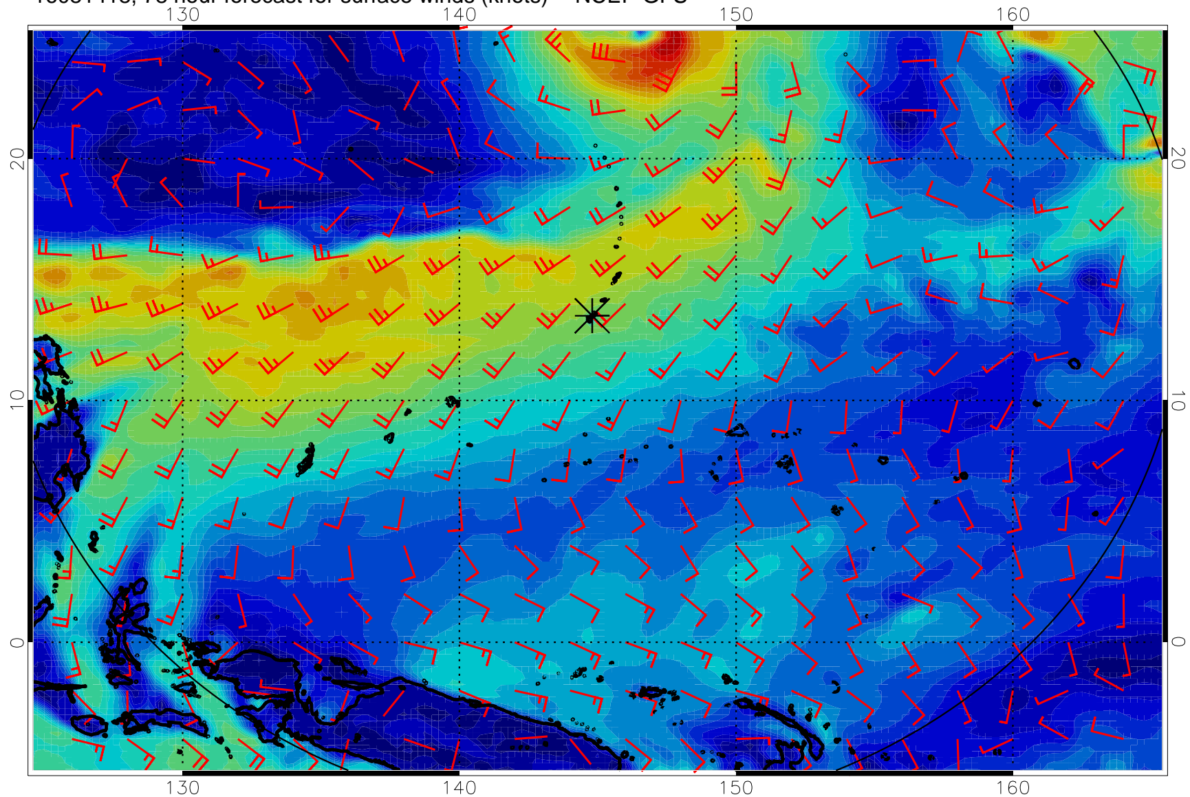
16081418, 78 hour forecast for surface winds (knots) -- NCEP GFS
