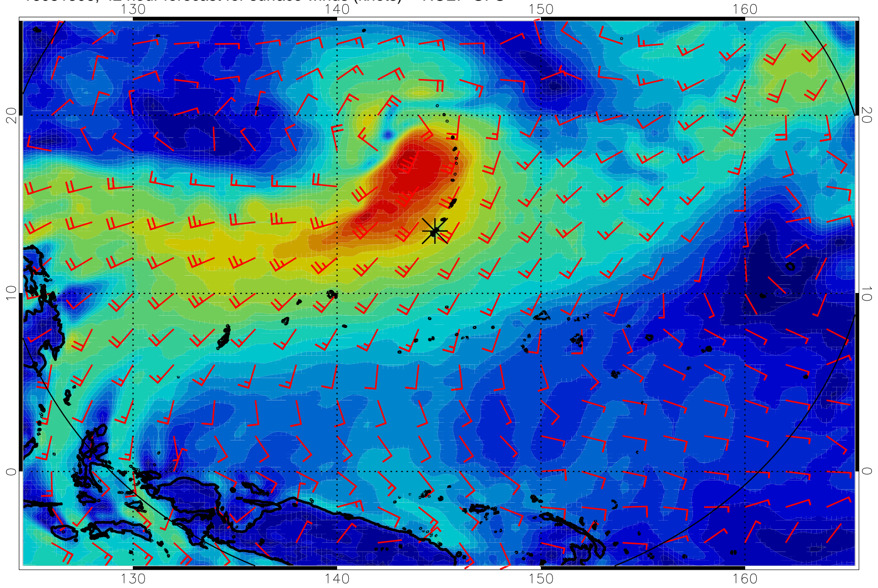
16081306, 42 hour forecast for surface winds (knots) -- NCEP GFS
