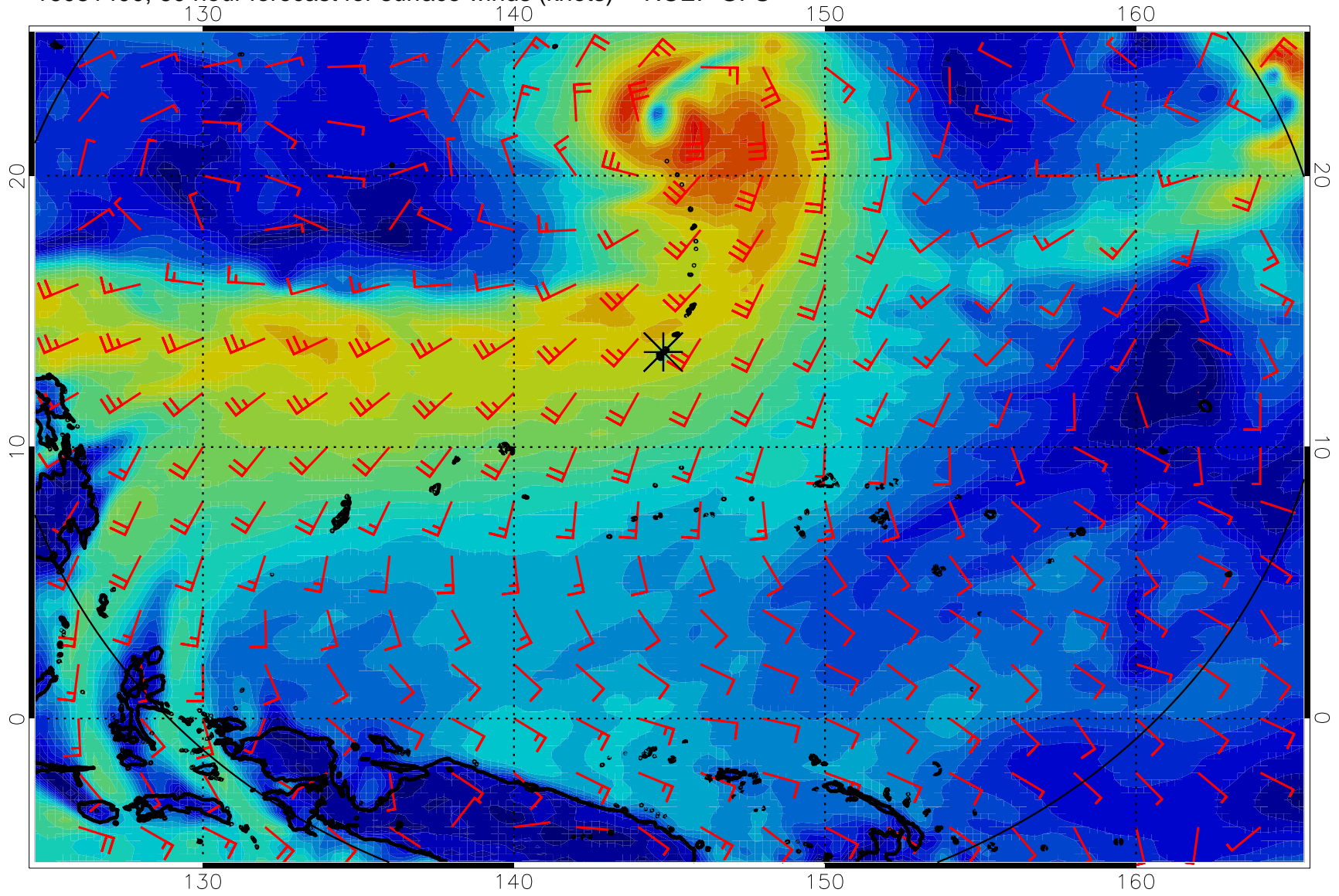
16081400, 60 hour forecast for surface winds (knots) -- NCEP GFS
