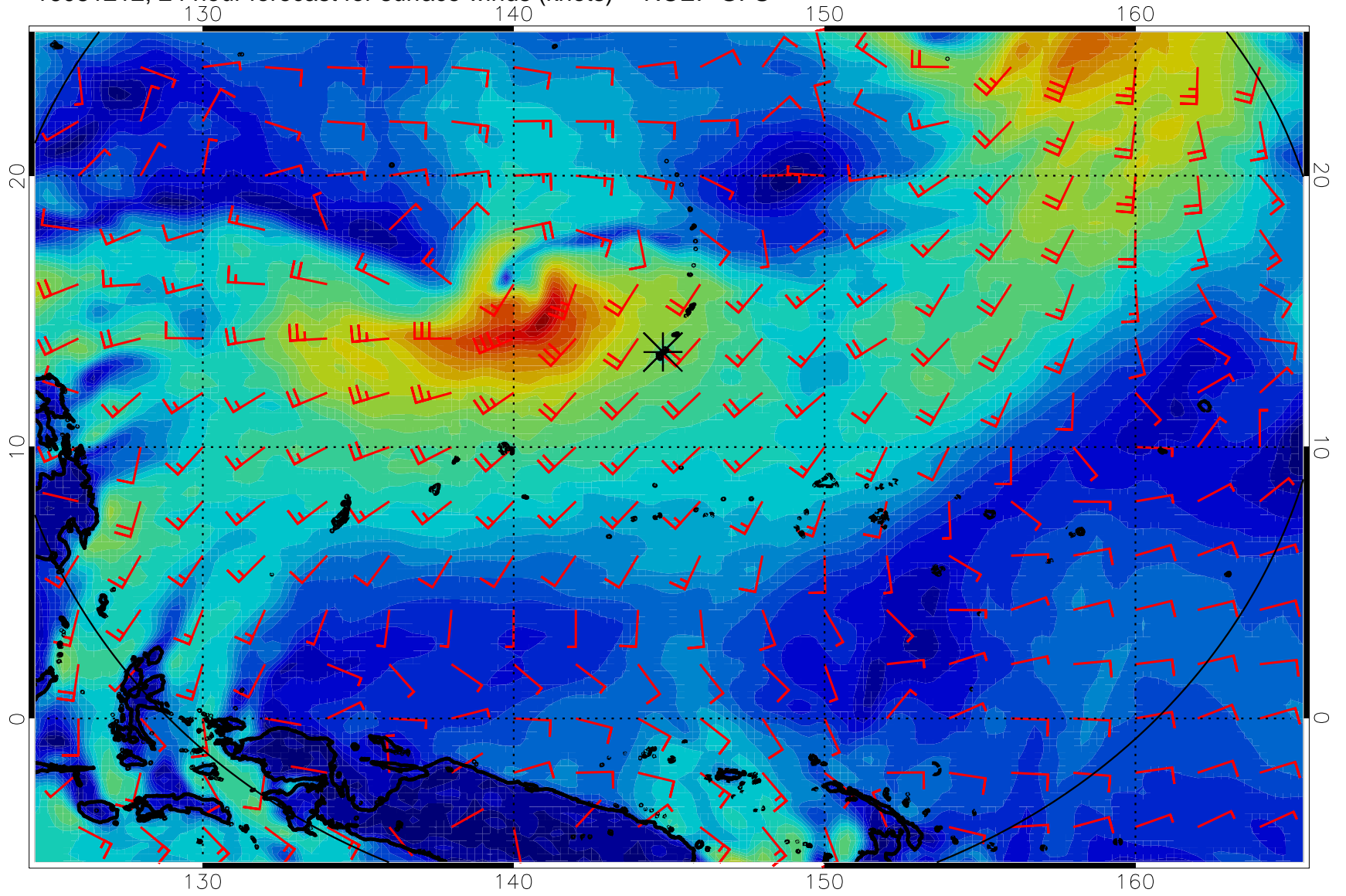
16081212, 24 hour forecast for surface winds (knots) -- NCEP GFS
