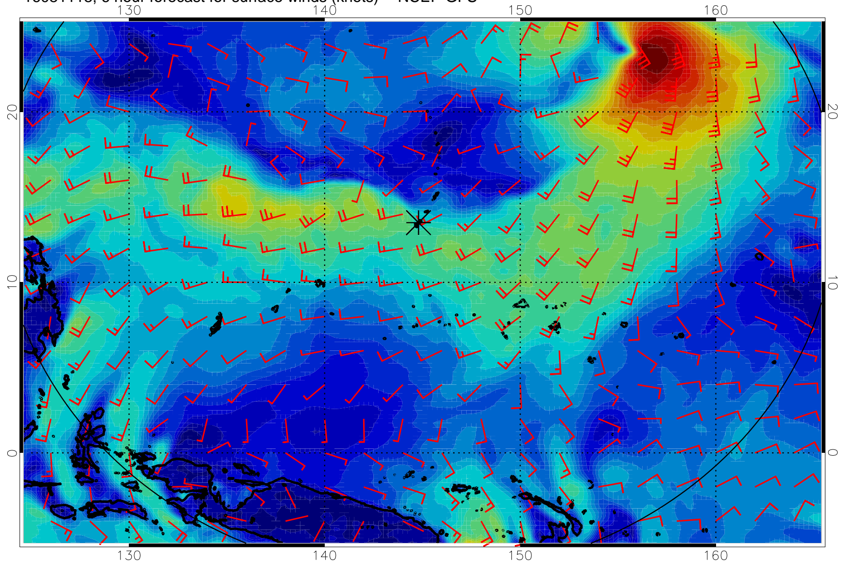
16081118, 6 hour forecast for surface winds (knots) -- NCEP GFS
