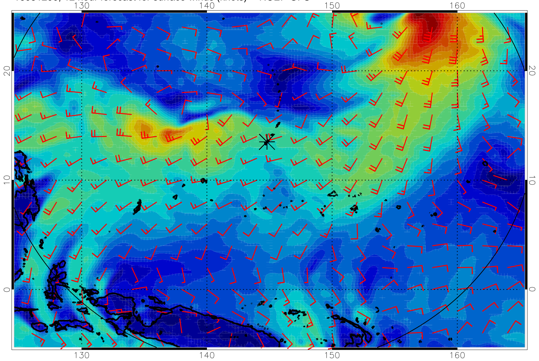
16081200, 12 hour forecast for surface winds (knots) -- NCEP GFS
