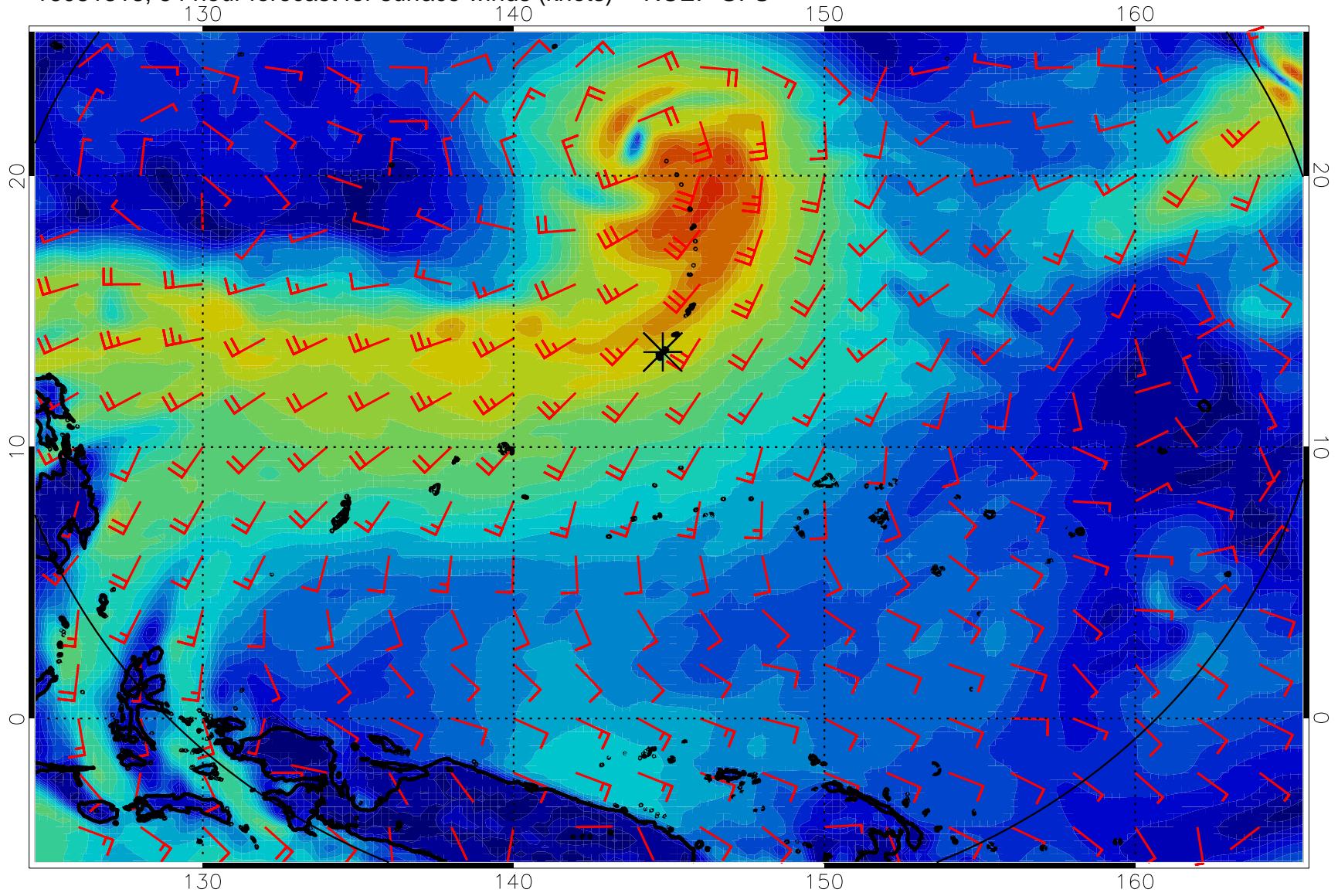
16081318, 54 hour forecast for surface winds (knots) -- NCEP GFS
