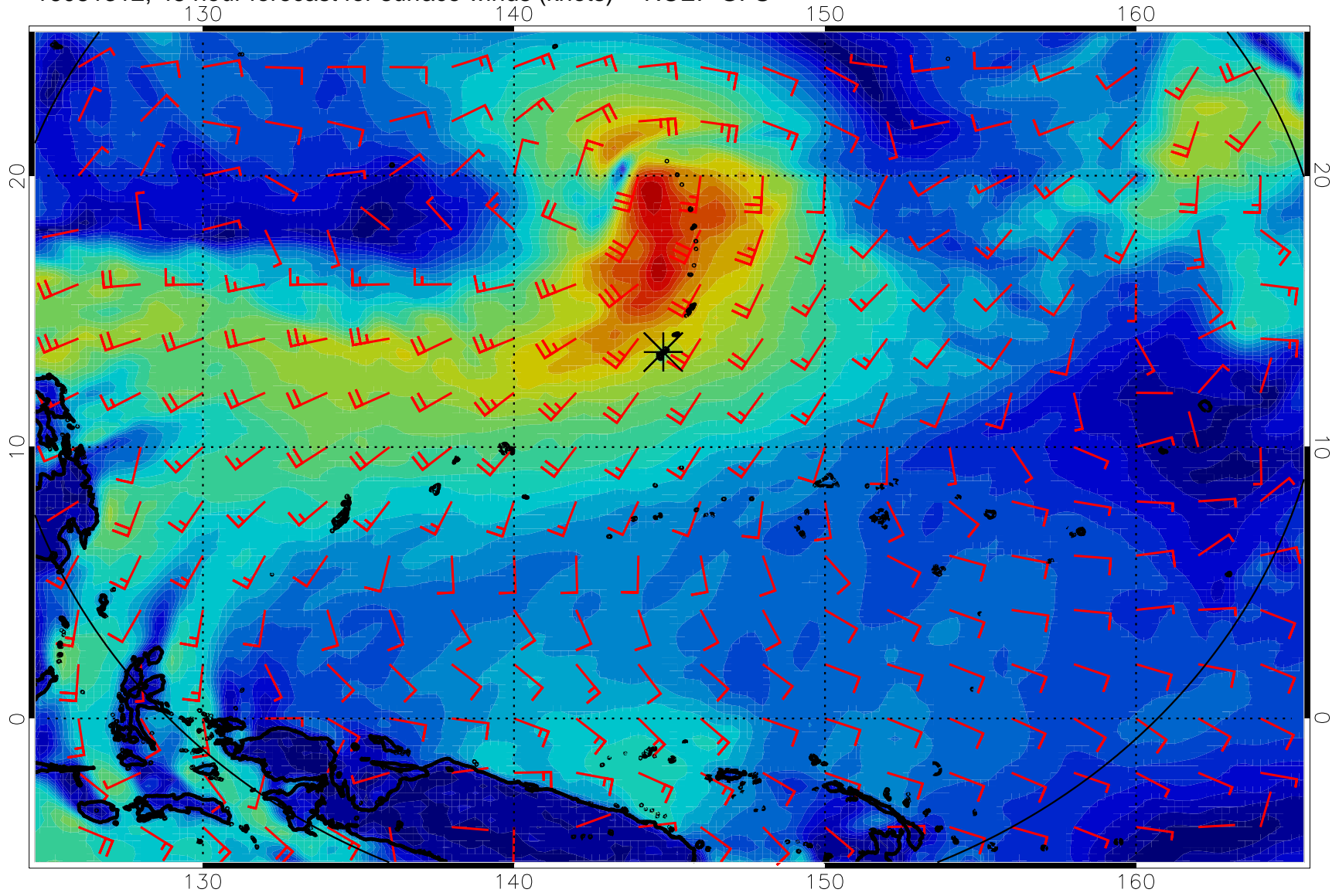
16081312, 48 hour forecast for surface winds (knots) -- NCEP GFS
