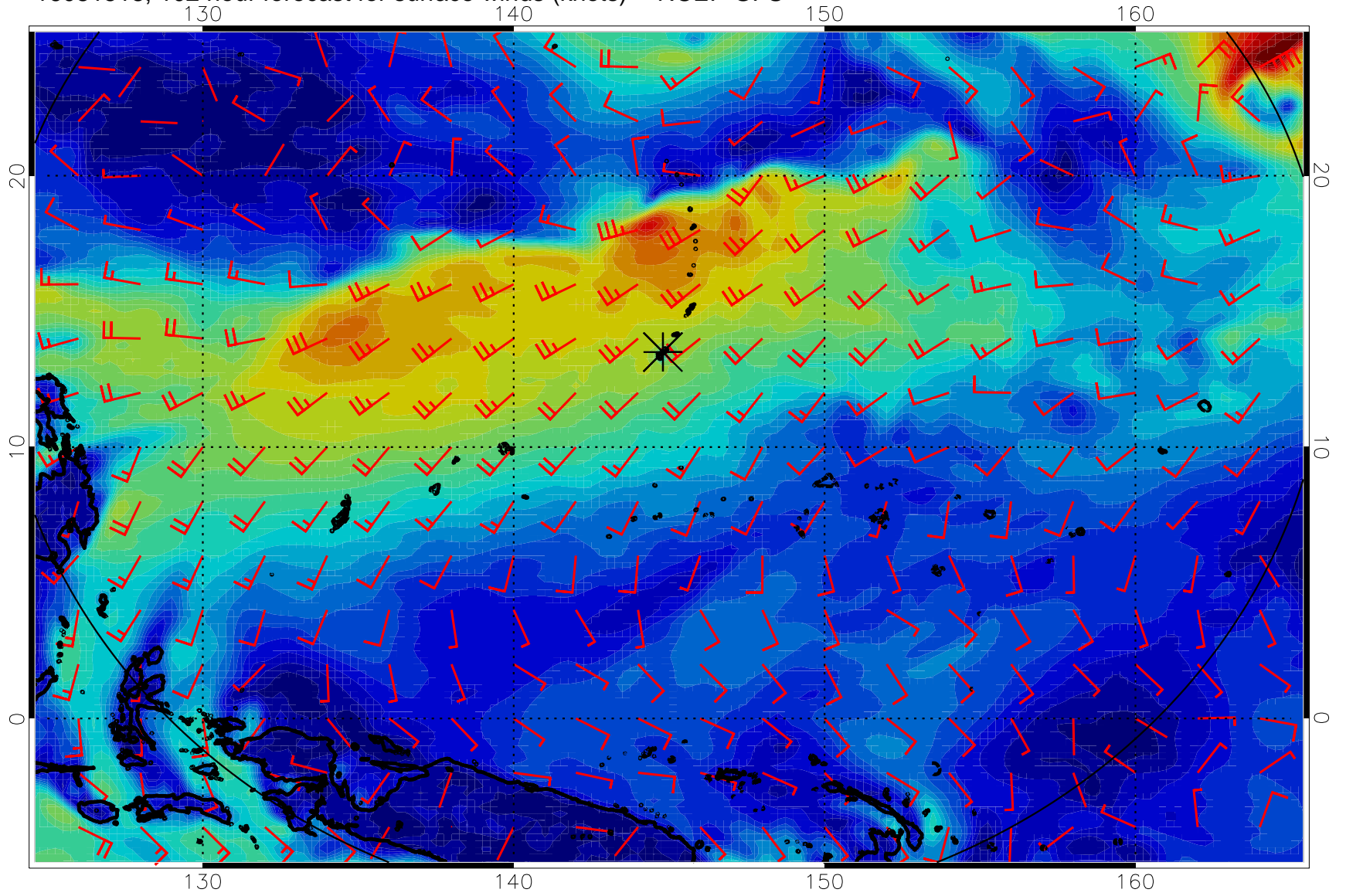
16081518, 102 hour forecast for surface winds (knots) -- NCEP GFS
