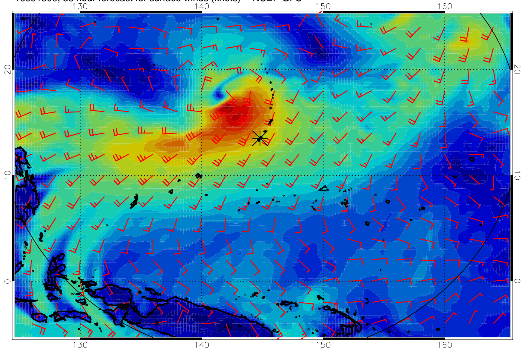
16081300, 36 hour forecast for surface winds (knots) -- NCEP GFS
