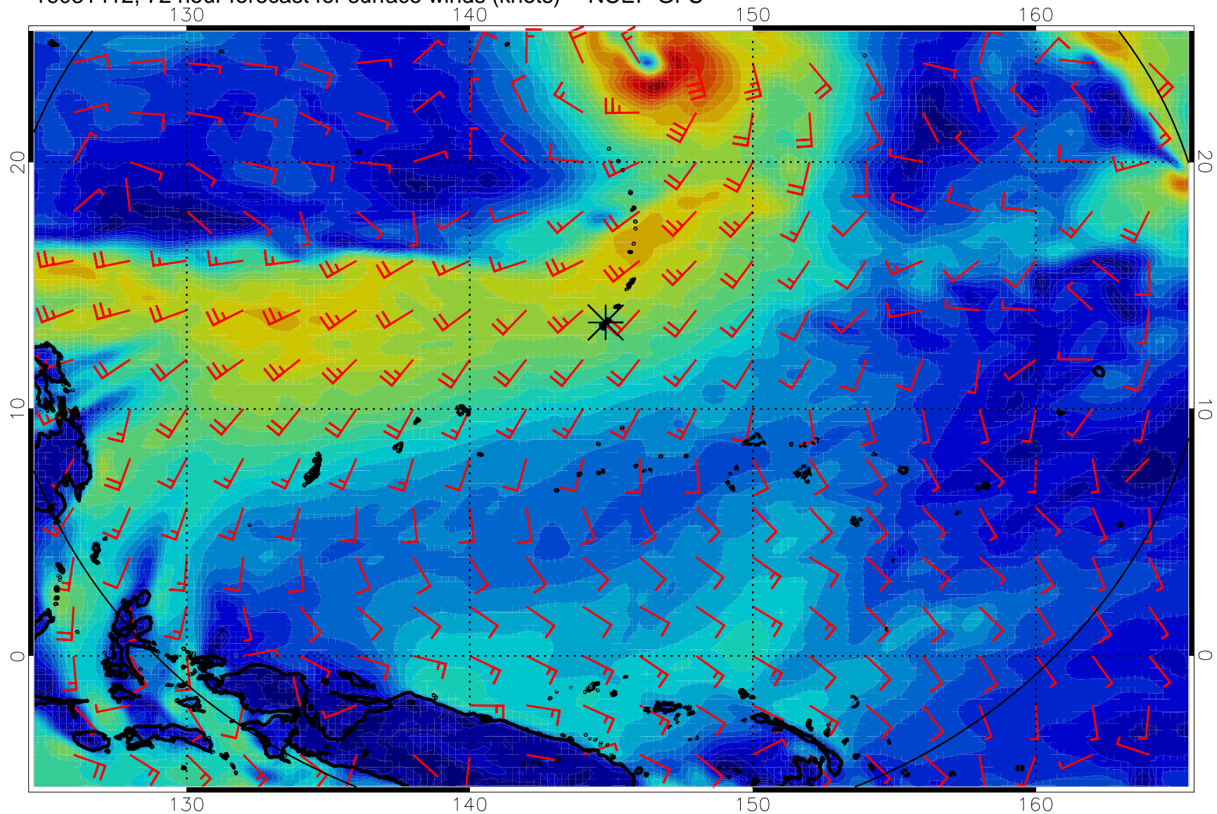
16081412, 72 hour forecast for surface winds (knots) -- NCEP GFS
