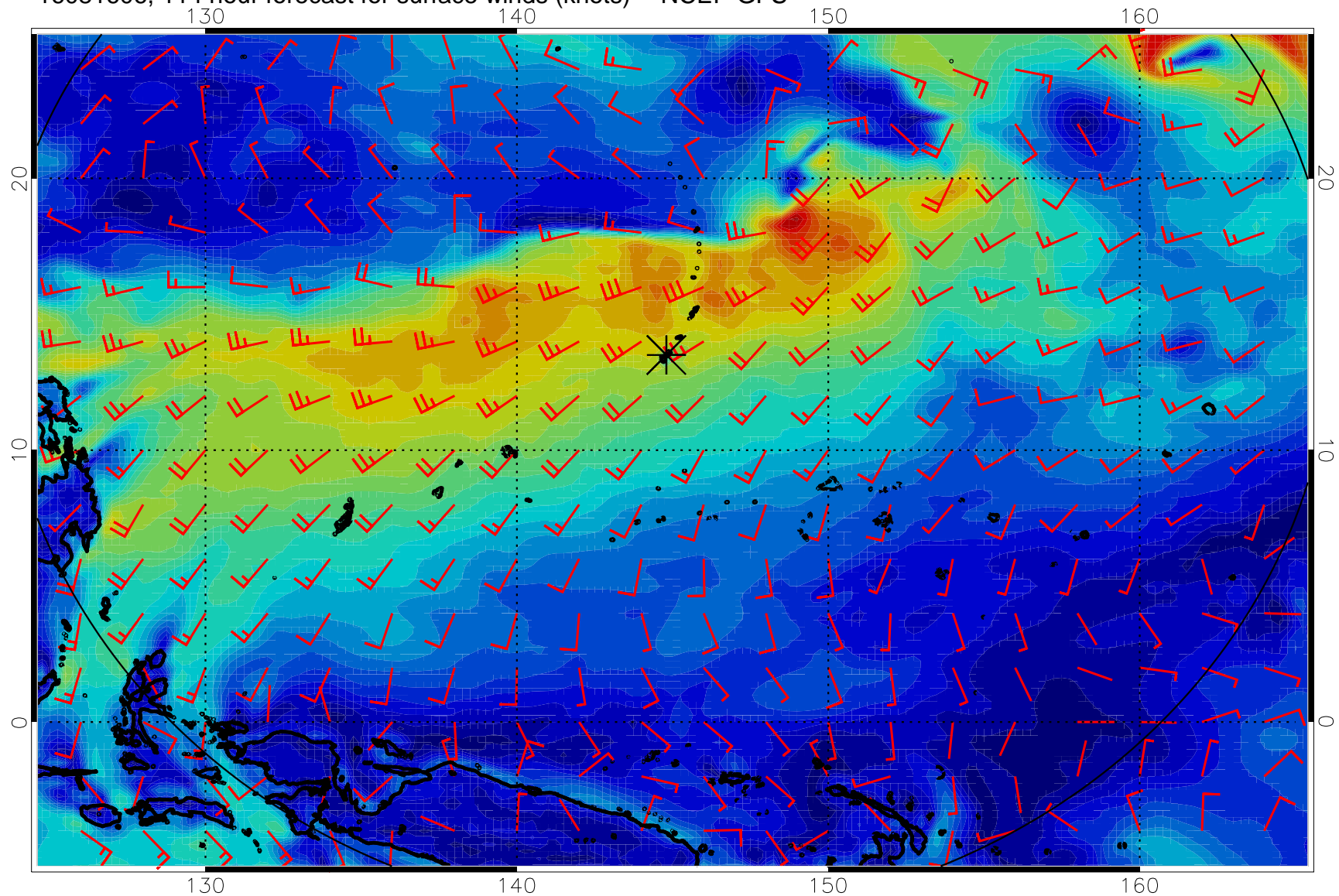
16081606, 114 hour forecast for surface winds (knots) -- NCEP GFS
