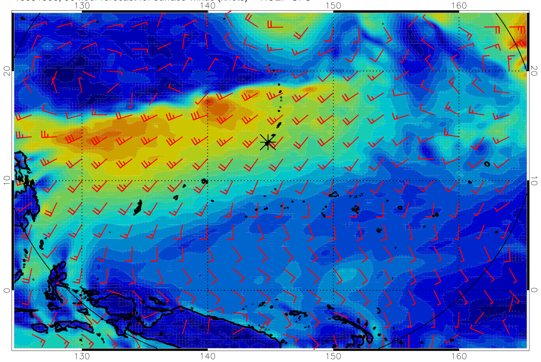
16081506, 90 hour forecast for surface winds (knots) -- NCEP GFS
