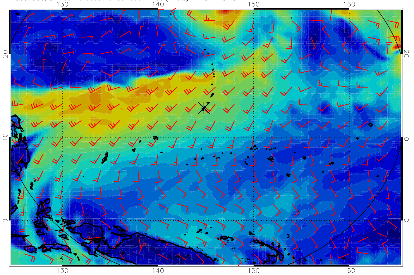
16081500, 84 hour forecast for surface winds (knots) -- NCEP GFS
