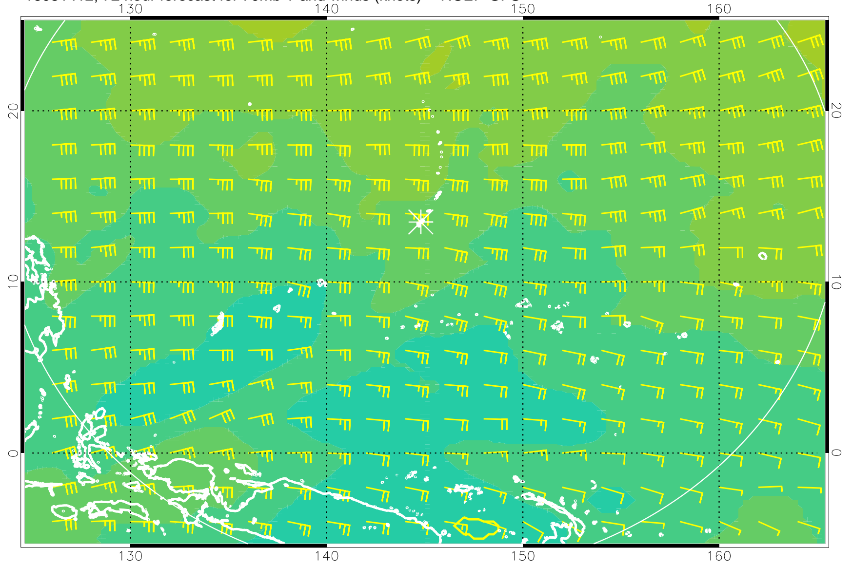
16081412, 72 hour forecast for 70mb T and winds (knots) -- NCEP GFS
