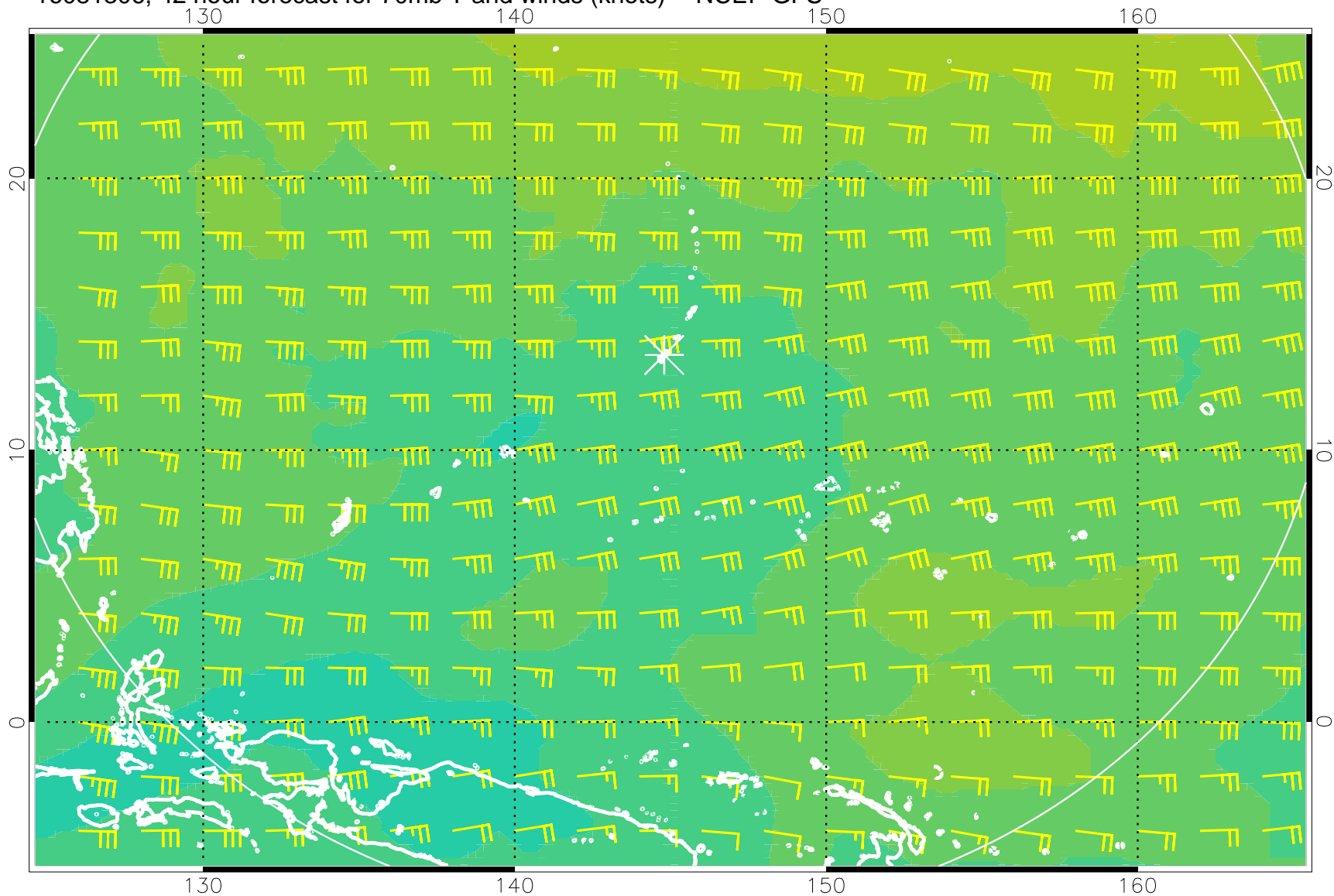
16081306, 42 hour forecast for 70mb T and winds (knots) -- NCEP GFS
