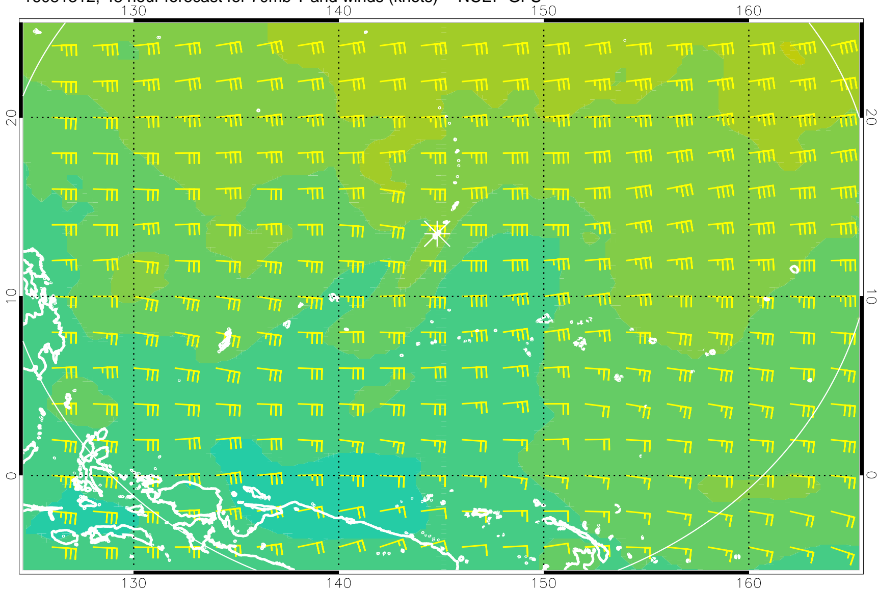
16081312, 48 hour forecast for 70mb T and winds (knots) -- NCEP GFS
