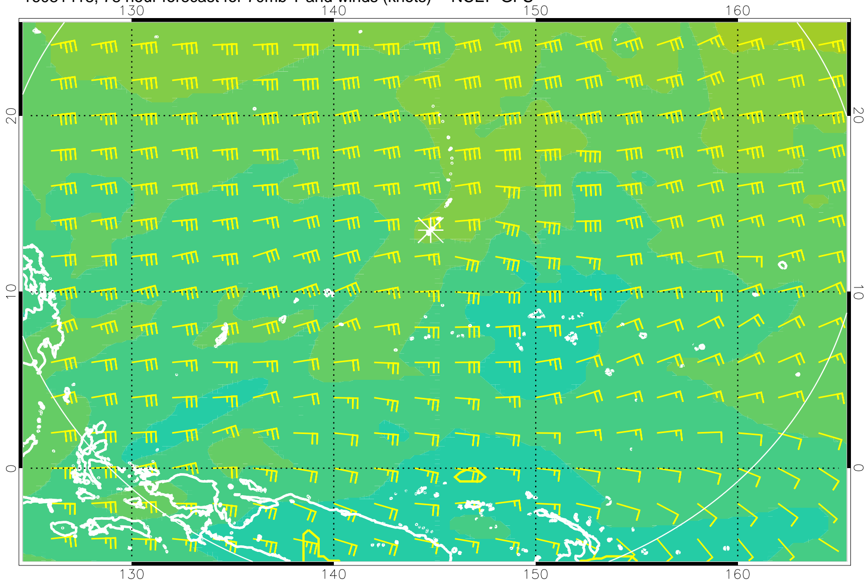
16081418, 78 hour forecast for 70mb T and winds (knots) -- NCEP GFS
