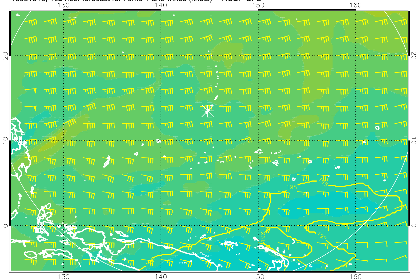
16081518, 102 hour forecast for 70mb T and winds (knots) -- NCEP GFS
