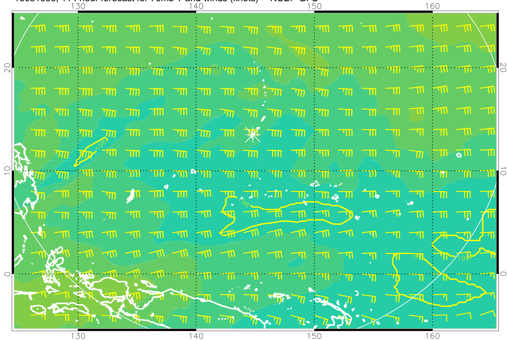
16081606, 114 hour forecast for 70mb T and winds (knots) -- NCEP GFS
