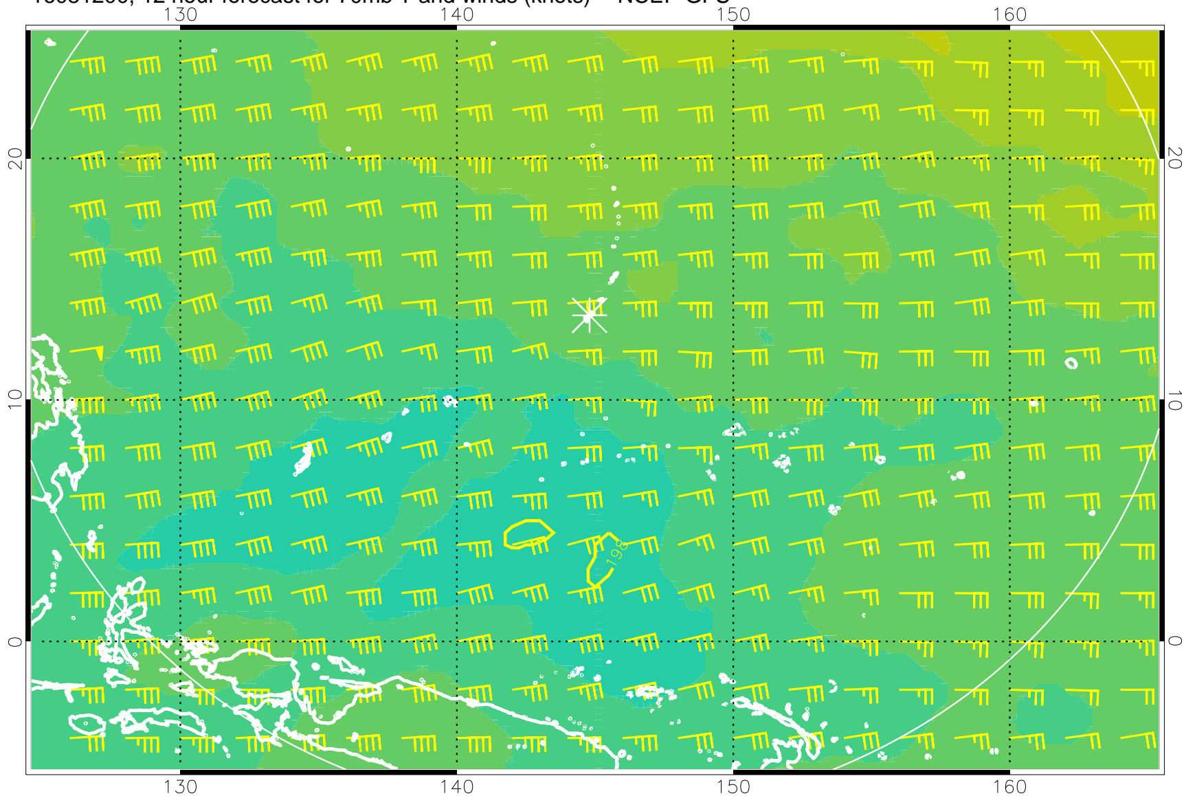
16081200, 12 hour forecast for 70mb T and winds (knots) -- NCEP GFS
