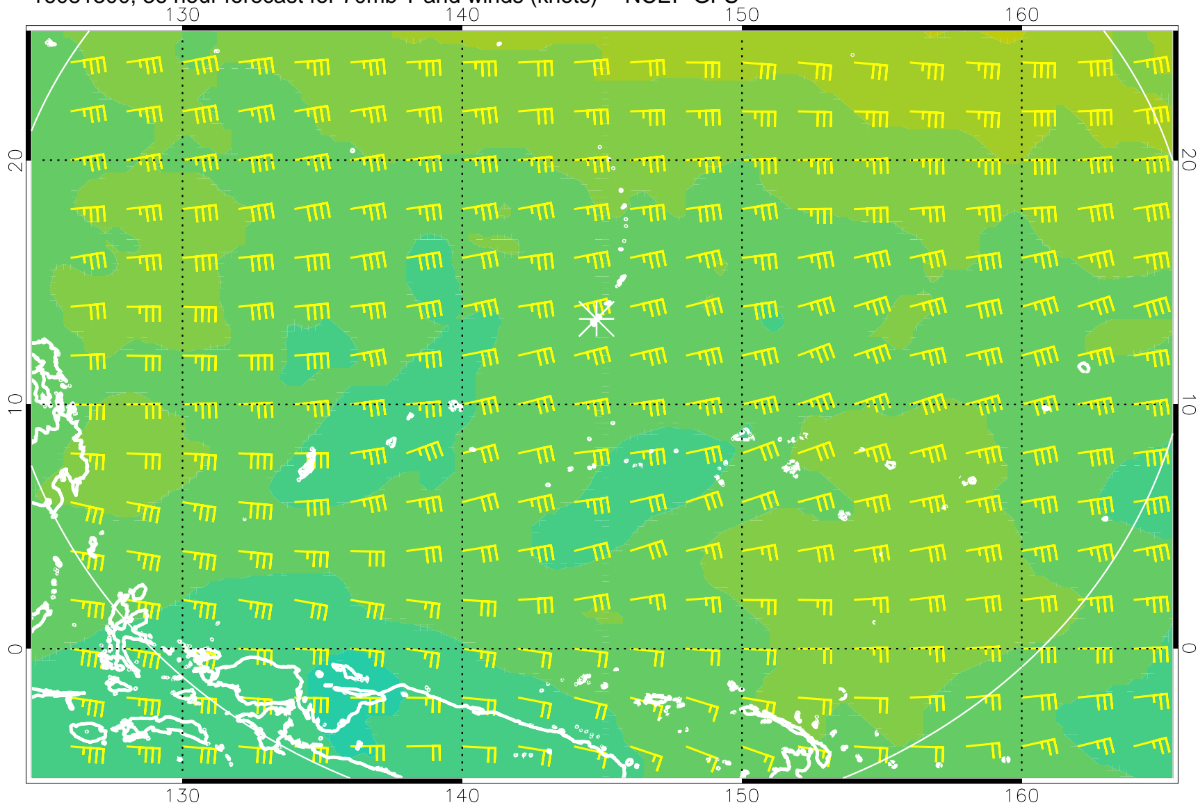
16081300, 36 hour forecast for 70mb T and winds (knots) -- NCEP GFS
