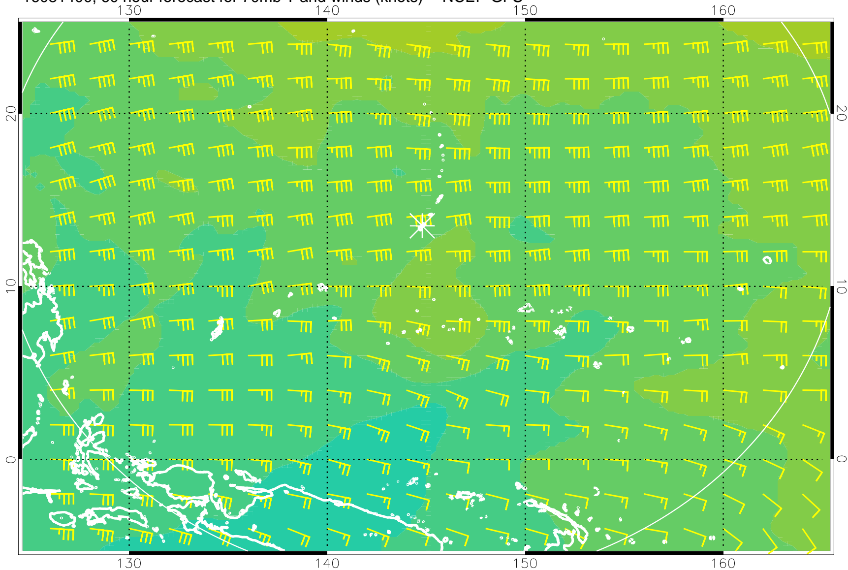
16081400, 60 hour forecast for 70mb T and winds (knots) -- NCEP GFS
