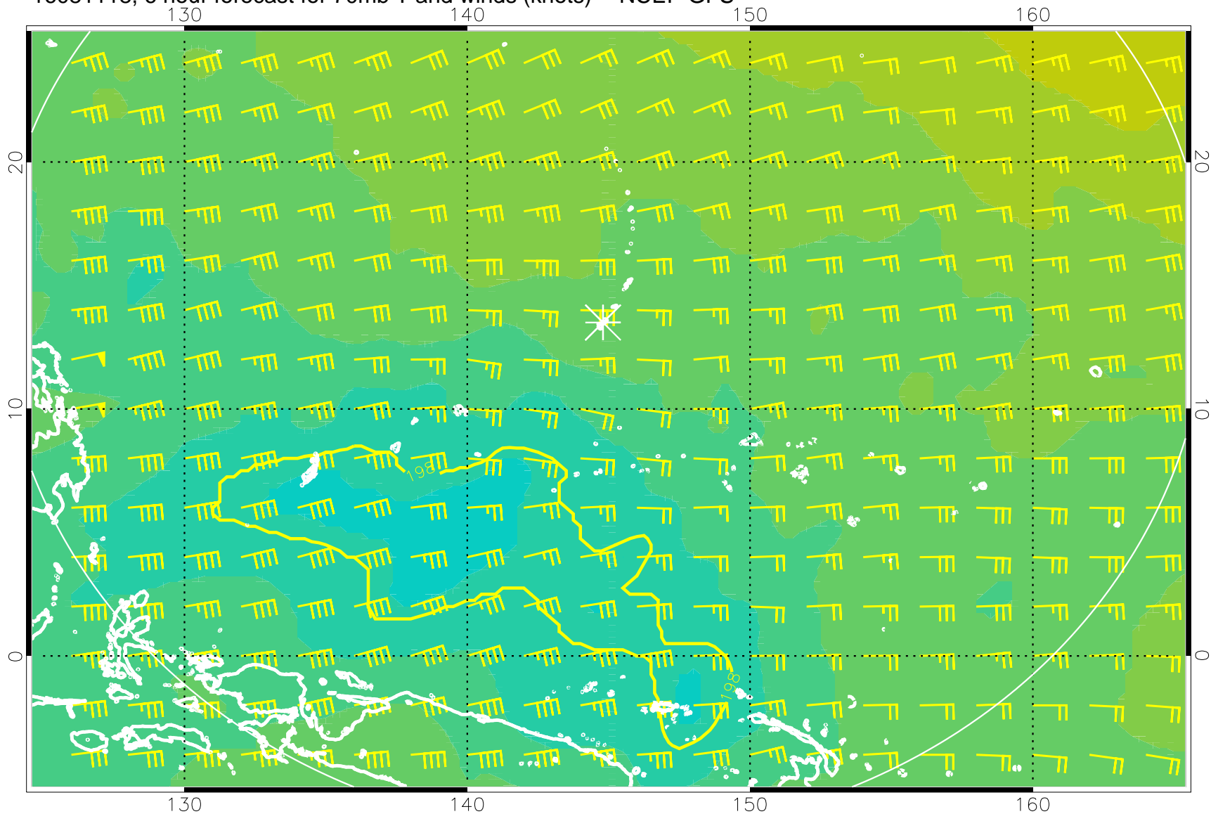
16081118, 6 hour forecast for 70mb T and winds (knots) -- NCEP GFS
