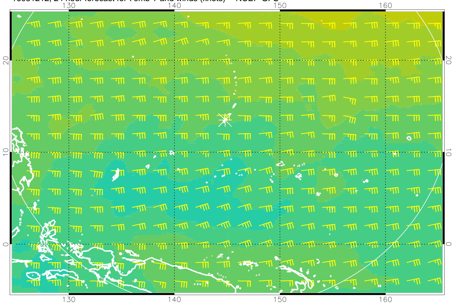
16081212, 24 hour forecast for 70mb T and winds (knots) -- NCEP GFS
