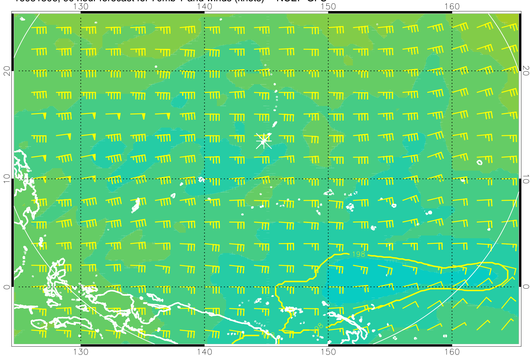
16081506, 90 hour forecast for 70mb T and winds (knots) -- NCEP GFS
