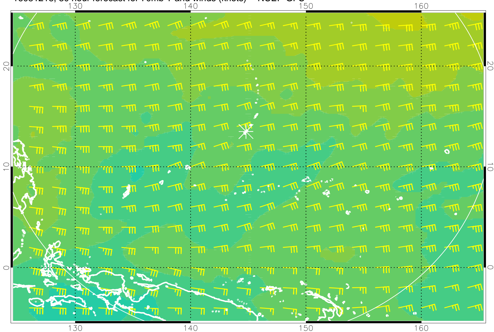
16081218, 30 hour forecast for 70mb T and winds (knots) -- NCEP GFS
