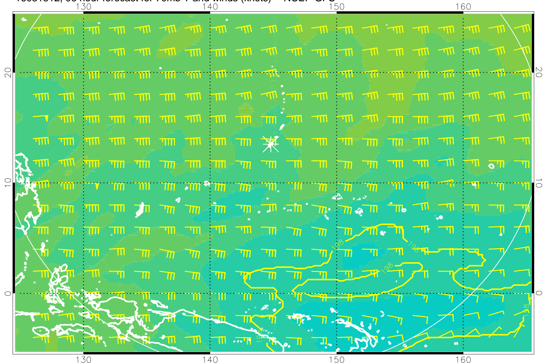
16081512, 96 hour forecast for 70mb T and winds (knots) -- NCEP GFS
