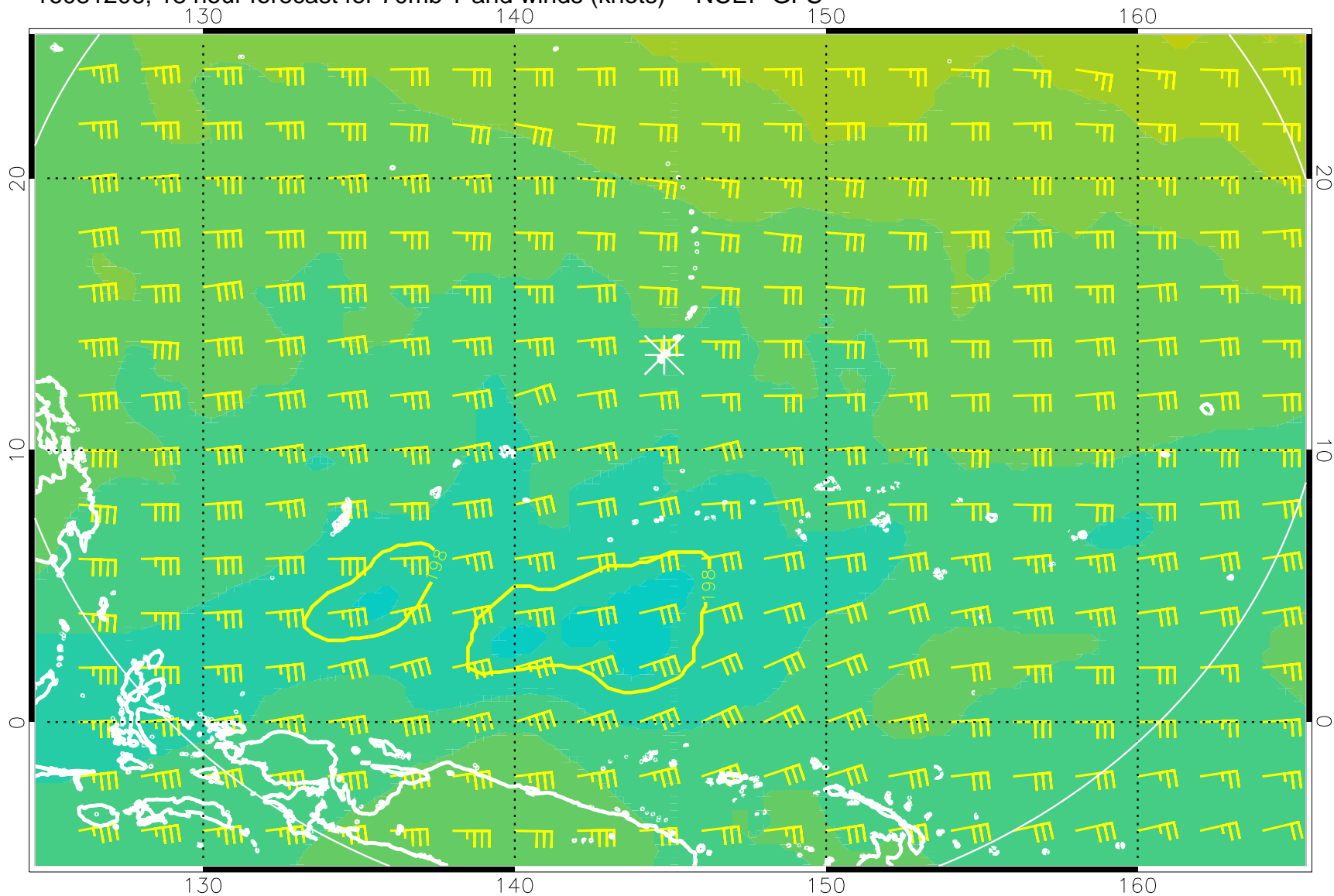
16081206, 18 hour forecast for 70mb T and winds (knots) -- NCEP GFS
