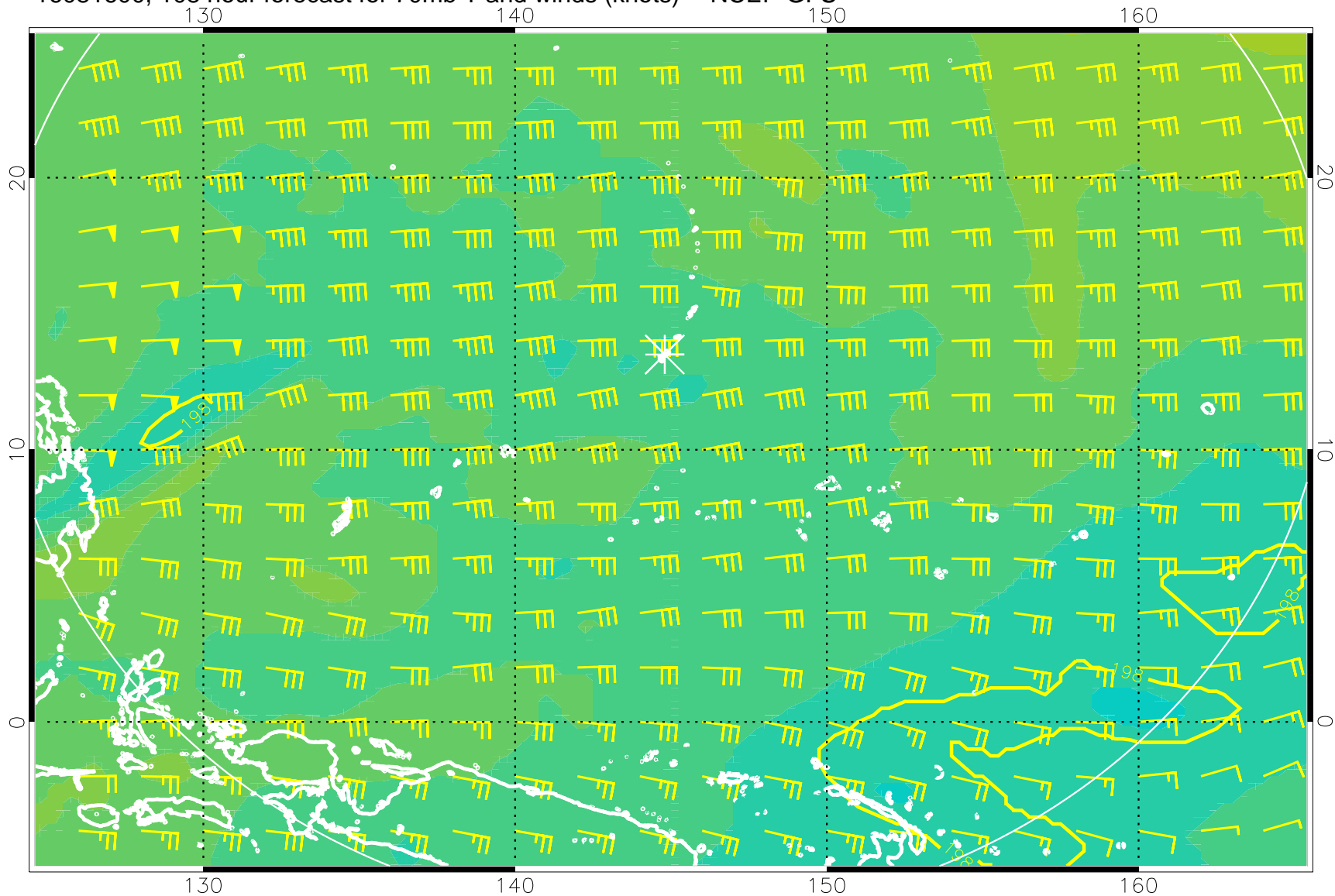
16081600, 108 hour forecast for 70mb T and winds (knots) -- NCEP GFS
