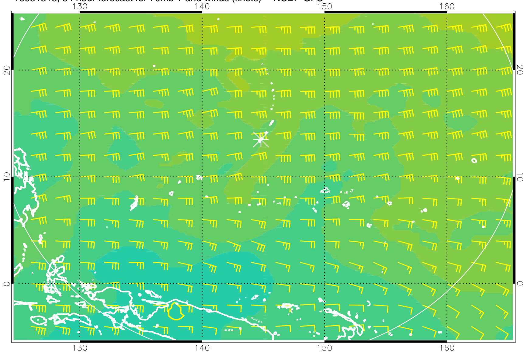
16081318, 54 hour forecast for 70mb T and winds (knots) -- NCEP GFS
