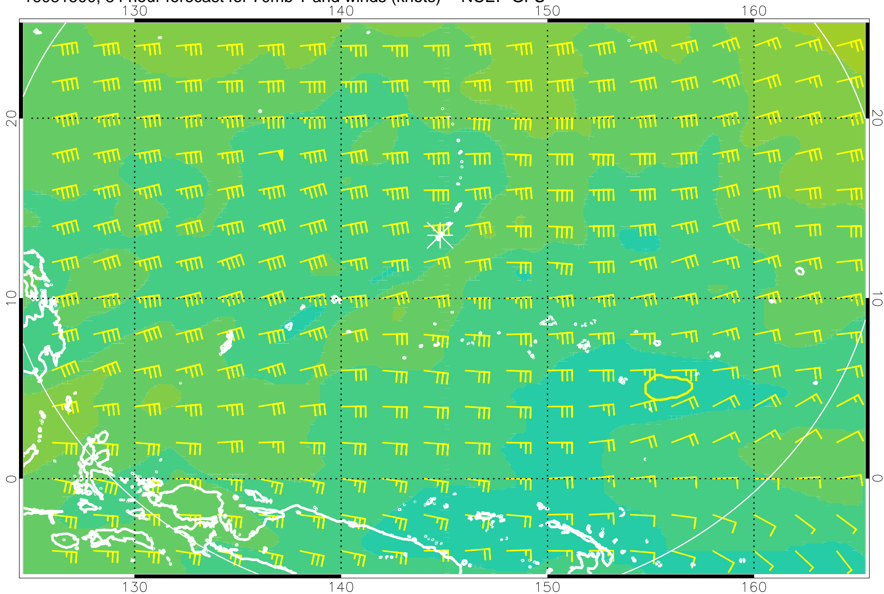
16081500, 84 hour forecast for 70mb T and winds (knots) -- NCEP GFS
