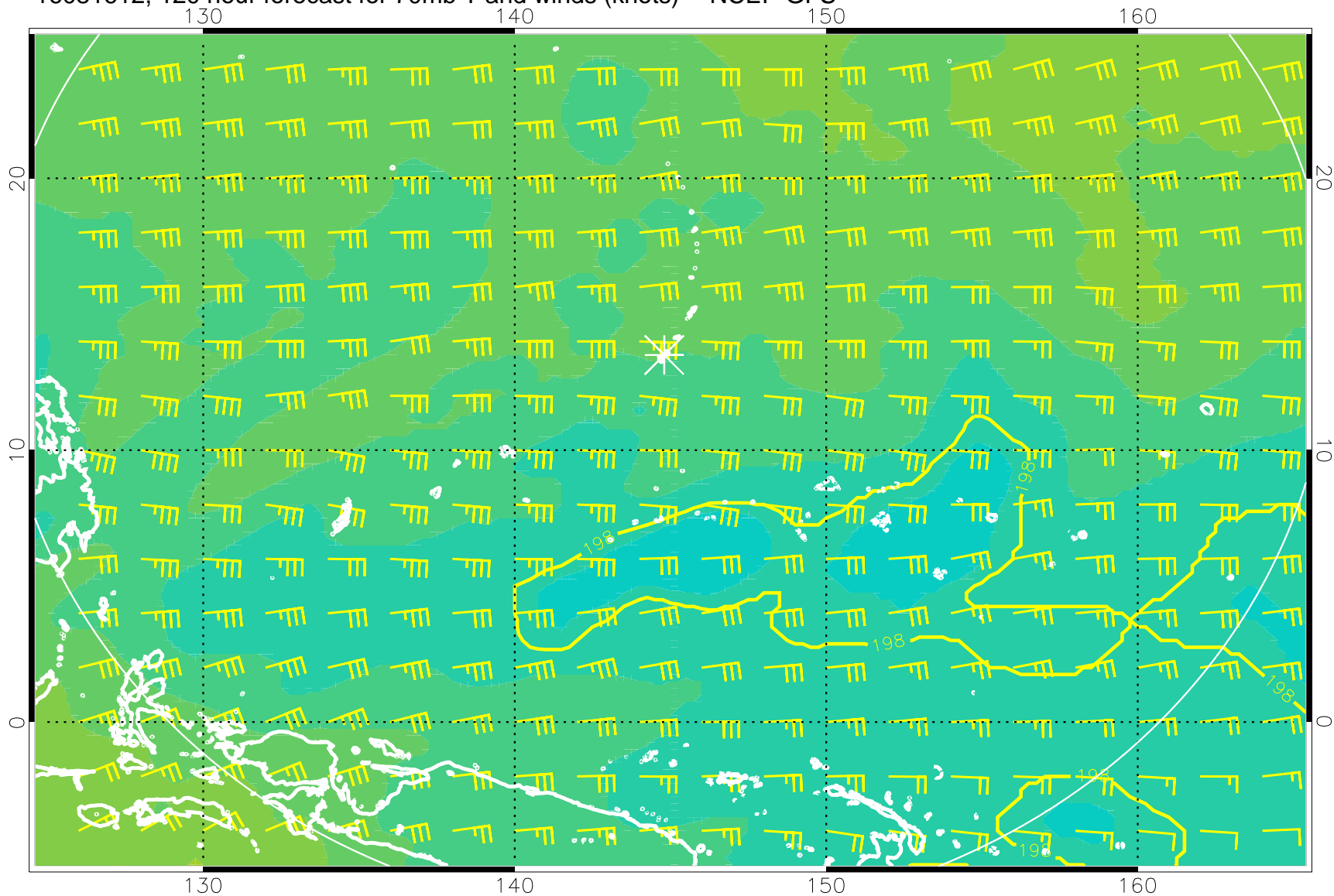
16081612, 120 hour forecast for 70mb T and winds (knots) -- NCEP GFS
