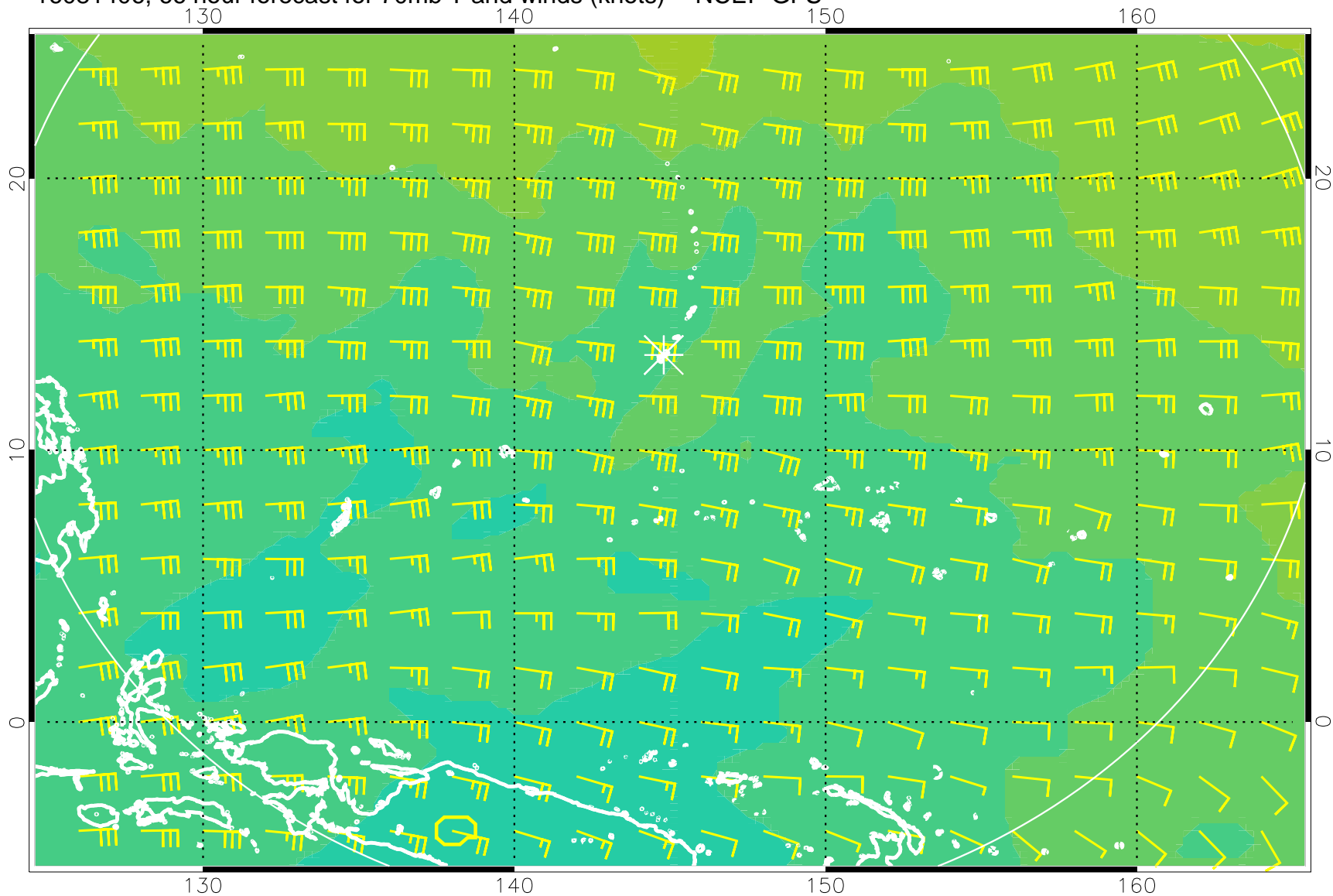
16081406, 66 hour forecast for 70mb T and winds (knots) -- NCEP GFS
