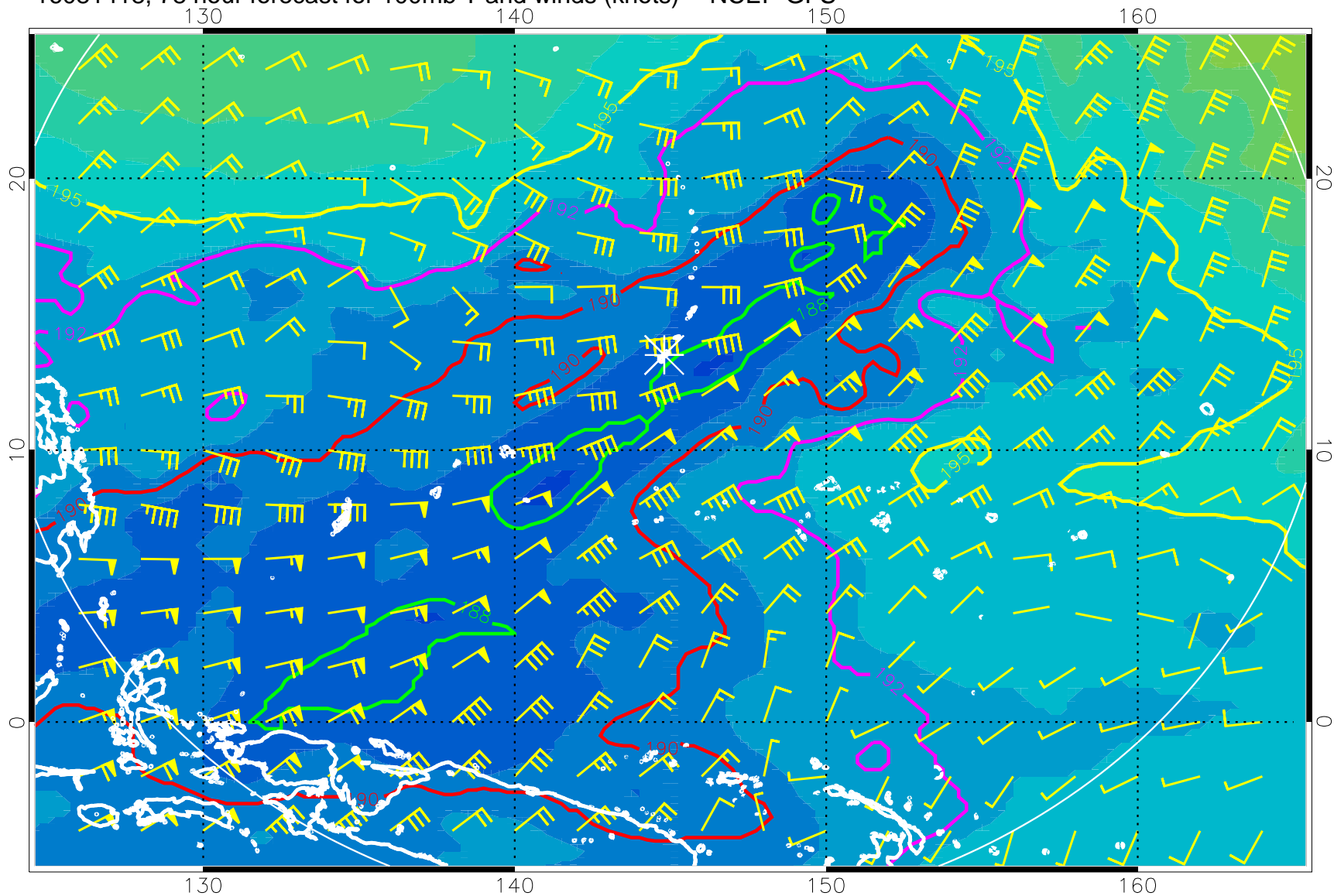
16081418, 78 hour forecast for 100mb T and winds (knots) -- NCEP GFS
