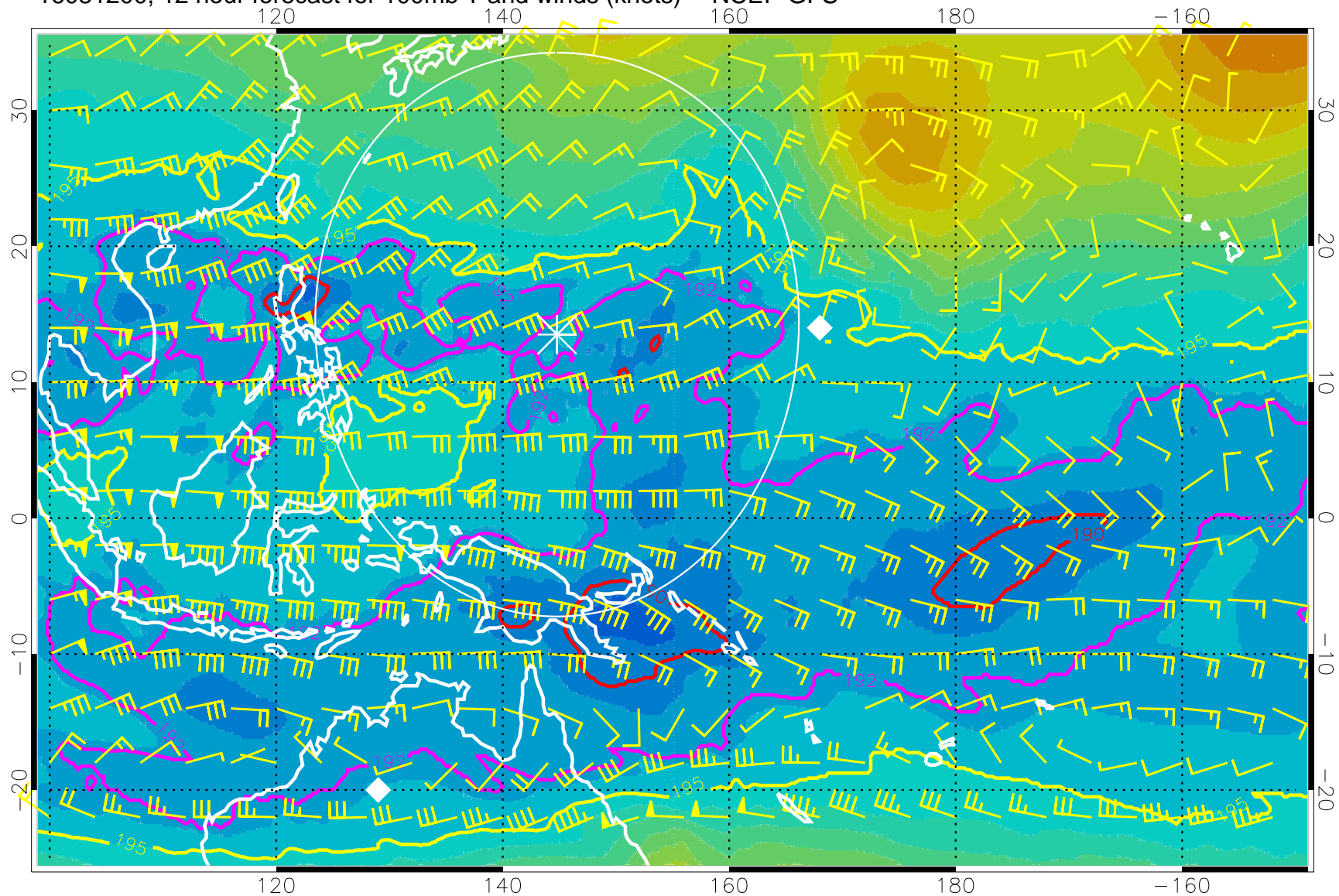
16081200, 12 hour forecast for 100mb T and winds (knots) -- NCEP GFS
