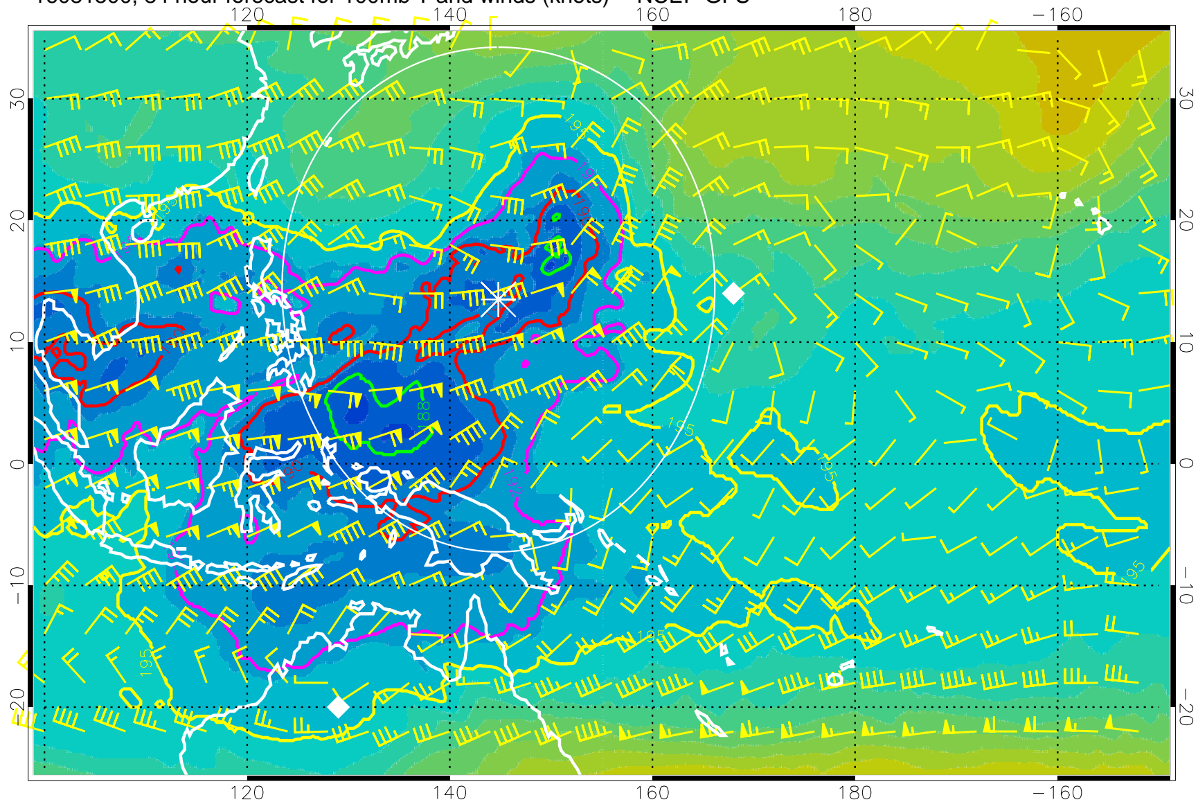
16081500, 84 hour forecast for 100mb T and winds (knots) -- NCEP GFS
