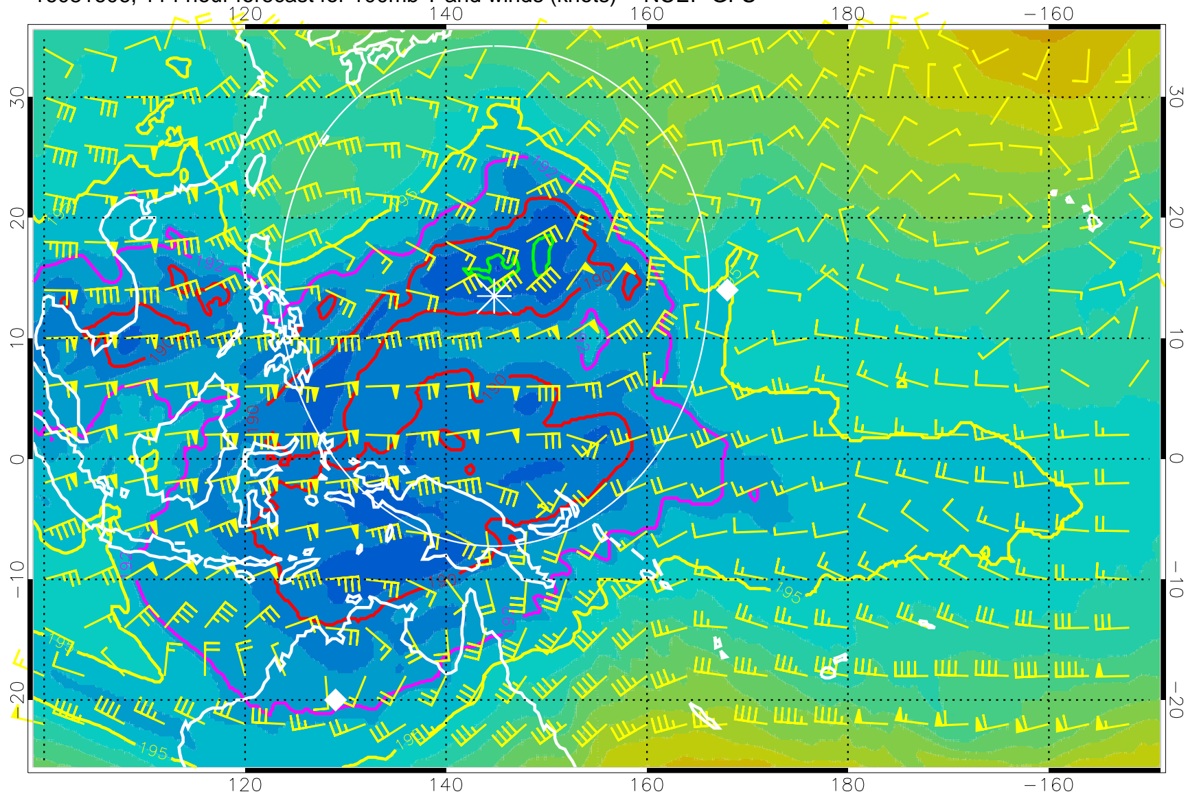
16081606, 114 hour forecast for 100mb T and winds (knots) -- NCEP GFS
