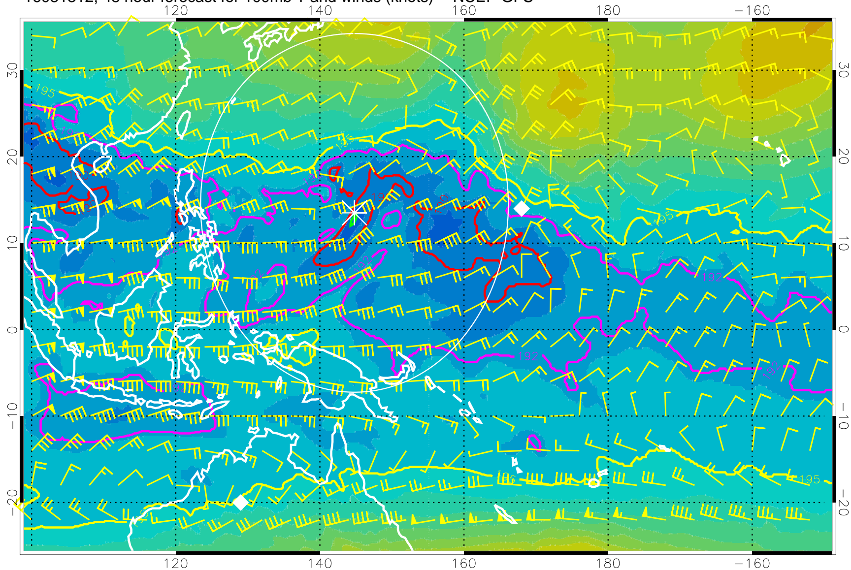
16081312, 48 hour forecast for 100mb T and winds (knots) -- NCEP GFS
