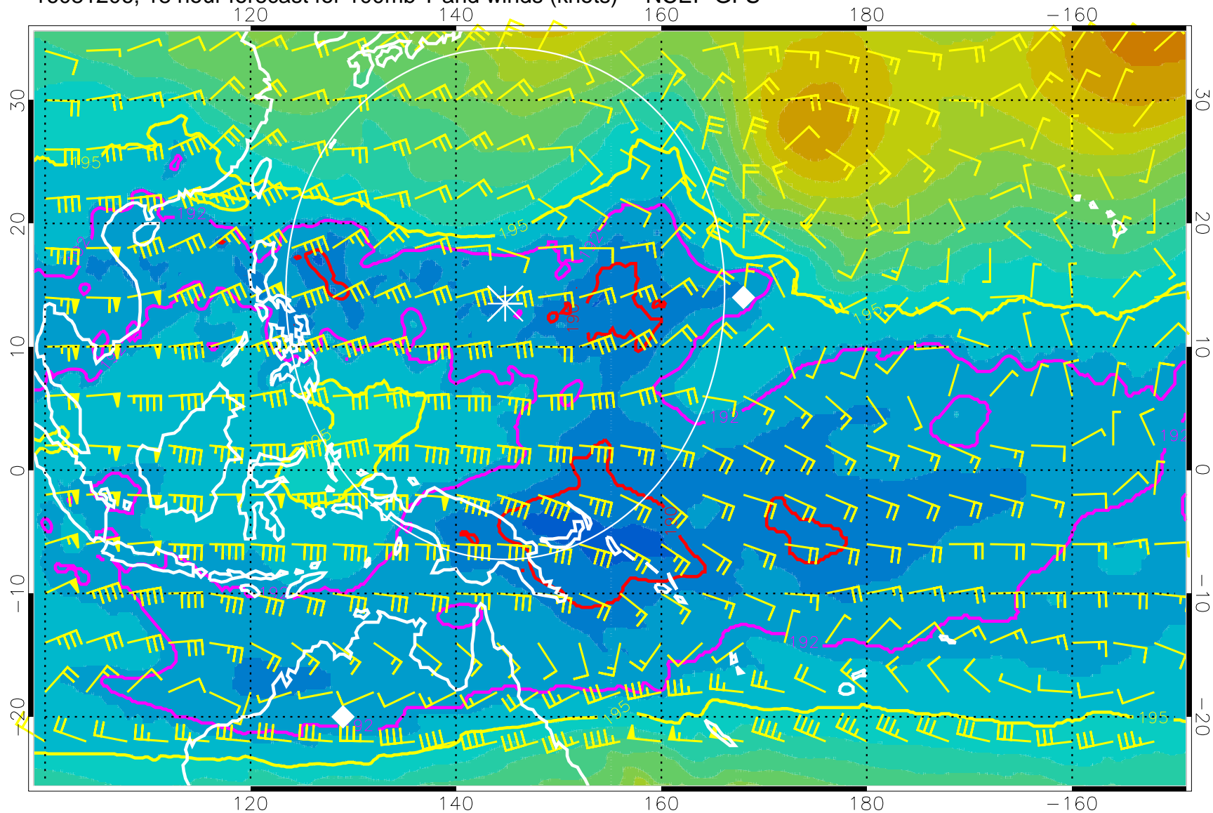
16081206, 18 hour forecast for 100mb T and winds (knots) -- NCEP GFS
