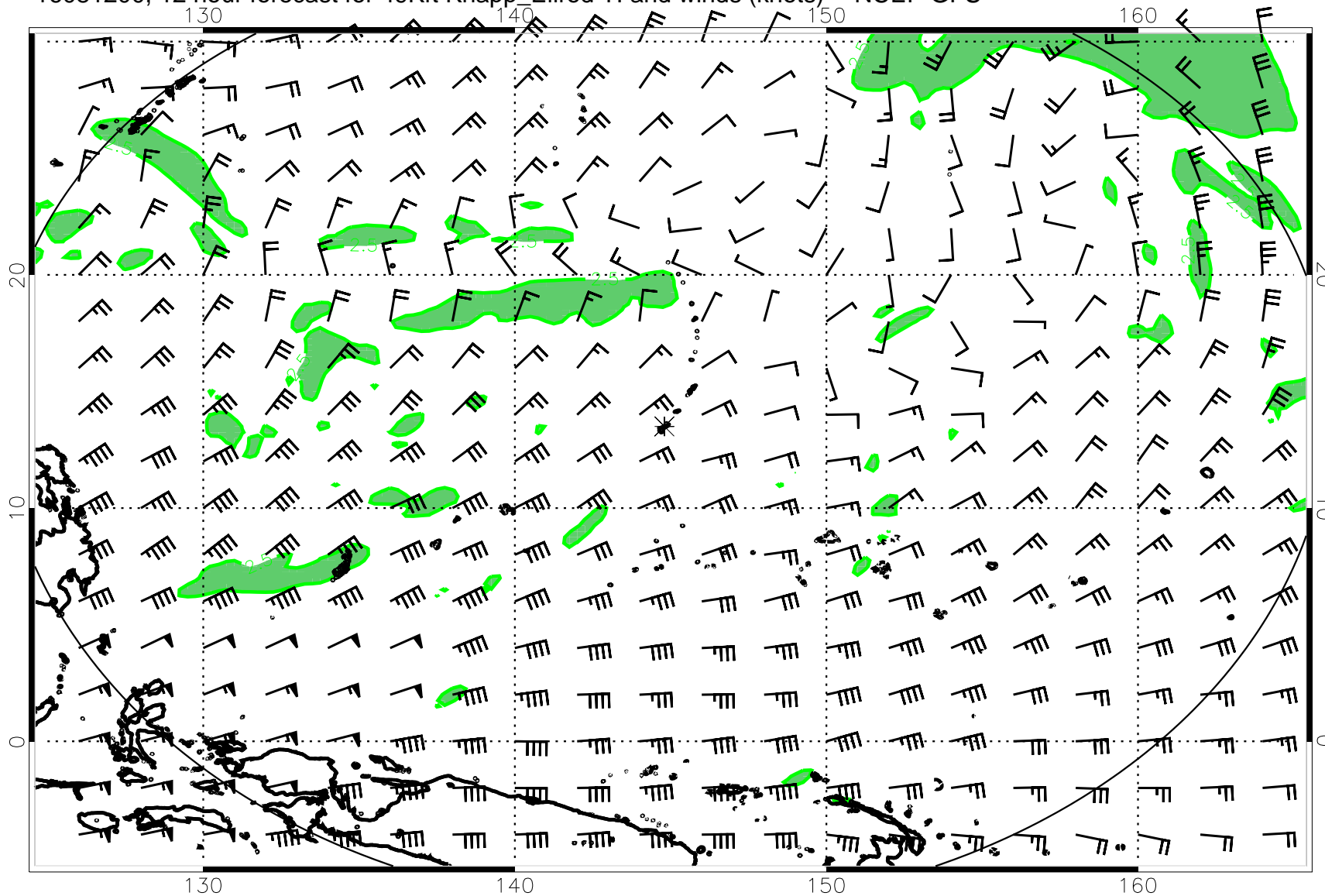
16081200, 12 hour forecast for 49Kft Knapp_Ellrod TI and winds (knots) -- NCEP GFS
