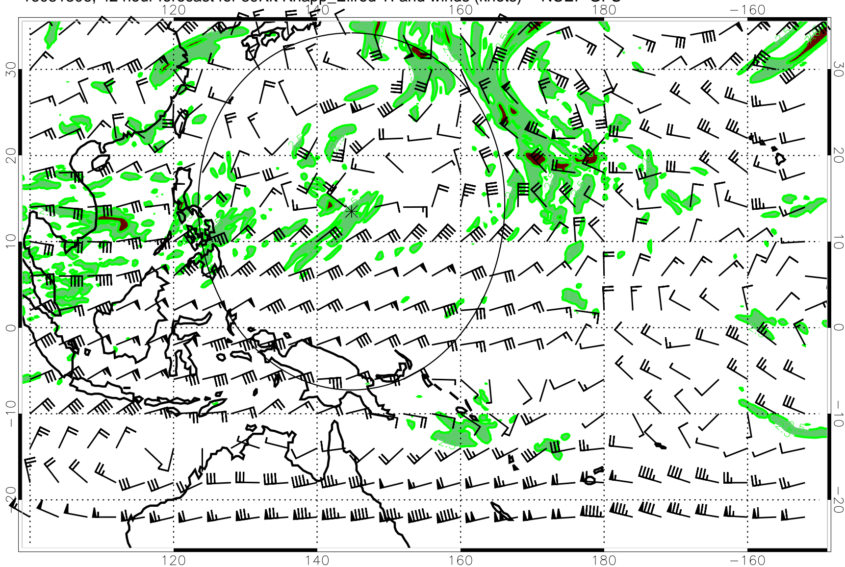
16081306, 42 hour forecast for 39Kft Knapp_Ellrod TI and winds (knots) -- NCEP GFS
