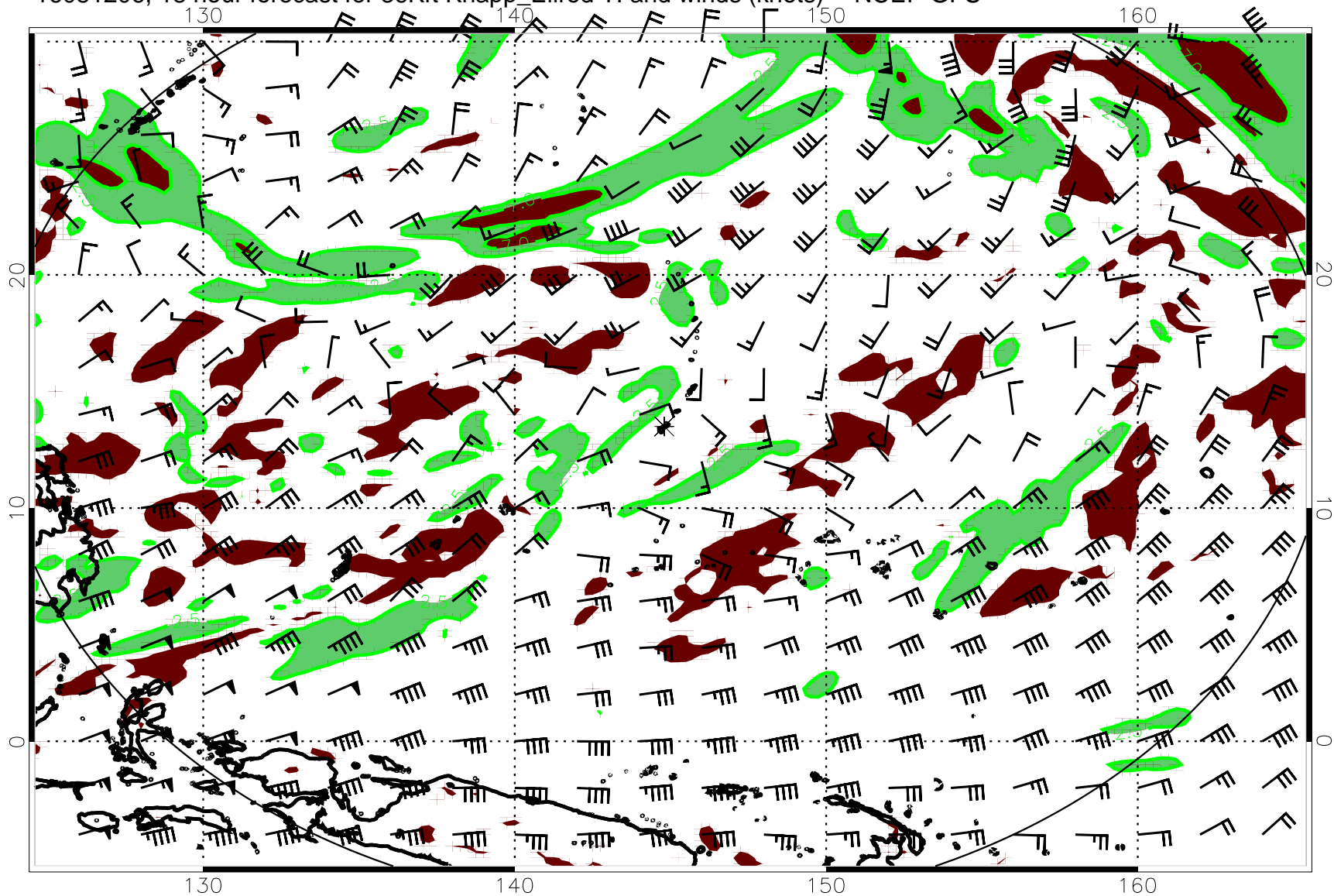
16081206, 18 hour forecast for 36Kft Knapp_Ellrod TI and winds (knots) -- NCEP GFS
