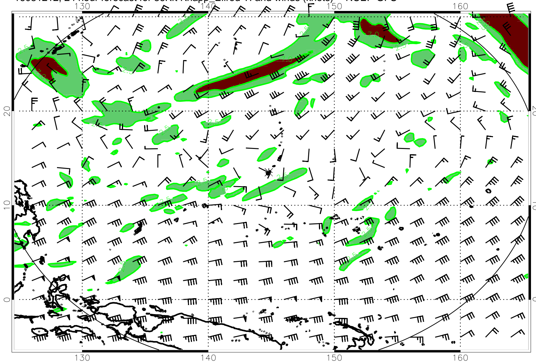
16081212, 24 hour forecast for 36Kft Knapp_Ellrod TI and winds (knots) -- NCEP GFS
