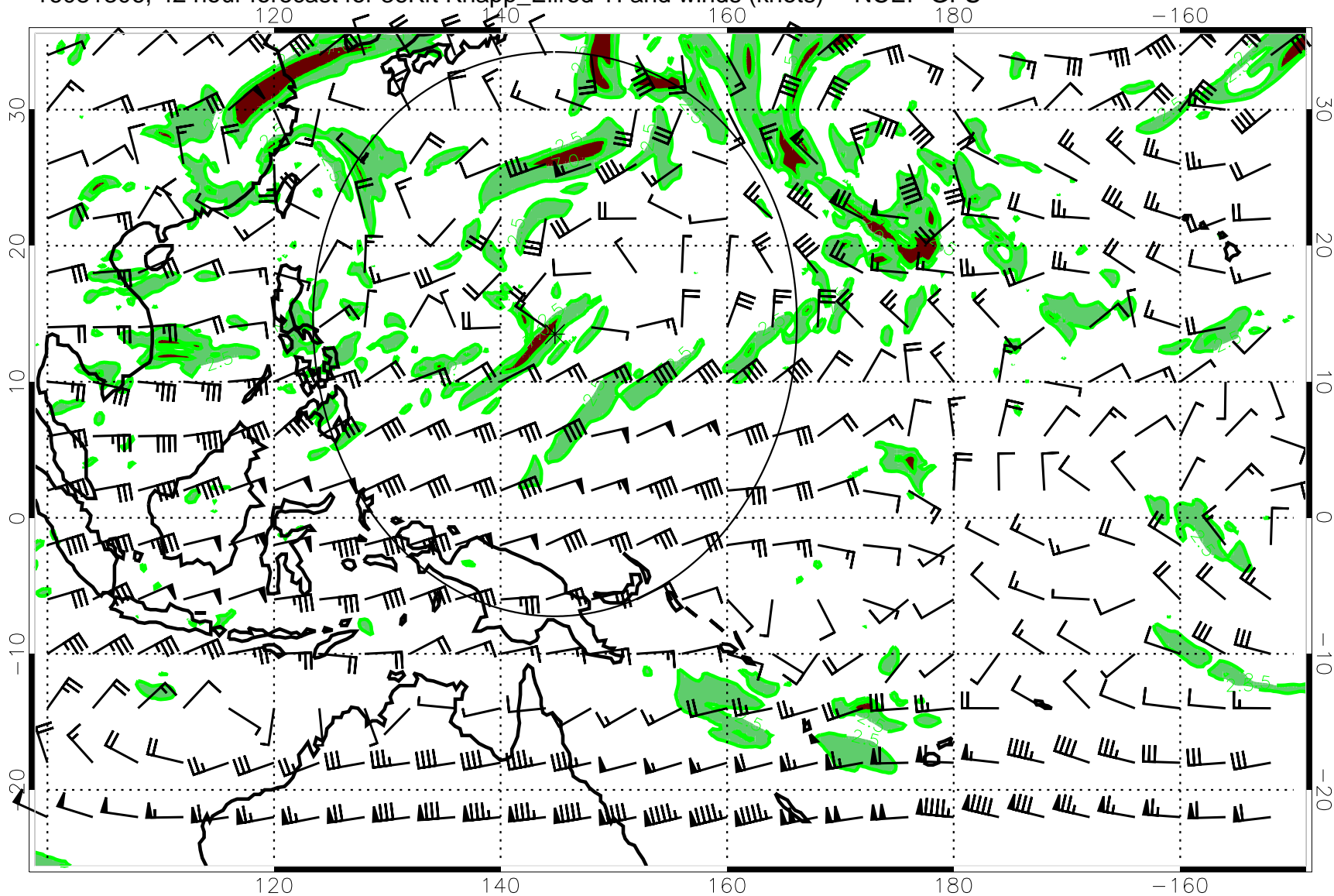
16081306, 42 hour forecast for 36Kft Knapp_Ellrod TI and winds (knots) -- NCEP GFS
