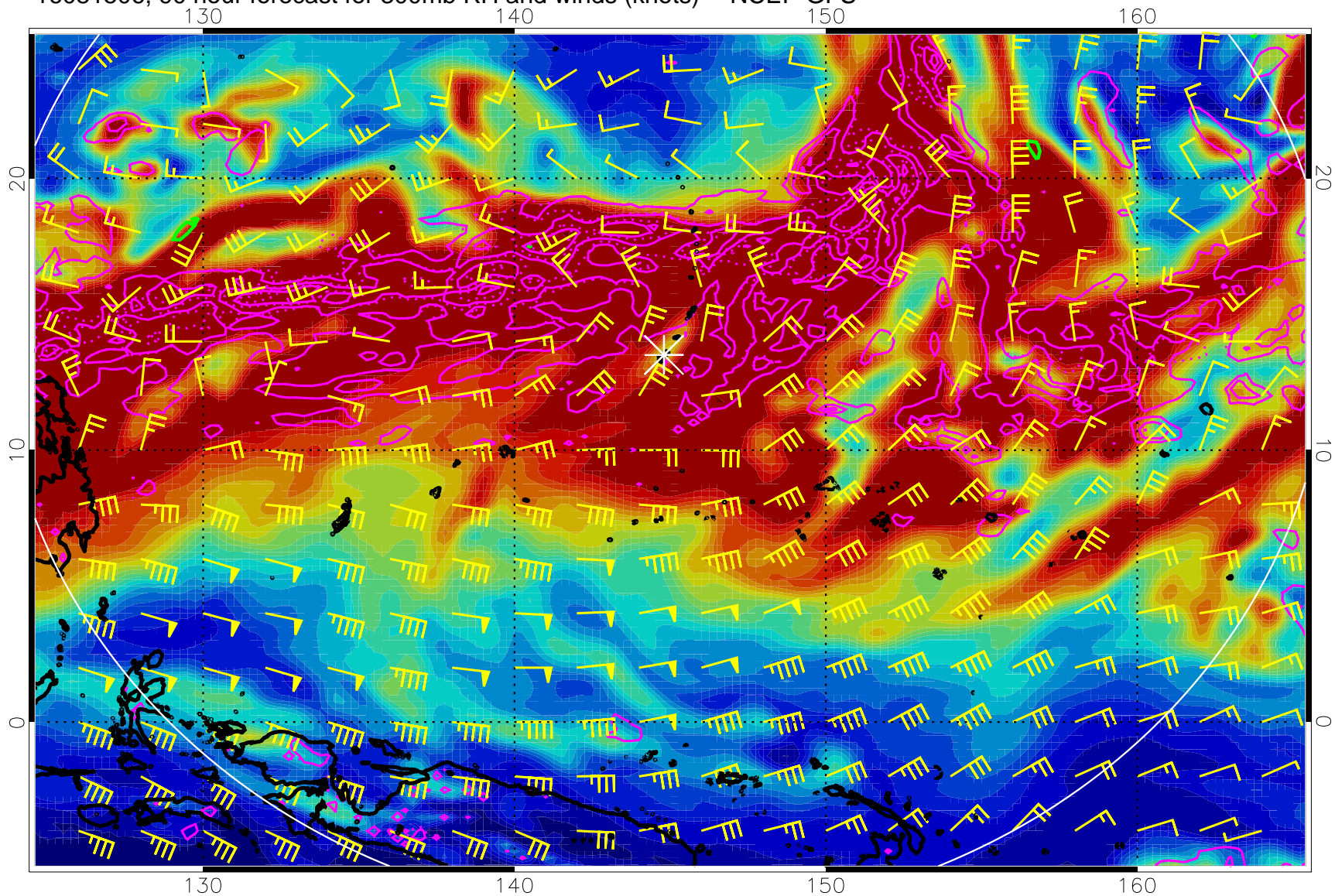
16081506, 90 hour forecast for 300mb RH and winds (knots) -- NCEP GFS
