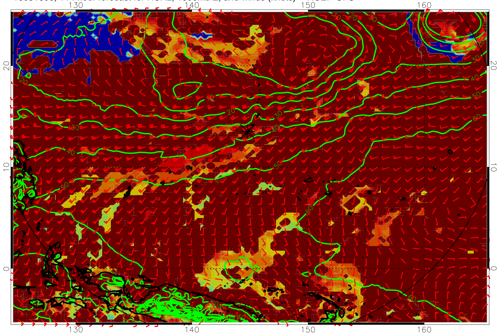
16081606, 114 hour forecast for HCAL, 1000mb Z, and winds (knots) -- NCEP GFS
