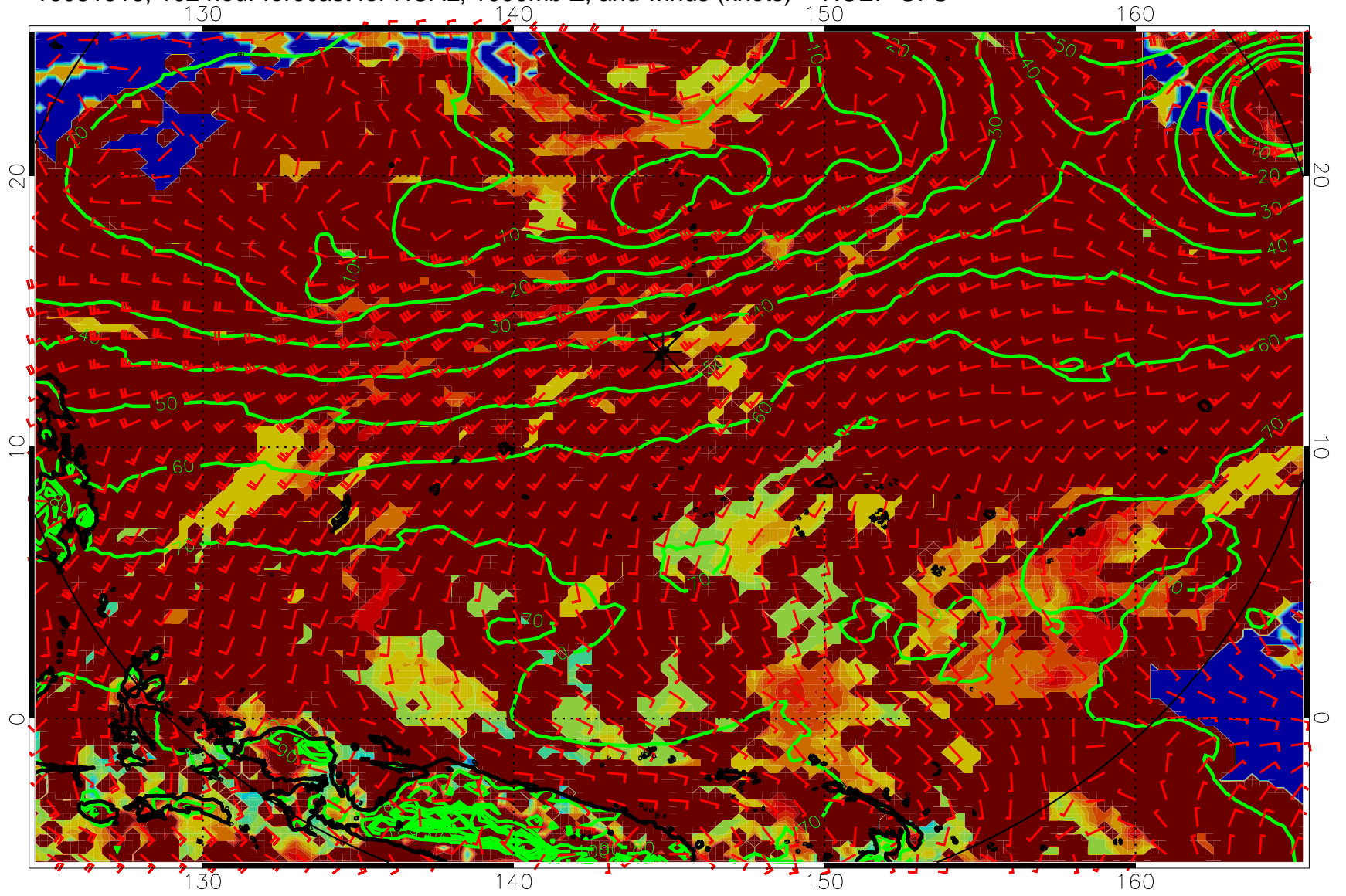
16081518, 102 hour forecast for HCAL, 1000mb Z, and winds (knots) -- NCEP GFS
