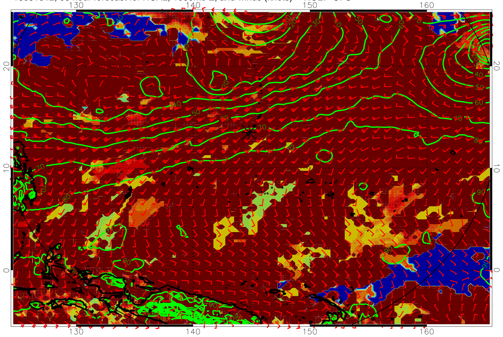
16081512, 96 hour forecast for HCAL, 1000mb Z, and winds (knots) -- NCEP GFS
