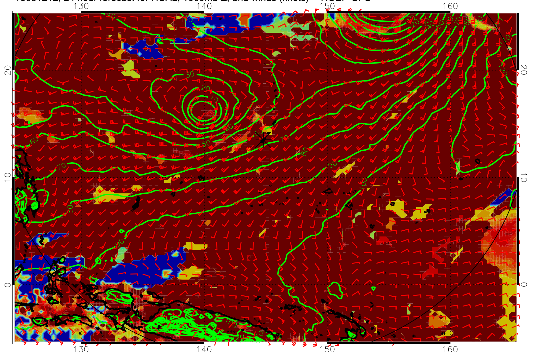
16081212, 24 hour forecast for HCAL, 1000mb Z, and winds (knots) -- NCEP GFS
