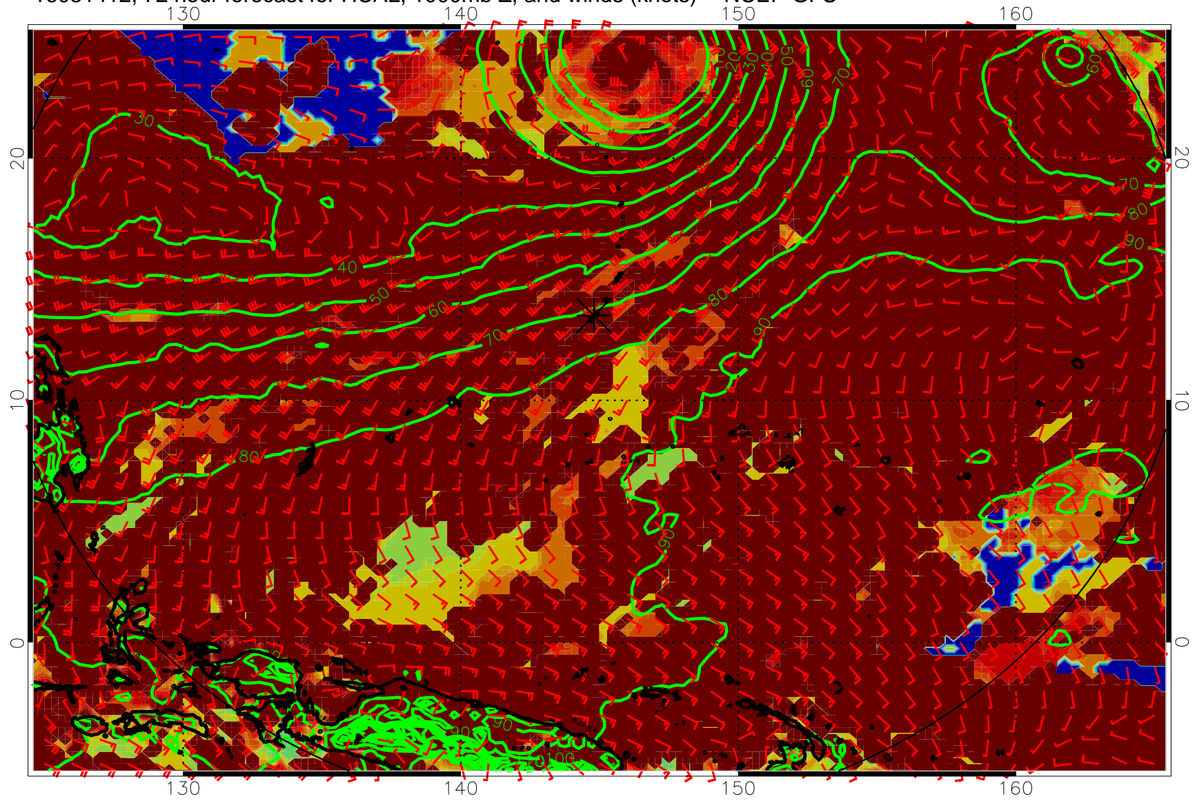
16081412, 72 hour forecast for HCAL, 1000mb Z, and winds (knots) -- NCEP GFS
