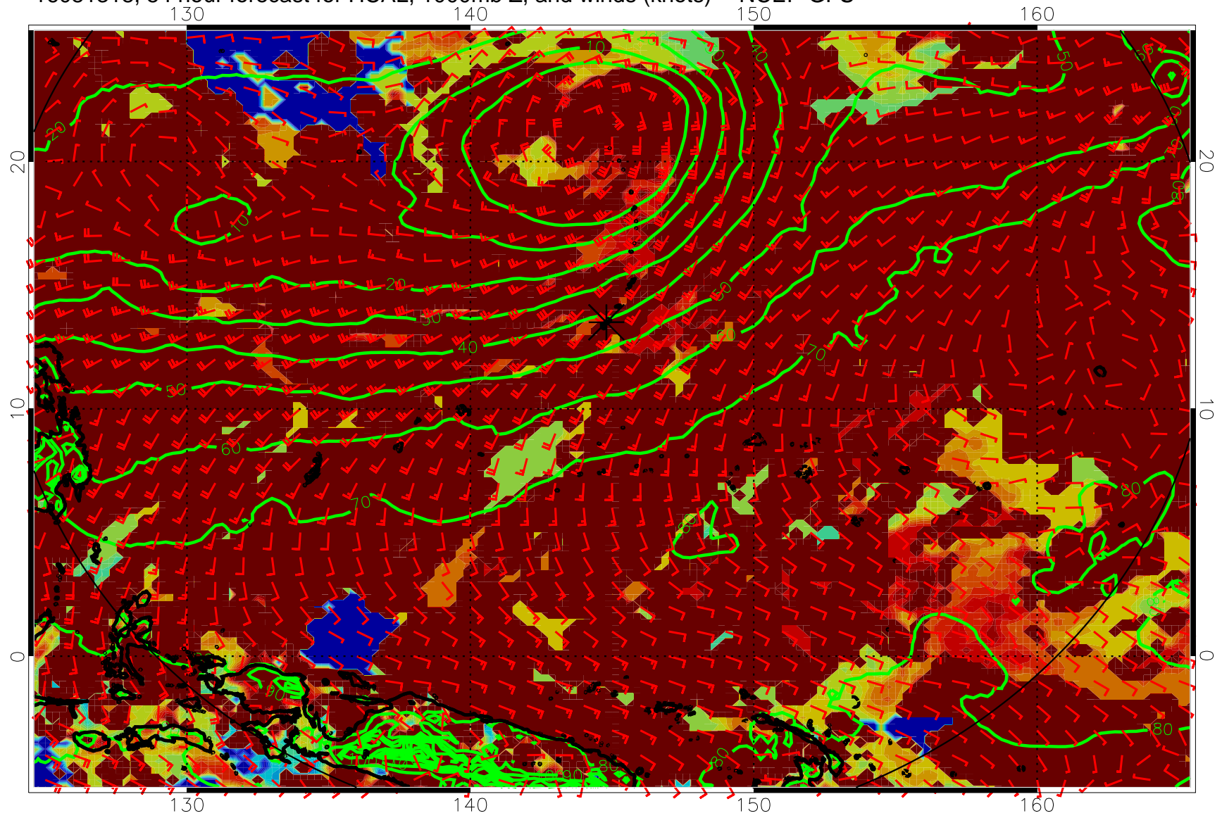
16081318, 54 hour forecast for HCAL, 1000mb Z, and winds (knots) -- NCEP GFS
