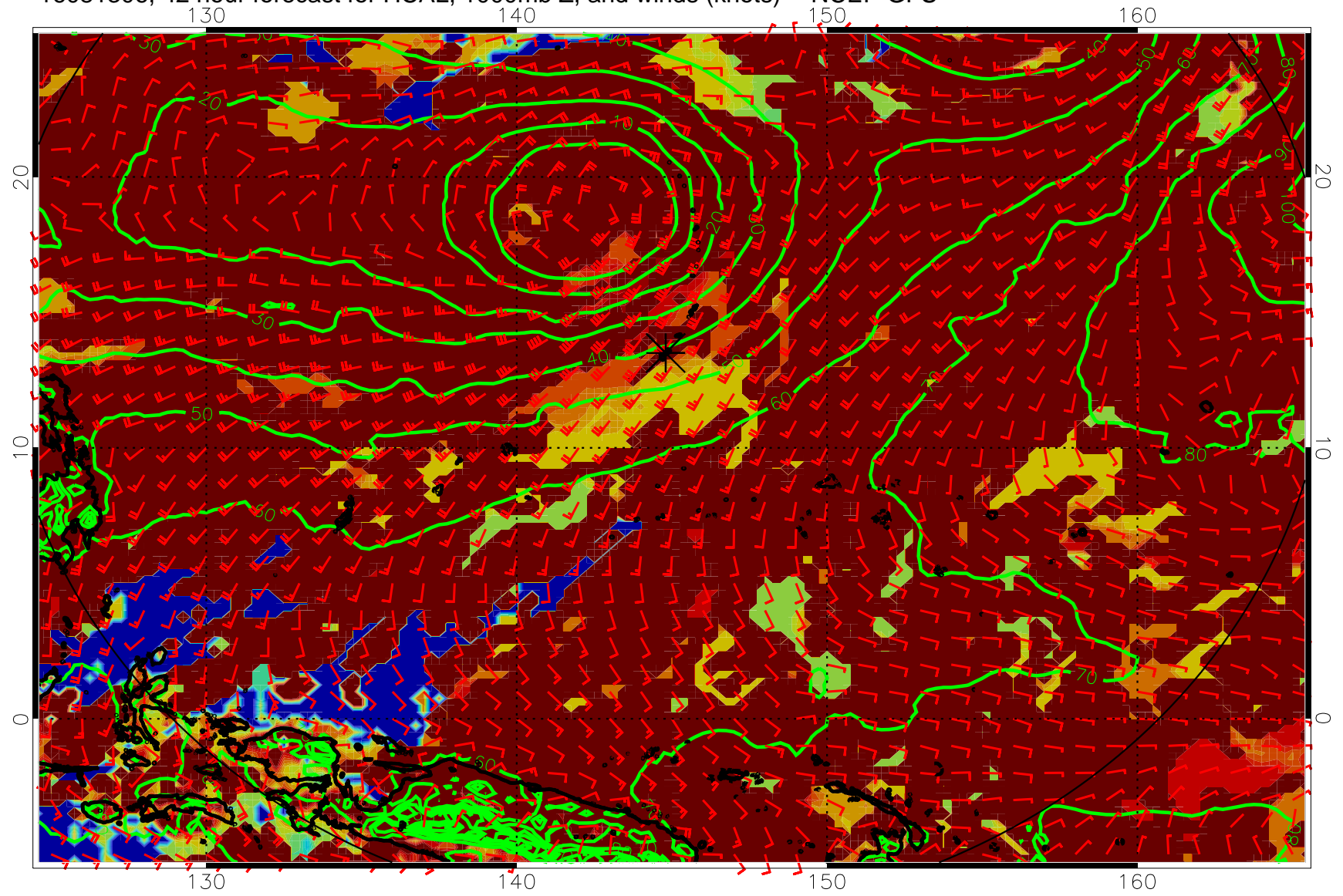
16081306, 42 hour forecast for HCAL, 1000mb Z, and winds (knots) -- NCEP GFS
