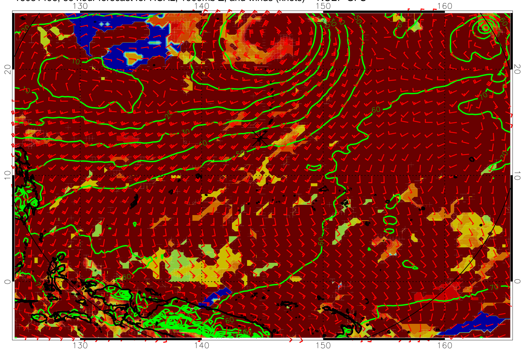
16081406, 66 hour forecast for HCAL, 1000mb Z, and winds (knots) -- NCEP GFS
