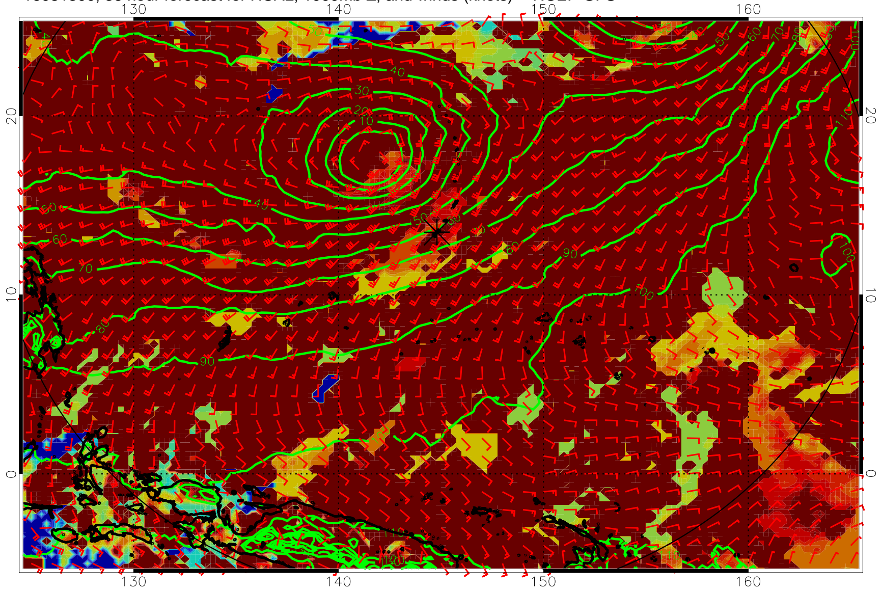
16081300, 36 hour forecast for HCAL, 1000mb Z, and winds (knots) -- NCEP GFS
