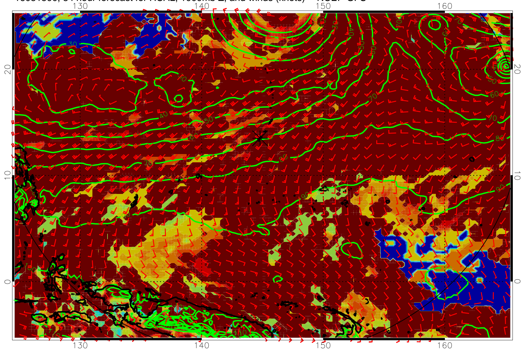
16081500, 84 hour forecast for HCAL, 1000mb Z, and winds (knots) -- NCEP GFS
