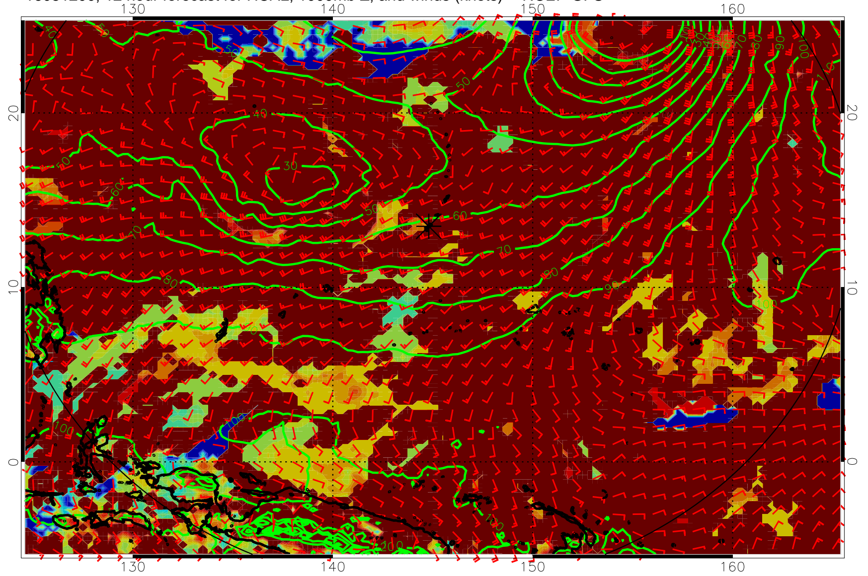
16081200, 12 hour forecast for HCAL, 1000mb Z, and winds (knots) -- NCEP GFS
