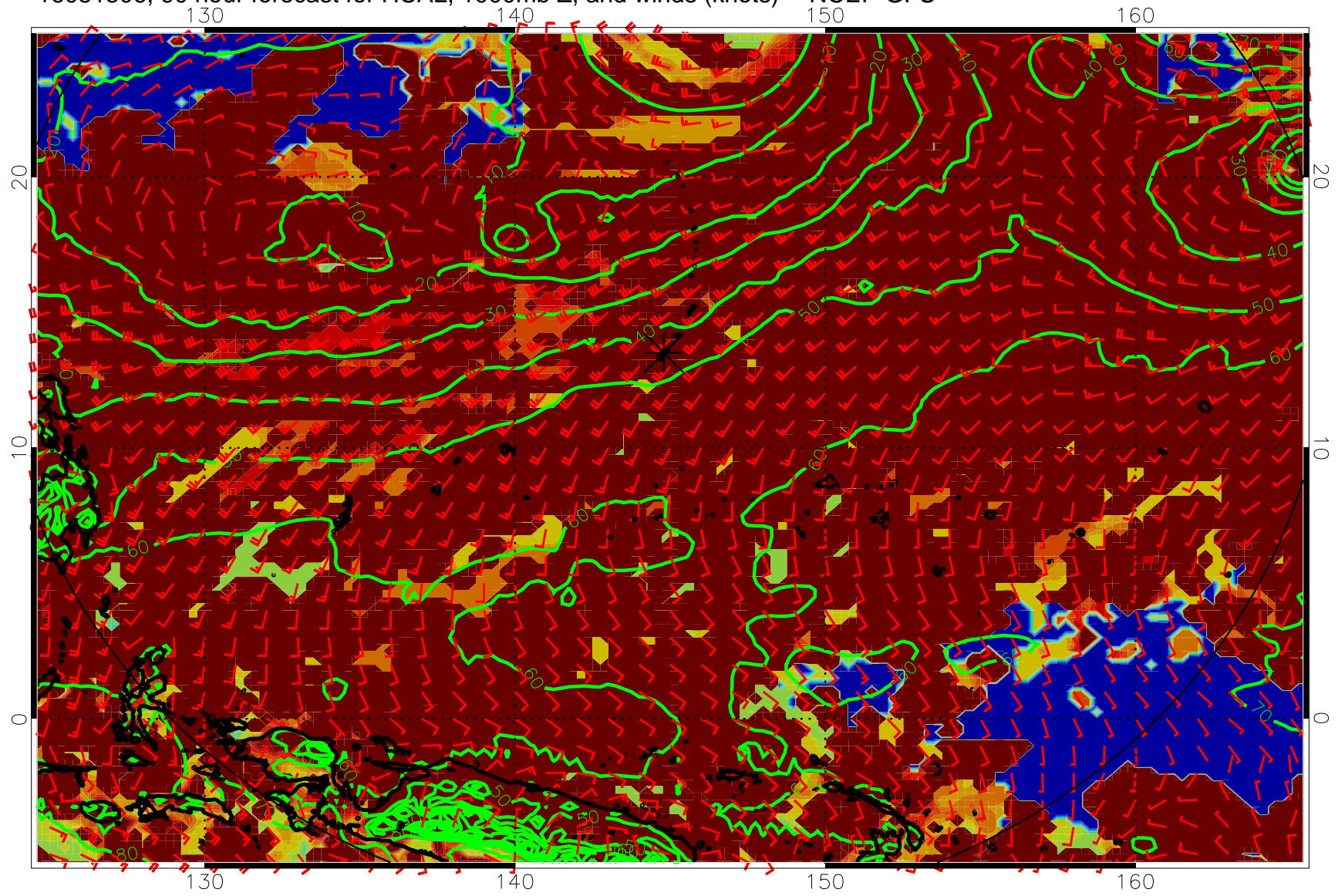
16081506, 90 hour forecast for HCAL, 1000mb Z, and winds (knots) -- NCEP GFS
