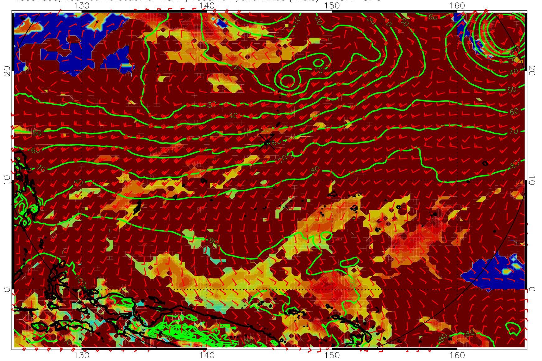
16081600, 108 hour forecast for HCAL, 1000mb Z, and winds (knots) -- NCEP GFS
