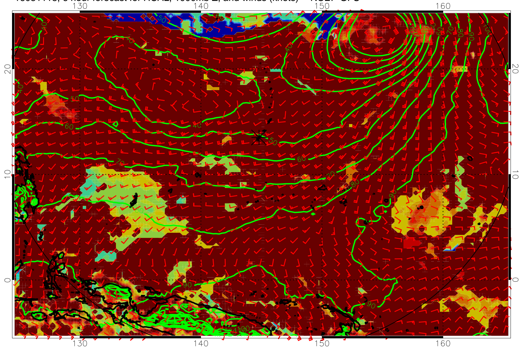
16081118, 6 hour forecast for HCAL, 1000mb Z, and winds (knots) -- NCEP GFS
