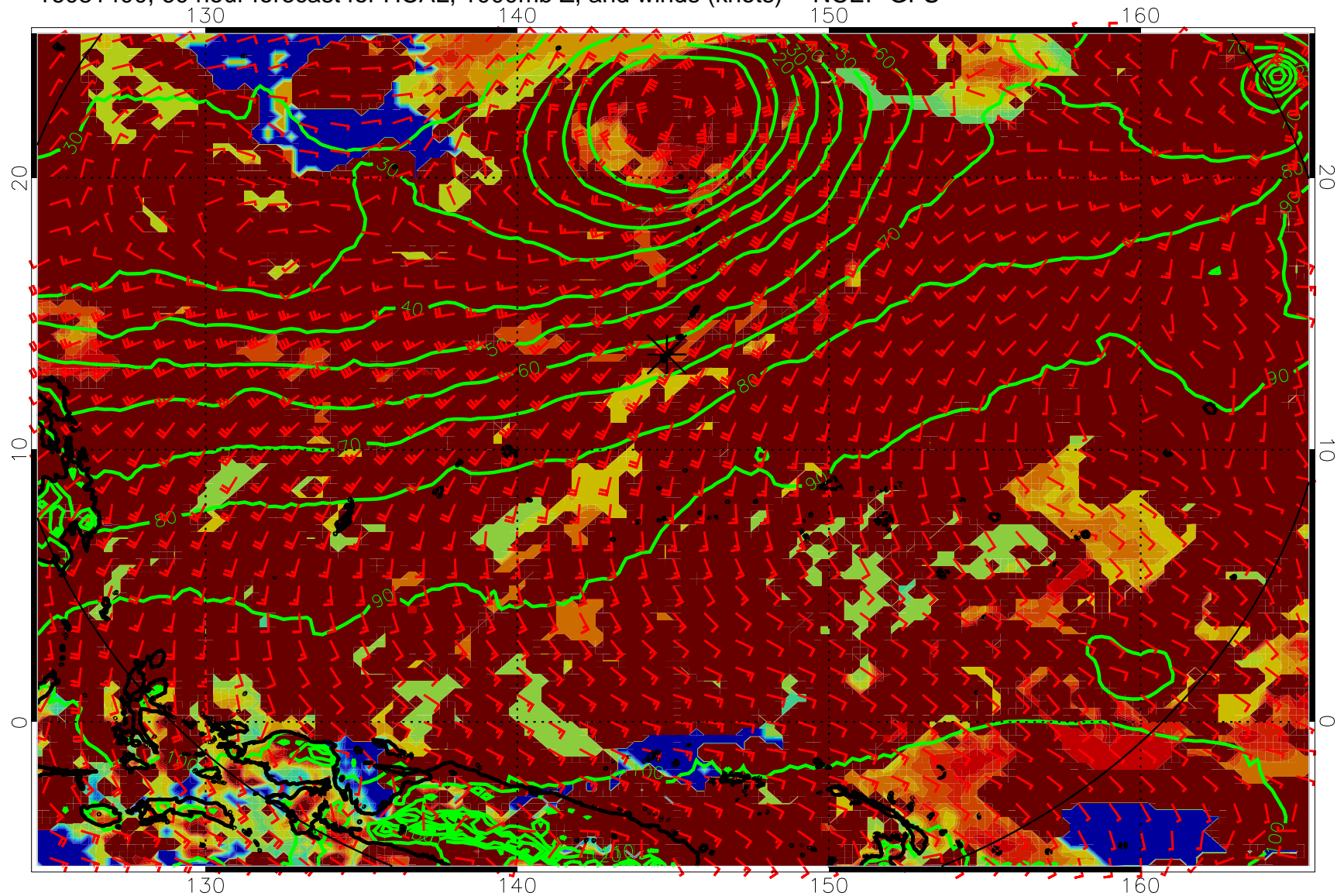
16081400, 60 hour forecast for HCAL, 1000mb Z, and winds (knots) -- NCEP GFS
