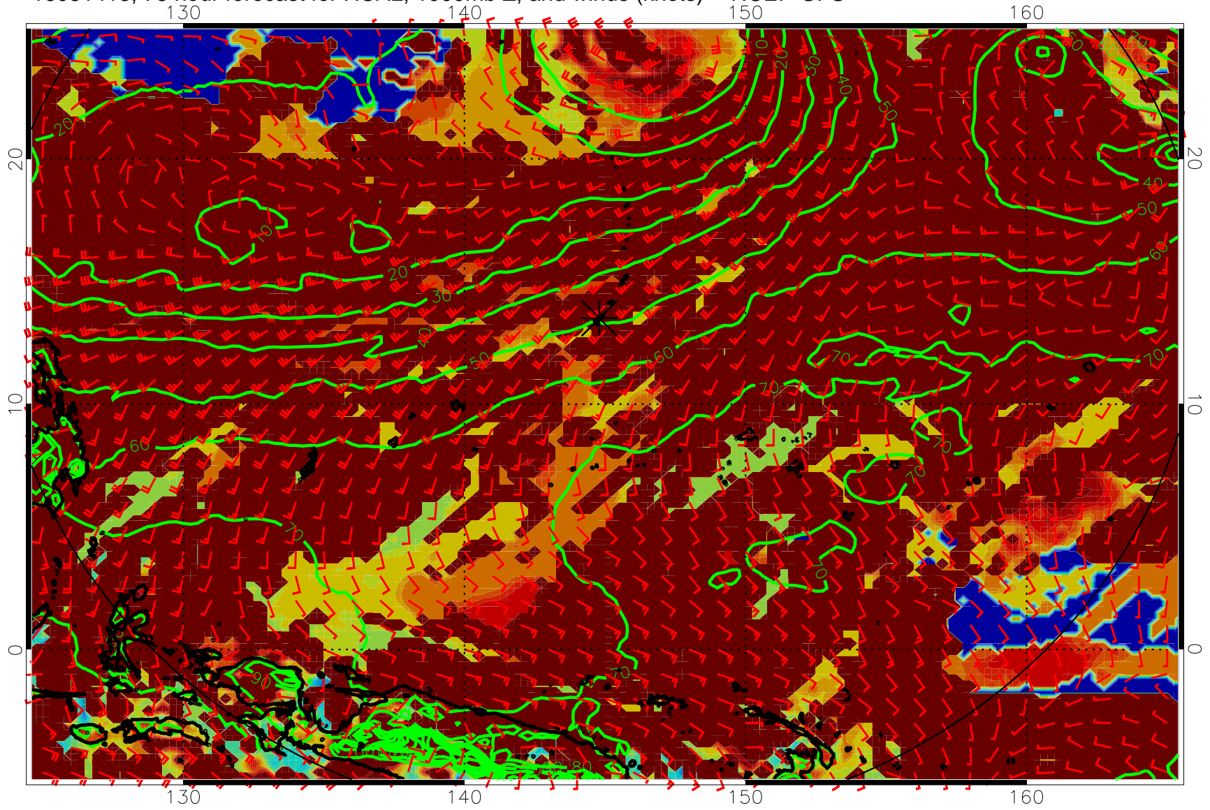
16081418, 78 hour forecast for HCAL, 1000mb Z, and winds (knots) -- NCEP GFS
