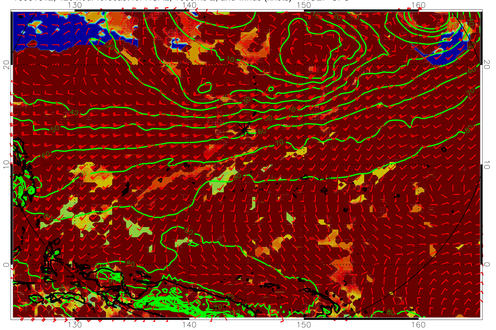
16081612, 120 hour forecast for HCAL, 1000mb Z, and winds (knots) -- NCEP GFS
