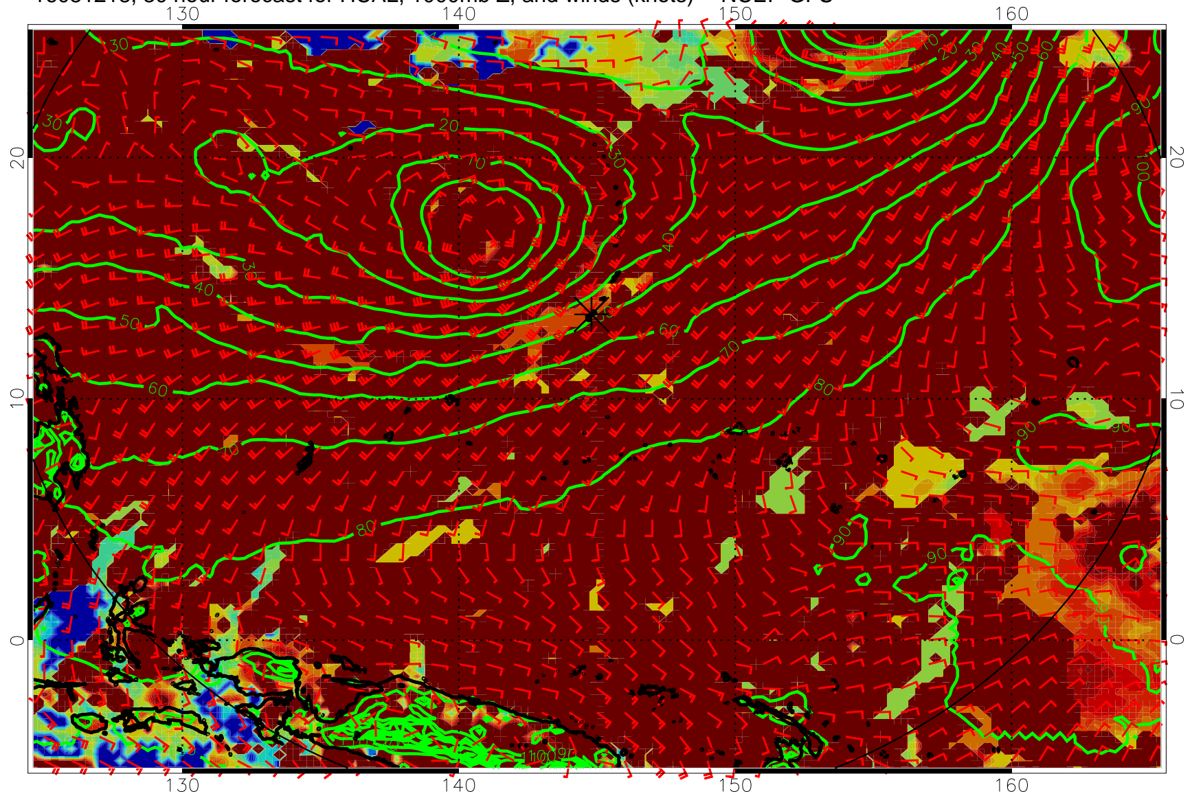
16081218, 30 hour forecast for HCAL, 1000mb Z, and winds (knots) -- NCEP GFS
