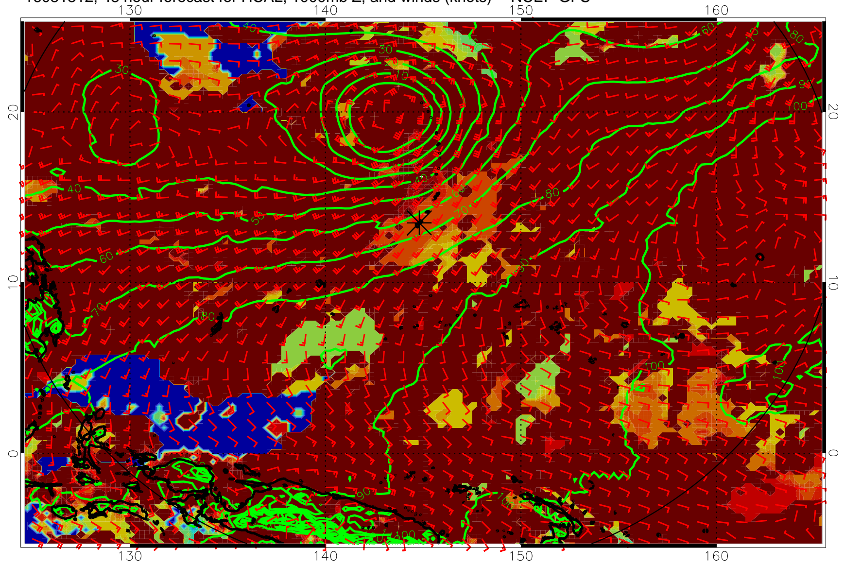
16081312, 48 hour forecast for HCAL, 1000mb Z, and winds (knots) -- NCEP GFS
