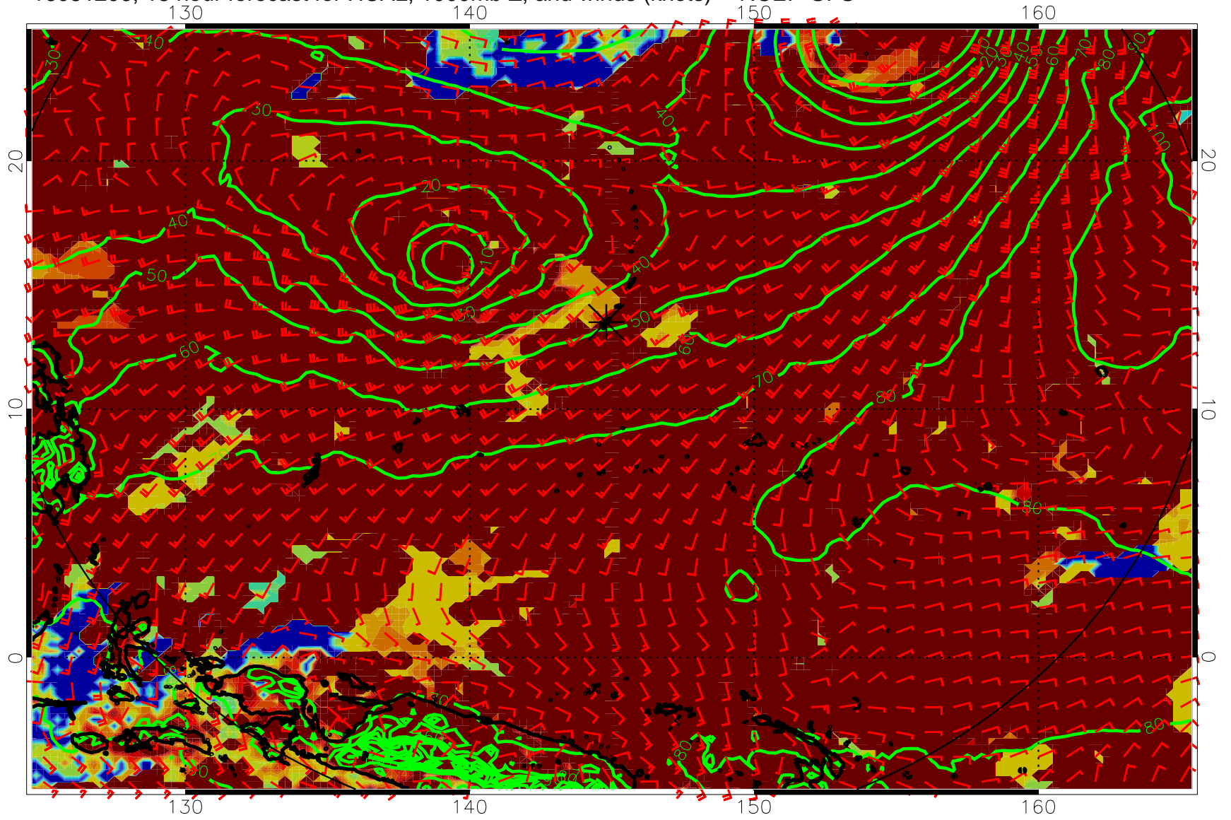
16081206, 18 hour forecast for HCAL, 1000mb Z, and winds (knots) -- NCEP GFS
