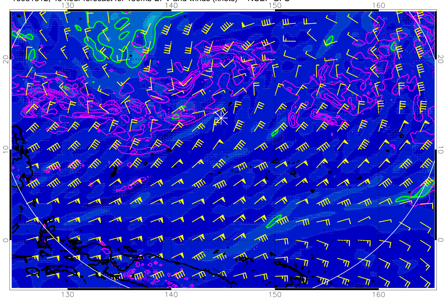
16081312, 48 hour forecast for 150mb EPV and winds (knots) -- NCEP GFS
