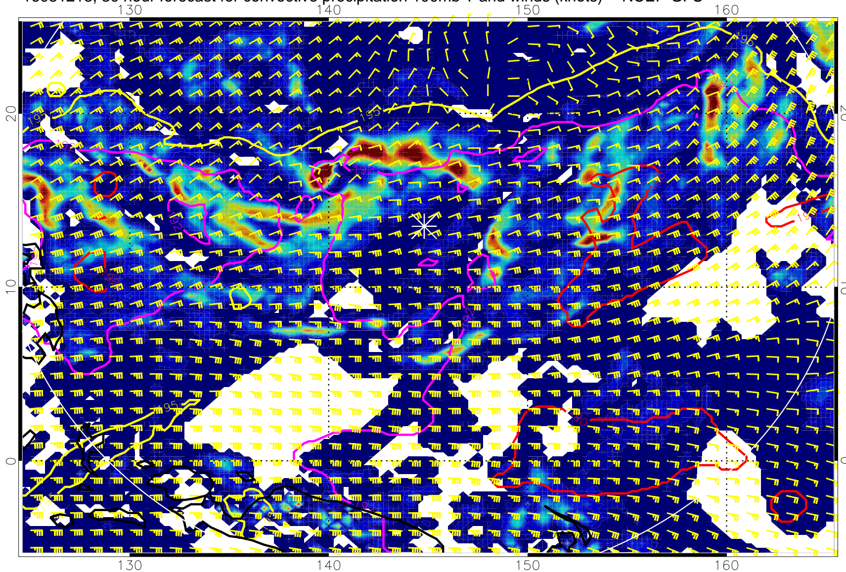
16081218, 30 hour forecast for convective precipitation 100mb T and winds (knots) -- NCEP GFS
