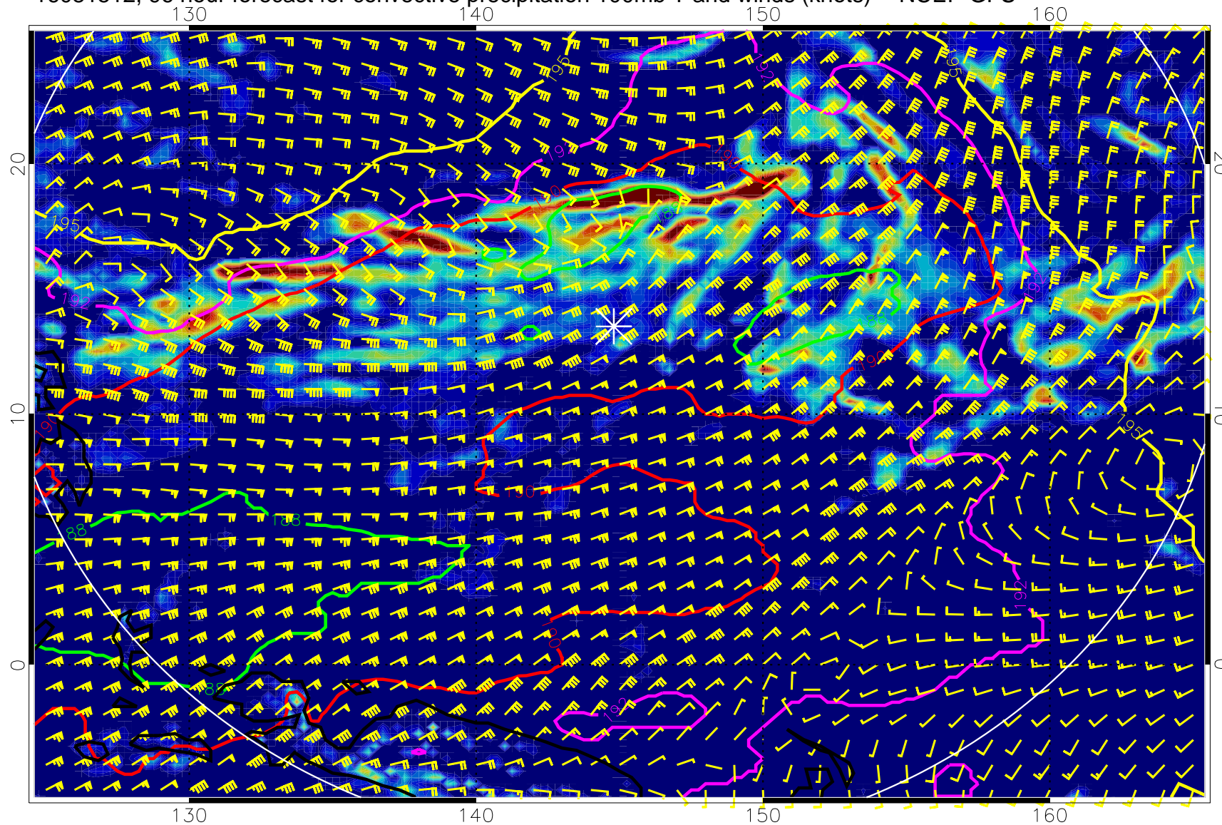
16081512, 96 hour forecast for convective precipitation 100mb T and winds (knots) -- NCEP GFS
