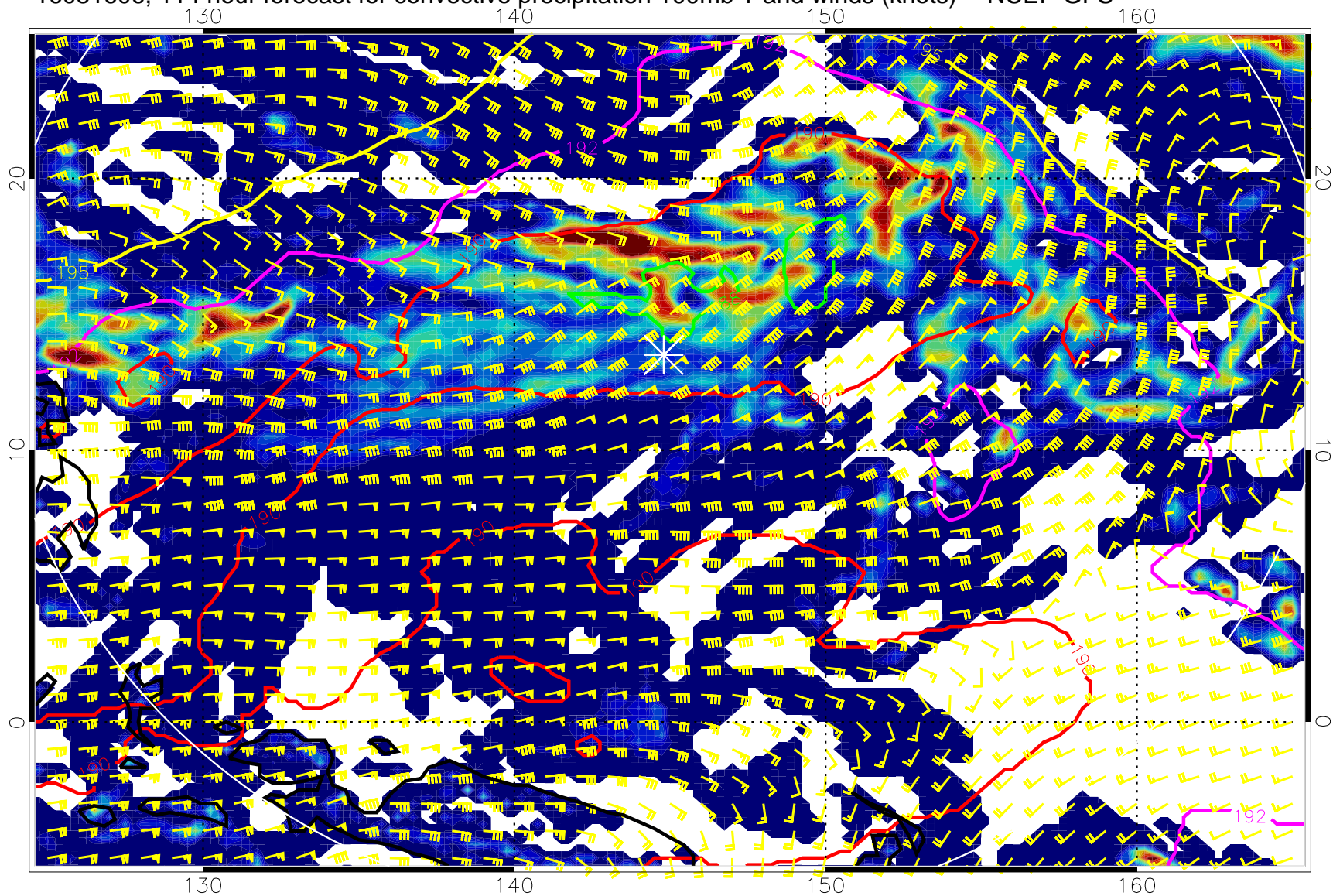
16081606, 114 hour forecast for convective precipitation 100mb T and winds (knots) -- NCEP GFS
