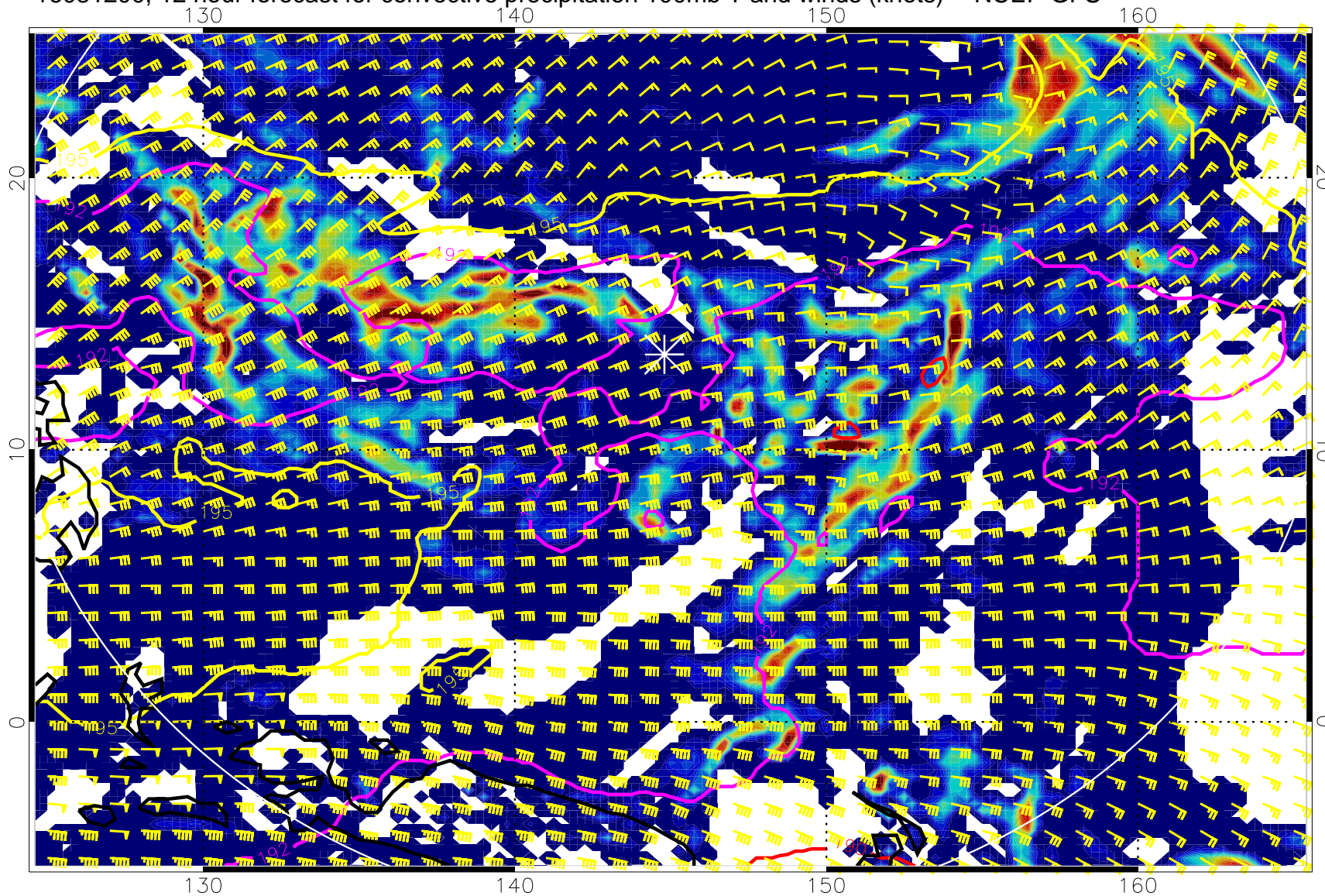
16081200, 12 hour forecast for convective precipitation 100mb T and winds (knots) -- NCEP GFS
