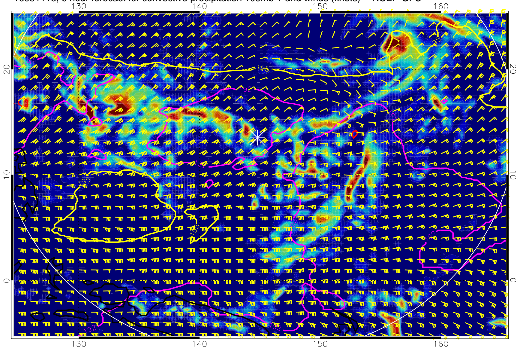
16081118, 6 hour forecast for convective precipitation 100mb T and winds (knots) -- NCEP GFS
