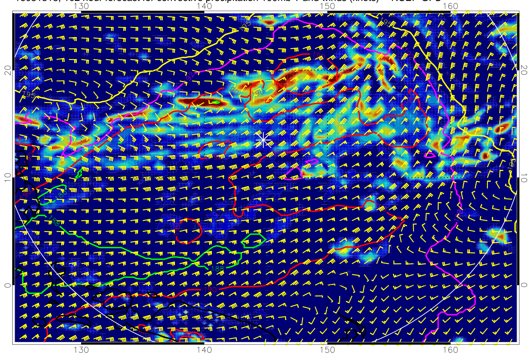
16081518, 102 hour forecast for convective precipitation 100mb T and winds (knots) -- NCEP GFS
