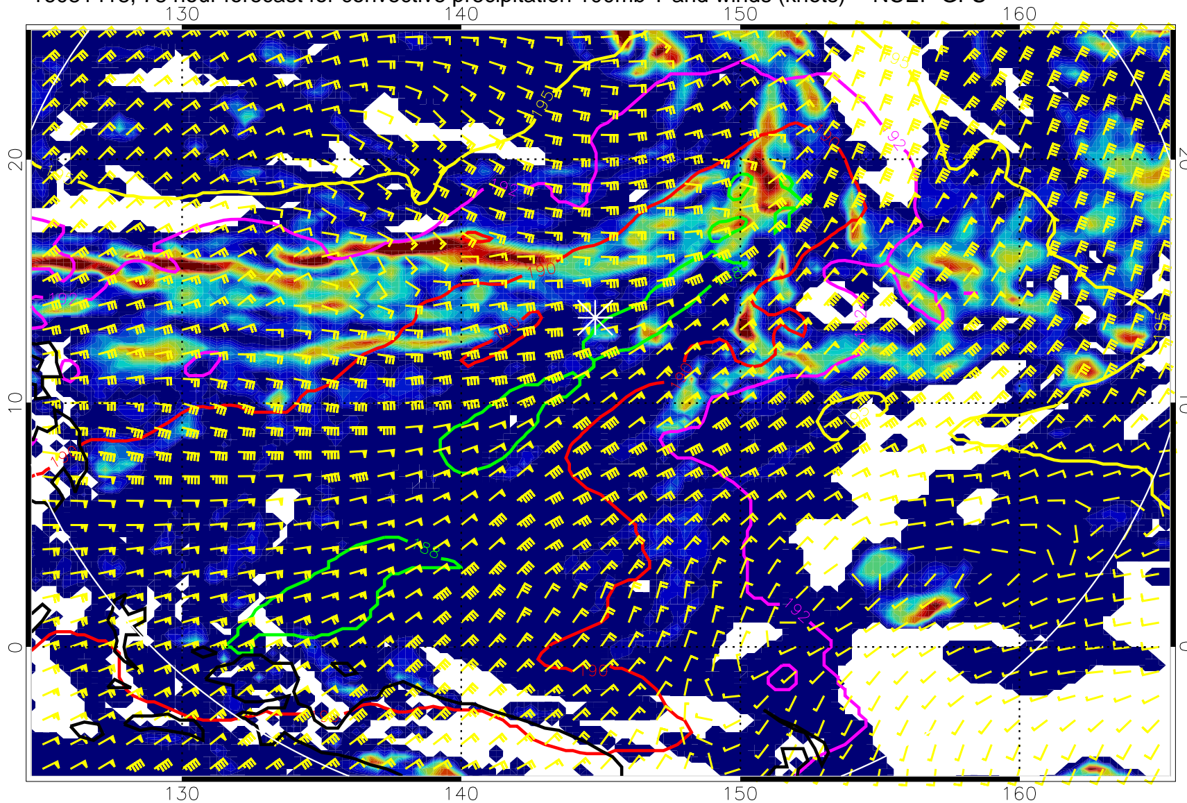
16081418, 78 hour forecast for convective precipitation 100mb T and winds (knots) -- NCEP GFS
