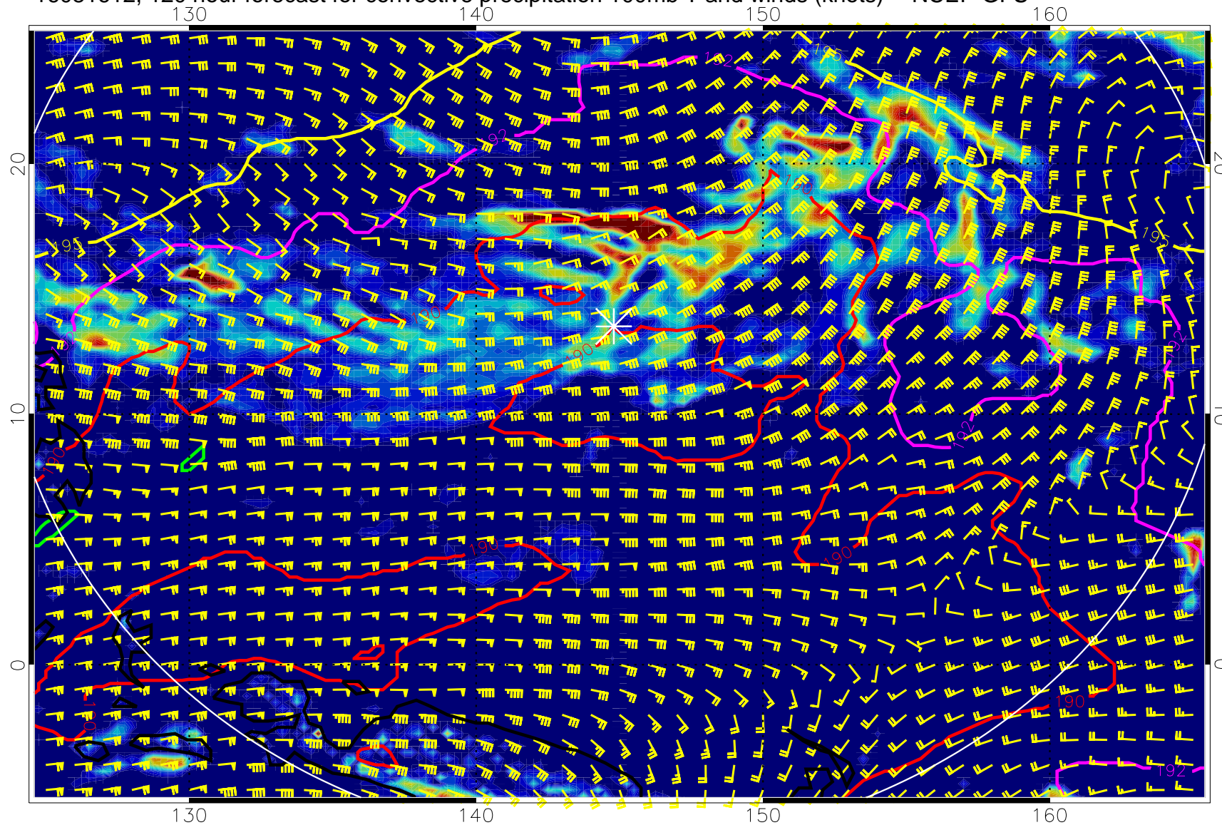
16081612, 120 hour forecast for convective precipitation 100mb T and winds (knots) -- NCEP GFS
