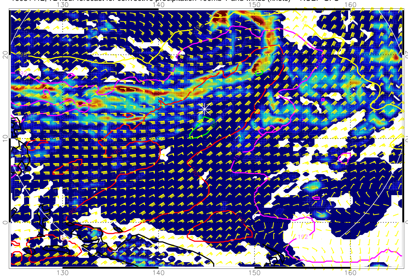
16081412, 72 hour forecast for convective precipitation 100mb T and winds (knots) -- NCEP GFS
