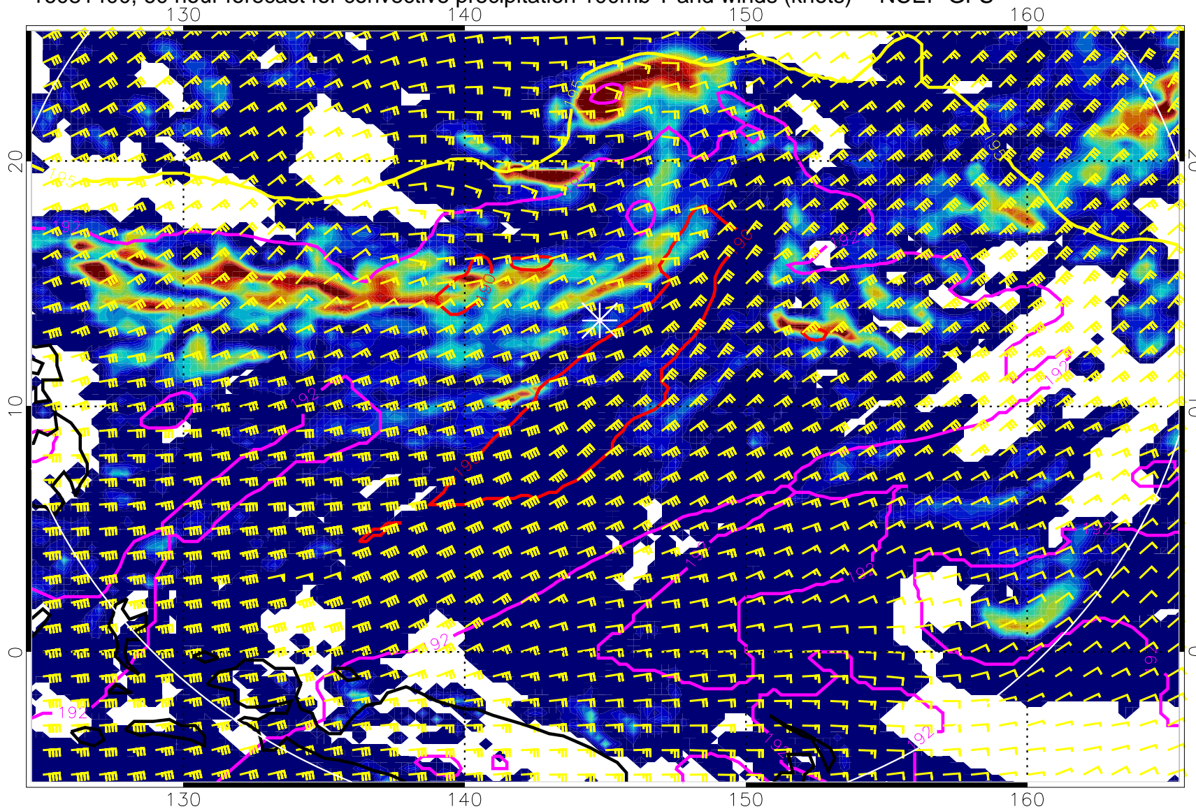
16081400, 60 hour forecast for convective precipitation 100mb T and winds (knots) -- NCEP GFS
