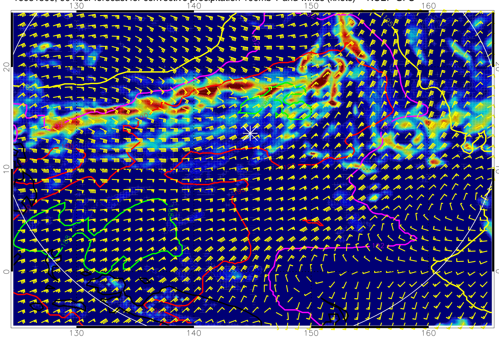
16081506, 90 hour forecast for convective precipitation 100mb T and winds (knots) -- NCEP GFS
