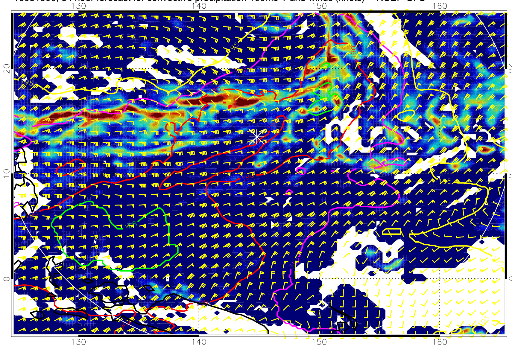
16081500, 84 hour forecast for convective precipitation 100mb T and winds (knots) -- NCEP GFS
