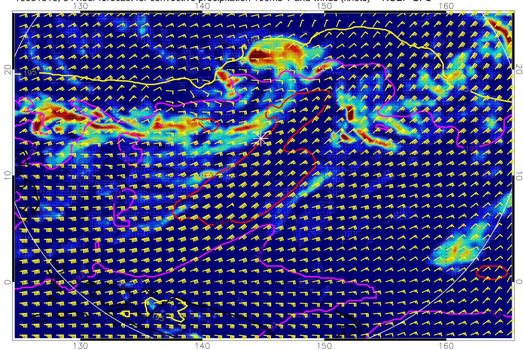
16081318, 54 hour forecast for convective precipitation 100mb T and winds (knots) -- NCEP GFS
