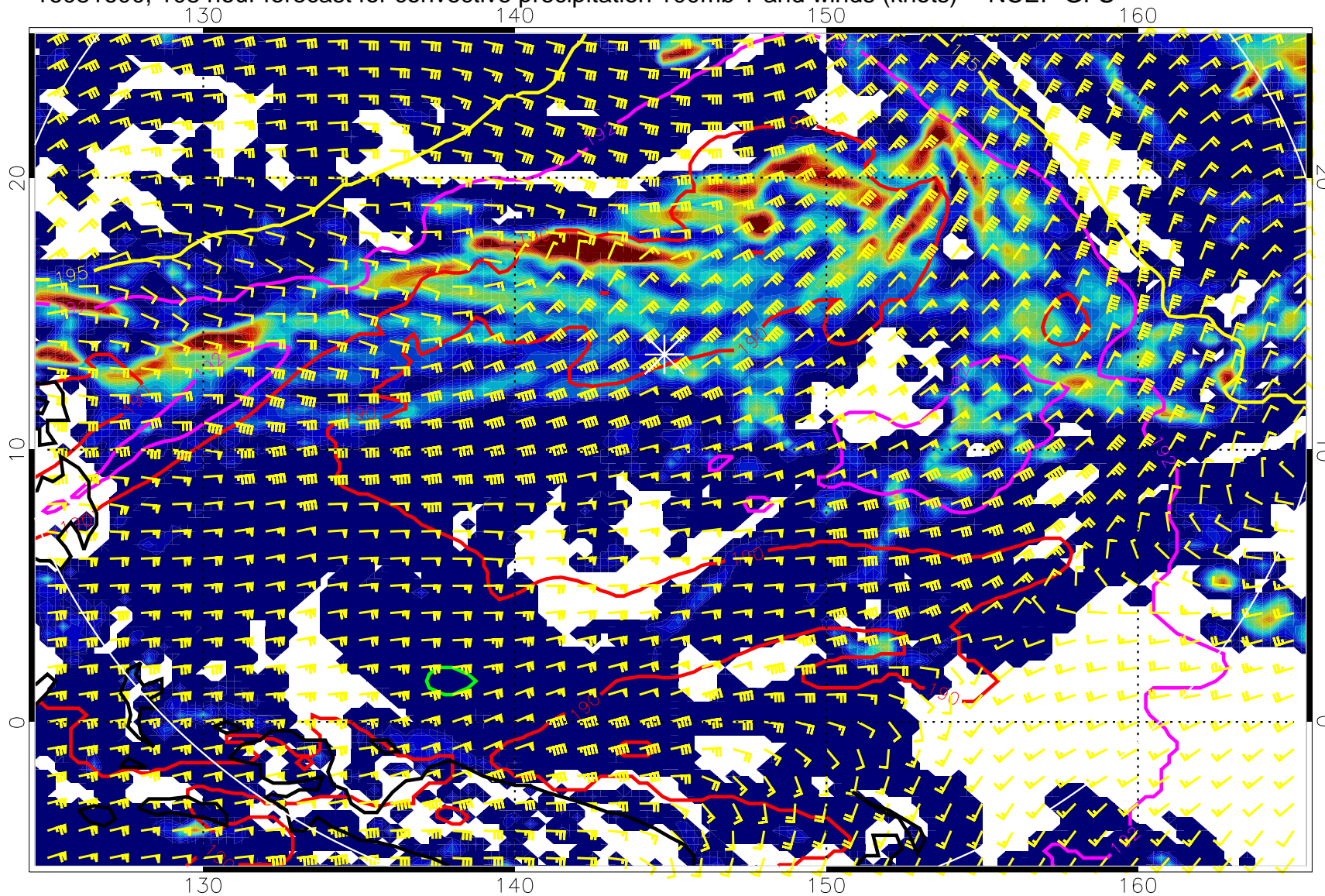
16081600, 108 hour forecast for convective precipitation 100mb T and winds (knots) -- NCEP GFS
