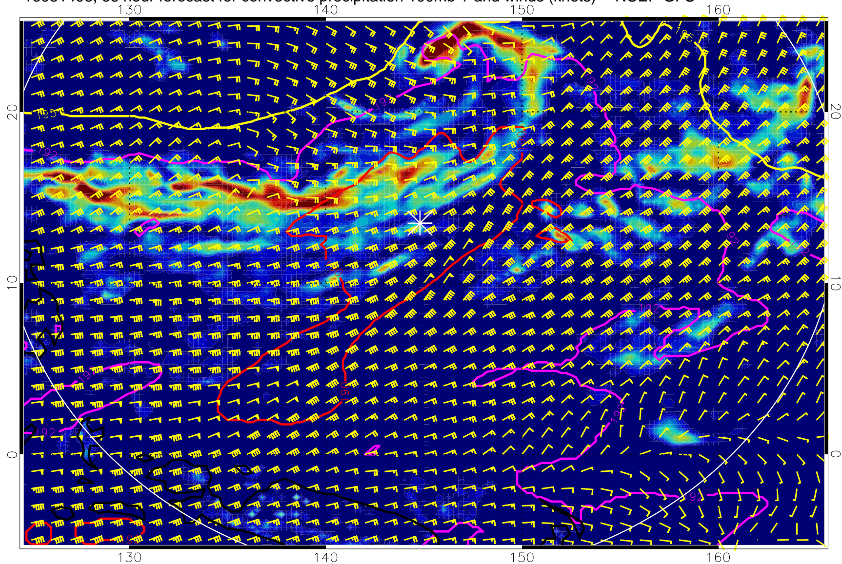
16081406, 66 hour forecast for convective precipitation 100mb T and winds (knots) -- NCEP GFS
