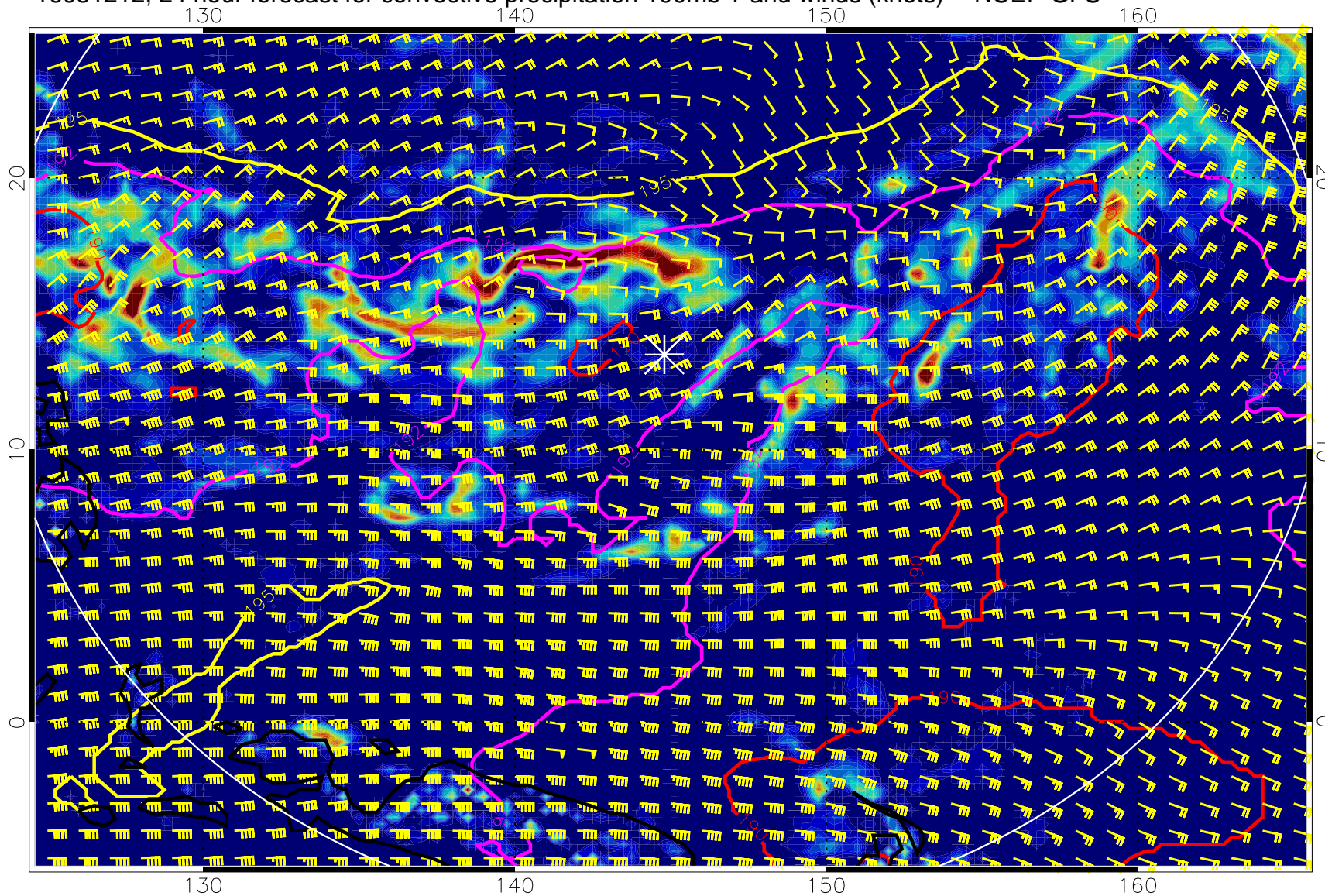
16081212, 24 hour forecast for convective precipitation 100mb T and winds (knots) -- NCEP GFS
