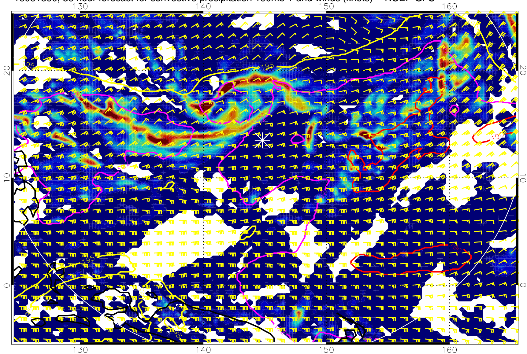
16081300, 36 hour forecast for convective precipitation 100mb T and winds (knots) -- NCEP GFS
