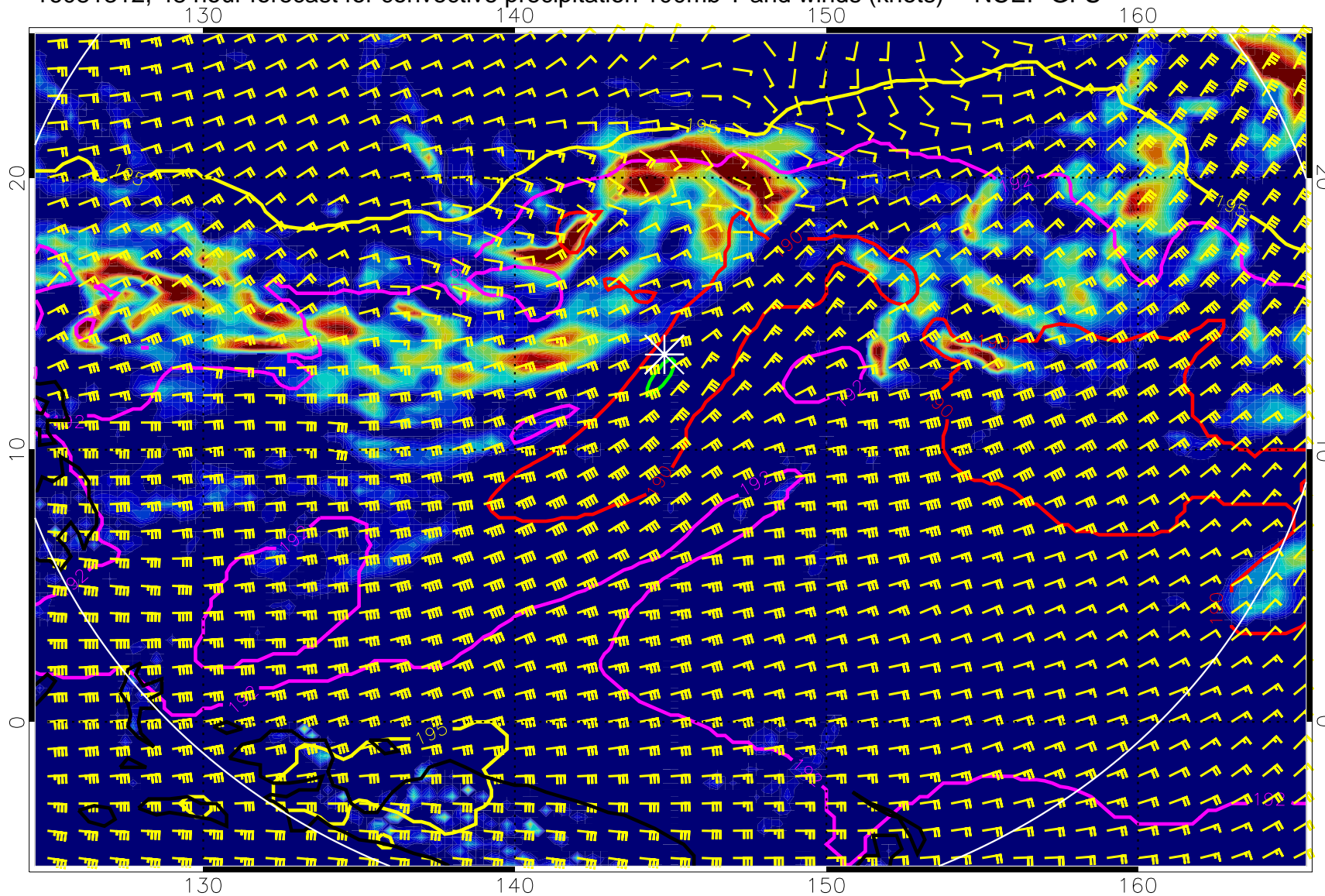
16081312, 48 hour forecast for convective precipitation 100mb T and winds (knots) -- NCEP GFS
