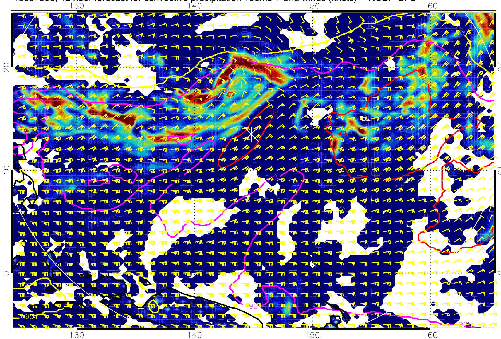
16081306, 42 hour forecast for convective precipitation 100mb T and winds (knots) -- NCEP GFS
