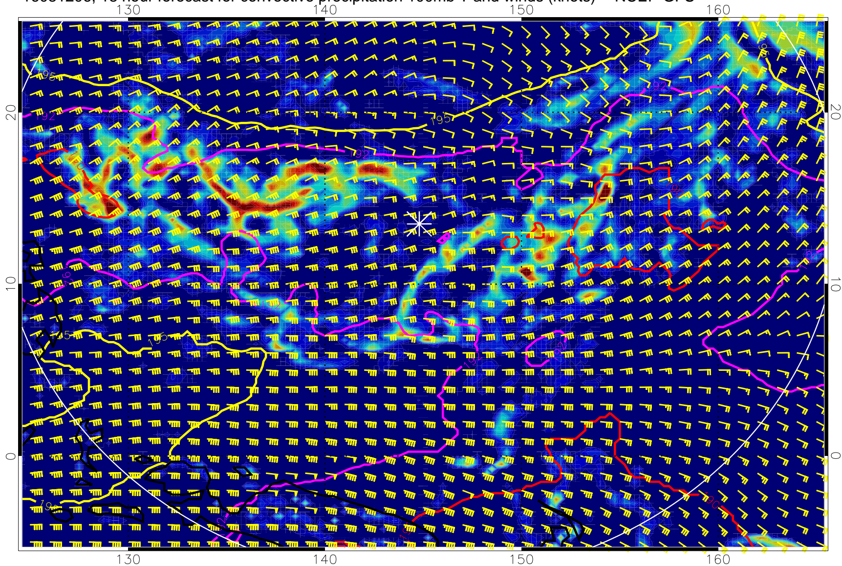
16081206, 18 hour forecast for convective precipitation 100mb T and winds (knots) -- NCEP GFS
