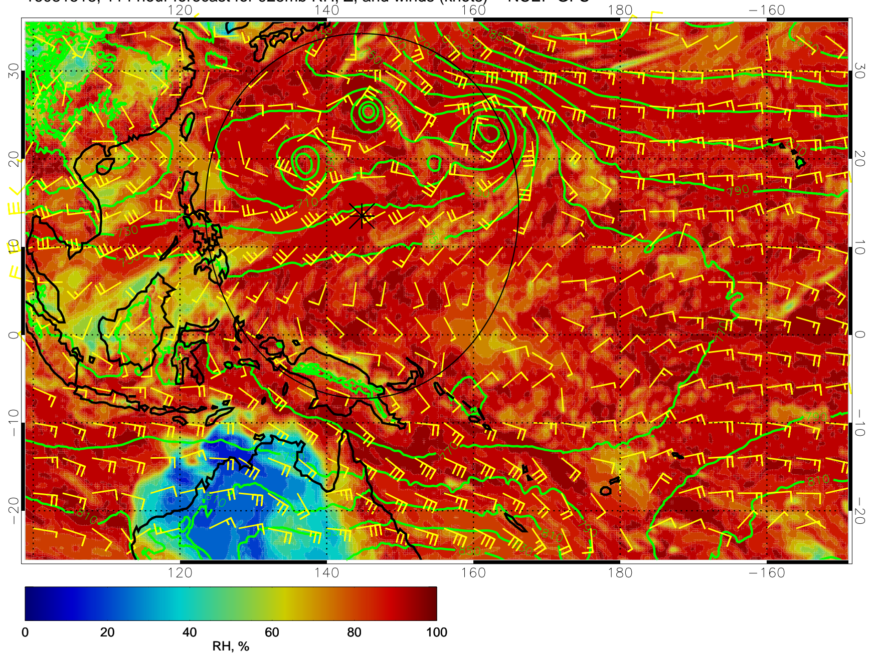
16081518, 114 hour forecast for 925mb RH, Z, and winds (knots) -- NCEP GFS
