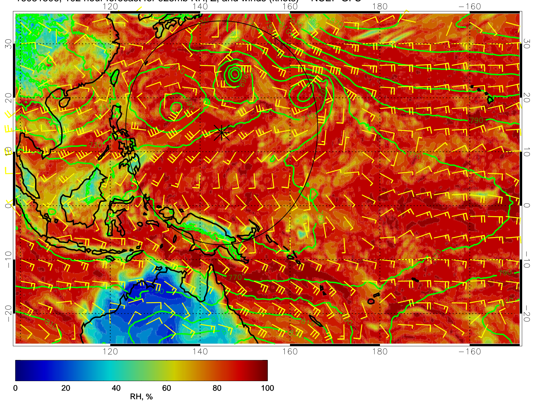
16081506, 102 hour forecast for 925mb RH, Z, and winds (knots) -- NCEP GFS
