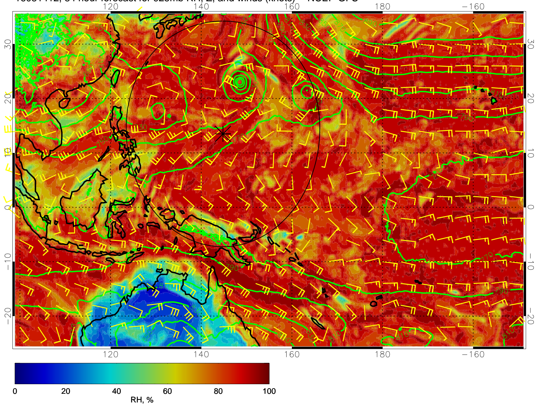
16081412, 84 hour forecast for 925mb RH, Z, and winds (knots) -- NCEP GFS
