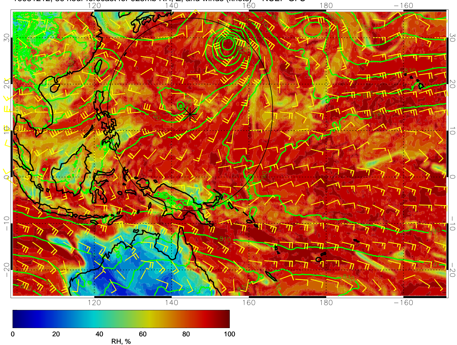
16081212, 36 hour forecast for 925mb RH, Z, and winds (knots) -- NCEP GFS
