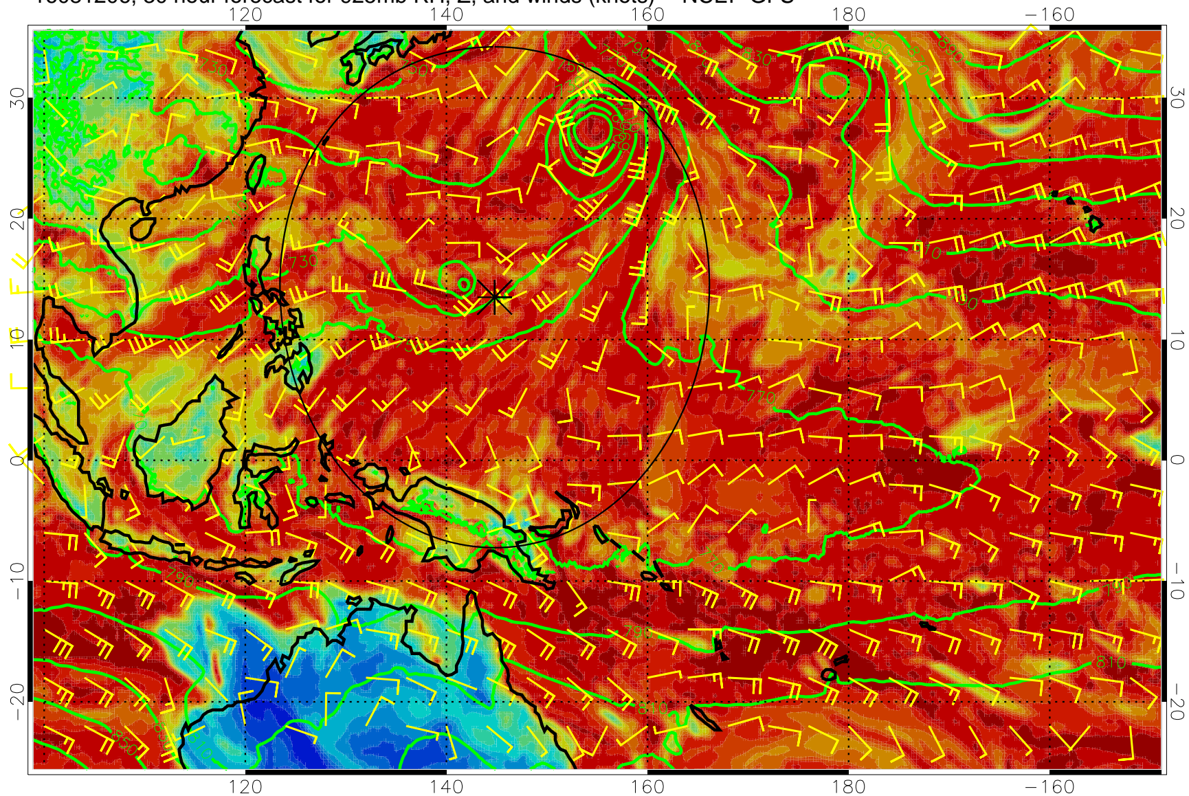
16081206, 30 hour forecast for 925mb RH, Z, and winds (knots) -- NCEP GFS
