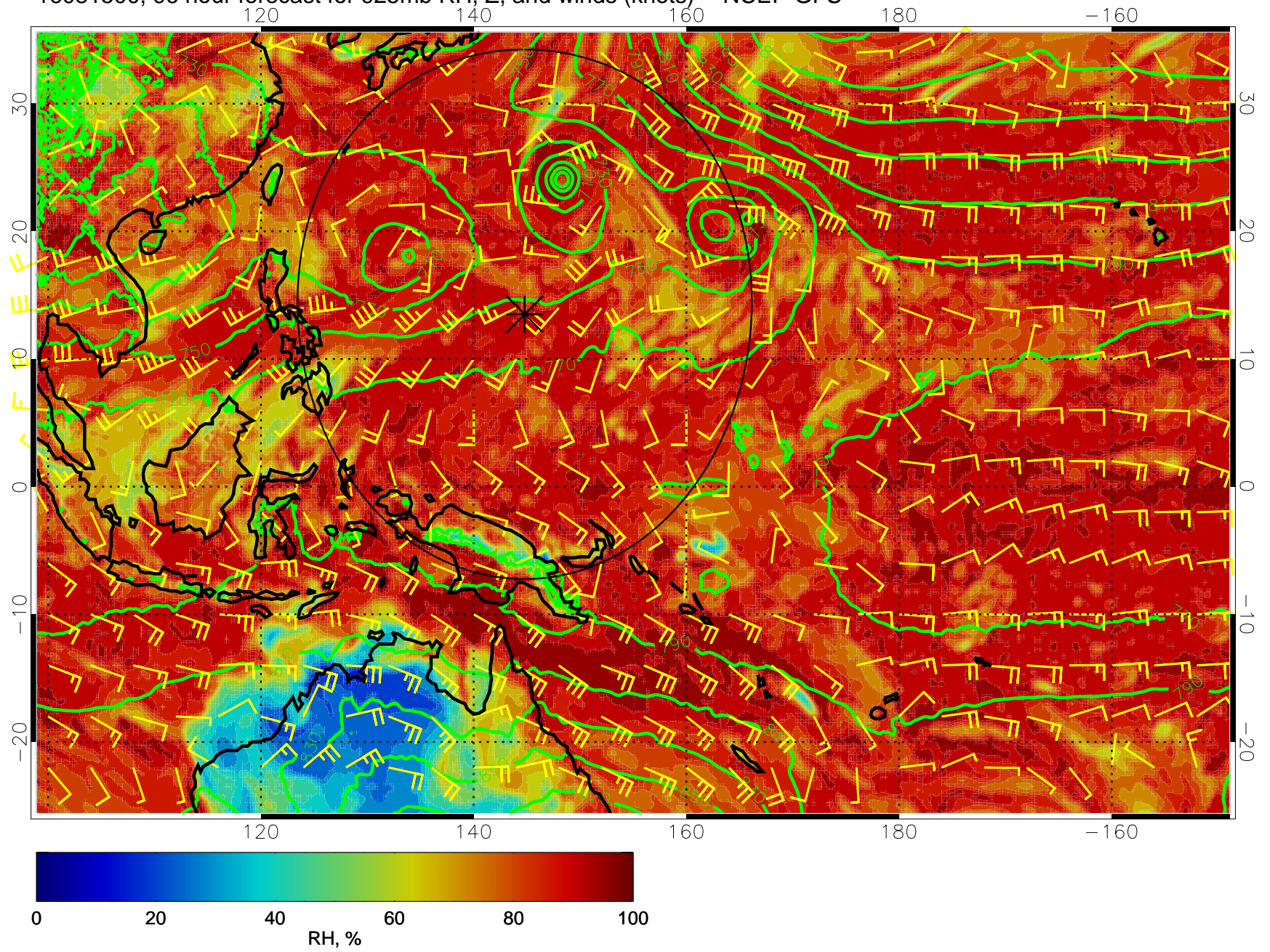
16081500, 96 hour forecast for 925mb RH, Z, and winds (knots) -- NCEP GFS
