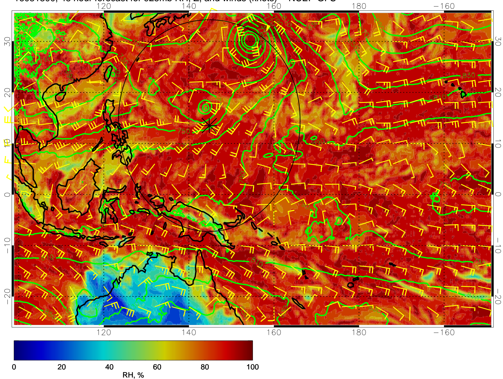
16081300, 48 hour forecast for 925mb RH, Z, and winds (knots) -- NCEP GFS
