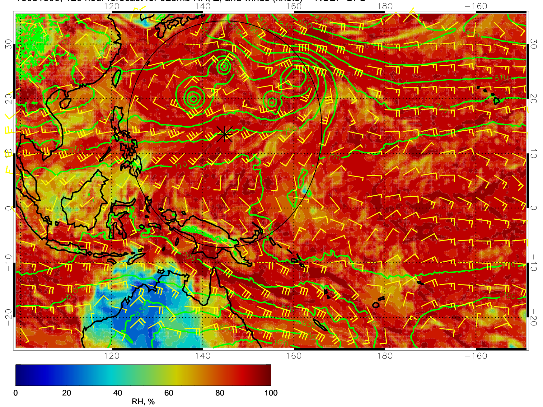
16081600, 120 hour forecast for 925mb RH, Z, and winds (knots) -- NCEP GFS
