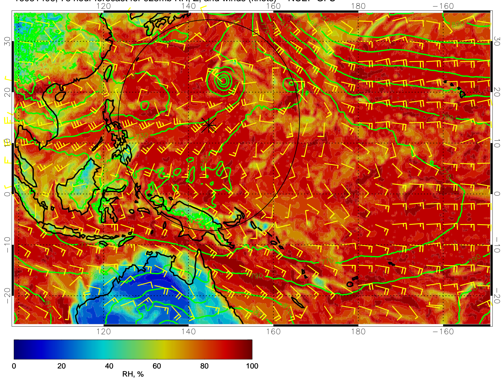
16081406, 78 hour forecast for 925mb RH, Z, and winds (knots) -- NCEP GFS
