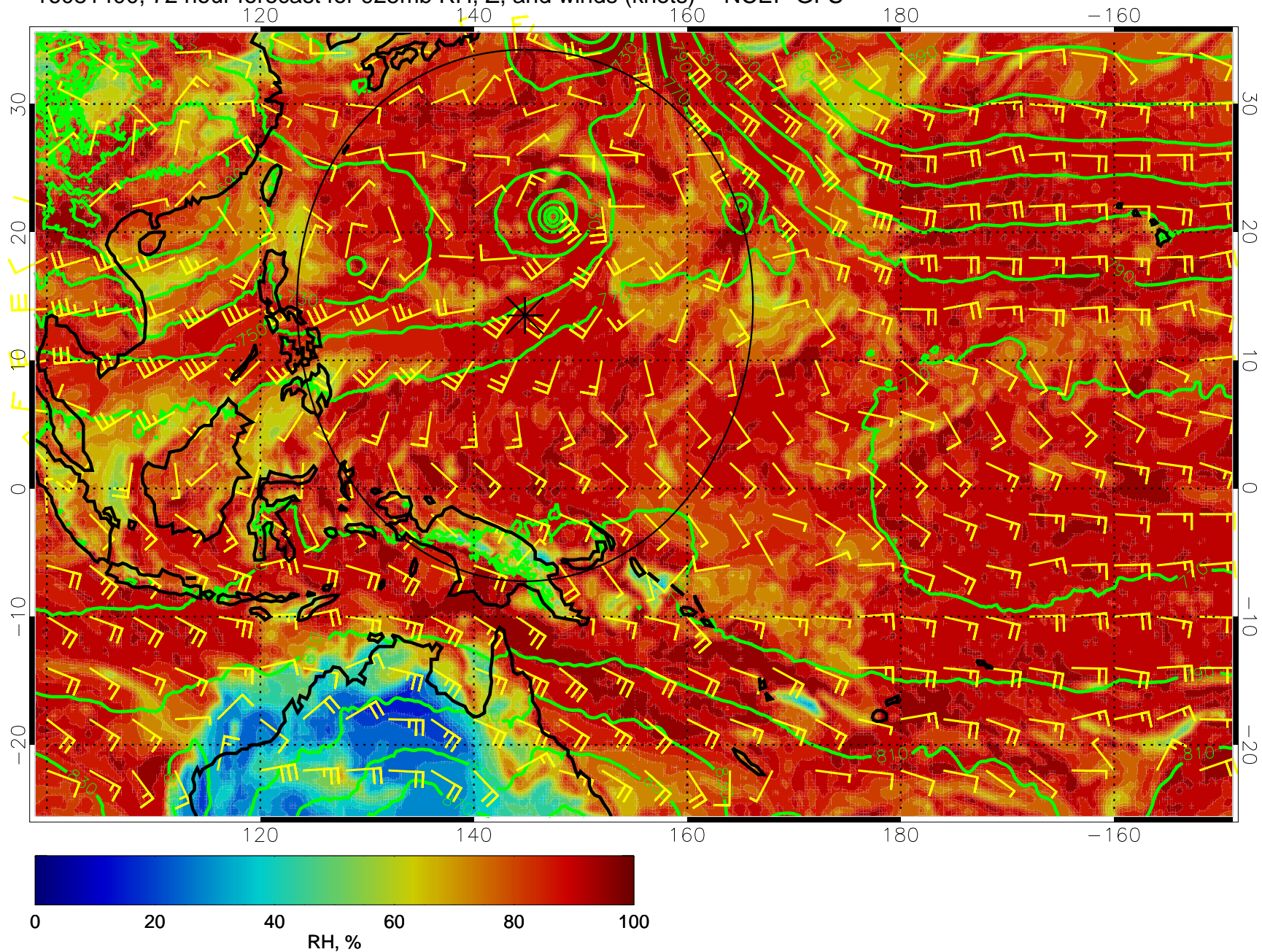
16081400, 72 hour forecast for 925mb RH, Z, and winds (knots) -- NCEP GFS
