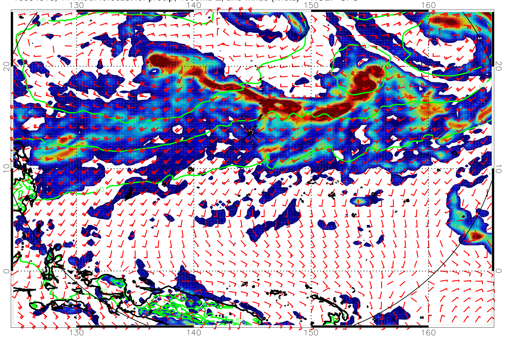
16081518, 114 hour forecast for precip, 1000mb Z, and winds (knots) -- NCEP GFS
