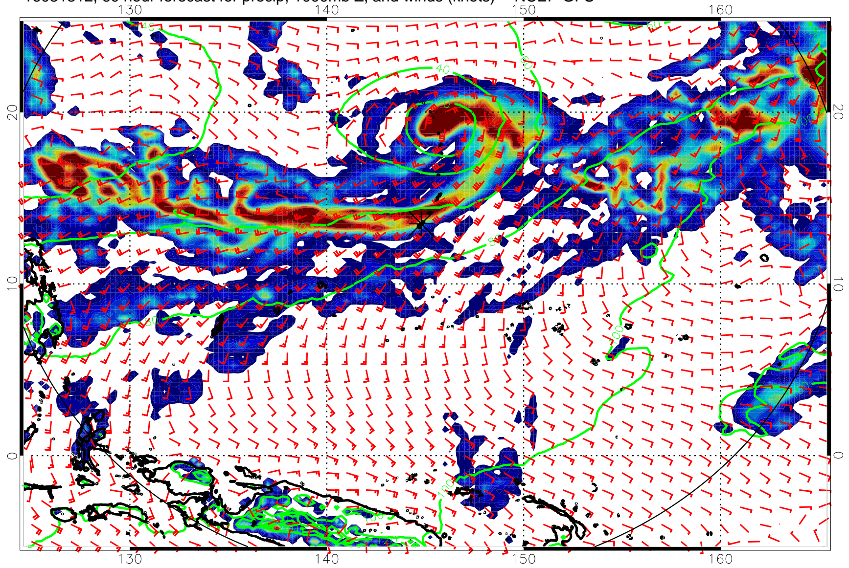
16081312, 60 hour forecast for precip, 1000mb Z, and winds (knots) -- NCEP GFS
