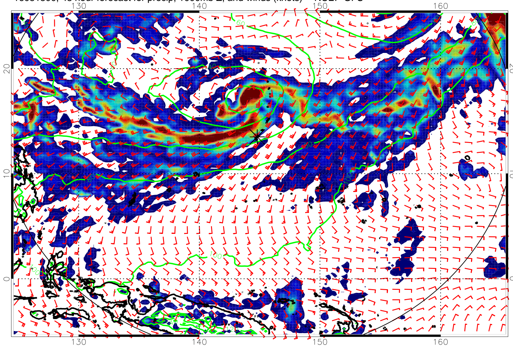
16081300, 48 hour forecast for precip, 1000mb Z, and winds (knots) -- NCEP GFS
