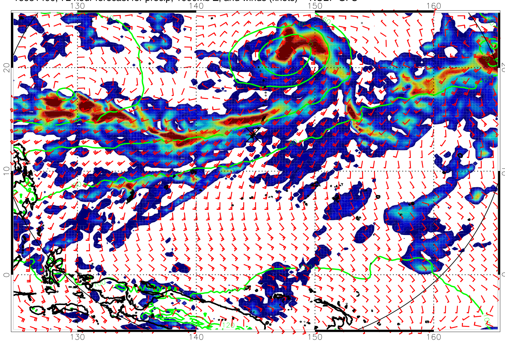
16081400, 72 hour forecast for precip, 1000mb Z, and winds (knots) -- NCEP GFS
