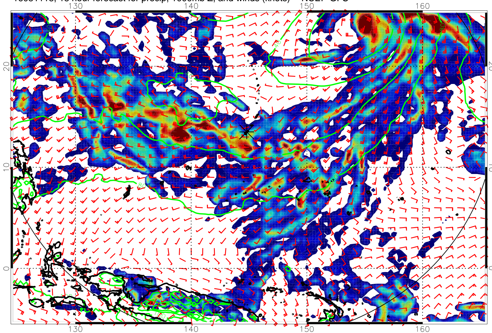
16081118, 18 hour forecast for precip, 1000mb Z, and winds (knots) -- NCEP GFS
