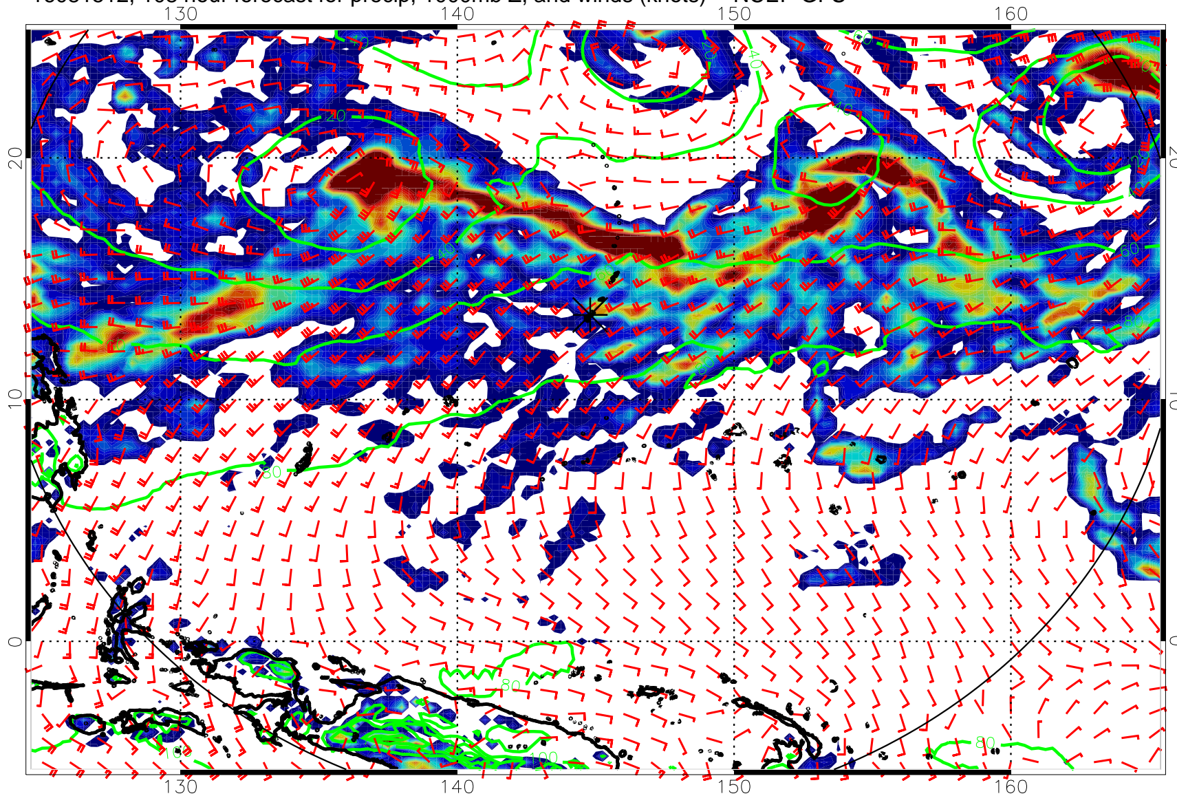
16081512, 108 hour forecast for precip, 1000mb Z, and winds (knots) -- NCEP GFS
