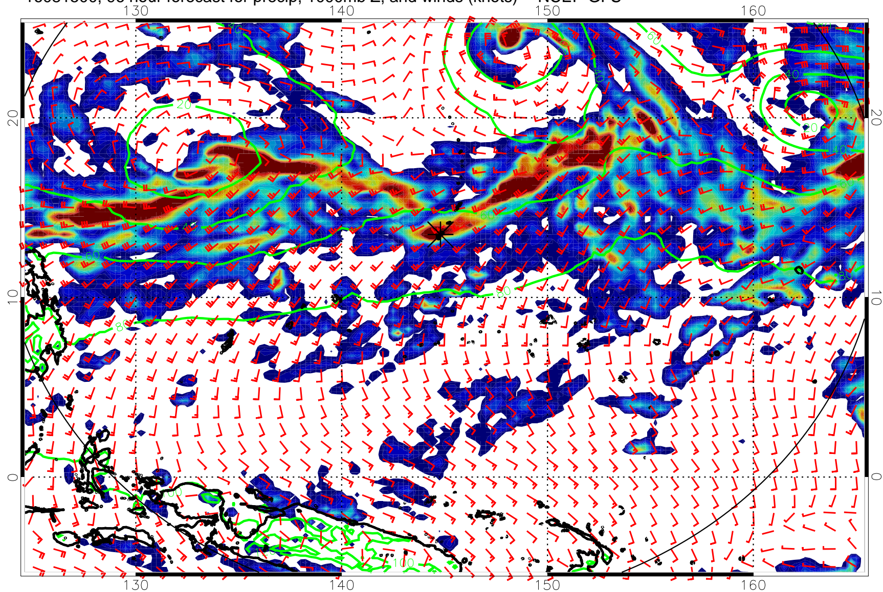
16081500, 96 hour forecast for precip, 1000mb Z, and winds (knots) -- NCEP GFS
