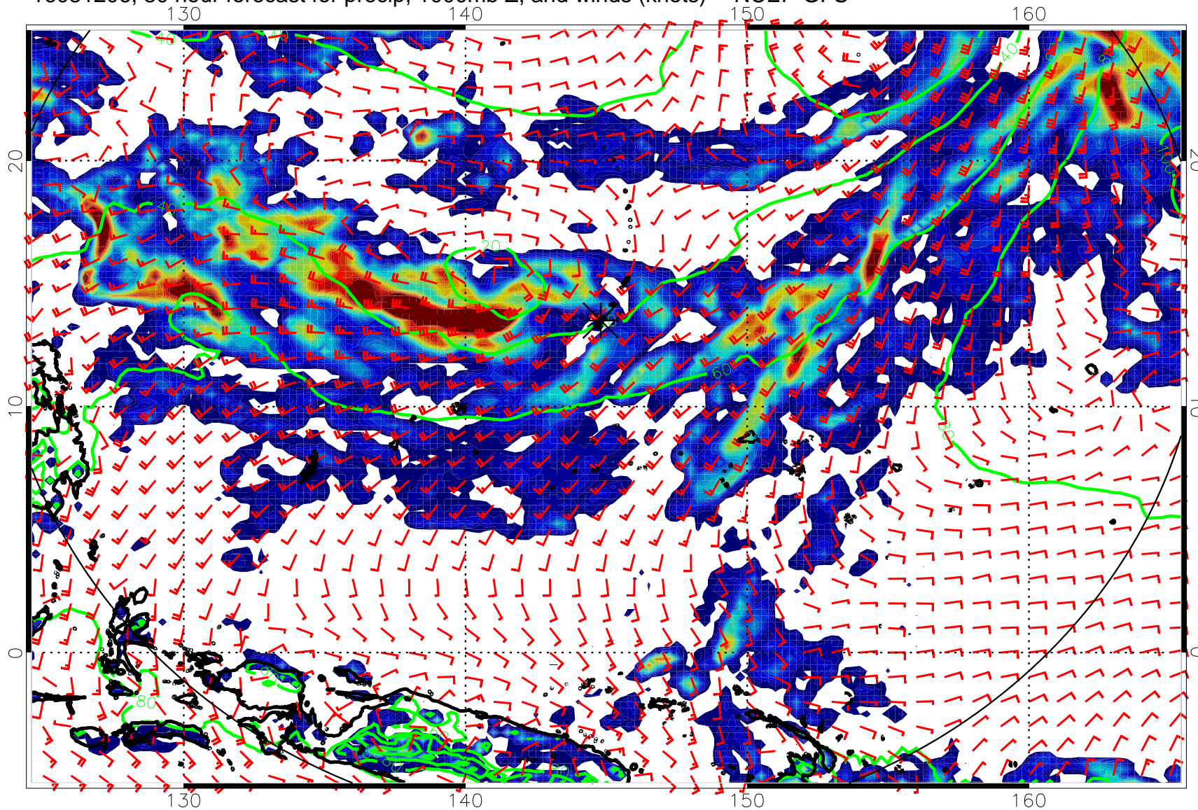
16081206, 30 hour forecast for precip, 1000mb Z, and winds (knots) -- NCEP GFS
