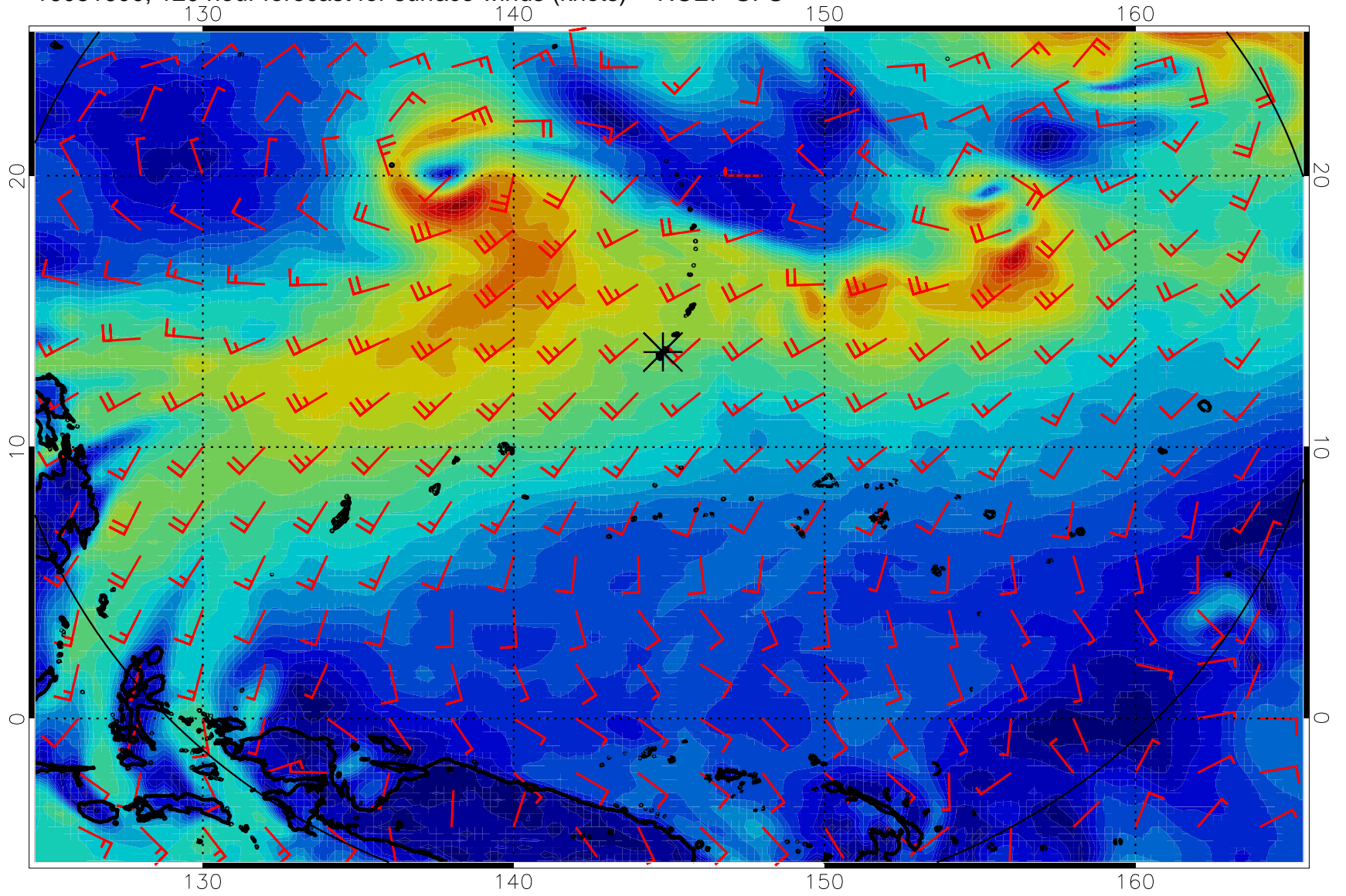
16081600, 120 hour forecast for surface winds (knots) -- NCEP GFS
