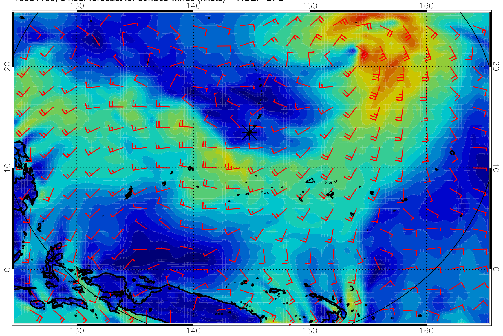
16081106, 6 hour forecast for surface winds (knots) -- NCEP GFS
