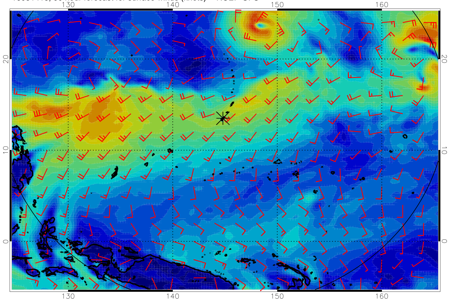
16081418, 90 hour forecast for surface winds (knots) -- NCEP GFS
