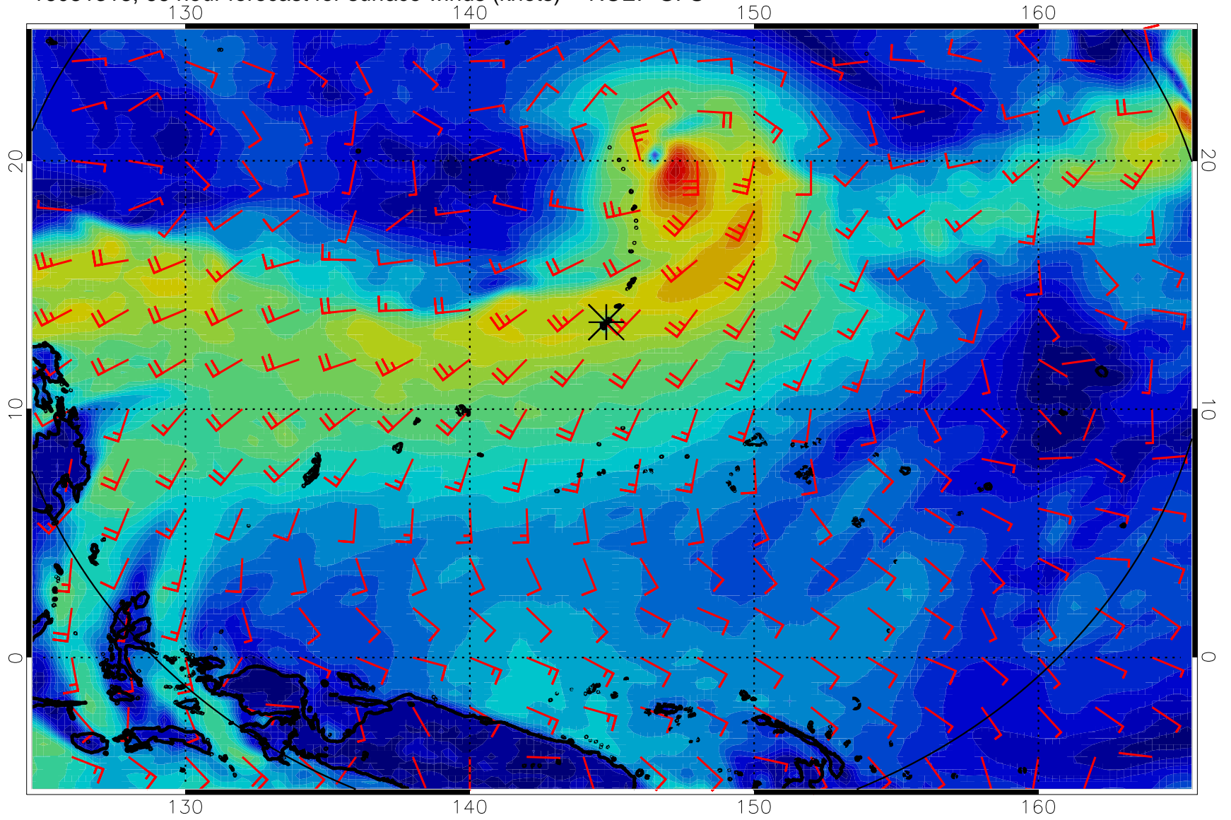
16081318, 66 hour forecast for surface winds (knots) -- NCEP GFS
