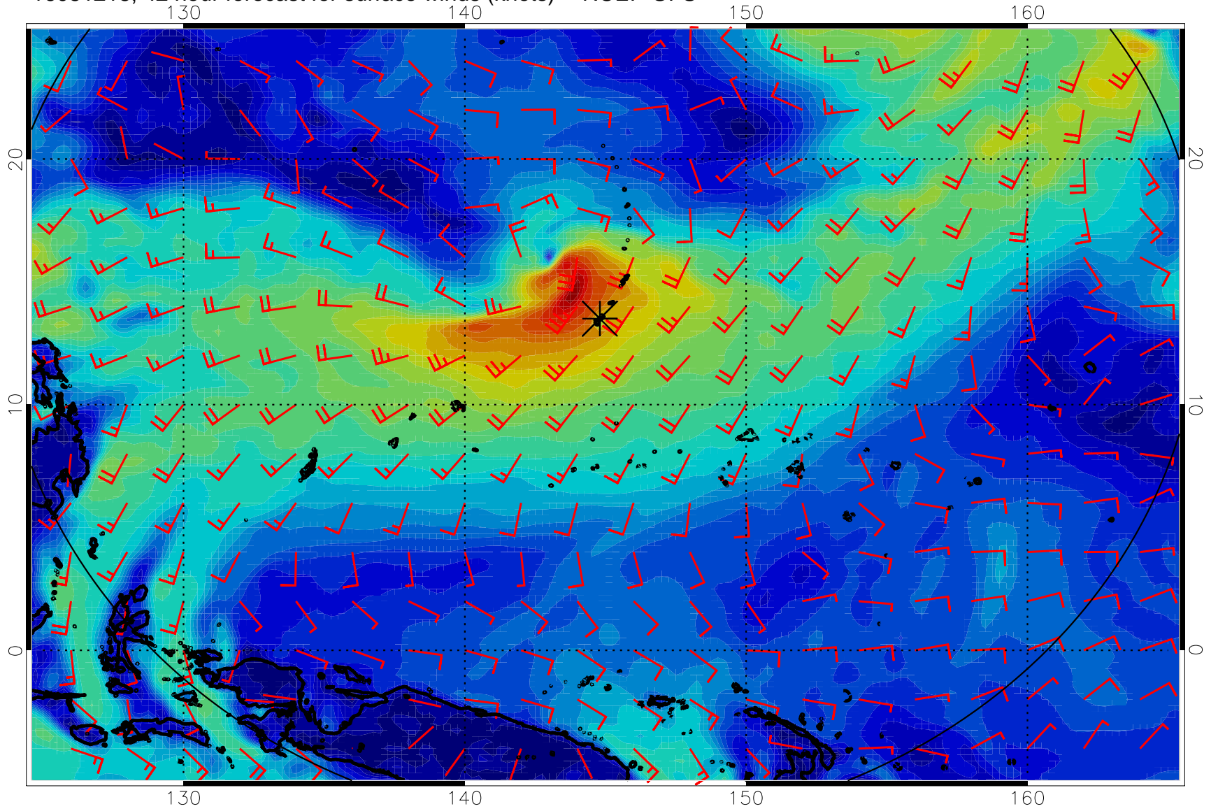
16081218, 42 hour forecast for surface winds (knots) -- NCEP GFS
