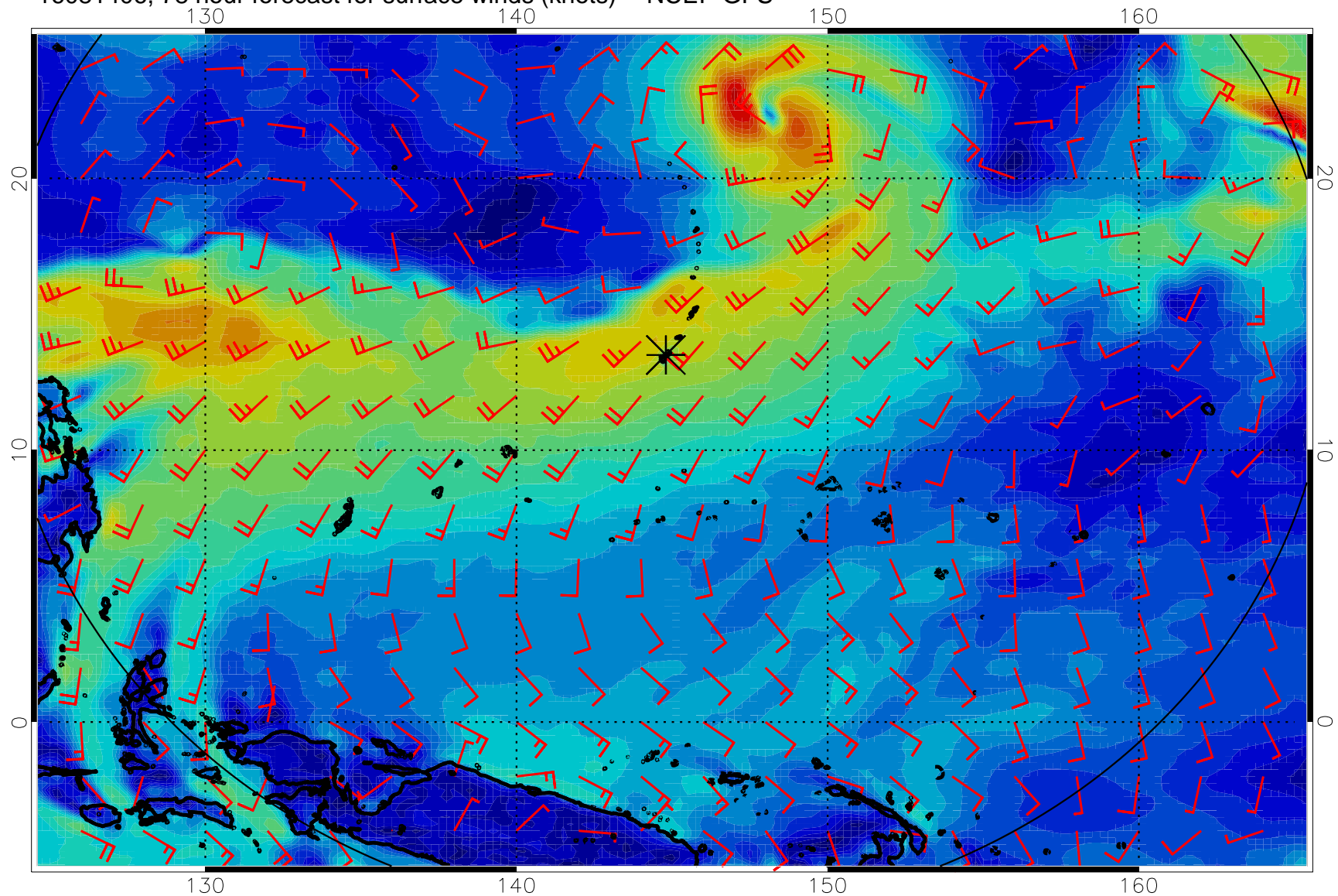
16081406, 78 hour forecast for surface winds (knots) -- NCEP GFS
