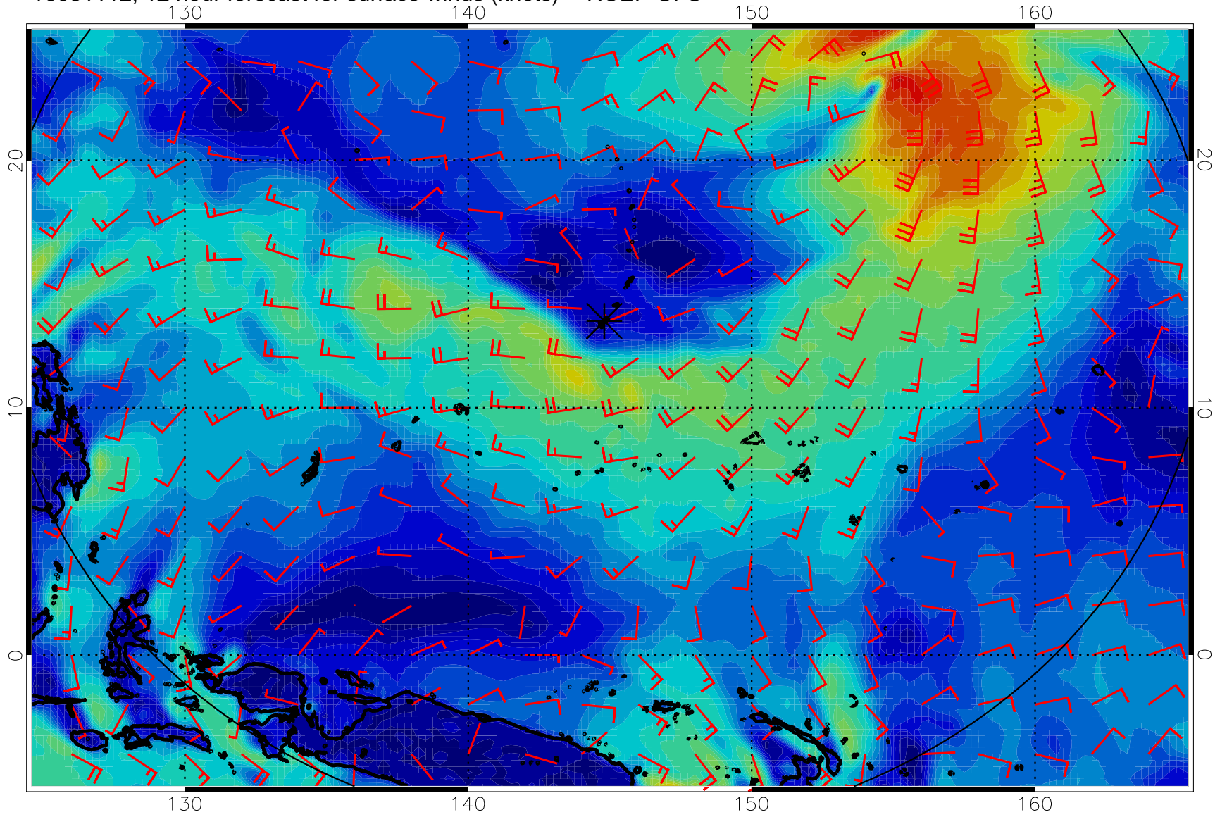
16081112, 12 hour forecast for surface winds (knots) -- NCEP GFS
