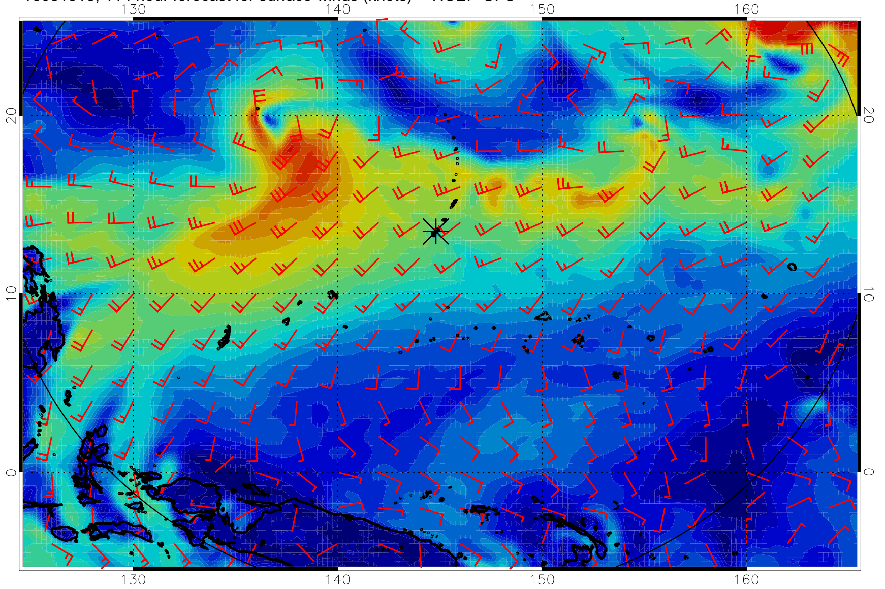
16081518, 114 hour forecast for surface winds (knots) -- NCEP GFS
