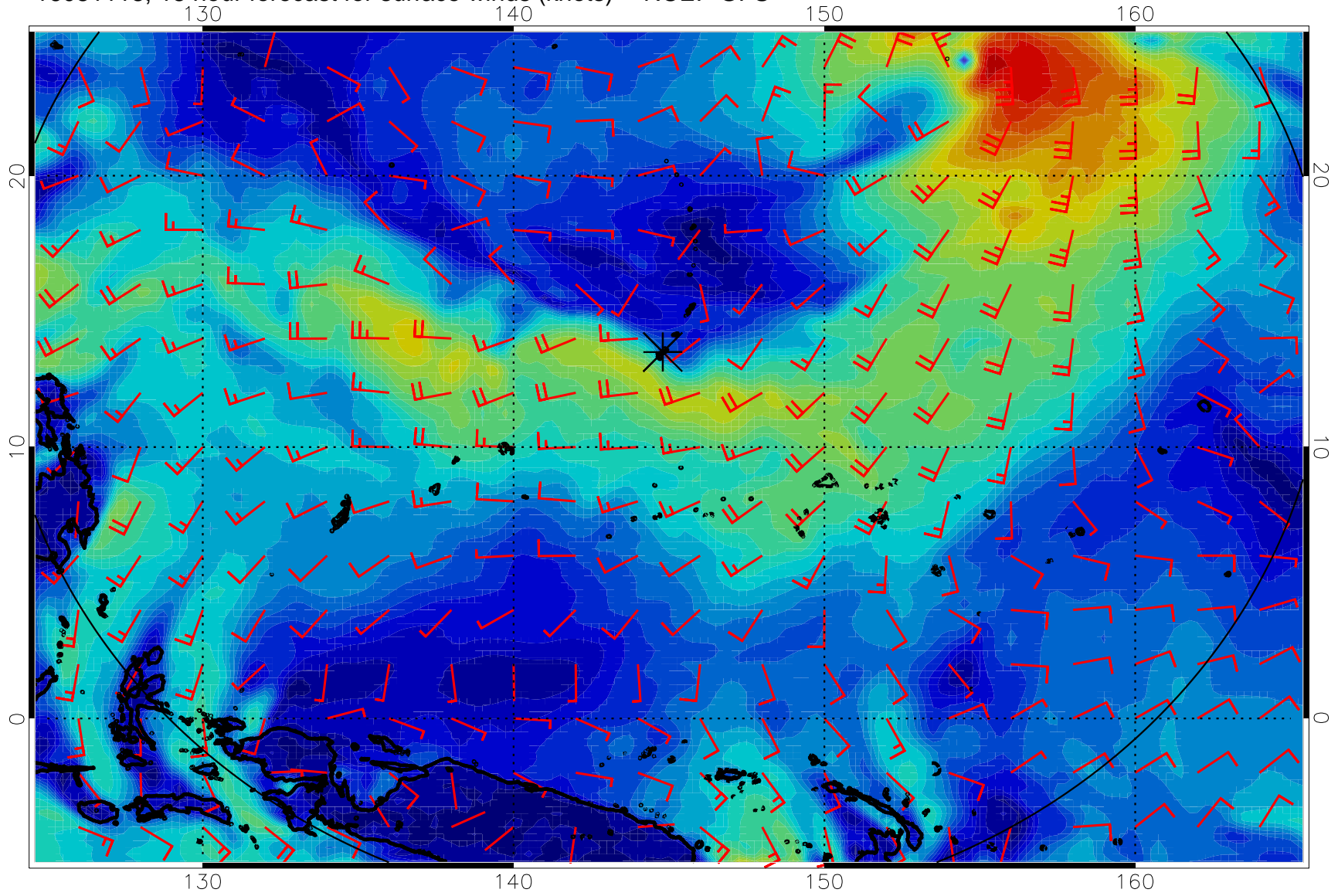
16081118, 18 hour forecast for surface winds (knots) -- NCEP GFS
