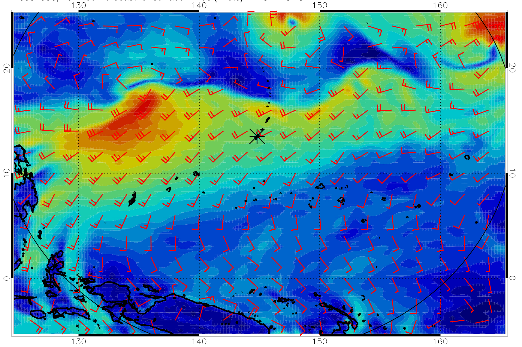
16081506, 102 hour forecast for surface winds (knots) -- NCEP GFS
