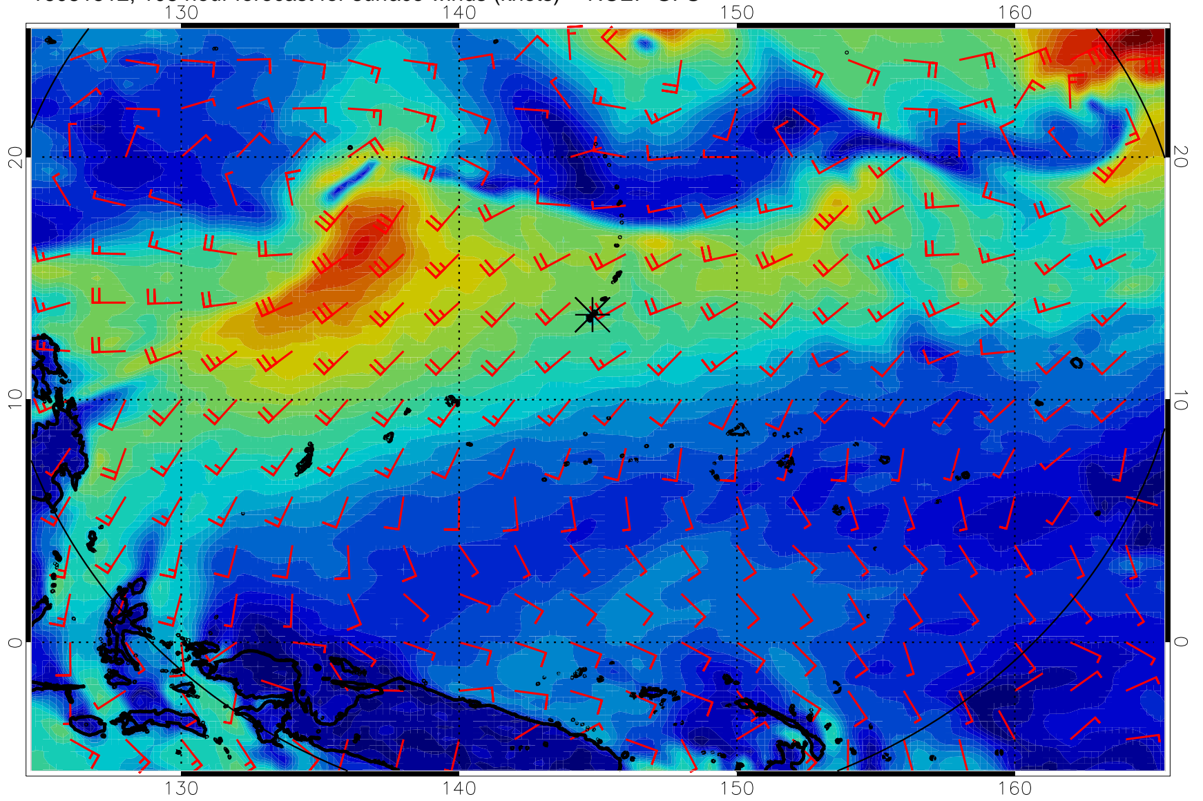
16081512, 108 hour forecast for surface winds (knots) -- NCEP GFS
