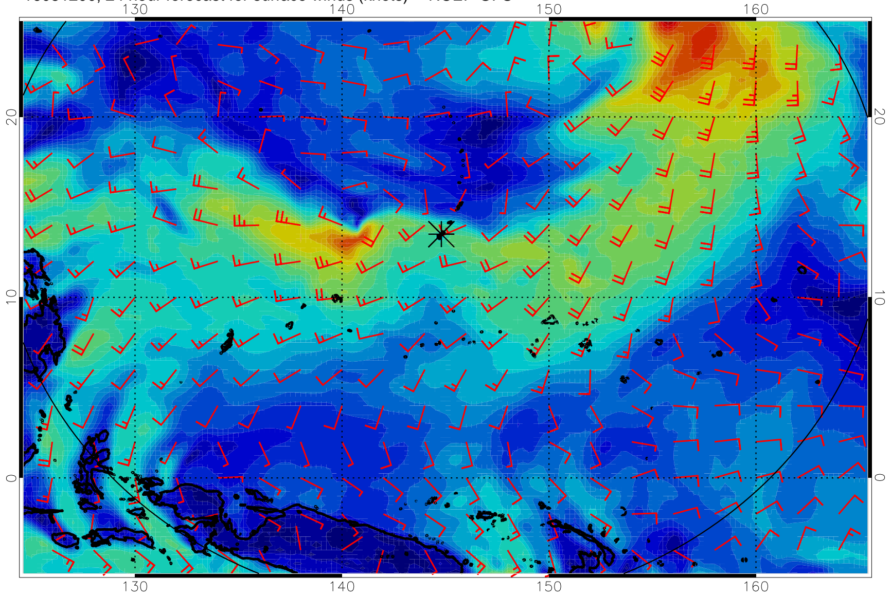
16081200, 24 hour forecast for surface winds (knots) -- NCEP GFS
