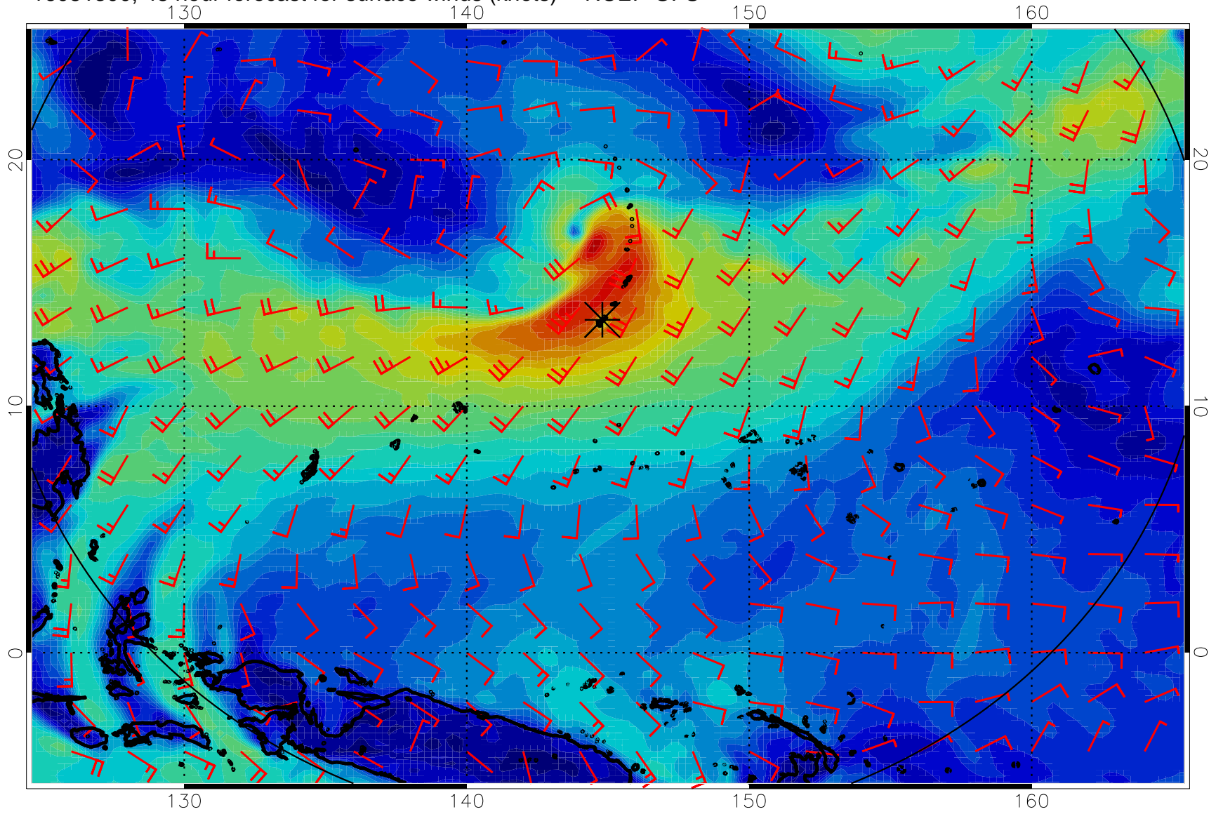
16081300, 48 hour forecast for surface winds (knots) -- NCEP GFS
