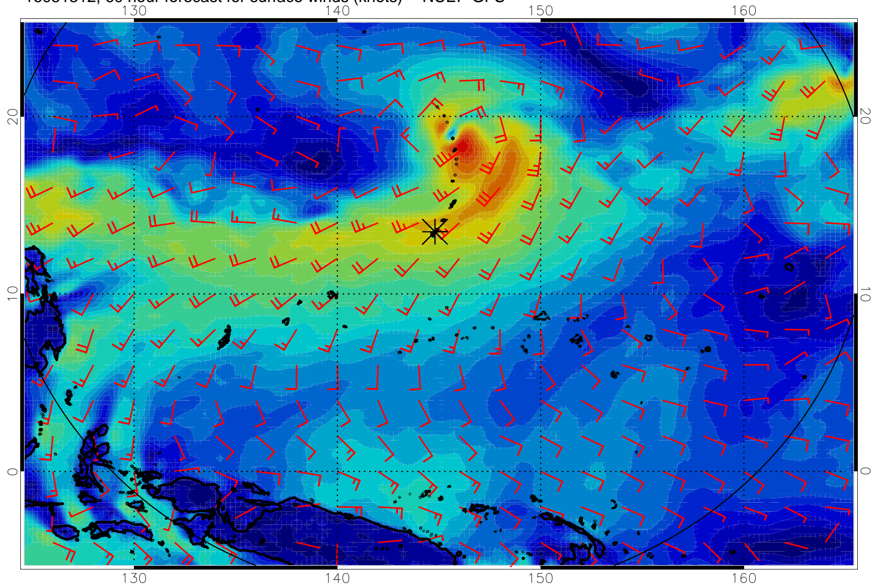
16081312, 60 hour forecast for surface winds (knots) -- NCEP GFS
