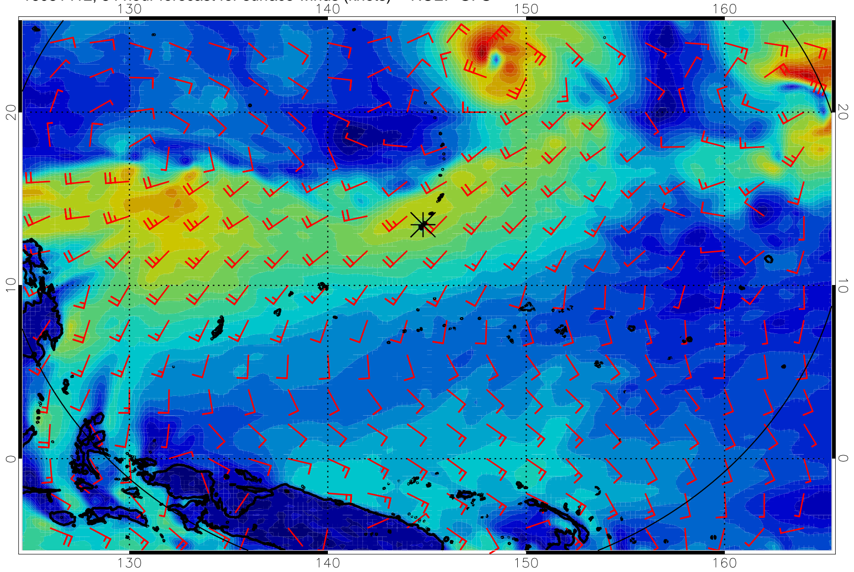
16081412, 84 hour forecast for surface winds (knots) -- NCEP GFS
