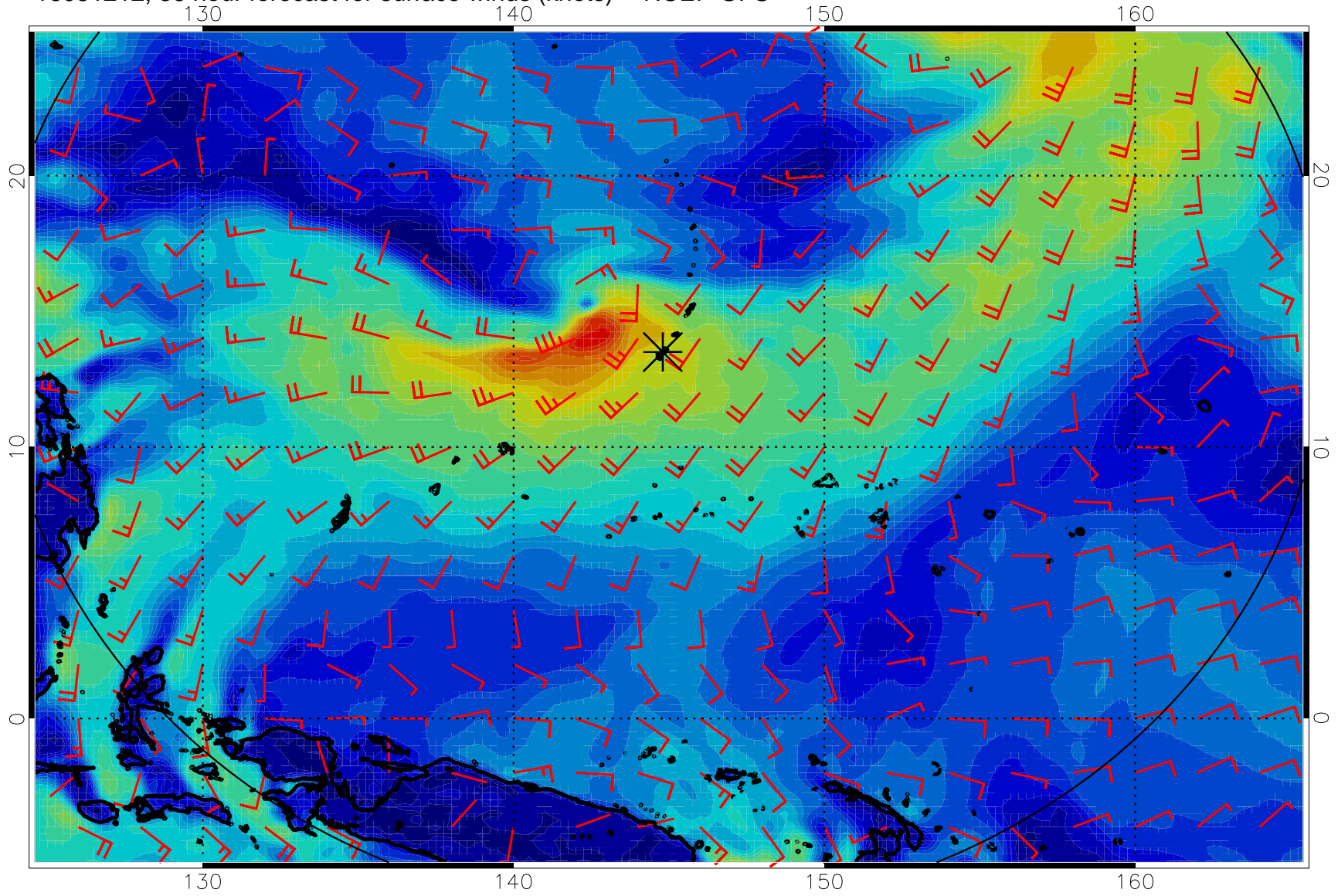
16081212, 36 hour forecast for surface winds (knots) -- NCEP GFS
