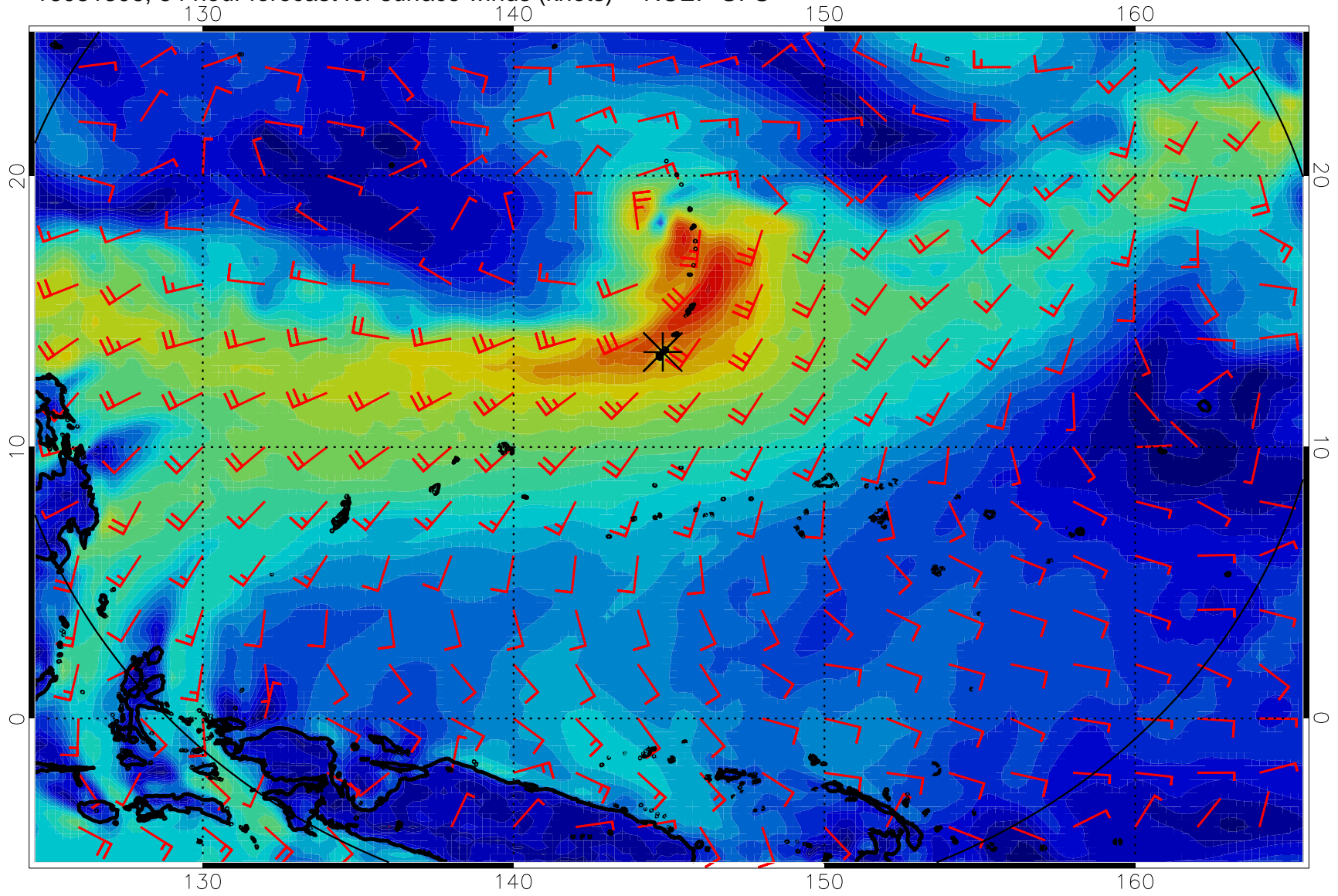
16081306, 54 hour forecast for surface winds (knots) -- NCEP GFS
