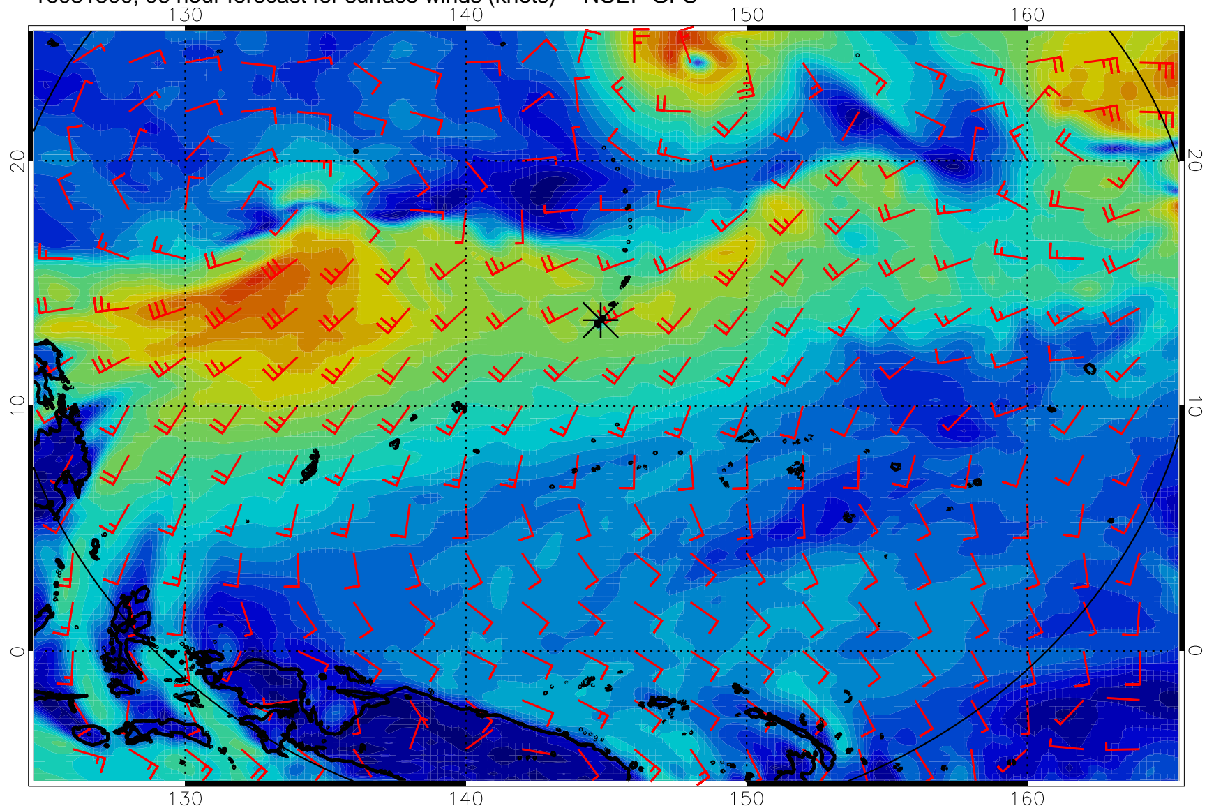
16081500, 96 hour forecast for surface winds (knots) -- NCEP GFS
