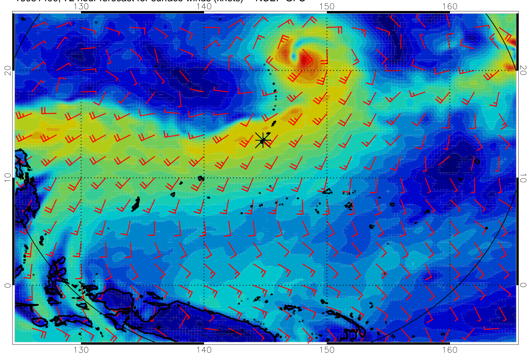
16081400, 72 hour forecast for surface winds (knots) -- NCEP GFS
