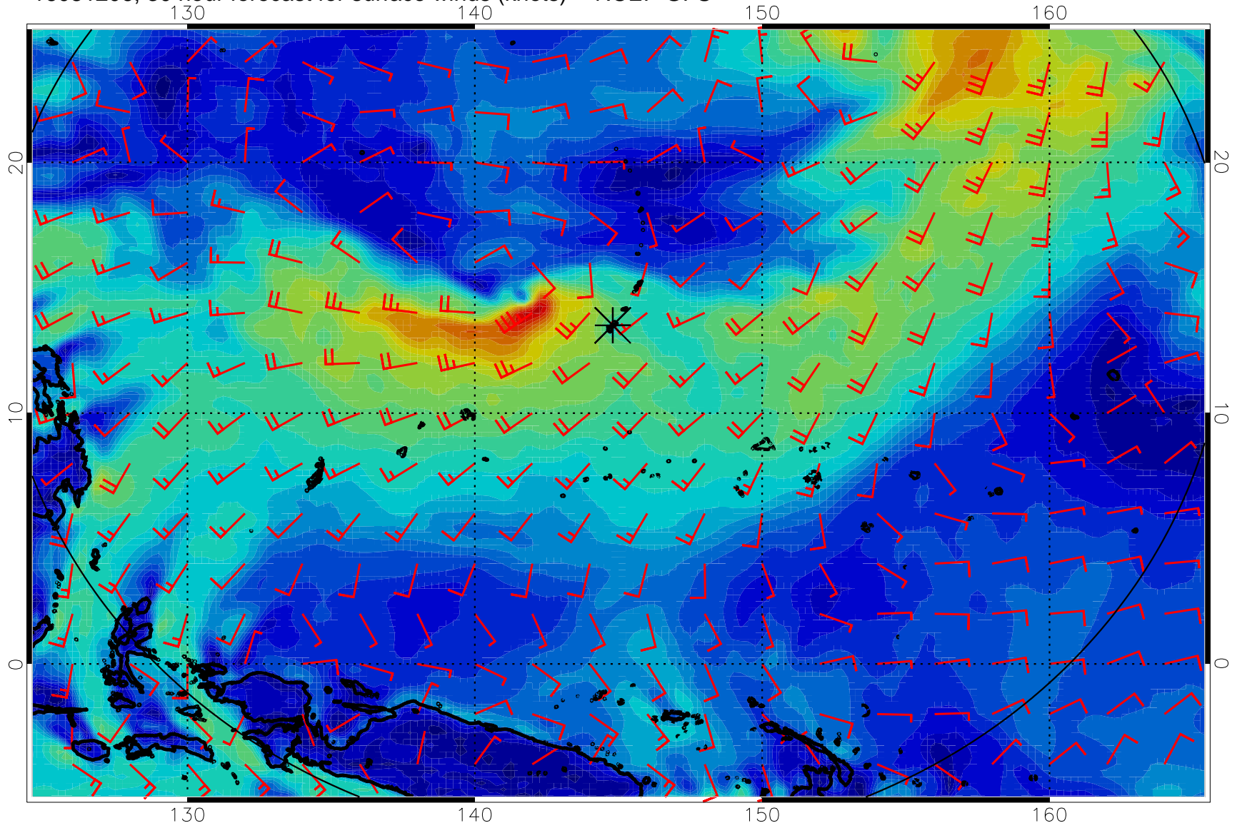
16081206, 30 hour forecast for surface winds (knots) -- NCEP GFS
